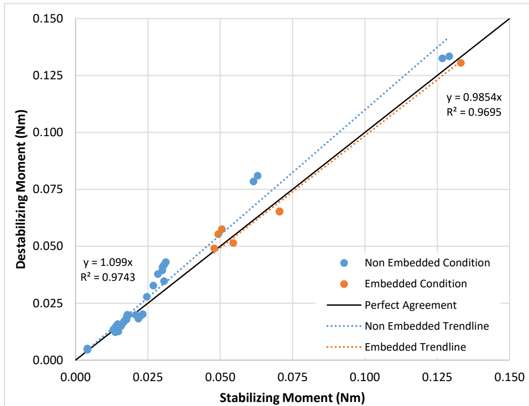
Figure 5-15: Relationship between stabilizing and destabilizing moments based on Equation (4-1) for boulder incipient motion experiments.
