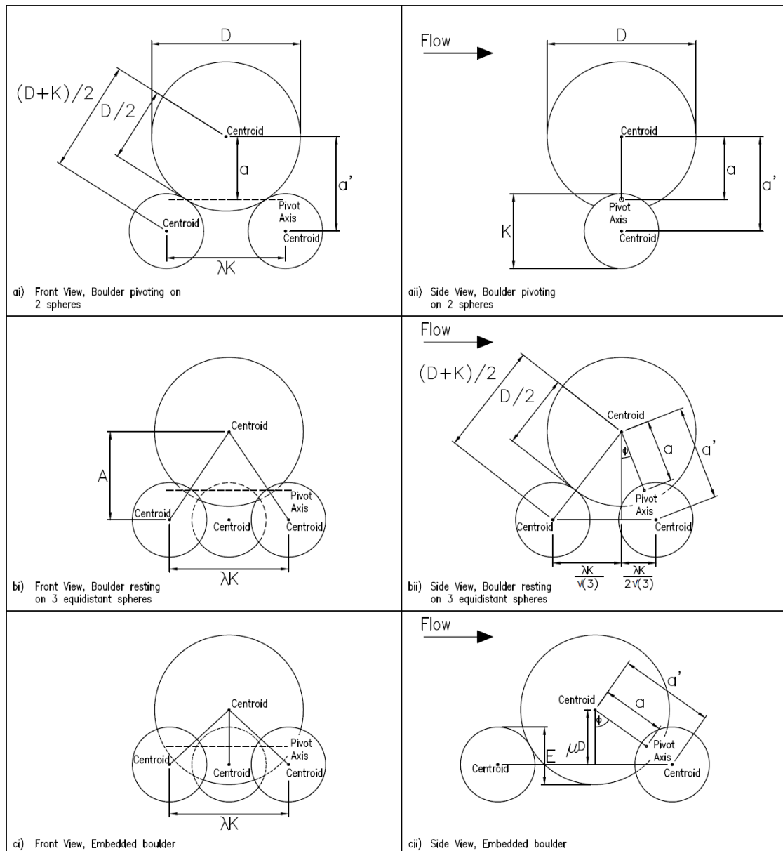
Figure 4-2: Pivoting geometry on bed material slope \alpha=0^\circ .
