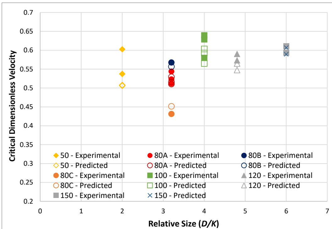
Figure 5-5: Relationship between relative size and critical dimensionless velocity.
