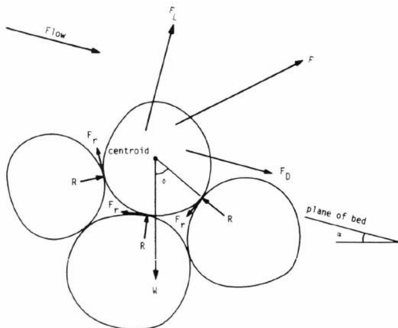
Figure 4-1: Forces acting on a particle (James 1990).
