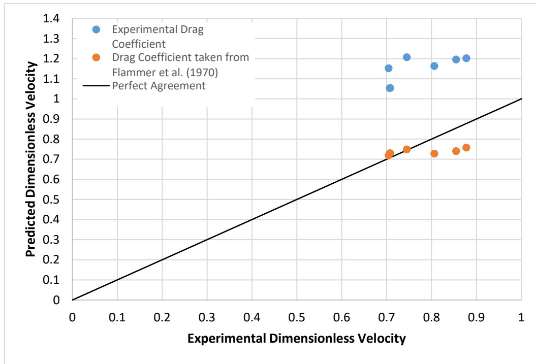
Figure 5-3: Comparison of predicted dimensionless velocity using experimental drag coefficients and drag coefficients taken from Flammer et al. (1970).
