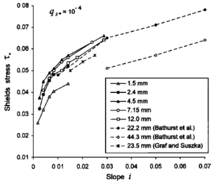
Figure 2-6: Shields stress as a function of slope corresponding to a q_{s^*} = 10^{-4} (Shvidchenko and Pender 2000).
