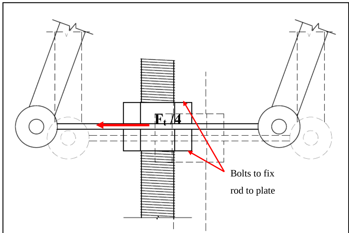
Figure 3-10: Schematic of rod fixed to load cell where F_t/4 is the force acting through the plate. Dashed lines indicate plate in rest position and solid lines represent plate after a force is applied.
