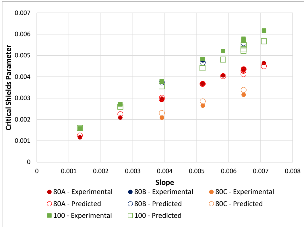
Figure 5-8: Relationship between slope and critical Shields parameter.
