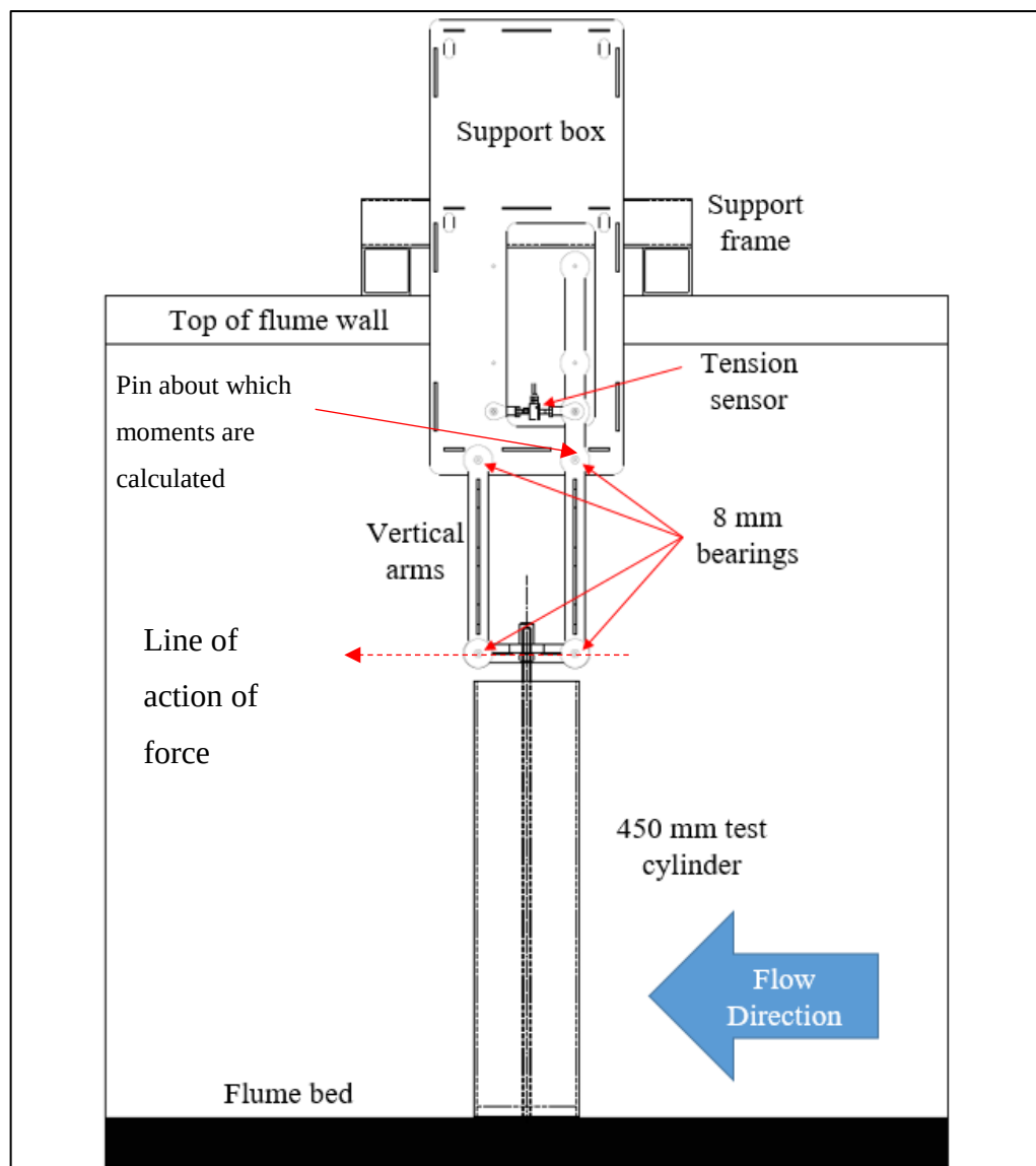
Figure 3-9: Schematic of set up taken from Jackson (2016).
