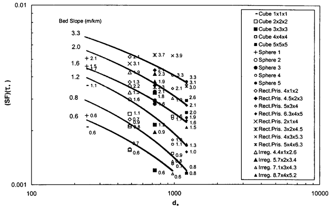
Figure 2-4: Shape Factor Correction for \tau^* versus d_* for different slopes (Gögüs and Defne 2005).
