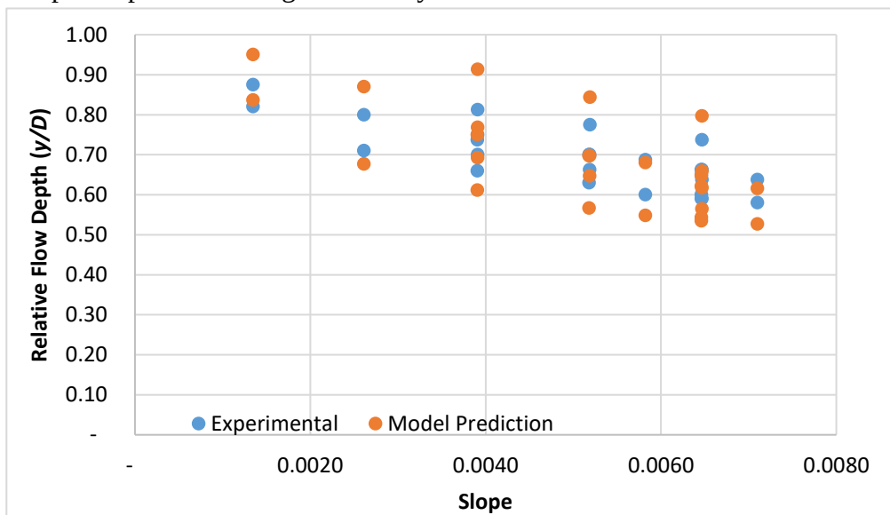
Figure 5-9: Relationship between slope and relative flow depth at incipient movement.
