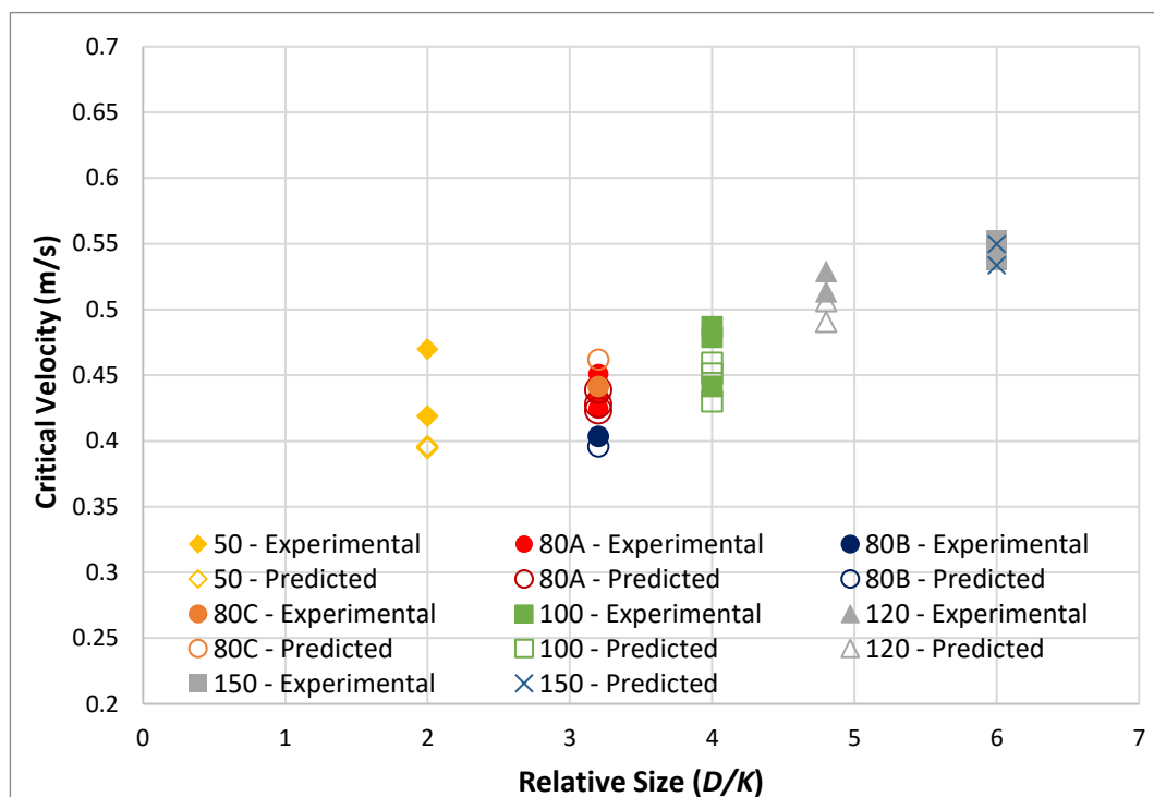
Figure 5-4: Relationship between relative size and critical average velocity.
