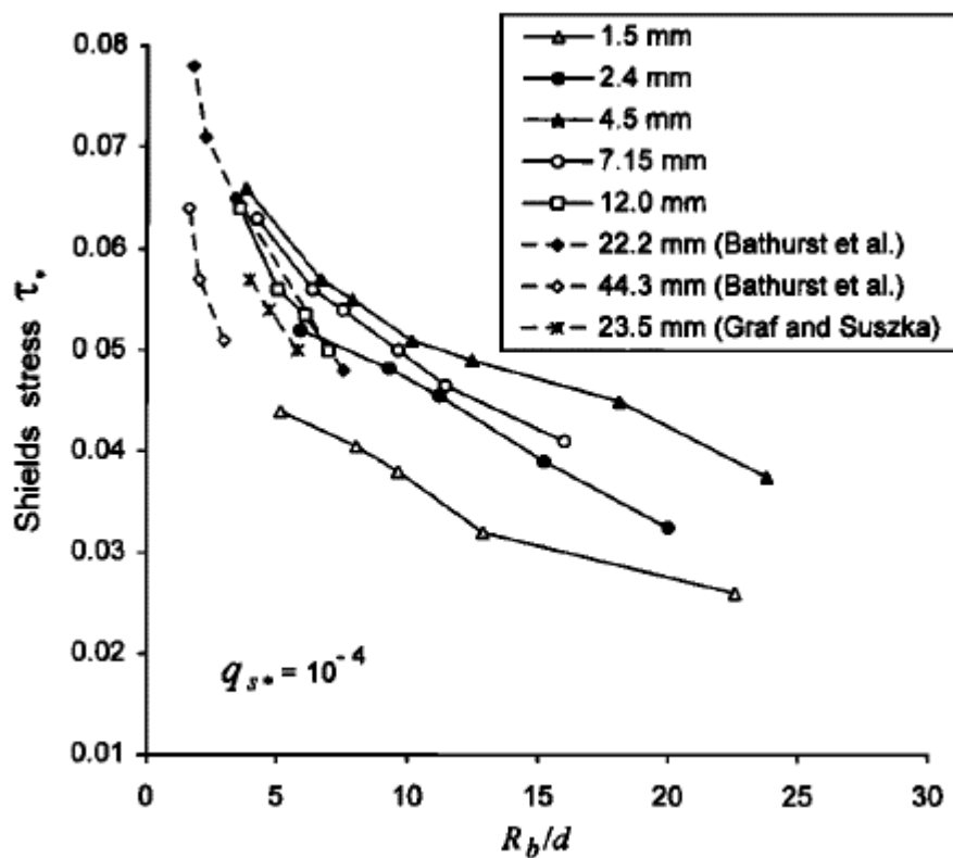
Figure 2-5: Shields stress as a function of R_b/d for different grain sizes (where R_b is the Hydraulic radius) (Shvidchenko and Pender 2000).
