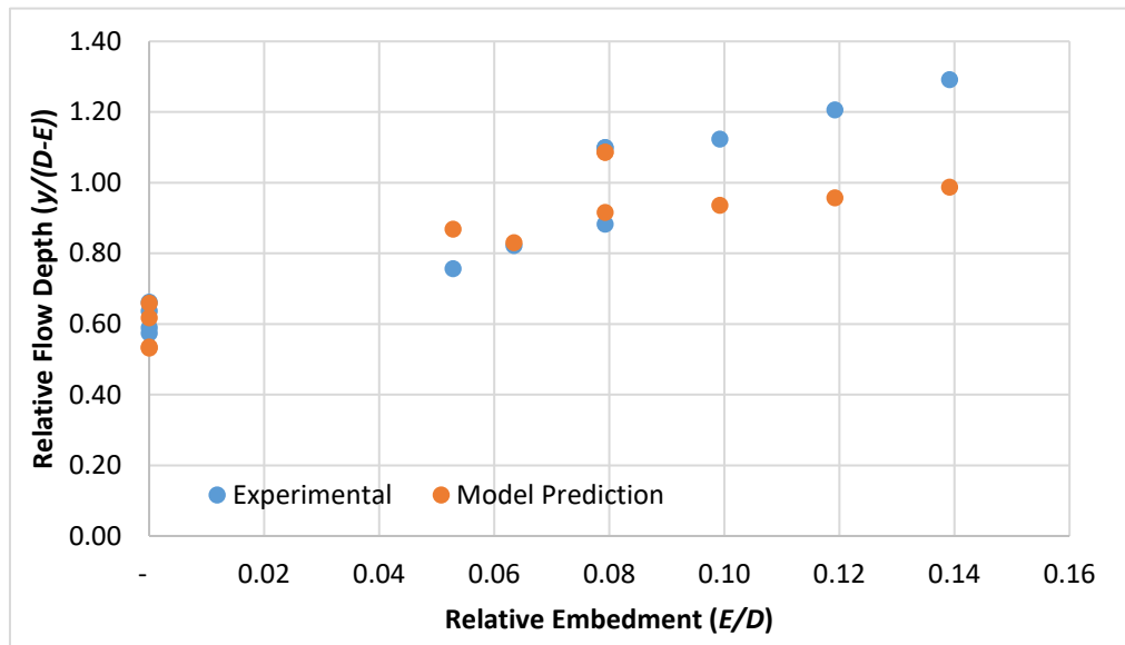
Figure 5-14: Relationship between relative embedment and relative flow depth at incipient movement.
