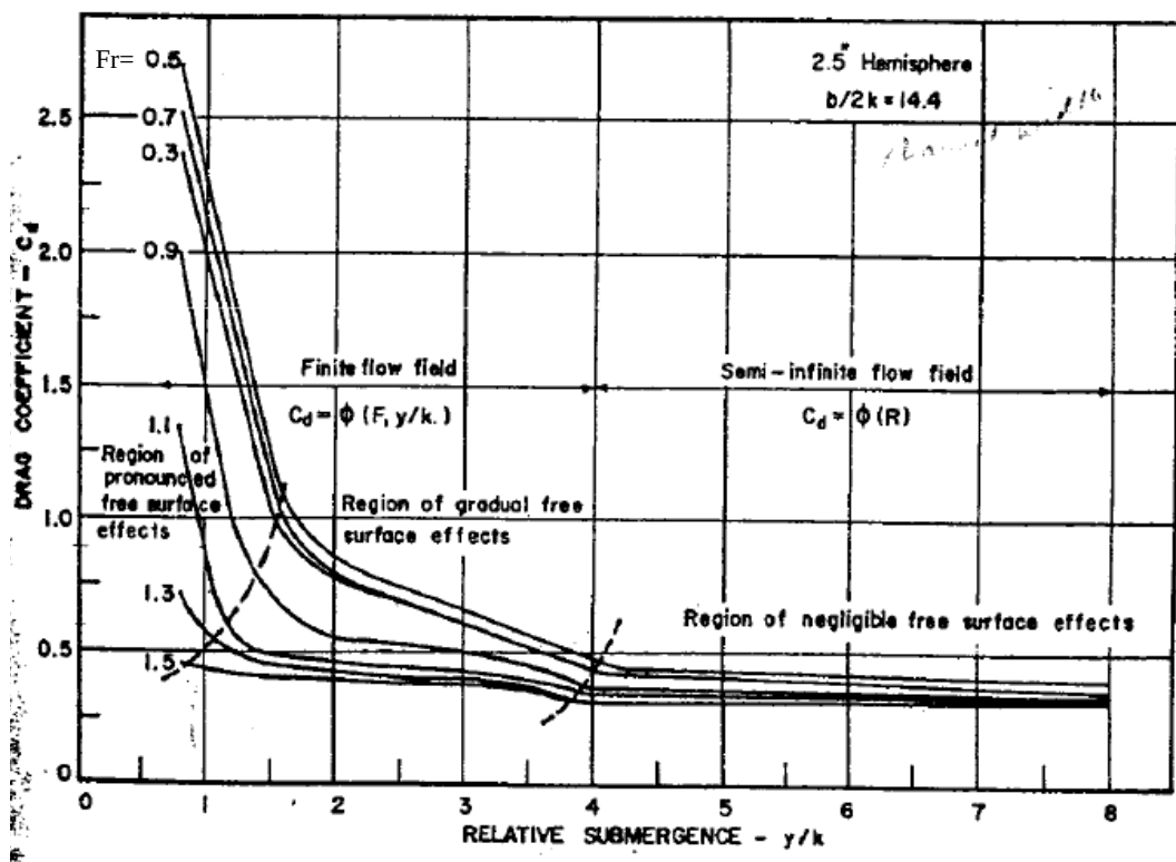
Figure 2-9: Relationship for relative submergence and drag coefficient for hemispheres. (Flammer et al, 1970).
