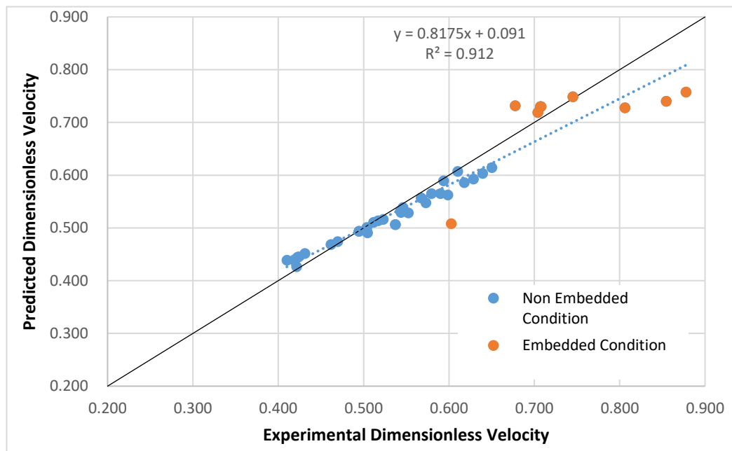
Figure 5-16: Comparison of experimental and predicted dimensionless velocities based on Equation 4-32.
