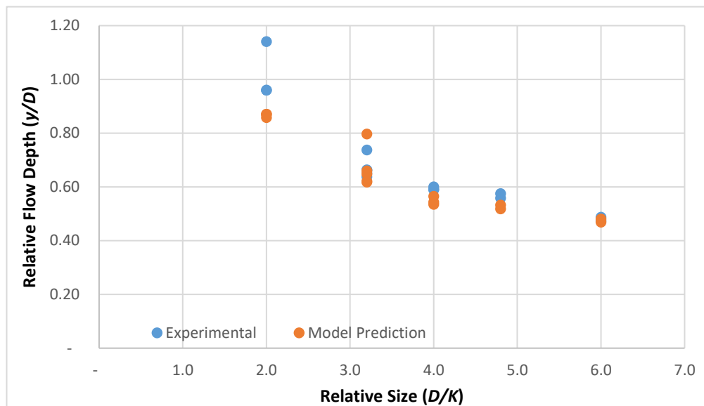
Figure 5-6: Relationship between relative boulder size and relative flow depth at incipient movement.
