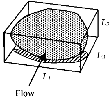
Figure 2-3: Parameters related to condition of incipient motion (symbols changed from Gögüs and Defne 2005).
