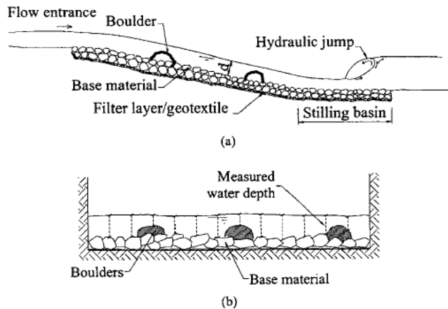
Figure 2-1: (a) Typical cross section of rock chute with protruding boulders and (b) criteria used for water depth measurements (Pagliara and Chiavaccini 2006).
