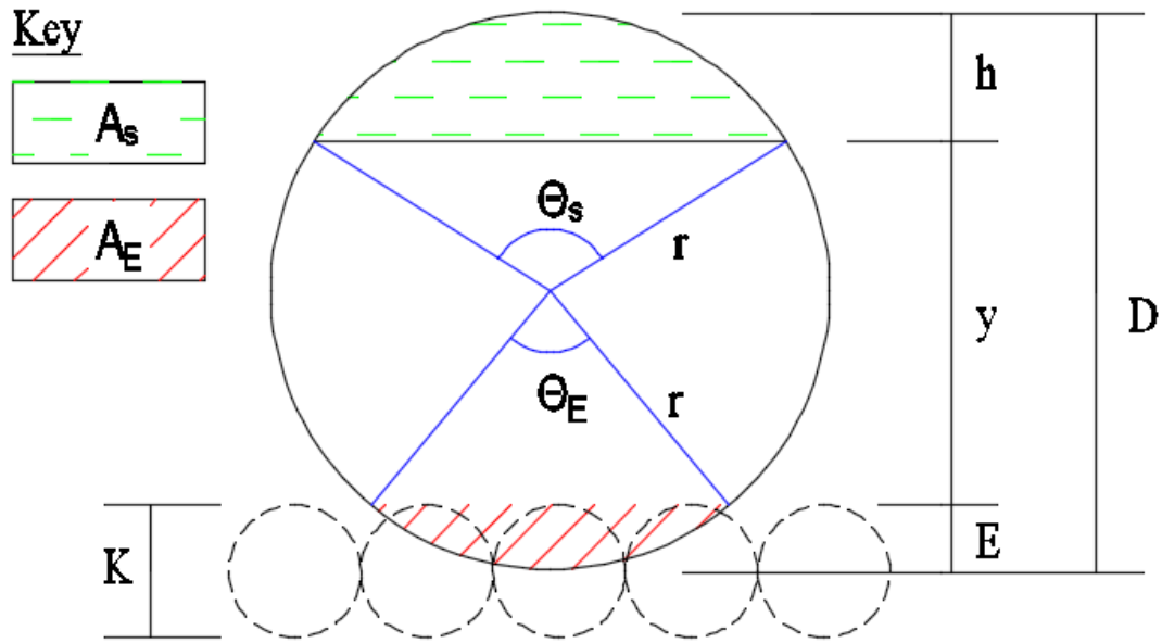
Figure 4-3: Schematic of boulder position for volume and area calculations.
