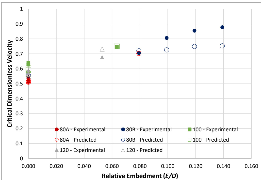
Figure 5-12: Relationship between relative embedment and critical dimensionless velocity.
