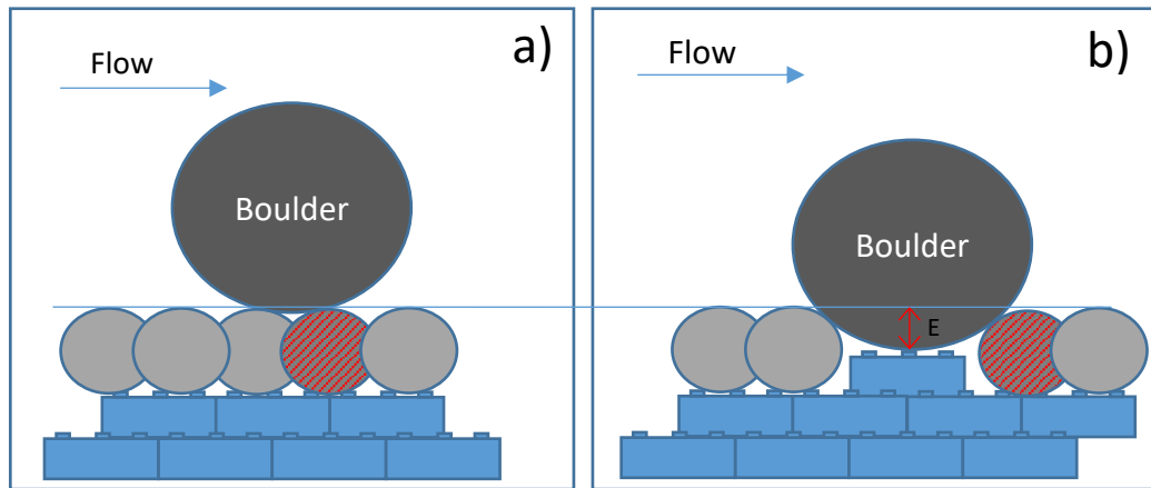
Figure 3-6: Schematic of boulder setup with hatched spheres representing the pivot spheres (a: no embedding, b: embedded a distance E ).
