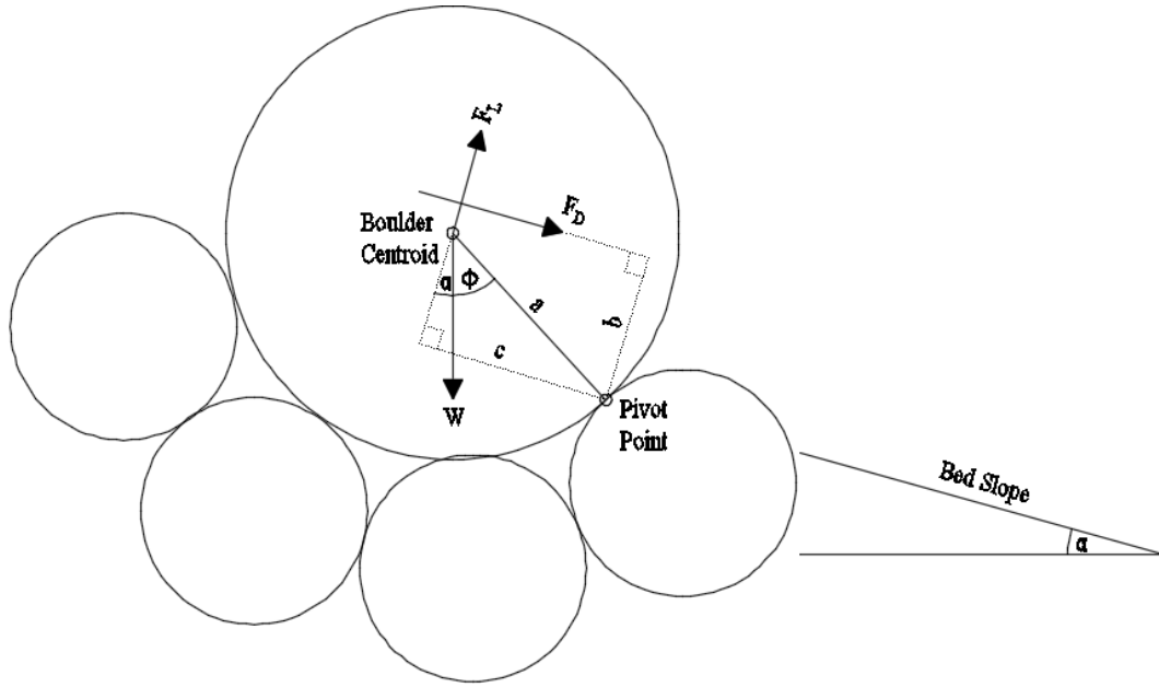
Figure 4-5: Moment lever arms a , b and c , about the pivot point.
