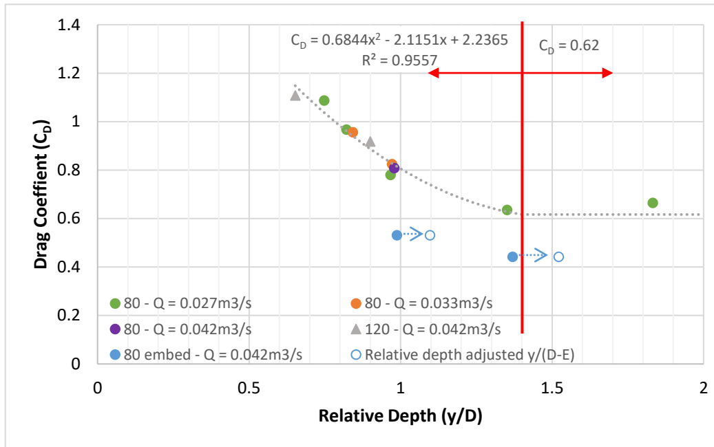
Figure 5-1: Relationship between relative flow depth and drag coefficient.
