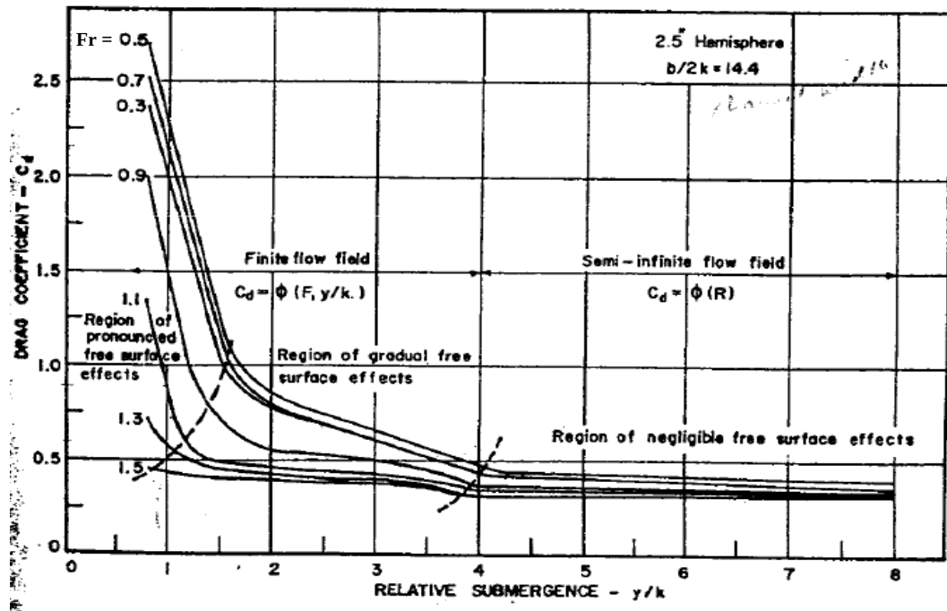
Figure 4-4: Relationship for relative submergence and drag coefficient for hemispheres (Flammer et al. 1970).
