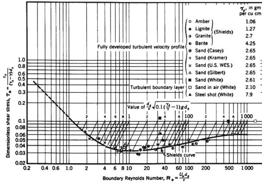
Figure 2-2: Shields Diagram for Incipient Motion (Vanoni 1975).
