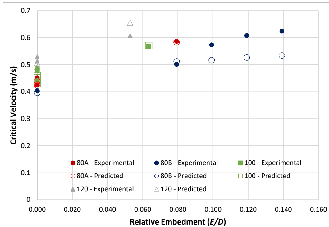
Figure 5-13: Relationship between relative embedment and critical average velocity.
