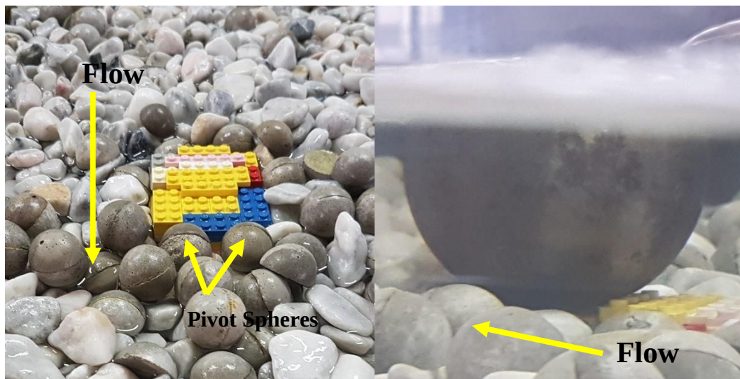
Figure 3-7: Lego configuration for boulder being embedded.
