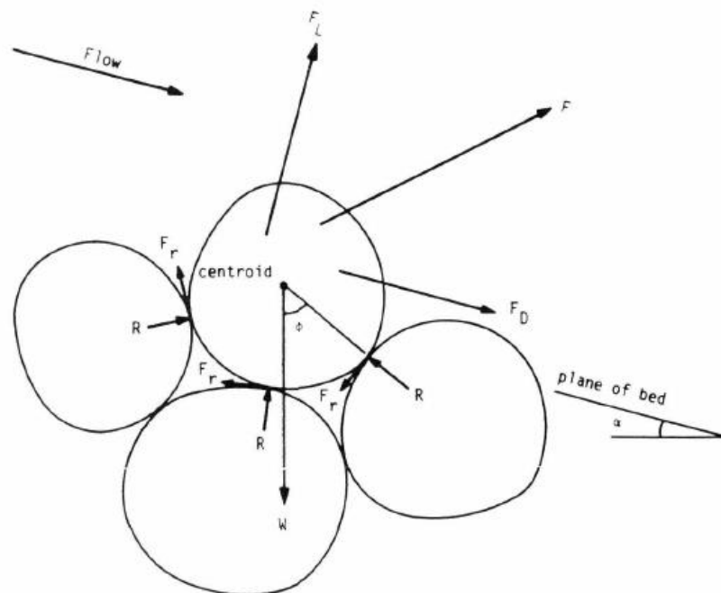
Figure 2-7: Forces acting on a particle (James 1990).
