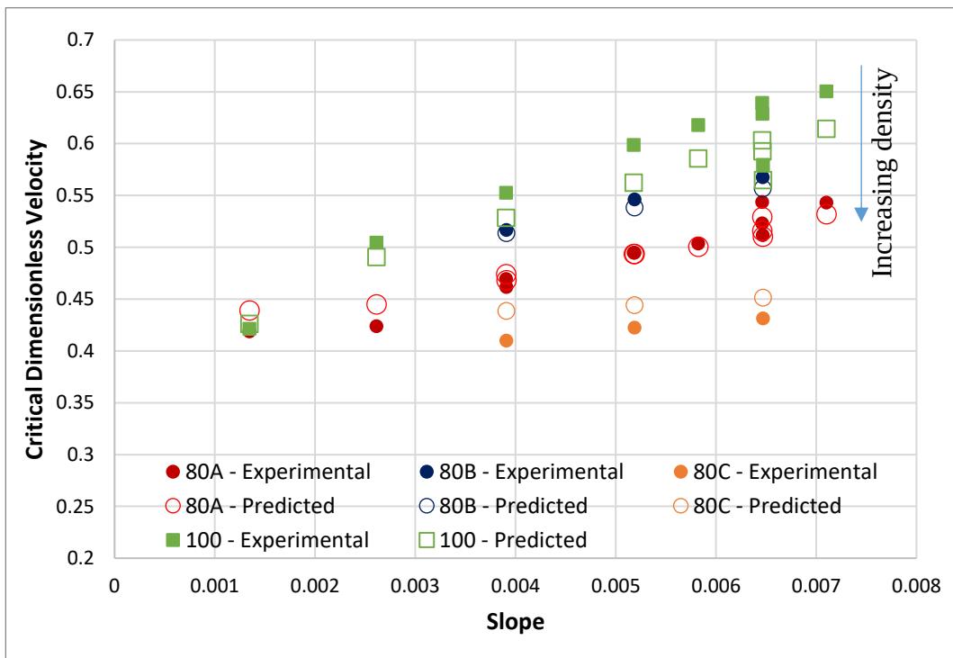
Figure 5-7: Relationship between slope and critical dimensionless velocity.
