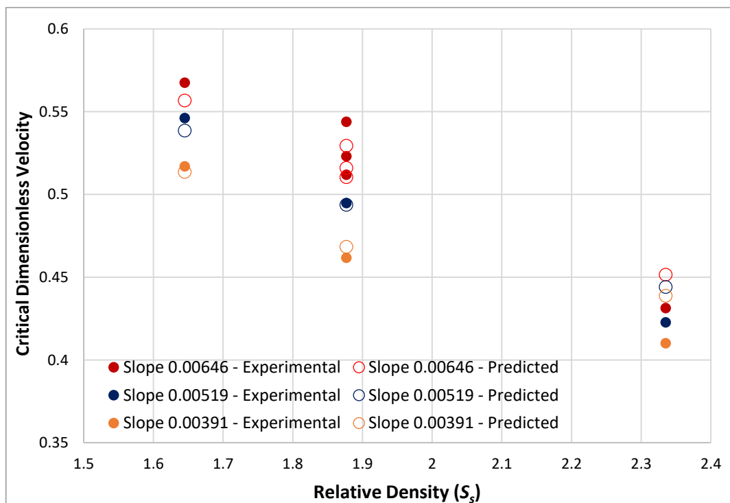
Figure 5-11: Relationship between relative density and critical dimensionless velocity.
