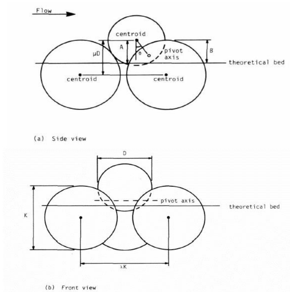
Figure 2-8: Pivoting Geometry (James 1990).
