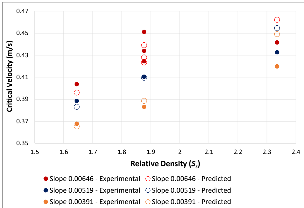
Figure 5-10: Relationship between relative density and critical average velocity.
