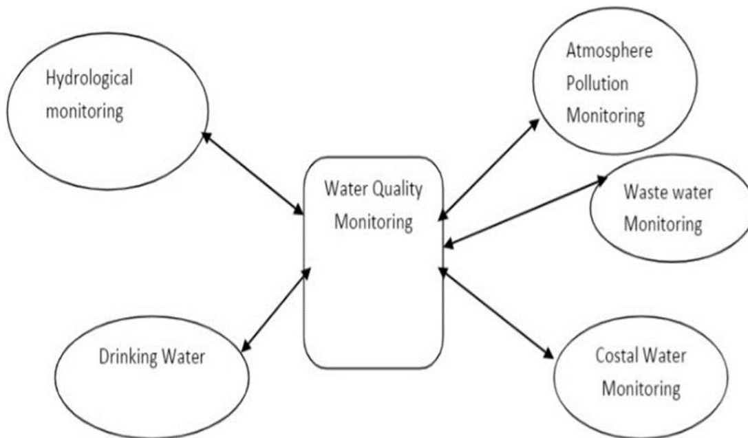
Figure 2.3. The interactions between the main environmental monitoring systems for water quality (Mishra and Dubey, 2015)
