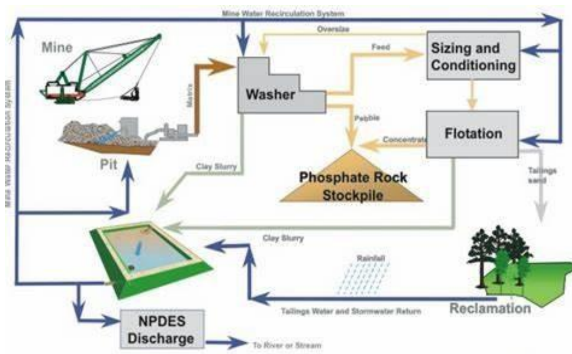
Figure 2.4 A graphical representation outlining the steps in a phosphate mine's process (Gold Sim Blog, October 2015)
