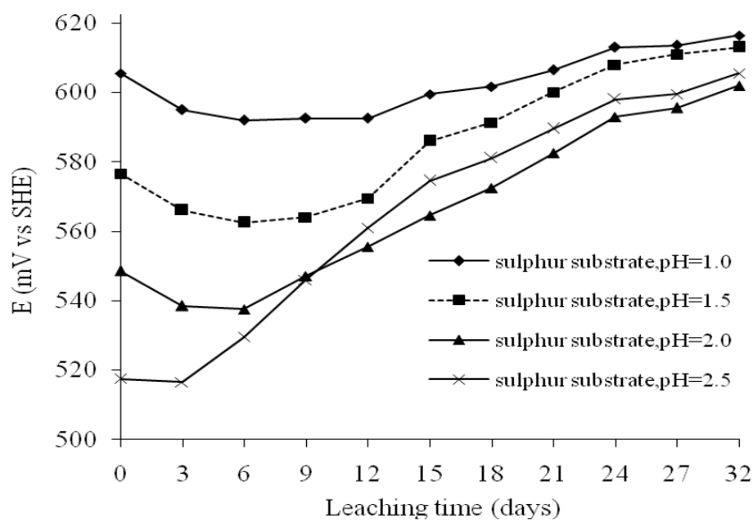
Figure 6.11. Evolution of ORP with time for sulphur substrate
