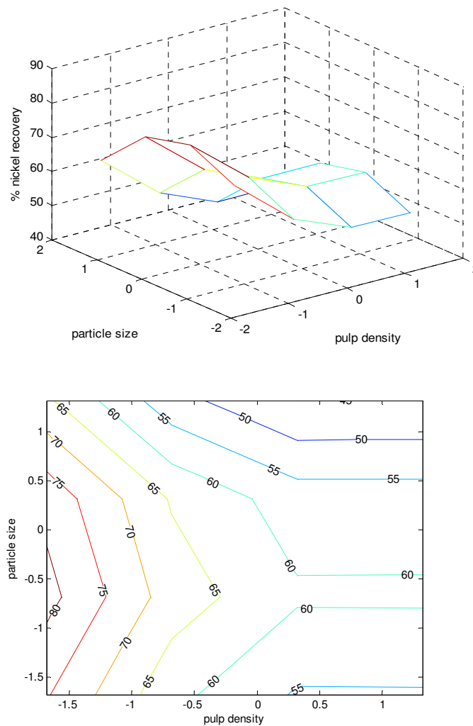
Figure 7.2. Response surface and contour plots at constant pH
