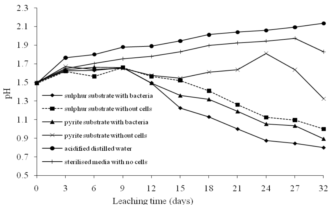
Figure 6.13. Evolution of pH with time at initial pH of 1.5 for different media compositions
