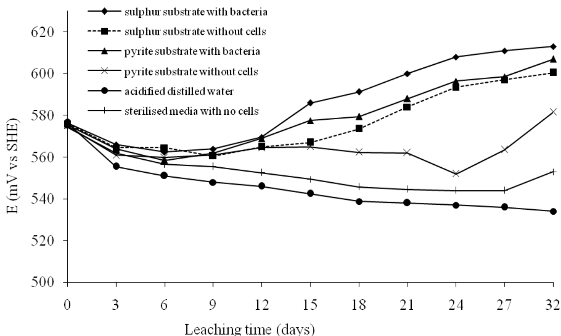
Figure 6.14. Evolution of ORP with time at initial pH of 1.5 for different media composition
