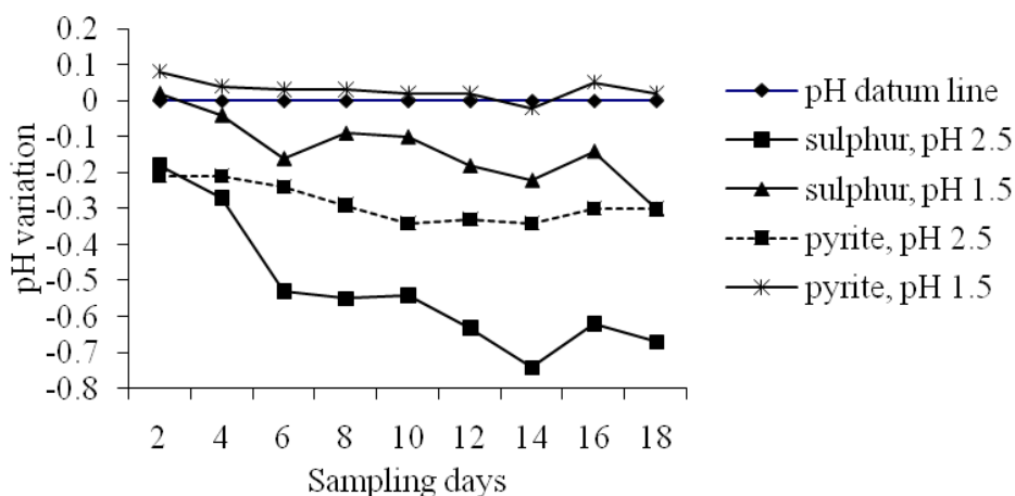
Figure 5.11. pH variation profiles (fold-over design)
