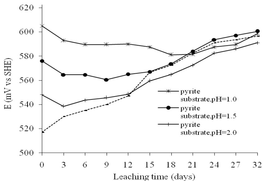
Figure 6.12. Evolution of ORP with time for pyrite substrate
