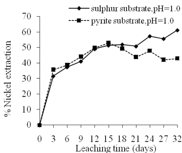
Figure 6.3. Dissolution rates of nickel laterites as a function of substrate type at initial pH of 1.0
