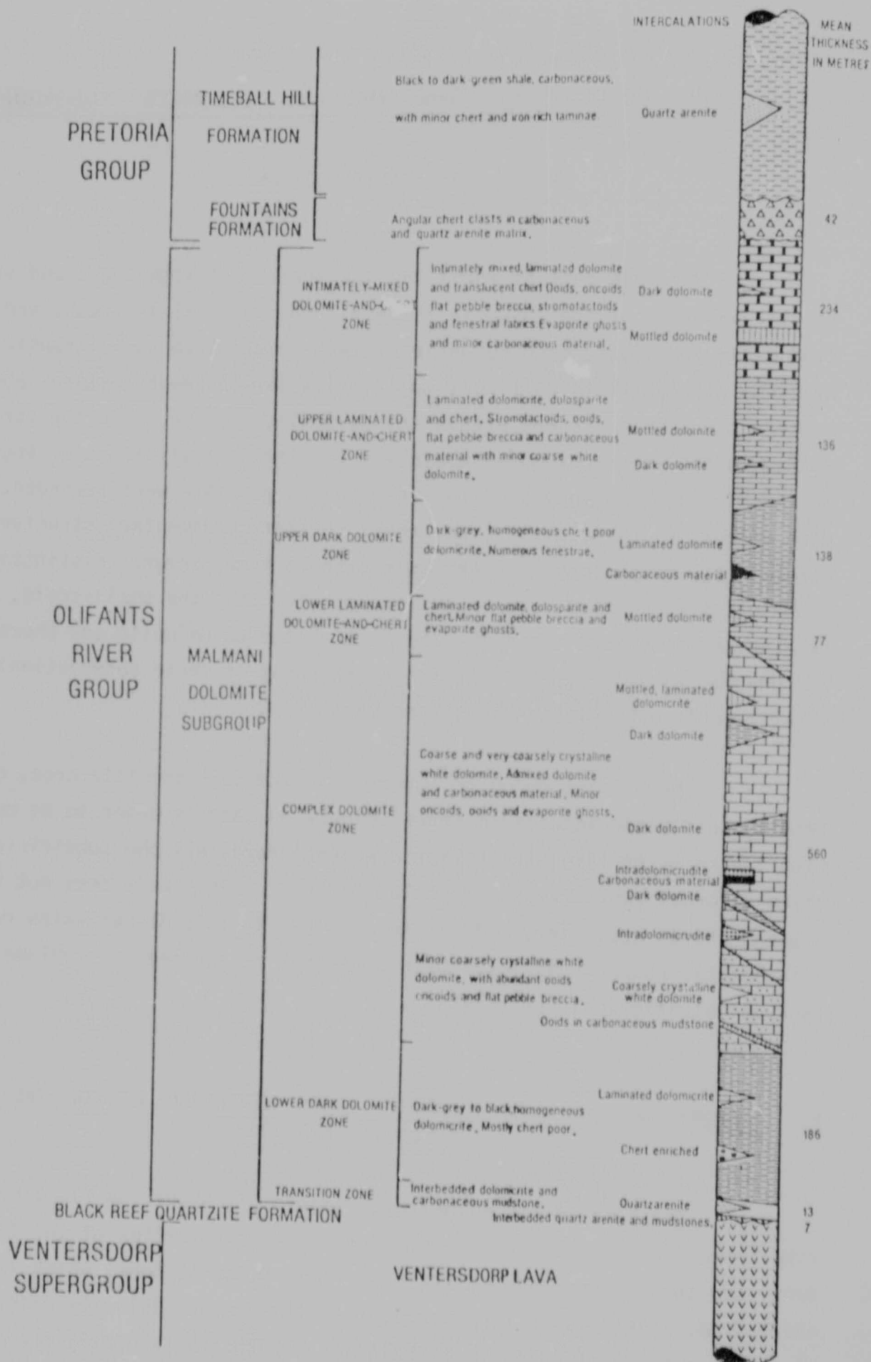
Figure 9 : The descriptive stratigraphy of the Transvaal Supergroup in the Carletonville area, showing the zonal subdivisions made within the Malmani dolomite.
