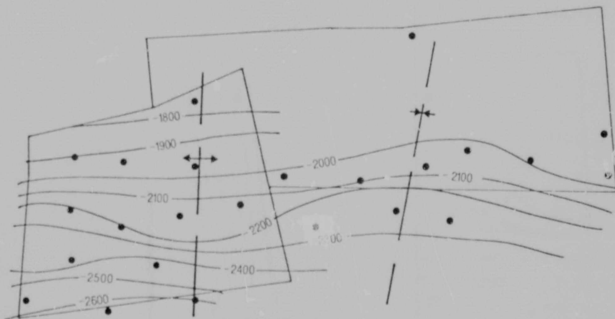
Figure 12 : A structure contour map of the top of the Ventersdorp lavas. Contour interval 100 metres. Datum 1828,74 metres above sea level.
