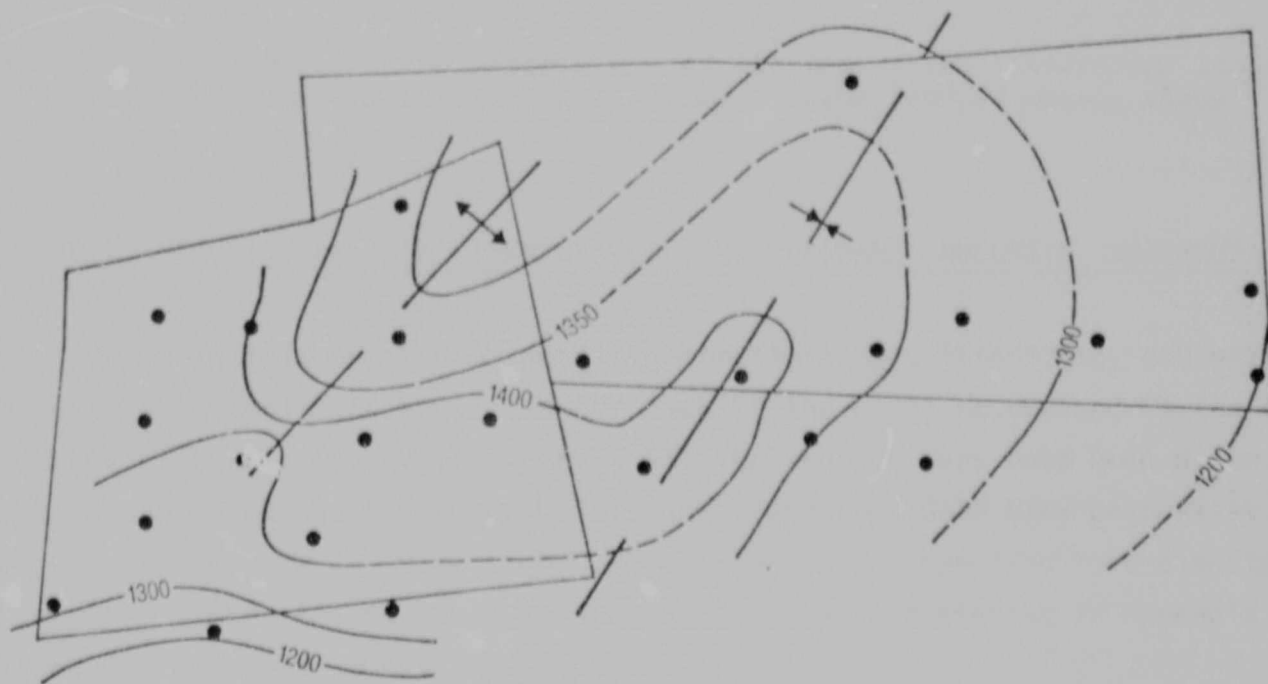
Figure 11 : An isopach map of the Malmani dolomite. Contour interval 100 metres.
