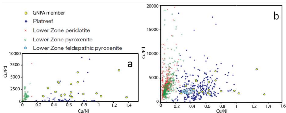
Figure 4.17: Binary variation diagrams of Cu/Ni, and Cu/Pd ratios, showing data for the GNPA member pyroxenite from this study, plotted against Platreef and the Lower Zone peridotite, pyroxenite, and feldspathic pyroxenite after Yudovskaya (2013). Samples plotted against (a) Sandsloot samples and (b) Turfspruit showing that the GNPA samples display a similar distribution to that of the Platreef on Turfspruit.
