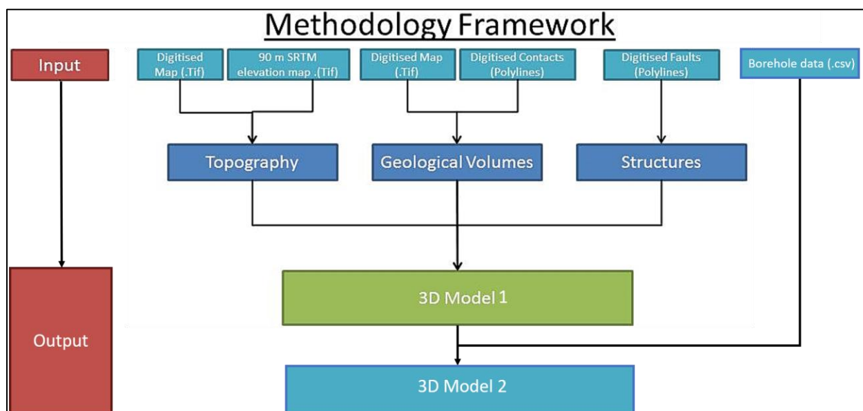
Figure 5.1: Modelling methodology framework followed to design a 3D geological model.
