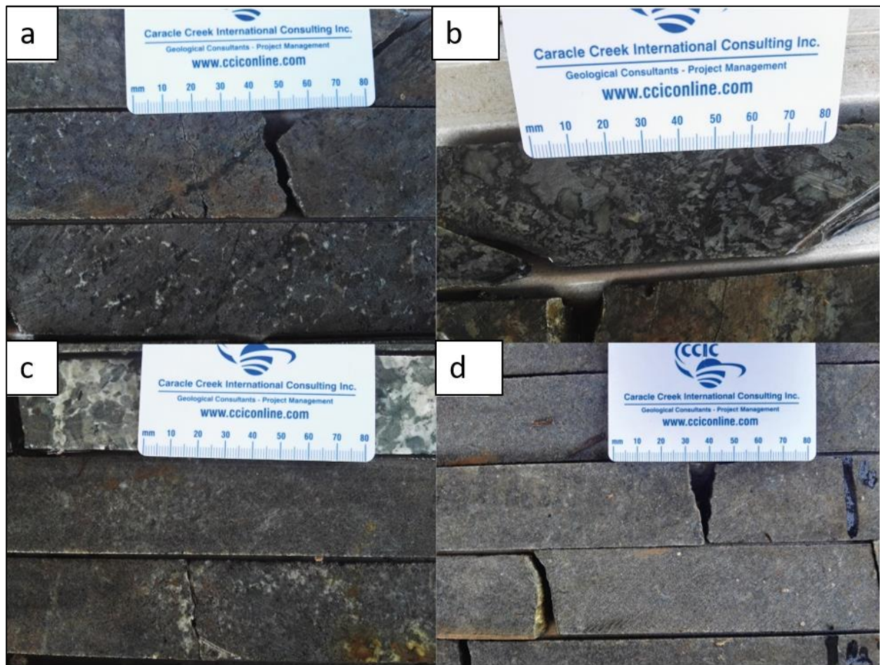
Figure 3.8: Various pyroxenites. (a) Coarse-grained feldspathic pyroxenite. (b) Altered coarse-grained feldspathic pyroxenite. (c) Fine-grained feldspathic pyroxenite with weathered mineralised sulphides. (d) Fine-grained pyroxenite with sulphide specks.
