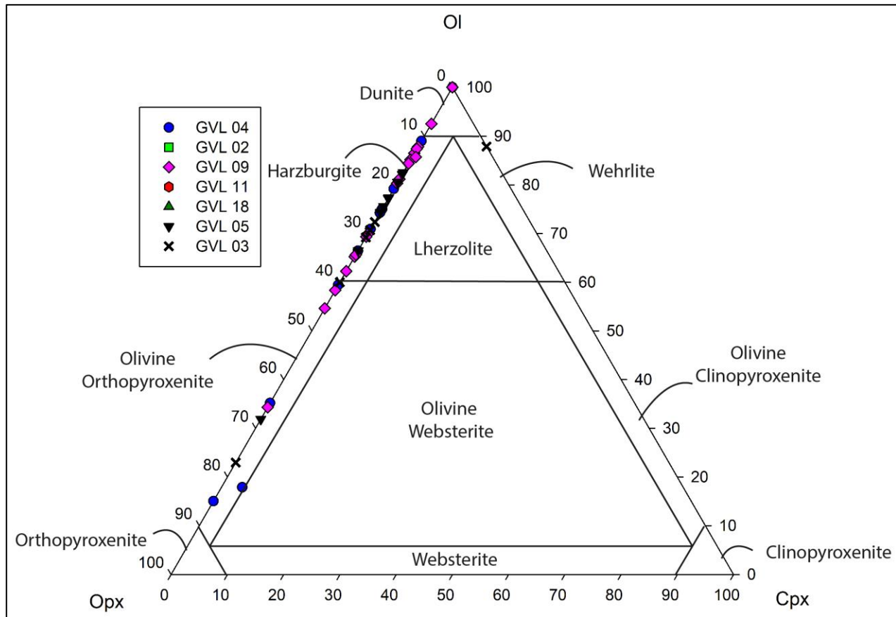
Figure 4.2: Classification and nomenclature of ultramafic rocks based on the CIPW proportions of olivine (Ol), orthopyroxene (Opx) and clinopyroxene (Cpx) (after Streckeisen, 1976).
