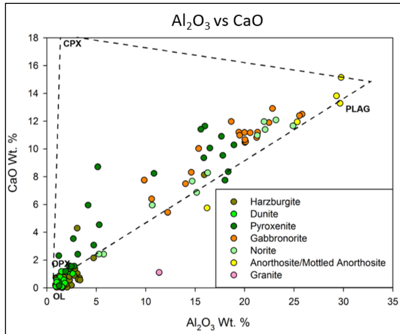
Figure 4.5: Classification of samples K-1 to K-133 showing \text{Al}_2\text{O}_3 against CaO wt. %. The classification parameters have been adopted from Hulbert (1983). Samples have been coloured according to the hand sample classification.
