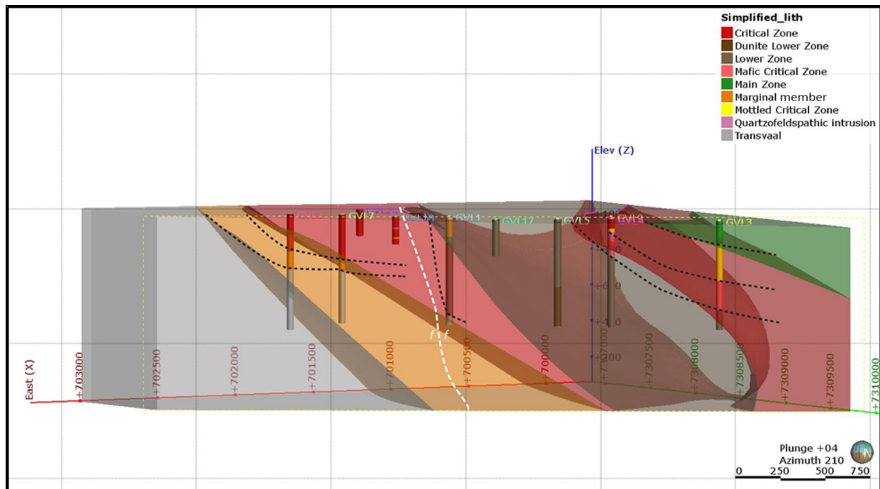
Figure 5.14: Sectional view of the Grasvally body looking south. Inferred boundaries in black stippled lines, and fault in white stippled line. The orange unit represents gabbro-norite which was interpreted as being part of the marginal member however modelling shows that within GVL 1 this gabbro-norite is part of the Critical Zone.
