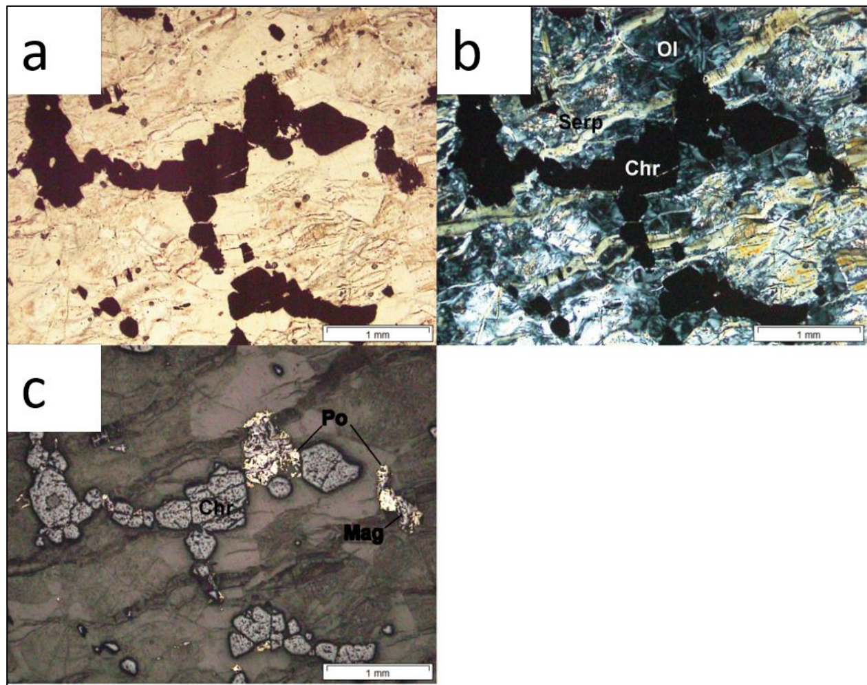
Figure 3.14: Photomicrographs of a serpentinised chromite-bearing harzburgite in both transmitted and reflected light. (a) serpentinised harzburgite in PPL with opaque chained chromite. (b) Serpentinised harzburgite in XPL dominated by secondary serpentine veins. (c) Serpentinised harzburgite in RL with chained chromite, chromite displaying atoll textures and interstitially disseminated pyrrhotite, chalcopyrite and magnetite.
