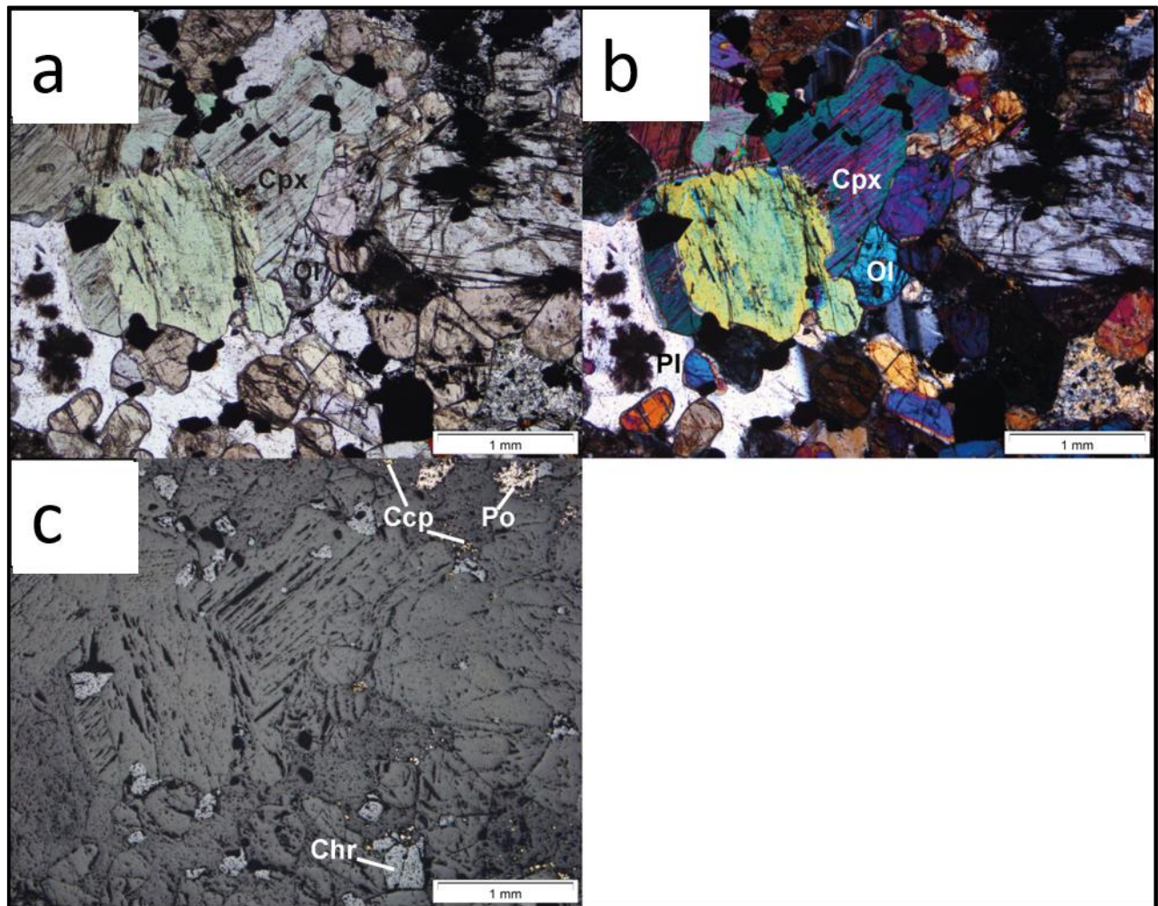
Figure 3.16: Photomicrographs of a mineralised pyroxenite in both transmitted and reflected light. (a) Pyroxenite in PPL displaying clinopyroxene with exsolution lamellae and annealed olivine and altered orthopyroxenes. (b) Pyroxenite with clinopyroxene displaying exsolution lamellae, olivine and orthopyroxene. (c) Pyroxenite in RL displaying chromite, interstitially disseminated pyrrhotite with lesser specks of disseminated chalcopyrite.
