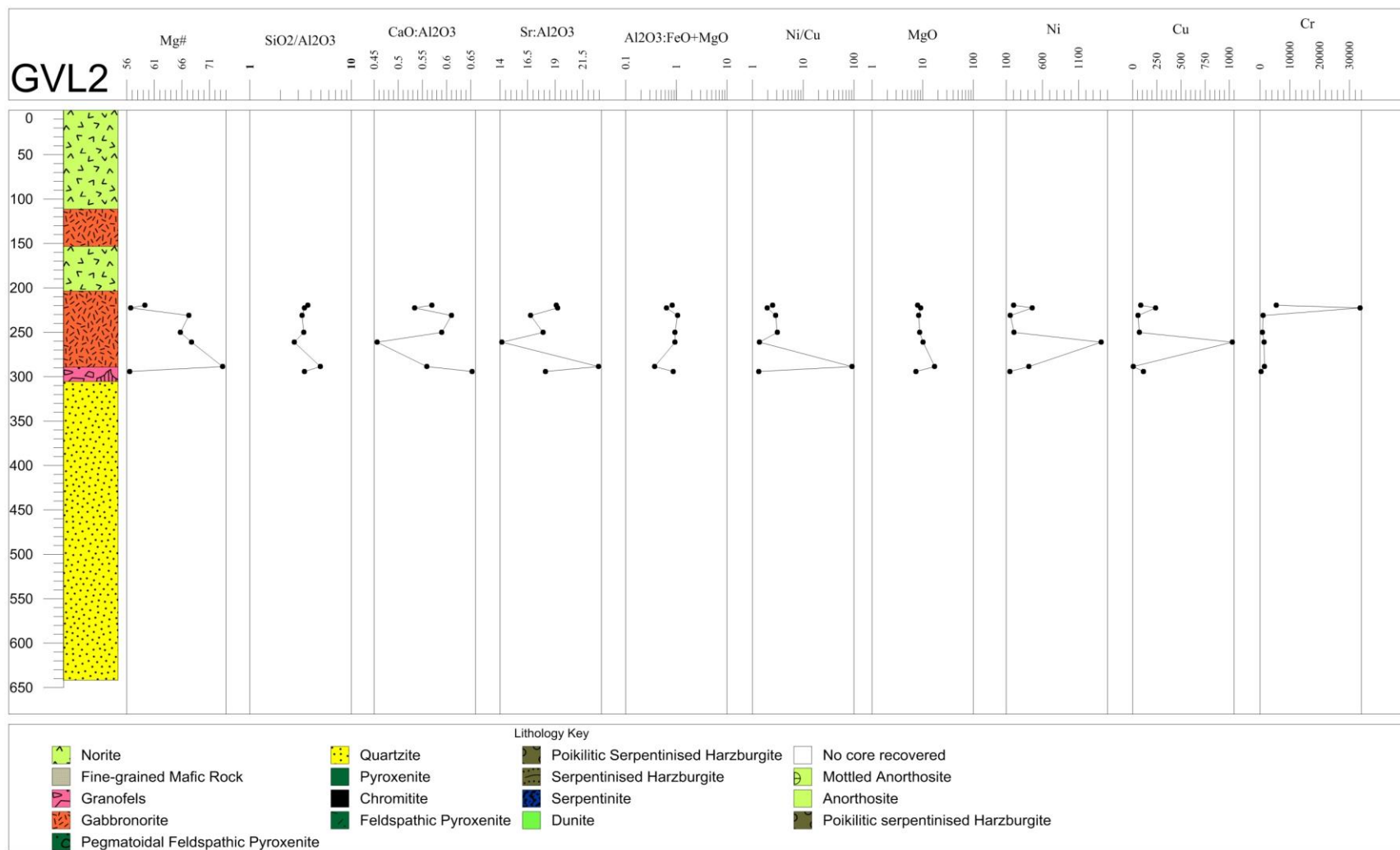
Figure 4.14: Variations of the whole-rock Mg#, major and trace element ratios and trace element contents through part of borehole the GVL 2. The Mg# displays a decrease up section within the gabbronorite. The Cr displays a sharp increase in Cr at 210 m whereas the Cr is below 200m ppm elsewhere within this unit.
