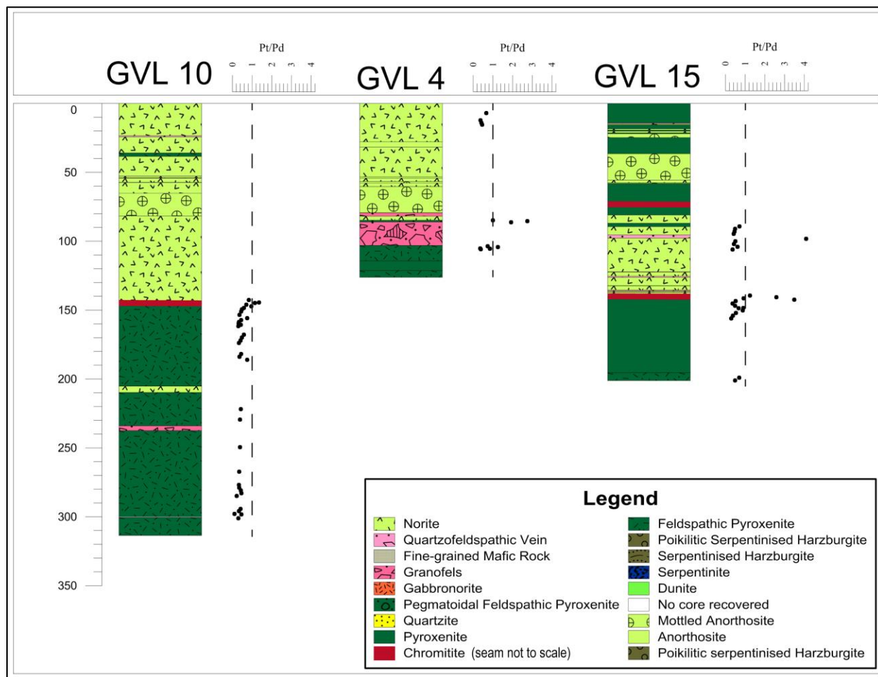
Figure 4.16: Pt/Pd ratios for boreholes GVL 10, GVL 4 and GVL 15 plotted against depth. The chromitite seam markers are not to scale. Stippled line indicates average Pt/Pd ratio for the overall Platreef although different sills within the Platreef as a whole have distinctly different Pt/Pd ratios (1:1 Pt/Pd) (Kinnaird, 2005a).
