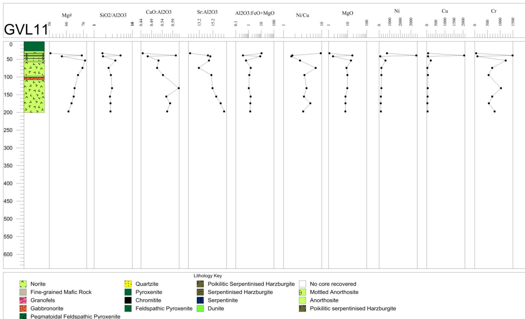
Figure 4.12: Variations of the whole-rock Mg#, major and trace element ratios and trace element contents through borehole GVL 11.
