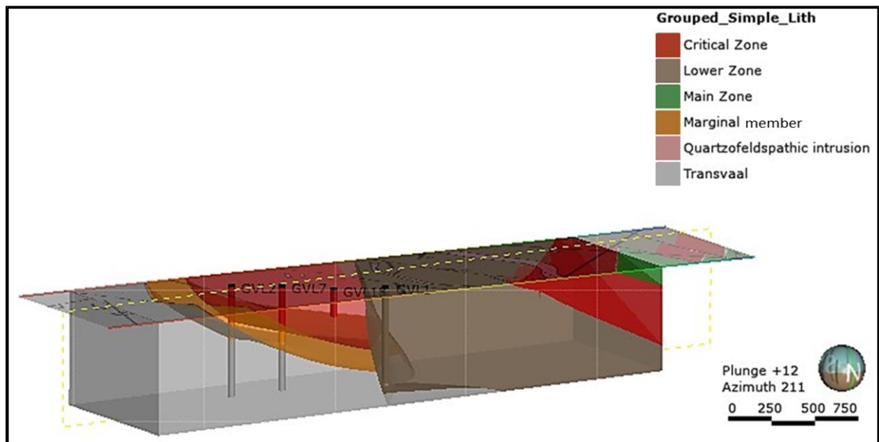
Figure 5.15: Sectional view of the Grasvally body looking south. Boundaries have been further constrained by the incorporation of simplified borehole data.
