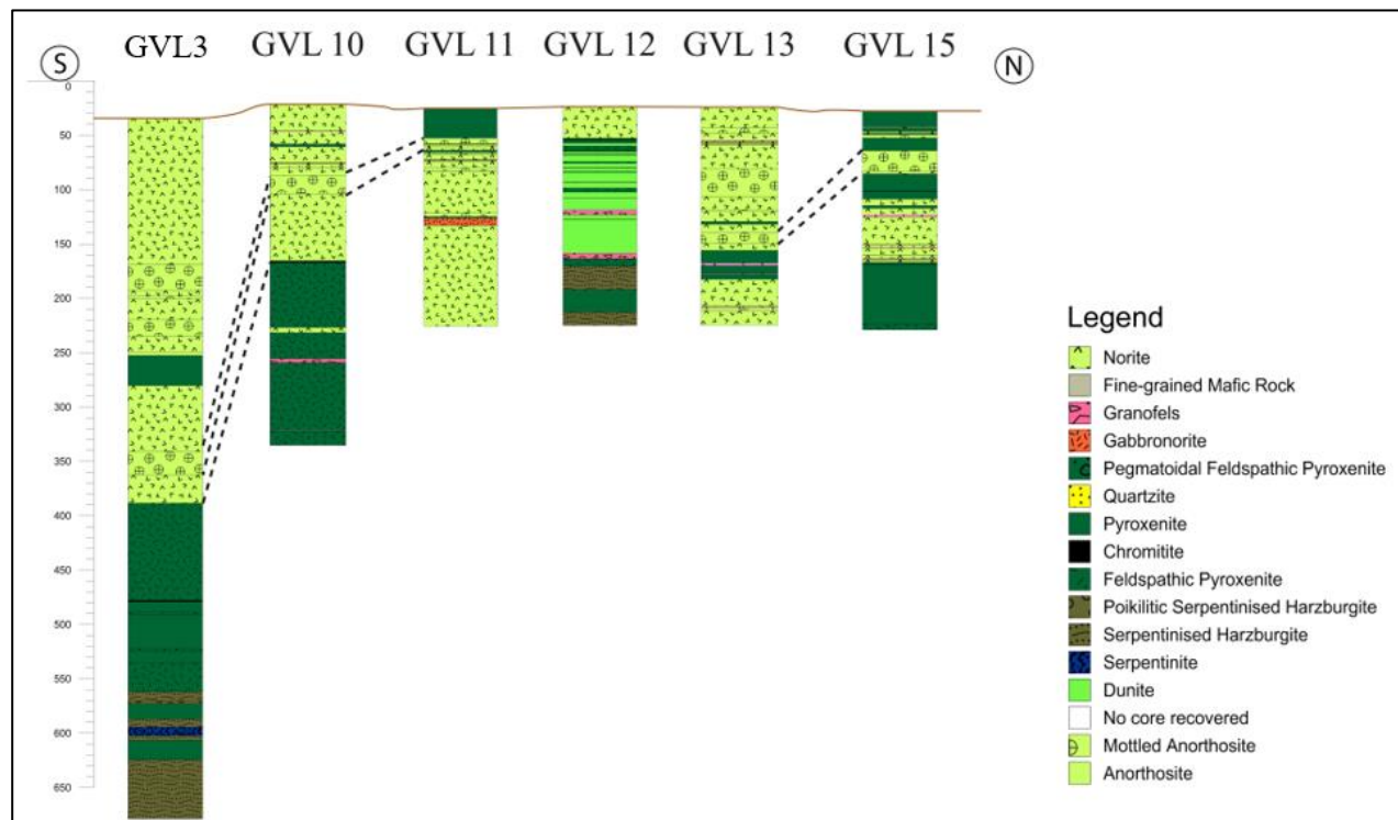
Figure 3.26: Tentative correlations based on hand sample and thin section descriptions of boreholes arranged from south to north.
