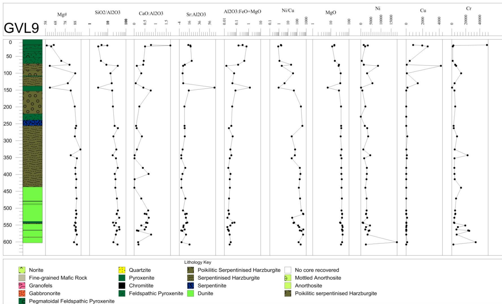
Figure 4.10: Variations of the whole-rock Mg#, major and trace element ratios and trace element contents through borehole GVL 9.
