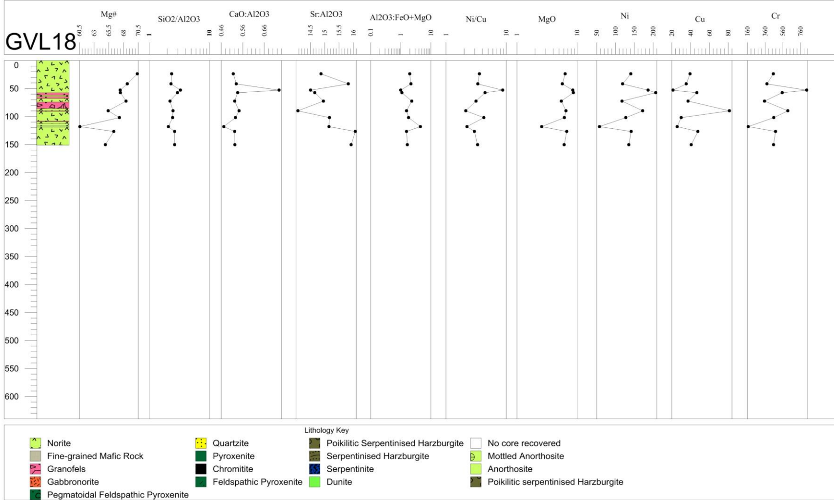
Figure 4.13: Variations of the whole-rock Mg#, major and trace element ratios and trace element contents through borehole GVL 18.
