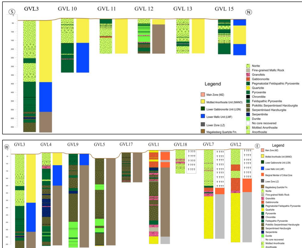
Figure 3.27: Simplified lithological logs of chosen representative holes correlated with the stratigraphic subdivisions of de Klerk (2005).
