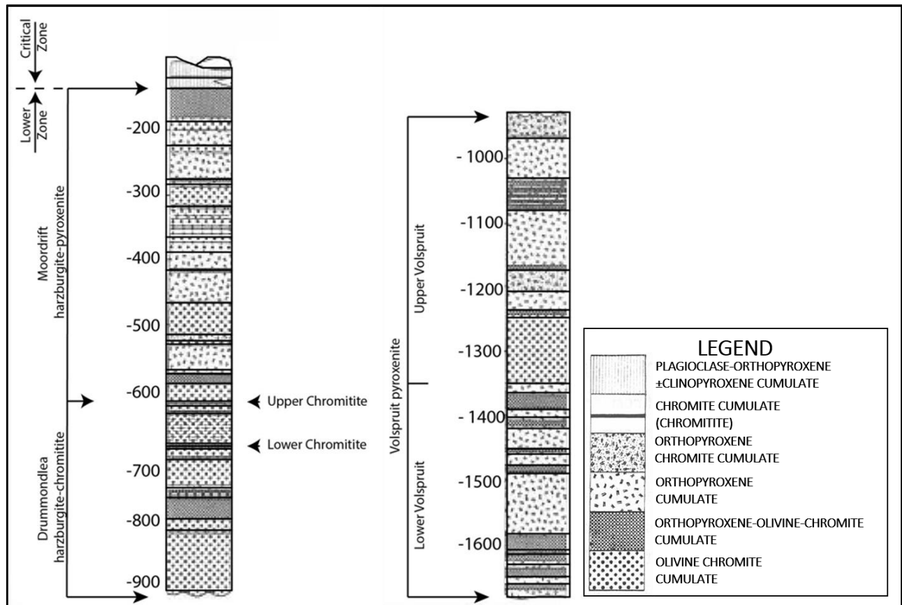
Figure 2.3: Stratigraphic column of the northern limb Lower Zone south of the Ysterberg-Planknek Fault. Adapted from Hulbert (1983).
