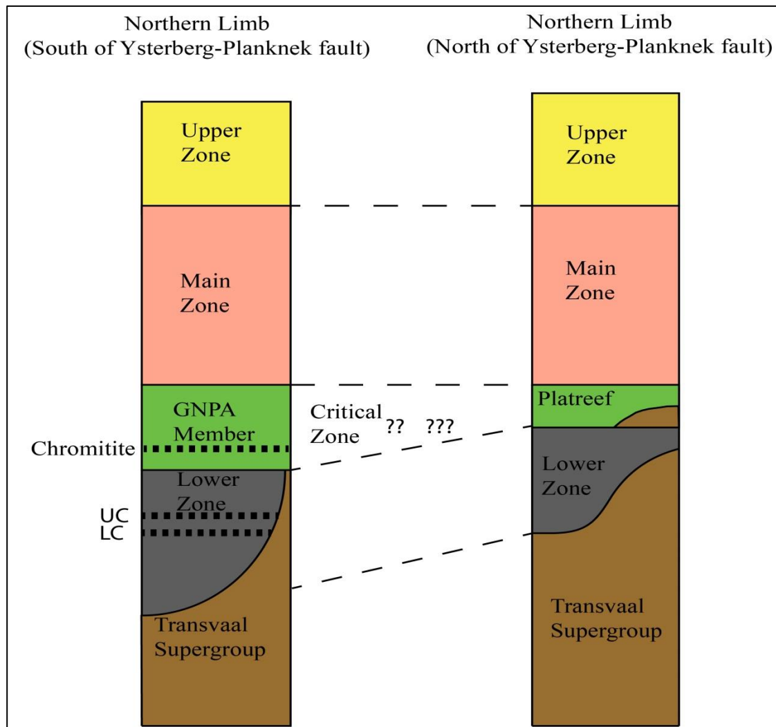
Figure 2.2: Differences between northern limb stratigraphy to the north and south of the Ysterberg-Planknek Fault Adapted from Smith et al. (2011).
