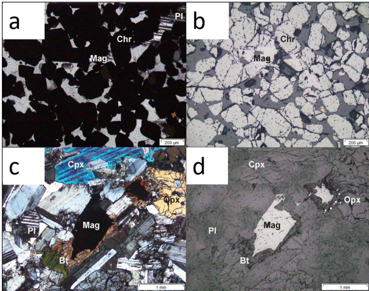
Figure 3.21: Photomicrographs of various opaque minerals observed in core. Interstitially distributed cumulus chromite and lesser magnetite in XPL within feldspathic gabbronorite (a) in PPL and (b) in RL. (c) Gabbronorite dominated by feldspar with interstitial clinopyroxene with exsolution lamellae highly fractured and altered orthopyroxene with inclusions of feldspar. (d) Interstitial intercumulus magnetite with associated biotite and minor specks of pyrite within gabbronorite.
