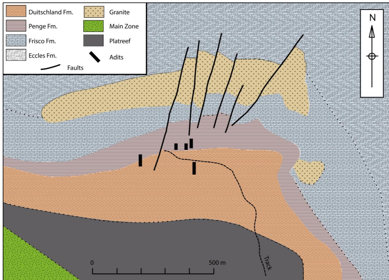
Figure 2.8: Geological map of Tweefontein Hill showing the distribution of lithologies, faults and adits. Stippled lines show inferred geological contacts and solid lines are observed contacts (Nex, 2005).
