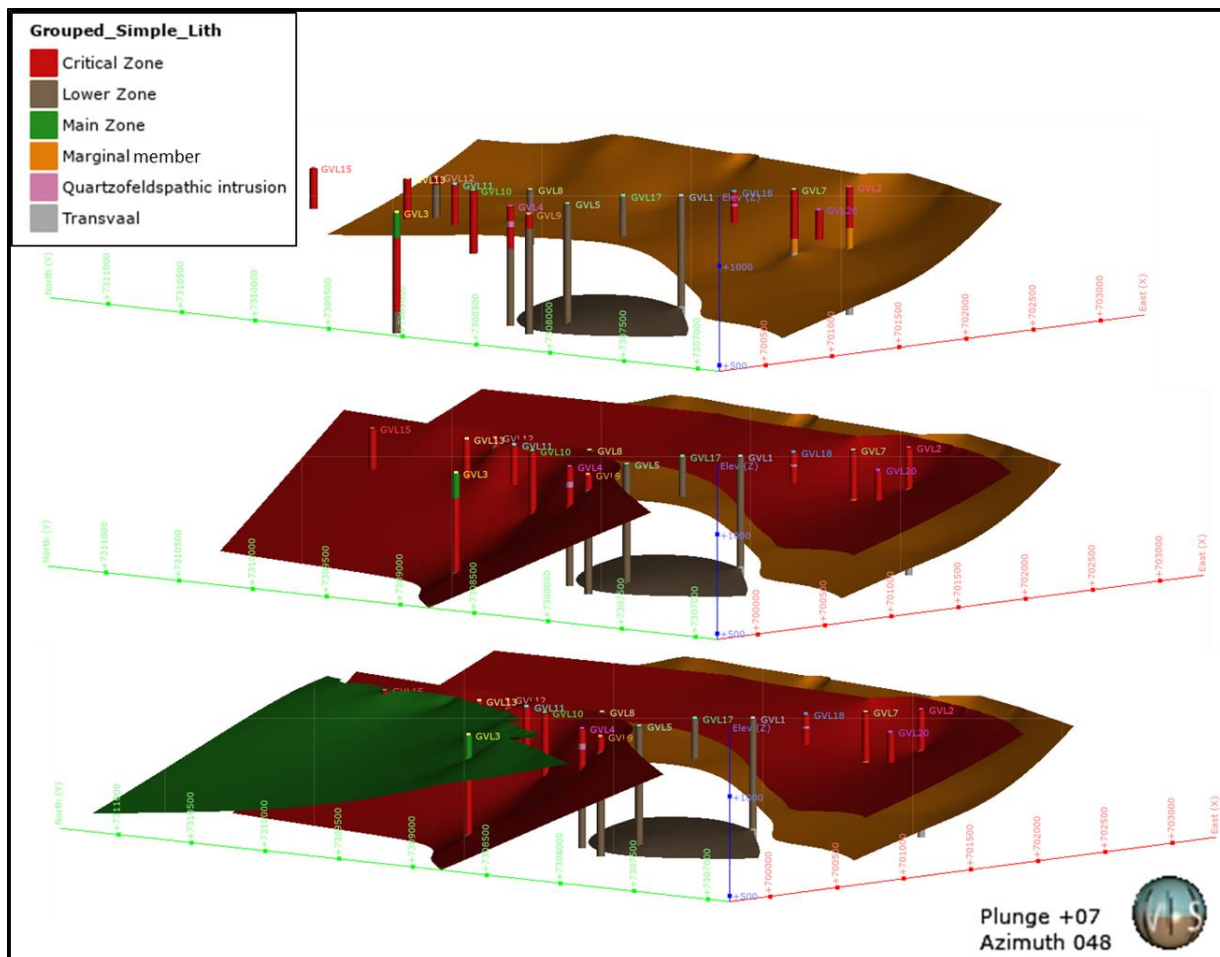
Figure 5.11: Three-dimensional surfaces further constrained with the use of simplified borehole data showing the general orientation of the contacts as well as the dip of the volumes to the east and to the west of the major N-S trending fault.
