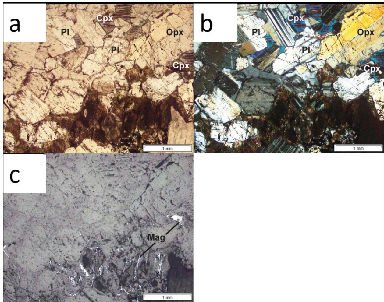
Figure 3.19: Photomicrographs of an altered anorthosite in both transmitted and reflected light. (a) Anorthosite in PPL with dominant plagioclase crystals as well as darker coloured areas of alteration. (b) Anorthosite displaying dominant plagioclase crystals heavily altered to sericite, interstitial clinopyroxene as well as orthopyroxene. (c) Secondary veinlets of magnetite as well as interstitial magnetite is present associated with the sericitised zone.
