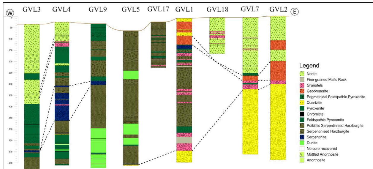
Figure 3.25: Tentative correlations based on hand sample and thin section descriptions of boreholes arranged from west to east.
