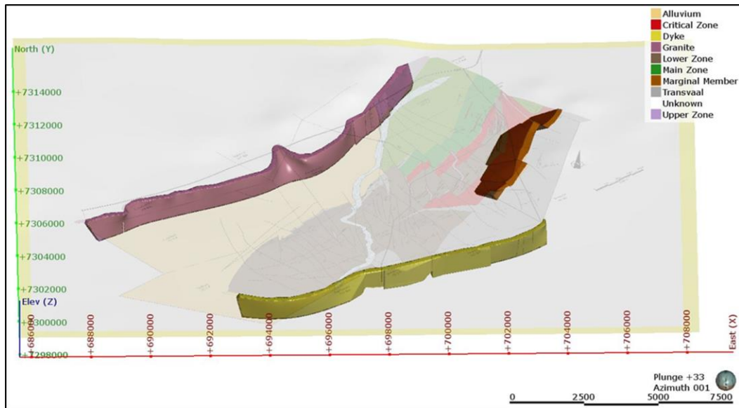
Figure 5.8: Orthographic view from the south of vein-type surfacing of dyke (yellow) marginal member (orange) and the granite body (pink).
