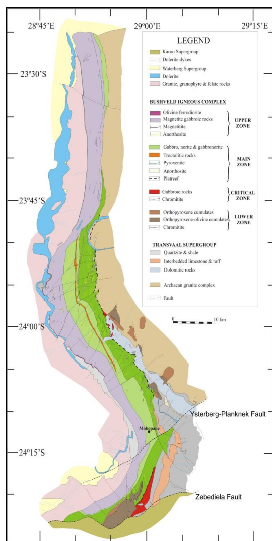
Figure 2.1: The general geology of the northern limb of the Bushveld Complex showing the different stratigraphic units, surrounding rocks and structural features. Original map by van der Merwe (1979); colour map generated by Ashwal et al. (2005); from Kinnaid and McDonald (2005).
