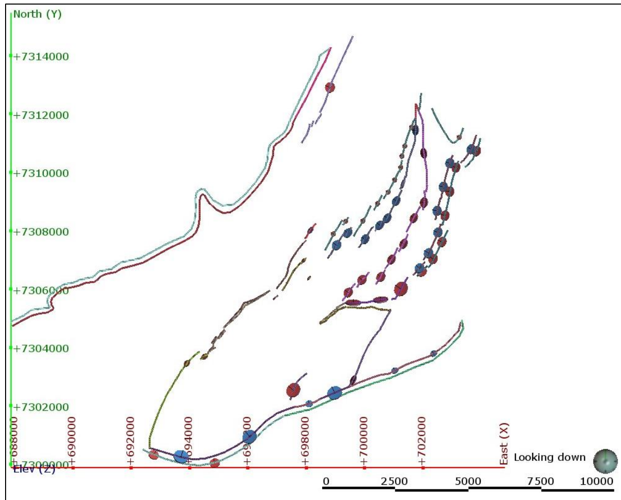
Figure 5.6: Digitised stratigraphic contacts with structural disks. Structural disks are a graphical representation of the orientation of each feature. The colour of the structural disks is based on the polarisation of each contact, red- positive, blue- negative, to influence the interaction of contacts with each other. The structural data was obtained from Hulbert (1983).
