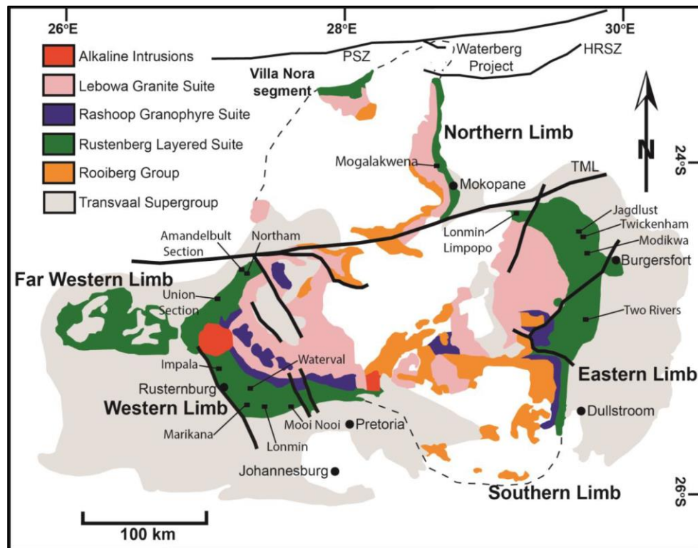
Figure 1.1: Simplified geological map of the Bushveld Complex, which includes the Rustenburg Layered Suite, the Rooiberg Volcanics and the Lebowa Granite Suite adapted from McCreesh, 2018. Major structural features such as the Thabazimbi -Murchison Lineament and the Hout River Shear Zone (HRSZ) are included.
