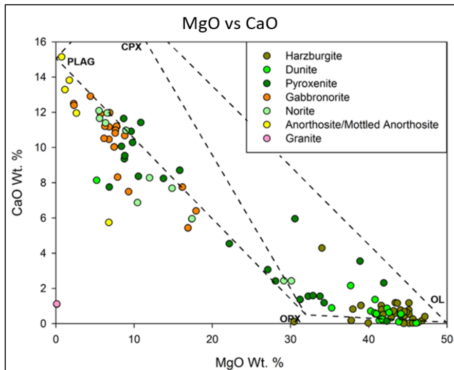
Figure 4.6: Classification for samples K-1 to K-133 on a diagram showing MgO against CaO wt. %. The classification parameters have been adopted from Hulbert (1983). Samples have been coloured according to the hand sample classification.
