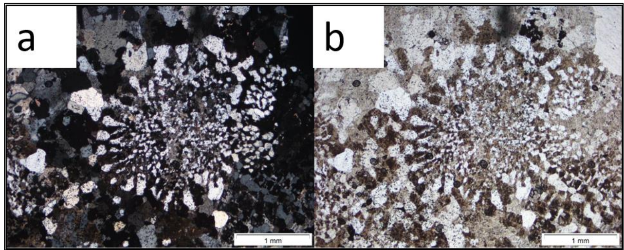
Figure 3.20: Photomicrographs of a granofels in transmitted light displaying granophyric texture. (a) Photomicrograph of quartzofeldspathic vein displaying granophyric texture in XPL. (b) Quartzofeldspathic vein displaying granophyric texture in PPL.
