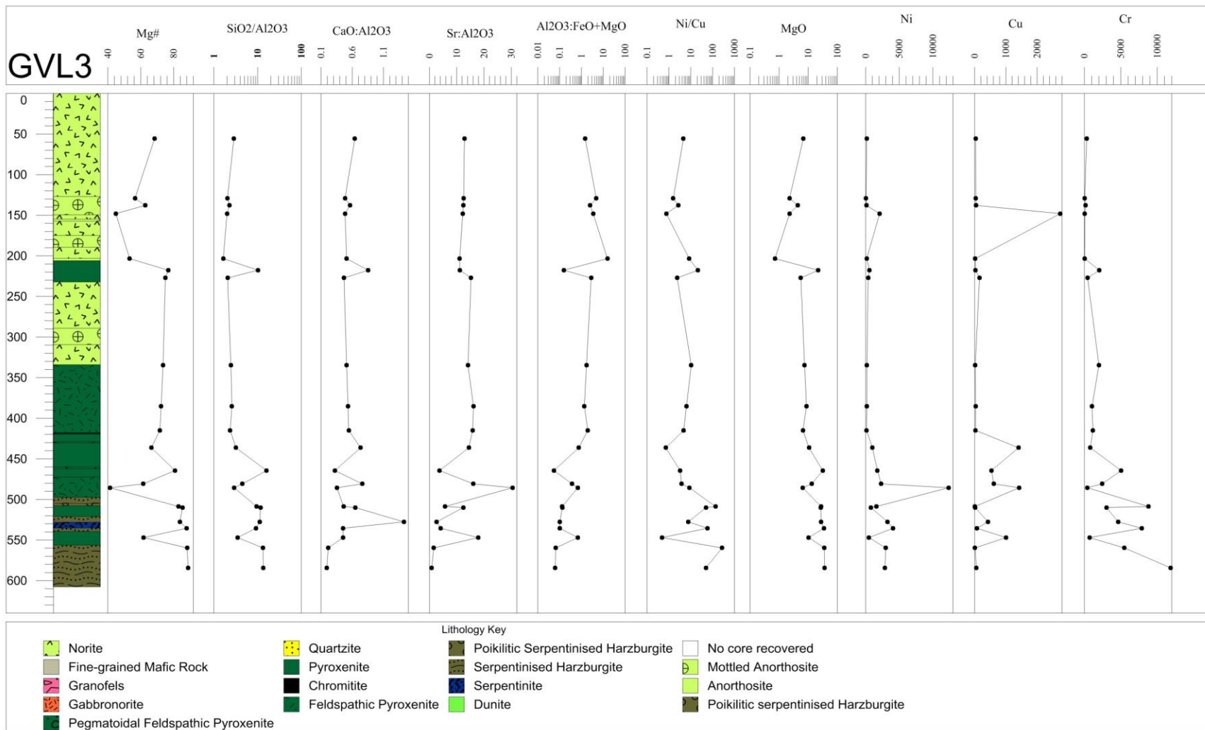
Figure 4.8: Variations of the whole-rock Mg#, major and trace element ratios and trace element contents through borehole GVL 3. Mg# and Cr (ppm) display generally decreasing trends up section as the package transitions into more leucocratic rocks.
