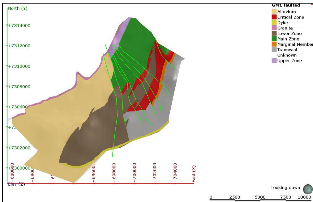
Figure 5.9: Plan view of model with major faults introduced showing how the ENE-WNW faults further offset and compartmentalise the major stratigraphic units within the Grasvally area.
