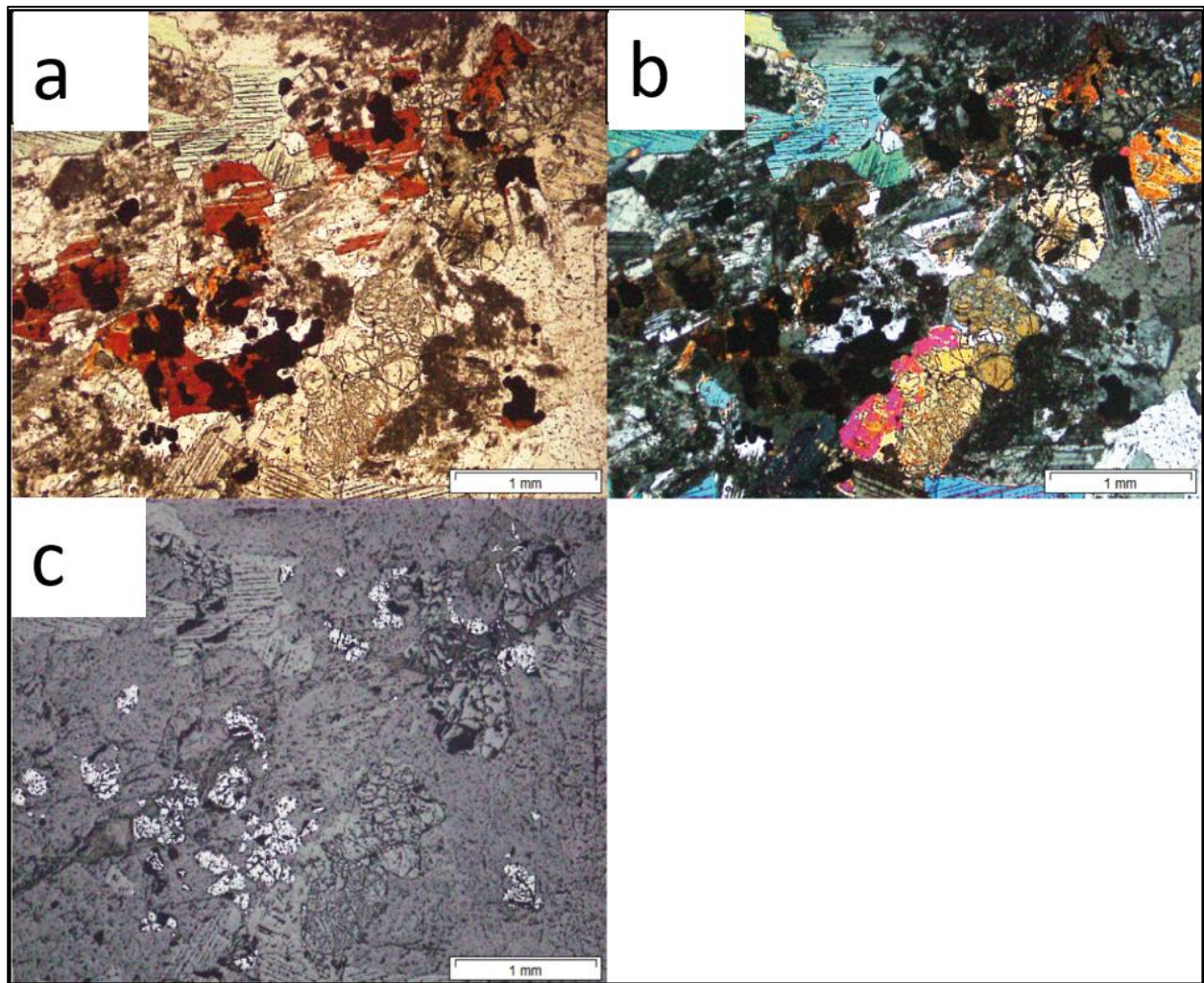
Figure 3.17: Photomicrographs of an altered gabbronorite in both transmitted and reflected light. (a) Gabbronorite in PPL with biotite associated with opaque magnetite. (b) gabbronorite in XPL with highly altered and fractured opx and cpx displaying exsolution lamellae. Sericitisation of feldspars is visible in places. (c) Gabbronorite in reflected light displaying grains of magnetite.
