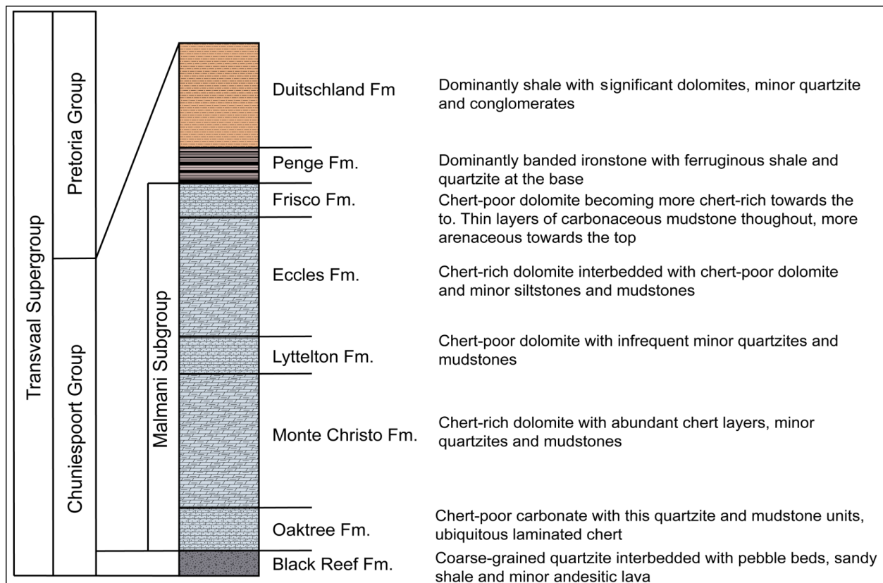
Figure 2.9: Schematic lithostratigraphic column of the lower part of the Transvaal Supergroup in the Mokopane Area after SACS, Greer (1983) and Nex (2005).
