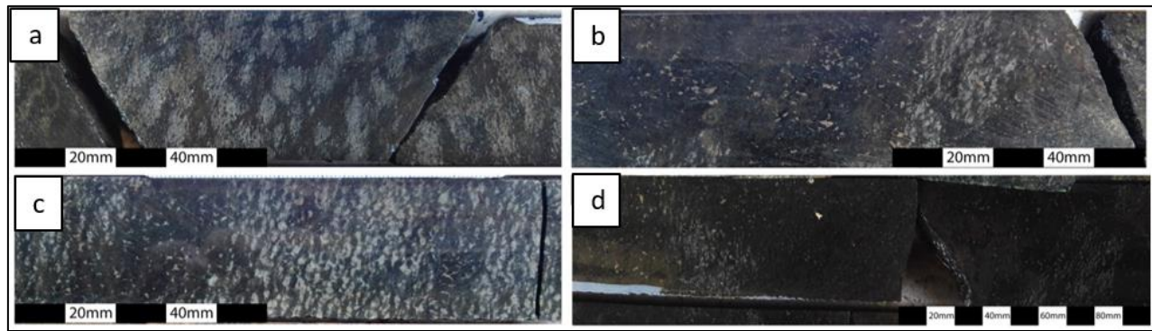
Figure 3.7: Various harzburgites. (a) Poikilitic harzburgite with 1 cm oikocrysts of orthopyroxene and olivine chadacrysts. (b) Serpentinised harzburgite with interstitially disseminated pyrrhotite. (c) Harzburgite with even proportions of orthopyroxene and olivine. (d) Extremely serpentinised harzburgite with widely spaced orthopyroxene oikocrysts.
