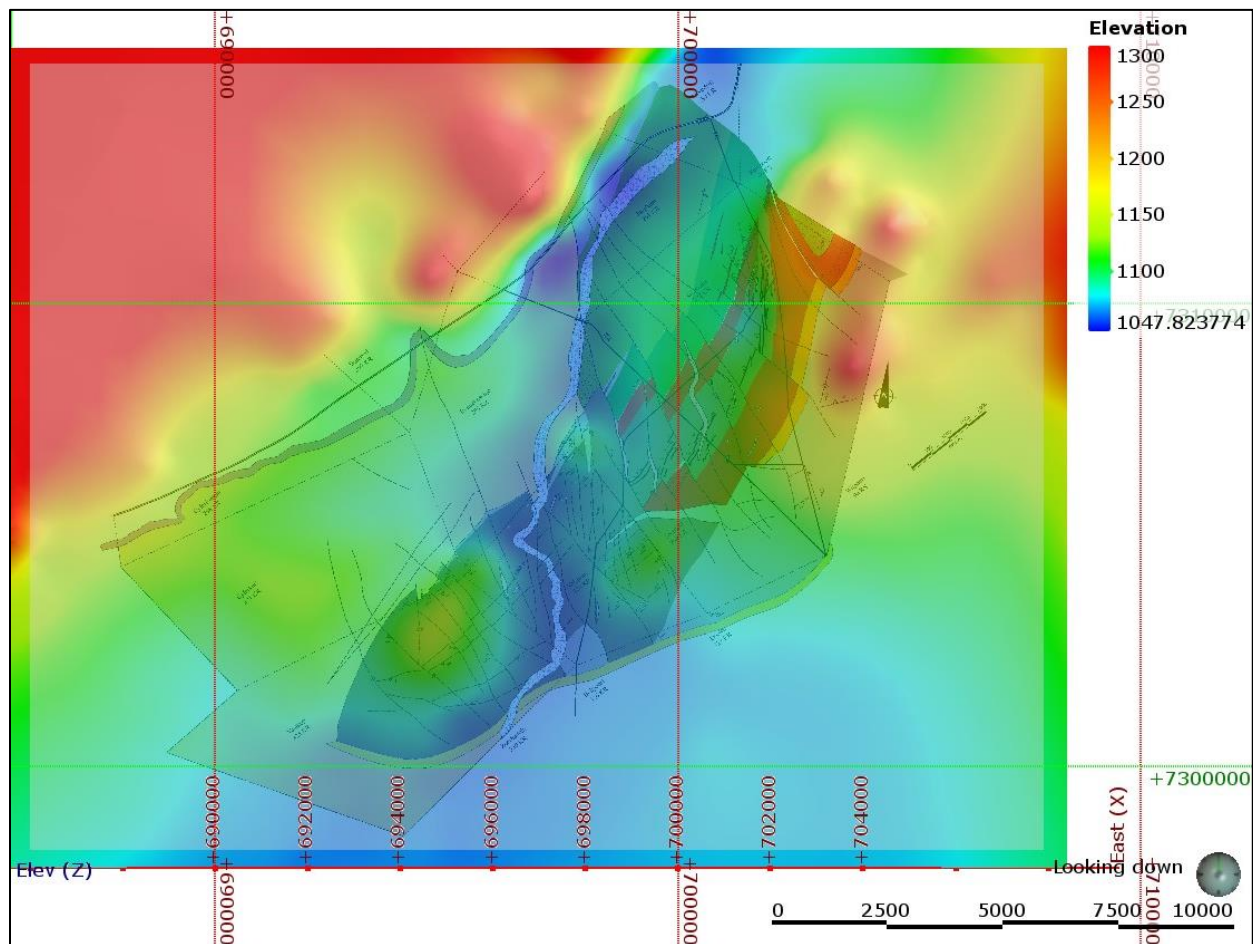
Figure 5.2: A topographic map of the Grasvally area with the geological map overlain, generated in Leapfrog Geo®.
