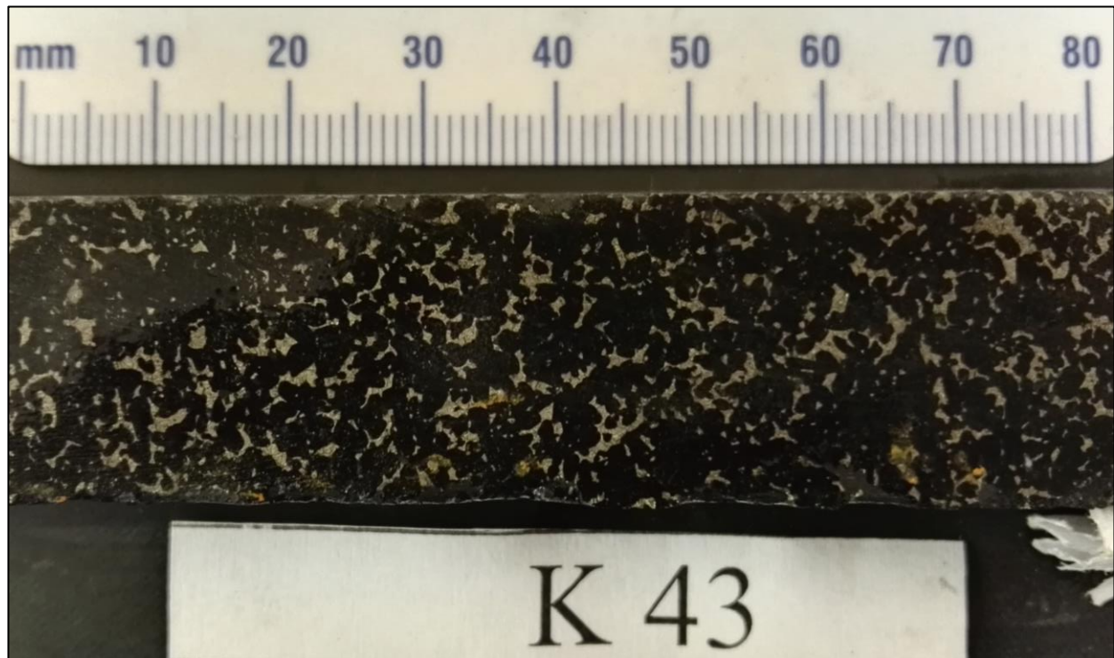
Figure 3.6: Serpentinised harzburgite with net-textured pyrrhotite and specks of interstitially disseminated chalcopyrite.
