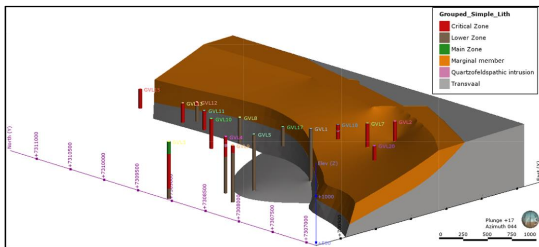
Figure 5.16: View of eastern section exposing the morphology and orientation of the marginal member and underlying Transvaal unit.
