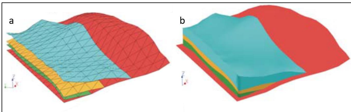
Figure 5.4: Simplistic generic depiction of model components. (a) Wireframes or surfaces which are representative of the lithological or stratigraphic boundaries which are then used to define (b) the lithological or stratigraphic volumes. Modified after Ross et al. (2007).
