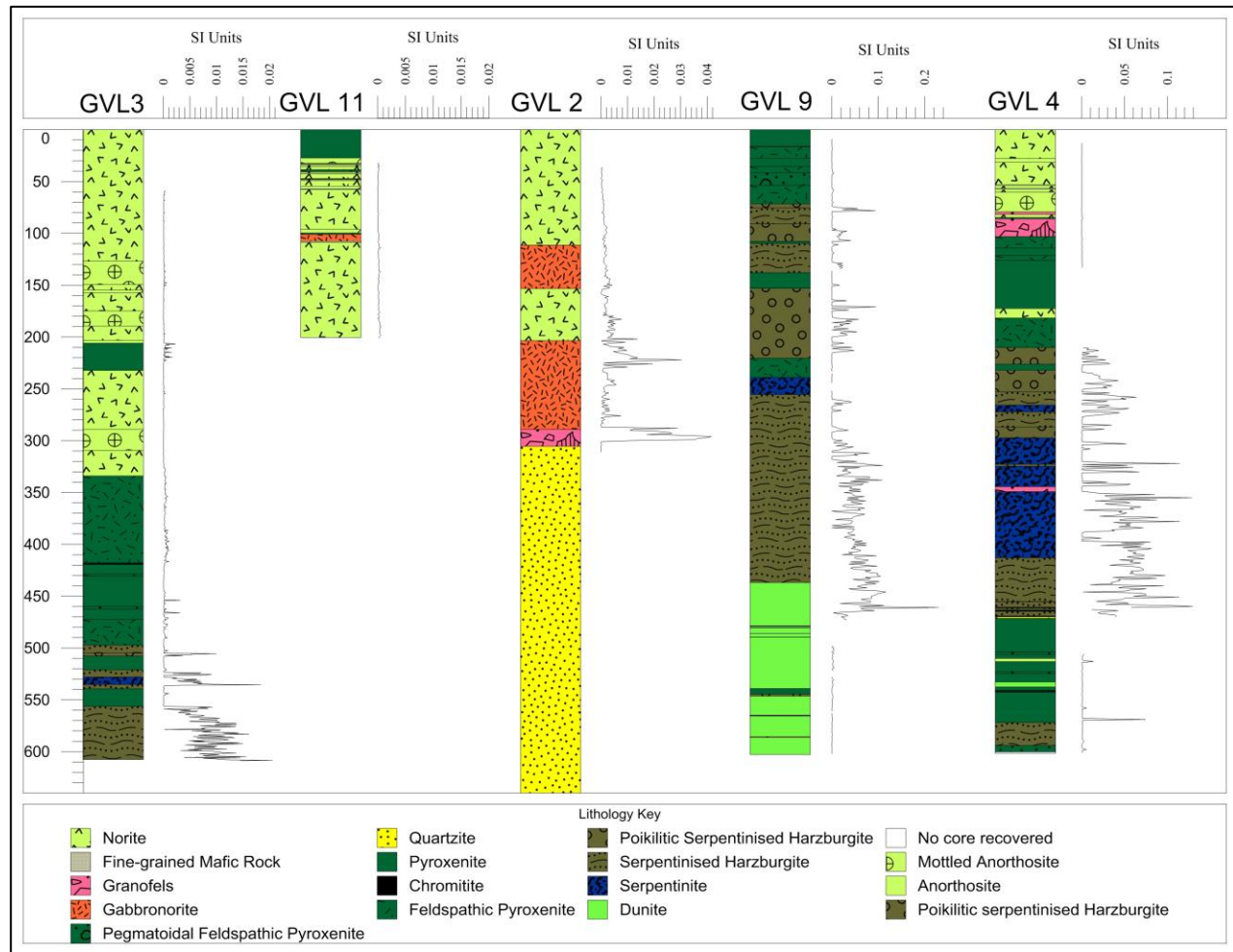
Figure 3.24: Magnetic susceptibility profiles (SI units) of selected holes GVL 3, GVL 11, GVL 2, GVL 9 and GVL 4 plotted against simplified geological logs.
