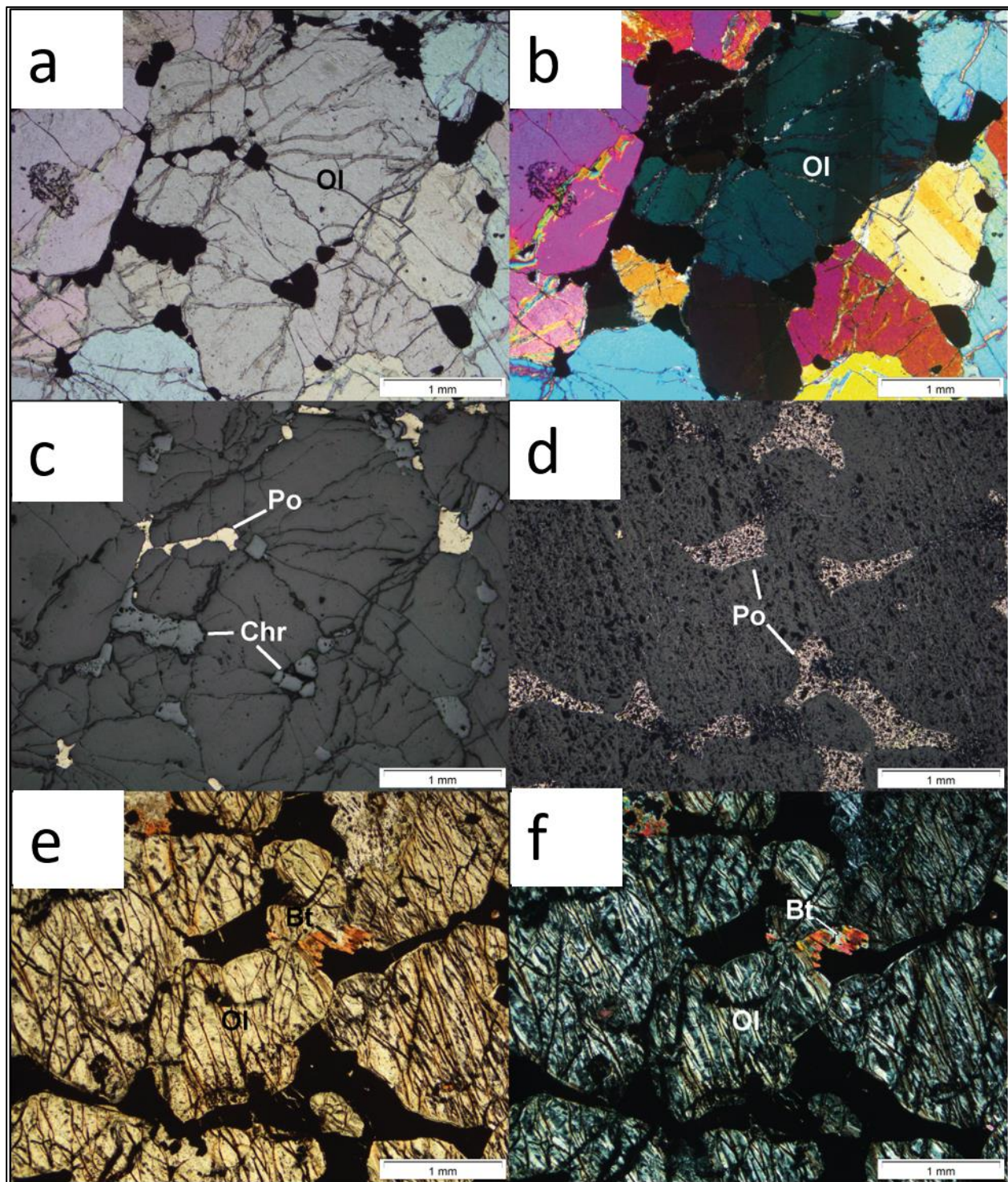
Figure 3.15: Photomicrographs of a serpentinised dunite in both transmitted and reflected light. (a) Dunite in PPL with olivine and interstitially disseminated opaques. (b) Dunite in XPL with annealed olivine crystals displaying kink banding. (c) Dunite in RL with interstitially disseminated pyrrhotite and chromite (d) Serpentinised dunite in RL displaying interstitially disseminated blebs of pyrrhotite. (e) Serpentinised dunite in PPL with altered olivine and secondary biotite associated with pyrrhotite (opaque). (f) Serpentinised dunite in XPL displaying serpentinised and highly fractured olivine grains with secondary biotite associated with pyrrhotite (Opaque).
