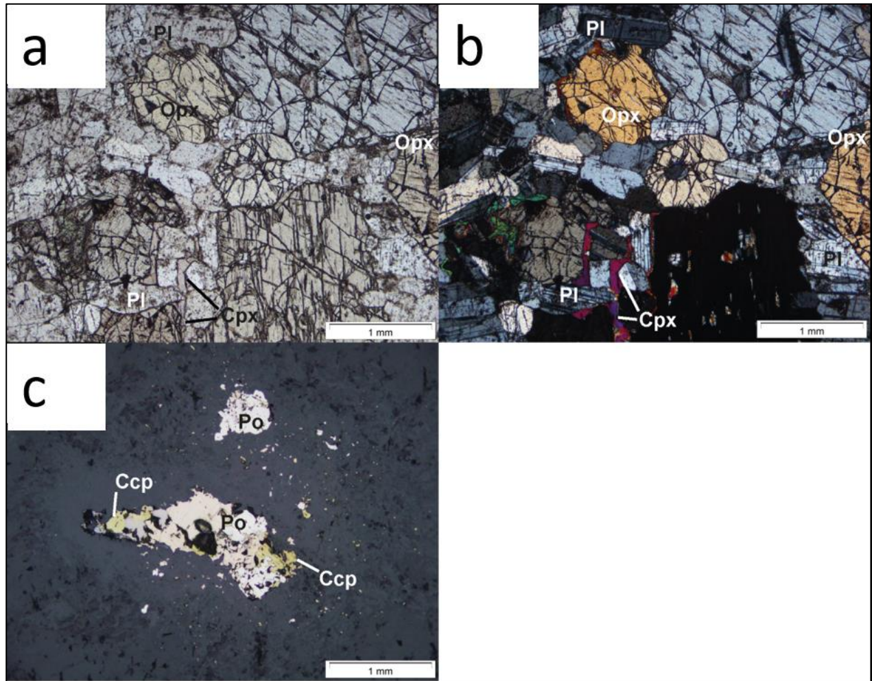
Figure 3.18: Photomicrographs of a norite in both transmitted and reflected light. (a) Highly fractured norite dominated by orthopyroxene in PPL. (b) Norite dominated by orthopyroxene, plagioclase with minor intercumulus clinopyroxene in XPL. (c) Blebby pyrrhotite with associated chalcopyrite and lesser interstitially disseminated chalcopyrite and pyrite specks.
