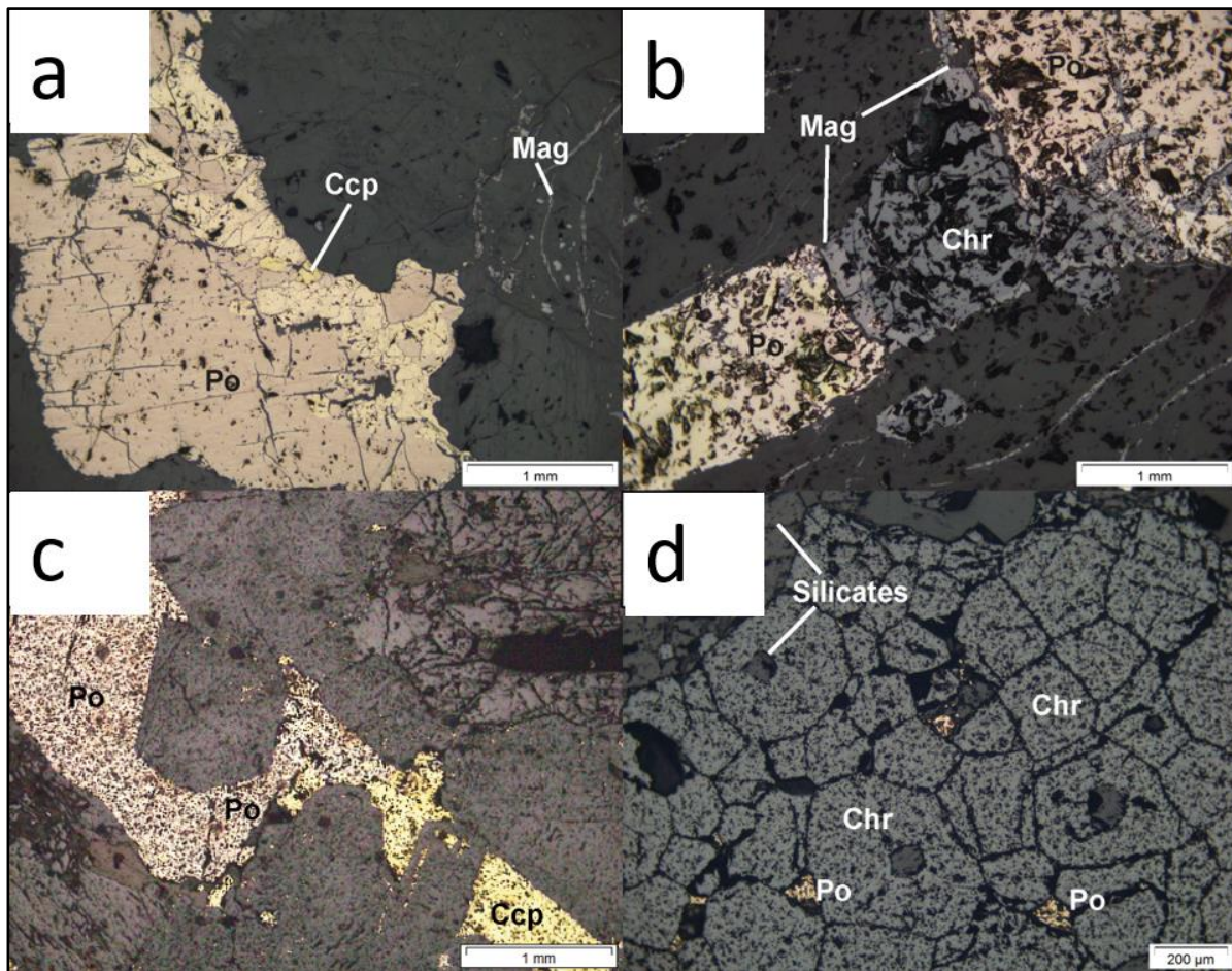
Figure 3.22: (a) A large pyrrhotite with marginal chalcopyrite. Veinlets and specks of secondary magnetite. (b) Pyrrhotite, chalcopyrite, magnetite and chromite. (c) interstitial pyrrhotite rimmed partially by chalcopyrite. (d) Chromitite grains displaying atoll texture with specks of interstitially disseminated pyrrhotite.
