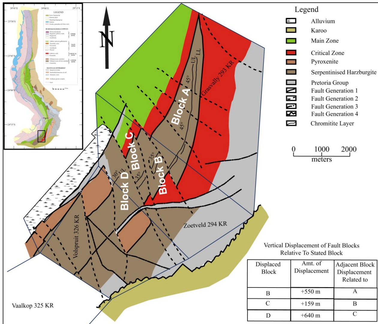
Figure 2.10: Generalised geological map of the Grasvally-Zoetveld-Volspruit area showing the four generations of faults, modified after Hulbert (1983). Map of general geology of the northern limb after Ashwal et al. (2005).
