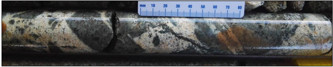
Figure 3.13: Pyroxenite brecciated by quartzofeldspathic veins.
