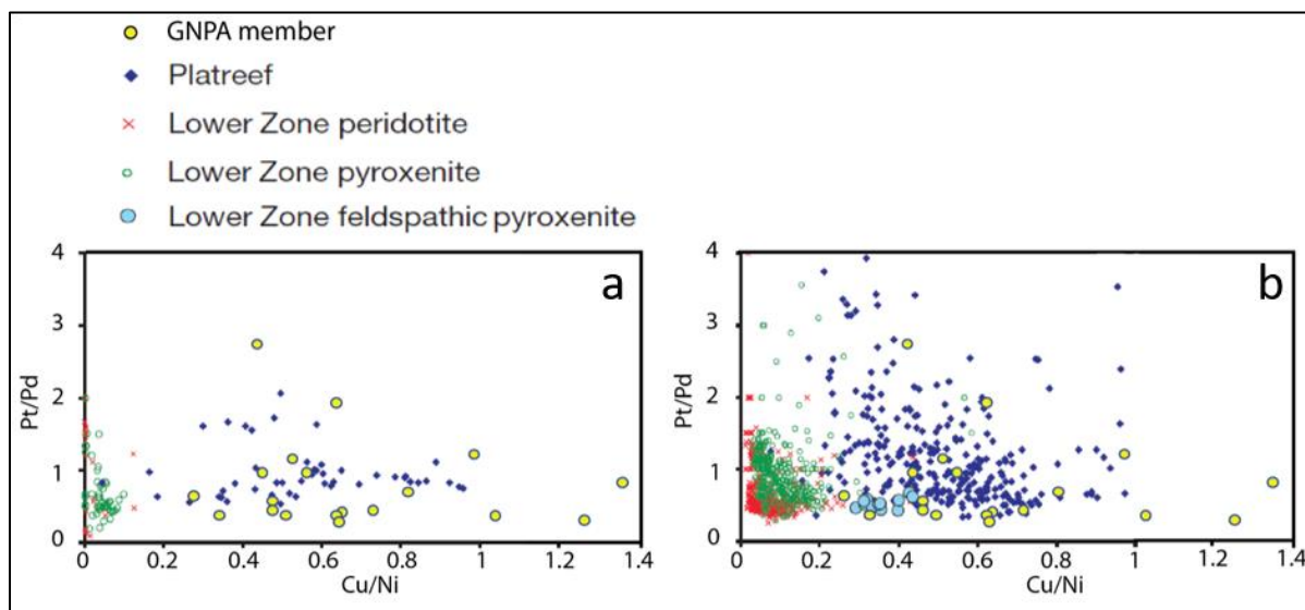
Figure 4.18: Binary variation diagrams of Cu/Ni, and Pt/Pd ratios, showing data for the GNPA member pyroxenite from this study, plotted against Platreef and the Lower Zone peridotite, pyroxenite, and feldspathic pyroxenite after Yudovskaya (2013). Samples plotted against (a) Sandsloot samples and (b) Turfspruit samples showing the samples of the GNPA member are generally palladium dominated with a similar distribution to the Platreef samples of Sandsloot.
