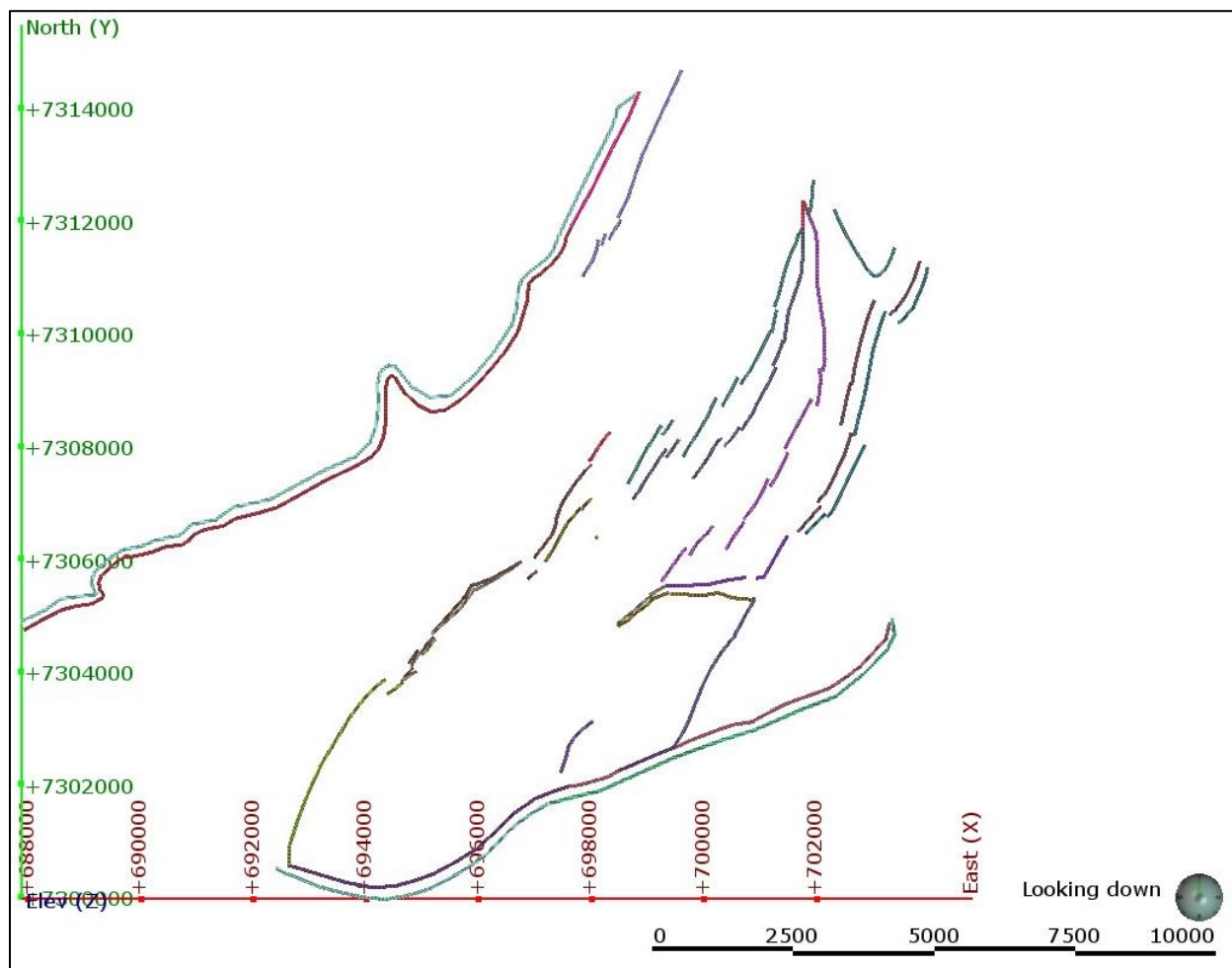
Figure 5.5: Digitised contacts between stratigraphic units. Stratigraphic contacts were obtained from Hulbert (1983).
