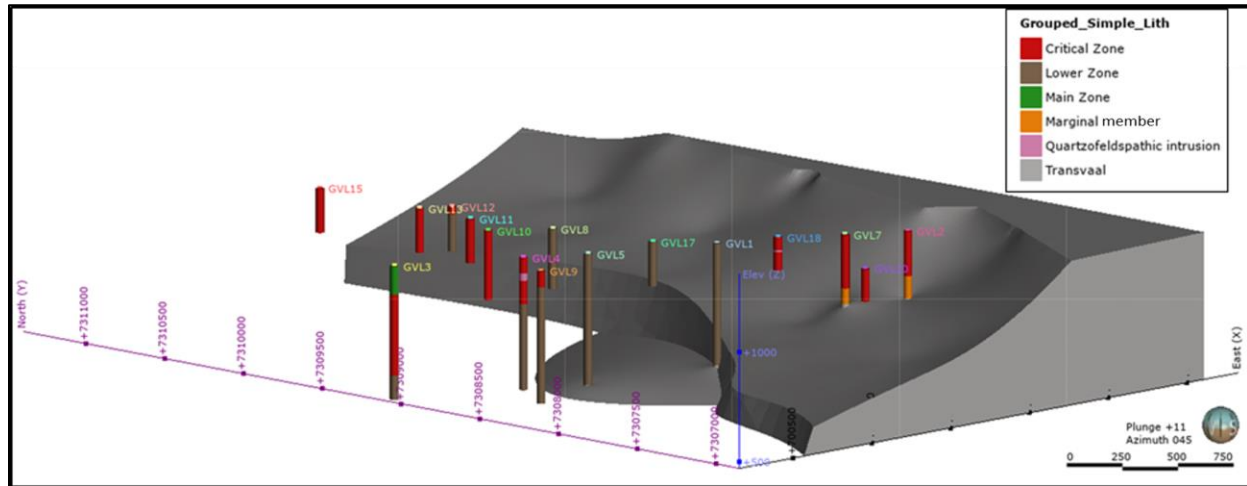
Figure 5.13: Orthographic view of Transvaal volume from a south-west perspective.
