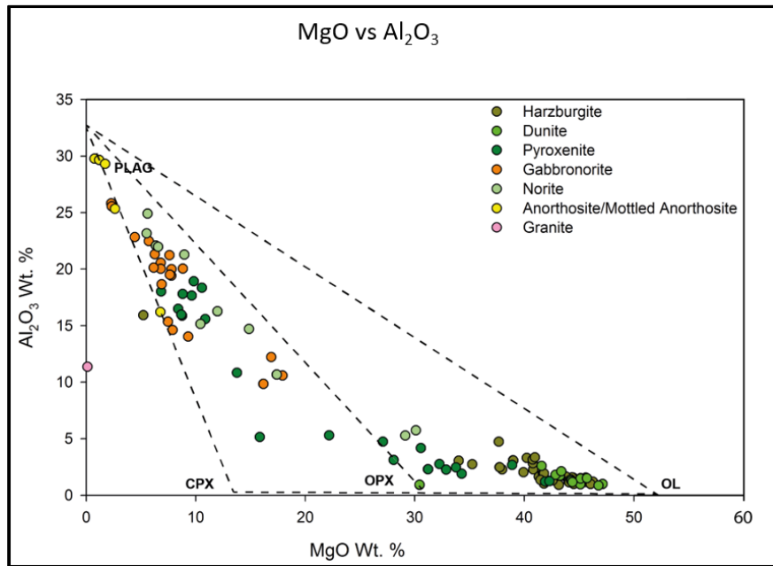
Figure 4.3: Classification of samples K-1 to K-133 on a diagram showing MgO wt % against Al 2 O 3 wt %. The classification parameters have been adopted from Hulbert (1983). Samples have been coloured according to the hand sample classification.
