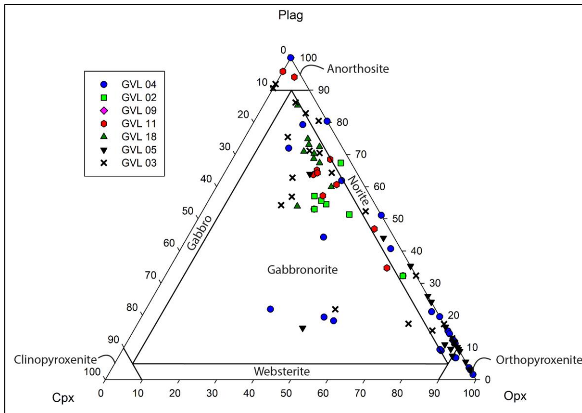
Figure 4.1: Classification and nomenclature of gabbroic rocks based on the CIPW normative proportions calculated from the modal geochemistry of plagioclase (Plag), clinopyroxene (Cpx) and orthopyroxene (Opx) (after Streckeisen, 1976).
