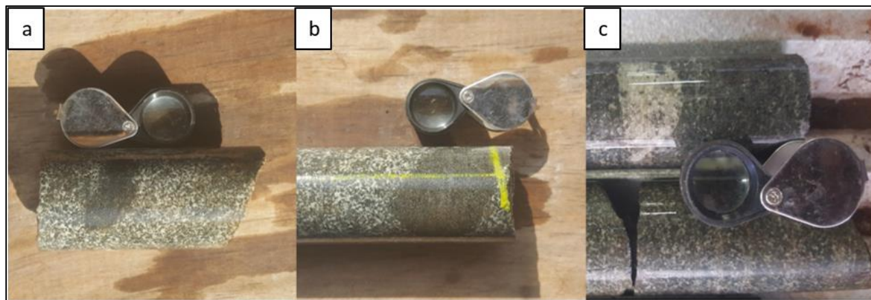
Figure 3.10: various xenoliths observed within the norites and gabbronorites in core GVL 2. (a) Chromitite pod with associated sulphides within gabbronorite. (b) Pyroxenite xenolith with interstitially disseminated sulphide specks. (c) Anorthosite xenolith within gabbronorite. All Samples are intersected in GVL 2.
