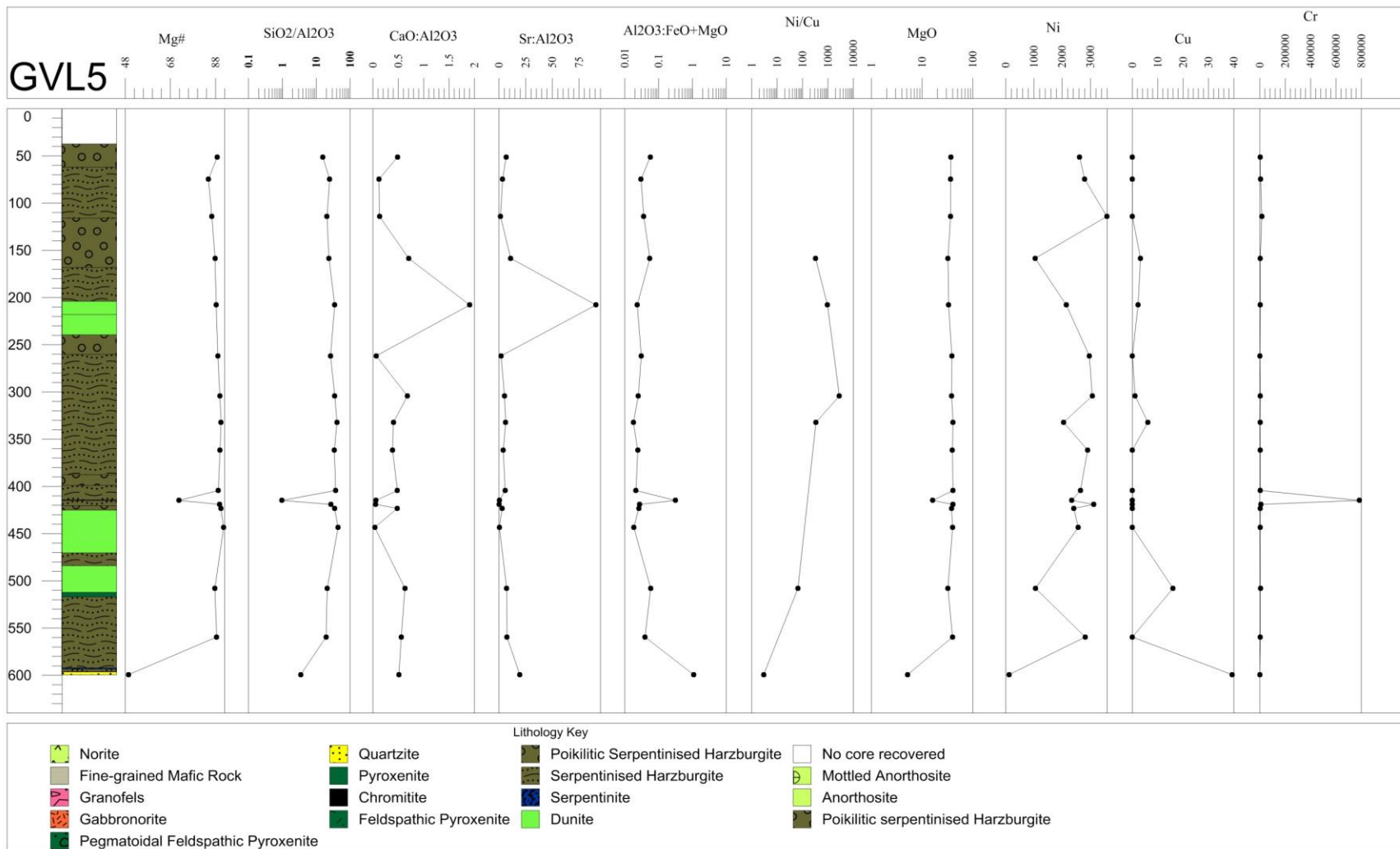
Figure 4.11: Variations of the whole-rock Mg#, major and trace element ratios and trace element contents through borehole GVL 5. Mg# displays little to no variation up section and is indicative of a lack of fractionation occurring within this package but perhaps a constant replenishment of magma.
