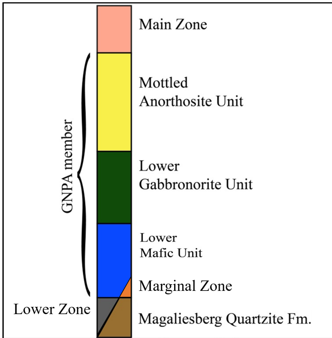
Figure 2.6: Stratigraphic column of the Rooipoort-Grasvally area. Adapted from Maier et al. (2008).
