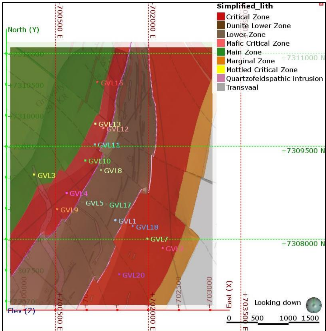
Figure 5.3: Plan view of modelled area with boreholes incorporated. Draped map adapted from Hulbert (1983).
