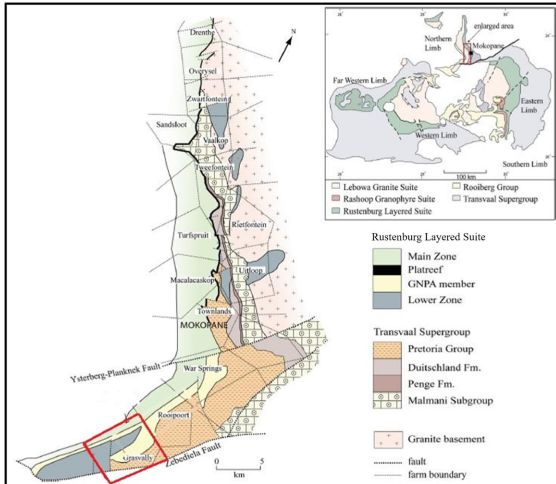
Figure 1.2: Geological map of the northern limb of the Rustenburg Layered Suite (RLS), showing the location of the research area on the farm of Grasvally. Adapted from Smith et al. (2014).
