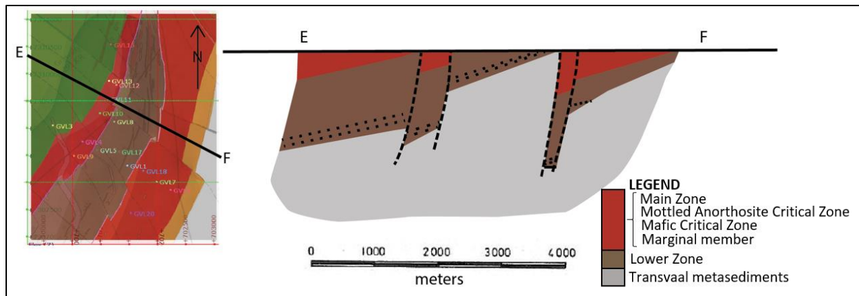
Figure 6.3: Interpretation of the footwall geometry through the use of gravity data taken along cross section E-F showing the complex nature of footwall lithologies (Barrett et al. , 1978). The marginal member, Critical Zone and Main Zone have been represented within this diagram as one unit (seen in red) after Barrett et al. (1978). The dotted lines represent the chromitite layers within the Lower Zone.
