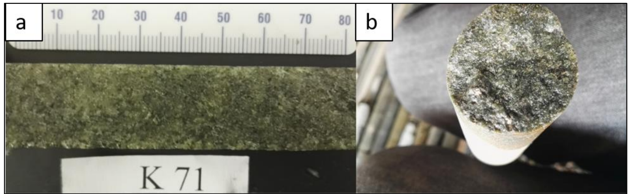
Figure 3.5: Fresh dunite with disseminated chromite intersected in GVL 9 (a) in quarter core and (b) in full core.
