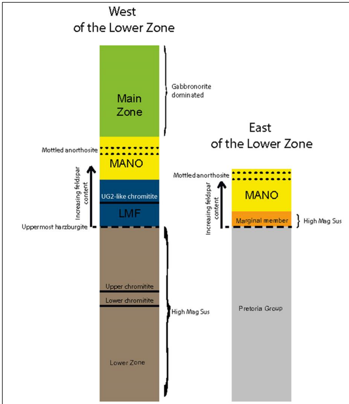
Figure 6.4: Schematic diagram of marker horizons identified, showing the mottled anorthosite marker within the MANO, the chromitite within the LMF, the marginal member with a distinct magnetic susceptibility, the Lower Zone - LMF boundary which is marked by an increase in feldspar, and the chromitite layers within the Lower Zone. These can be correlated between boreholes.
