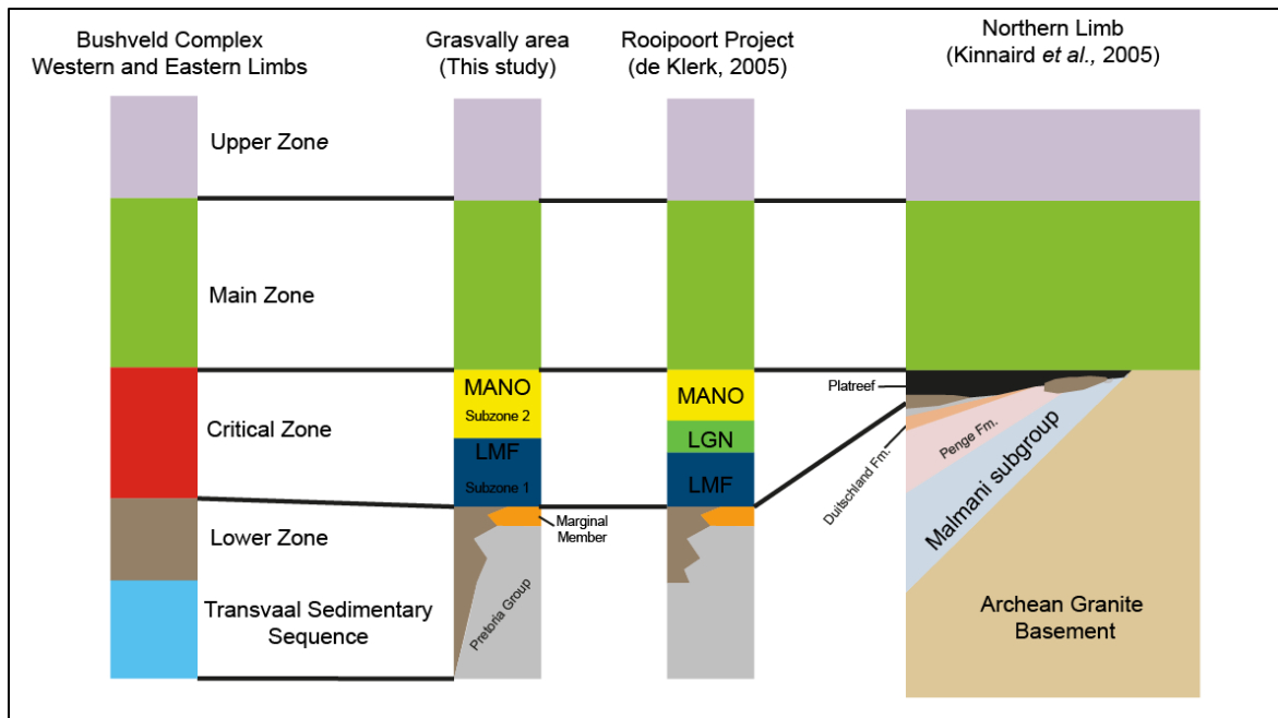
Figure 6.1: A schematic diagram displaying the differences and similarities in stratigraphy between the eastern and western limbs of the Bushveld Complex, the Grasvally area, the Rooipoort Project (de Klerk, 2005) and the generalised northern limb stratigraphy (Modified from Kinnaird et al. (2005)).
