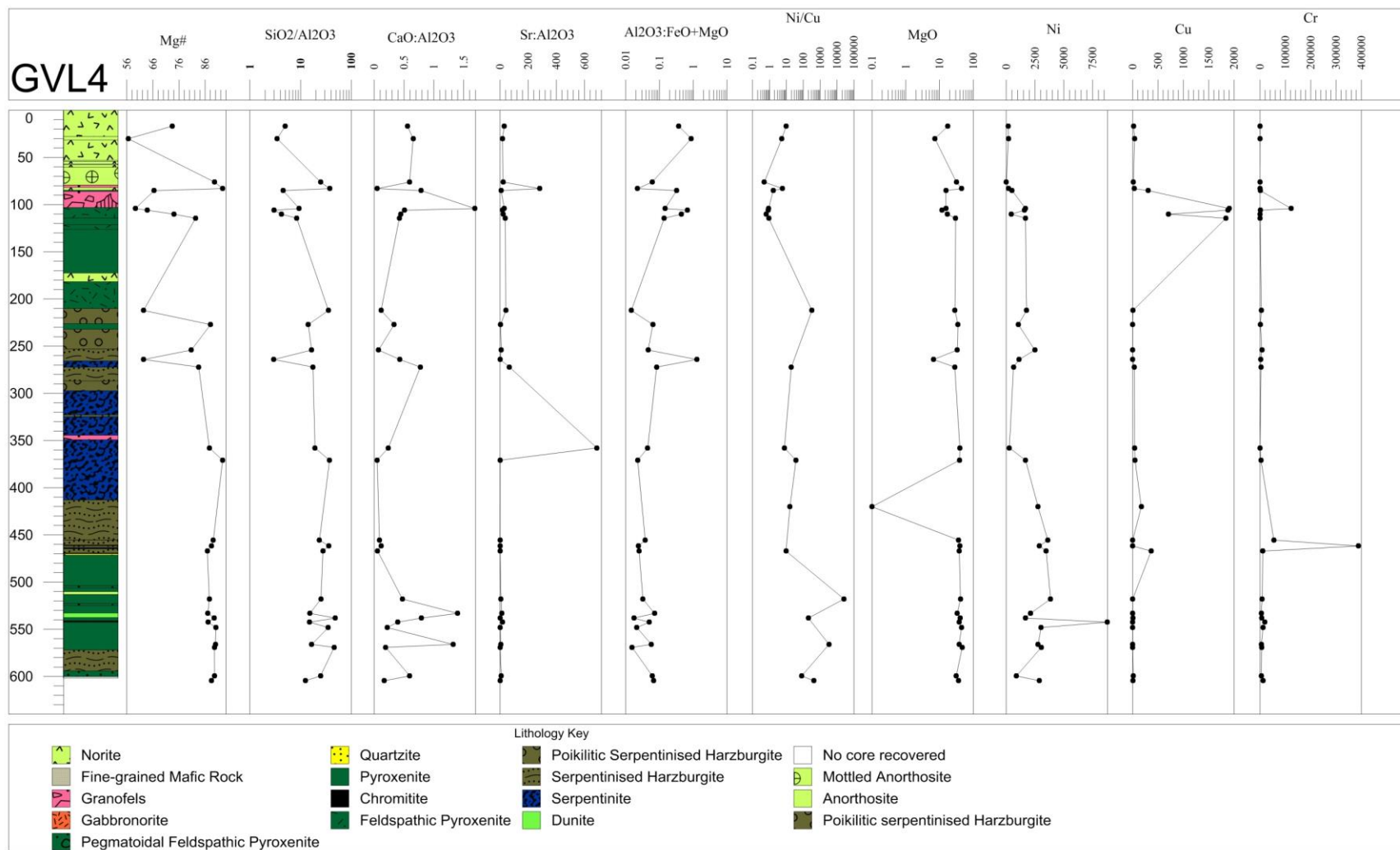
Figure 4.9: Variations of the whole-rock Mg#, major and trace element ratios and trace element contents through borehole GVL 4.
