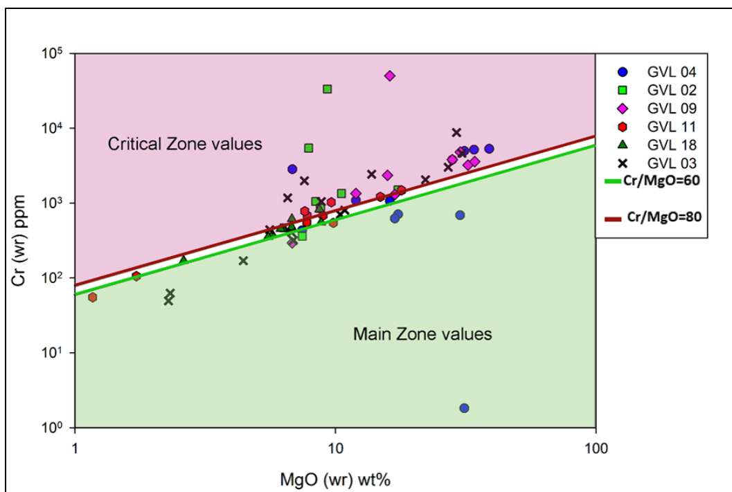
Figure 4.15: Whole rock Cr (ppm) and MgO (wt. %) for samples from boreholes GVL 2, GVL 3, GVL 4, GVL 9, GVL 11 and GVL 18 with the exclusion of Lower Zone samples. The classification fields are defined by the Cr/MgO ratios of 80 and 60 for the Critical Zone and Main Zone respectively (Seabrook et al. , 2005).
