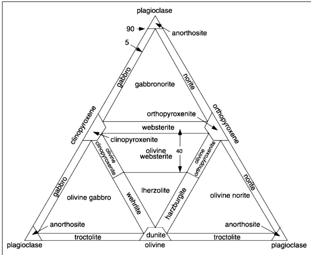
Figure 3.2: IUGS classification scheme for mafic rocks. The Grasvalley rock types fall mainly in the orthopyroxenite, olivine orthopyroxenite and harzburgite fields (le Bas and Streckeisen, 1991).
