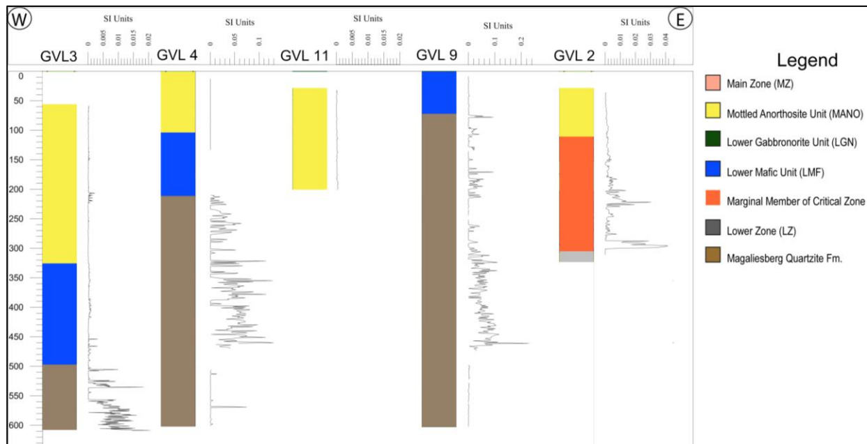
Figure 3.28: Magnetic susceptibility signatures of boreholes GVL 3, 4, 11, 9, and 2 correlated with possible stratigraphic units. Stratigraphic units adapted from Hulbert (1983) and (de Klerk, 2005).
