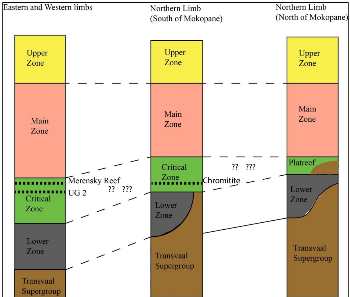
Figure 2.4: Differences in magmatic stratigraphy of Critical Zone, and its equivalents across the Bushveld Complex. Adapted from Smith et al. (2011).
