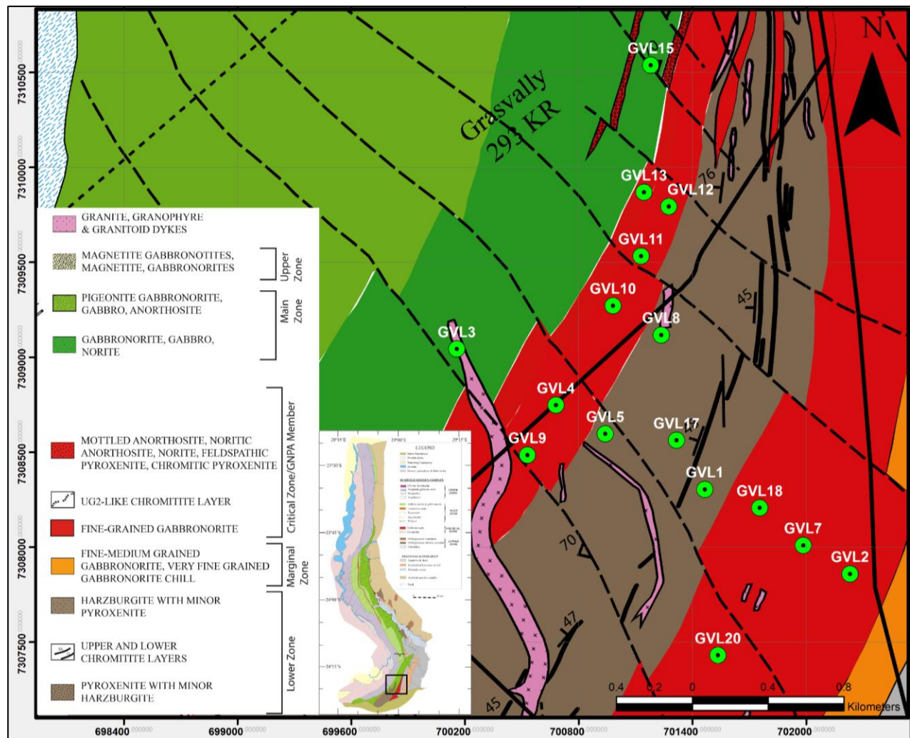
Figure 3.1: Borehole distribution on the farm Grasvally drilled by Samancor in 2004. Map modified after Hulbert (1983).
