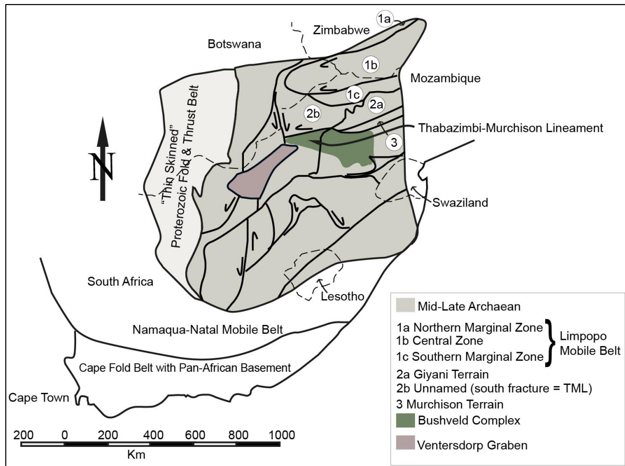
Figure 2.7: Granite-greenstone terrains of the Kaapvaal Craton displaying outline of the Bushveld Complex and Thabazimbi-Murchison Lineament modified after de Wit and Hart (1993).
