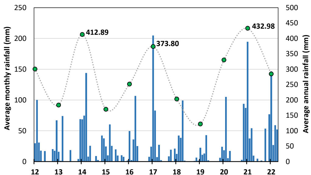
Figure 4.1. Average monthly (bars) and annual (dashed line) rainfall at Tswalu Kalahari Reserve over the last 10 years (2012–2022). The highest rainfall was recorded in 2014, 2017 and 2021 (Annual rainfall, in mm, provided in bold text).
