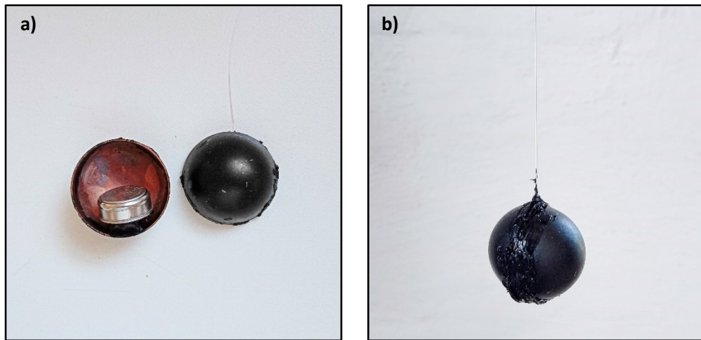
Figure 3.1: a) The inside of a mini black globe during construction, and b) The finished mini black globe once sealed with silicone.
