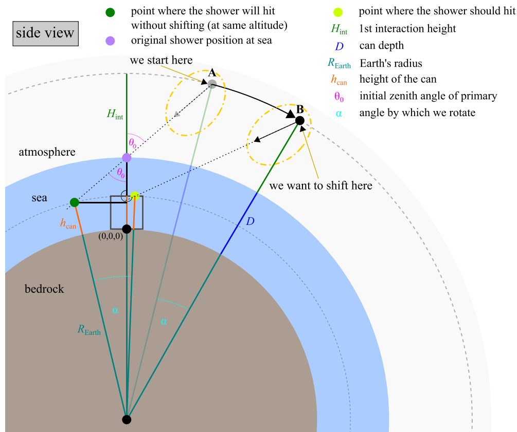
Fig. A.12. Sketch of the geometry of shower reorientation, shown from the side.
