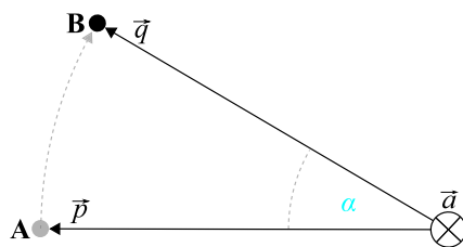
Fig. A.13. Sketch of the vector \vec{p} rotated onto the vector \vec{q} by an angle \alpha around the axis of rotation defined by the orthogonal vector \vec{a} .
