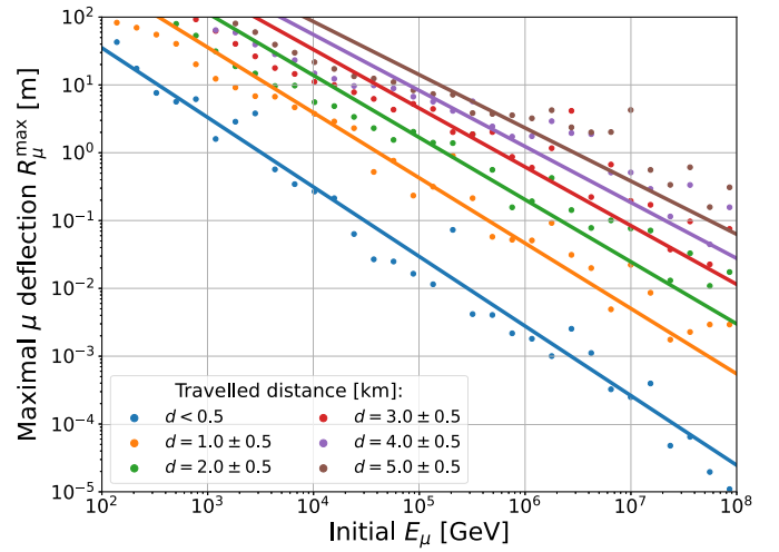
Fig. A.9. Maximal lateral muon deflections fitted as a function of E_\mu . The fitting function is R(E_\mu) = 10^{a_d \cdot \log_{10}(E_\mu) + b_d} .
