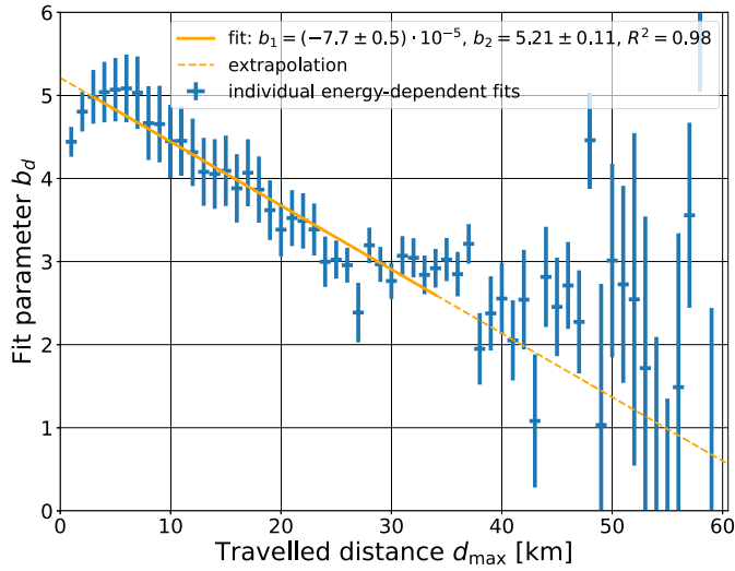
Fig. A.11. Dependence of the energy-dependent fit parameter of the maximal lateral muon deflection b_d on the distance travelled. The fitting function is b_d = b_1 \cdot \frac{d_{\max}}{m} + b_2 and R^2 is the coefficient of determination.
