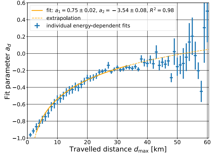
Fig. A.10. Dependence of the energy-dependent fit parameter of the maximal lateral muon deflection a_d on the distance travelled. The fitting function is a_d = a_1 \cdot \log_{10}(\frac{d_{\max}}{m}) + a_2 and R^2 is the coefficient of determination.
