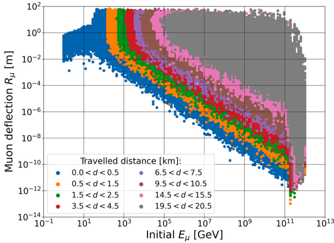
Fig. A.8. Lateral deflection of muons R_\mu as a function of their initial energy E_\mu and distance d travelled in seawater.
