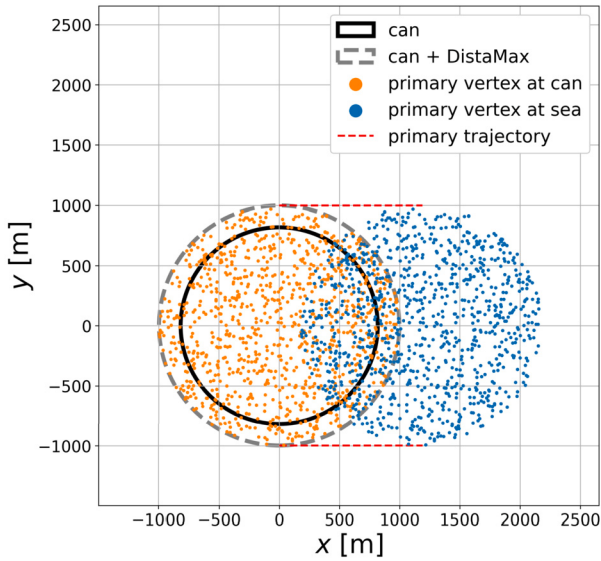
Fig. 3. Sketch of the projection of the can top cap area onto the sea surface (after increasing it by the appropriate DistaMax projection onto the horizontal direction) in the top view.
