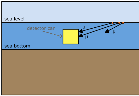
Fig. 1. Sketch of the new geometry in gSeaGen, with an example of a multi-muon CORSIKA event, with two muons reaching the can and one stopping in seawater. The curvature of the Earth has been neglected in this drawing, however it is explicitly handled by the gSeaGen code, as detailed in Sec. Appendix A.2.3. (For interpretation of the colours in the figure(s), the reader is referred to the web version of this article.)
