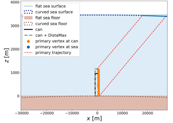
Fig. 4. Sketch of the projection of the can side area onto the sea surface (after increasing it by the appropriate DistaMax projection onto the vertical direction) in the side view.
