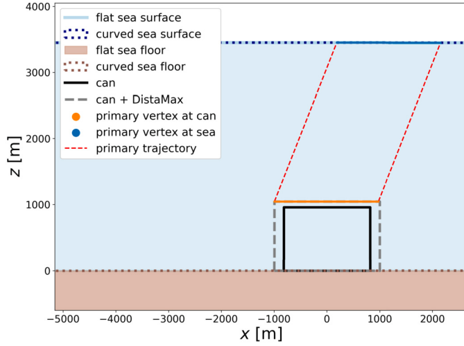
Fig. 2. Sketch of the projection of the can top cap area onto the sea surface (after increasing it by the appropriate DistaMax projection onto the horizontal direction) in the side view.
