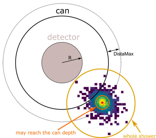
Fig. 7. Top view of the geometry of shooting the shower at the can. The drawing assumes a perfectly vertical shower for simplicity; however, an actual histogram of an EeV proton shower simulated with CORSIKA (without thinning) from a KM3NeT CORSIKA simulation has been used, showing the muon density at the sea level. The yellow and orange circles are sketched to illustrate the qualitative effect of muon selection by range, which is effectively a cut on muon energy. The more energetic muons are typically closer to the shower axis since they are harder to deflect. This leads to the narrowing of the shower when the muons with insufficient range are discarded.
