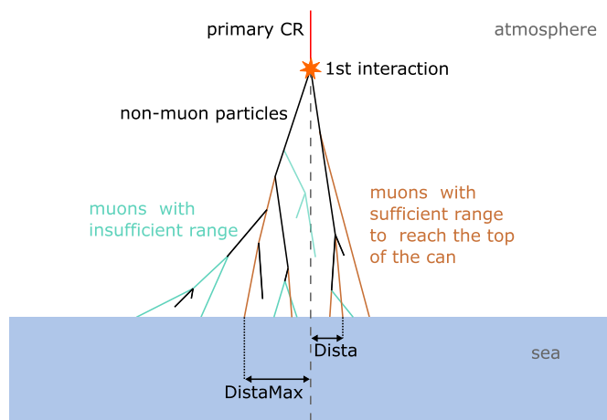
Fig. 6. Sketch illustrating the meaning of DistaMax using the example of a vertical shower. The value of DistaMax is always evaluated for muon positions at the sea surface.
