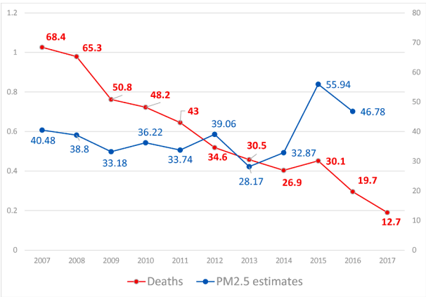
Fig. 3. Annual mean PM 2.5 (µg/m 3 ) levels and deaths rate per 1000 live births in the Navrongo Heath and Demographic Surveillance Site 2007–2017.
