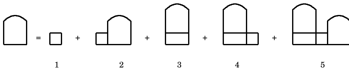
Figure 1: Wasp-waist decomposition of bargraphs.
