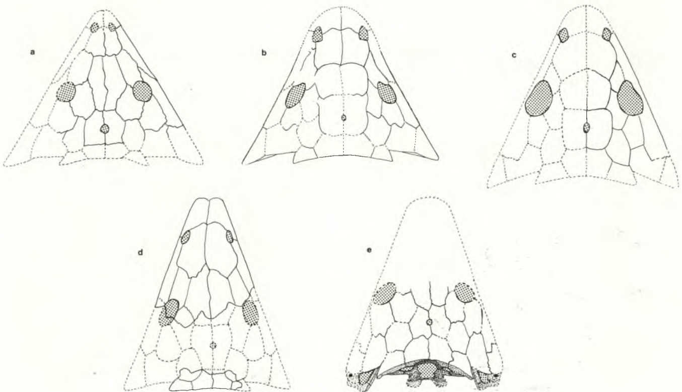
Figure 8. Restorations of dorsal views of rhytidosteid skulls (not to scale): a, Pneumatostega potamia ; b, Deltasaurus kimberleyensis (after Cosgriff, 1965); c, Deltasaurus pustulatus (after Cosgriff, 1965); d, Rhytidosteus capensis (after Cosgriff, 1965); e, Peltostega erici (after Nilsson, 1946).
