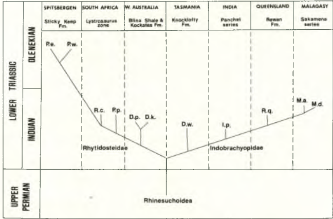
Figure 13. Phylogeny of the Rhytidosteidae plotted against stratigraphic and geographic data. Note: D. kimberleyensis is also found in the Knocklofty Formation of Tasmania.
