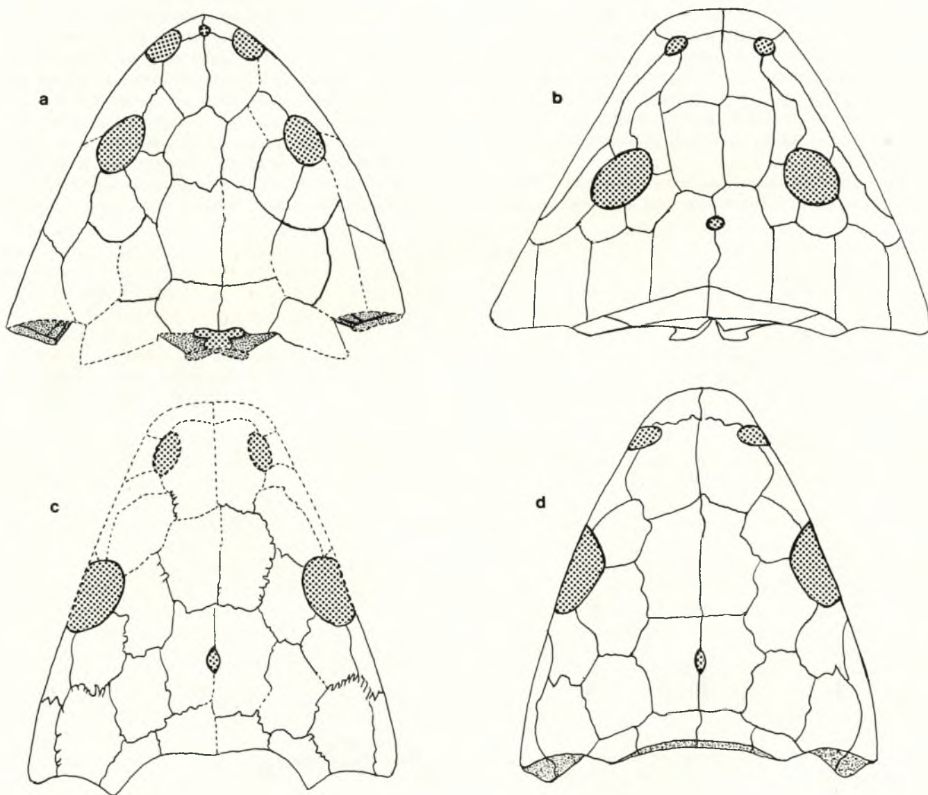
Figure 9. Restorations of dorsal views of indobrachyopid skulls (not to scale): a, Derwentia warreni (after Cosgriff, 1974); b, Indobrachyops panchetensis (after Von Huene and Sahni, 1958); c, Mahavisaurus dentatus (after Lehman, 1966); d, Mahavisaurus (Lyrosaurus) australis (after Lehman, 1966).
