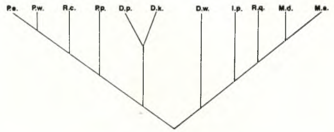
Figure 12. Cladistic relationships among the Rhytidosteoidea, based on computer processed morphologic data.
