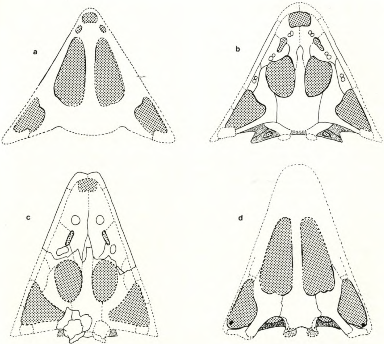
Figure 10. Restorations of palatal views of rhytidosteid skulls (not to scale): a, Pneumatostega potamia ; b, Deltasaurus kimberleyensis (after Cosgriff, 1965); c, Rhytidosteus capensis (after Cosgriff, 1965); d, Peltostega erici (after Nilsson, 1946).
