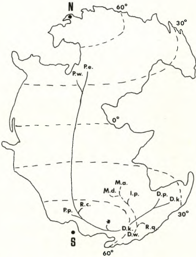
Figure 14. Proposed dispersal pattern of the Rhytidosteidae (solid line) and Indobrachiopidae (dashed line) across the Pangaea continent during the lower Triassic. Note, the asterisk indicates the new undescribed rhytidosteid from Antarctica. Continental outlines, paleolatitudes and polar positions are from Smith and Briden (1977, map 52).
