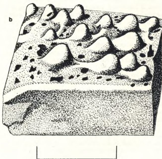
Figure 7. Pneumatostega potamia , n.g. and sp., magnified (scale: 1 cm) piece from labial side of right angular bone of paratype, SAM 11188, to show sculpture details and vascularisation: a, section view, showing vascularisation; b, surface view, showing sculpture nodes and vessel foramina opening on to surface.
