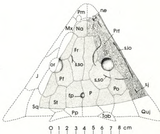
Figure 1. Pneumatostega potamia , n.g. and sp., reconstruction of dorsal surface of skull, based on holotype, BPI F.no.981. Shaded area indicates portion of skull roof impression retained on the specimen. Only right lateral bones of the impression have sculpture pattern indicated in this drawing although sculpture extends over the entire impression. Abbreviations for Figure 1 and following figures: a.p.v., anterior palatal vacuity; dia, diapophysis; fa.cl., clavicular facet; fo.st., subtemporal fossa; f.p., parietal foramen; Fr, frontal; Ic, intercentrum; i.p.v., interpterygoid vacuity; J, jugal; Mx, maxillary; Na, nasal; n.a., neural arch; n.e., external naris; n.i., internal naris; or, orbit; P, parietal; par, parapophysis; Pc, pleurocentrum; p.c., cultriform process; p.cl., cleithral process; Pf, postfrontal; Pm, premaxillary; Po, postorbital; Pp, postparietal; Prf, prefrontal; Ps, parasphenoid; Pt, pterygoid; Qu, quadrate; Quj, quadratojugal; S.io., infraorbital groove; s.j., jugal groove; Sq, squamosal; s.s.o., supraorbital groove; St, supratemporal; Tab, tabular; z.a., anterior zygapophysis.
