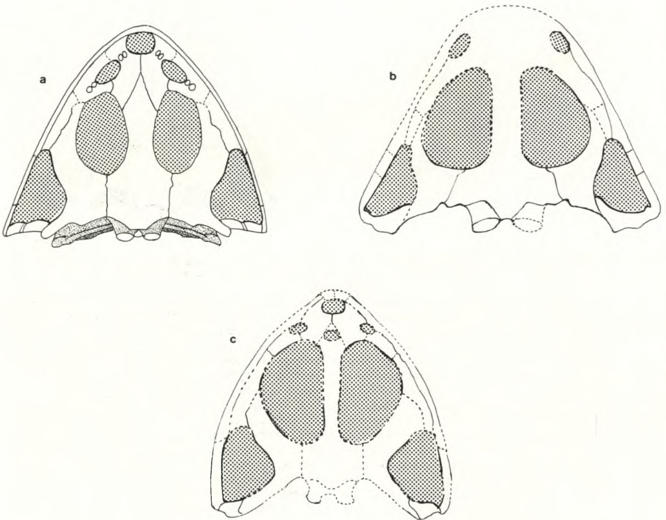
Figure 11. Restorations of palatal views of indobrachyopid skulls (not to scale): a, Derwentia warreni (after Cosgriff, 1974); b, Indobrachyops panchetensis (after Von Huene and Sahni, 1958); c, Rewana quadricuneata (after Howie, 1972).
