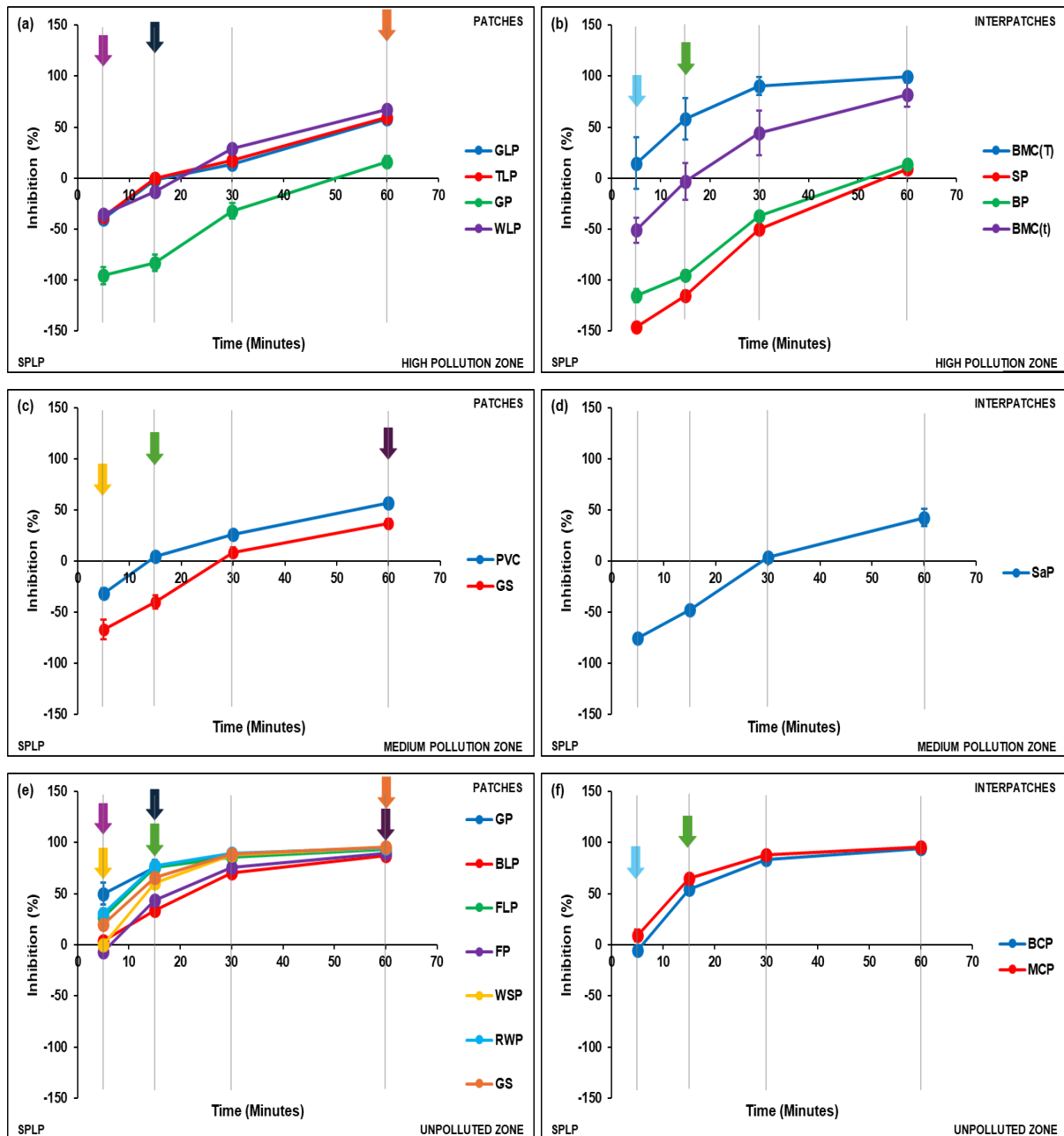
Figure 3.6: Mean ( \pm standard error) percentage inhibition of Aliivibrio fischeri bioluminescence after exposure to SPLP solutions of patch and interpatch soils from the high, medium, and unpolluted zones. Lines along each graph represent the time points when bioluminescence readings were taken: 5, 15, 30, and 60 minutes . Graphs that share arrows of a similar colour are significantly different to each other at that time point. A red star indicates a significant difference between patch and interpatch response at that time point. Means were determined from triplicate samples for each patch and interpatch type.
