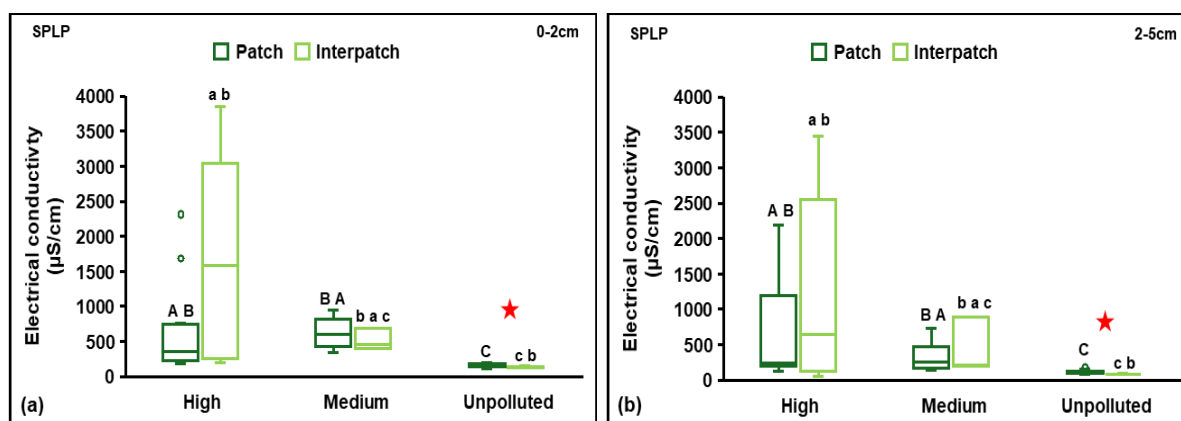
Figure 2.15: Electrical conductivity values of SPLP solutions for soil samples from patches and interpatches along the high r and medium s in 2021, and unpolluted t zone in 2023 at depths of (a) 0-2 cm and (b) 2-5 cm. Patch soil samples labelled with differing upper-case letters were found to be significantly different along each site. Interpatch soil samples labelled with differing lower-case letters were significantly different along each site based on a post hoc Dunn's test ( p < 0.05 ). A red star indicates a significant difference between the patches and interpatches.
