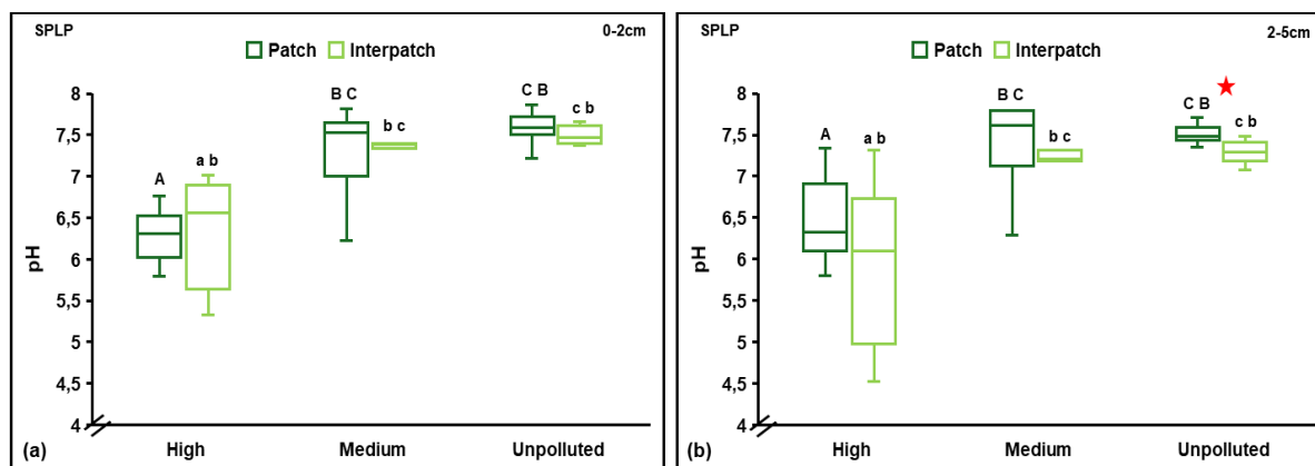
Figure 2.13: pH values of SPLP leachate solutions for soil samples collected from patches and interpatches along the high l and medium m in 2021, and unpolluted n in 2023 at depths of (a) 0-2 cm and (b) 2-5 cm. Bars labelled with differing upper-case letters were found to be significantly different from each other, based on a post hoc Dunn's test ( p < 0.05 ). A red star indicates a significant difference between patch and interpatch soils.
