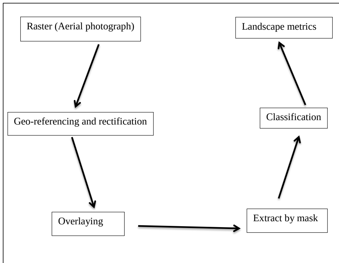
Figure 2: Flow chart showing all steps involved in processing aerial photographs
