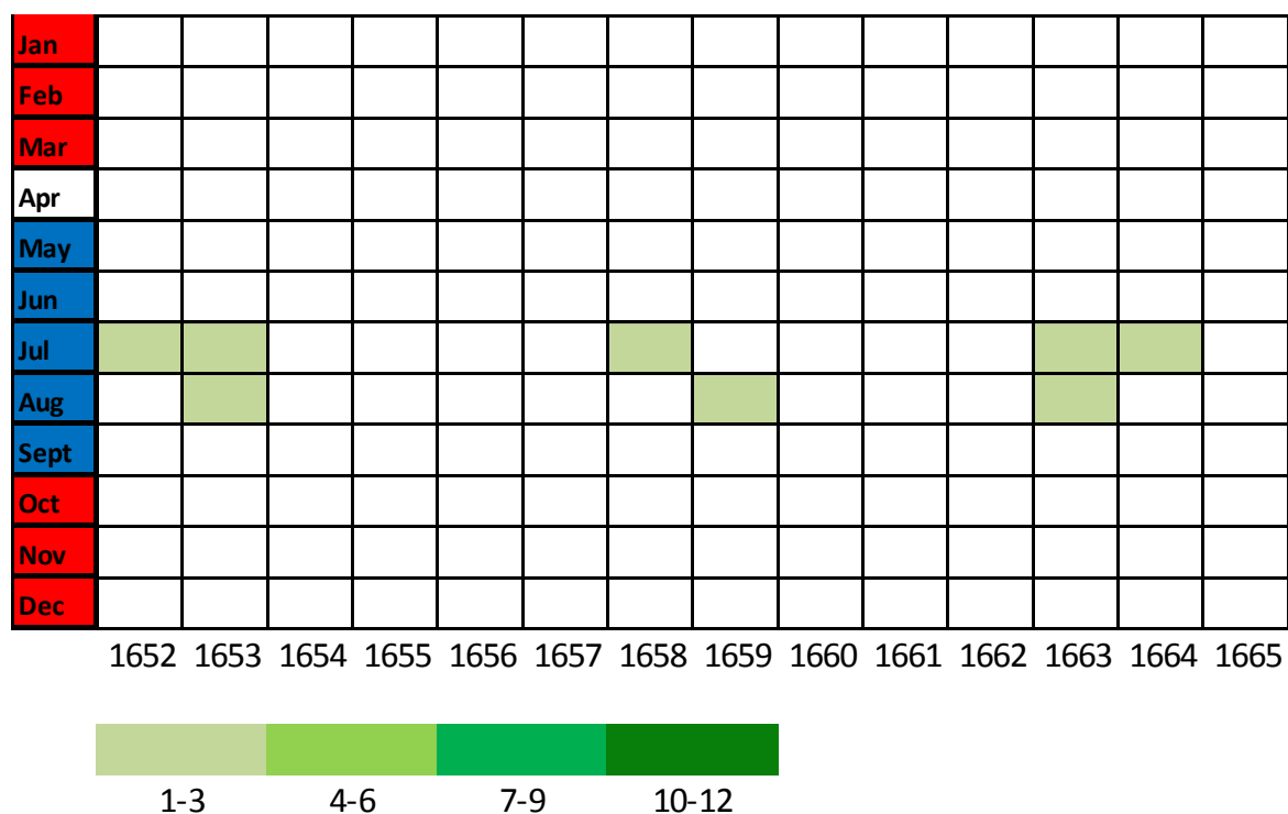
Figure 5.18: Snow, frost and ice grid for the historical period: 1652-1665
