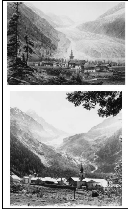
Figure 3.2: The first image is an etching produced between 1850 and 1860 of the Argentiene glacier in the French Alps and the second image is a photograph captured at a similar vantage point in 1966 showing the glacial retreat, Mann (2002).
