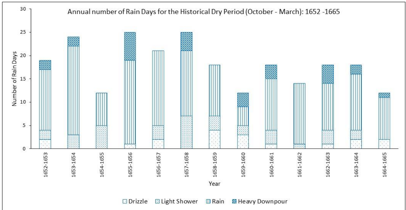
Figure 5.3: Annual dry periods according to rainfall intensity for the period 1652-1665
