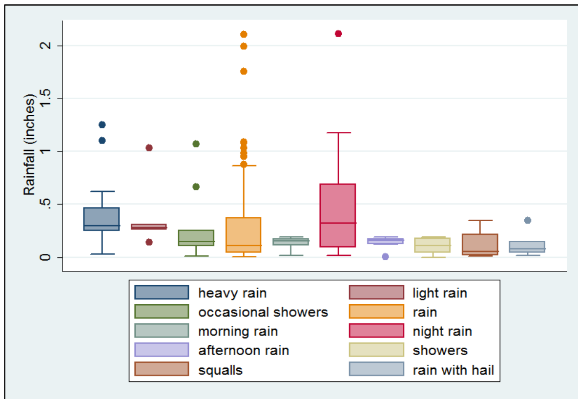
Figure 5.14: Box and whisker plots representing variance of rainfall categories for the Royal Observatory data: 1843-1847
