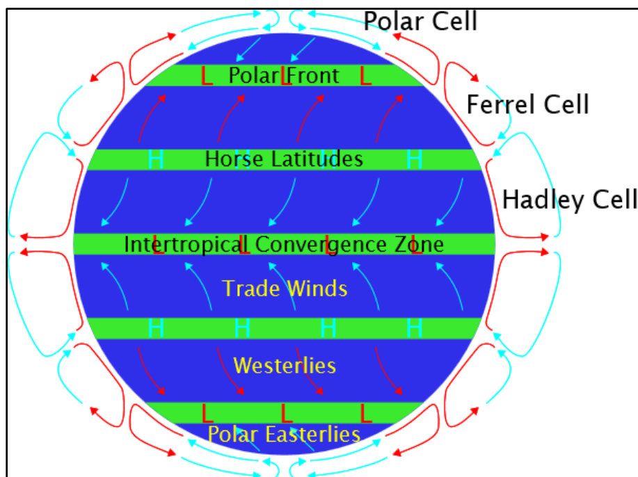
Figure 5.11: The Global Atmospheric Circulation and resultant wind bands (Windrum, 2004)
