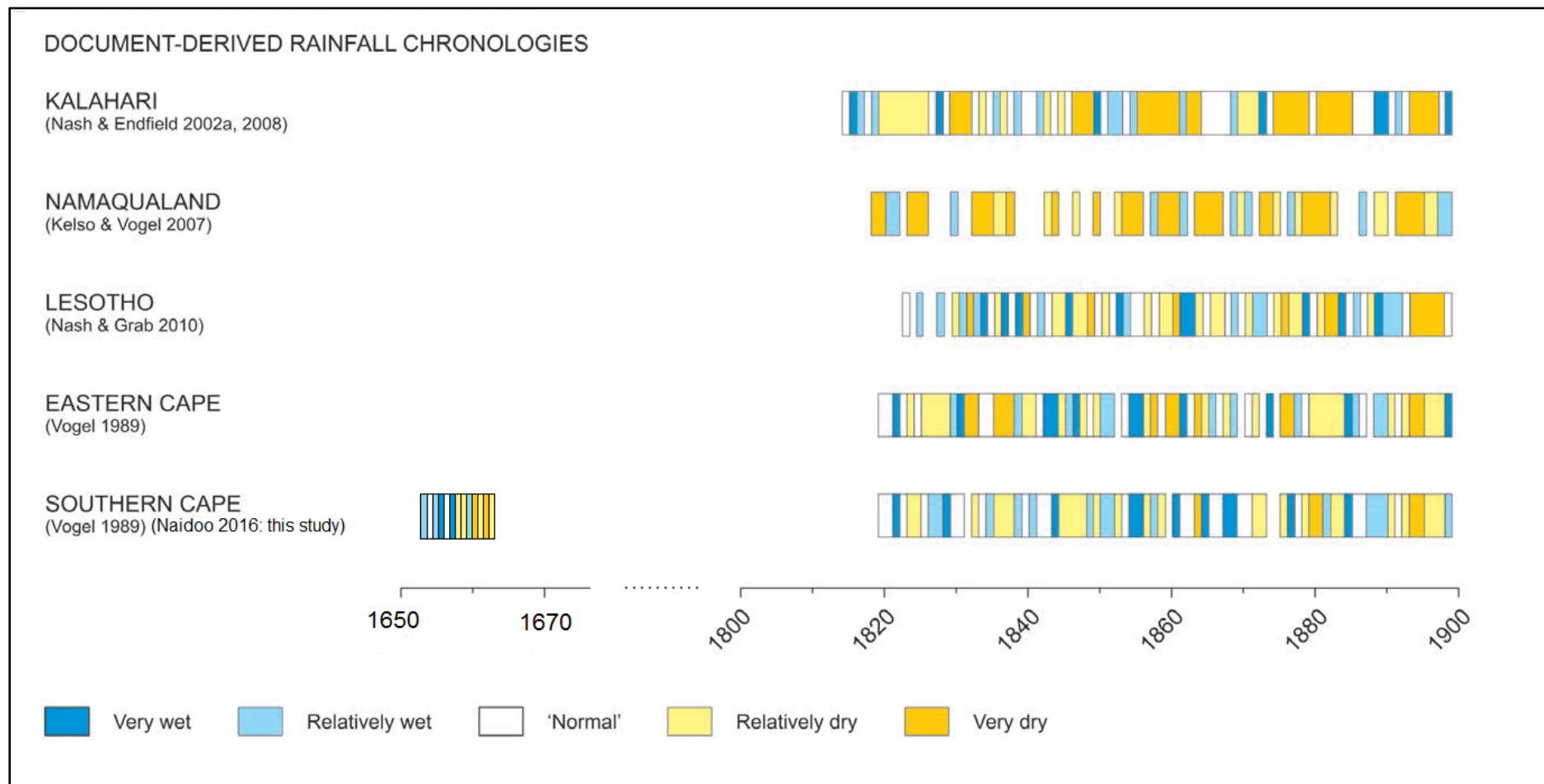
Figure 7.2: Graphical display extending the rainfall chronology for southern Africa including the results from this study with relative wetness inferred from numbers of mentions of rainfall (after Nash and Adamson, 2014).
