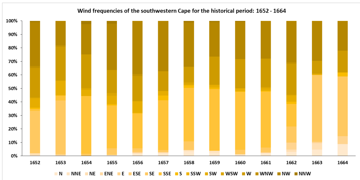
Figure 5.12: Wind frequencies at the Cape during Historical times
