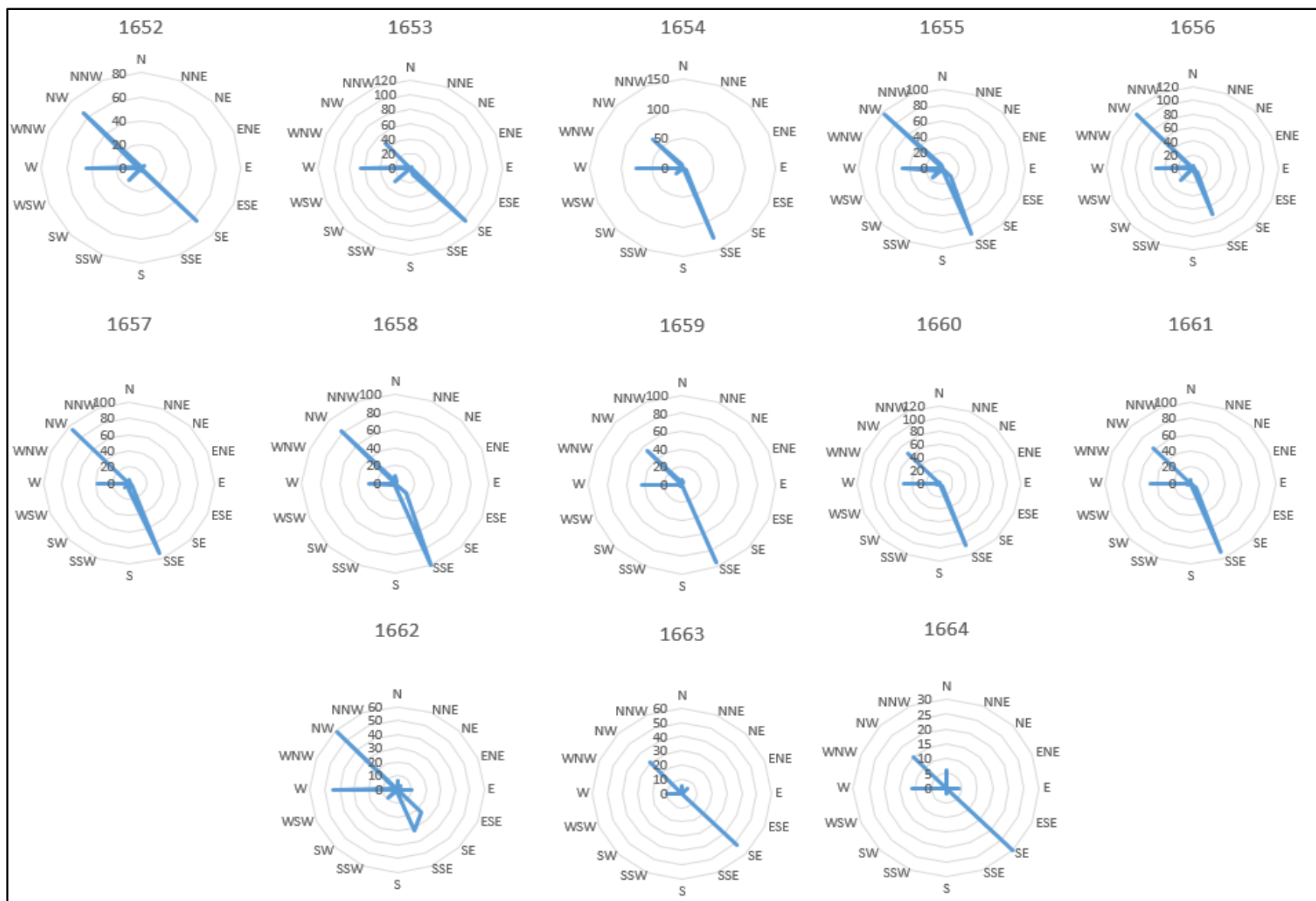
Figure 5.13: Web graphs depicting annual dominant wind directions for the historical period: 1652-1664
