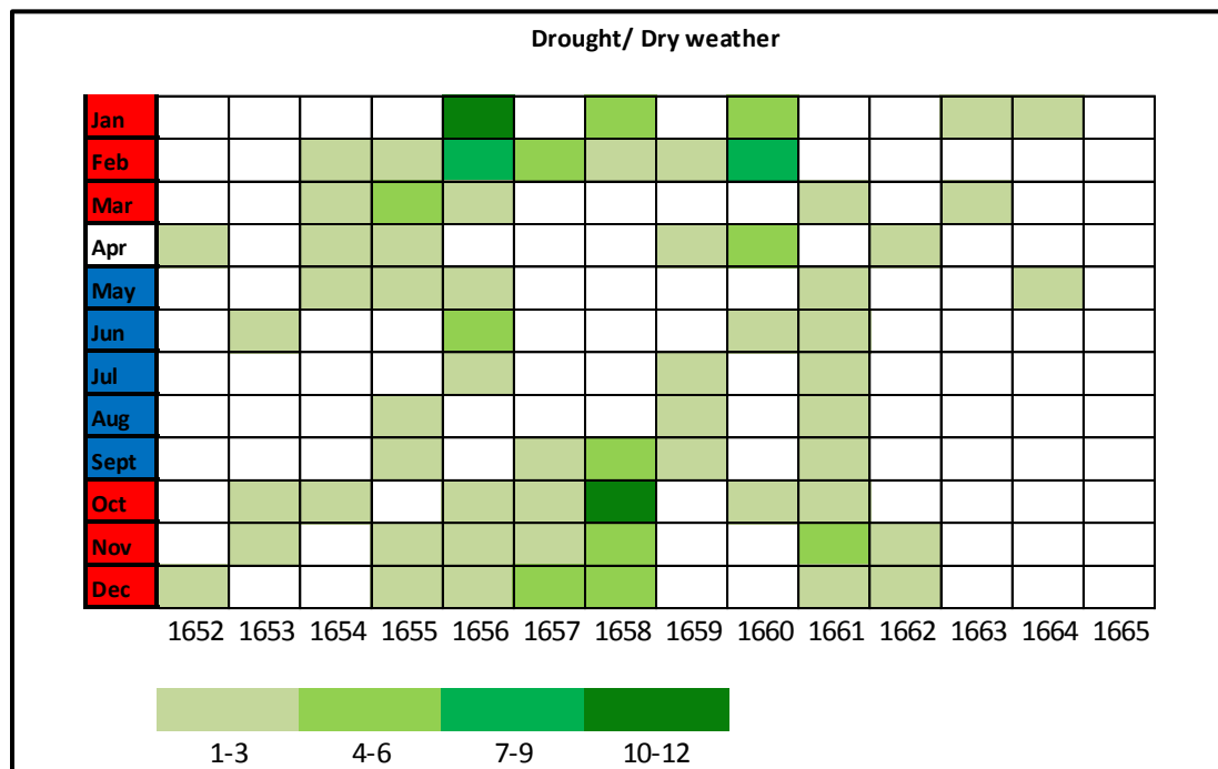
Figure 5.10: Mentions of drought or dry weather incidents
