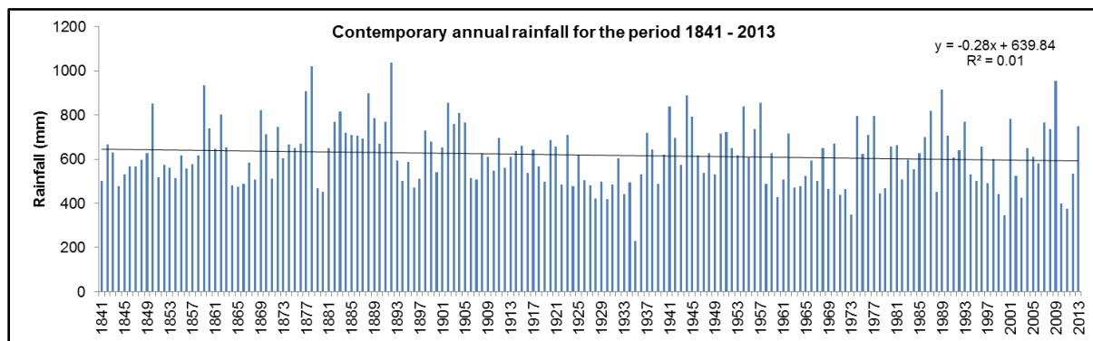
Figure 5.6: Annual rainfall for the contemporary period: 1841-2013
