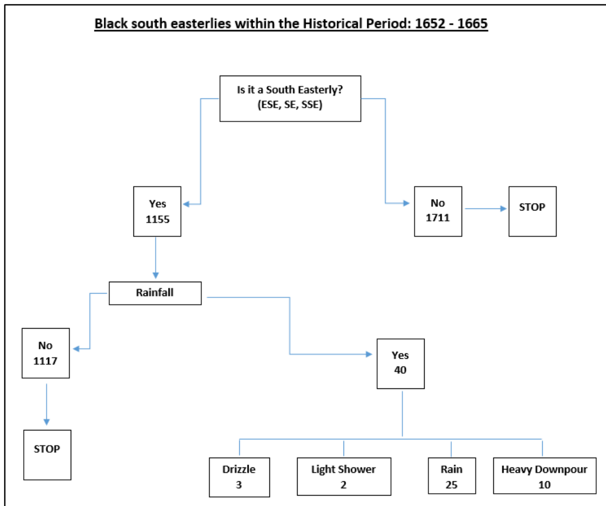
Figure 5.16: Flow diagram indicating weather patterns which coincide with south-easterlies winds. Numbers indicated reflect the number of mentions of each weather condition.
