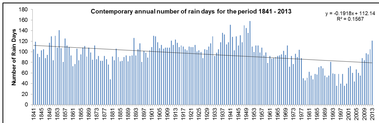
Figure 5.5: Annual number of rain days for the contemporary period: 1841-2013
