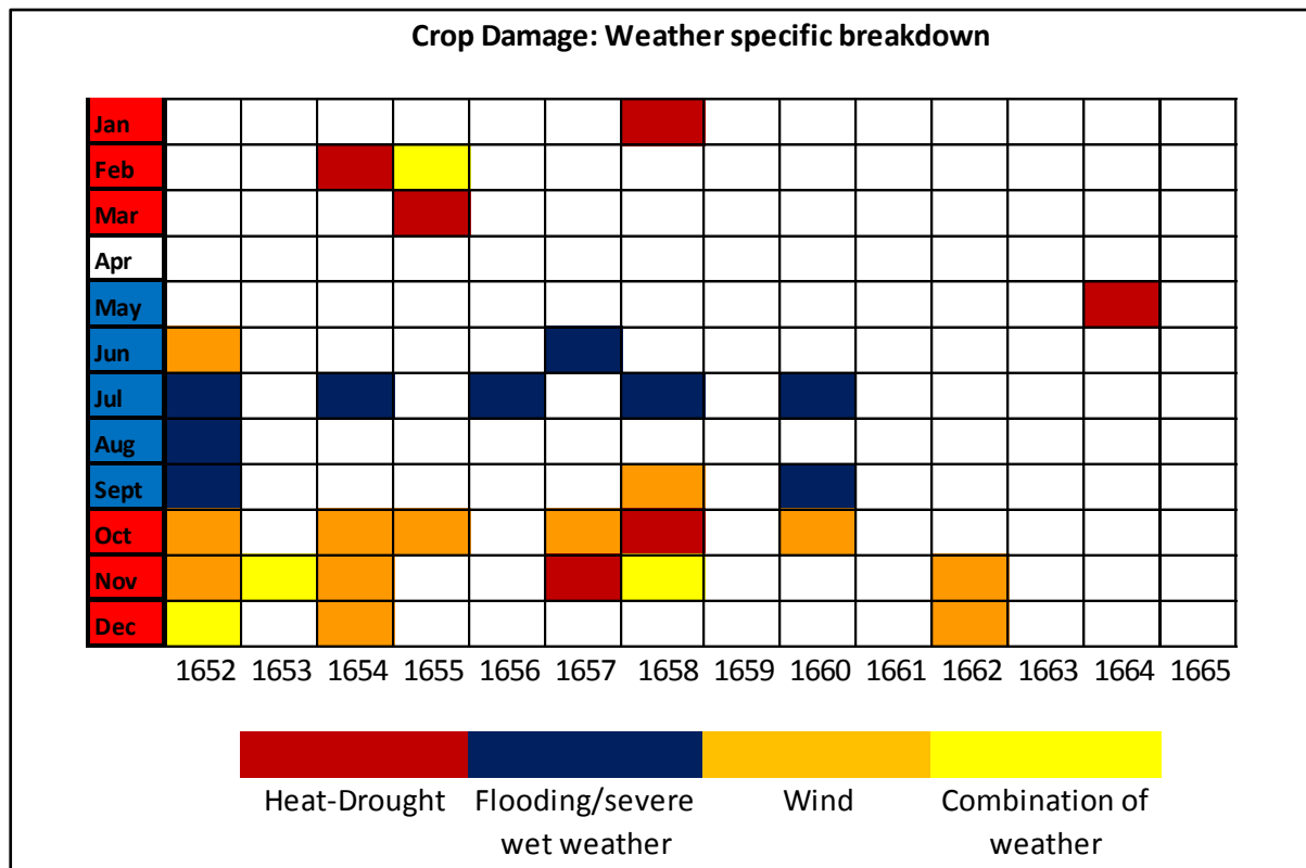
Figure 6.3: Grid showing the breakdown of weather conditions resulting in crop damage
