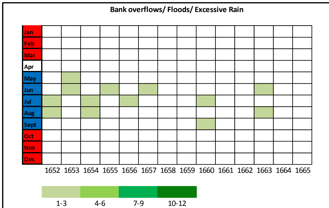
Figure 5.9: Mentions of wet weather incidents
