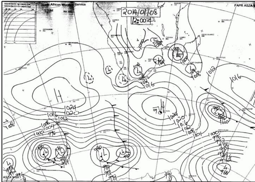
Figure 2.5: Synoptic Chart of South Africa in the summer. Notable are the more southerly location of mid-latitude cyclones, the high pressure system over the interior, and numerous coastal lows.
