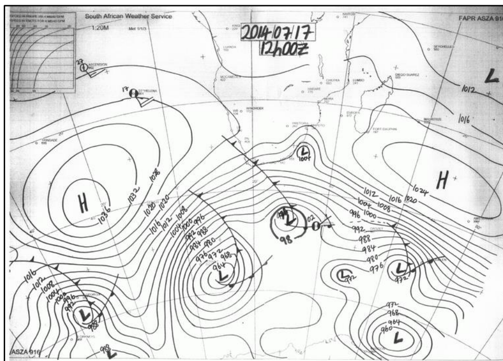
Figure 2.4: Synoptic Chart of South Africa in the winter, demonstrating the frequent passage and landfall of mid-latitude cyclones, and the less dominant high pressure cells over the interior.
