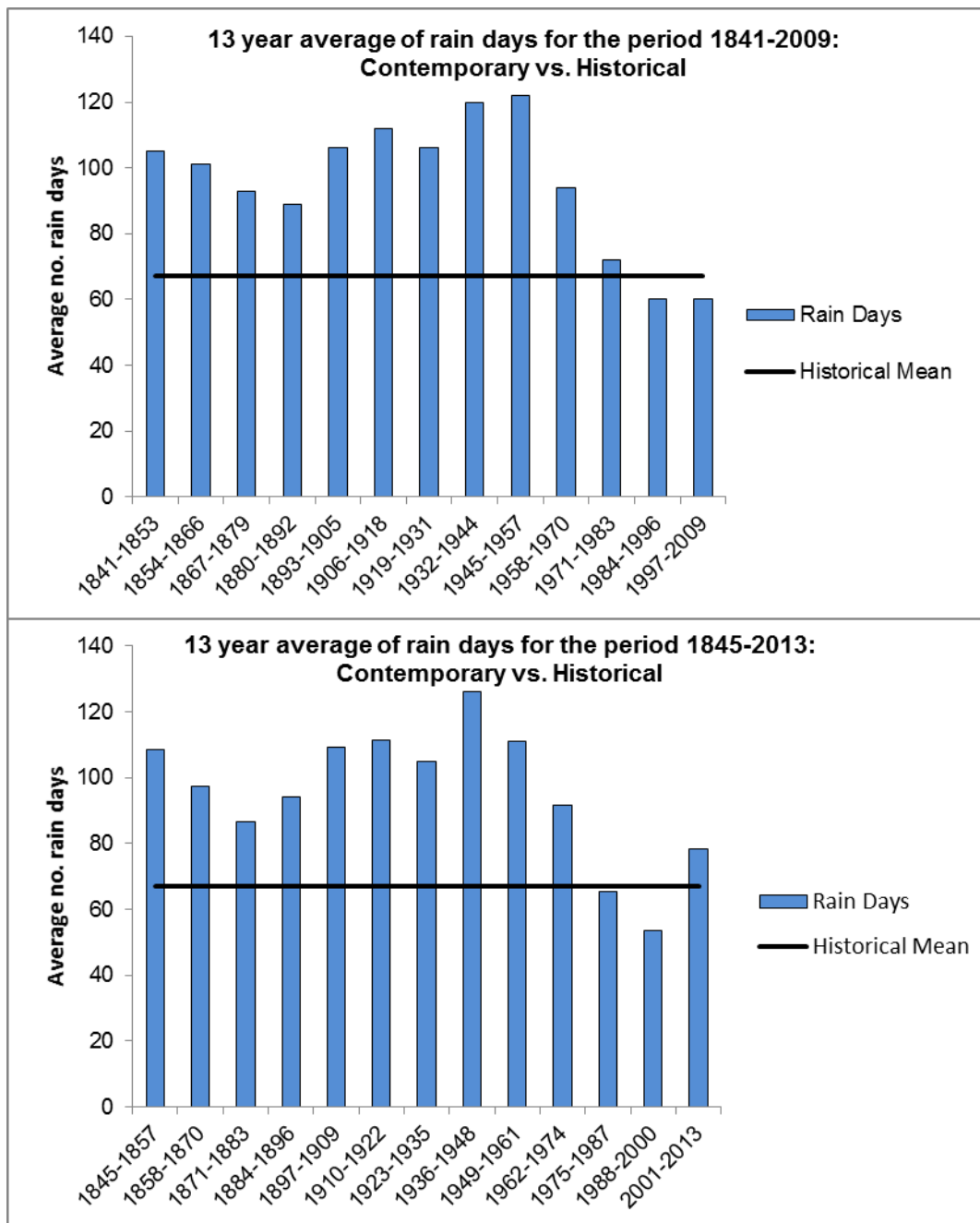
Figure 5.8: Thirteen year average rain day sets for the contemporary period: 1841-2009 and 1845-2013
