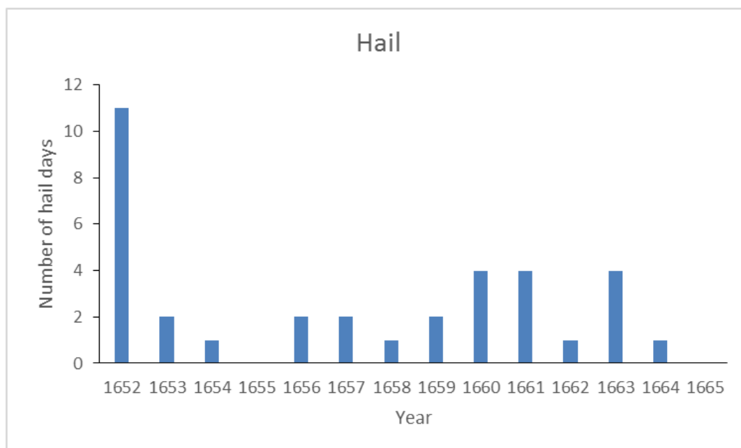
Figure 5.17: Number of hail days for the historical period: 1652-1665
