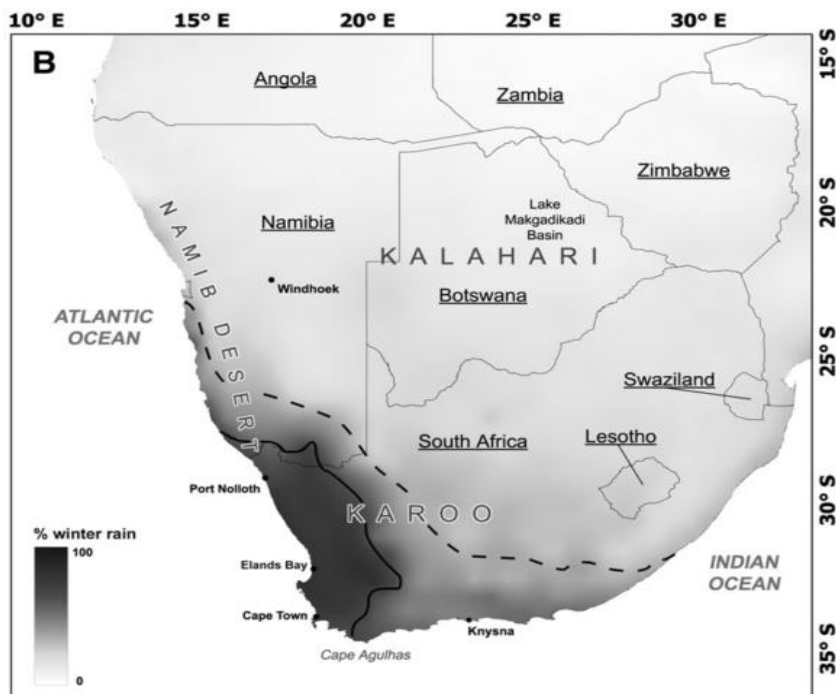
Figure 2.6: The extent of the WRZ (left of the solid black line), SRZ (right of the dotted line) and the YRZ (between the solid and dotted lines) (Chase and Meadows, 2007).
