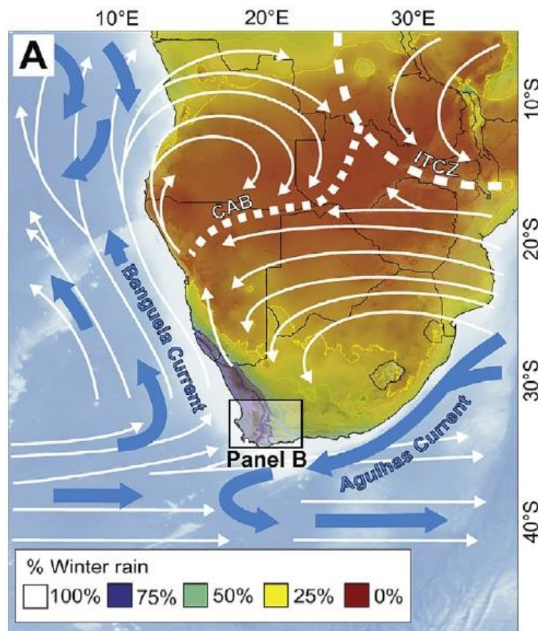
Figure 2.3: Map of southern Africa showing seasonality of rainfall. Dominant summer rainfall (red) and winter rainfall (blue) zones (Chase et al., 2015).
