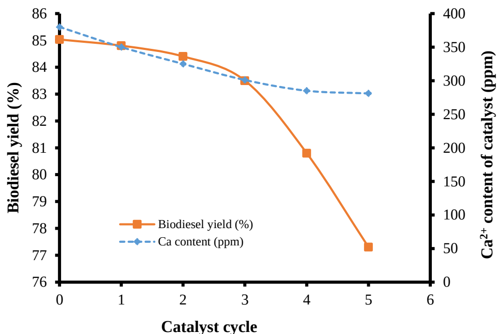
Figure 4.21: Effects of \text{Ca}^{2+} ion leaching from reused catalyst on biodiesel yield (%) at optimum conditions
