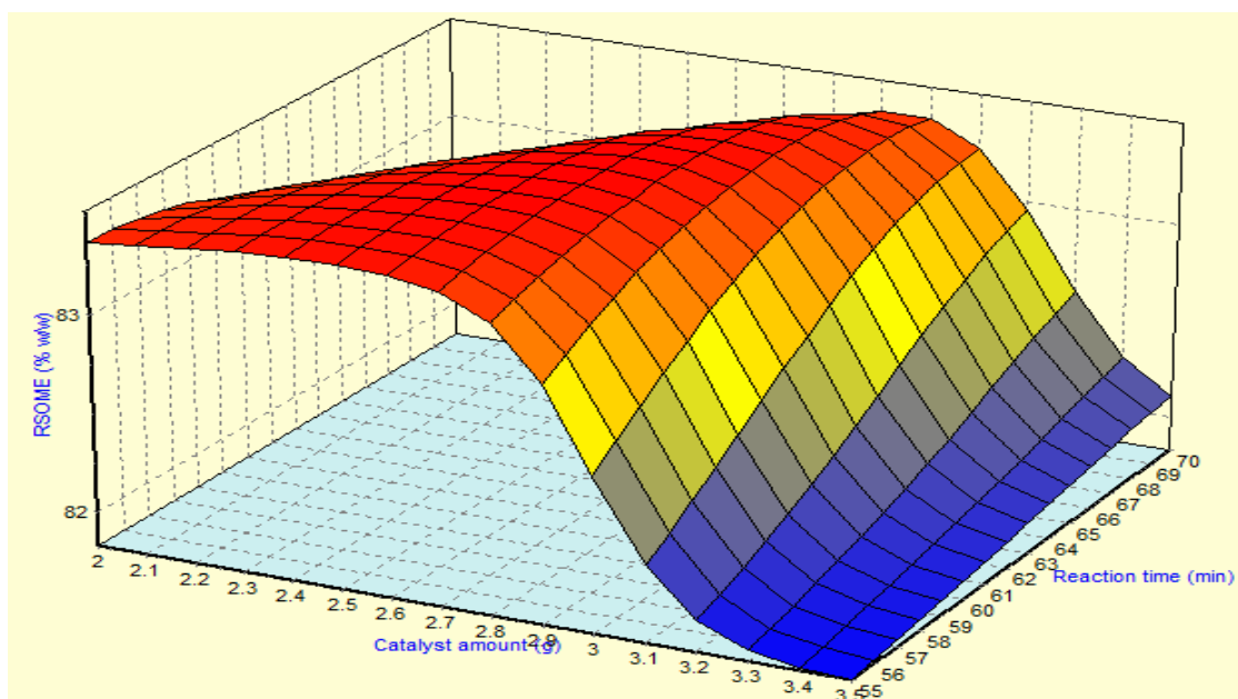
Figure 4.26: ANN Surface plot for the interactive effect of catalyst amount with reaction time on (biodiesel) RSOME yield
