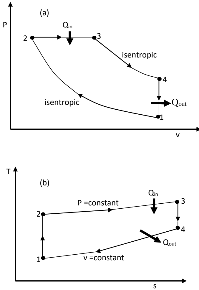
Figure 2.13: P–v (a) and T–s (b) diagrams for the ideal Diesel cycle (Adapted from Çengel & Boles, 1994)
