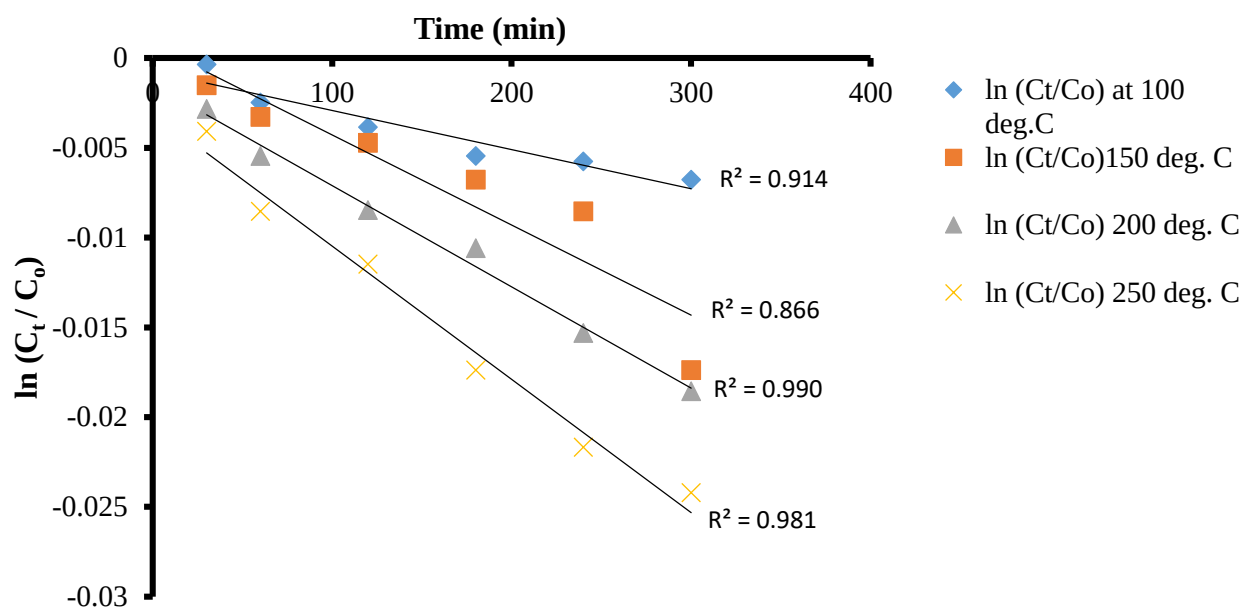
Figure 4.8: \ln(C_t/C_o) vs. time for iodine values at 100, 150, 200 and 250 °C (Adapted from Onoji et al., 2016b)
