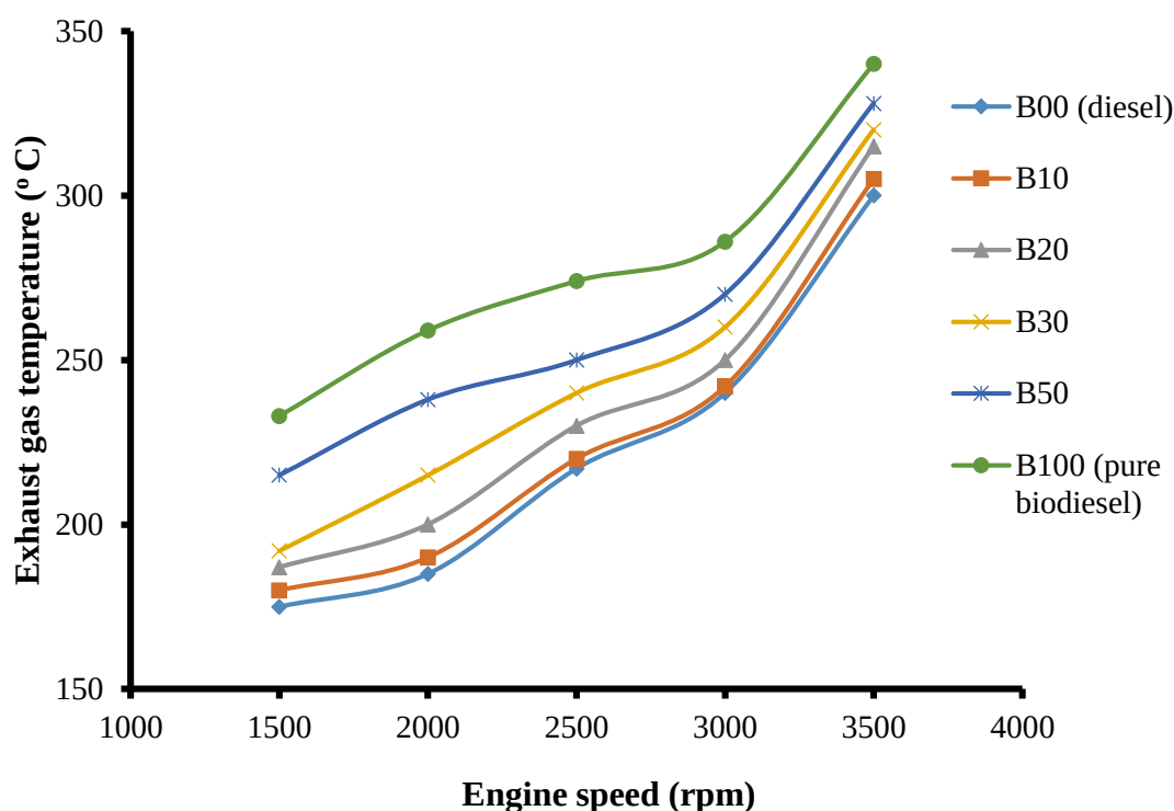
Figure 4.34: Variation of exhaust gas temperature with speed for diesel and biodiesel blends
