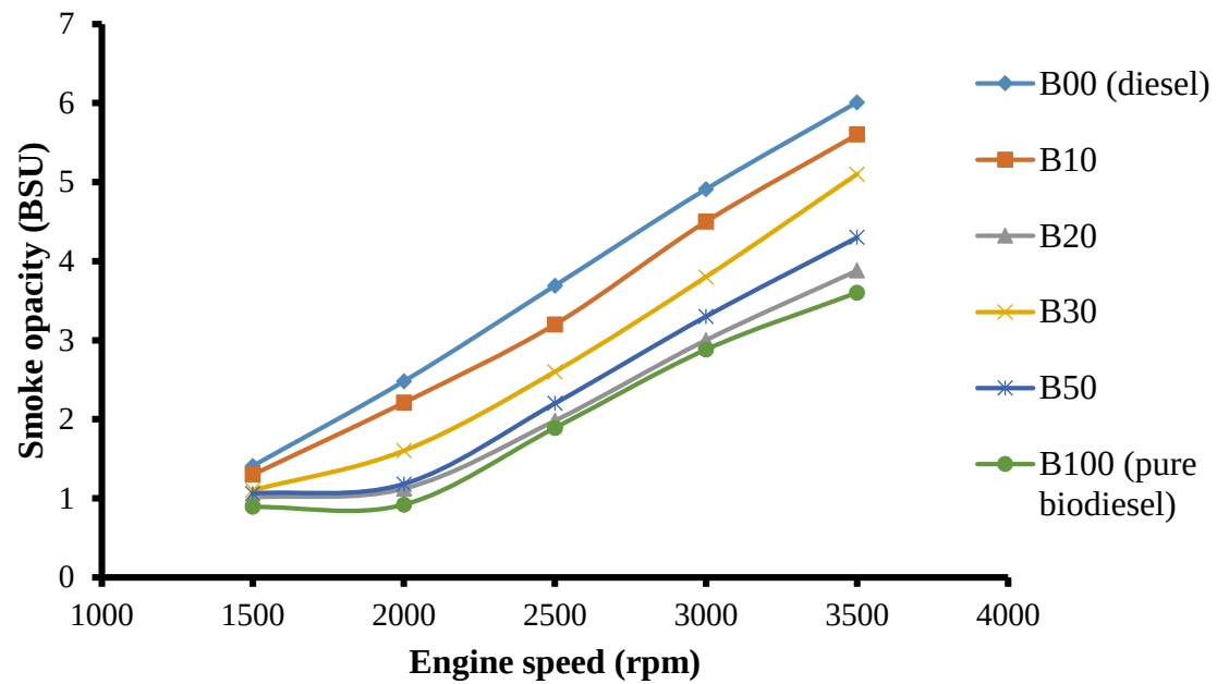
Figure 4.39: Variation of smoke opacity with speed for diesel and biodiesel blends
