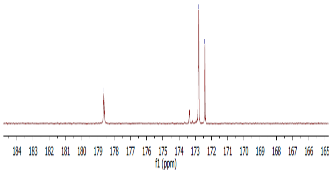
Figure G.5: ^{13}\text{C} NMR spectra of rubber seed oil (165–184 ppm)
