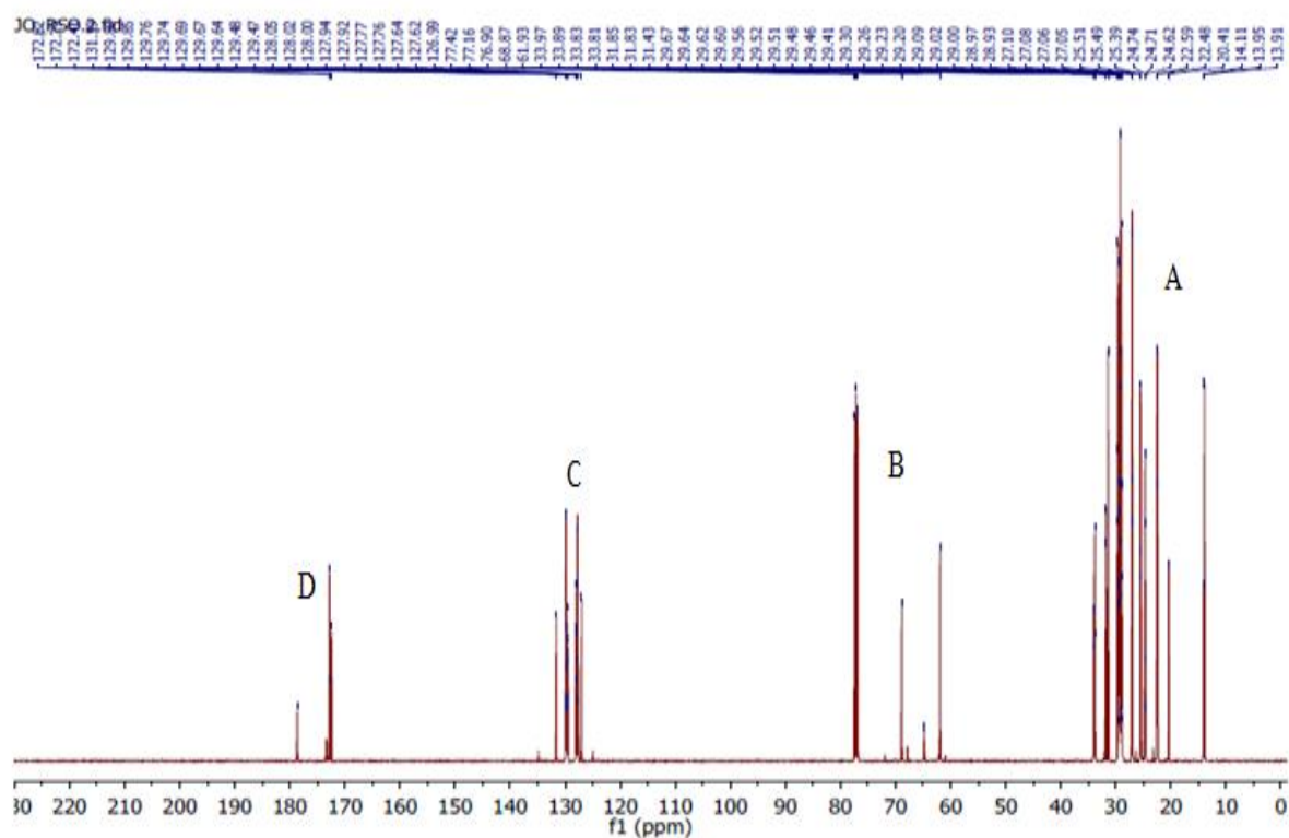
Figure 4.5: ^{13}\text{C} NMR spectrum of the rubber seed oil
