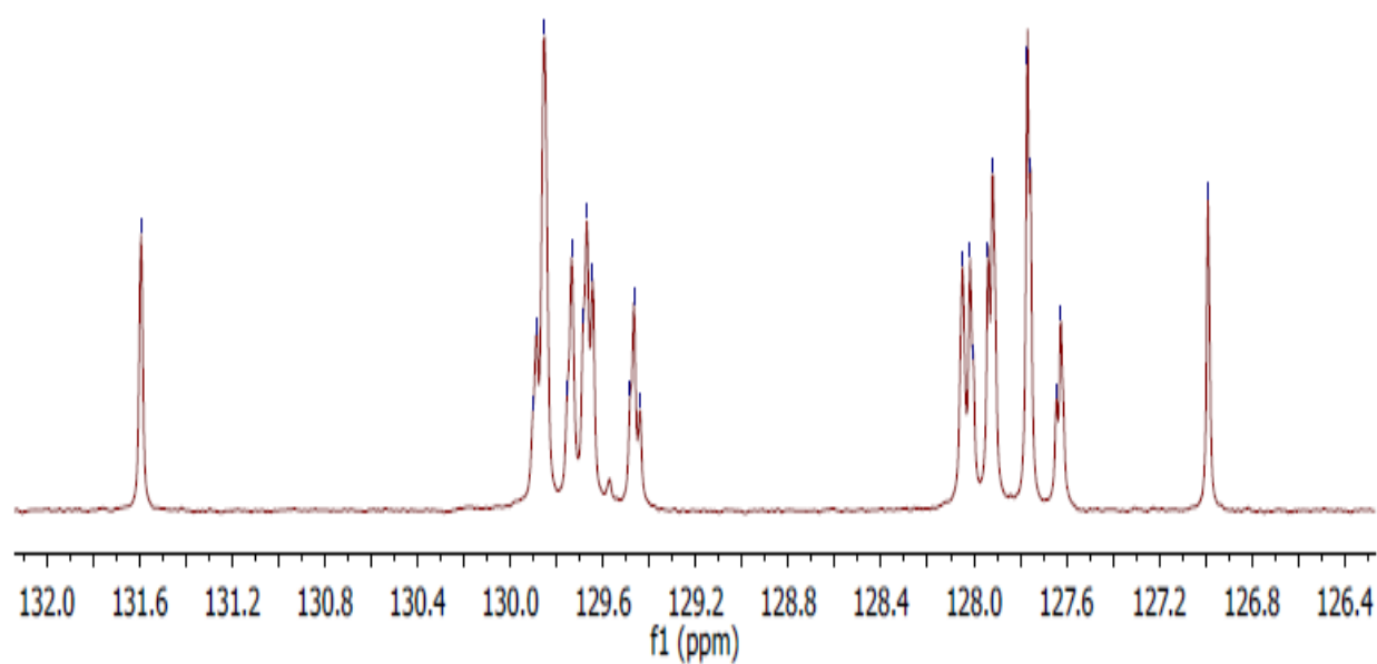
Figure G.4: ^{13}\text{C} NMR spectra of rubber seed oil (126.4–132.0 ppm)
