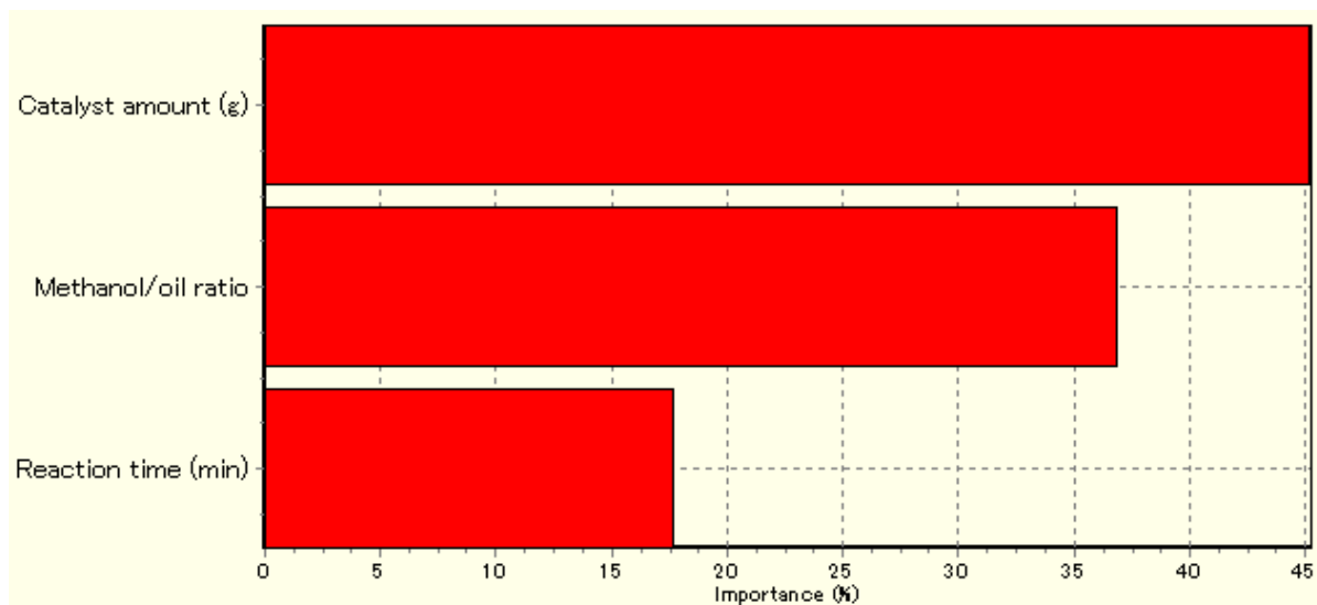
Figure 4.28: Percentage contribution of process variables to biodiesel production via ANN model (catalyst amount 45.62%, methanol/oil ratio 36.87%, and reaction time 17.51%)
