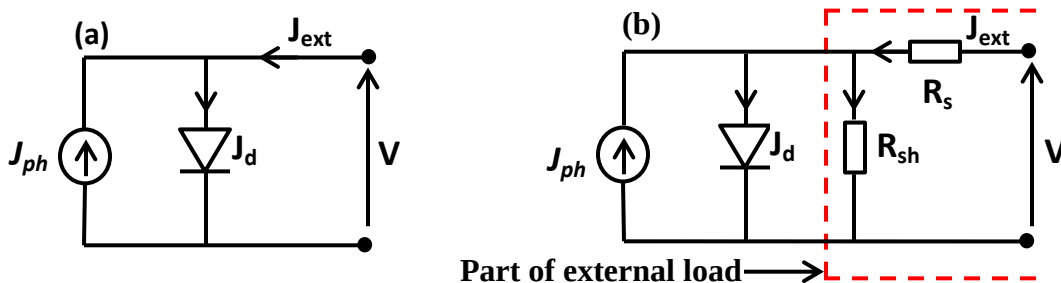
Figure 6.9 Equivalent circuits for (a) an ideal and (b) a real (practical) solar cell. J_{ph} is the photogenerated current density, J is the current density flow in the external load, R_s and R_{sh} are the series and shunt resistances respectively, J_d is the current density through the diode and V is the applied voltage
