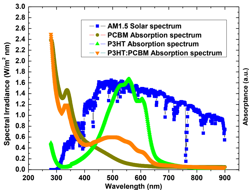
Figure 4.13 Extractable portion of AM1.5 solar spectrum as defined by the experimental materials
