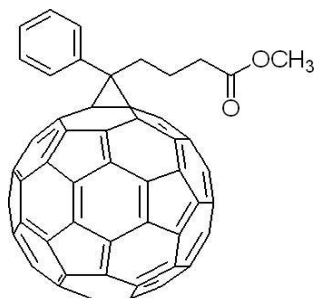
Figure 4.4 Structural form of PCBM
