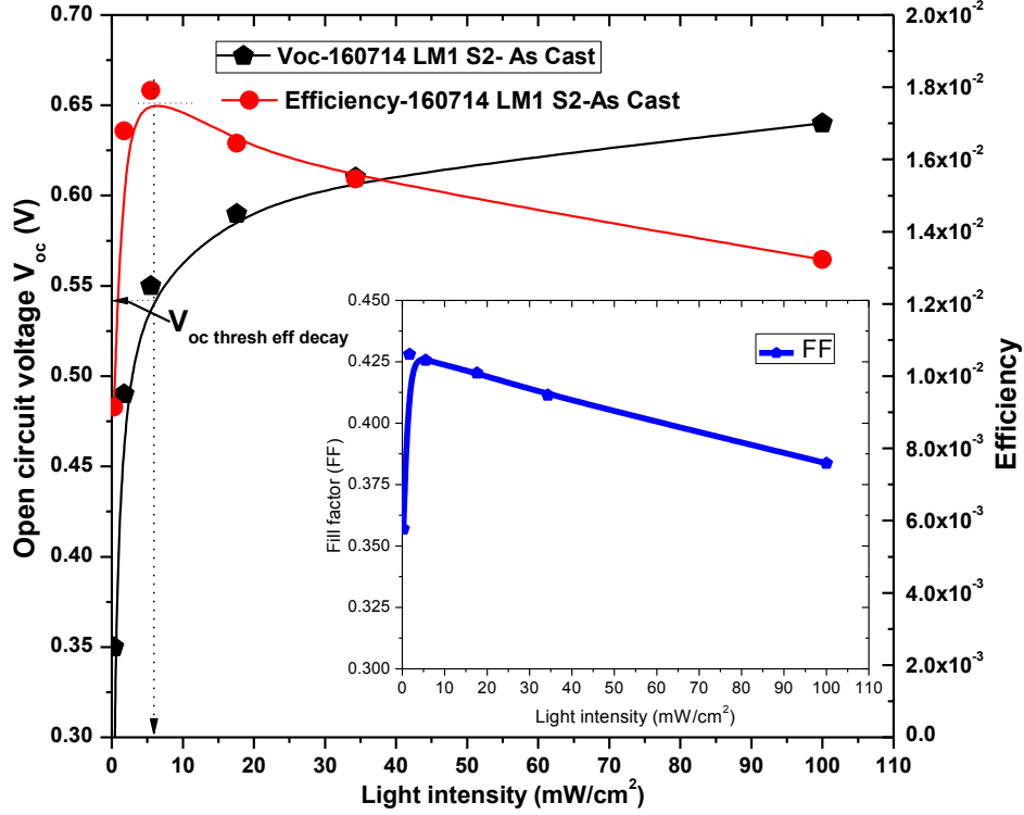
Figure 5.5 Variation of efficiency \eta and open circuit voltage V_{oc} with light intensity. The smooth curves are lines of best fit to the respective data points. Inset is for the variation of the corresponding fill factor with light intensity.
