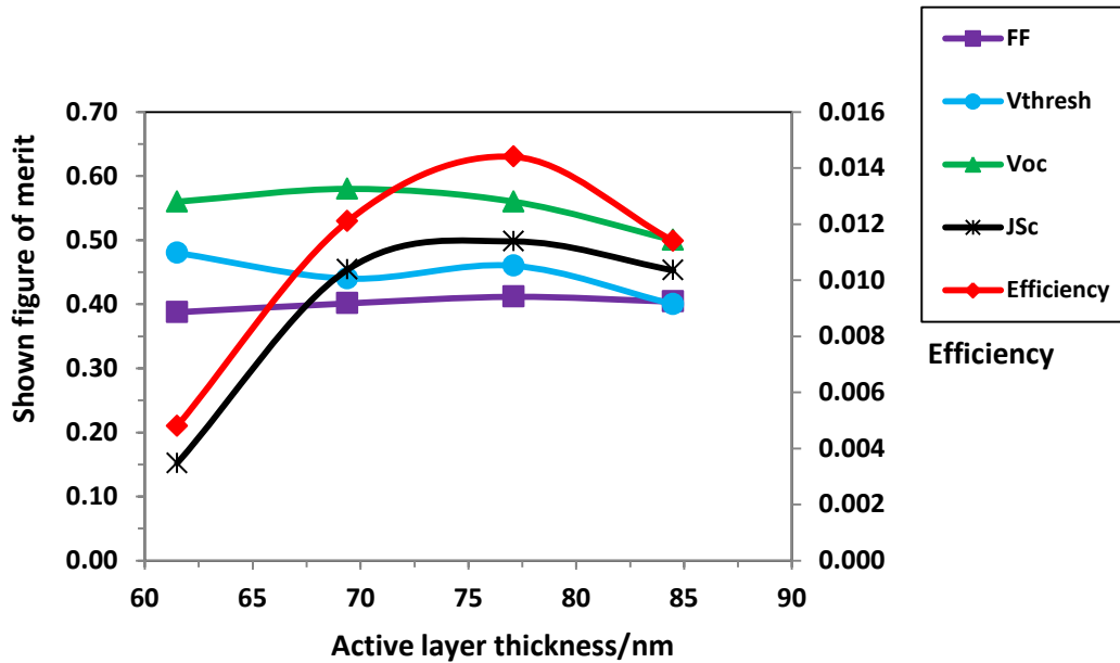
Figure 6.10 Variations of parameters of merit – V_{oc} , J_{sc} , efficiency \eta , fill factor ( FF ) and V_{thres} with active layer thickness for the P3HT:PCBM blend based solar cell
