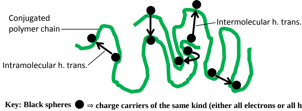
Figure 2.27 Intramolecular (intrachain) and intermolecular (interchain) hopping transport
