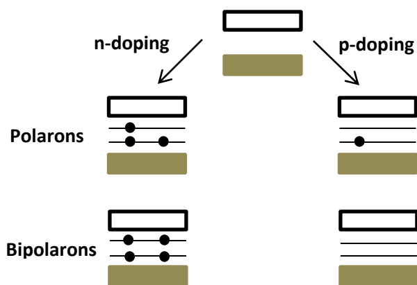
Figure 2.24 Schematic illustration of an electron polaron and bipolaron to the left and a hole polaron and bipolaron to the right [32], [33]
