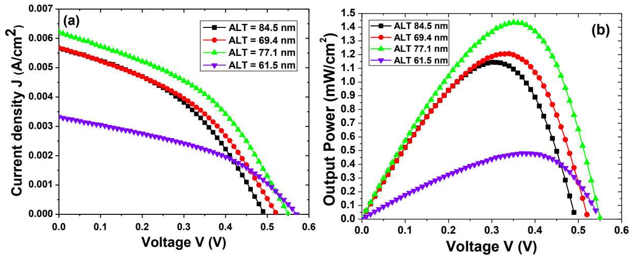
Figure 6.6 (a) J(V) and (b) output power characteristics for different active layer thicknesses (ALTs) under solar simulated white light illumination intensity of 100 mW/cm 2 incident on the ITO/PEDOT:PSS/P3HT:PCBM/Al devices
