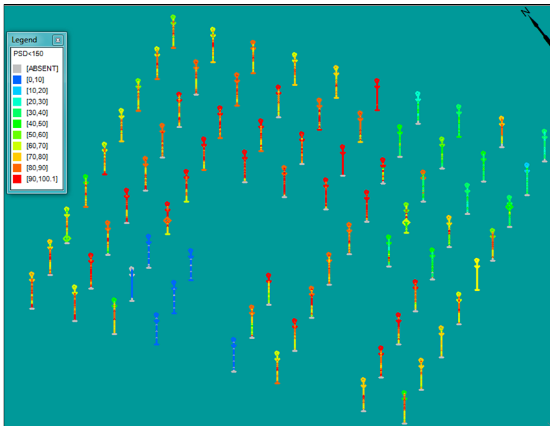
Figure 27: A 3D view of grain size < 150µm (%) on all boreholes across the dam.
