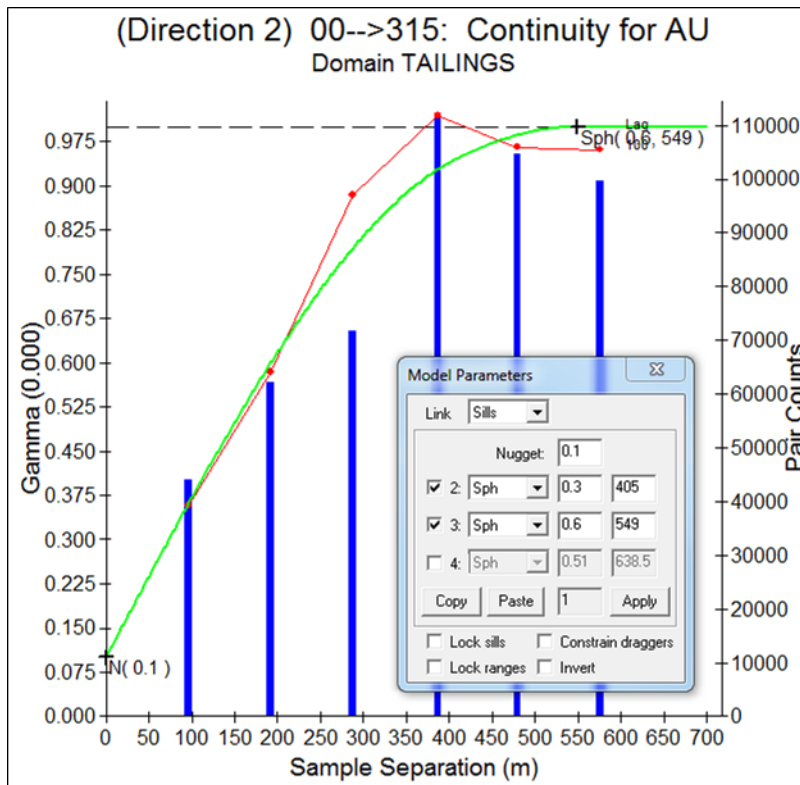
Figure A11: Au variogram model along secondary direction
