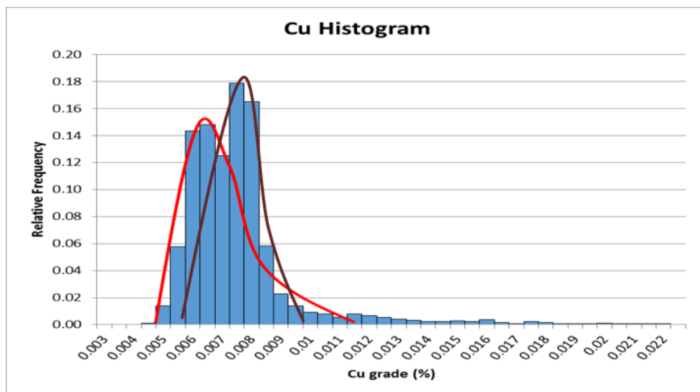
Figure 20: Copper (%Cu) Histogram.
