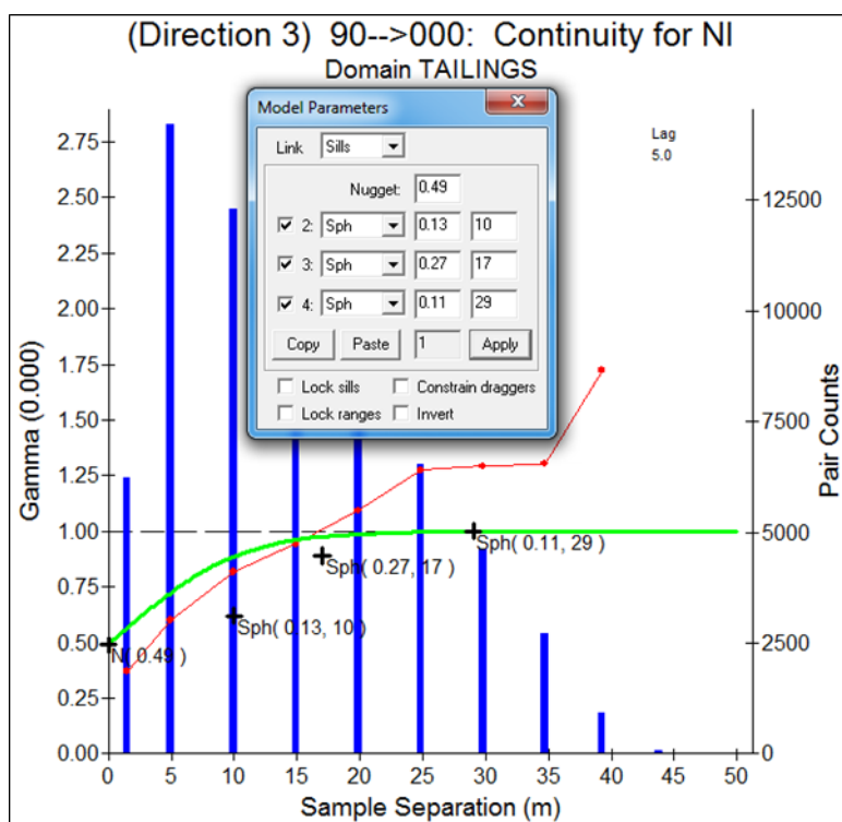
Figure A16: Ni downhole variogram model
