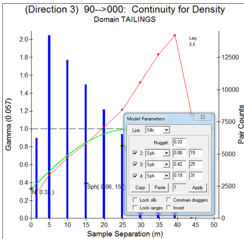
Figure A19: Density downhole variogram model
