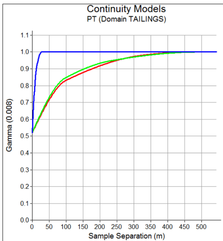
Figure A6: Pt variogram models (all three directions – blue, green & red)
