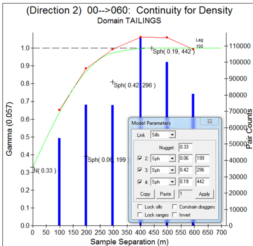
Figure A20: Density variogram model along secondary direction
