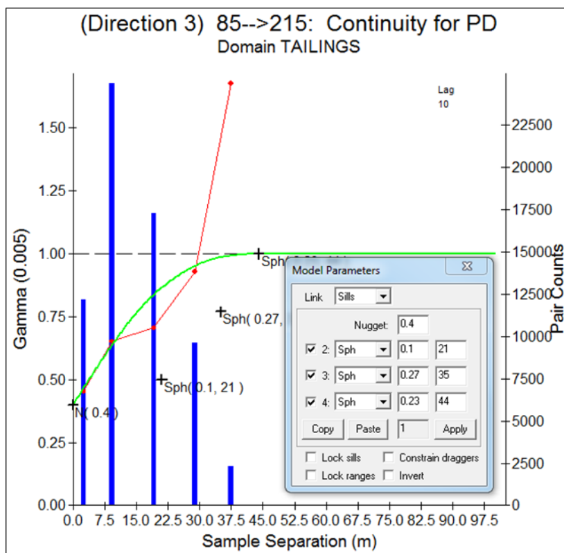
Figure A7: Pd downhole variogram model
