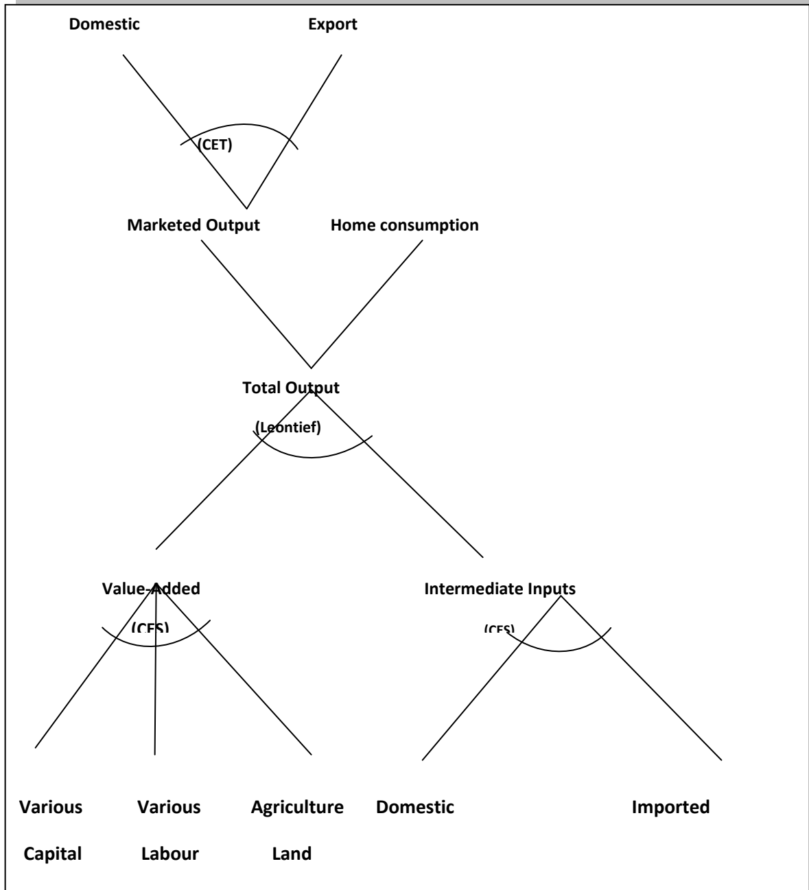
Figure 3.1: Structure of Production in Zambia CGE VAT Model
