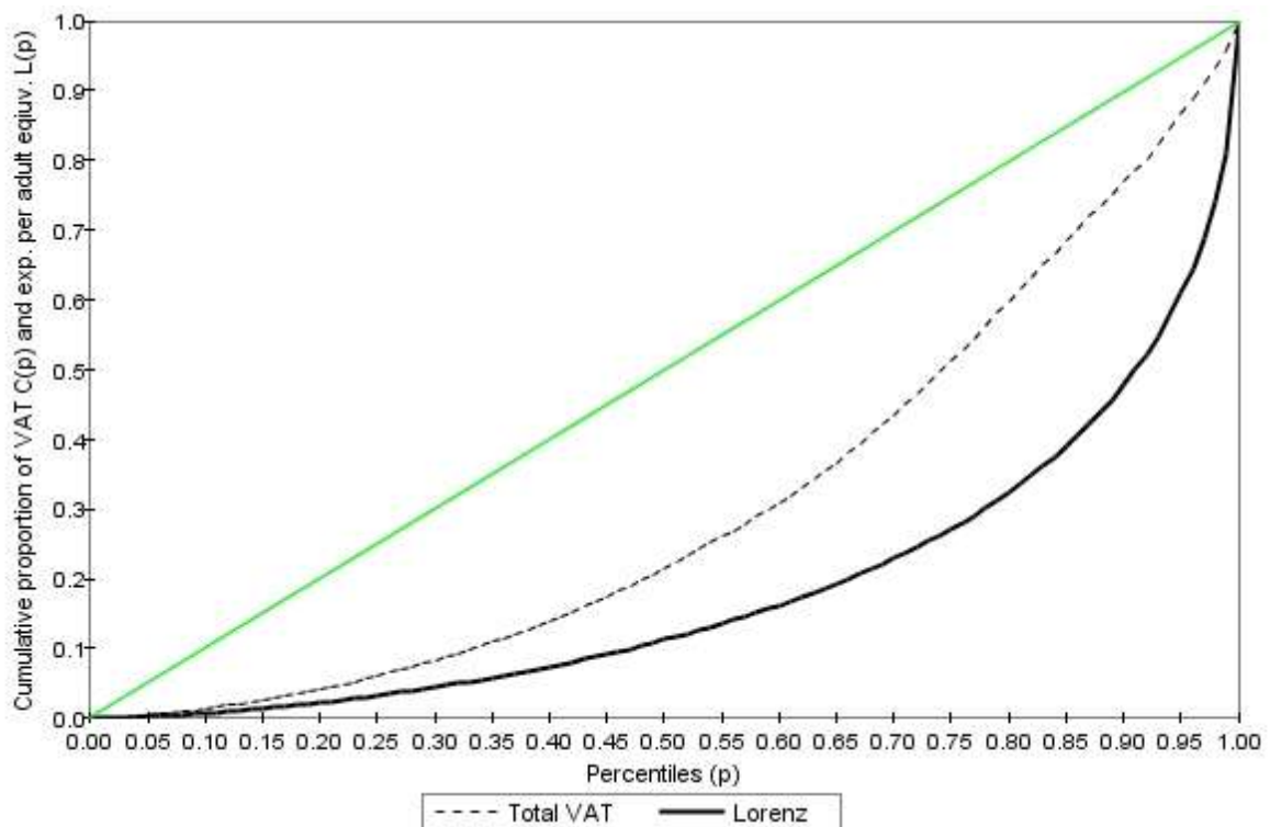
Figure 2.3: Concentration Curve of Total VAT Payments
