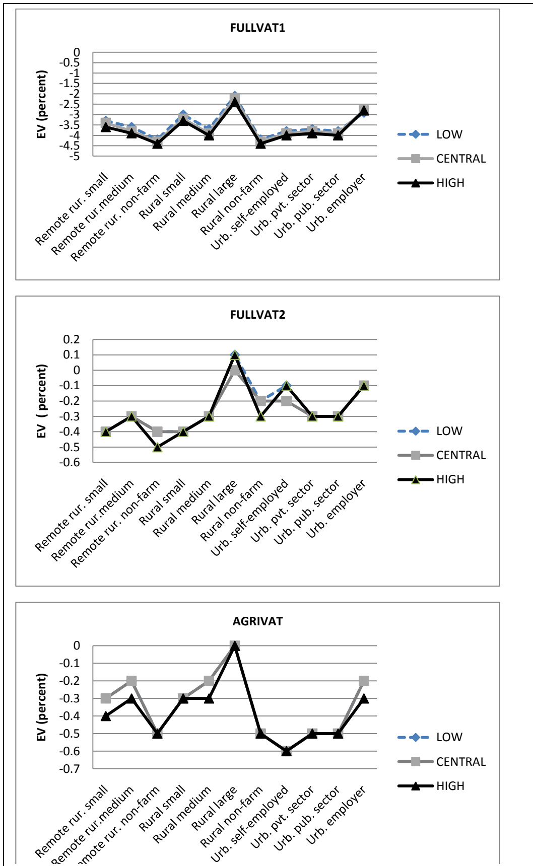
Figure 3.12: Welfare Sensitivity to Import ( \sigma_q ) Elasticities
