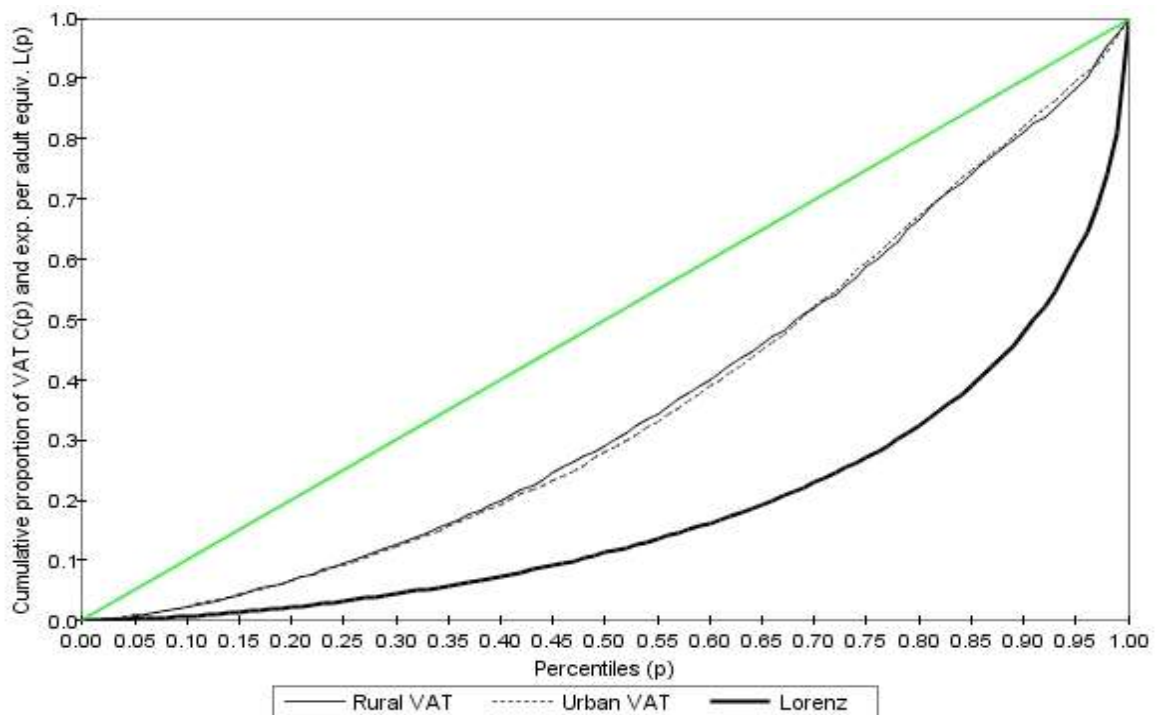
Figure 2.4: Concentration Curves for VAT Payments by Rural-Urban
