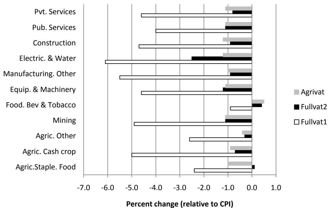
Figure 3.5: Relative Changes in Prices of Aggregate Intermediate Inputs
