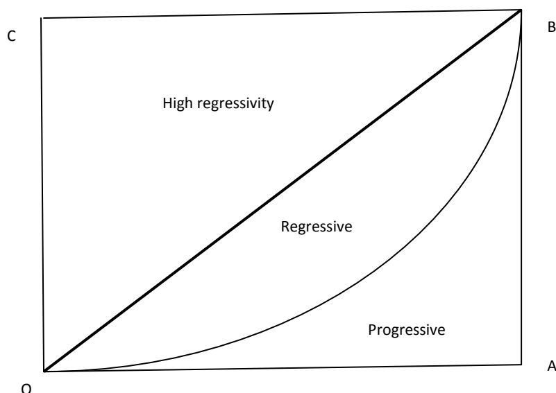
Figure 2.2: Concentration Curve for Taxes
