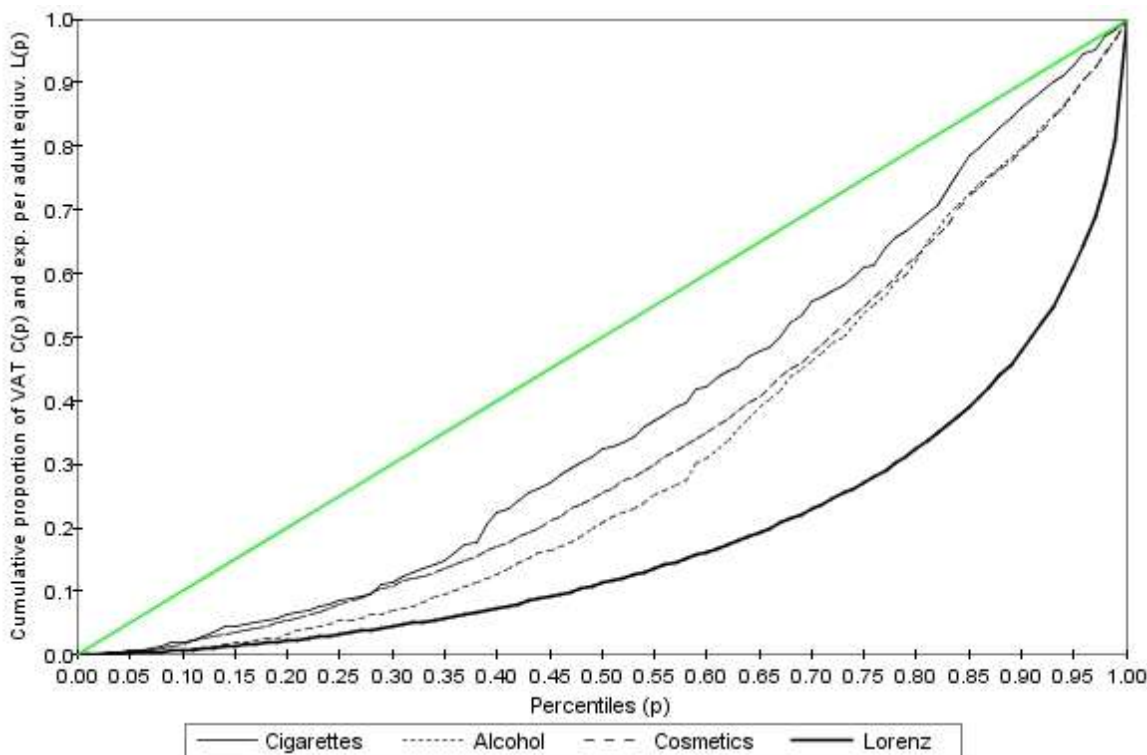
Figure 2.7: Concentration Curves for VAT on Cigarettes, Alcohol and Cosmetics
