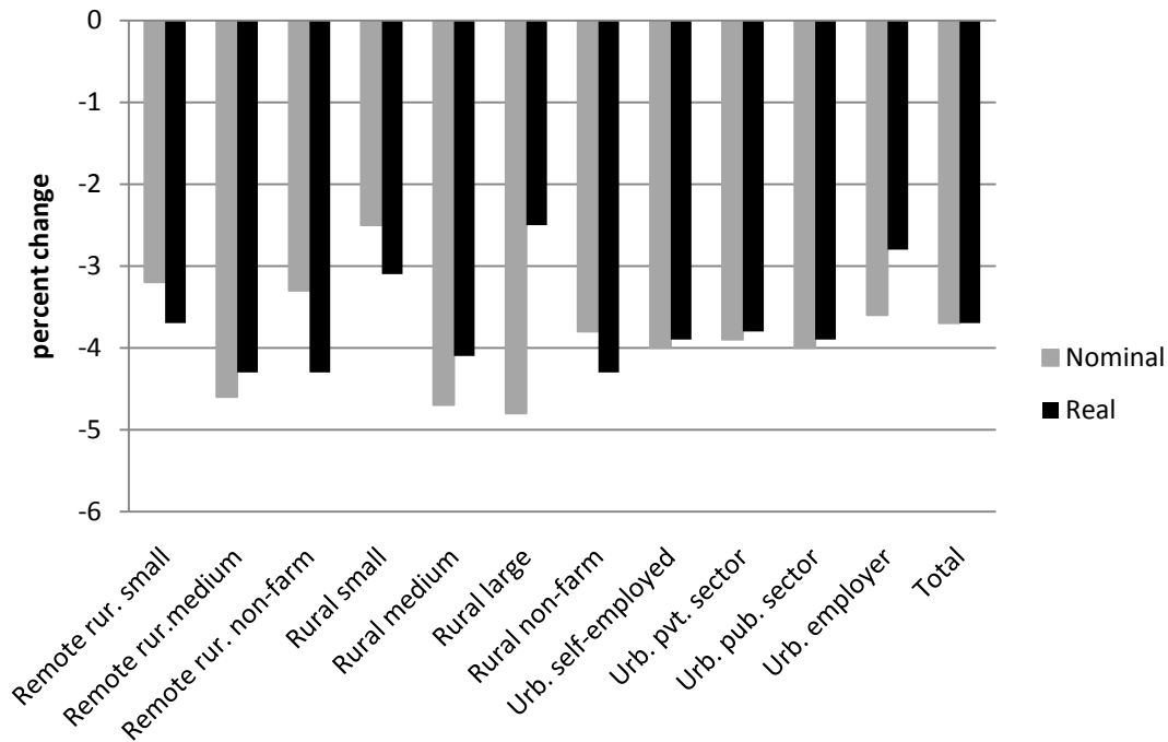
Figure 3.8: Household Consumption Effects from a full VAT Reform (1)
