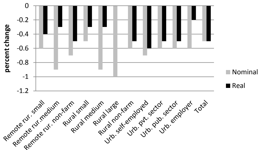
Figure 3.10: Household Expenditure Effects from an Agriculture VAT Reform
