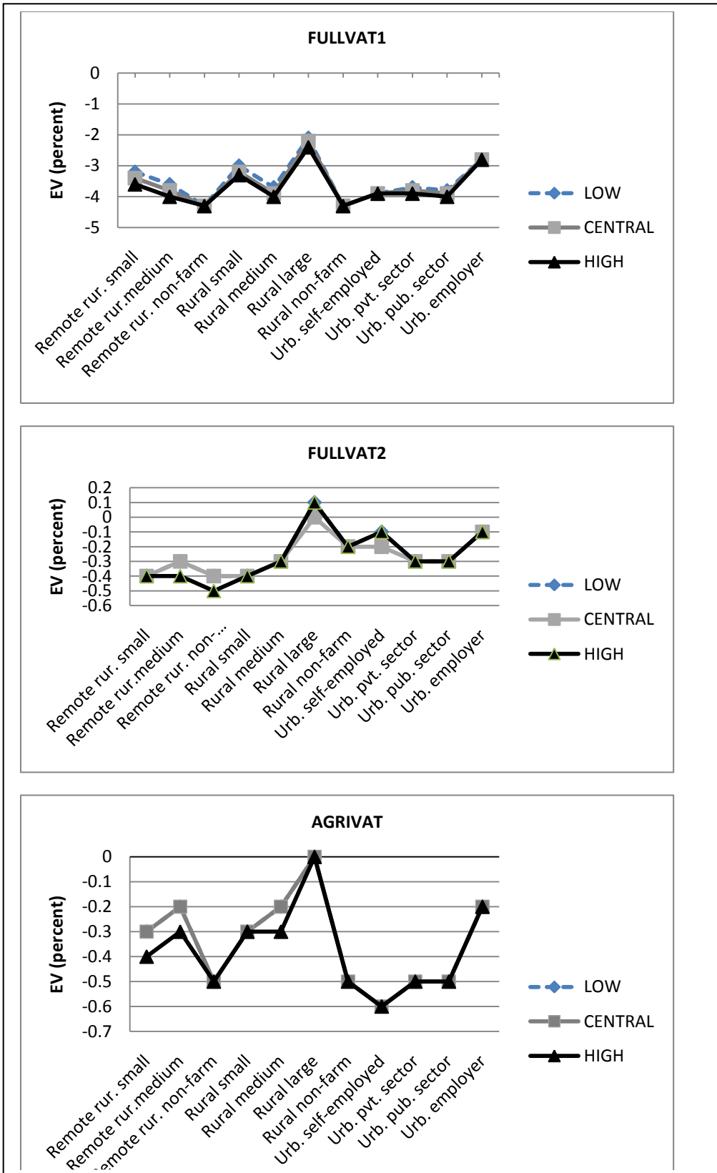
Figure 3.13: Welfare Sensitivity to Export ( \sigma_t ) Elasticities
