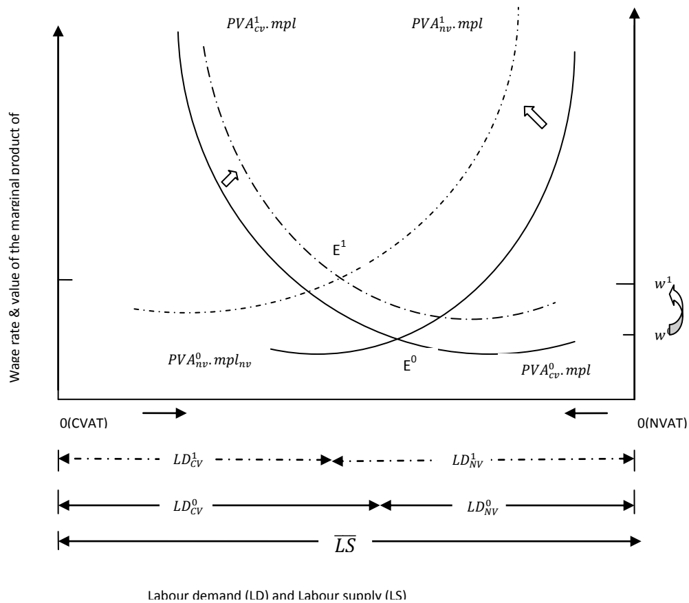
Figure 3.3: Short-run VAT effects on Resource Allocation
