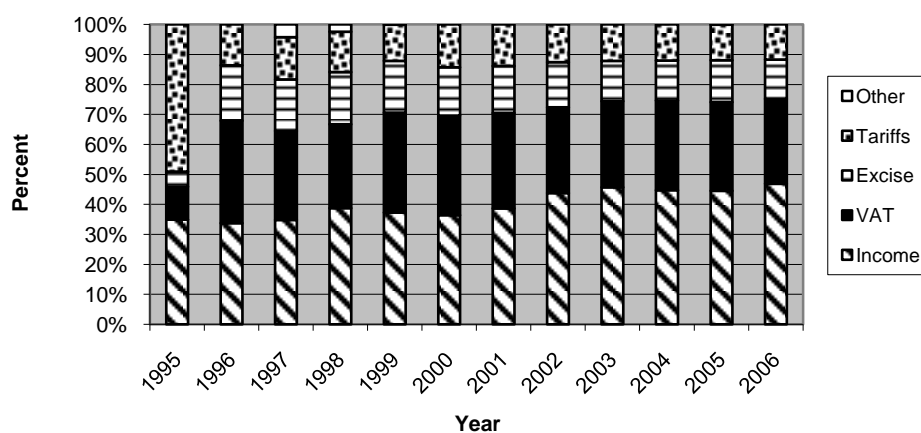
Figure 1.1: Tax Revenue Collections in Zambia 1995-2006 (percentages)
