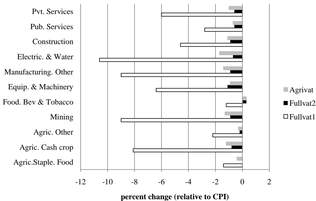
Figure 3.6: Relative Changes in Prices of Production Output
