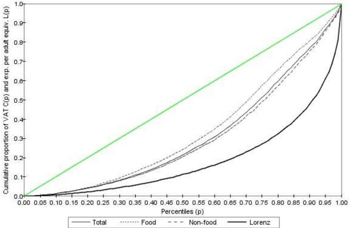
Figure 2.5: Concentration Curves for Food and Non-food VAT
