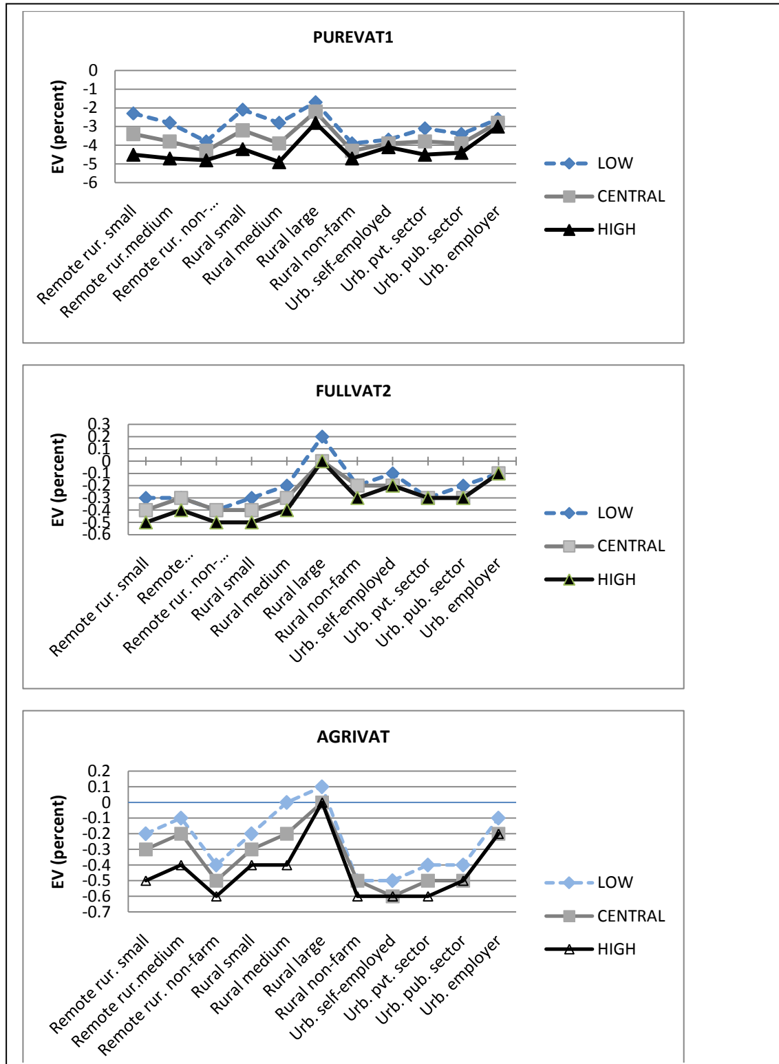
Figure 3.11: Welfare Sensitivity to Production ( \sigma_{va} ) Elasticities
