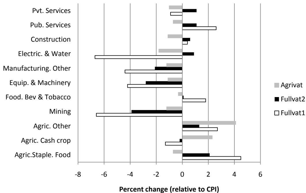
Figure 3.4: Relative Changes to Purchaser Prices of Composite Commodities
