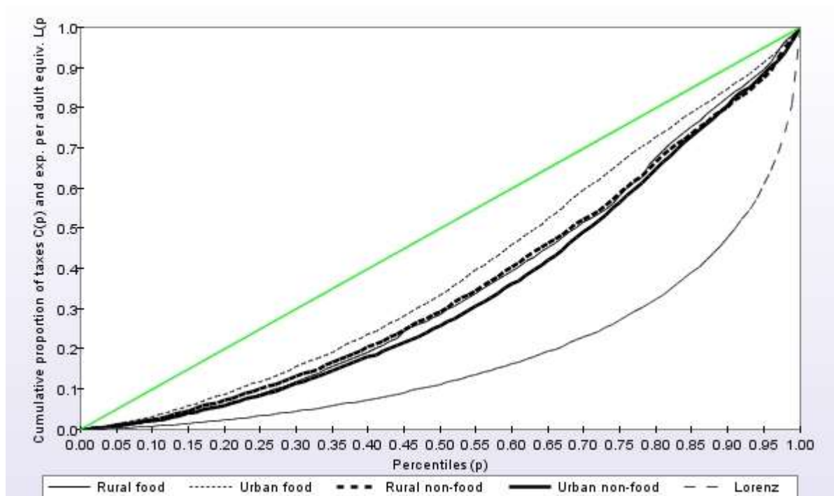
Figure 2.6: Concentration Curves for Food VAT and non-food VAT by Rural and Urban.
