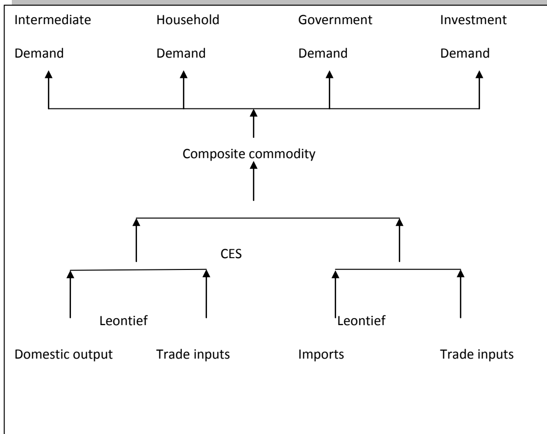
Figure 3.2: Commodity Markets in Zambia CGE VAT Model
