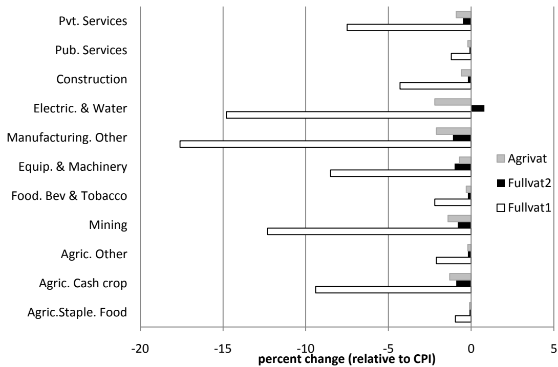
Figure 3.7: Relative Changes in Prices of Value Added
