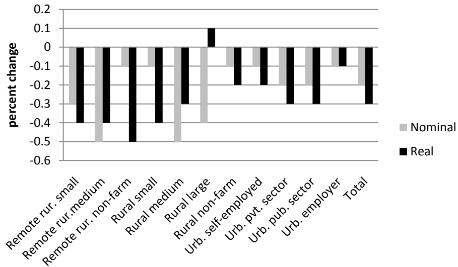
Figure 3.9: Household Consumption Effects from a full VAT Reform (2)
