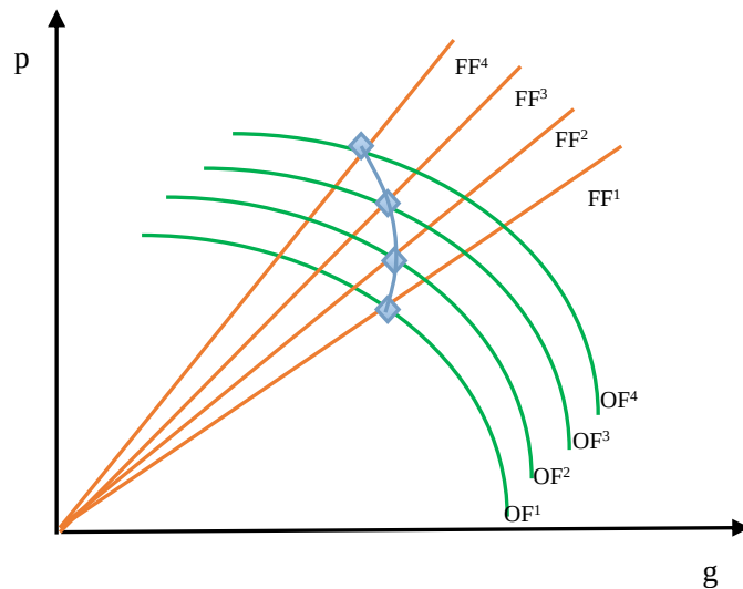
Figure 2: Illustration of the locus of optimal growth points for varying best-practice techniques
