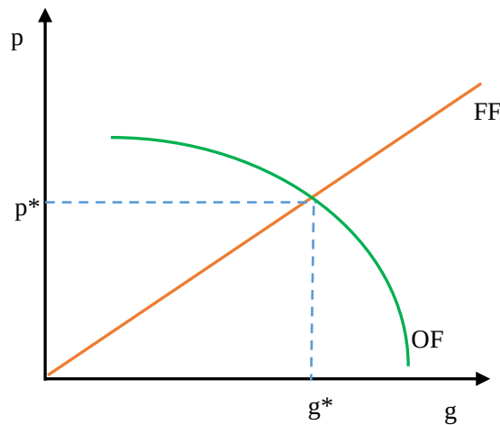
Figure 1: Illustration of the Opportunity Frontier (OF) and the Finance Frontier (FF)
