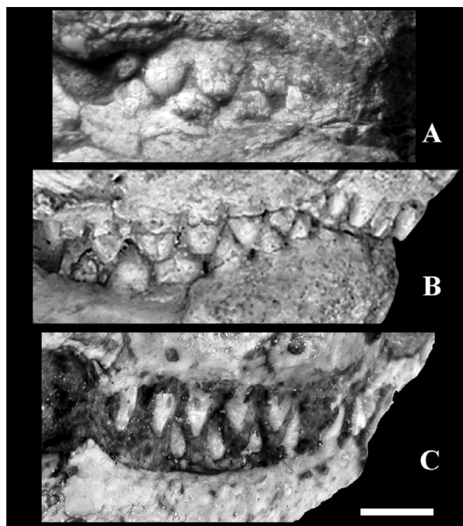
Figure 9. Comparison between A, Teratophon spinigenis (BP/1/4587), B, Eumetabolodon bathycephalus (IVPP V6064) and C, Procolophon trigoniceps (BP/1/5927b); showing differences in dentition. Scale bar = 5 mm for A, B and 3.5 mm for C.
