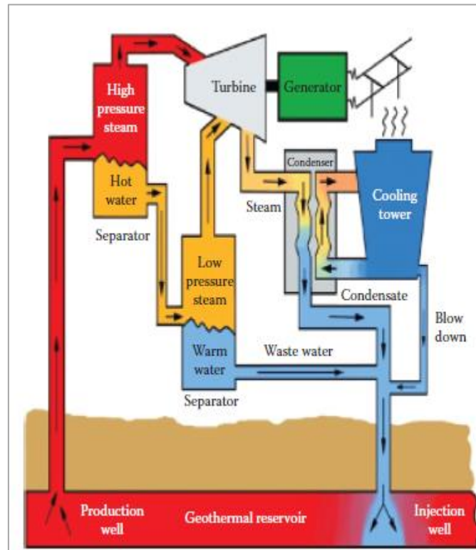
Figure 13: The configuration of binary plant for geothermal power generation (Boden, 2017).
