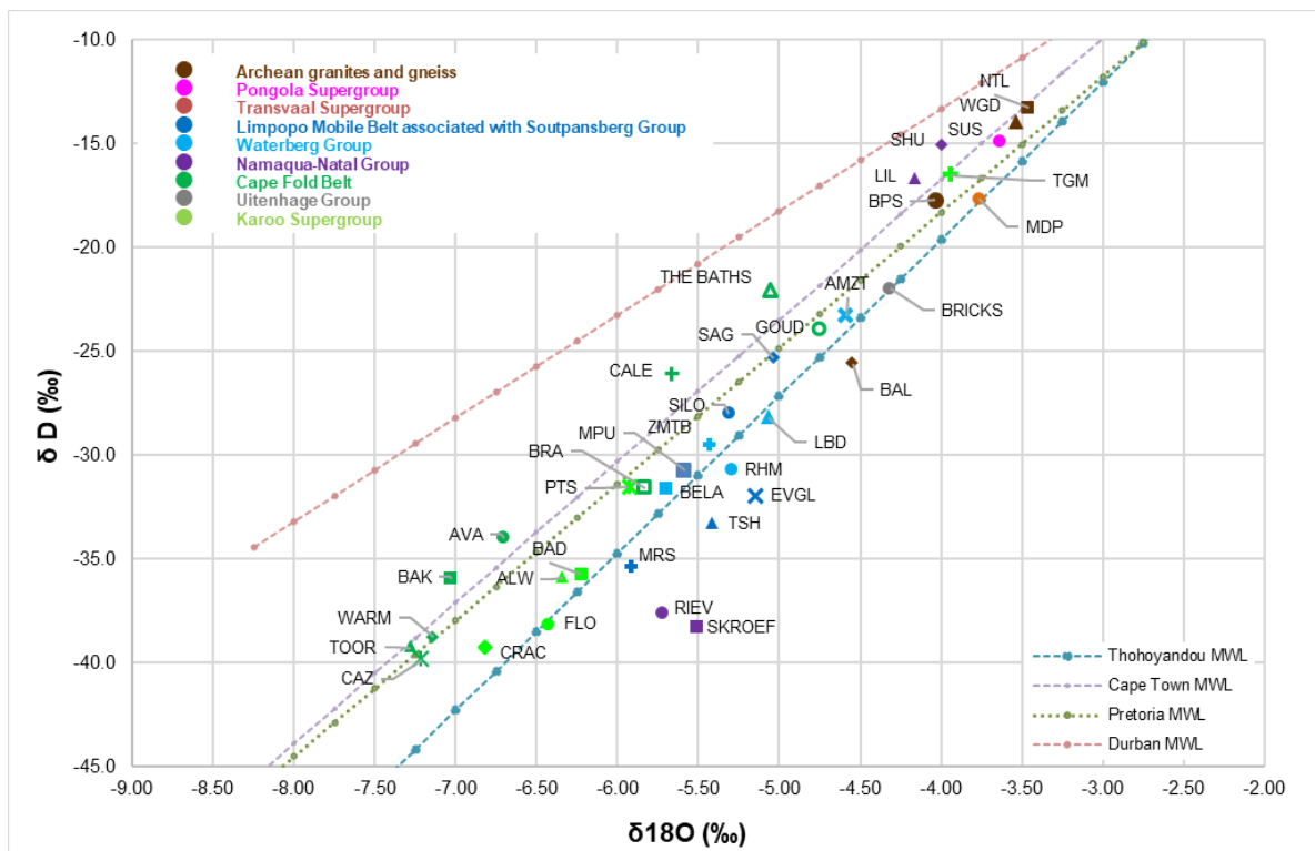
Figure 29: A plot of \delta\text{D} versus \delta^{18}\text{O} for the sampled geothermal waters, Local Meteoric Water Line (LMWL). The geothermal waters are colour coded per geological domain.
