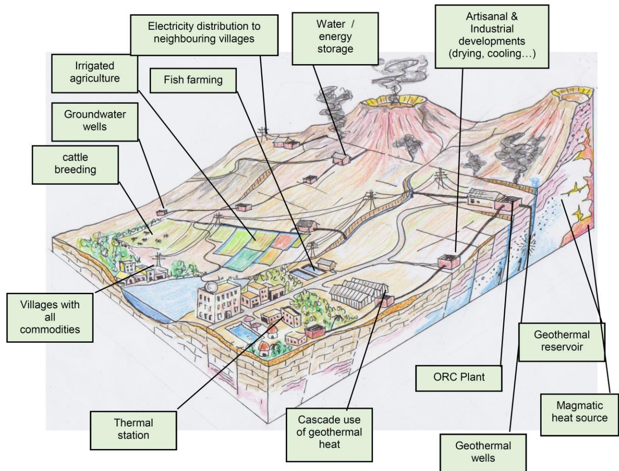
Figure 40: Schematic diagram of a conceptual model for harnessing geothermal energy in a cascading manner (Onyango and Varet, 2014).
