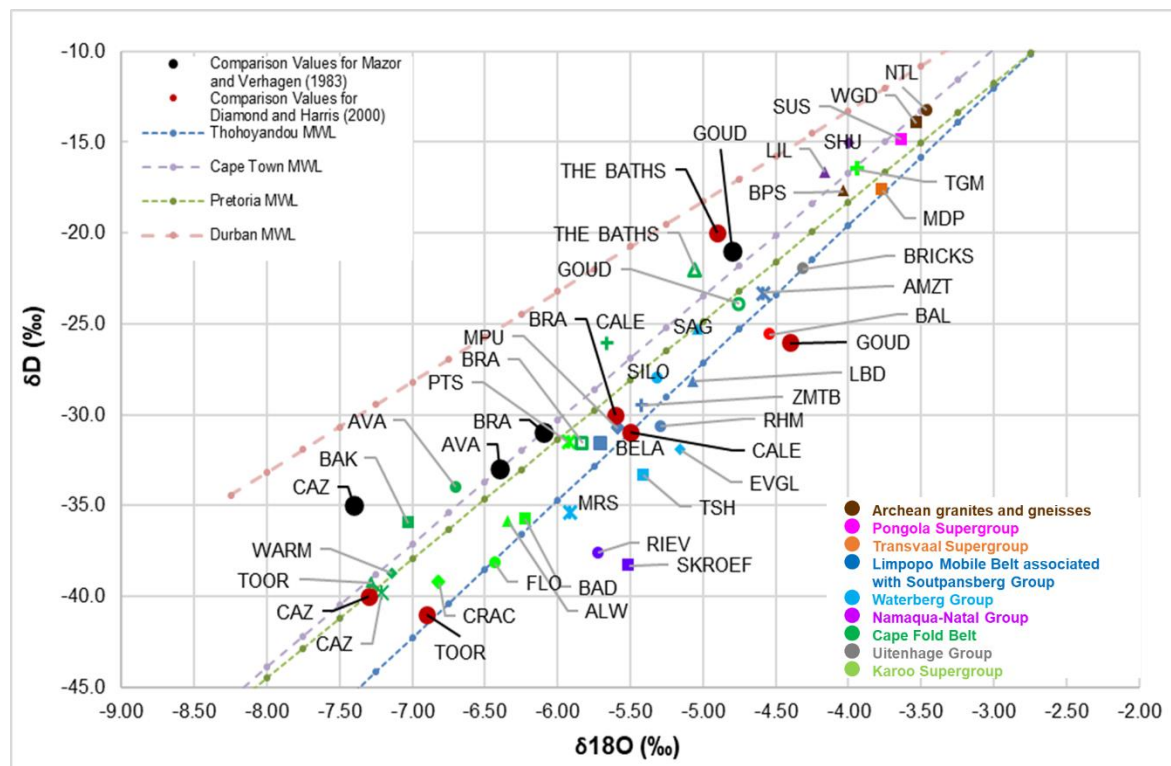
Figure 38: A plot of \delta\text{D} versus \delta^{18}\text{O} for the South African geothermal waters and the Local Meteoric Water Line (LMWL). Previous isotope analyses plotted in red (Diamond and Harris, 2000) and black (Mazor and Verhagen, 1983). Colour coded per geological domain.
