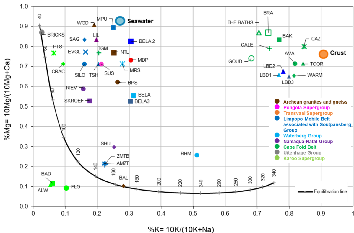
Figure 26: 10\text{Mg}/(\text{Mg}+\text{Ca}) versus 10\text{K}/(10\text{K}+\text{Na}) binary plot (Baoumy et al., 2015), of geothermal waters that were sampled for this study. The black line displays the equilibration line at various temperatures. The geothermal waters are colour coded per geological domain.
