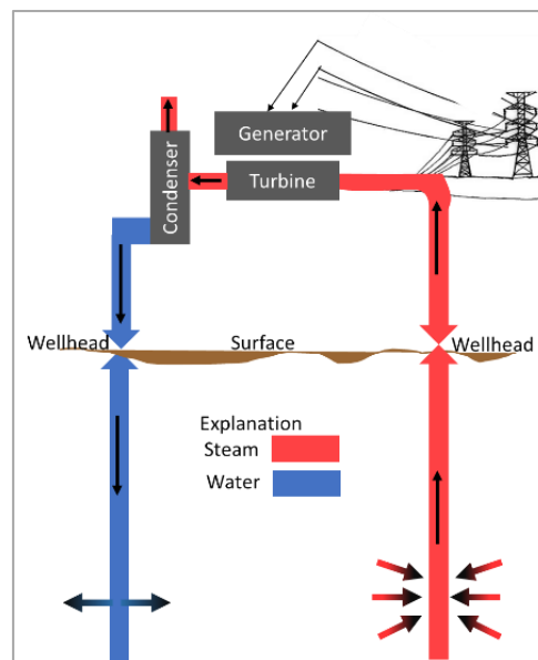
Figure 11: The configuration of dry steam for geothermal power generation (Boden, 2017).
