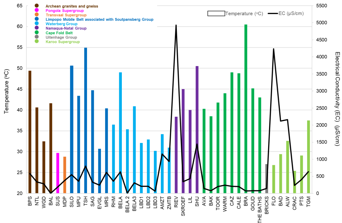
Figure 20: Illustration showing the inverse correlation of temperature (°C) (measured at surface manifestations) versus the electrical conductivity (EC) of the geothermal waters. The geothermal waters are colour coded per geological domain.
