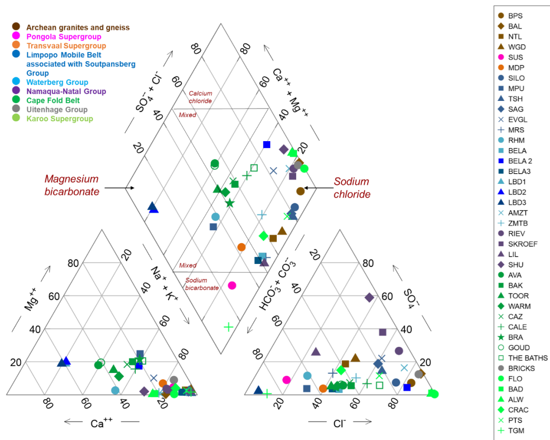
Figure 23: Piper diagram of the sampled geothermal waters in South Africa showing the cation and anion concentrations based on hydrochemical analyses (Piper, 1944; Bethke et al., 2022). The geothermal waters are colour coded per geological domain.
