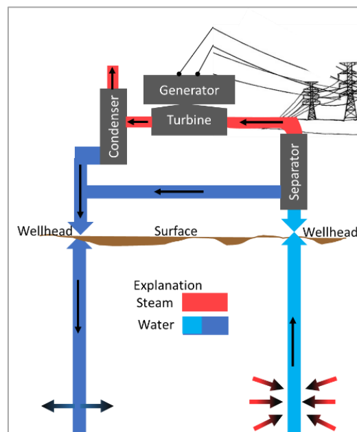
Figure 12: The configuration of flash plant for geothermal power generation (Boden, 2017).
