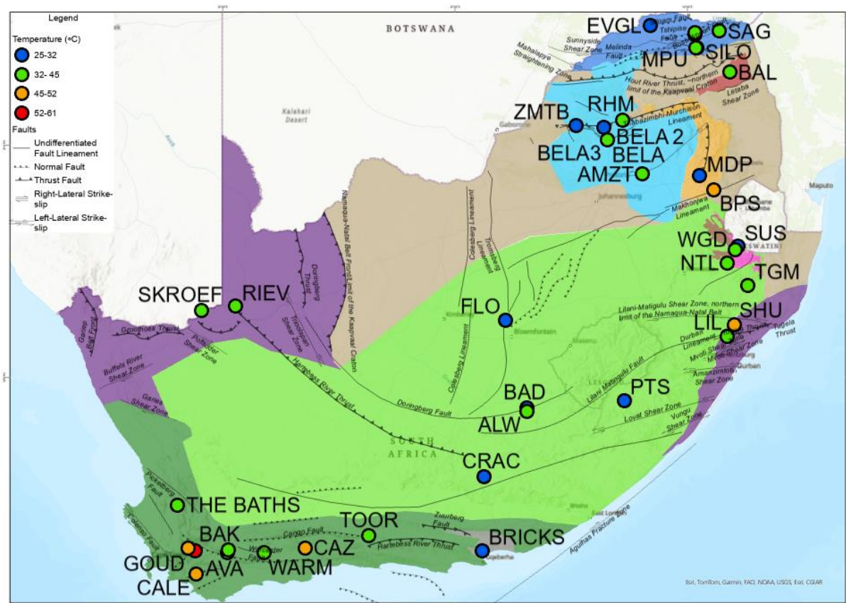
Figure 19: The geothermal waters in South Africa, underlying geology and tectonic domains (modified from Dhansay et al., 2017).
