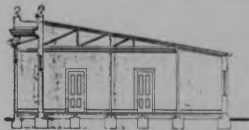
Section - El. 75
