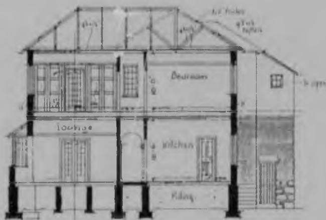
SECTION A.D.
