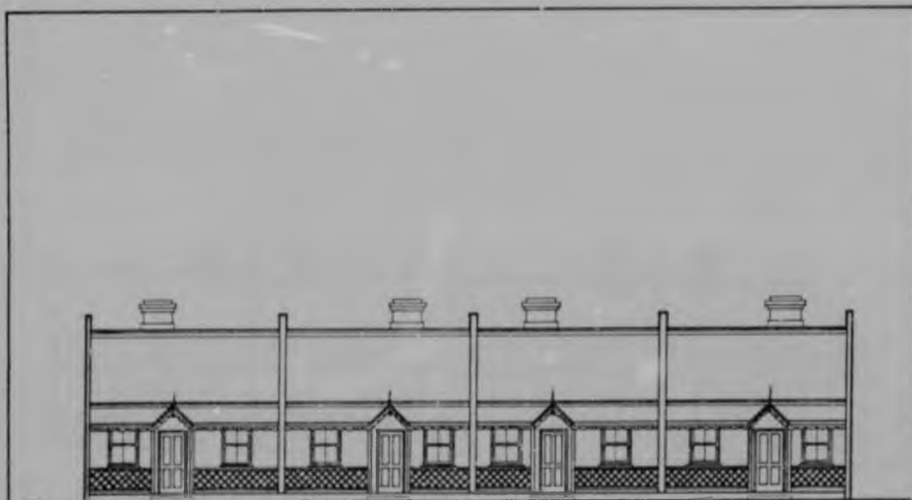
FRONT ELEVATION.
