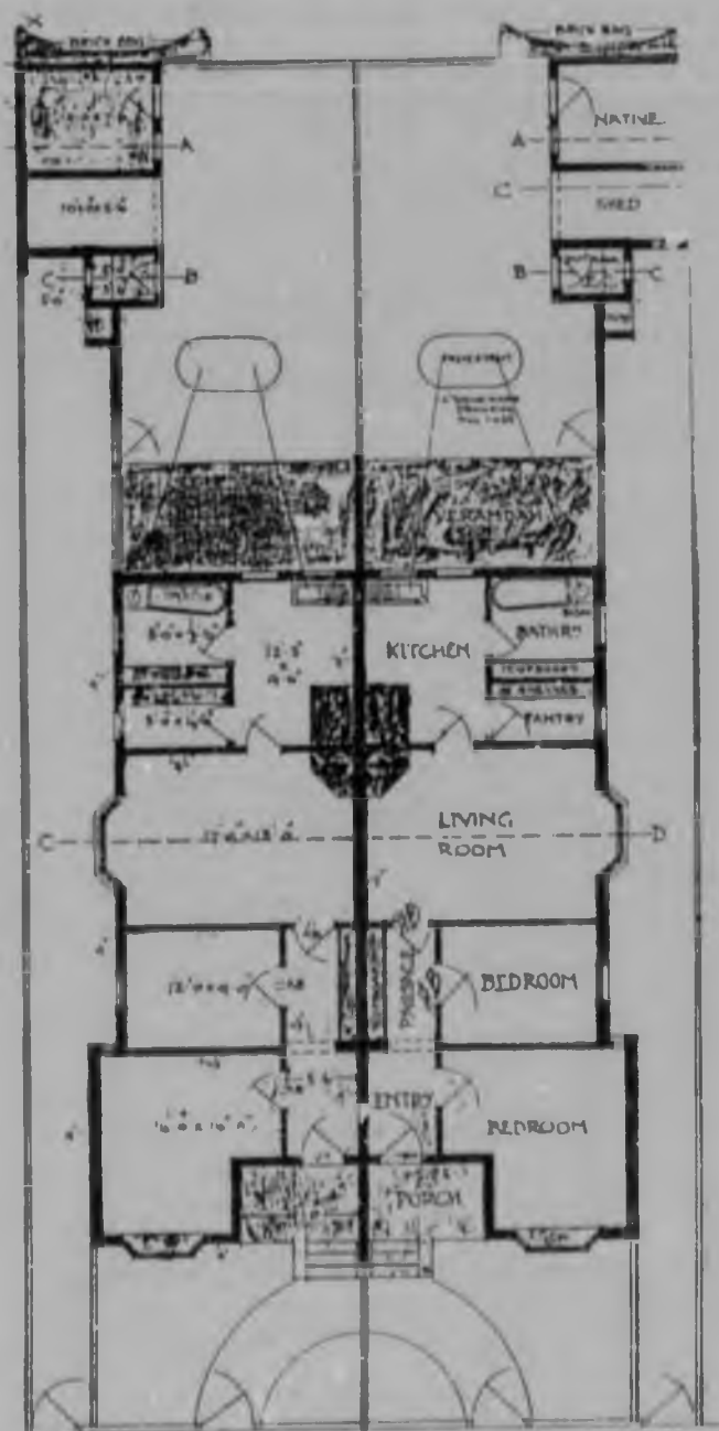
PLAN
