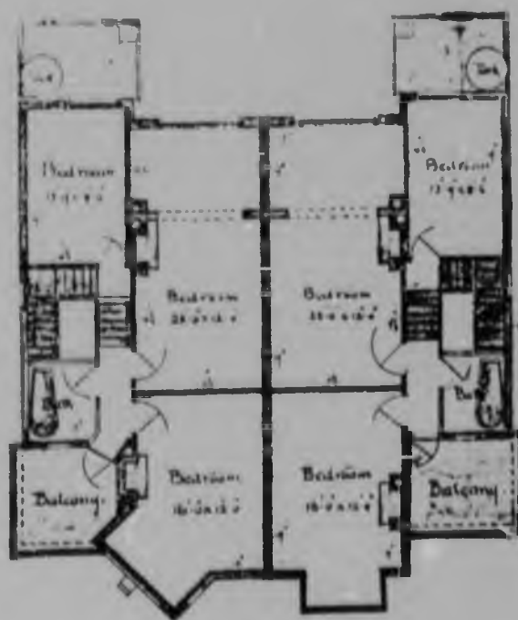
Plan of the First Floor
