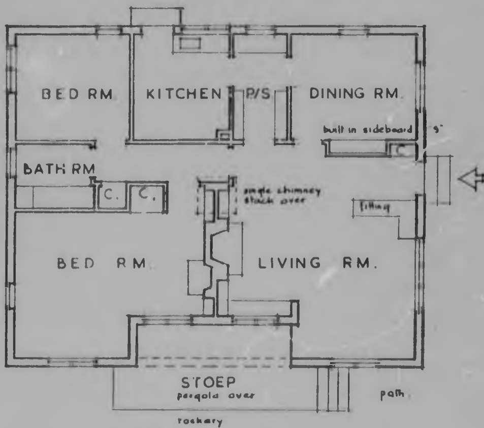
PLAN Scale 1/8" = 1 FT
