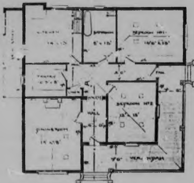
— GROUND PLAN —
