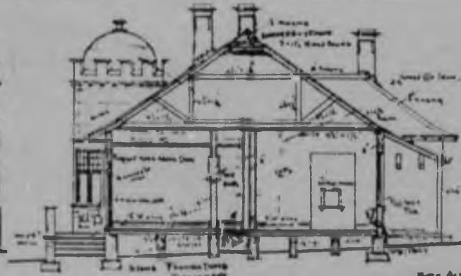
SECTION E.F.
