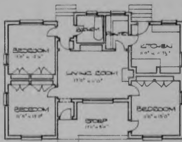
GROUND PLAN
