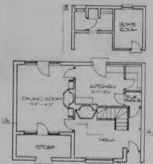
GROUND PLAN
