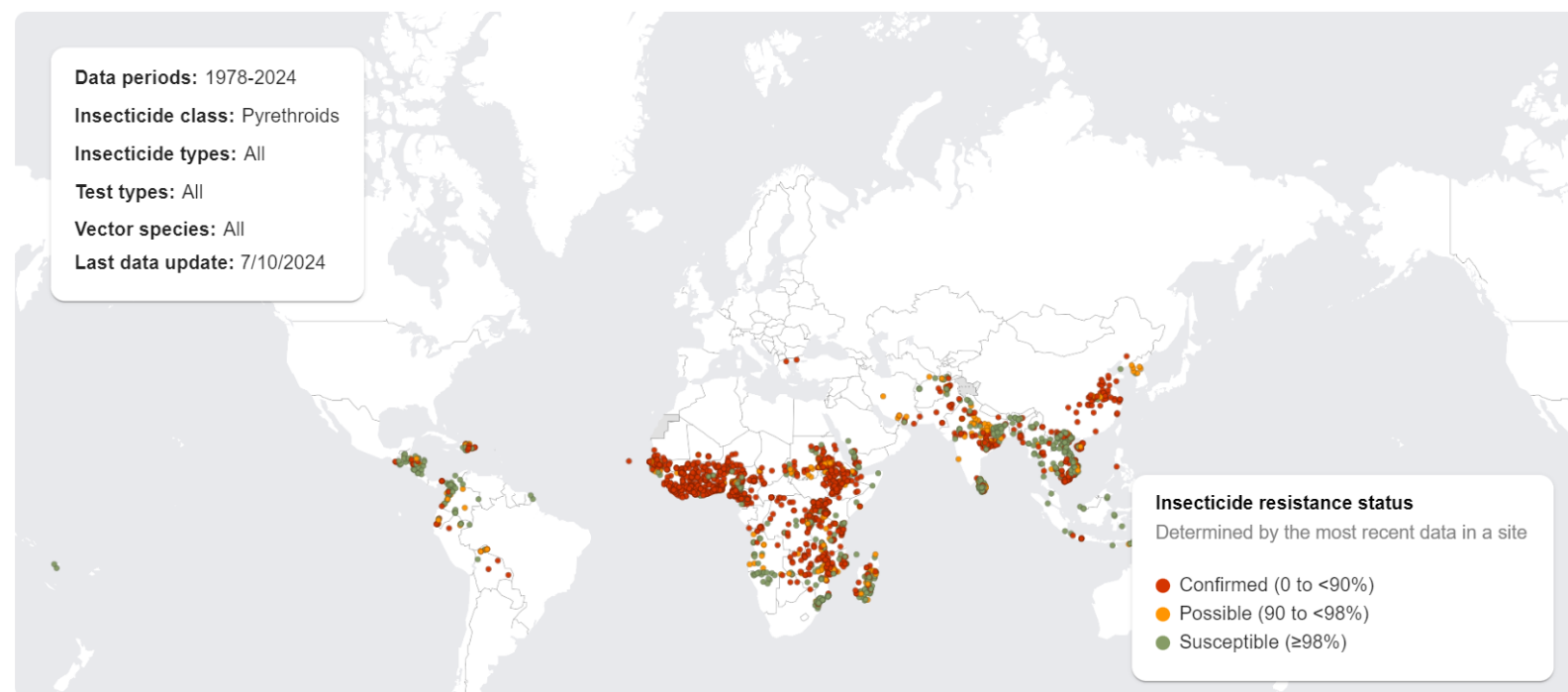
Figure 4.1. Global incidence of pyrethroid resistance between 1978 and 2023 occurring in Anopheles vector species (World Health Organization, 2024a).
