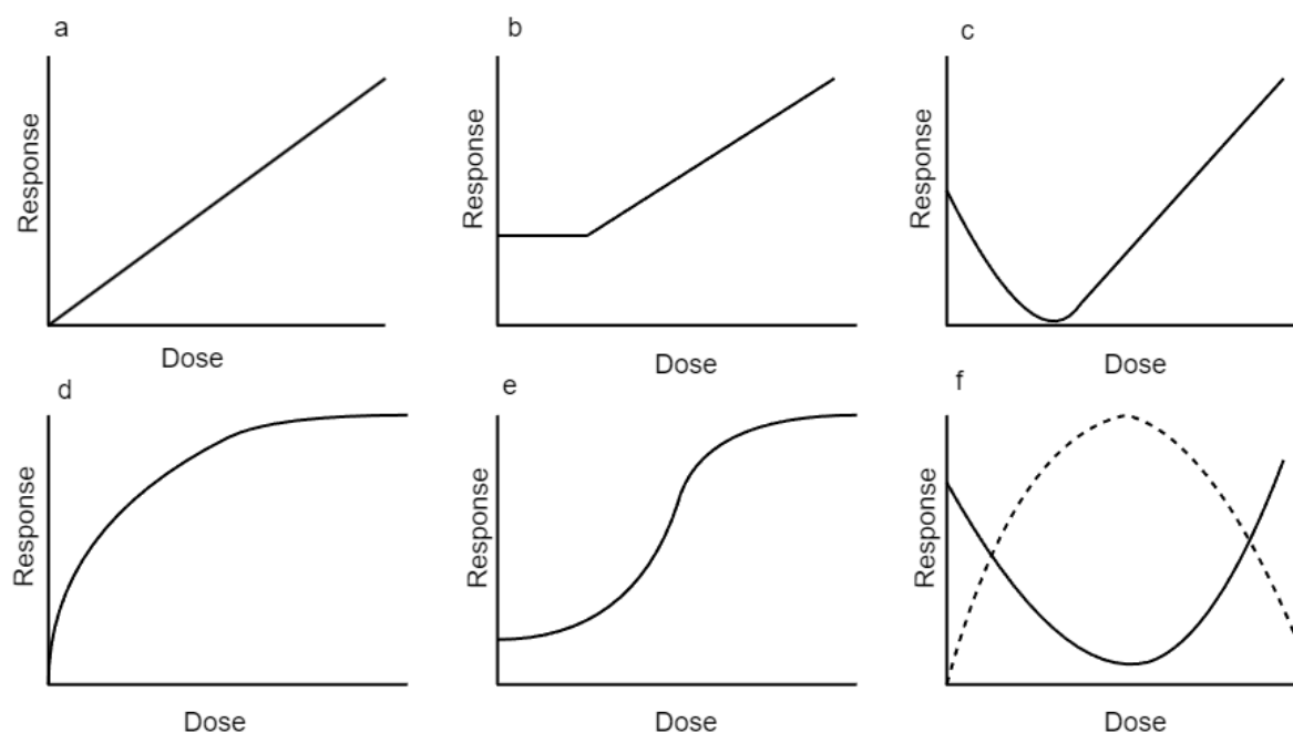
Figure 5.1. Most common dose-response curves in toxicology.
