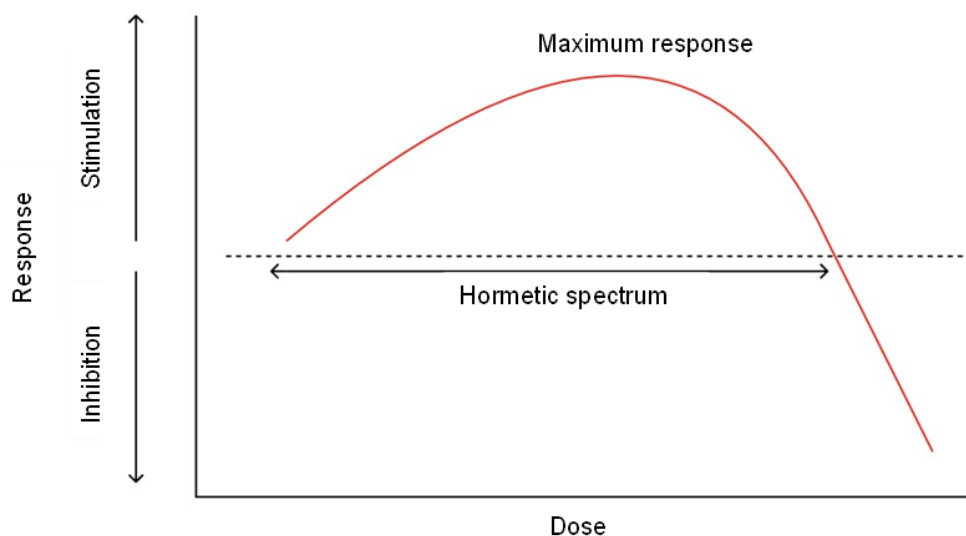
Figure 5.2. Schematic diagram of a hormetic response.
