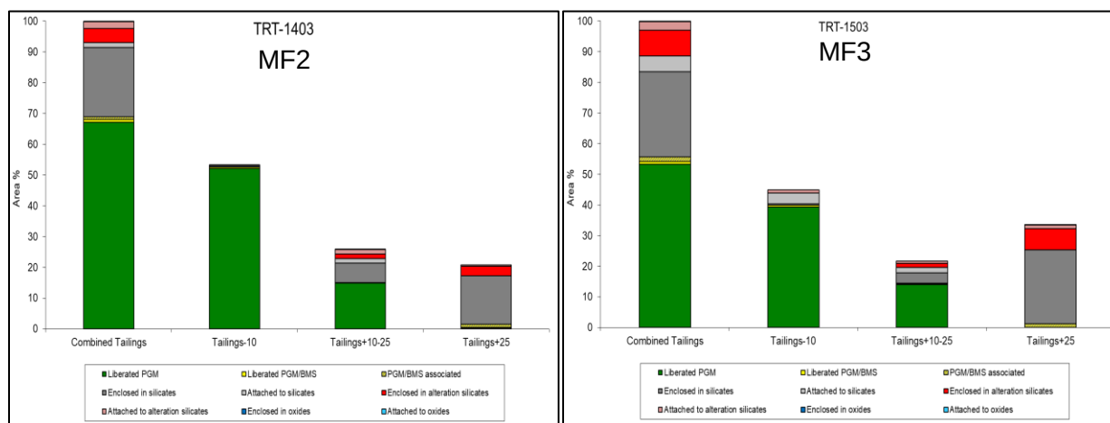
Figure 4.10: PGM association for sized tailings from different circuit configurations
