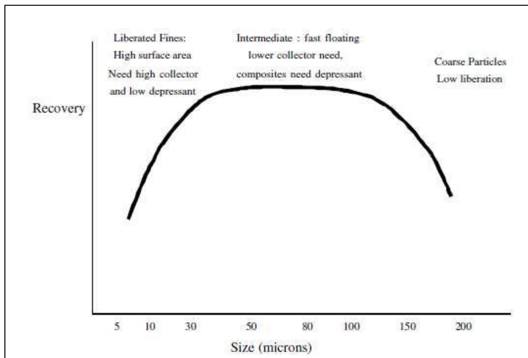
Figure 2.10: The conventional view (Pease et al 2006)
