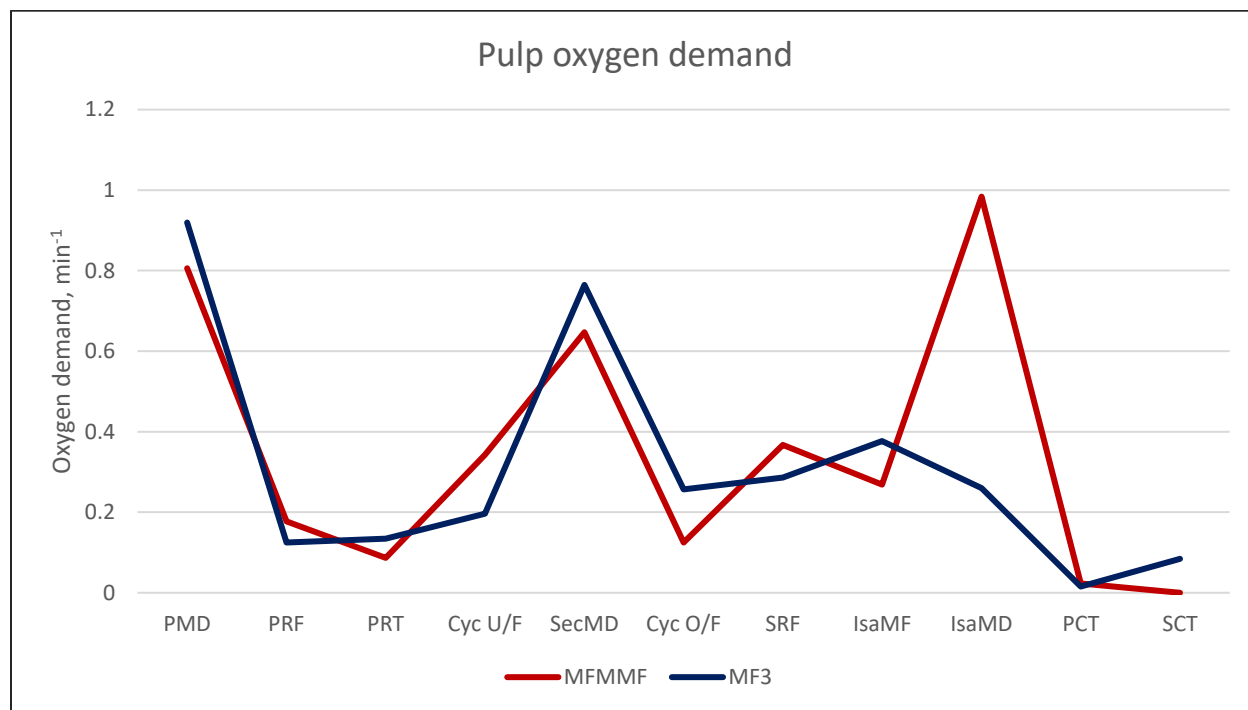
Figure 4.22: Oxygen demand of the different process streams
