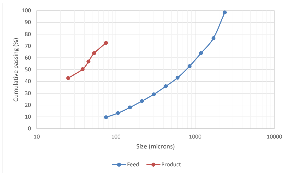
Figure 4.1: Feed and product size distribution profile
