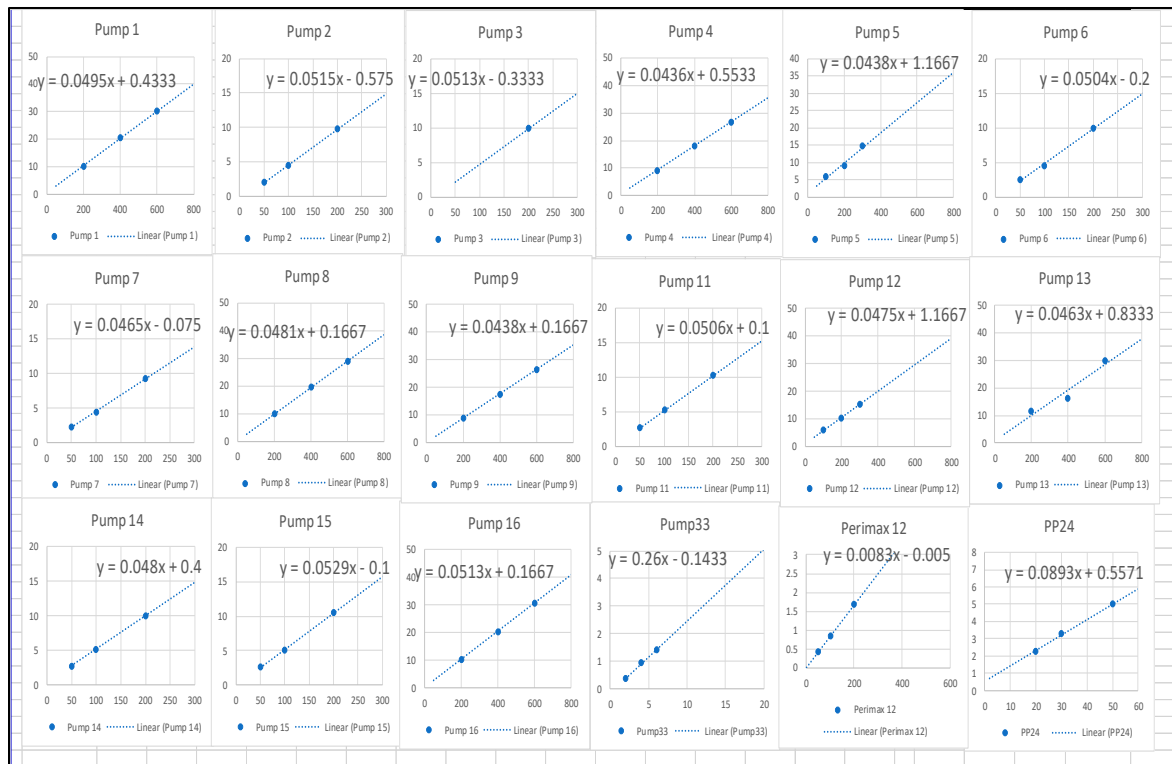
Figure 7.1: Flexi-float pump calibration
