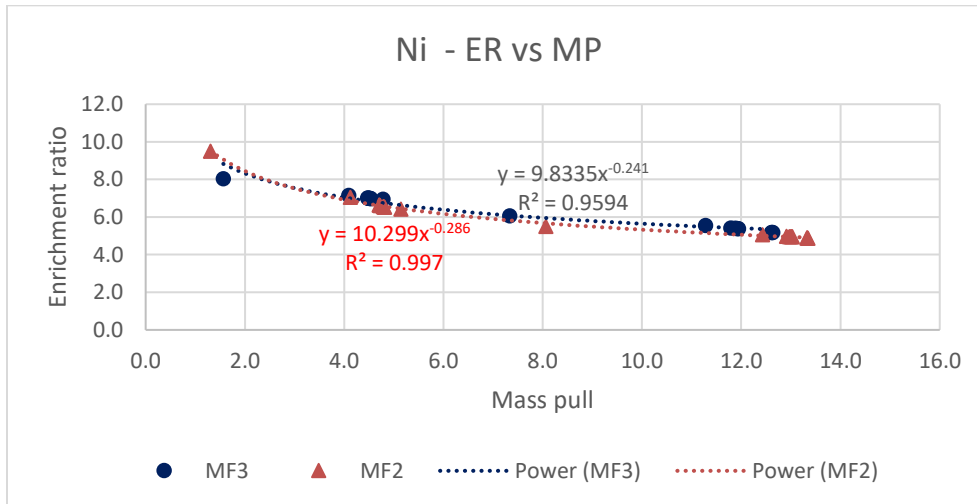
Figure 4.14: Nickel Enrichment ratio vs mass pull relationship
