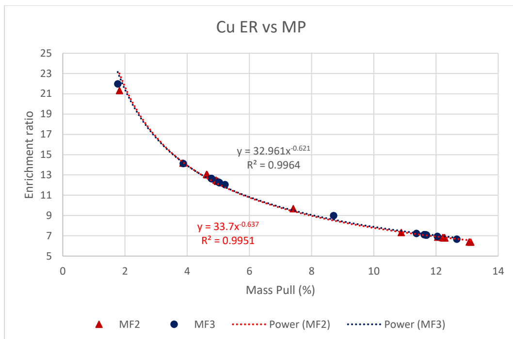
Figure 4.9: Enrichment ratio vs mass pull relationship
