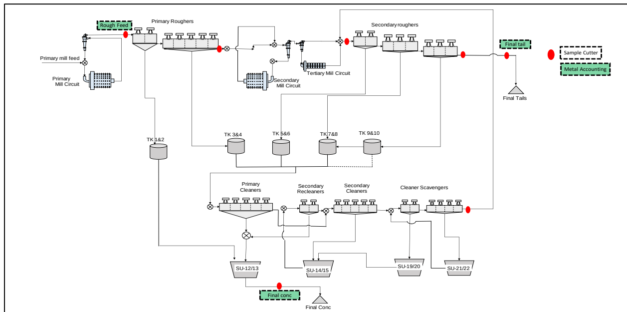
Figure 2.1: Mogalakwena North Concentrator current wet circuit configuration
