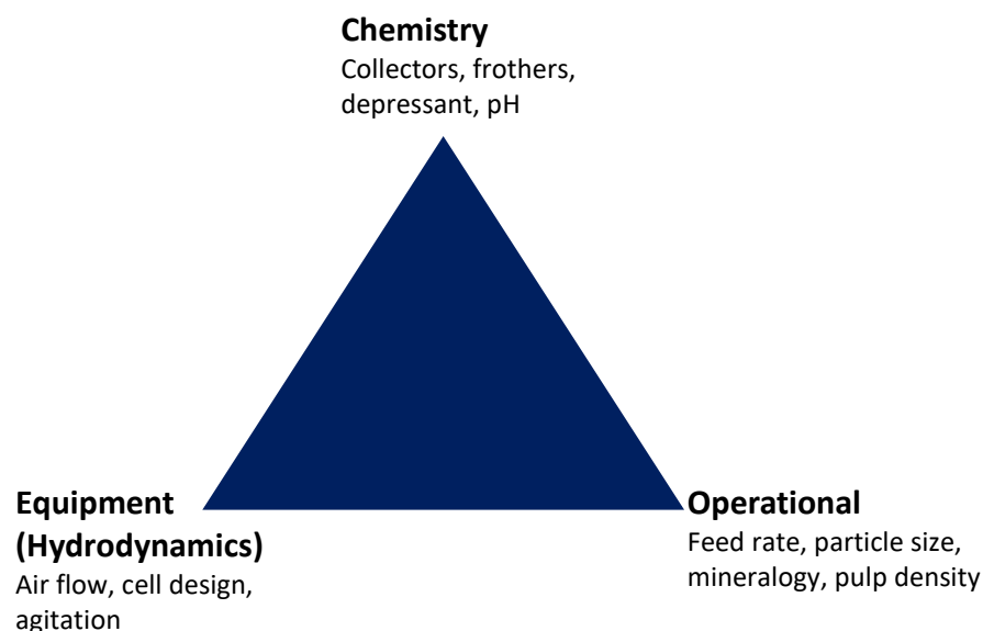
Figure 2.8: Categories of critical flotation parameters (Klimpel, 1984)
