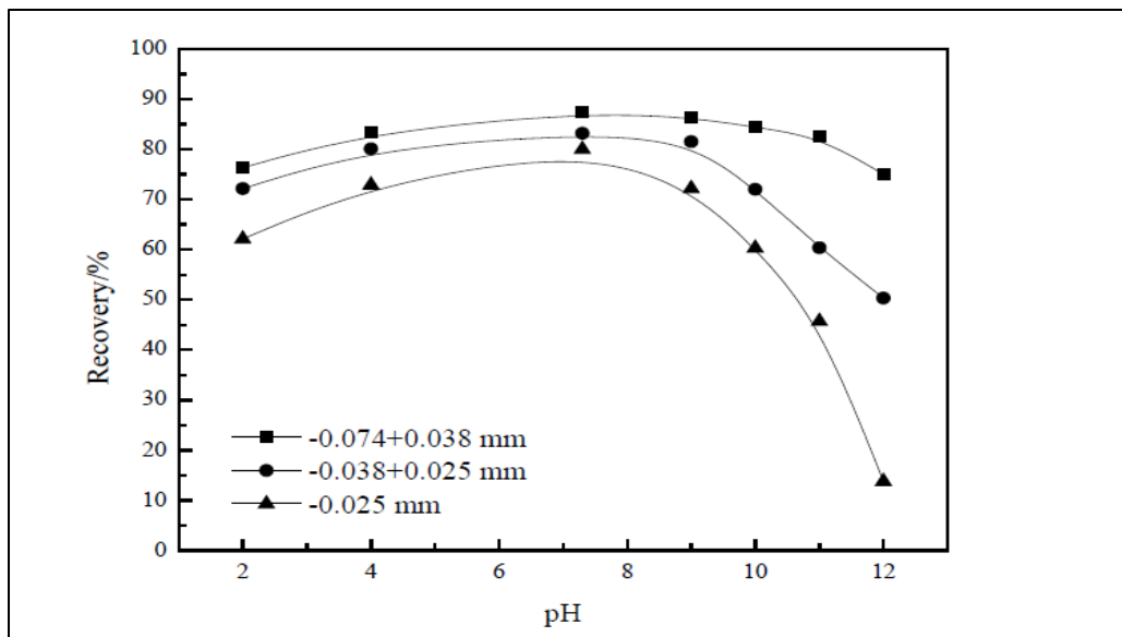
Figure 2.17: Flotation behavior of the three different size fractions of galena (Lu et al, 2018)
