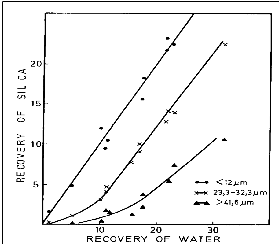
Figure 2.13: Size by size recovery in relation to water recovery (Engelbrecht and Woodburn, 1975)
