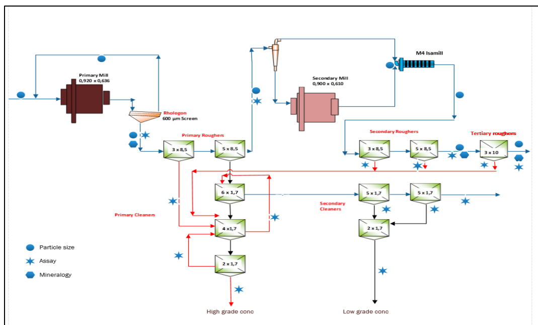
Figure 3.2: Flexi-float MF2 circuit sampling points and analysis conducted
