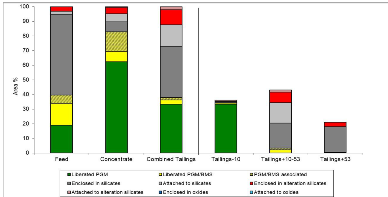
Figure 2.7: Benchmark Mineralogical Investigation of Mogalakwena North Concentrator –March 2018
