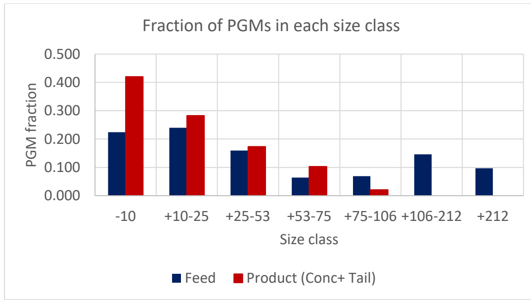
Figure 2.3: PGM fraction per size class for the feed and product streams
