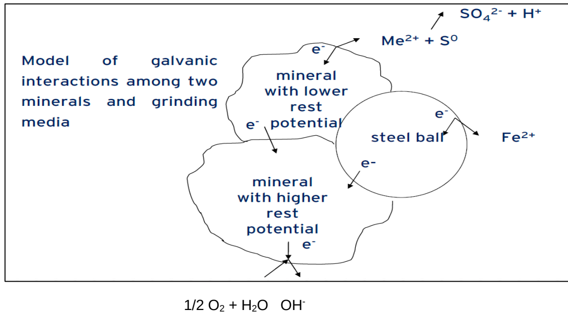
Figure 2.16: Galvanic interactions model (Greet, 2019)
