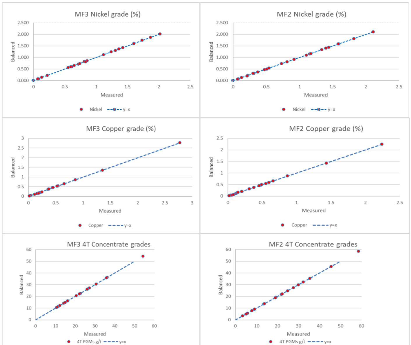
Figure 7.2: Campaign 3 data integrity
