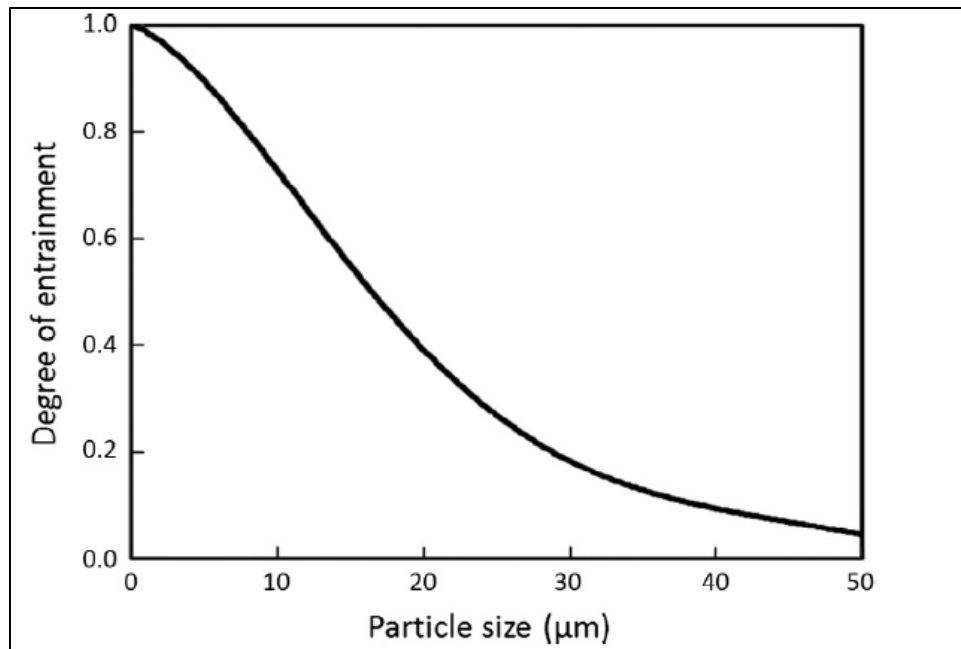
Figure 2.14: The relationship between degree of entrainment and the particle size for hydrophilic silica in a laboratory flotation cell (Bisshop, 1974)
