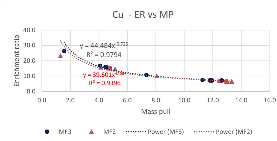
Figure 4.15: Copper Enrichment ratio vs mass pull relationship
