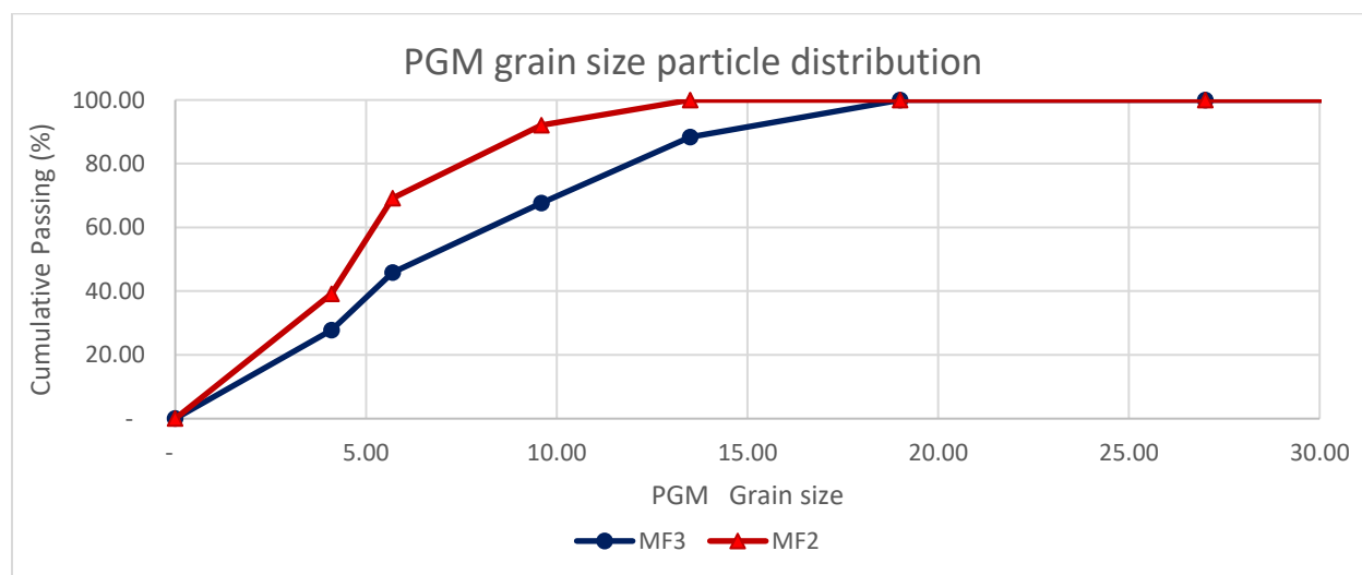
Figure 4.16: Particle size distribution comparison of the tailings streams
