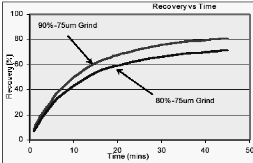
Figure 2.15: Rougher Recovery vs time (Anyimadu et al, 2006)
