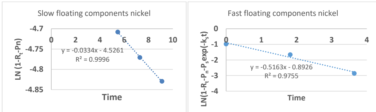
Figure 4.21: Nickel flotation rate constants
