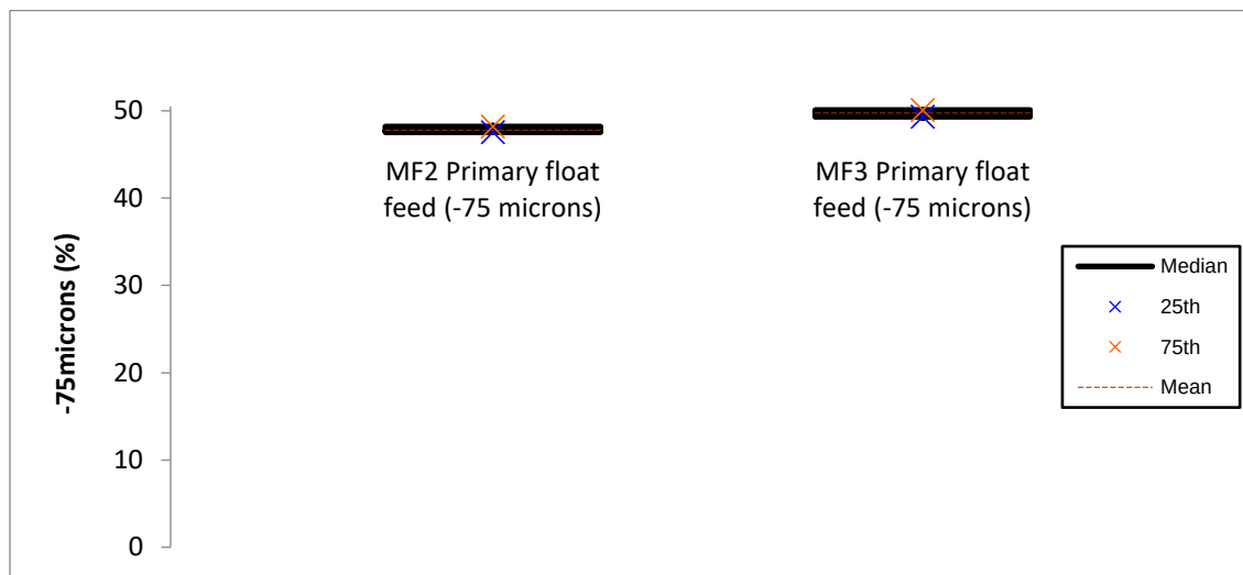
Figure 4.3: Primary mill grind cumulative passing 75 microns
