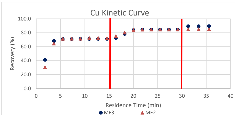
Figure 4.13: Campaign 2 Copper kinetic curve for the different configurations
