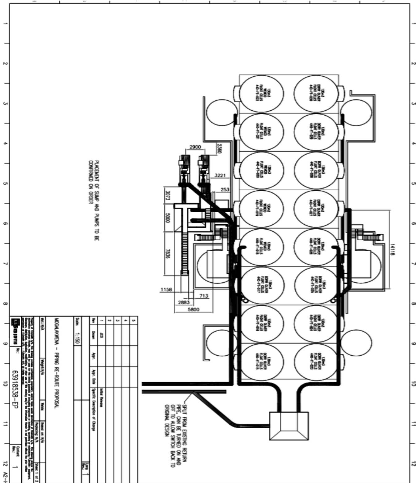
Figure 7.6: Proposed plant layout for secondary roughers and tertiary roughers
