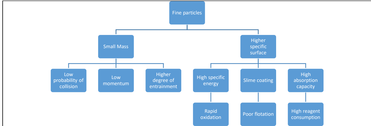
Figure 2.12: Fine particles and their behavior in flotation (Mugadza, 2015)
