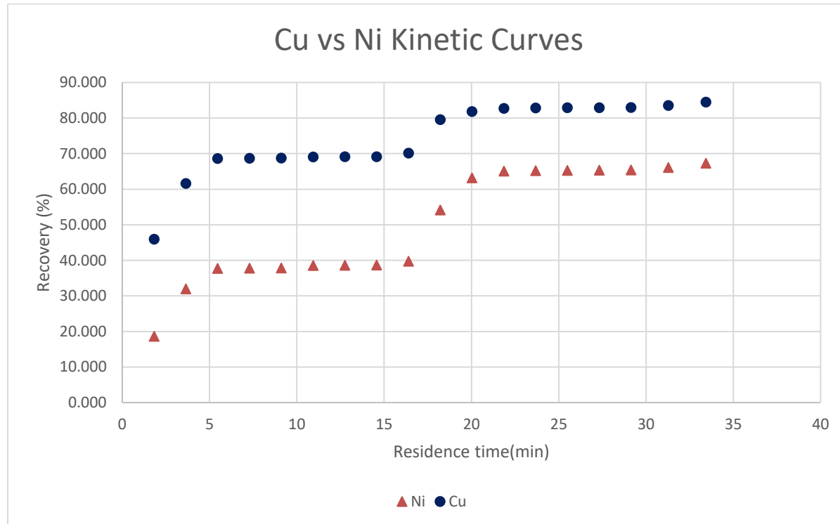
Figure 4.19: Comparison of copper and nickel kinetics
