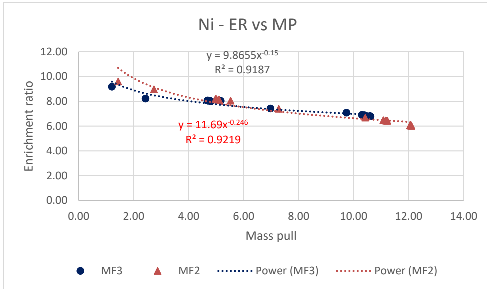
Figure 4.17: Nickel Enrichment ratio vs mass pull relationship
