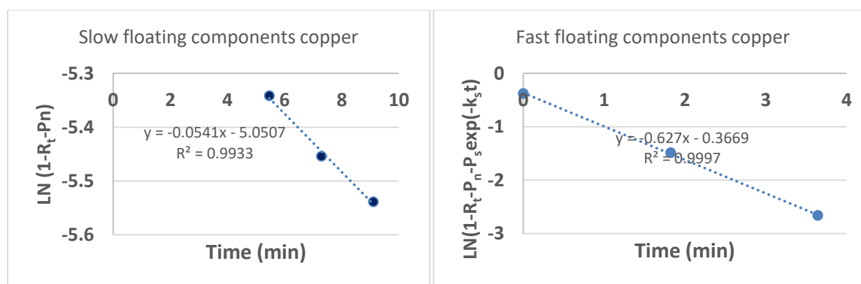
Figure 4.20: Copper flotation rate constants
