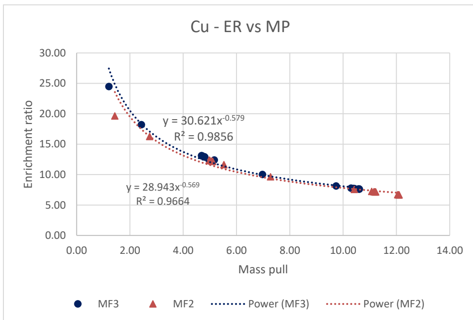
Figure 4.18: Copper Enrichment ratio vs mass pull relationship
