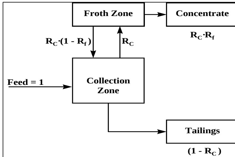
Figure 2.9: Interaction between zones in a flotation cell (Dobby et al, 1982)
