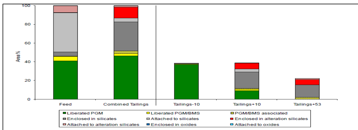
Figure 2.5: Benchmark Mineralogical Investigation of Mogalakwena North Concentrator –February 2017
