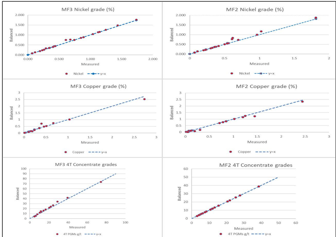
Figure 4.11: Campaign 2 mass balance data integrity
