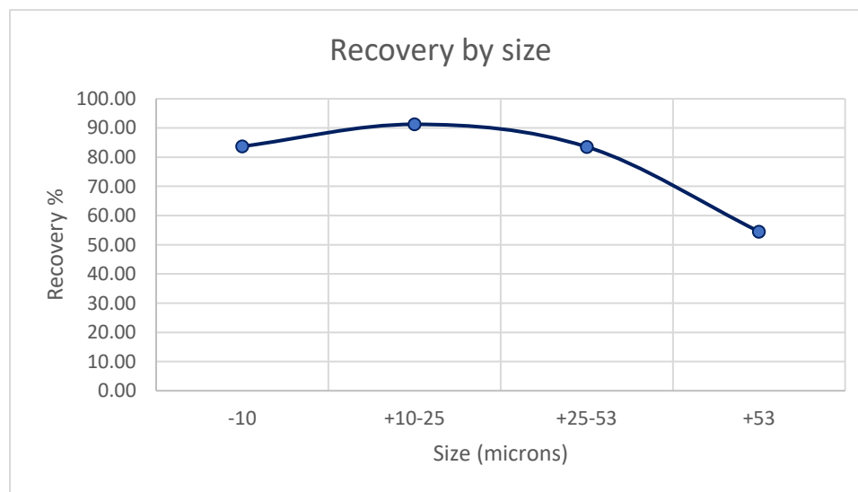
Figure 2.11: Recovery by size based on March 2018 performance
