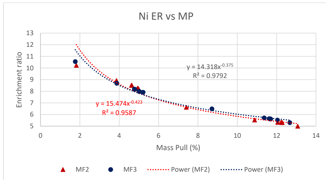
Figure 4.8: Enrichment ratio vs mass pull relationship
