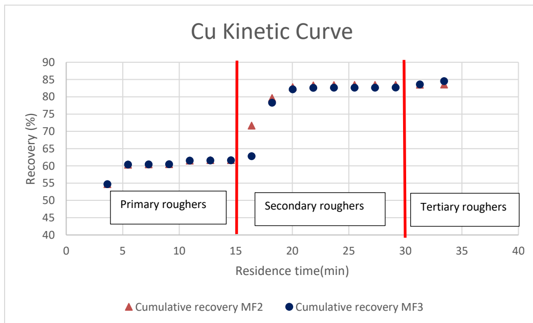
Figure 4.7: Copper kinetic curve for the different configurations
