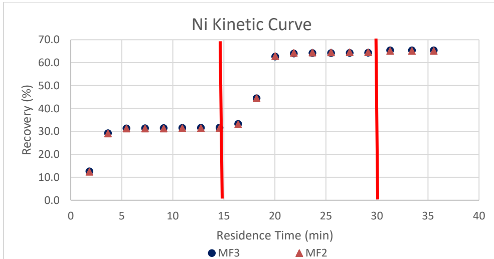
Figure 4.12: Campaign 2 Nickel kinetic curve for the different configurations
