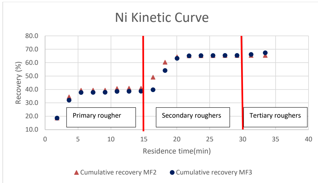
Figure 4.6: Nickel kinetic curve for the different configurations
