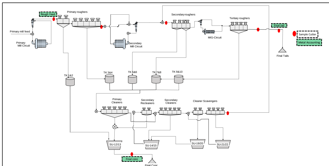
Figure 7.4: Proposed MF3 Circuit plant setup
