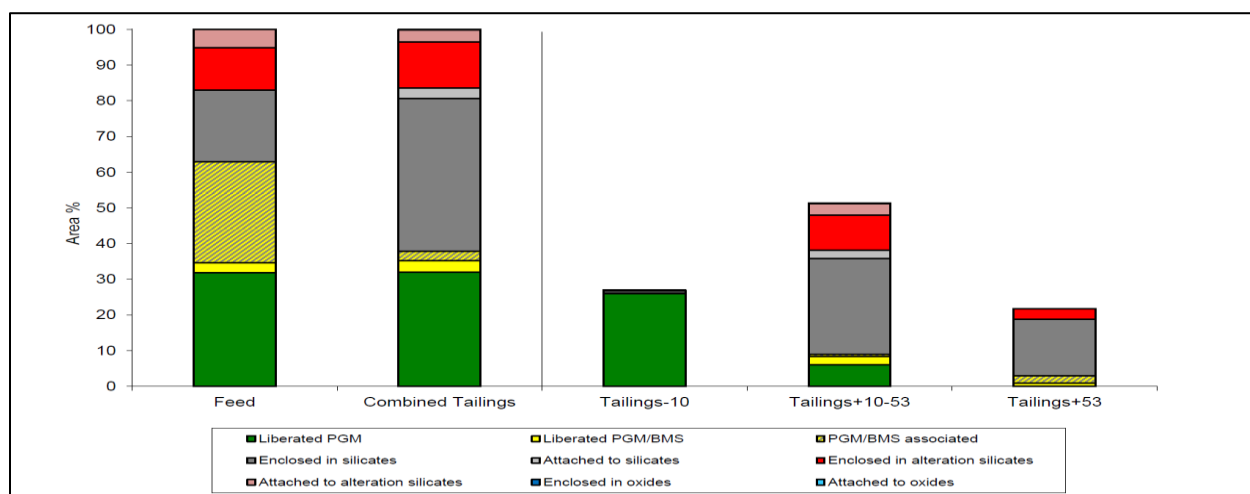
Figure 2.6: Benchmark Mineralogical Investigation of Mogalakwena North Concentrator –November 2017
