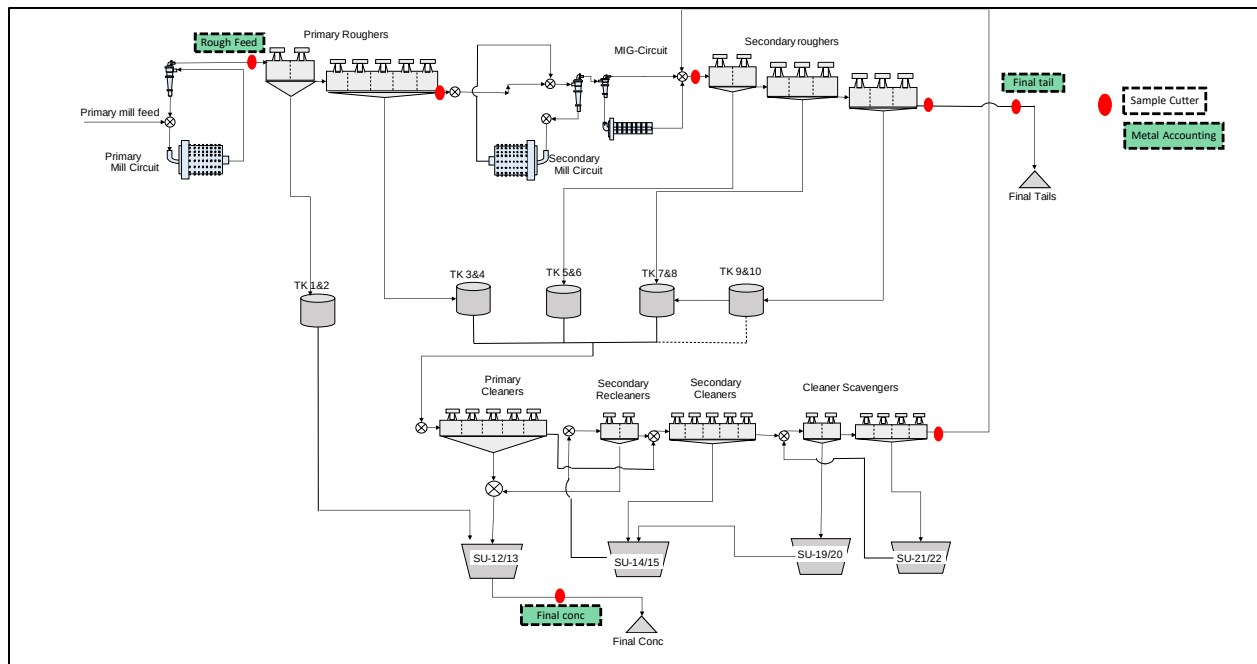
Figure 7.3: Current wet section plant setup
