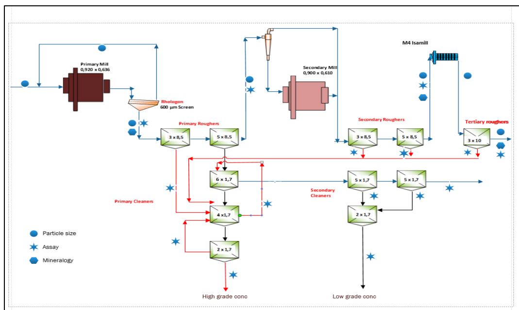
Figure 3.3: Flexi-float MF3 circuit sampling points and analysis conducted
