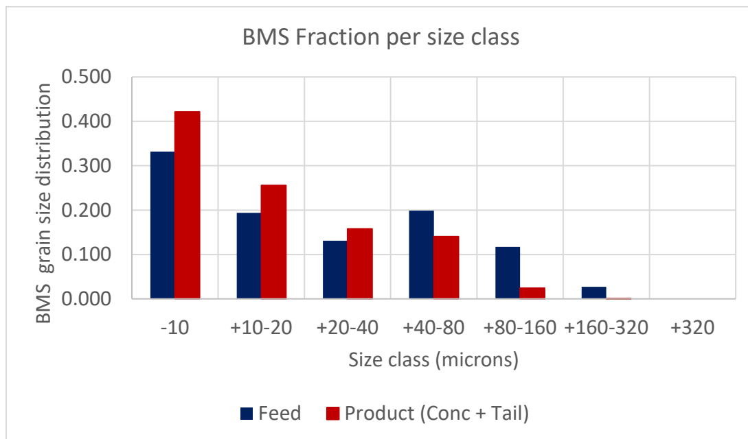
Figure 2.4: BMS fraction per size class in the feed and combined product stream
