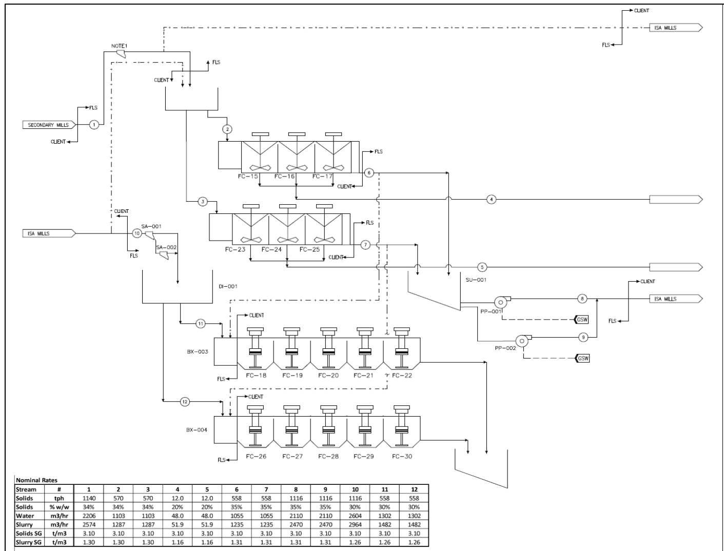
Figure 4.23: MF3 Secondary rougher setup at Mogalakwena North Concentrator
