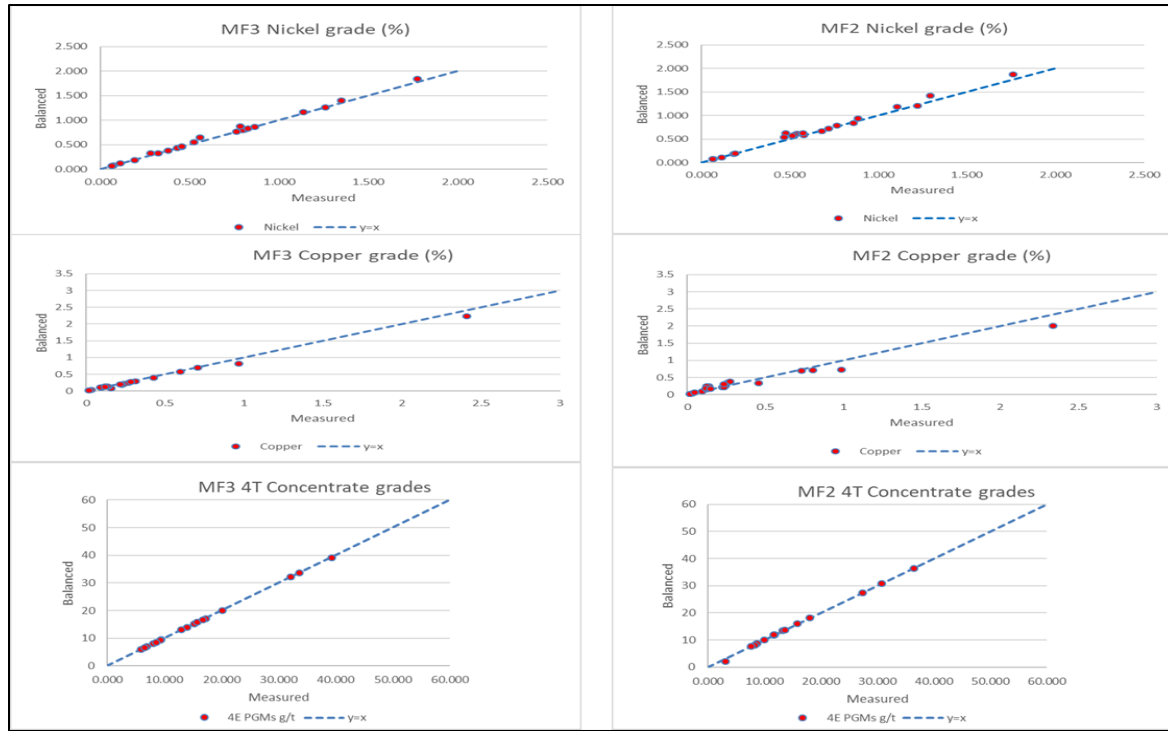
Figure 4.5: Campaign 1 mass balance data integrity
