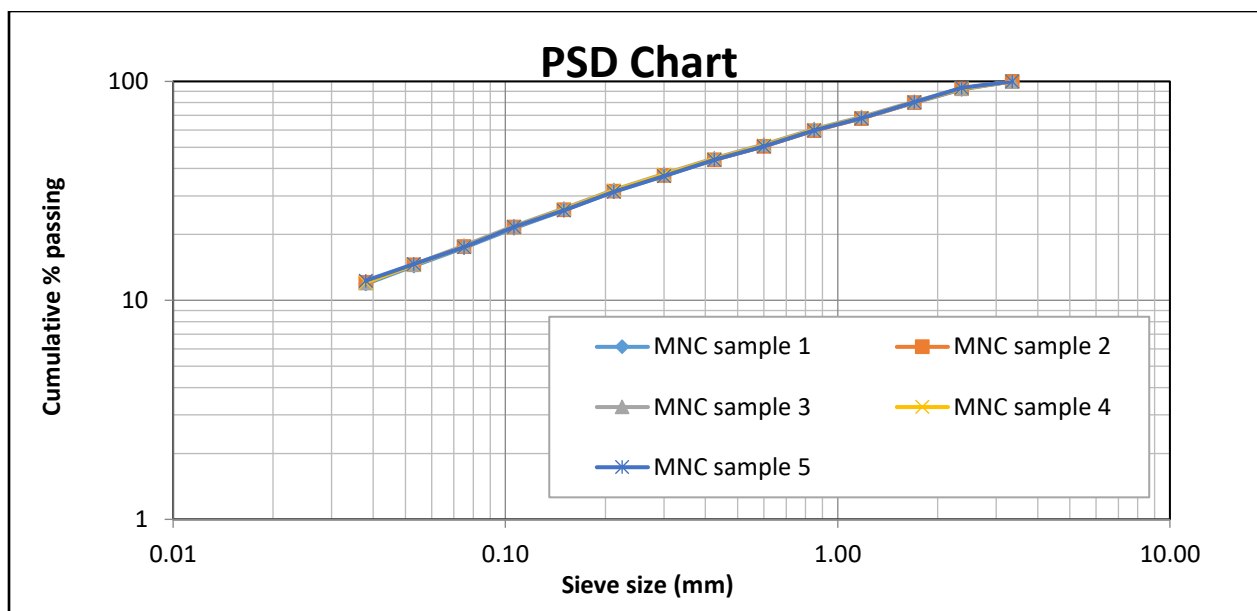
Figure 4.2: Particle size distribution of flexi-float feed
