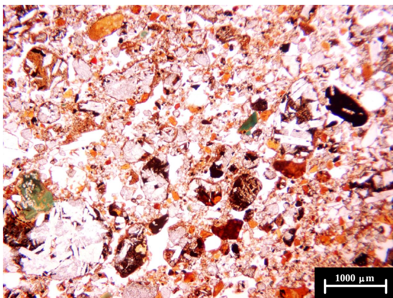
Figure 6.34 Coarse material with very little fine fractions taken in PPL in trench 3 at 150 cm depth.
