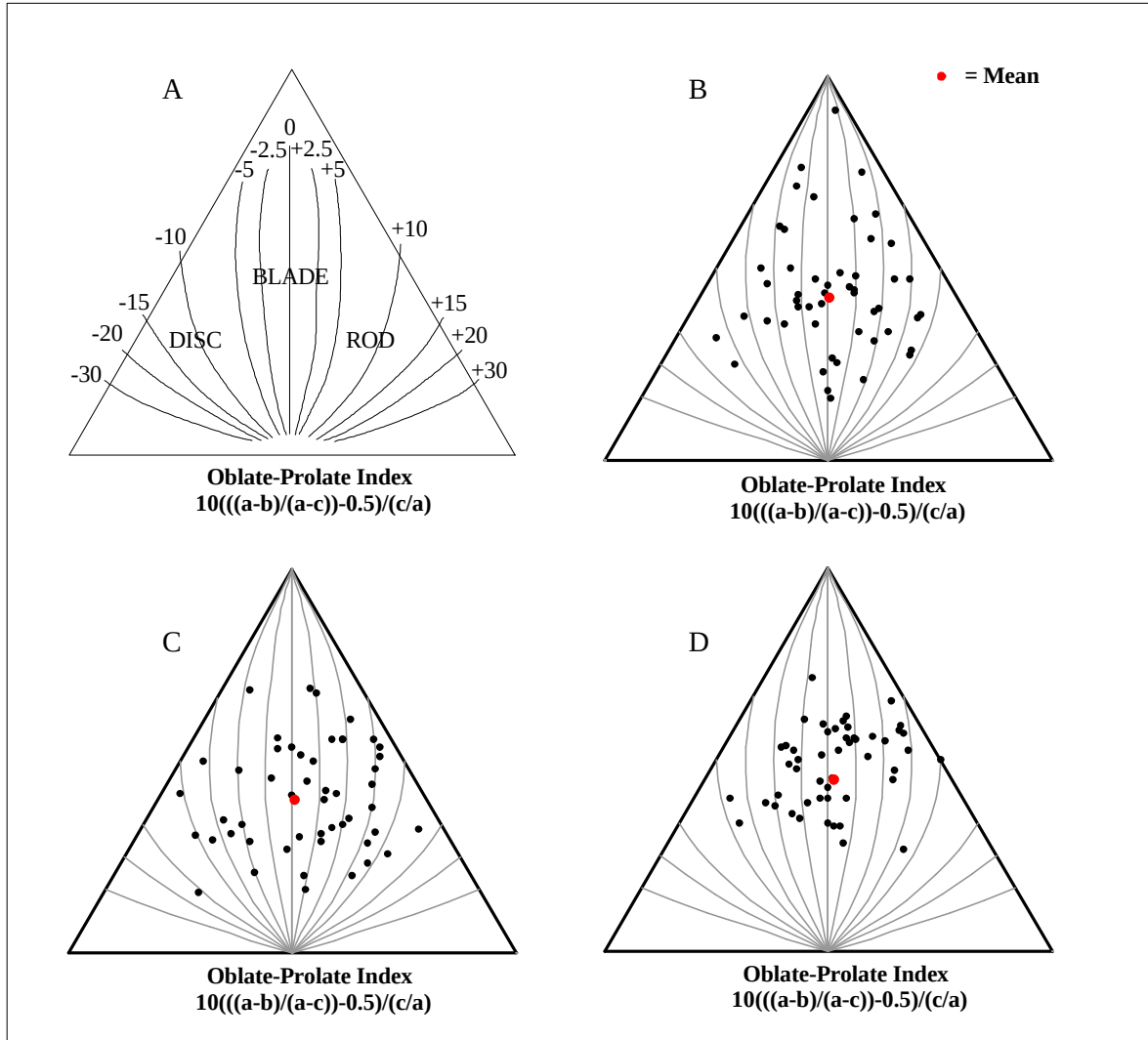
Figure 6.13 Triangular diagrams after Sneed and Folk (1958). (A) Isolines of the Oblate-prolate index according to Dobkins and Folk (1970). Triangular diagrams for Trenches 1, 2 and 3 respectively at Sekhokong Site 1 (n = 50).
