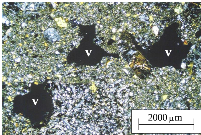
Figure 5.24 An example of typical vugh voids taken in XPL (cross polarized light) (v =voids).
