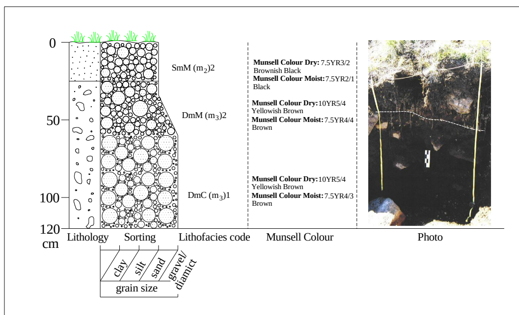
Figure 5.5 Sedimentological and stratigraphical data for trench 2 at Tsatsa-La-Mangaung.
