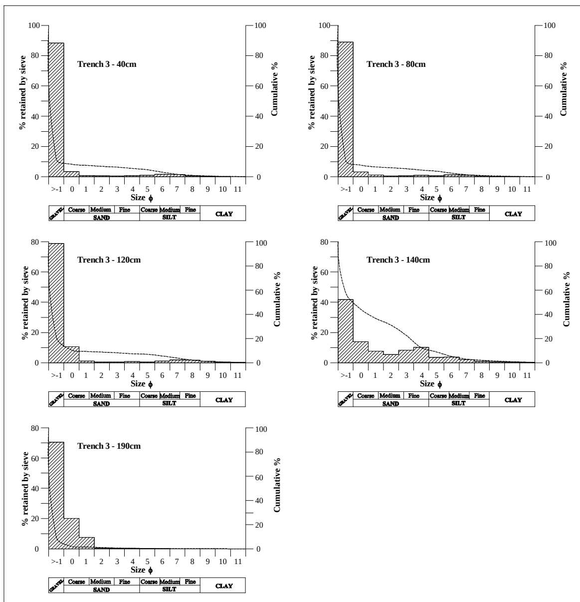
Figure 6.26 Grain size distributions for the sediment from trench 3 at Sekhokong Site 2.
