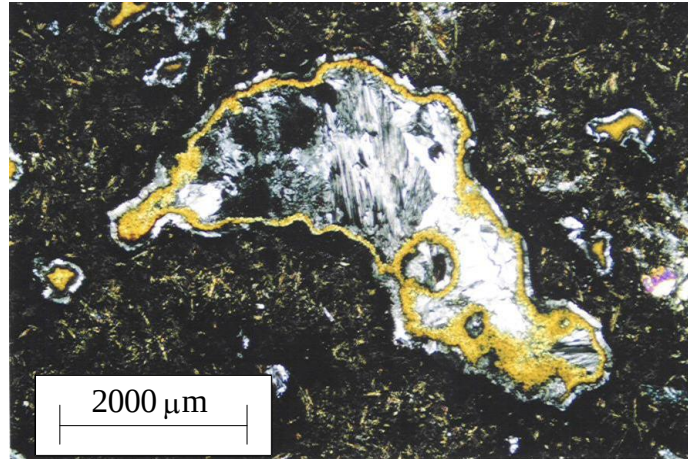
Figure 5.27 An example of an olivine crystal with a brown rim taken in XPL.
