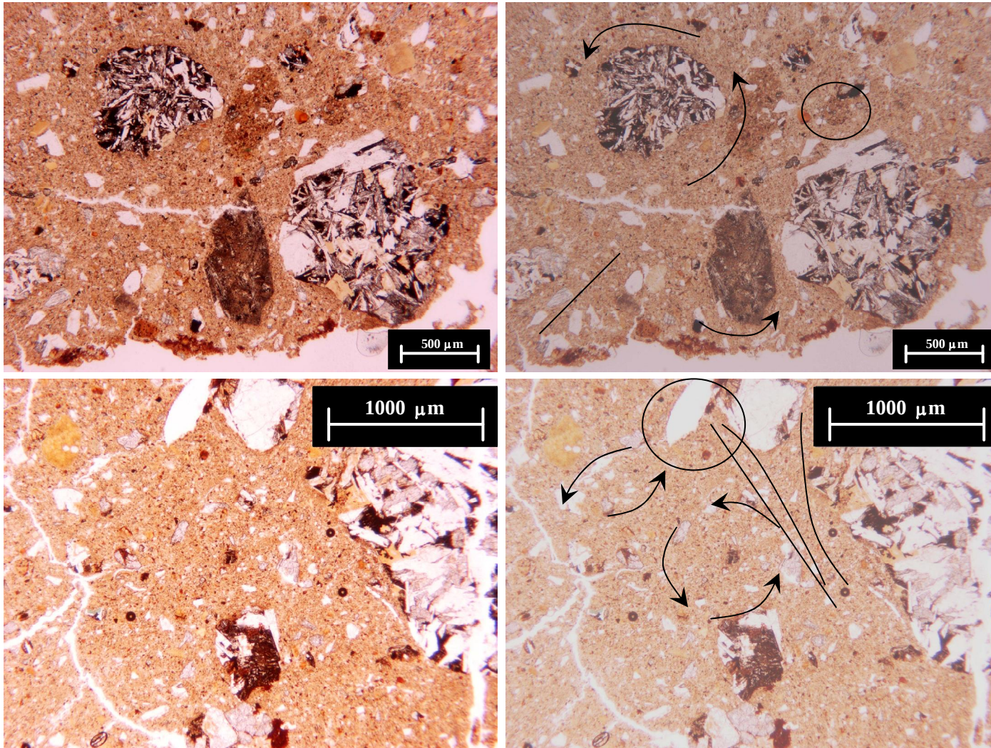
Figure 6.18 Rotation structures within trench 3 at 125 cm depth. Note images are paired with original and annotated versions.
