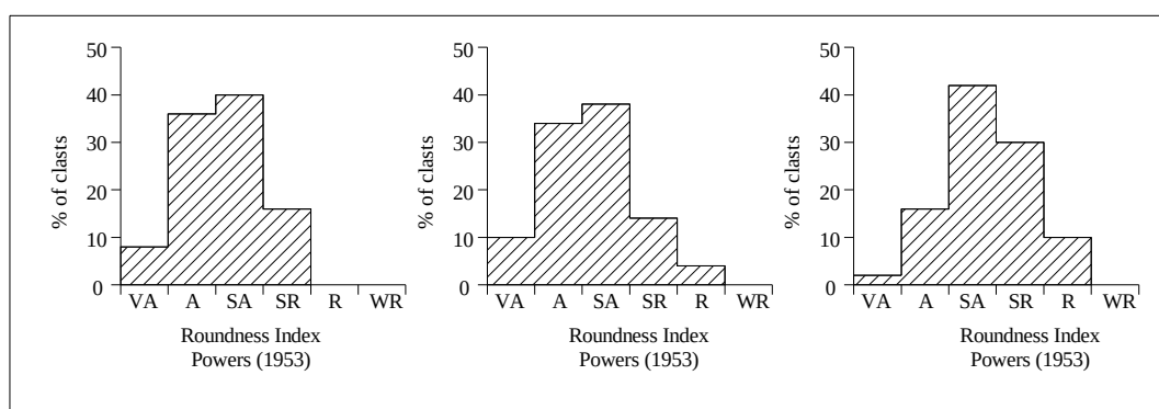
Figure 6.33 Graphs representing visual roundness of clasts (after Powers 1953) in trenches 1 (A), 2 (B) and 3 (C) at Sekhokong Site 2. VA = Very Angular, A = Angular, SA = Sub Angular, SR = Sub Rounded, R = Rounded, WR = Well Rounded. n = 50.
