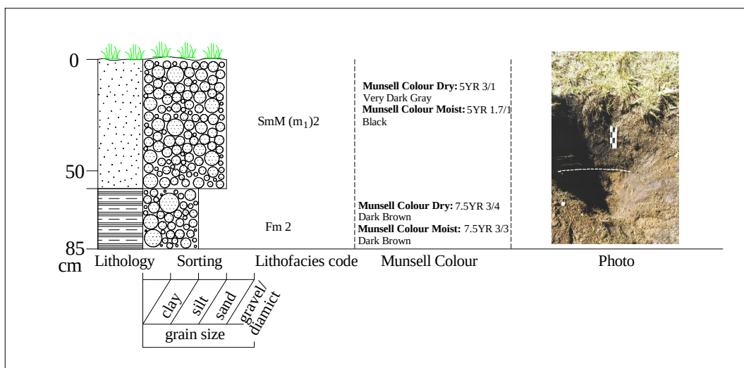
Figure 5.10 Sedimentological and stratigraphical data for Pit 4 at Tsatsa-La-Mangaung.
