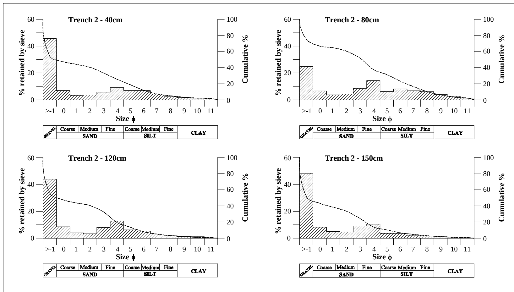
Figure 6.25 Grain size distributions for the sediment from trench 2 at Sekhokong Site 2.
