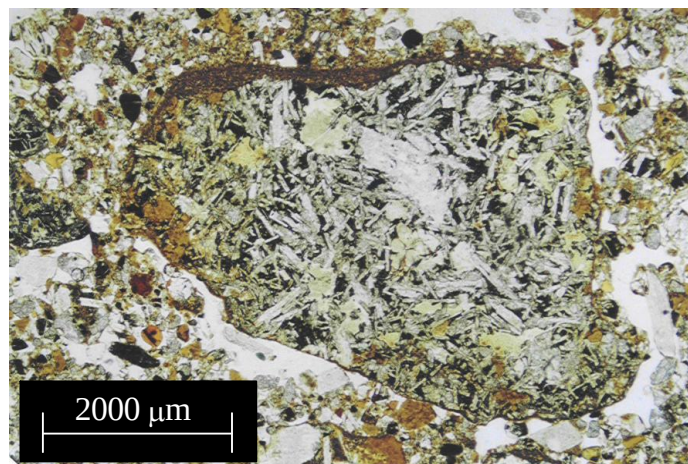
Figure 5.28 A basalt clast with a non-laminated silt capping taken in PPL.
