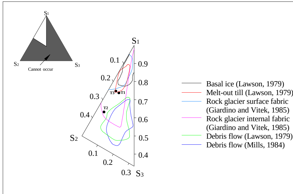
Figure 5.18 Triangular plot of normalised eigenvalues for the Tsatsa-La-Mangaung deposit, showing envelopes suggested by various authors. The usable field diagram occupies one sixth of the diagram because S_1 > S_2 > S_3 .
