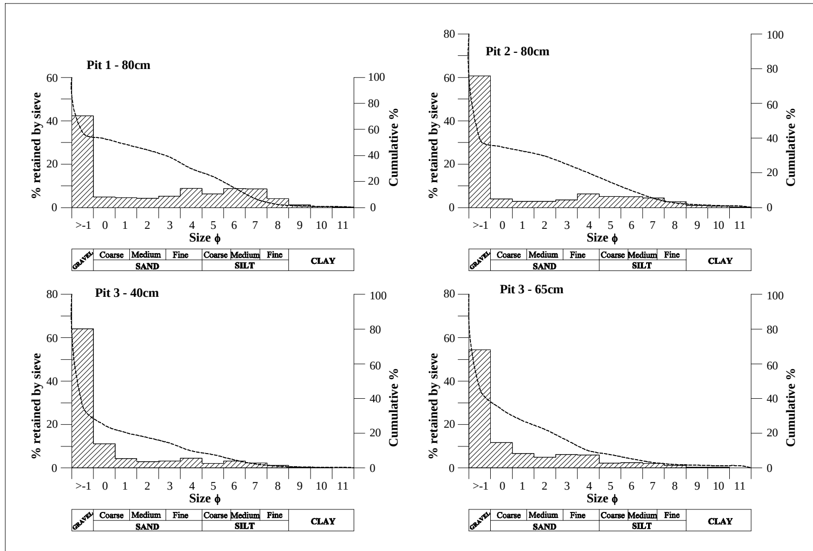
Figure 5.15 Grain size distributions for the sediment from the pits at the Tsatsa-La-Mangaung site.
