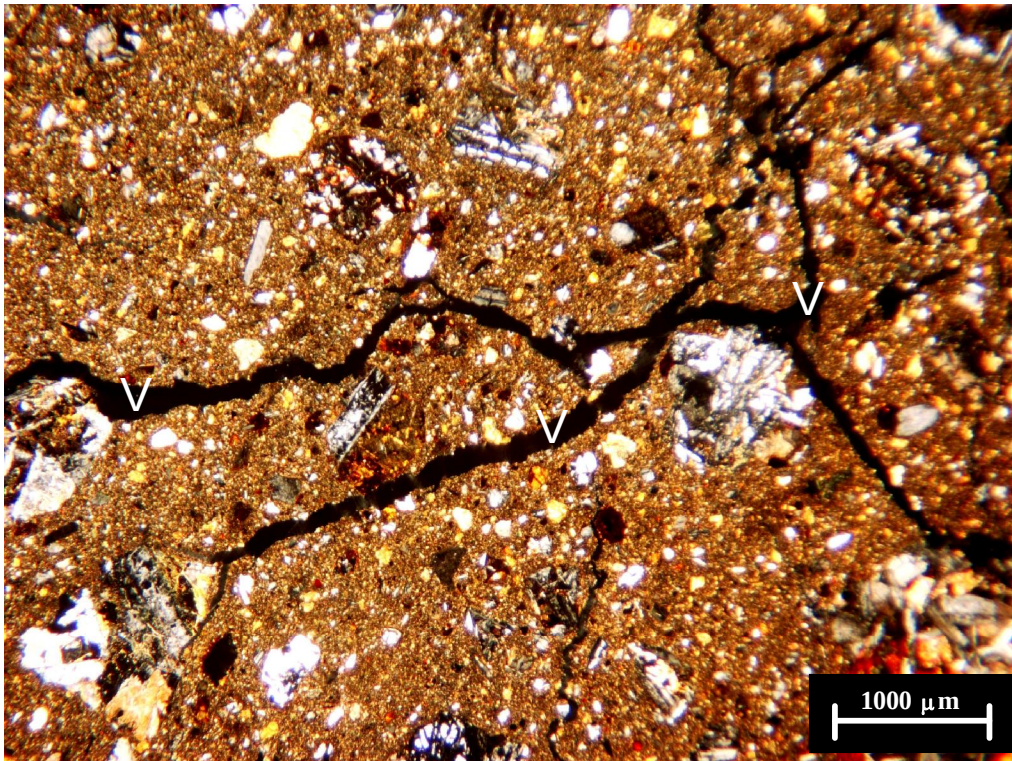
Figure 6.16 An example of plane voids in trench 3 at 125 cm depth taken in XPL (v = void).
