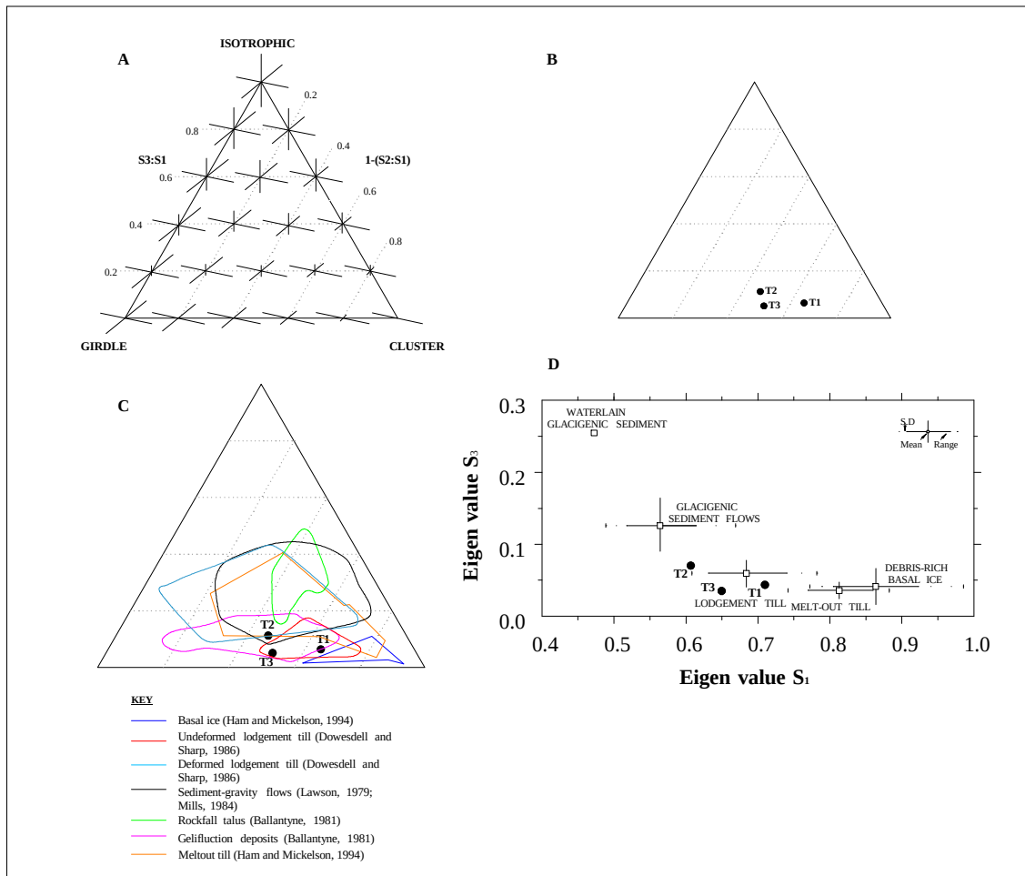
Figure 6.10 Till fabric using eigenvalue data for the Sekhokong Site 1 deposit. (A) The range of orthorhombic fabric shapes. (B) Fabric data from the three trenches. (C) Comparison with envelopes from a range of deposits. (D) Comparison with modern data fabrics from various environments (Dowdeswell et al. , 1985).
