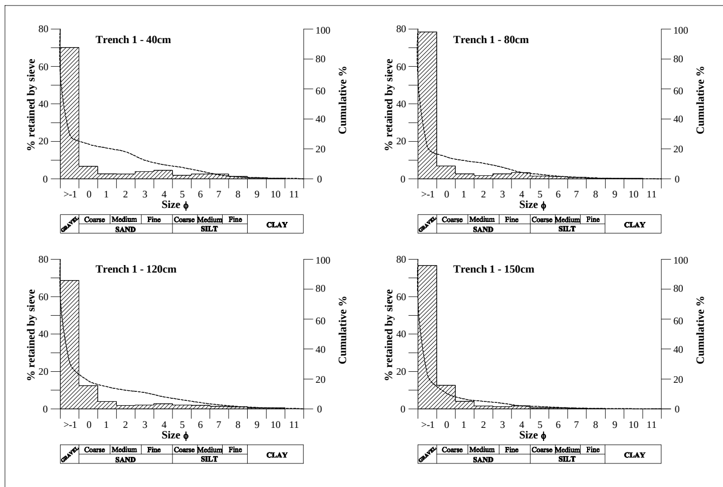
Figure 6.24 Grain size distributions for the sediment from trench 1 at Sekhokong Site 2.
