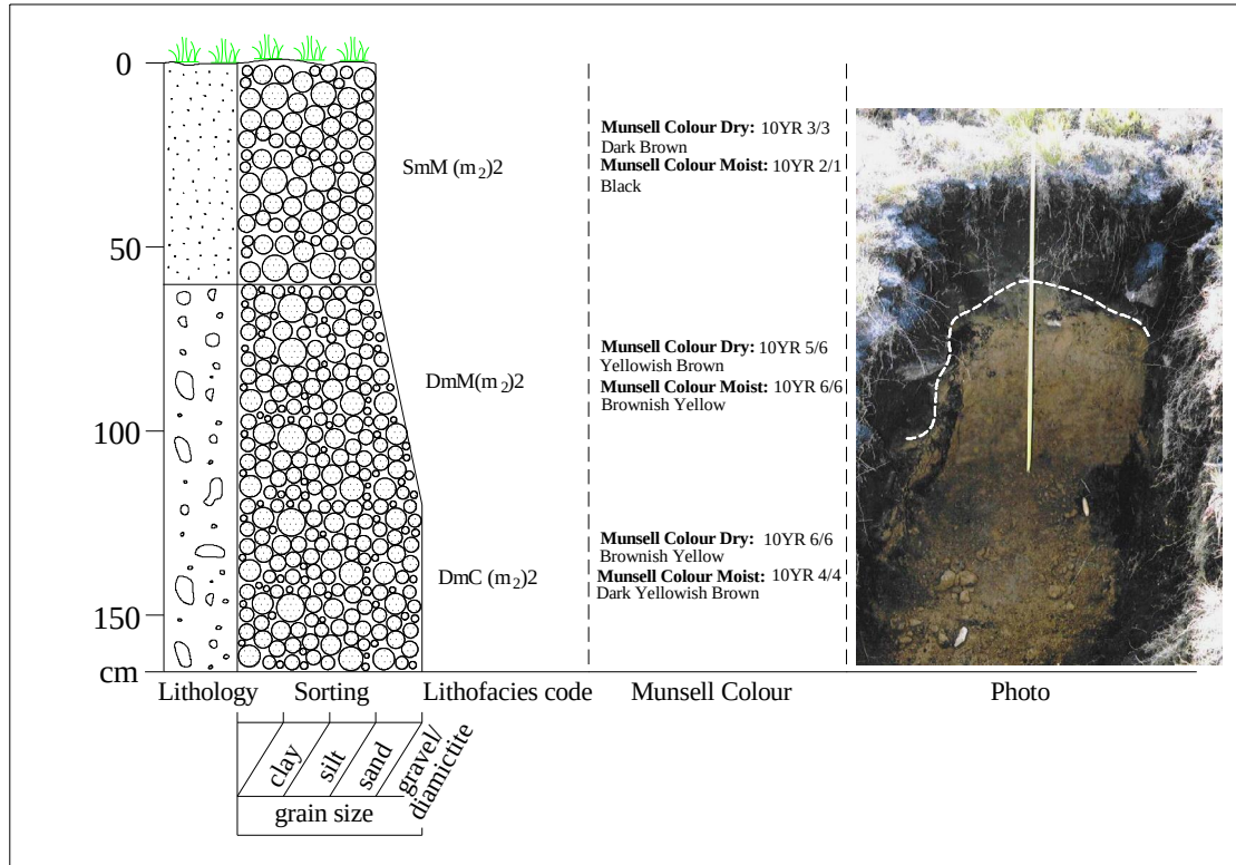
Figure 6.5 Sedimentological and stratigraphical data for trench 3 at Sekhokong Site 1.
