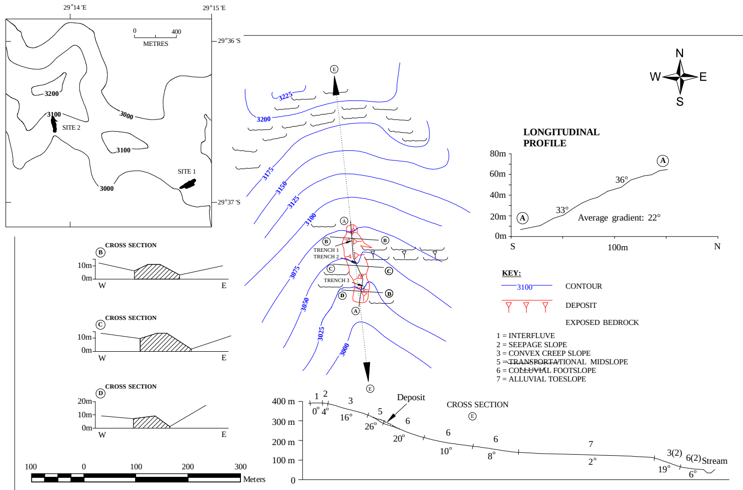
Figure 6.20 Morphological map of the Sekhokong Site 2 deposit.
