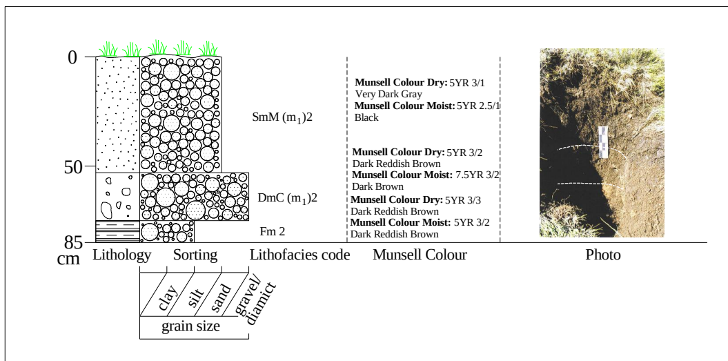
Figure 5.9 Sedimentological and stratigraphical data for Pit 3 at Tsatsa-La-Mangaung.
