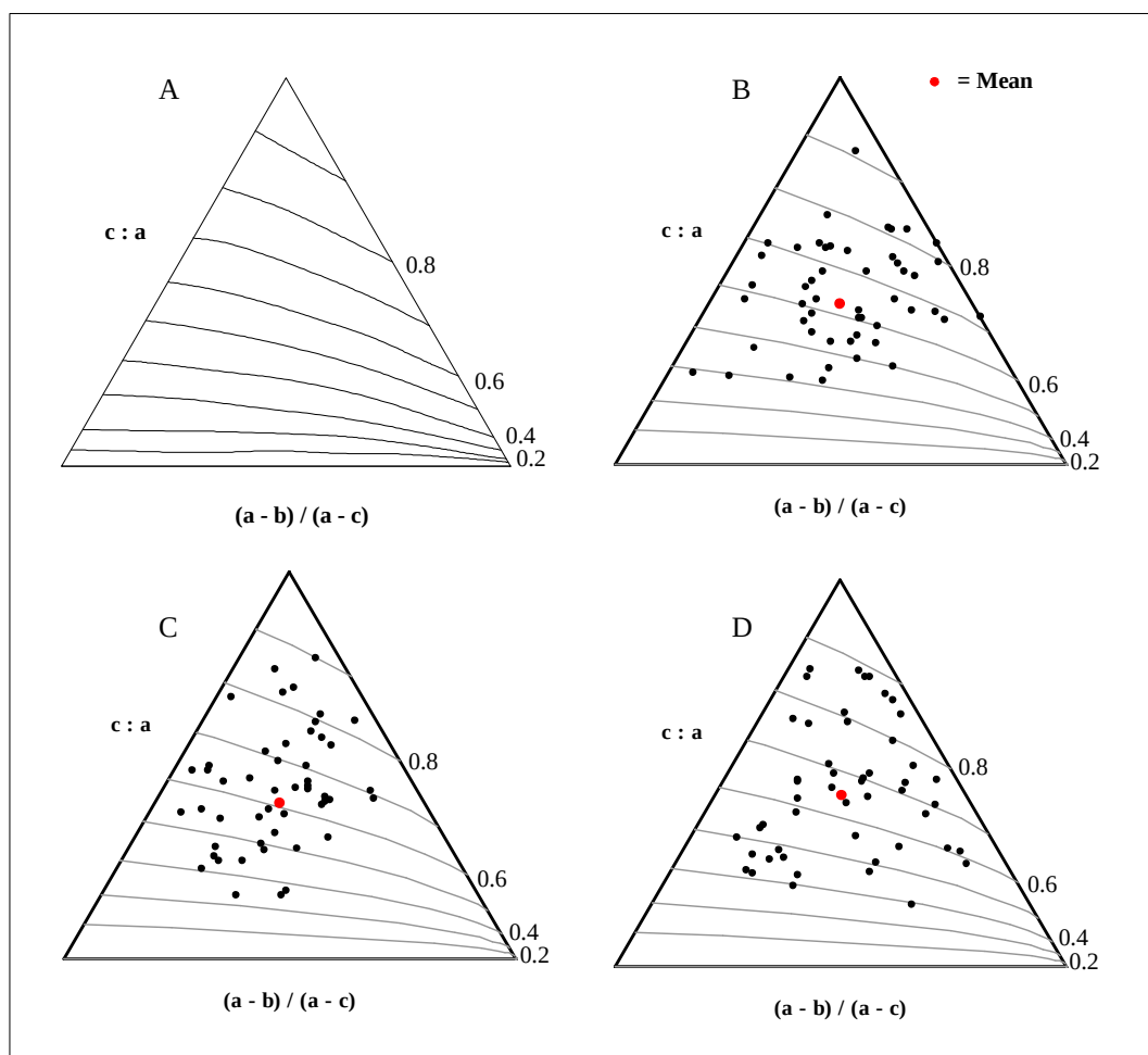
Figure 6.32 Triangular diagrams after Sneed and Folk (1958). (A) Isolines of the maximum projection sphericity according to Sneed and Folk (1958). Triangular diagrams for trenches 1, 2 and 3 respectively at Sekhokong Site 2 ( n = 50 ).
