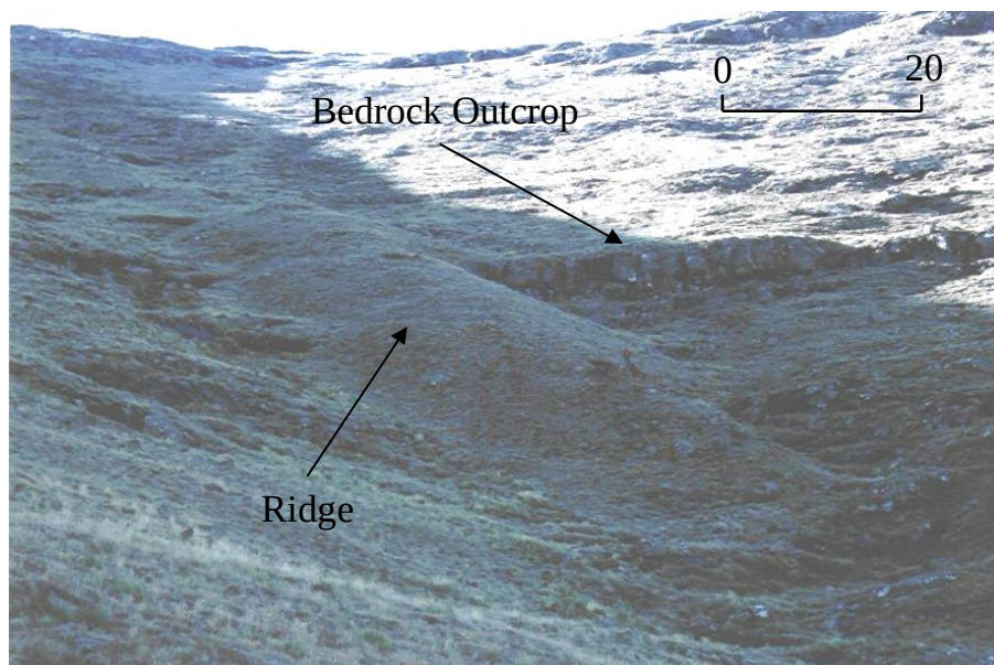
Figure 6.19 The Sekhokong Site 2 slope deposit (photo by S. Mills).
