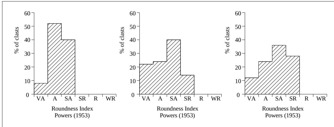
Figure 6.15 Graphs representing Powers (1953) visual roundness in trenches 1 (A), 2 (B) and 3 (C) at Sekhokong Site 1. VA = Very Angular, A = Angular, SA = Sub Angular, SR = Sub Rounded, R = Rounded, WR = Well Rounded (n = 50).
