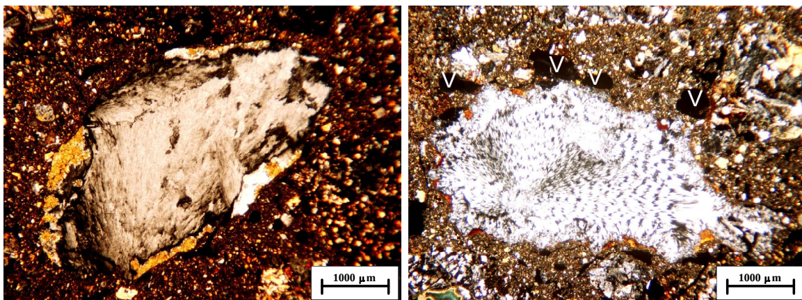
Figure 6.17 Single crystals within groundmass at Sekhokong Site 1, trench 3, taken in XPL.
