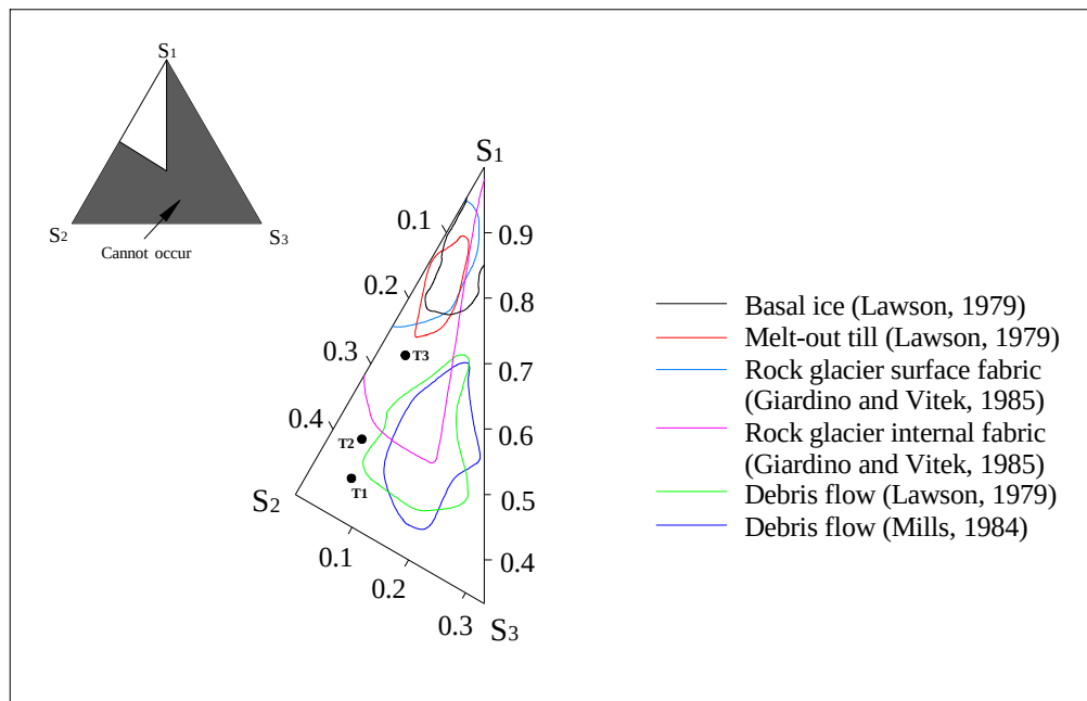
Figure 6.29 Triangular plot of normalised eigenvalues for the Sekhokong Site 2 deposit, showing envelopes suggested by various authors. The usable field diagram occupies one sixth of the diagram because S_1 > S_2 > S_3 .
