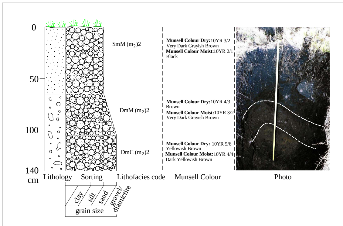
Figure 6.3 Sedimentological and stratigraphical data for trench 1 at Sekhokong Site 1.
