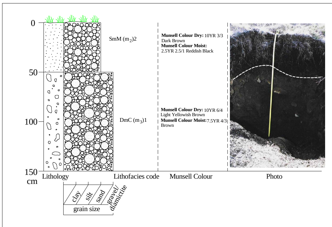
Figure 6.21 Sedimentological and stratigraphical data for trench 1 at Sekhokong Site 2.
