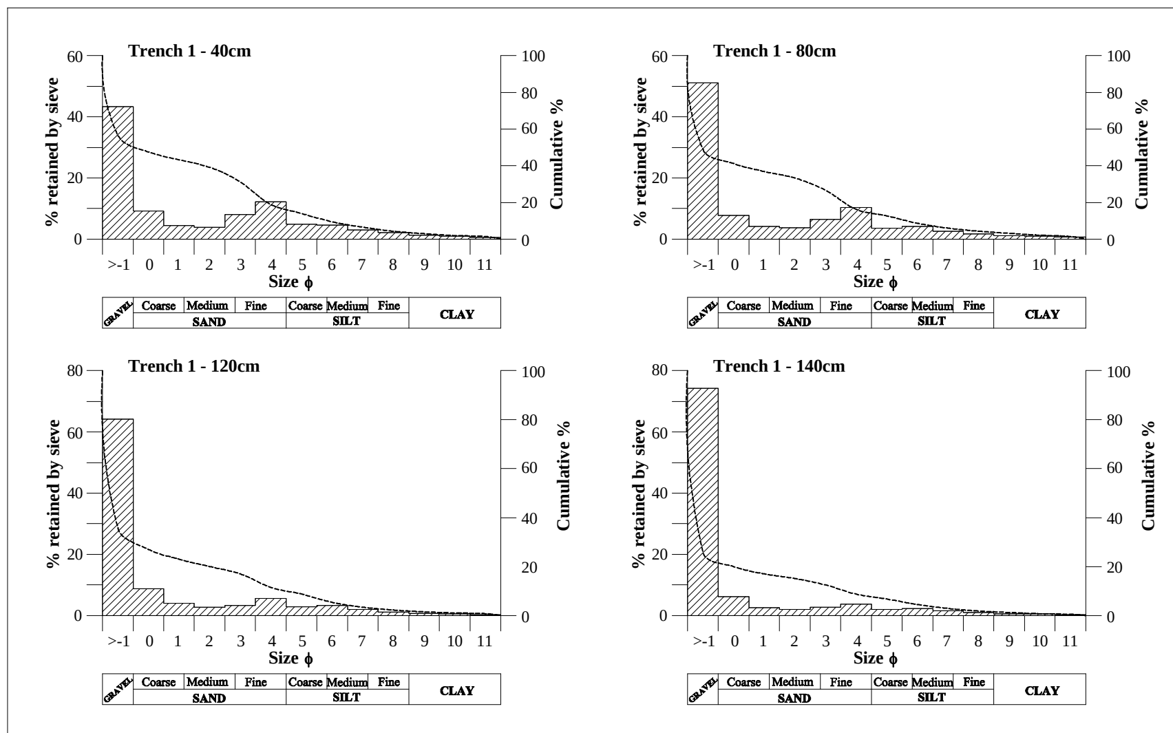
Figure 5.12 Grain size distributions for the sediment from trench 1 at the Tsatsa-La-Mangaung Site.
