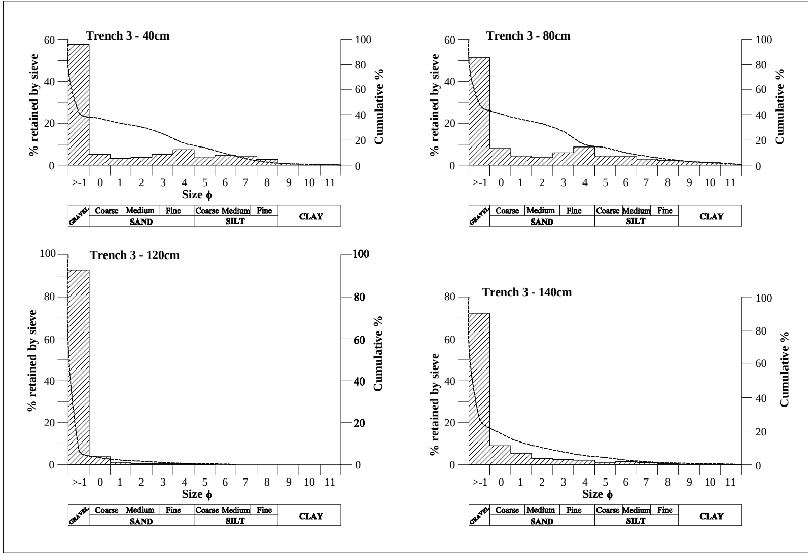
Figure 5.14 Grain size distributions for the sediment from trench 3 at the Tsatsa-La-Mangaung Site.
