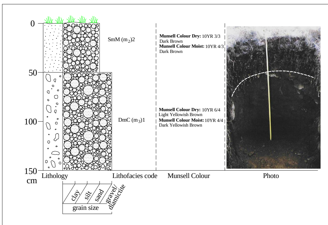
Figure 6.22 Sedimentological and stratigraphical data for trench 2 at Sekhokong Site 2.
