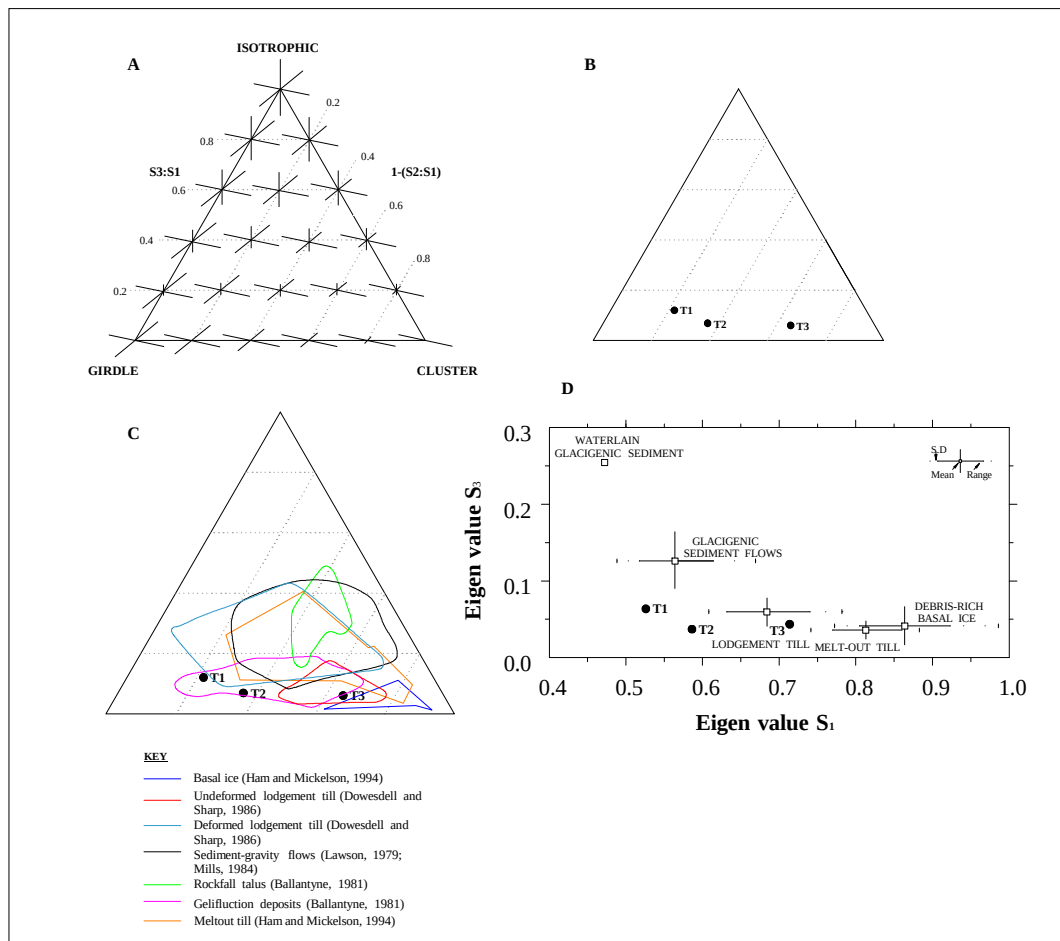
Figure 6.28 Till fabric using eigenvalue data. (A) The range of orthorhombic fabric shapes. (B) Fabric data from the three trenches. (C) Comparison with envelopes from a range of deposits. (D) Comparison with modern data fabrics from various environments (Dowdeswell et al. , 1985).
