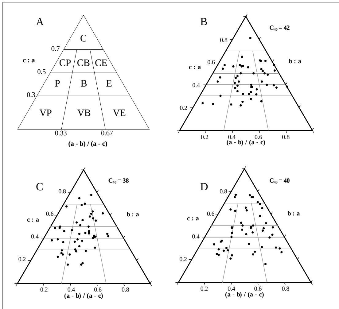
Figure 6.30 Triangular diagrams after Sneed and Folk (1958). (A) The descriptive classes according to Sneed and Folk (1958) where C = compact, P = platy, B = bladed, E = elongate and V = very. (B-D) Triangular diagrams for Trenches 1, 2 and 3 respectively at Sekhokong Site 2. C_{40} is the percentage of sample with c:a \leq 0.4 (Benn and Ballantyne, 1993) ( n = 50 ).
