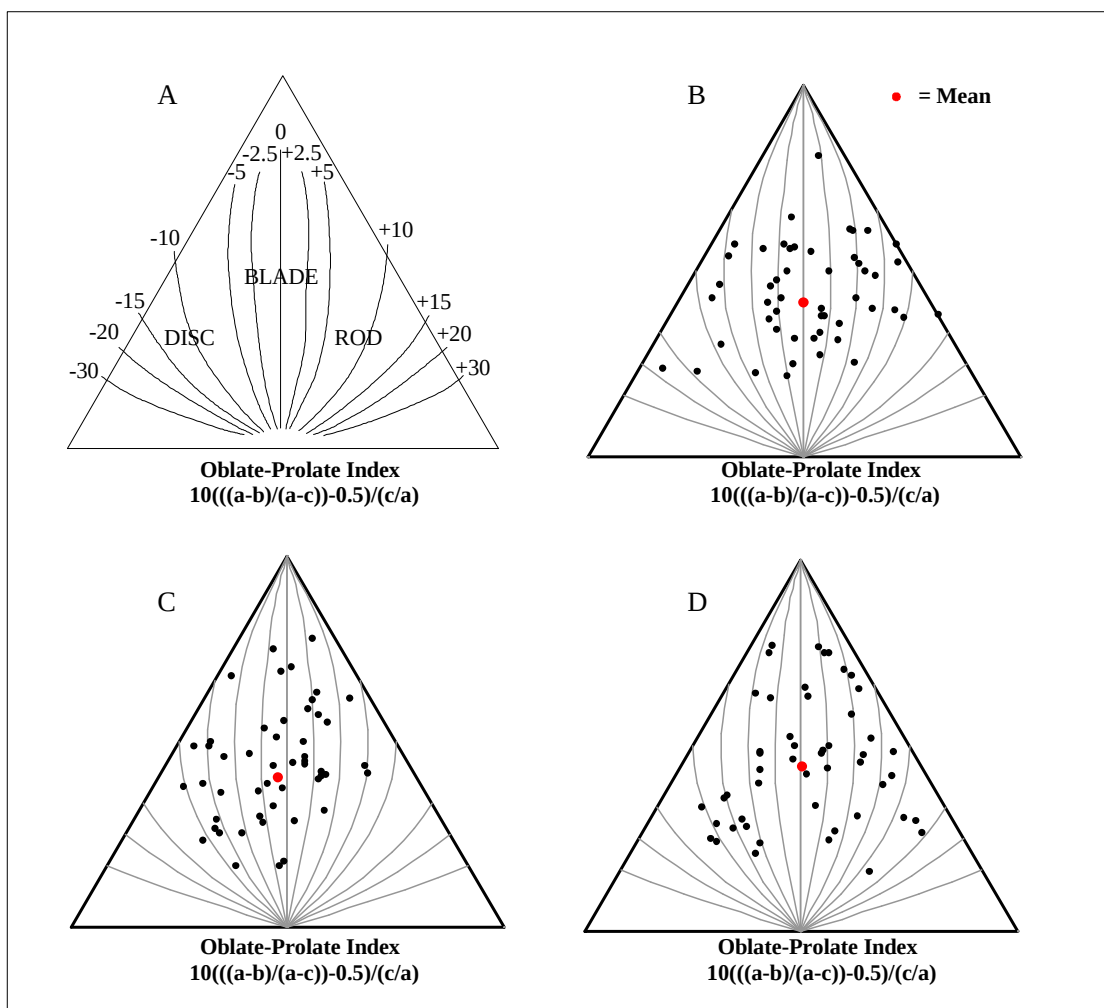
Figure 6.31 Triangular diagrams after Sneed and Folk (1958). (A) Isolines of the Oblate-prolate index according to Dobkins and Folk (1970). Triangular diagrams for Trenches 1, 2 and 3 respectively at Sekhokong Site 2 ( n = 50 ).
