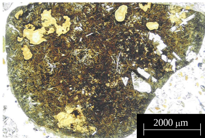
Figure 5.26 An example of a basalt grain taken in PPL.
