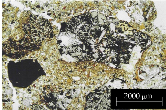
Figure 5.23 An example of coarse, weakly oriented, platy, subangular, undulating particles taken in PPL (Plane Polarized Light).
