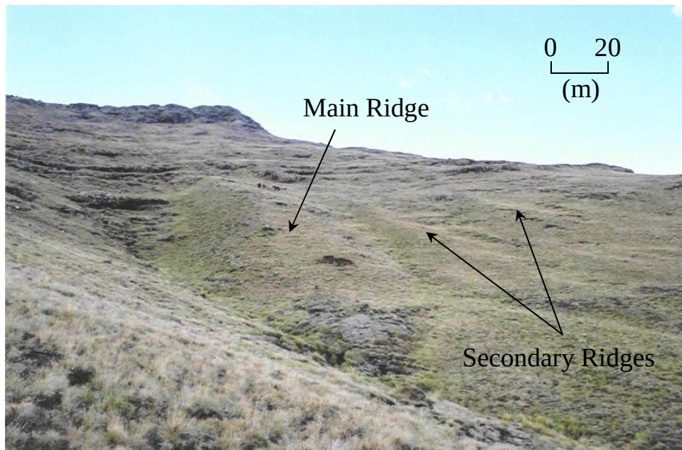
Figure 6.1 The Sekhokong Site 1 slope deposit (photo by S. Mills).
