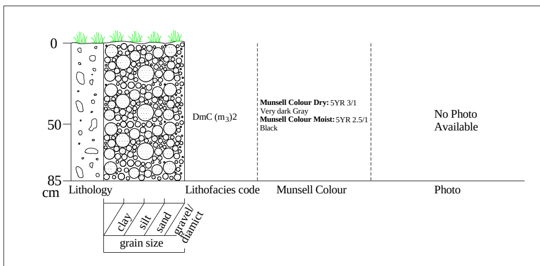
Figure 5.11 Sedimentological and stratigraphical data for Pit 5 at Tsatsa-La-Mangaung.
