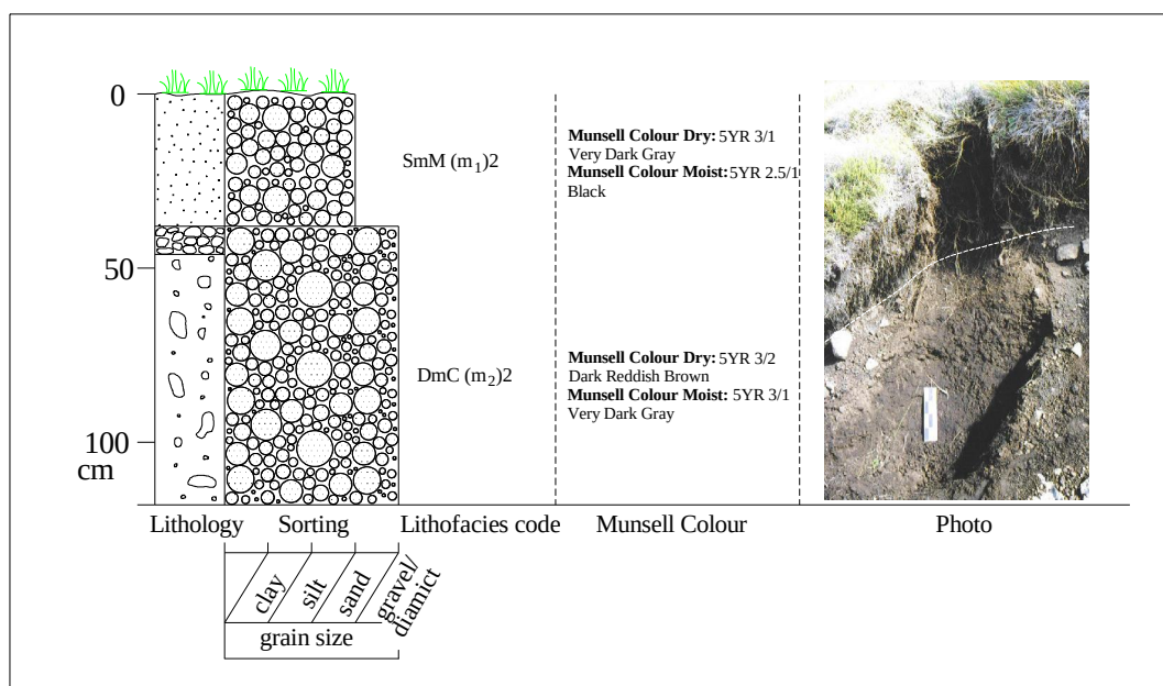
Figure 5.8 Sedimentological and stratigraphical data for Pit 2 at Tsatsa-La-Mangaung.
