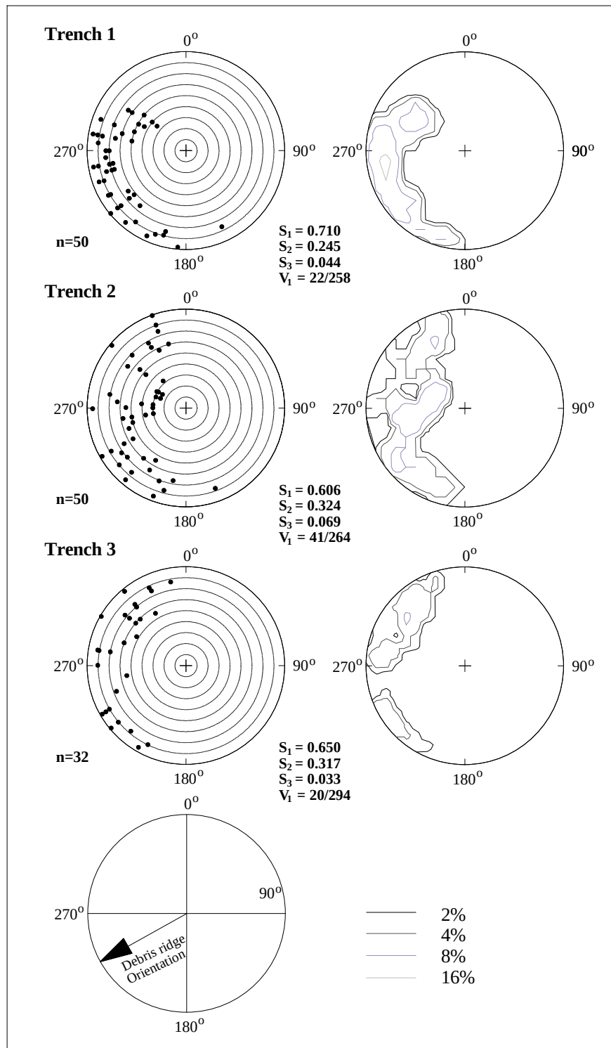
Figure 6.9 Clast orientation, dip and contouring at trenches 1, 2 and 3 at Sekhokong Site 1.
