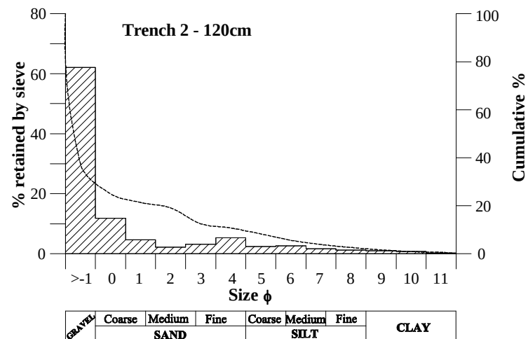
Figure 6.7 Grain size distributions for the sediment from trench 2 at Sekhokong Site 1.
