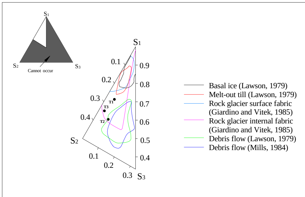
Figure 6.11 Triangular plot of normalised eigenvalues for the Sekhokong Site 1 deposit, showing envelopes suggested by various authors. The usable field diagram occupies one sixth of the diagram because S_1 > S_2 > S_3 .
