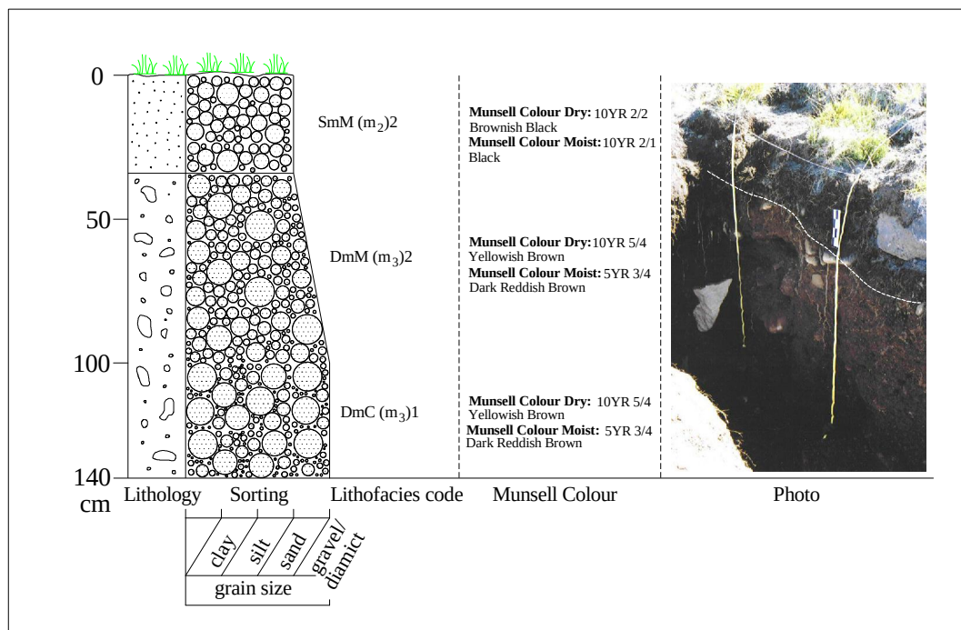
Figure 5.4 Sedimentological and stratigraphical data for trench 1 at Tsatsa-La-Mangaung.
