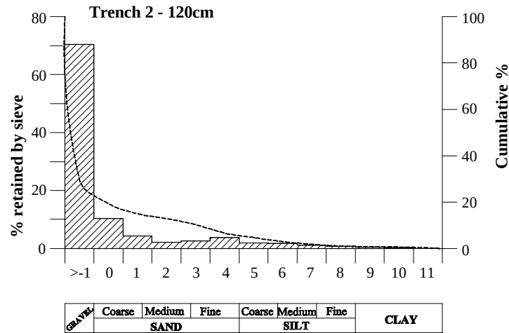
Figure 5.13 Grain size distributions for the sediment from trench 2 at the Tsatsa-La-Mangaung Site.
