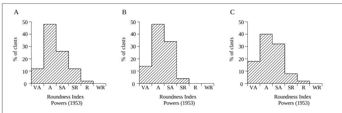
Figure 5.22 Graphs representing visual roundness of clasts (after Powers 1953) in trenches 1 (A), 2 (B) and 3 (C) at Tsatsa-La-Mangaung. VA = Very Angular, A = Angular, SA = Sub Angular, SR = Sub Rounded, R = Rounded, WR = Well Rounded (n = 50).
