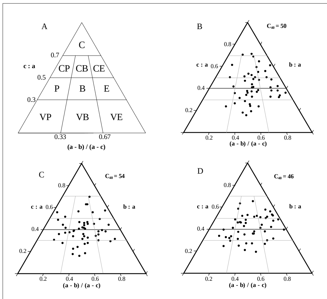
Figure 5.19 Triangular diagrams after Sneed and Folk (1958). (A) The descriptive classes according to Sneed and Folk (1958) where C = compact, P = platy, B = bladed, E = elongate and V = very. (B-D) Triangular diagrams for clasts in trenches 1, 2 and 3 respectively at Tsatsa-La-Mangaung. C_{40} is the percentage of sample with c:a \leq 0.4 (Benn and Ballantyne, 1993) ( n = 50 ).
