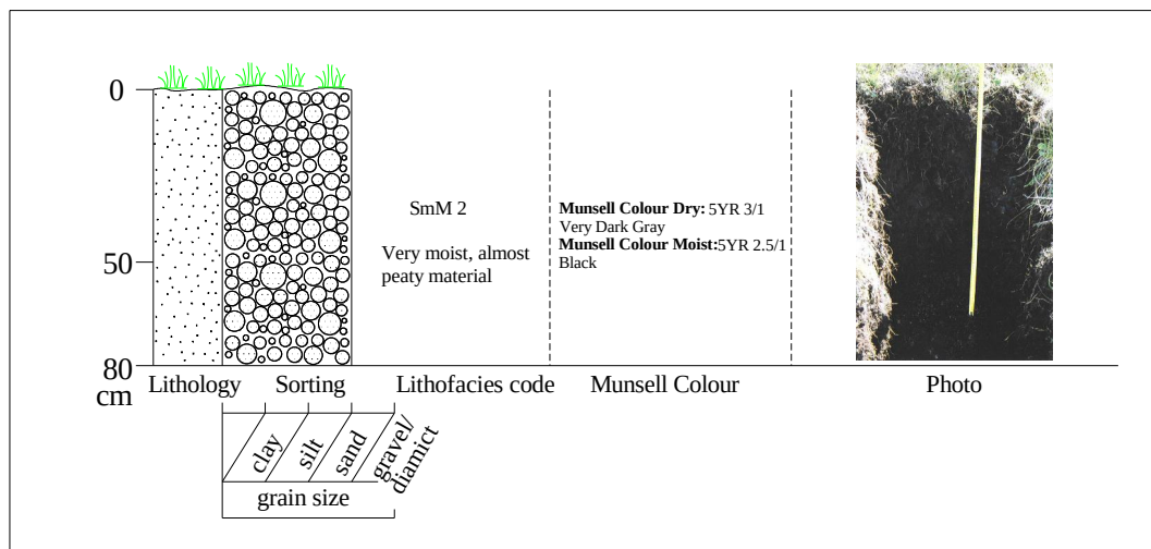
Figure 5.7 Sedimentological and stratigraphical data for Pit 1 at Tsatsa-La-Mangaung.
