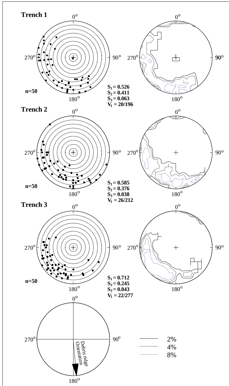
Figure 6.27 Clast orientation, dip and contouring at trenches 1, 2 and 3 at Sekhokong Site 2.
