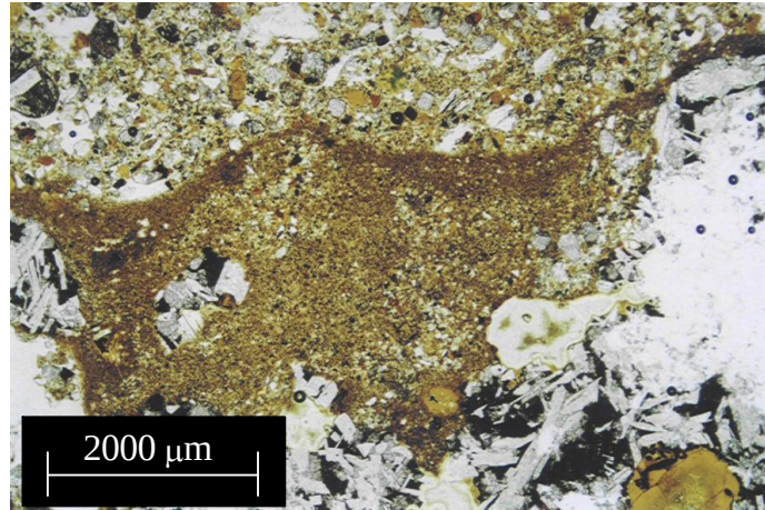
Figure 5.29 A basalt clast with a laminated silt capping taken in PPL.
