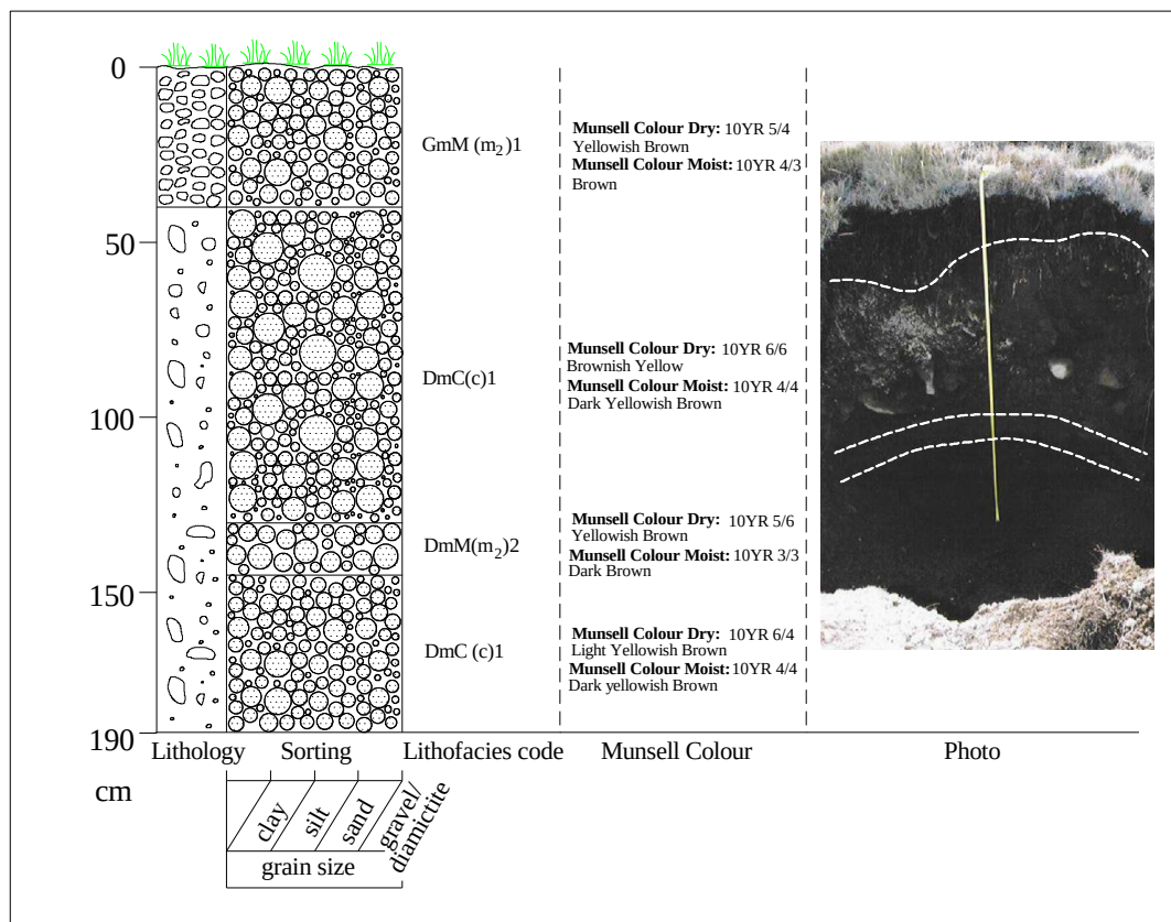
Figure 6.23 Sedimentological and stratigraphical data for trench 3 at Sekhokong Site 2.
