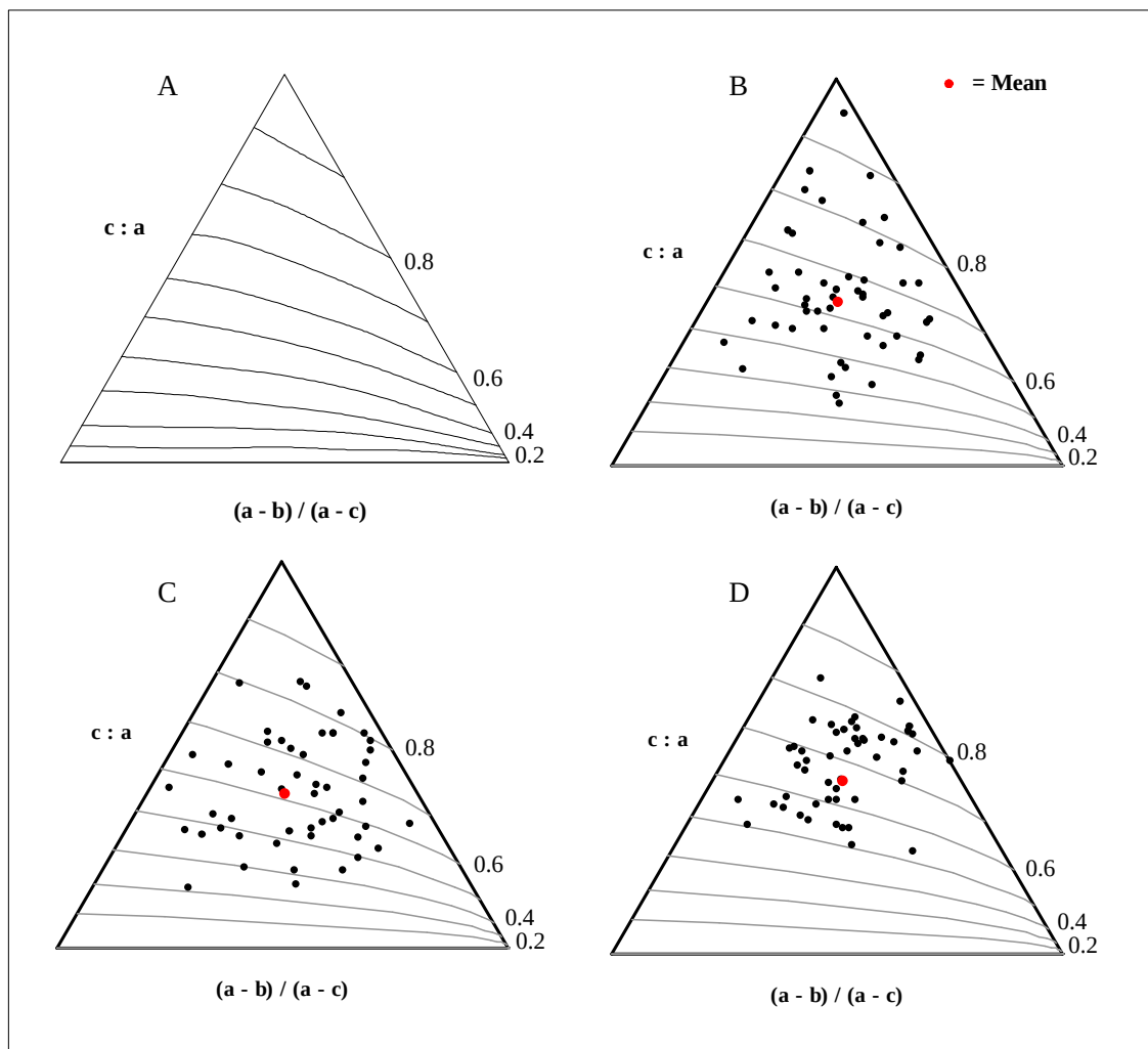
Figure 6.14 Triangular diagrams after Sneed and Folk (1958). (A) Isolines of the maximum projection sphericity according to Sneed and Folk (1958). Triangular diagrams for trenches 1, 2 and 3 respectively at Sekhokong Site 1 ( n = 50 ).
