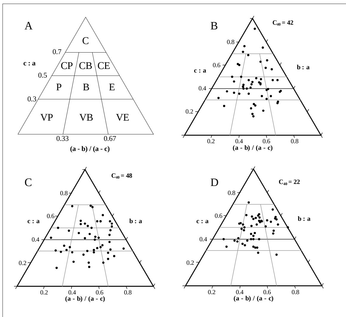
Figure 6.12 Triangular diagrams after Sneed and Folk (1958). (A) The descriptive classes according to Sneed and Folk (1958) where C = compact, P = platy, B = bladed, E = elongate and V = very. (B-D) Triangular diagrams for trenches 1, 2 and 3 respectively at Sekhokong Site 1. C_{40} is the percentage of sample with c:a \leq 0.4 (Benn and Ballantyne, 1993) ( n = 50 ).
