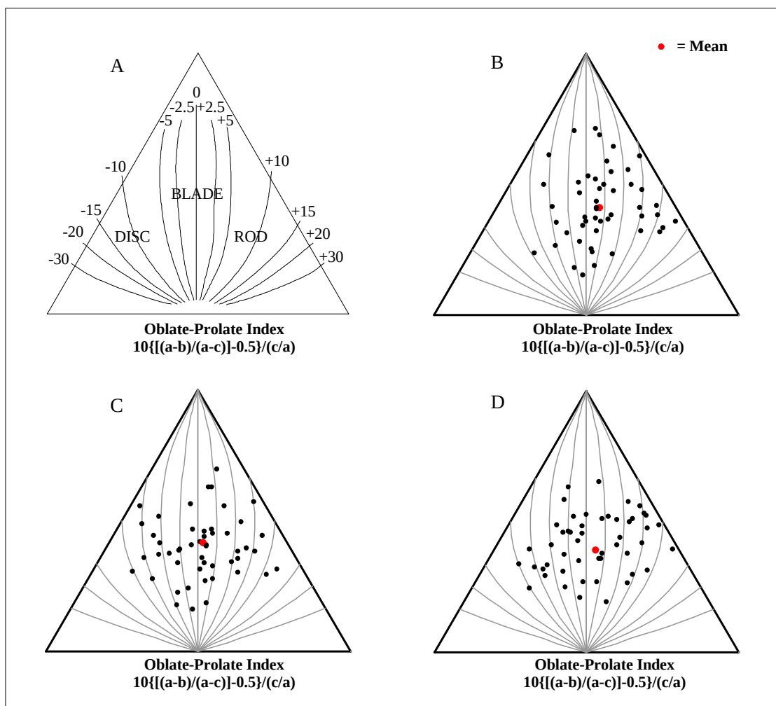
Figure 5.20 Triangular diagrams after Sneed and Folk (1958). (A) Isolines of the Oblate-prolate index according to Dobkins and Folk (1970). Triangular diagrams for trenches 1, 2 and 3 respectively at Tsatsa-La-Mangaung ( n = 50 ).
