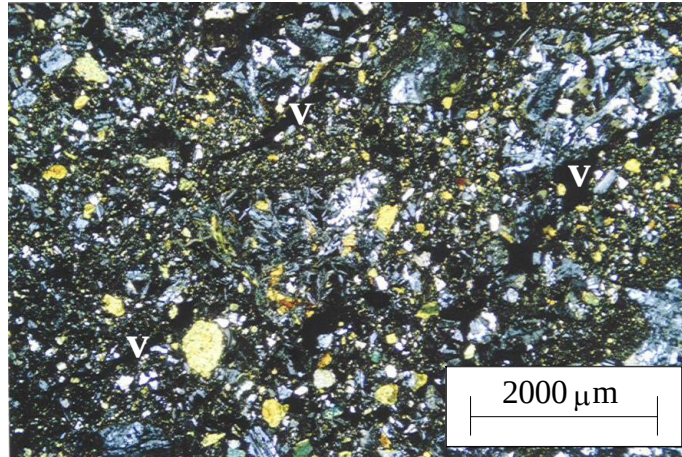
Figure 5.25 An example of typical channel voids taken in XPL (v = voids).
