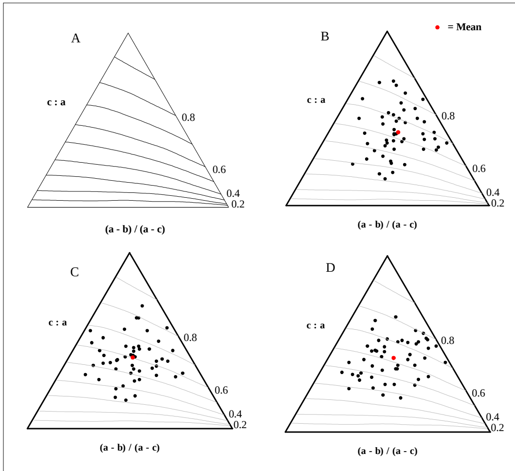
Figure 5.21 Triangular diagrams after Sneed and Folk (1958). (A) Isolines of the maximum projection sphericity according to Sneed and Folk (1958). Triangular diagrams for trenches 1, 2 and 3 respectively at Tsatsa-La-Mangaung ( n = 50 ).
