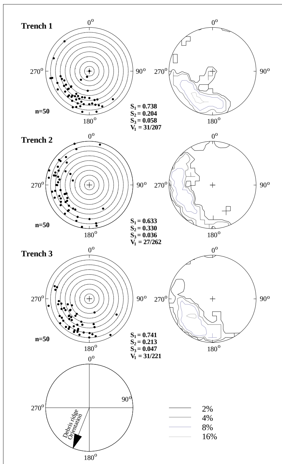
Figure 5.16 Clast orientation, dip and contouring at trenches 1, 2 and 3 at Tsatsa-La-Mangaung ( n = 50 ).
