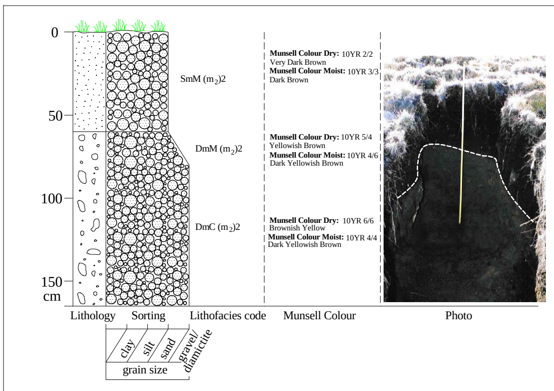
Figure 6.4 Sedimentological and stratigraphical data for trench 2 at Sekhokong Site 1.
