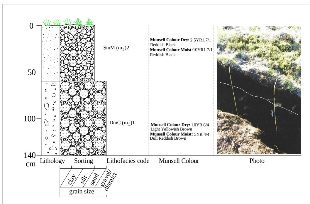
Figure 5.6 Sedimentological and stratigraphical data for trench 3 at Tsatsa-La-Mangaung.
