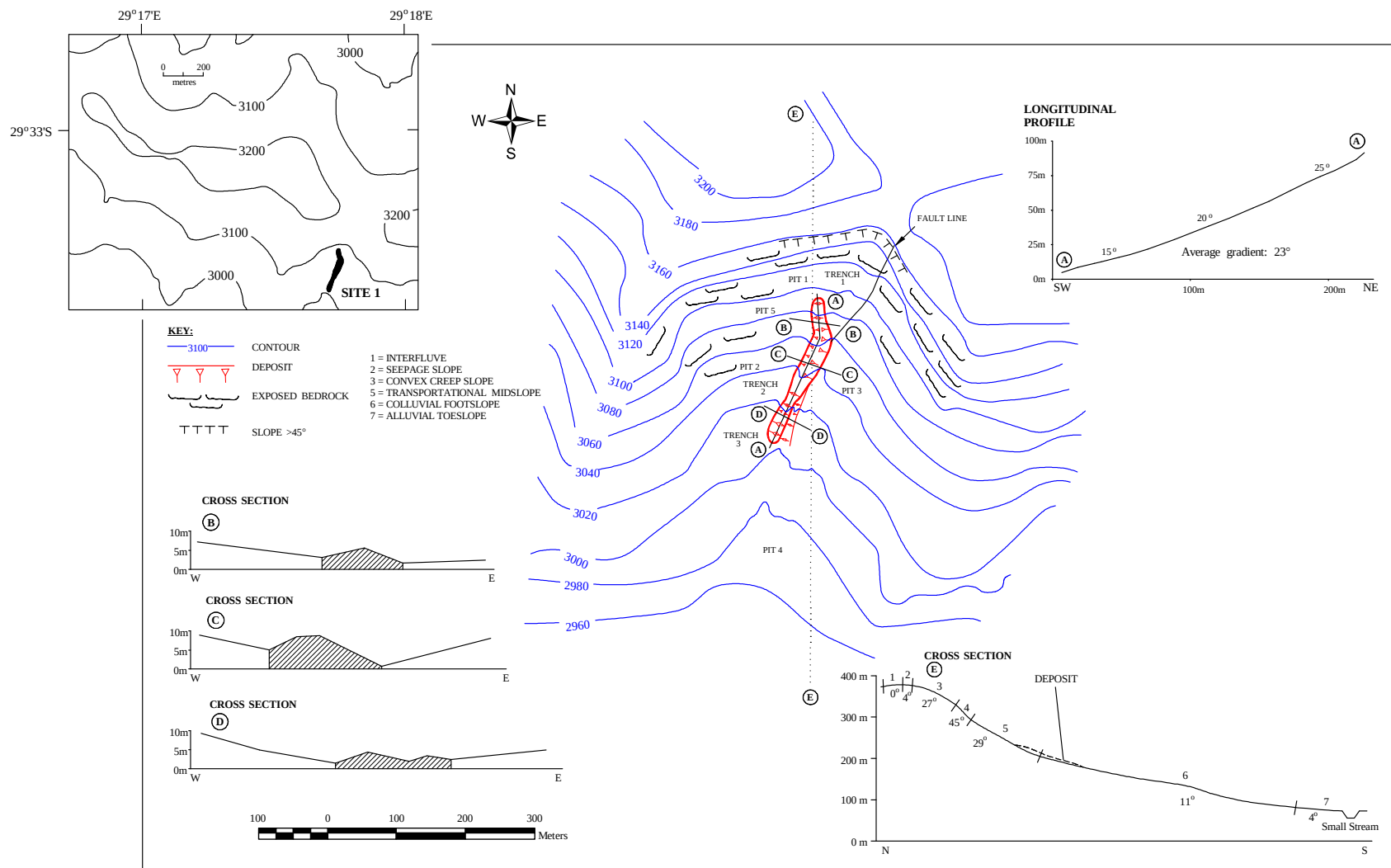
Figure 5.2 Morphological map of the Tsatsa-La-Mangaung deposit.
