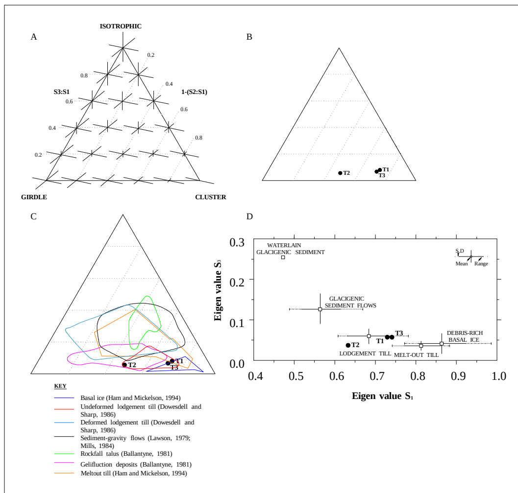
Figure 5.17 Till fabric using eigenvalue data for the Tsatsa-La-Mangaung deposit. (A) The range of orthorhombic fabric shapes. (B) Fabric data from the three trenches. (C) Comparison with envelopes from a range of deposits. (D) Comparison with modern data fabrics from various environments (Dowdeswell et al. , 1985).
