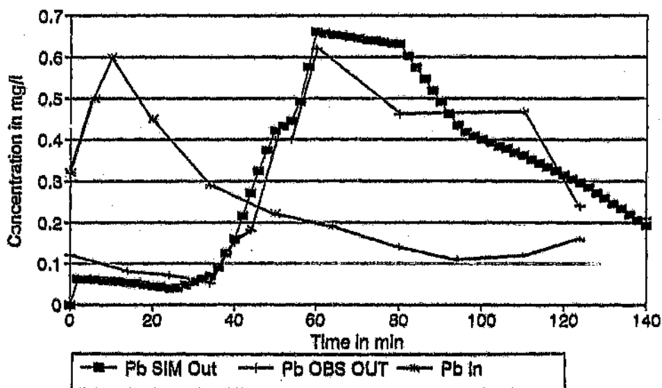
Figure 6.16 WITQUAL Simulation of lead during the storm event of 29/11/1995
