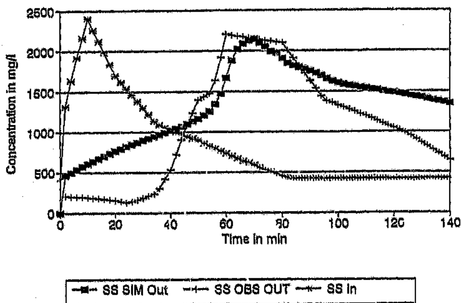
Figure 6.15 WITQUAL Simulation of SS during the storm event of 29/11/1995
