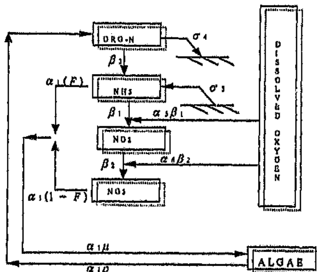
Figure 5.3 QUAL2EU modelling of nitrogen species
