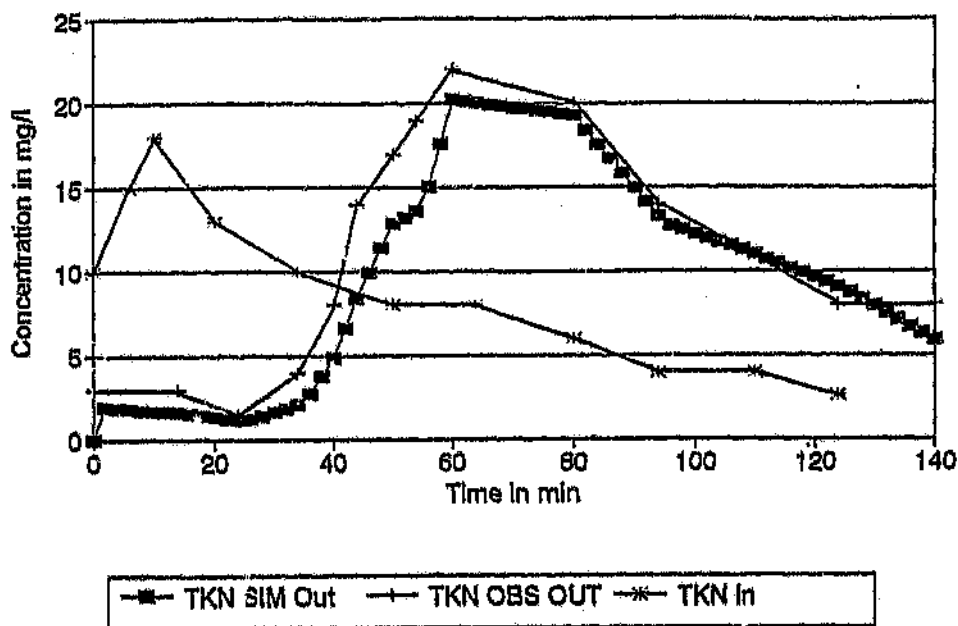
Figure 6.17 WITQUAL Simulation of TKN during the storm event of 29/11/1995
