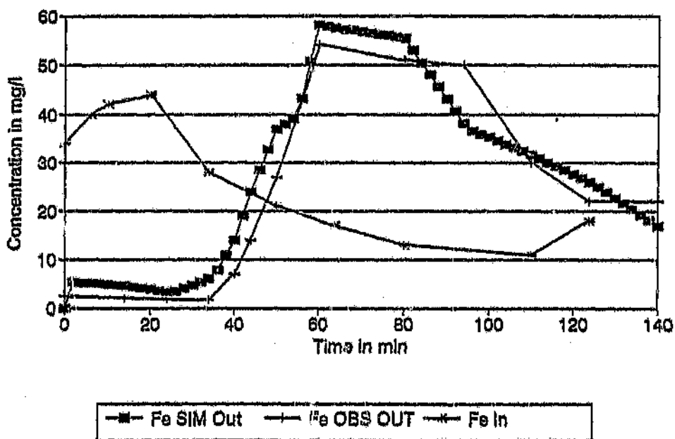
Figure 6.18 WITQUAL Simulation of Iron during the storm event of 29/11/1995
