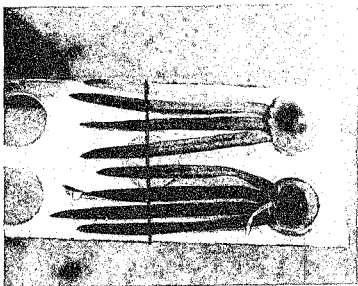
PLATE 2. Showing the eight prepared barley leaves for \text{CO}_2 compensation point determination.
