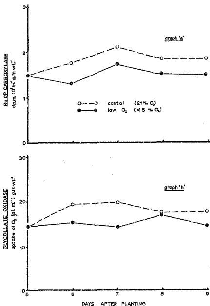
Appendix 11. Graphs showing the effect of low levels of O_2 ( < 5\% ) on ribulose 1-5, diphosphate carboxylase (graph 'a') and glycollate oxidase (graph 'b').
