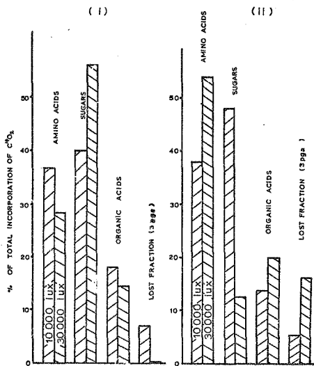
FIGURE 20. Histograms showing the distribution of C^{14}O_2 in (i) a young expanding leaf and (ii) a fully expanded leaf.
