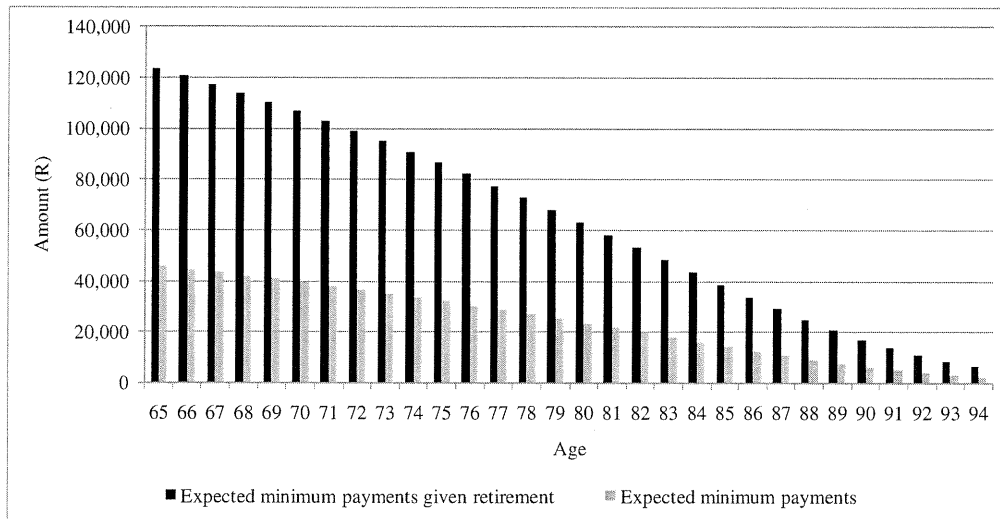
Figure 8.7: Projected cashflow profiles
