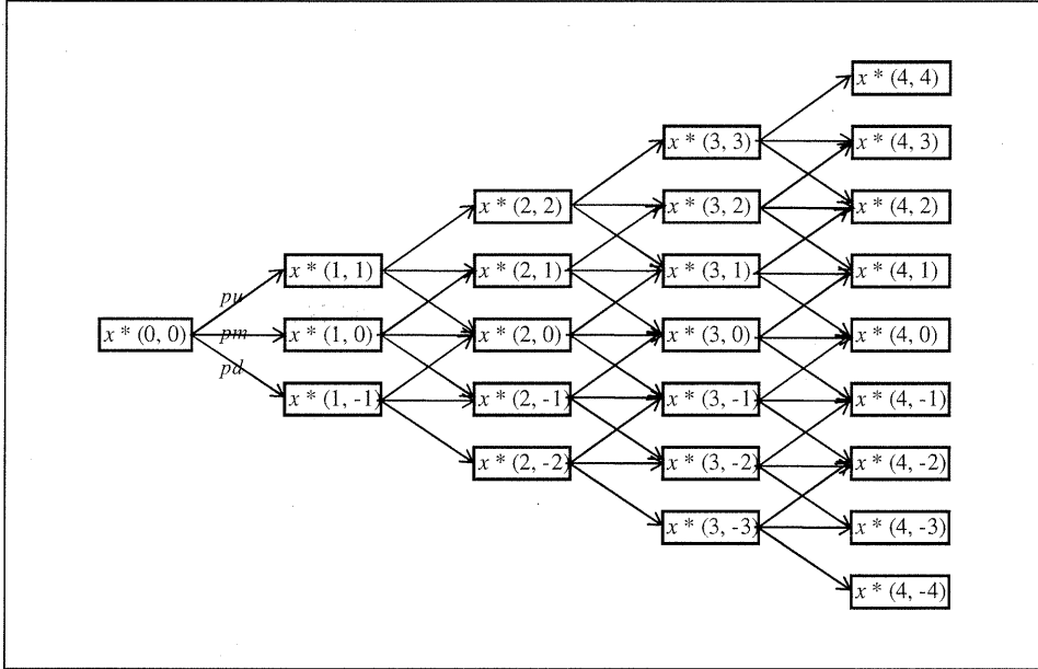
Figure 5.12: Stage 1 interest-rate tree
