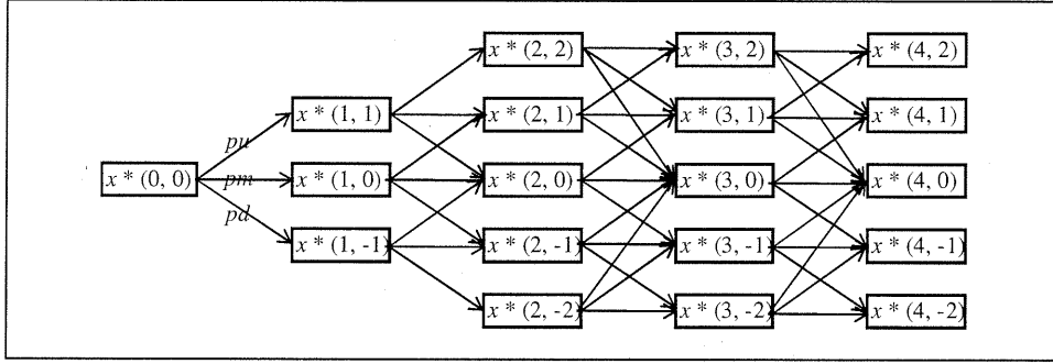
Figure 5.14: Stage 1 trimmed interest-rate tree.
