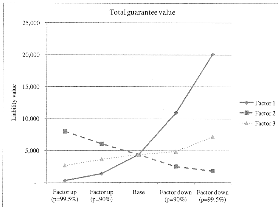
Figure 8.3: Sensitivity of total reserves to the changes in term structure of interest rates
