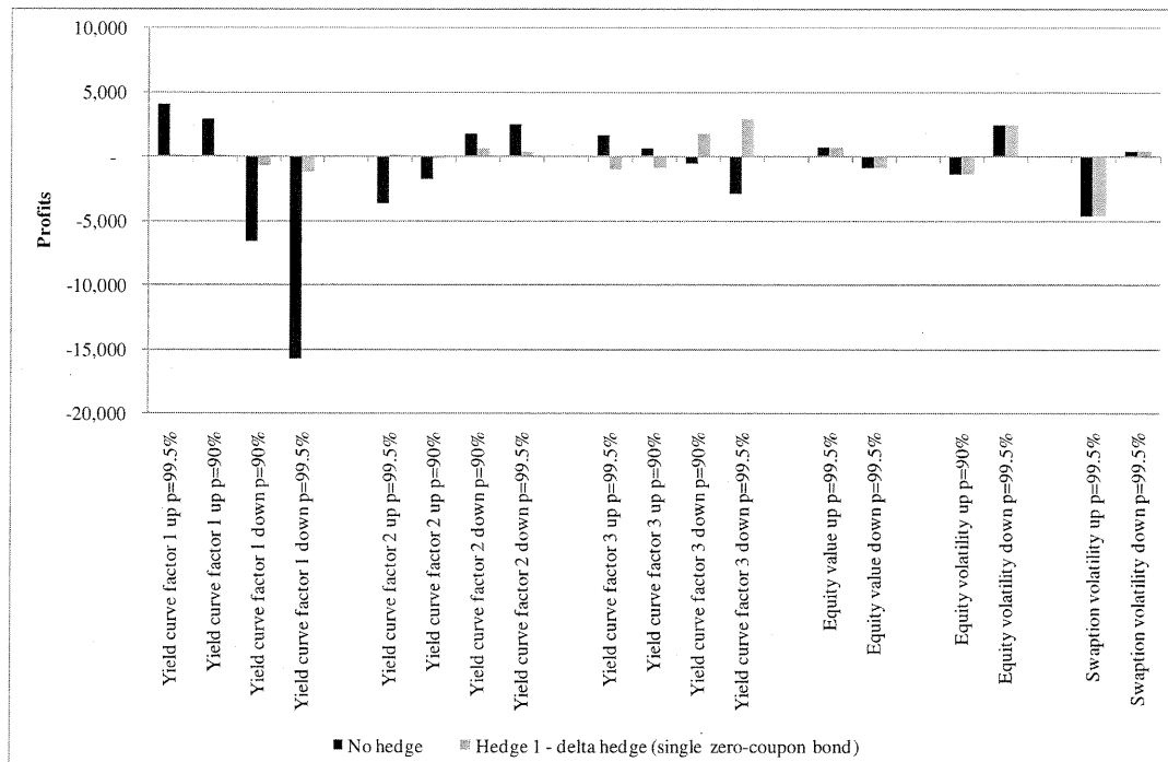
Figure 8.5: Comparison of the value at risk between (a) no hedge, and (b) duration hedge with a ZCB of 61.7 years
