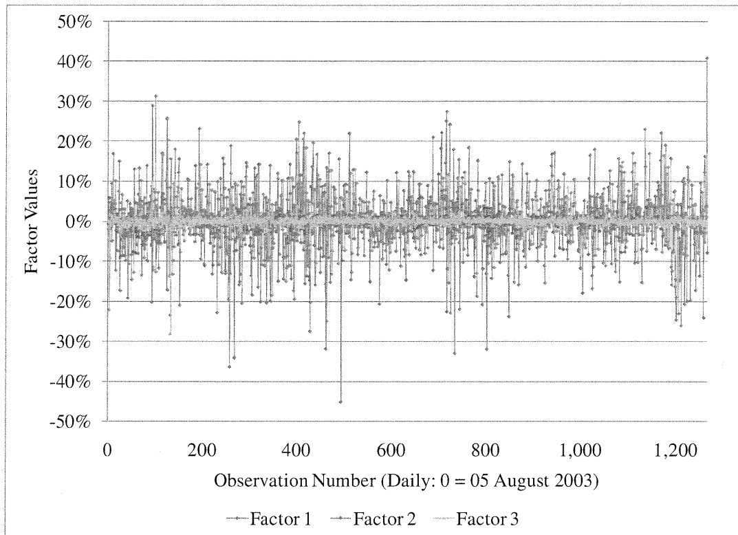
Figure 7.2: Historic observed log changes mapped onto the new axes
