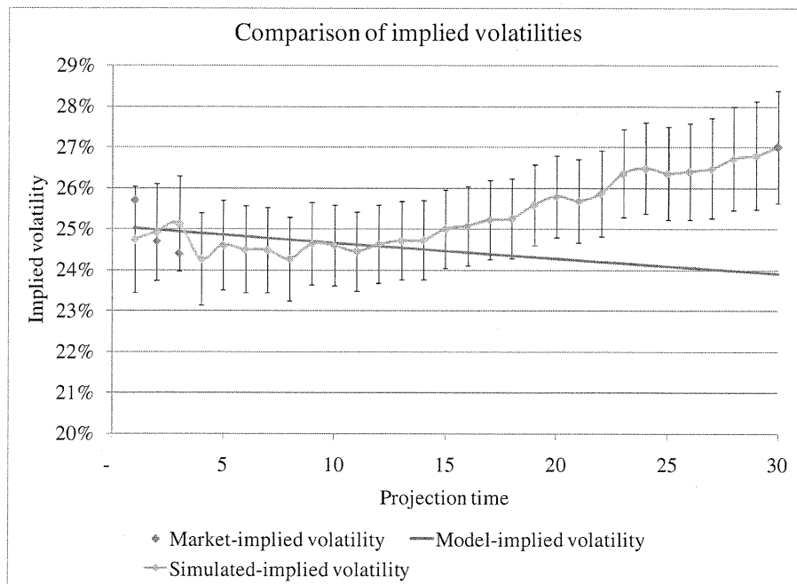
Figure 5.10: Market implied-volatility and its comparison against those calculated using the model and simulations
