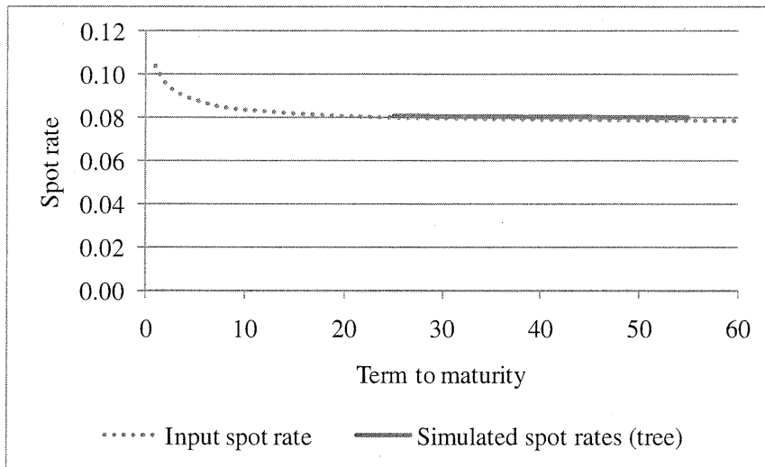
Figure 5.20: Comparison of simulated ZCB prices ( t=25 ) to the calibration targets
