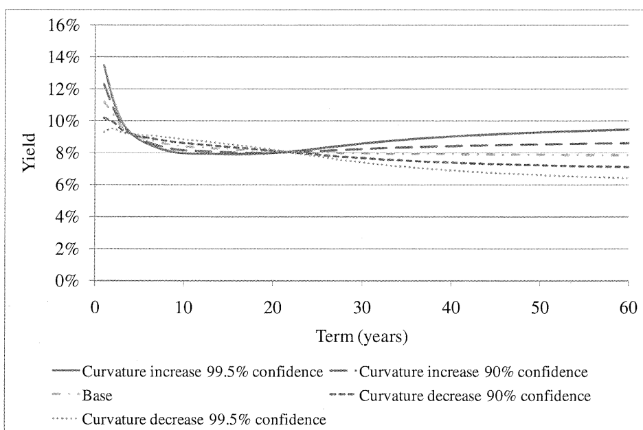
Figure 7.5: Shocked term structures of interest rates when using the third factor
