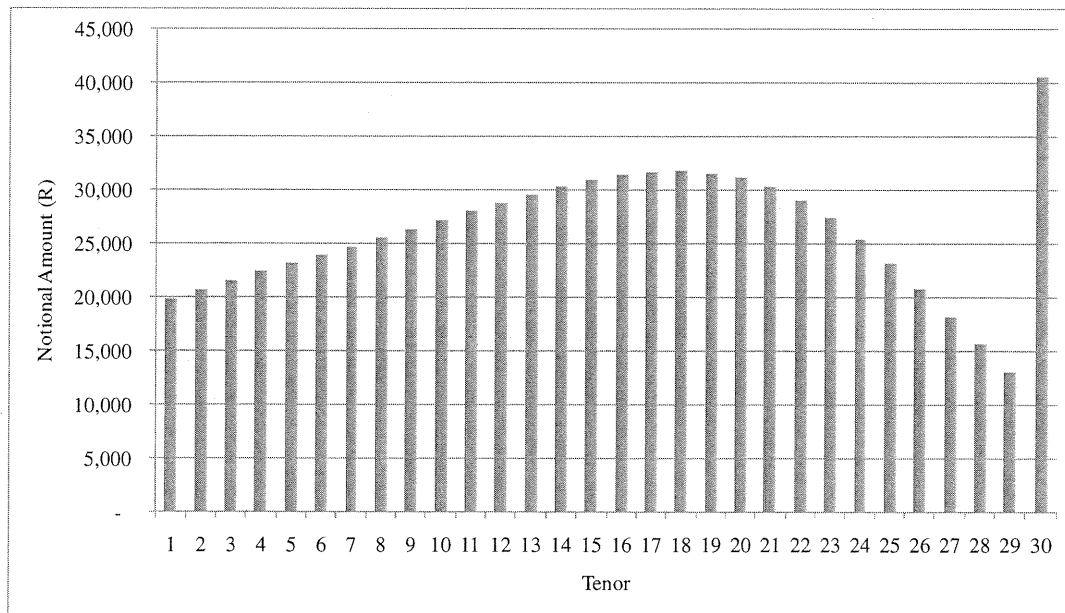
Figure 8.8: Notional amounts of 25-year swaptions of various tenors to be held in the hedge portfolio
