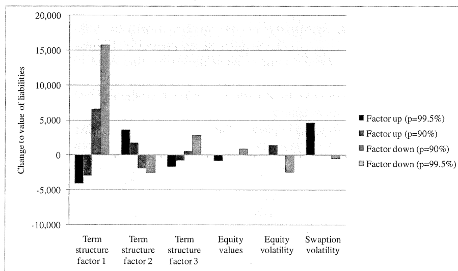
Figure 8.4: The effects of the various shocks at various confidence levels on the total guarantee liabilities
