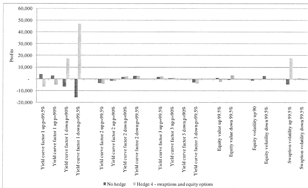
Figure 8.11: Comparison of VaR of all guarantee liabilities when (a) no hedge is held in respect of the risks and (b) rho and vega hedge consisting of receiver swaptions, equity puts and cash
