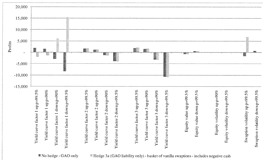
Figure 8.9: Comparison of the VaR for GAO liabilities only when (a) no hedge is held in respect of the risks; and (b) a hedge consisting of receiver swaptions and cash is held
