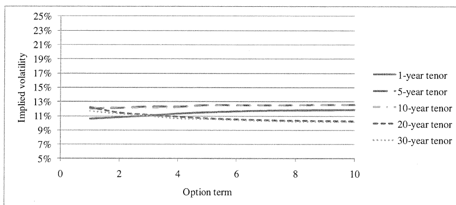
Figure 7.8: Implied volatility on swaptions where a downward shock corresponding to a 99.5% confidence is applied to the first factor
