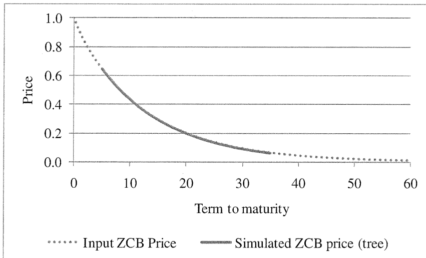
Figure 5.17: Comparison of simulated spot yields ( t=5 ) to the calibration targets
