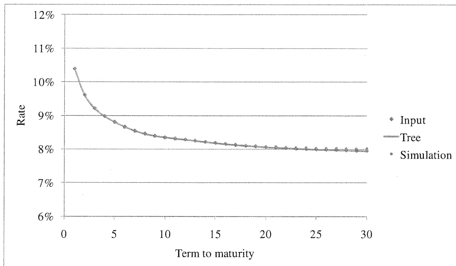
Figure 5.6: A comparison of yield curve generated by the interest-rate tree and Monte-Carlo simulations to the input
