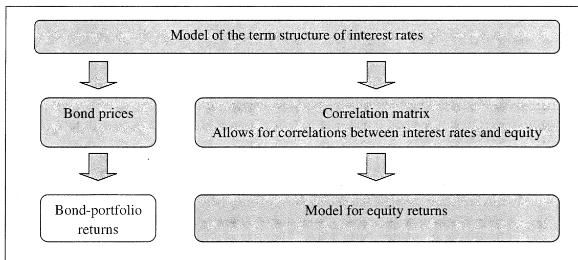
Figure 5.1 High-level structure of the economic scenario generator
