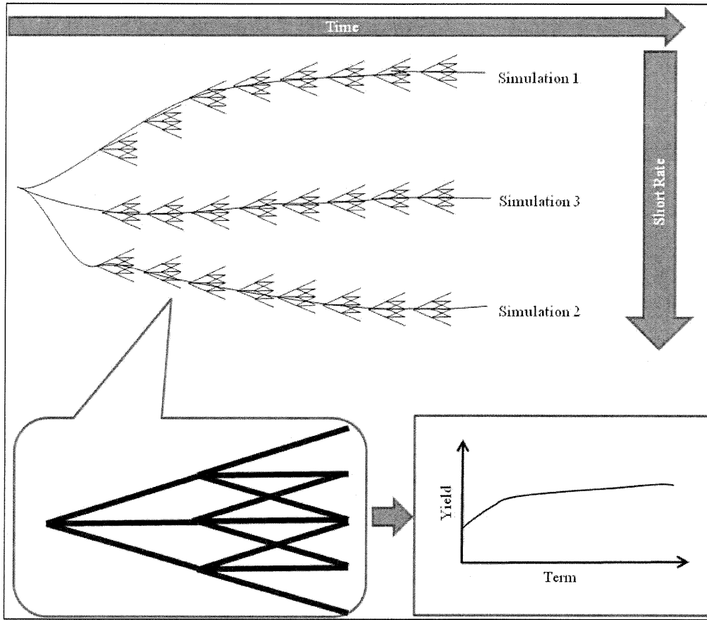
Figure 5.3: Simulating future term-structures by nesting lattices within simulations
