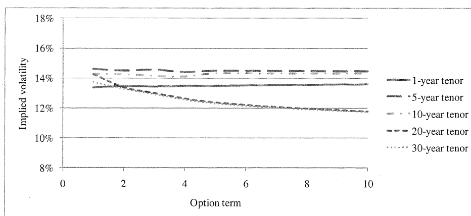
Figure 7.6: Implied volatility on swaptions before any shocks
