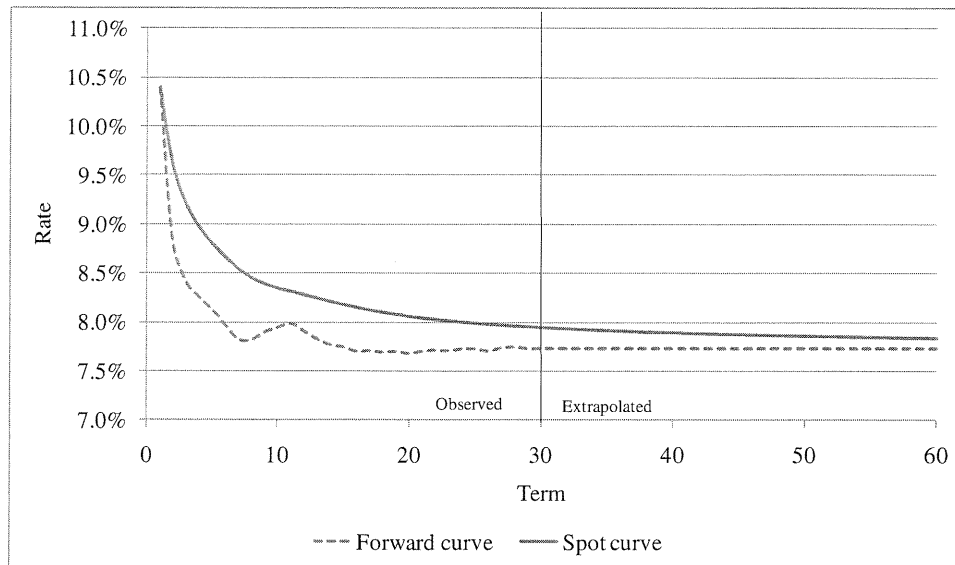
Figure 5.5: Extrapolation of spot curve by assuming constant forward curve
