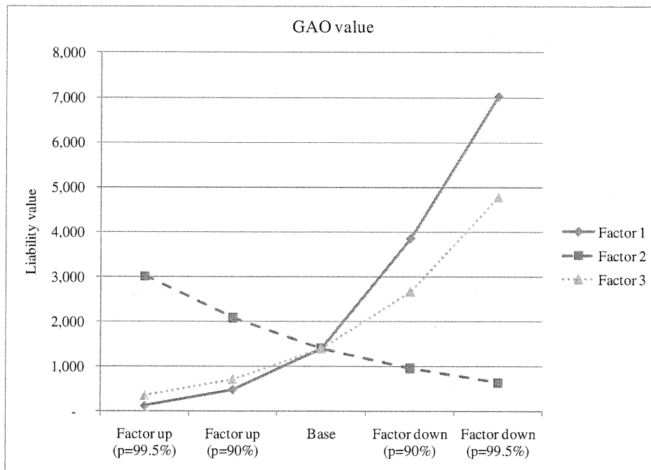
Figure 8.2: Sensitivity of GAO reserves to the changes in term structure of interest rates
