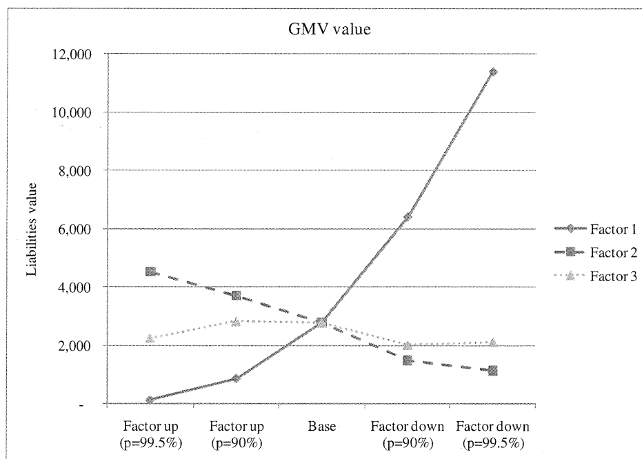
Figure 8.1: Sensitivity of GMV reserves to the changes in term structure of interest rates
