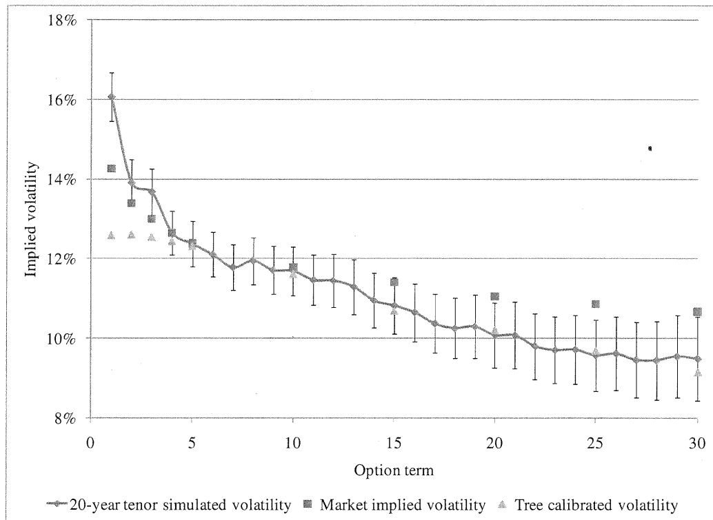
Figure 5.7: A comparison of implied volatilities of receiver swaptions with 20-year tenor: market, simulated and interest-rate lattice
