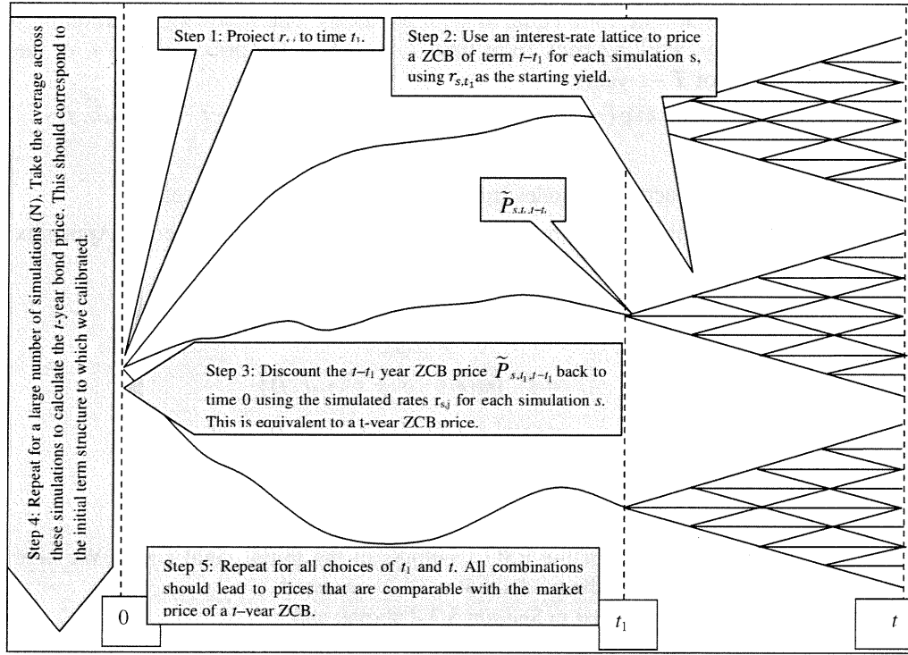
Figure 5.4: Illustration of the testing of future term structures
