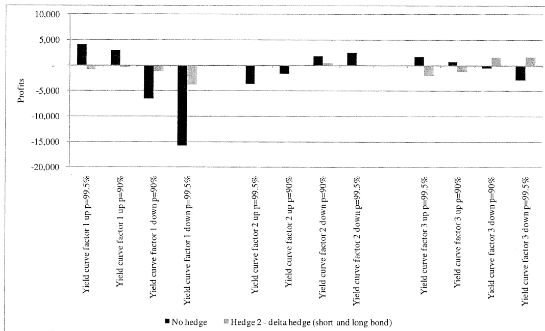
Figure 8.6: Comparison of the value at risk between (a) no hedge, and (b) duration hedge with a long and short positions in ZCBs of 30 and 29 years respectively
