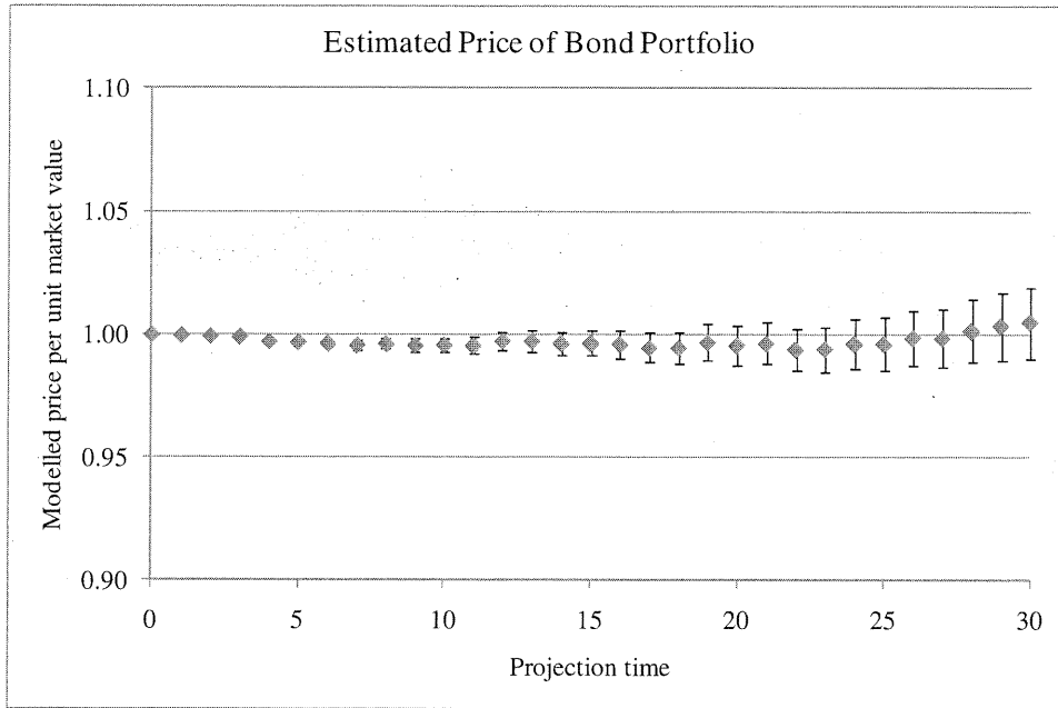
Figure 5.9: Martingale test for a bond portfolio with six ZCBs in equal weightings
