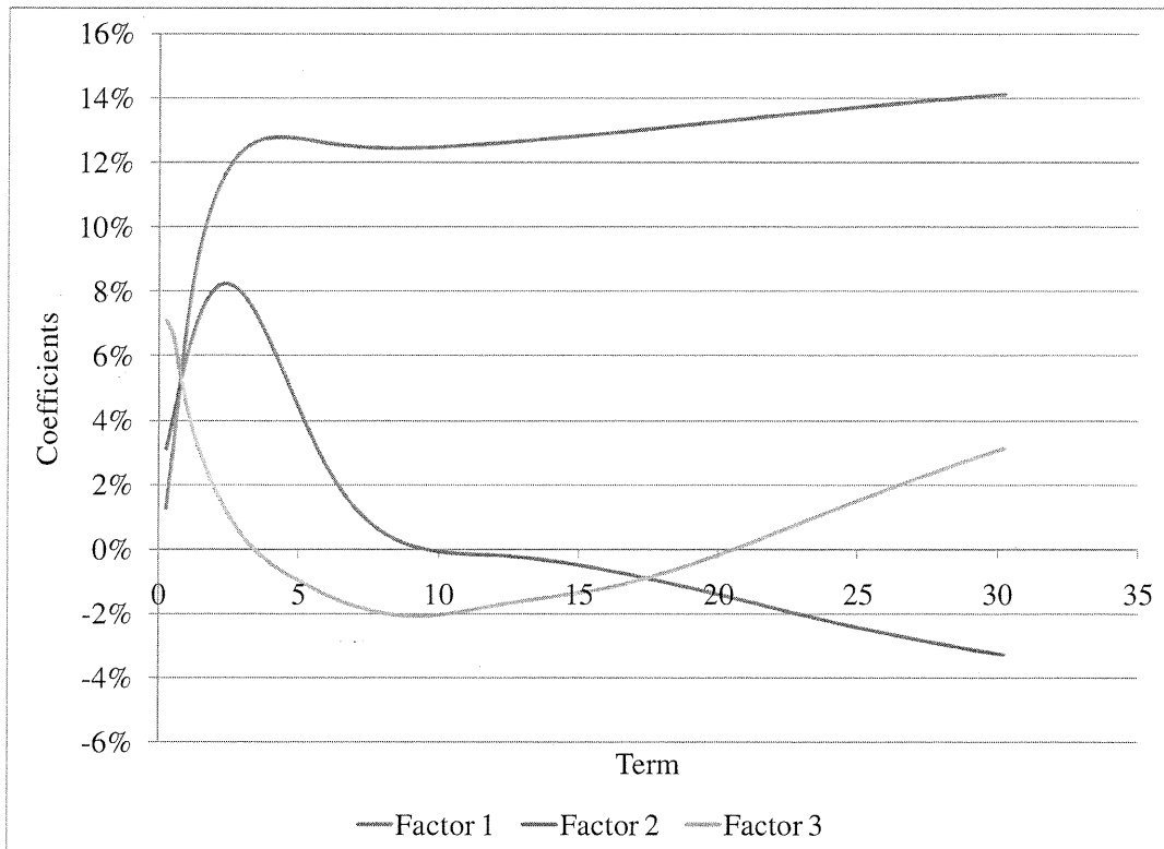
Figure 7.1: Coefficients for mapping observations from the old axes to the new axes
