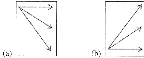
Figure 5.13: Trimming of the tree at the (a) uppermost and (b) lowermost nodes respectively
