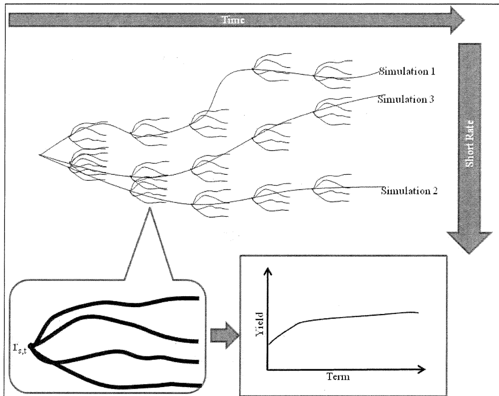
Figure 5.2: Simulating future term-structures by nested simulations
