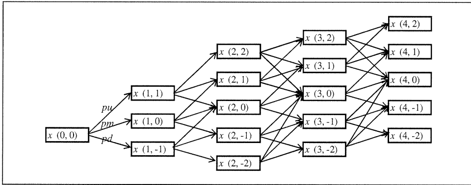
Figure 5.15: Stage 2 trimmed lattice
