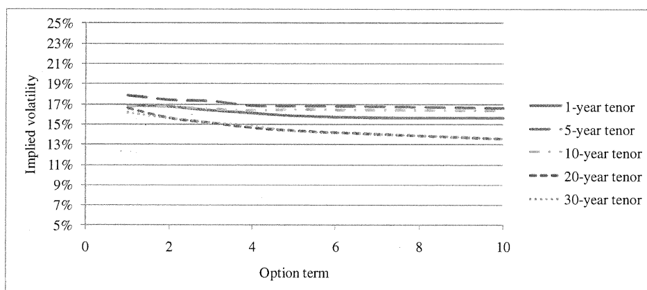
Figure 7.7: Implied volatility on swaptions where an upward shock corresponding to a 99.5% confidence is applied to the first factor
