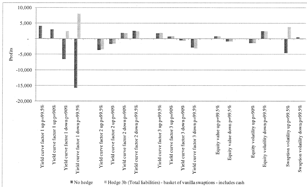
Figure 8.10: Comparison of VaR of all guarantee liabilities when (a) no hedge is held in respect of the risks; and (b) a hedge consisting of receiver swaptions and cash is held
