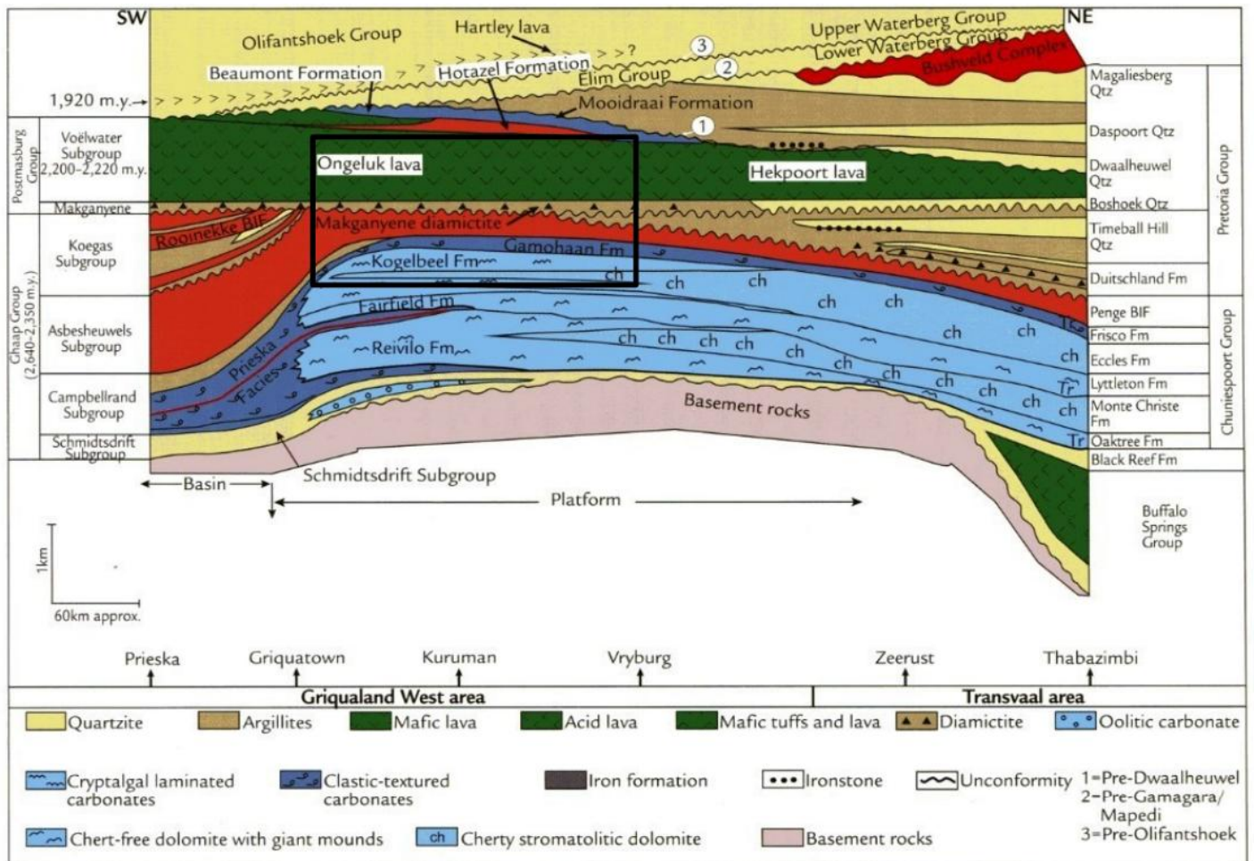
Figure 2.2: The composite stratigraphic column across the Kaapvaal, from Thabazimbi through Vryburg to Prieska (Almond, 2018).
