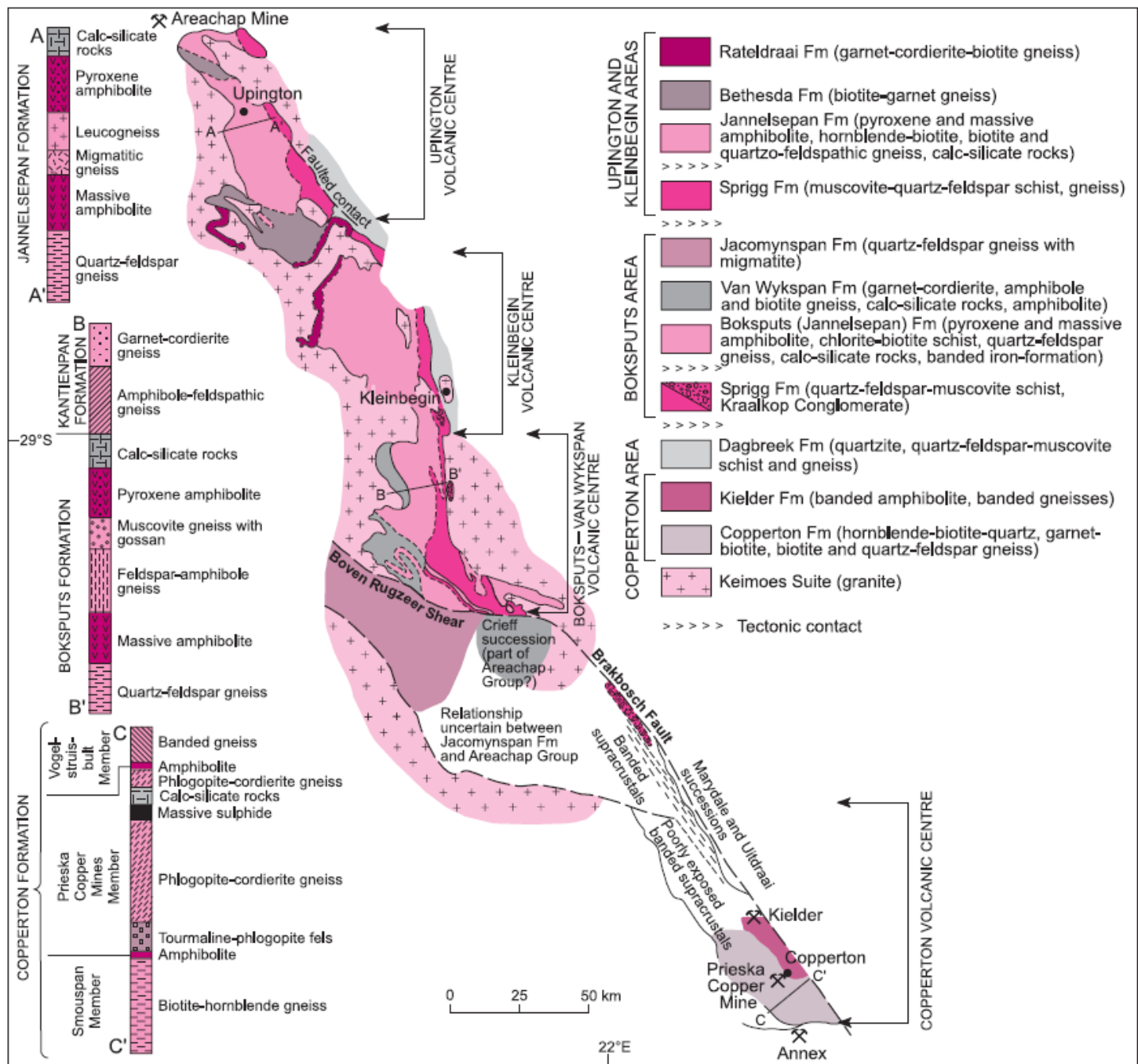
Figure 2.3: The Map illustrating the Areachap Group volcanic centres Lithostratigraphy (after Cornell et al., 2006 and references therein).
