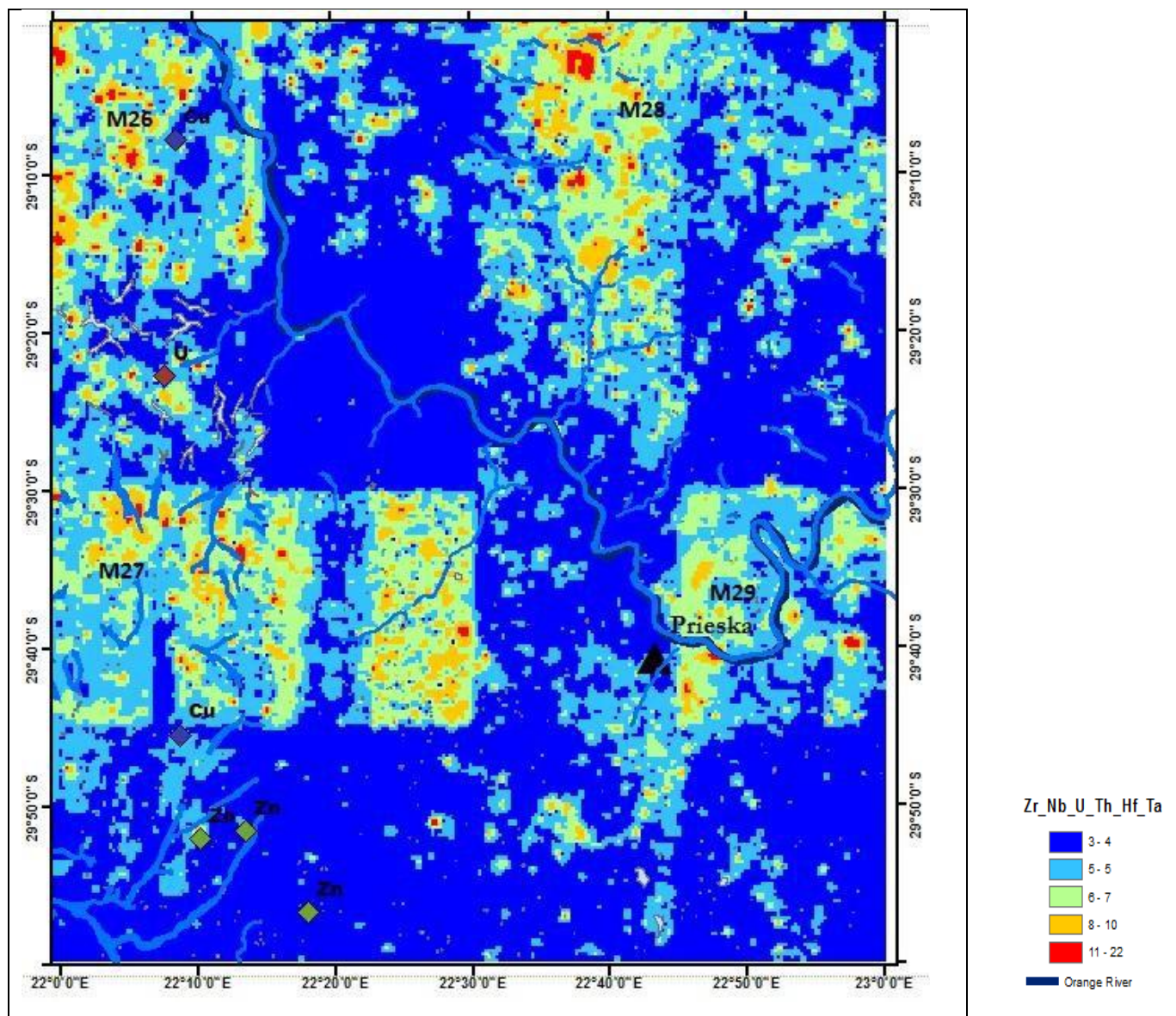
Figure 4.4.3: the Fuzzy OR overlay of Zr_Nb_U_Th_Hf_Ta
