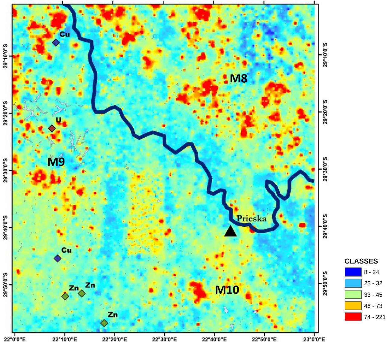
Figure 4.3.3: the Fuzzy OR overlay of Mo, Nb, Sc, Ta, and U
