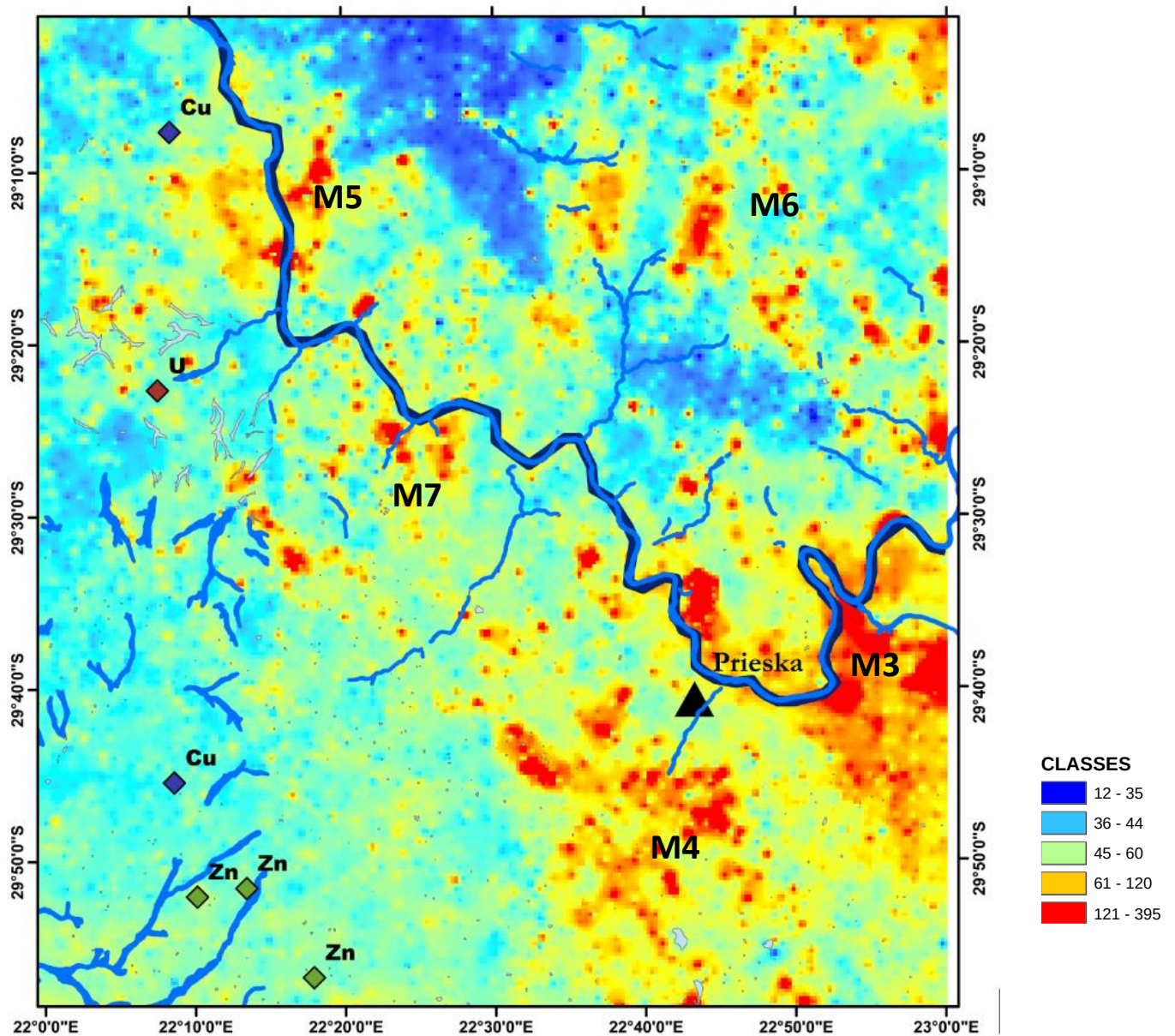
Figure 4.3.2: the Fuzzy OR overlay multi-element map index of Co and Ni
