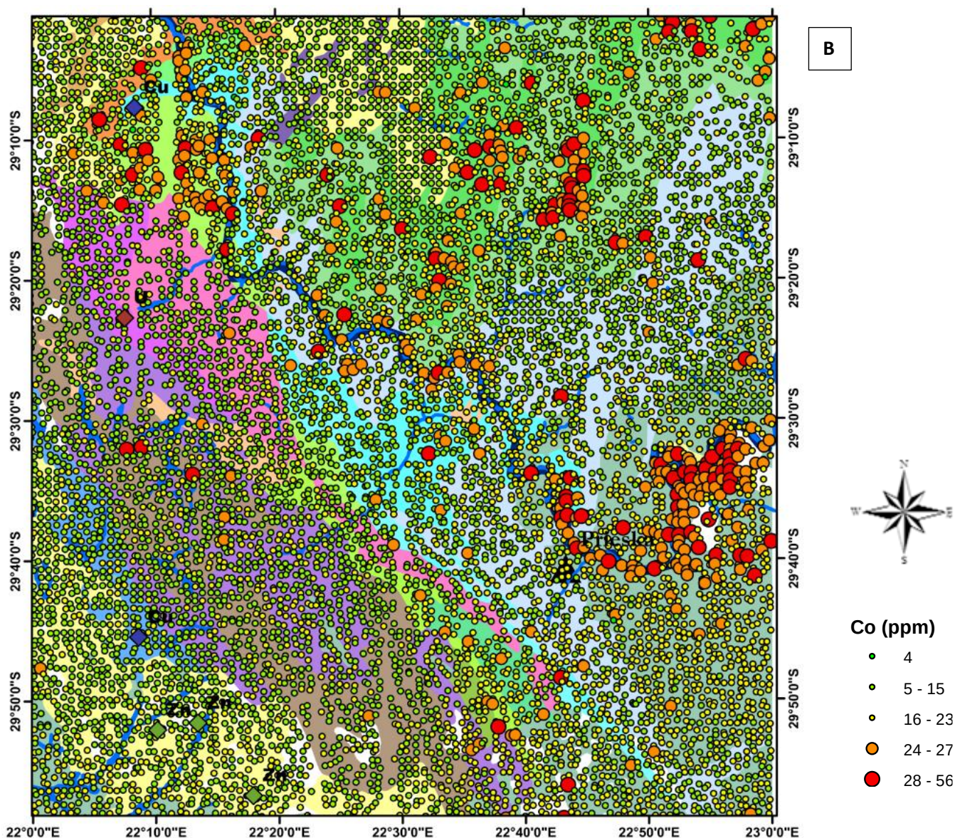
Figure 4.1.2 a) Histogram frequency distribution showing the skewness and Kurtosis of Co (ppm) dataset, b) The Regional geochemical distribution map illustrating the location of Co (ppm) anomalies.
