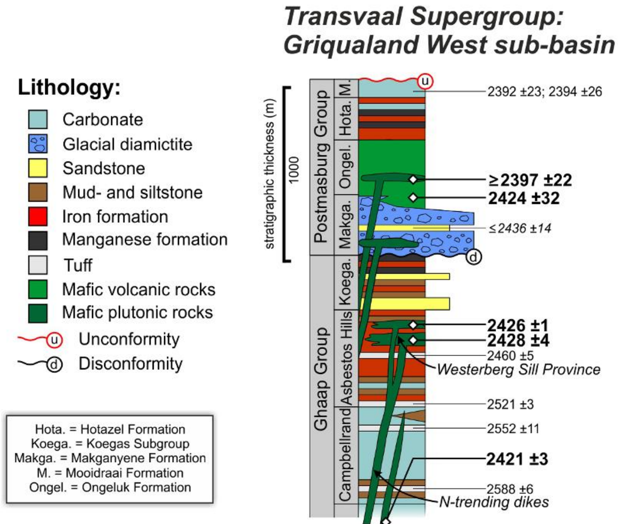
Figure 2.7: The Lithostratigraphy of the upper Transvaal Supergroup as preserved in the Griqualand West basin (Gumsley, A. 2017).
