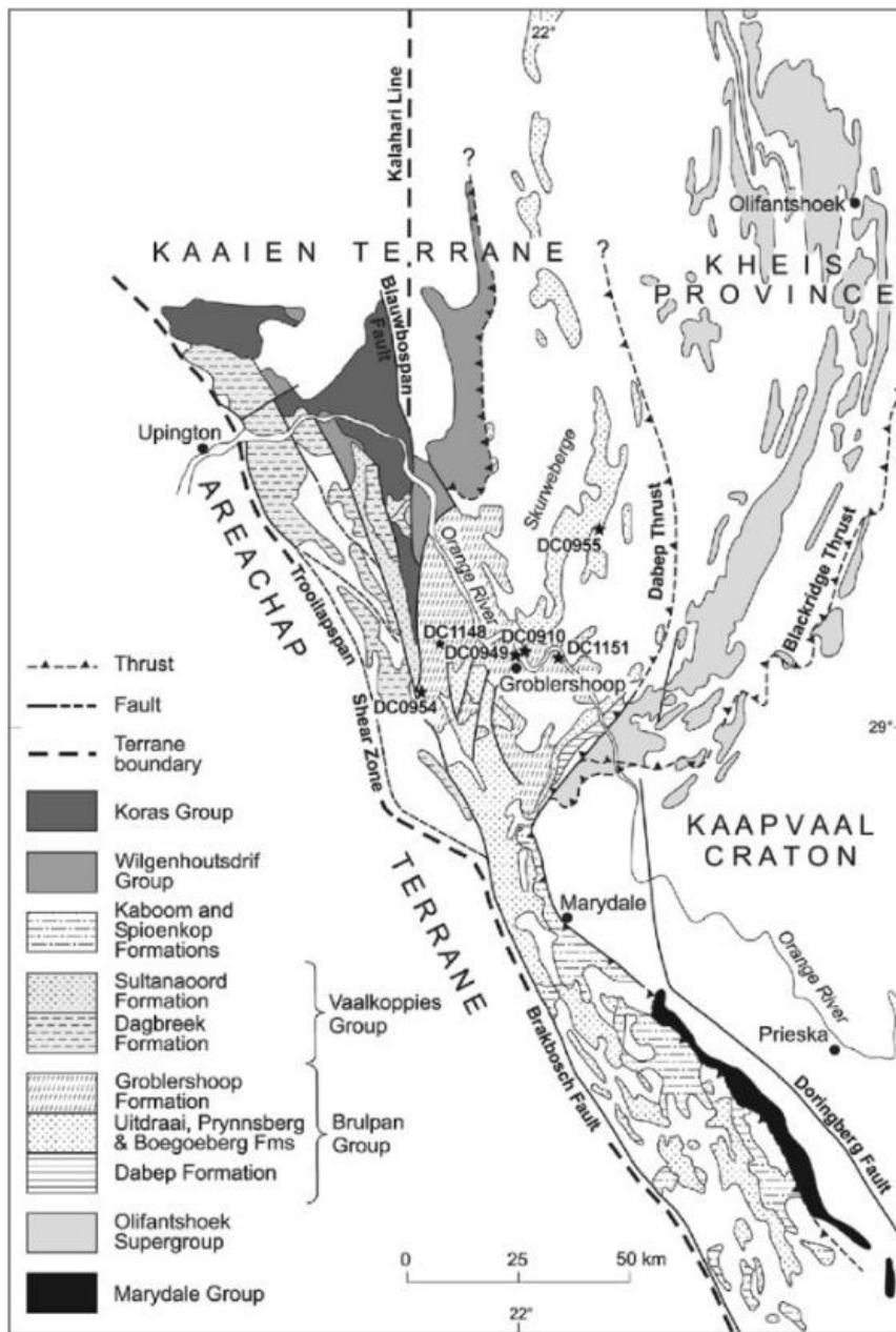
Figure 2.4: The Map illustrating the Lithostratigraphy of the Kaaian Terrane and Kheis Province (van Schijndel et al., 2019).
