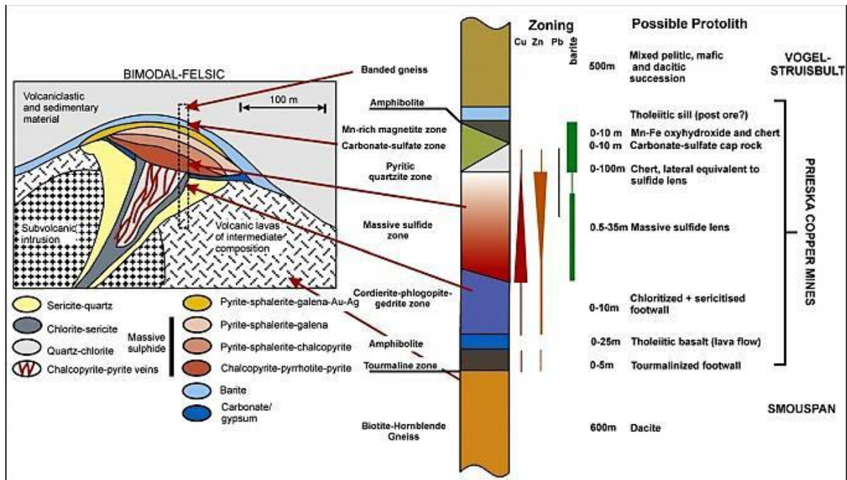
Figure 2.9: A simplified architecture of the Copperton deposit as related to a model of a biomodal felsic type of VMS deposit. (Baillie and Gutzmer, 2011 and reference therein; Theart et al. , 1989).
