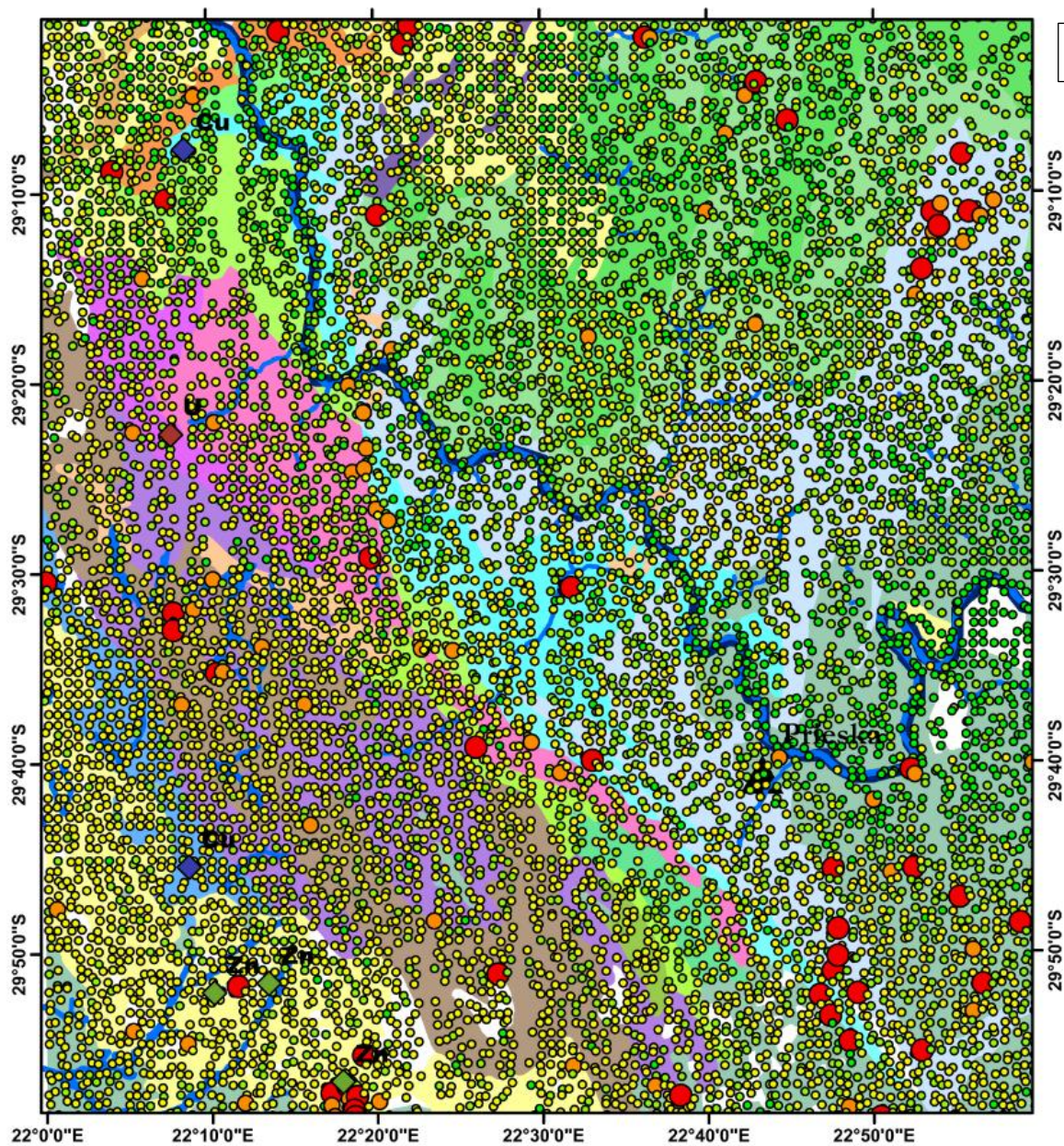
Figure 4.1.5 a) Histogram frequency distribution showing the skewness and Kurtosis of Pb (ppm) dataset, b) The Regional geochemical distribution map illustrating the location of Pb (ppm) anomalies.
