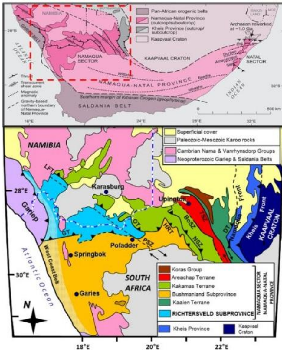
Figure 2.1: a) The NNMP stretching from Namibia to the Tugela Valley and b) The Tectono-stratigraphic position of the Namaqua sector of the NNMP. : GT= Grootfontein Thrust; OT = Onseepkans Thrust; PSZ = Pofadder Shear-zone; HRT = Hartbees River Thrust; BRSZ = Buffels River Shear-zone; NSZ = Neusberg Shear-zone; BoSZ = Boven Rugzeer Shear-zone; BSZ = Brakbos Shear-zone; DT= Dabep Thrust.
