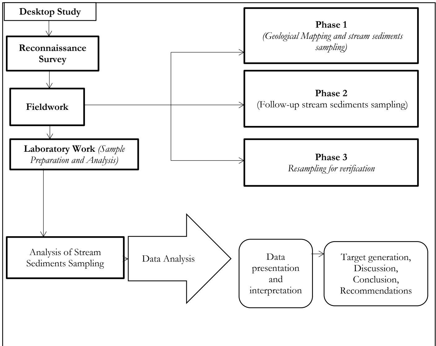
Figure 3.1 Flow chart indicating methods and procedures applied during the study.
