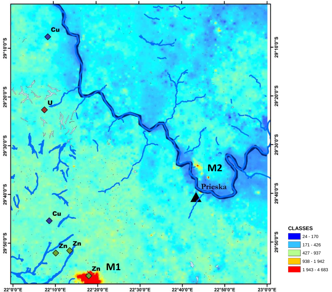
Figure 4.3.1: Fuzzy OR overlay multi-element map index of Cu, Ga, Zn, and Rb
