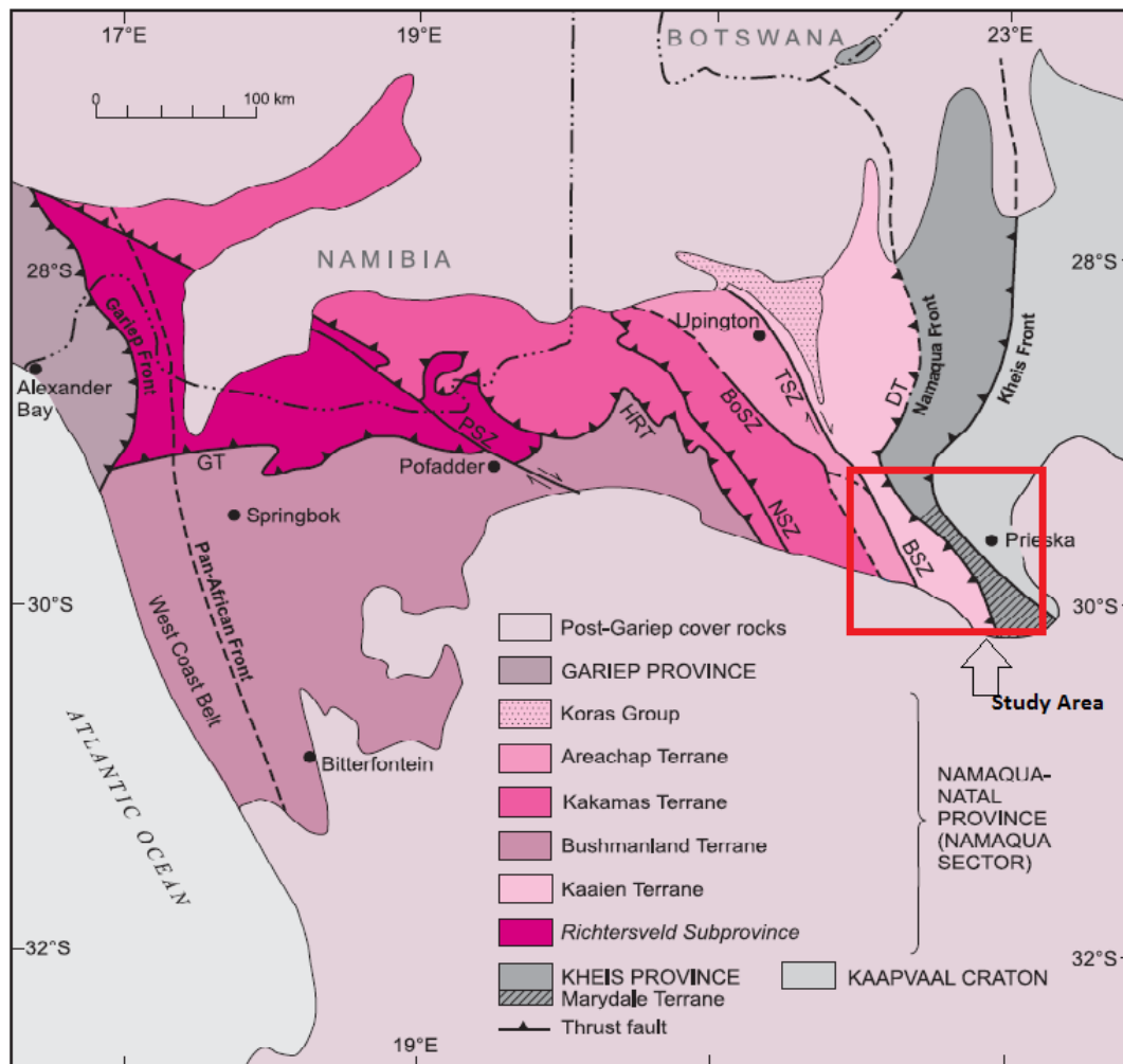
Figure 1.1: The Map of different terranes in the Namaqua Sector. (Duchesne et al., 2007)
