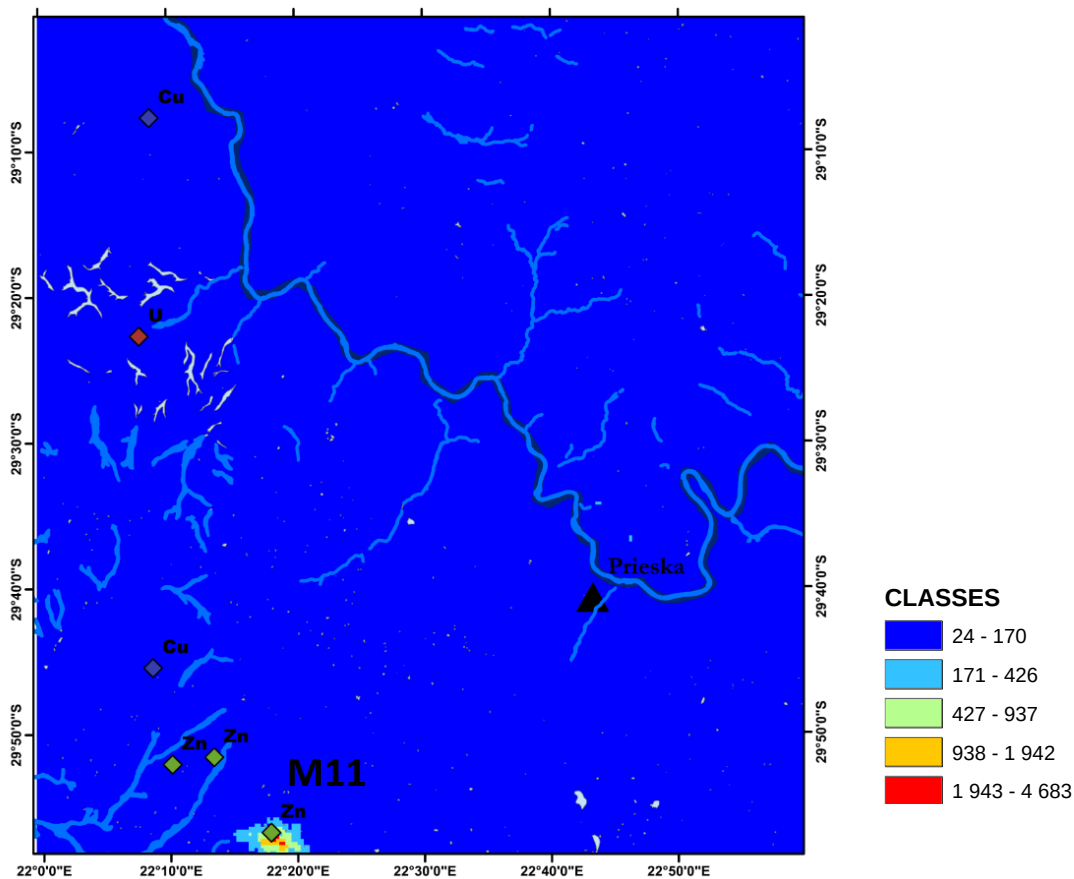
Figure 4.4.1: the Fuzzy OR overlay map for Cu_Zn index.
