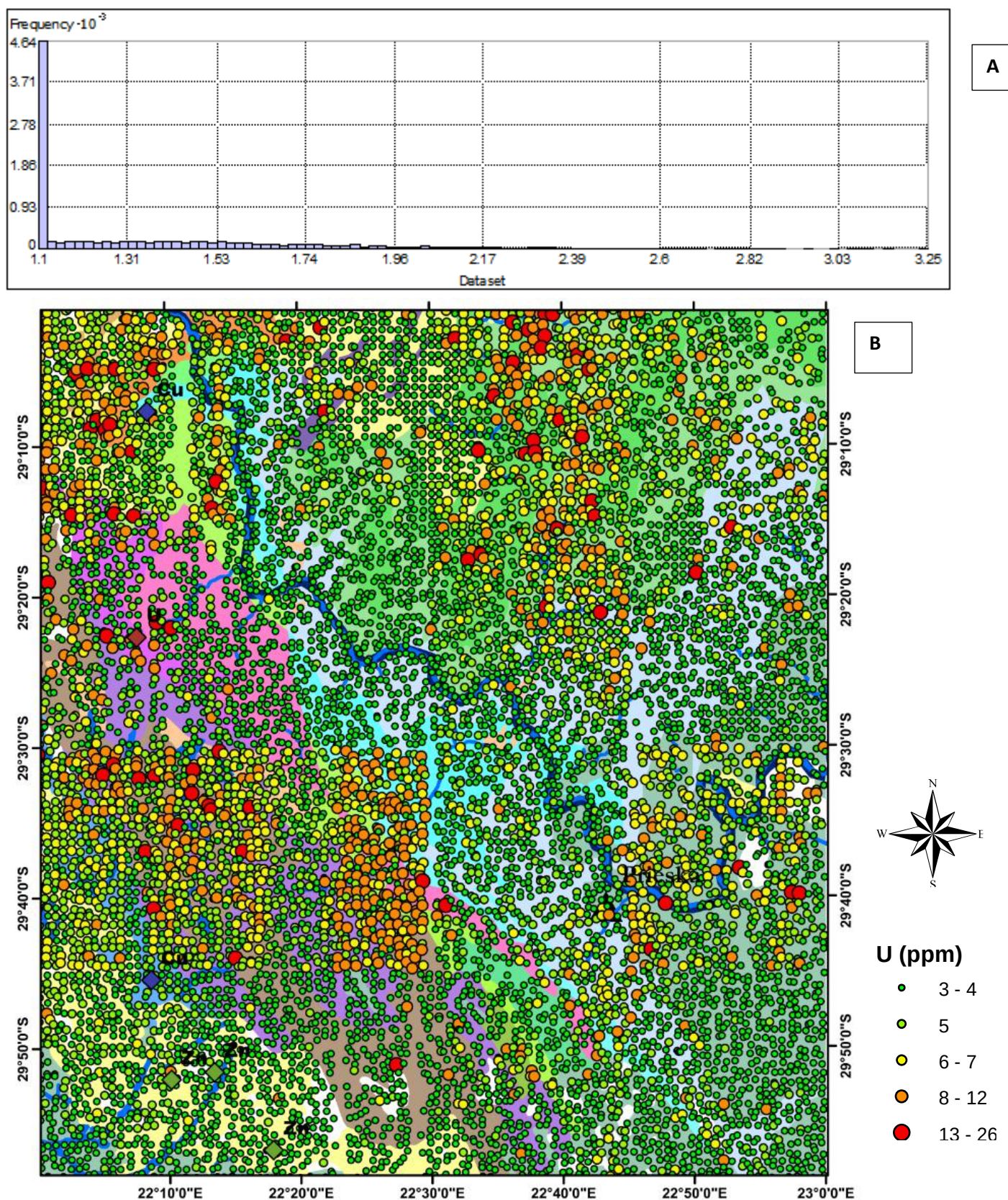
Figure 4.1.6 a) Histogram frequency distribution showing the skewness and Kurtosis of U (ppm) dataset, b) The Regional geochemical distribution map illustrating the location of U (ppm) anomalies.
