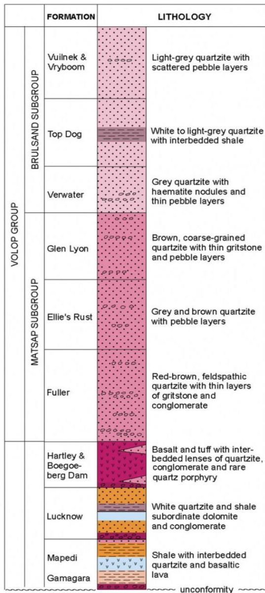
Figure 2.6: The stratigraphy of the Olifantshoek Supergroup. (Cornell et al. , 2016).
