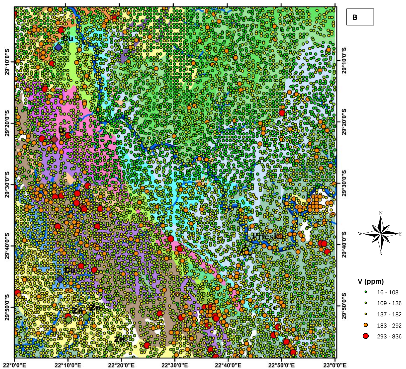
Figure 4.1.7 a) Histogram frequency distribution showing the skewness and Kurtosis of V (ppm) dataset, b) The Regional geochemical distribution map illustrating the location of V (ppm) anomalies.
