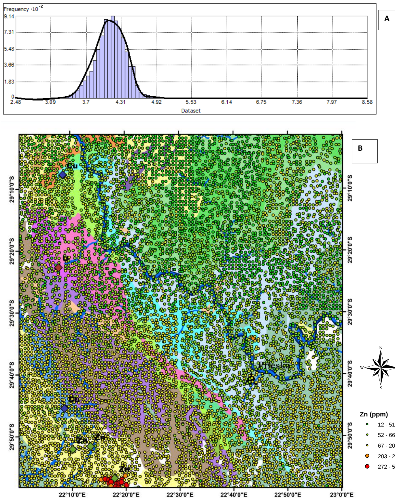
Figure 4.1.8 a) Histogram frequency distribution showing the skewness and Kurtosis of Zn (ppm) dataset, b) The Regional geochemical distribution map illustrating the location of Zn (ppm) anomalies.
