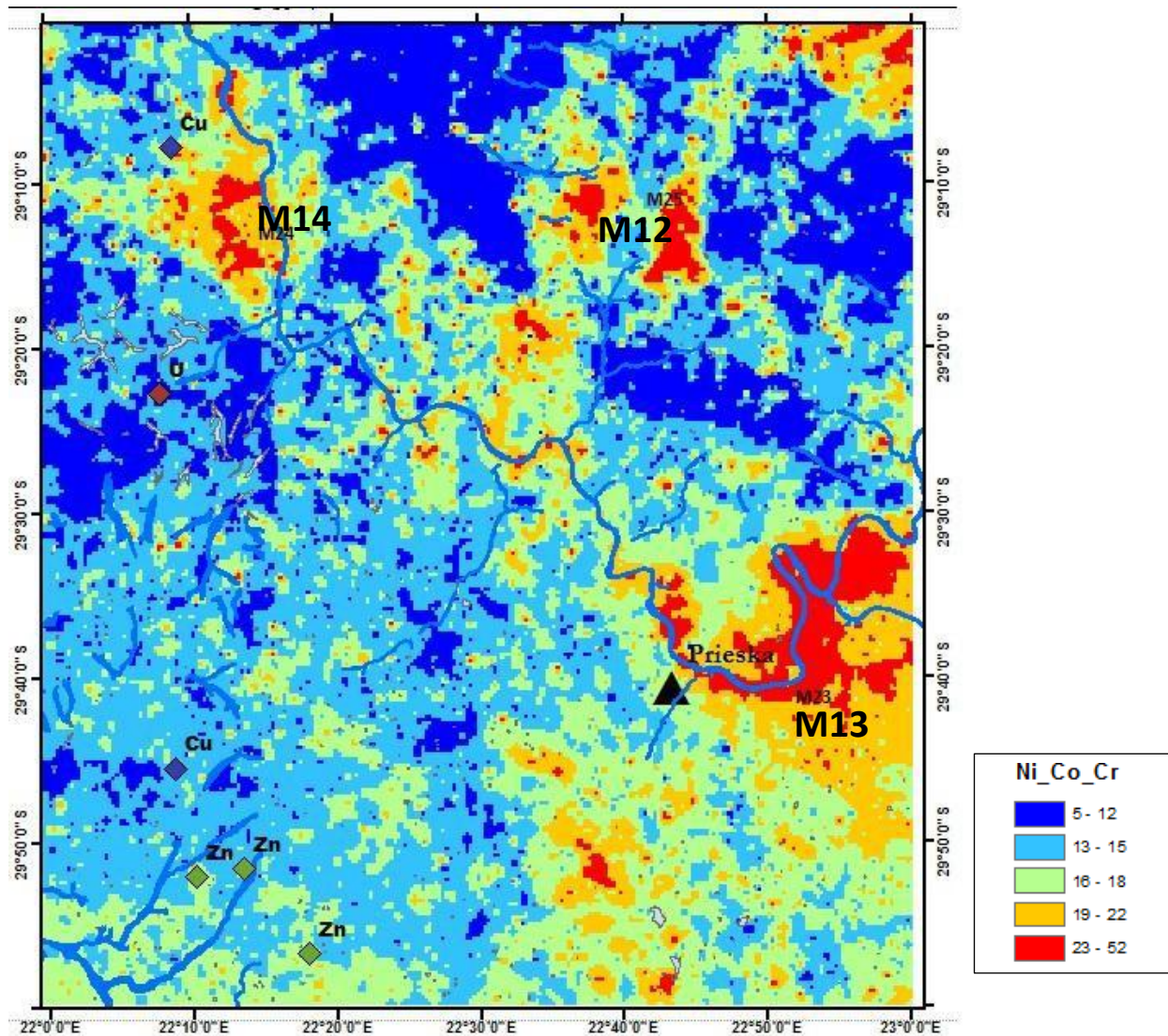
Figure 4.4.2: the Fuzzy OR overlay map for Ni, Co and Cr index.
