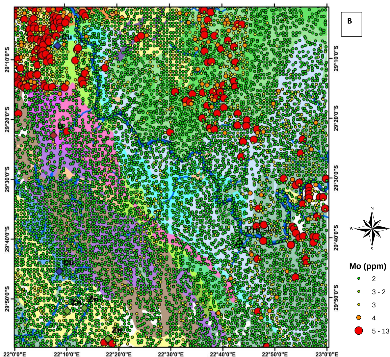
Figure 4.1.4 a) Histogram frequency distribution showing the skewness and Kurtosis of Mo (ppm) dataset, b) The Regional geochemical distribution map illustrating the location of Mo (ppm) anomalies.
