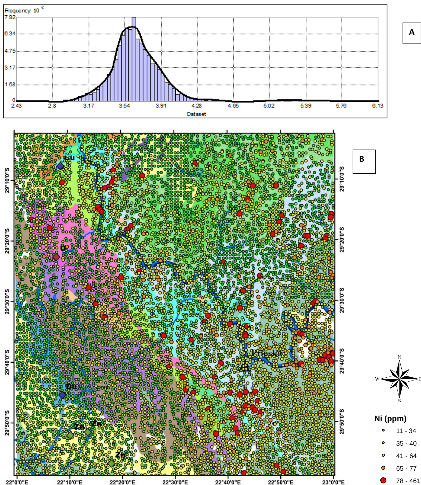
Figure 4.1.10 a) Histogram frequency distribution showing the skewness and Kurtosis of Ni (ppm) dataset, b) The Regional geochemical distribution map illustrating the location of Ni (ppm) anomalies.
