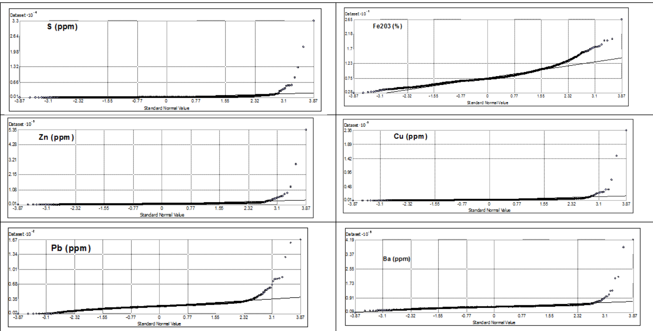
Figure 4.2: Normal Q-Q plots for data after none transformation, in order to preserve symmetry for the expected values (y-axis) negative values (observed values) on the x-axis are included.
