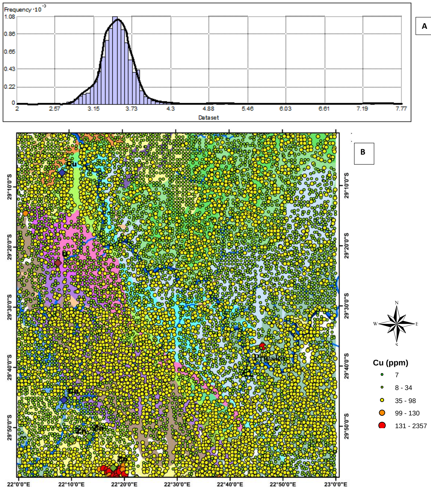
Figure 4.1.3 a) Histogram frequency distribution showing the skewness and Kurtosis of Cu (ppm) dataset, b) The Regional geochemical distribution map illustrating the location of Cu (ppm) anomalies.
