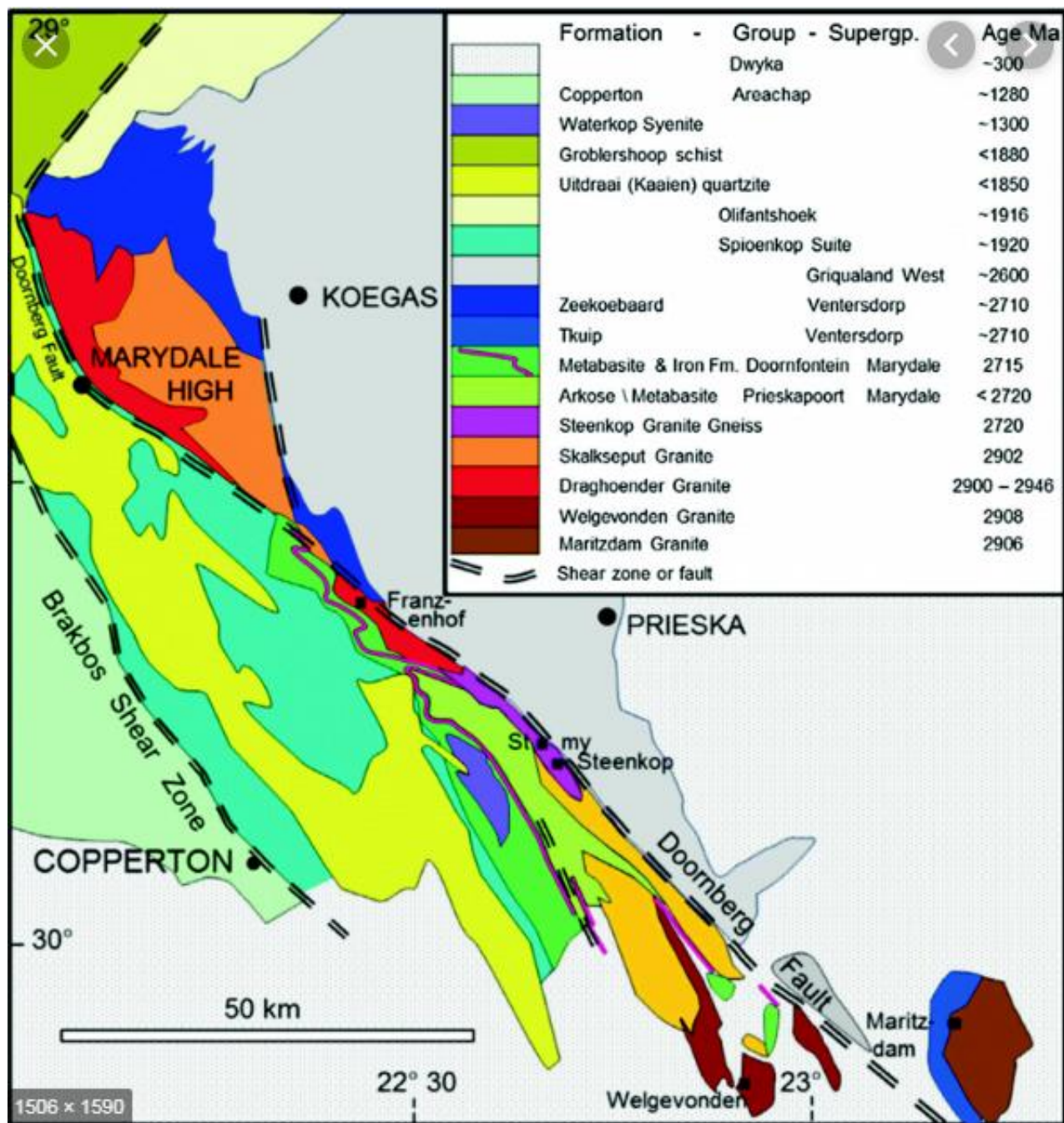
Figure 2.8: The 2922 Prieska map illustrating the lithostratigraphy from the Maritzdam Granite to the Copperton Formation. (Modified after Anhaeusser, 2019).
