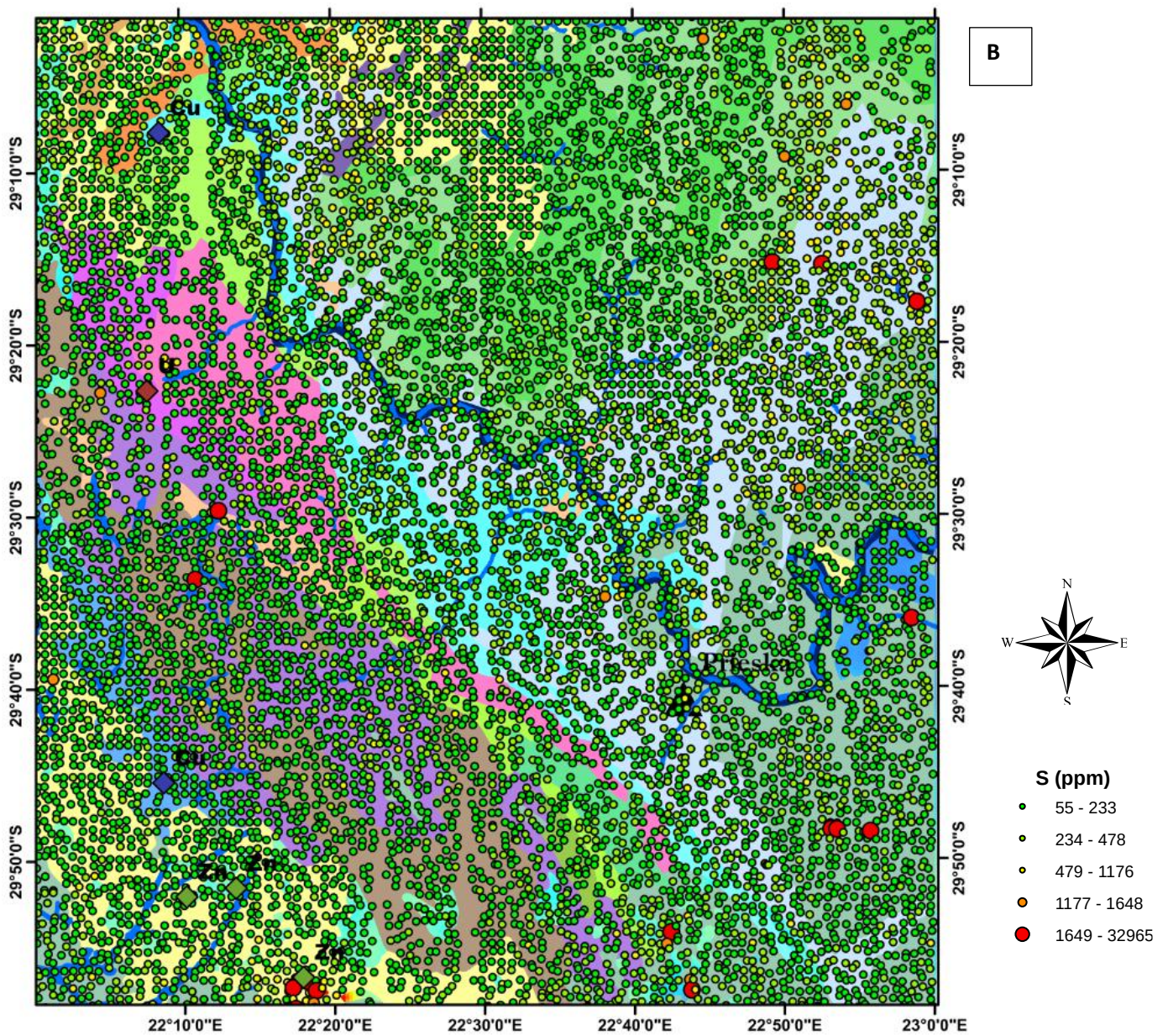
Figure 4.1.9 a) Histogram frequency distribution showing the skewness and Kurtosis of S (ppm) dataset, b) The Regional geochemical distribution map illustrating the location of S (ppm) anomalies.
