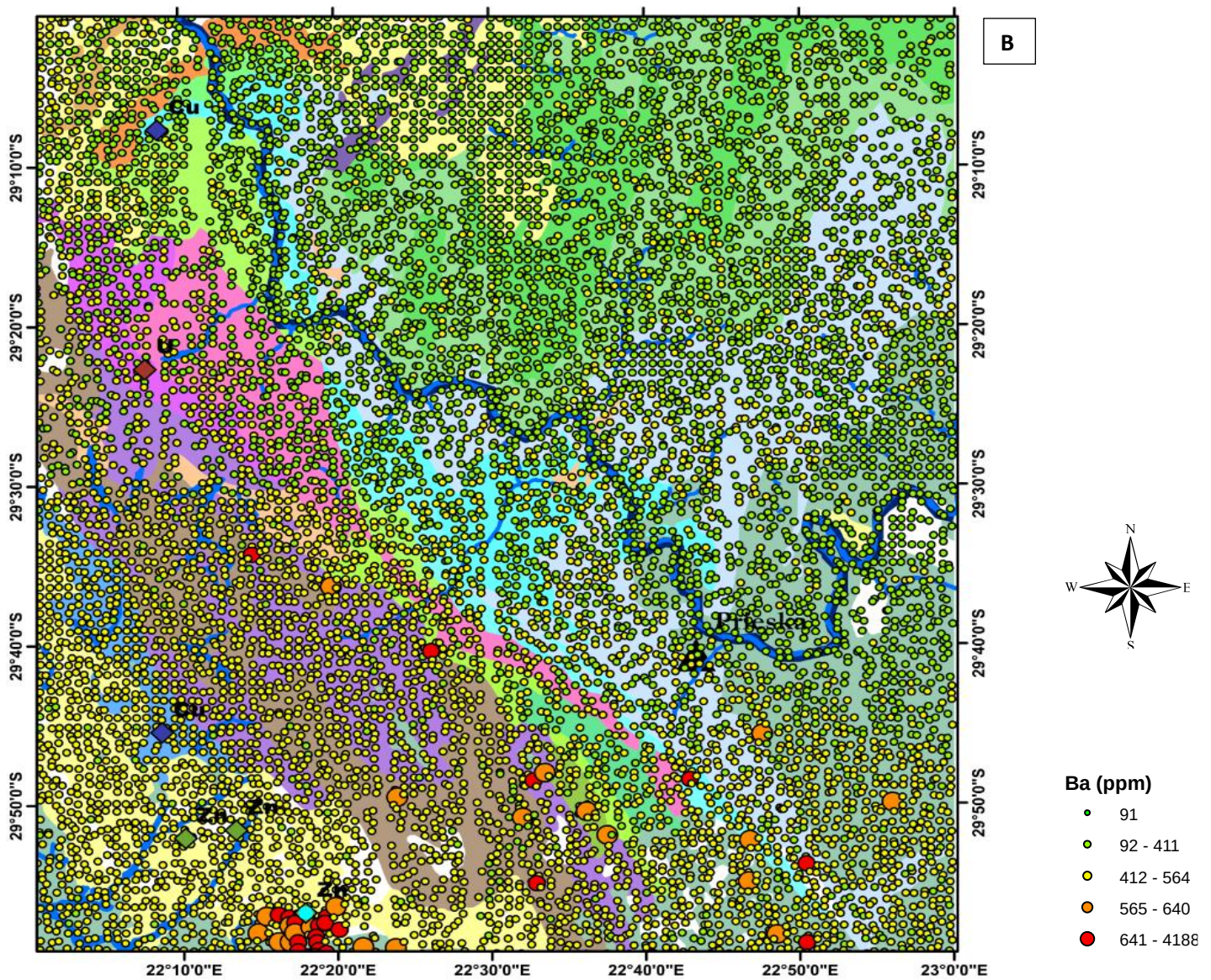
Figure 4.1.1 a) Histogram frequency distribution showing the skewness and Kurtosis of Ba (ppm) dataset, b) The Regional geochemical distribution map illustrating the location of Ba (ppm) anomalies.
