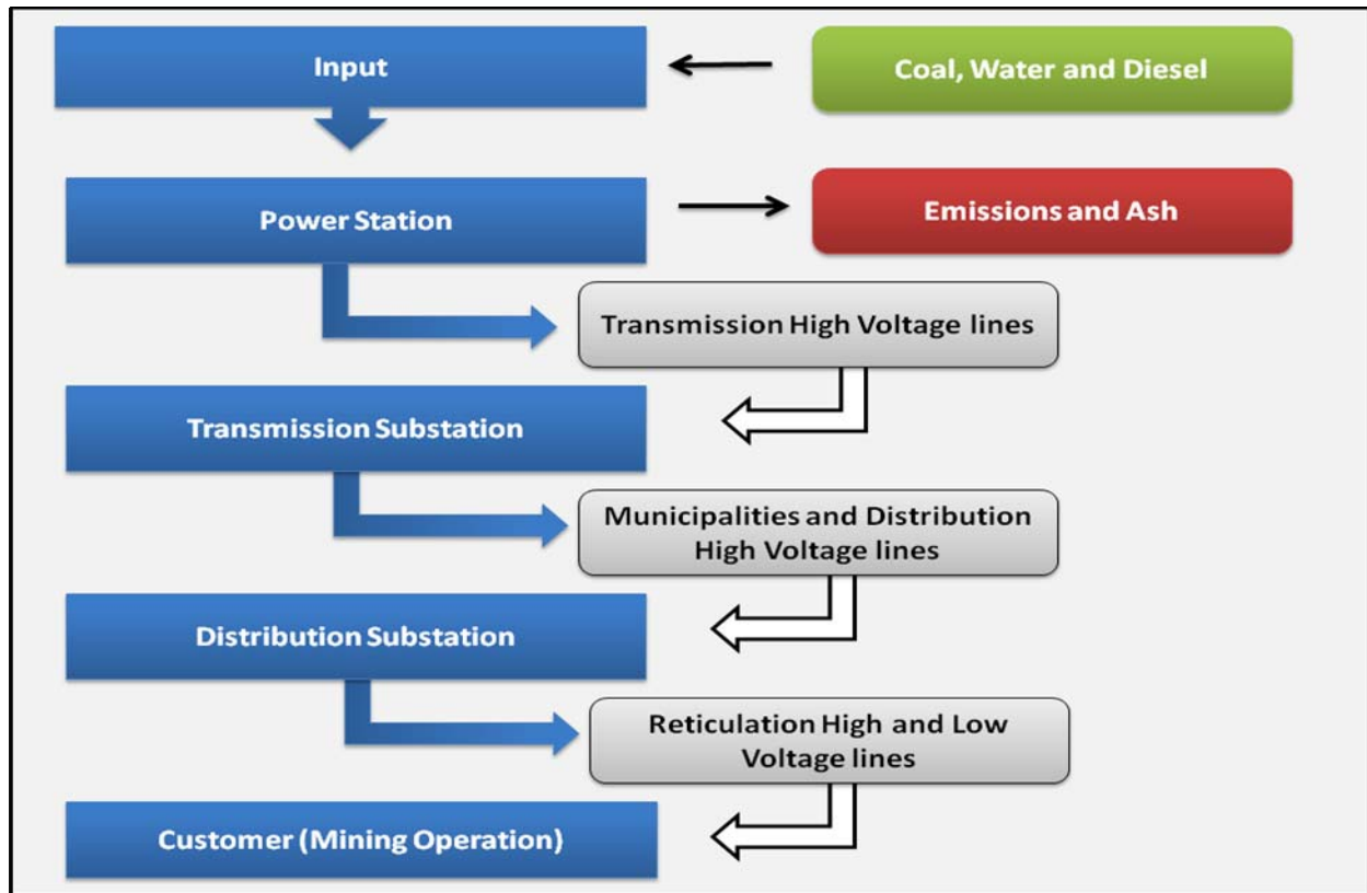
Figure 9: Electricity generation, transmission and distribution (Eskom, 2009).
