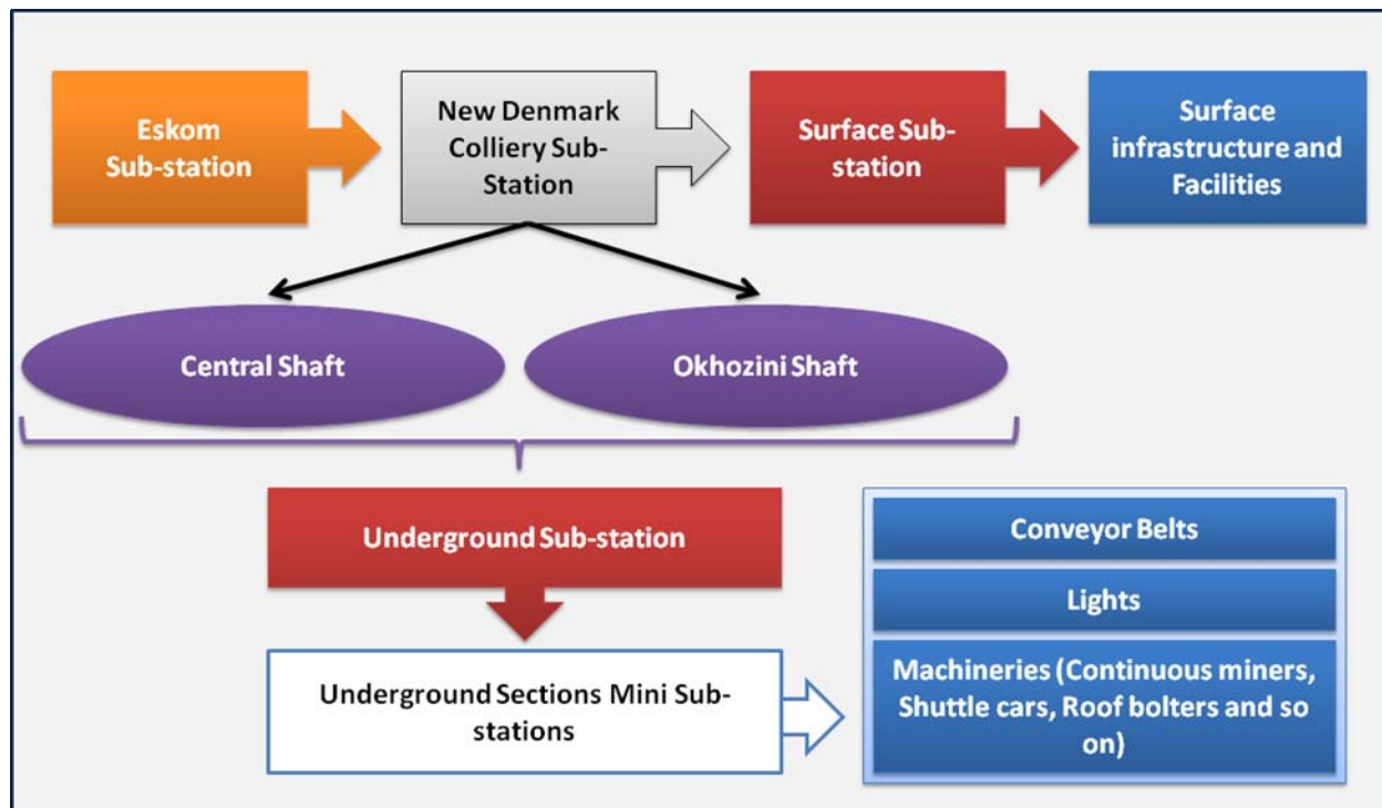
Figure 27: Transmission and distribution of energy at New Denmark Colliery.
