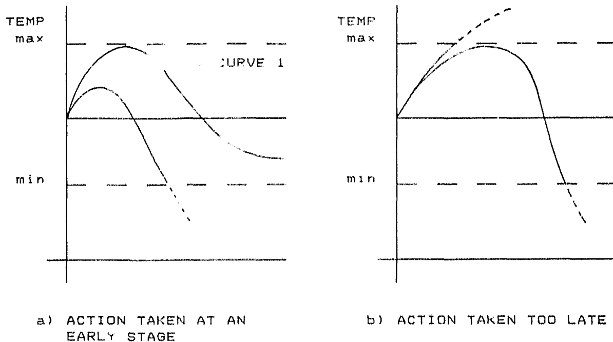
FIGURE 2.4: OPERATOR REACTION TO POTENTIALLY CRITICAL TEMPERATURE RISES
