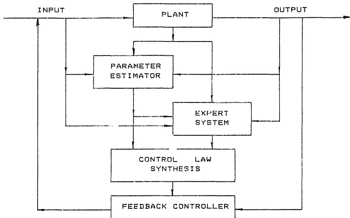
FIGURE 2.2: THE ROLE OF EXPERT SYSTEMS IN ADAPTIVE CONTROL
