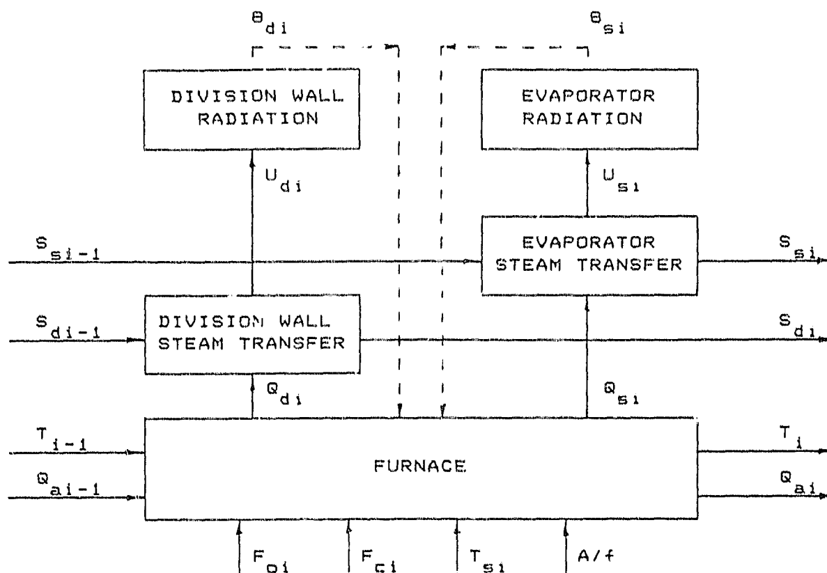
FIGURE 4.3: THE BLOCK DIAGRAM OF THE MODEL FOR THE I'TH CELL
