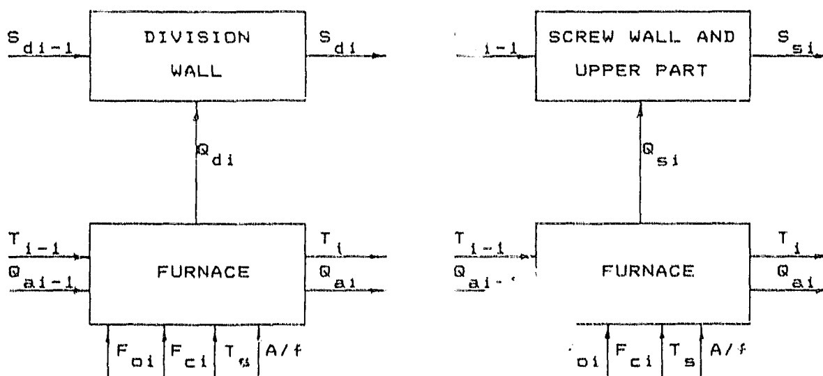
FIGURE 4.4: THE BLOCK DIAGRAM OF THE MODELS FOR THE EVAPORATOR AND THE DIVISION WALL
