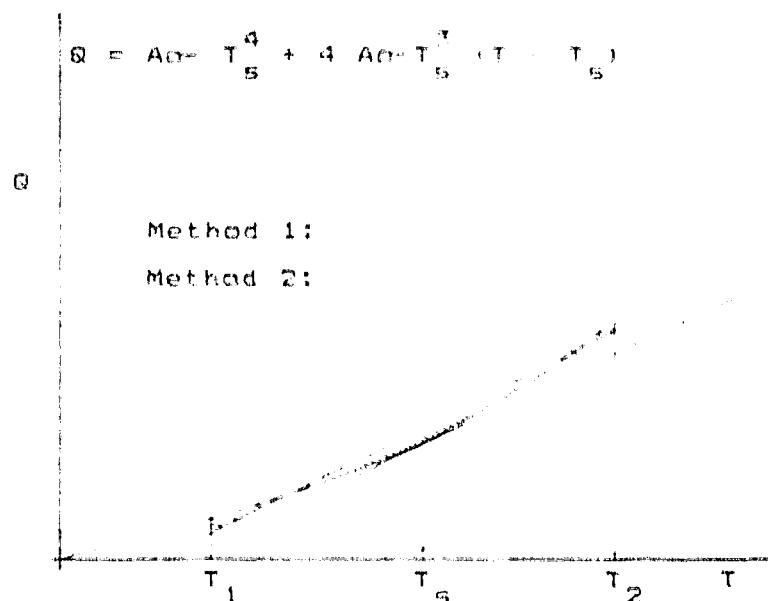
FIGURE A.1: LINEARIZATION OF THE HEAT RADIATION EQUATION
