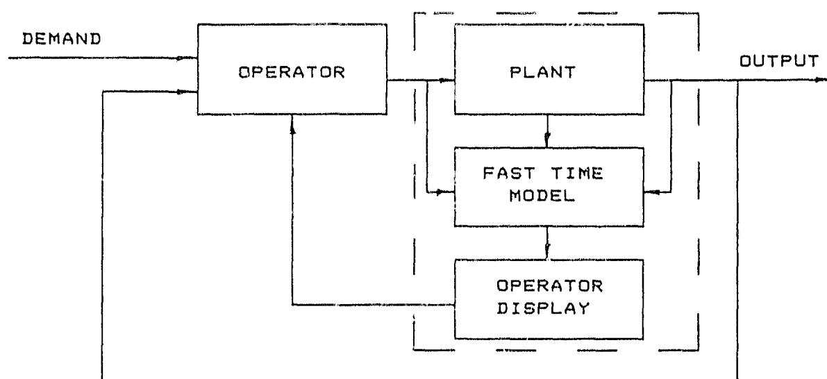
b) PLANT CONTROLLED BY OPERATOR WITH AID OF PREDICTOR INSTRUMENT
