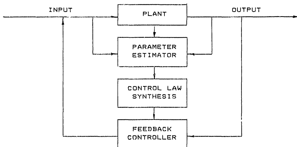
FIGURE 2.1: THE BLOCK DIAGRAM FOR AN ADAPTIVE CONTROLLER
