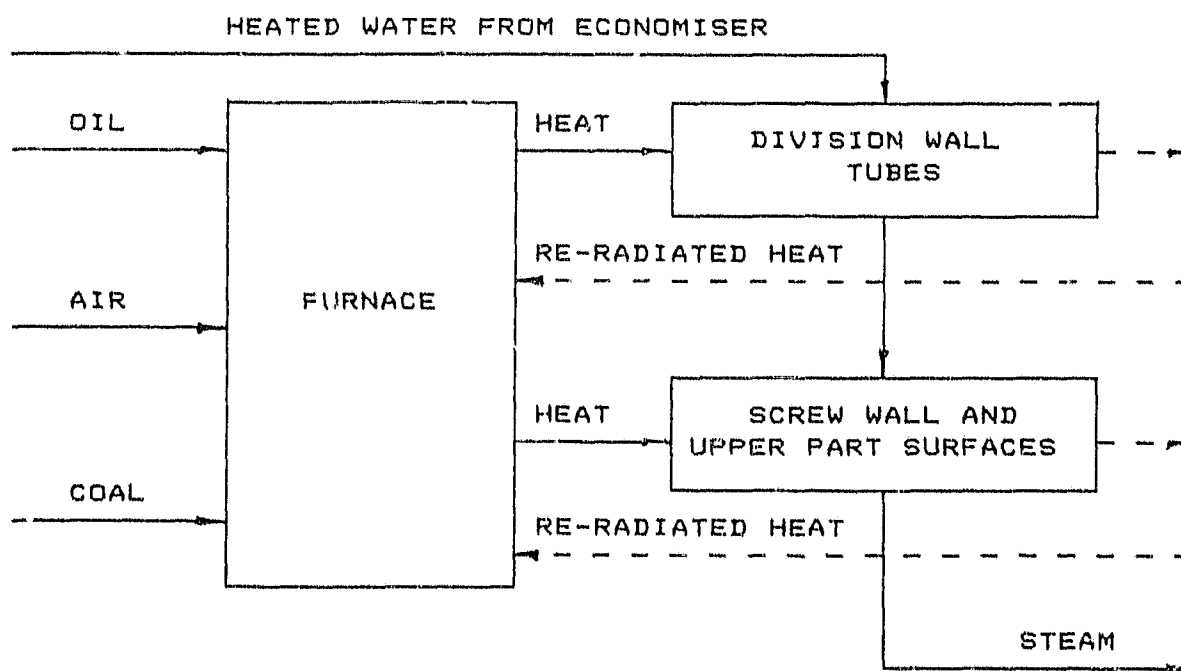
FIGURE 4.1: THE BOILER UNIT SHOWING THE SUB-UNITS OF INTEREST
