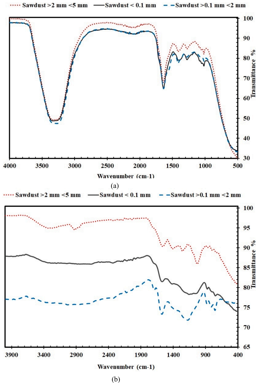
Fig. 7. FTIR spectra of WSD (a) bio-oil and (b) bio-char.
