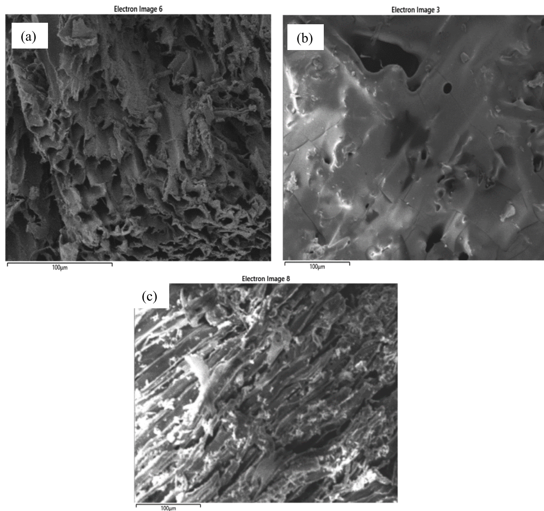
Fig. 8. FESEM image of biochar at particle size (a) < 0.1 mm, (b) (0.5 – 2) mm, and (c) (2.5 – 5) mm, all samples are at 450 °C.
