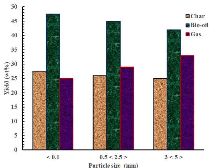
Fig. 4. Particle size influence on the gas, char, and bio-oil, yield.
