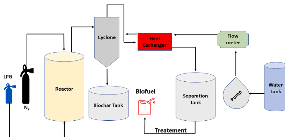
Fig. 1. Sawdust pyrolysis reactor.
