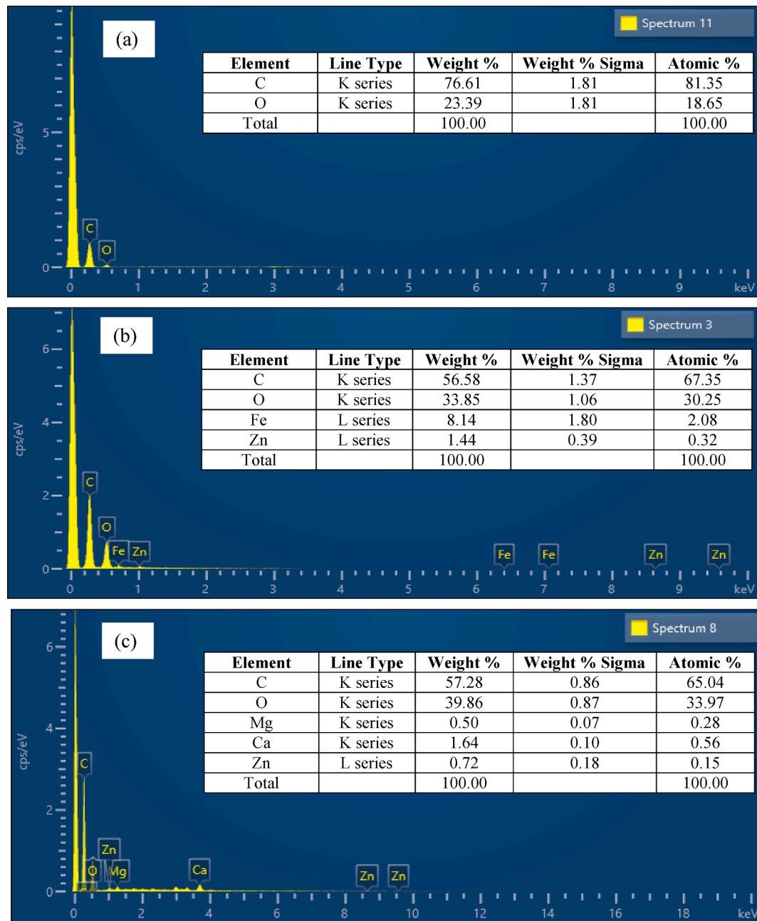
Fig. 9. EDX spectra of biochar particle size (a) < 0.1 mm, (b) (0.5 – 2) mm, and (c) (2.5 – 5) mm, all samples are at 450 °C.
