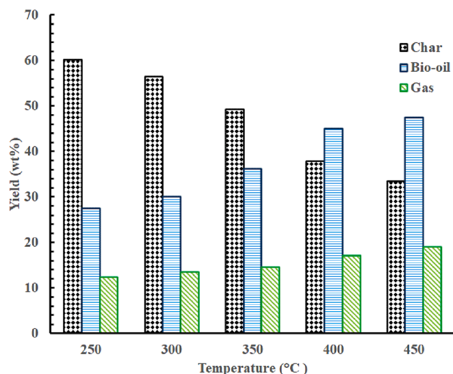
Fig. 3. Temperature influence on gas, char, and bio-oil pyrolysis yield.
