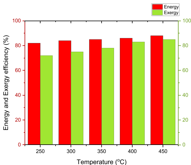
Fig. 6. Energy and exergy efficiency of sawdust pyrolysis at various temperatures.
