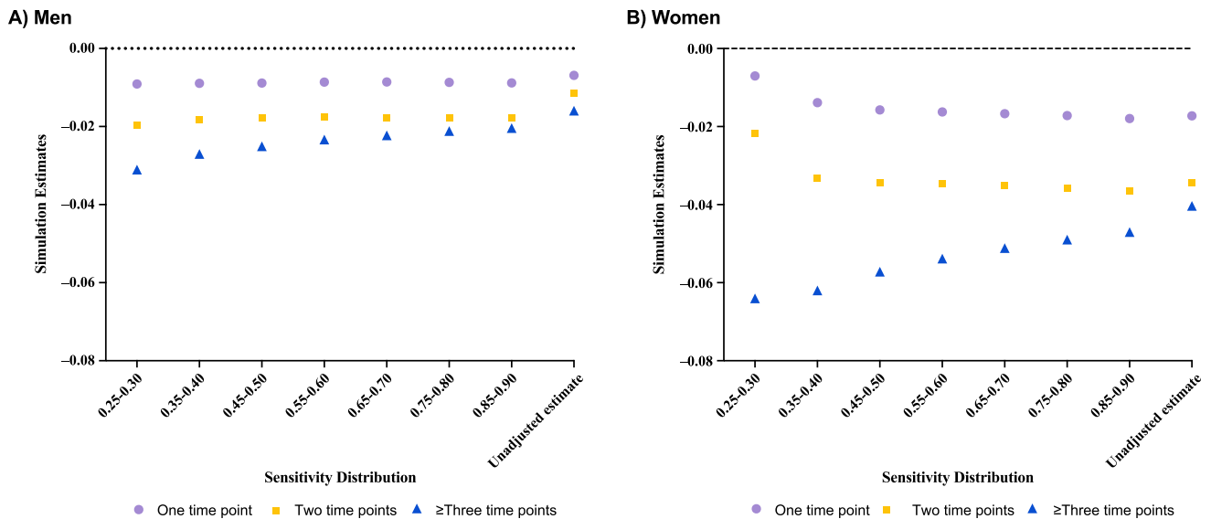
Figure 3. Gender-specific simulation estimates for the interaction between loneliness exposure duration (categorical) and years of follow-up, the US Health and Retirement Study ( n = 9032 ), 1996–2016. These estimates were from gender-stratified subgroup analyses: A) men; B) women. We conducted additional pooled analyses to derive gender-specific simulation estimates (Figure S3). Results were consistent with those shown in Figure 3.
