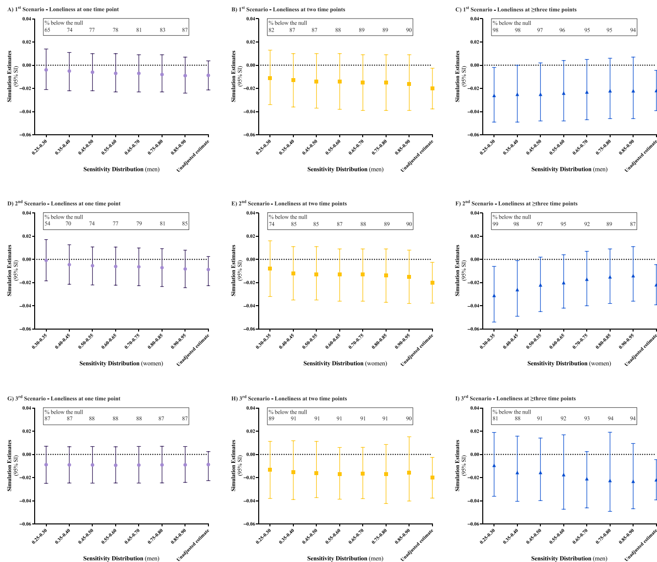
Figure 4. Simulation estimates and 95% simulation intervals (SIs) for the 3-way interaction between loneliness exposure duration (categorical), years of follow-up (1, 2, and \geq 3 time points in the respective columns), and gender in each of the three simulation scenarios (first, second, and third scenarios in the respective rows), the US Health and Retirement Study, 1996-2016 ( n = 9032 ). The % below the null represents the proportion of the simulation estimates below the null in the 10,000 replications for each situation.
