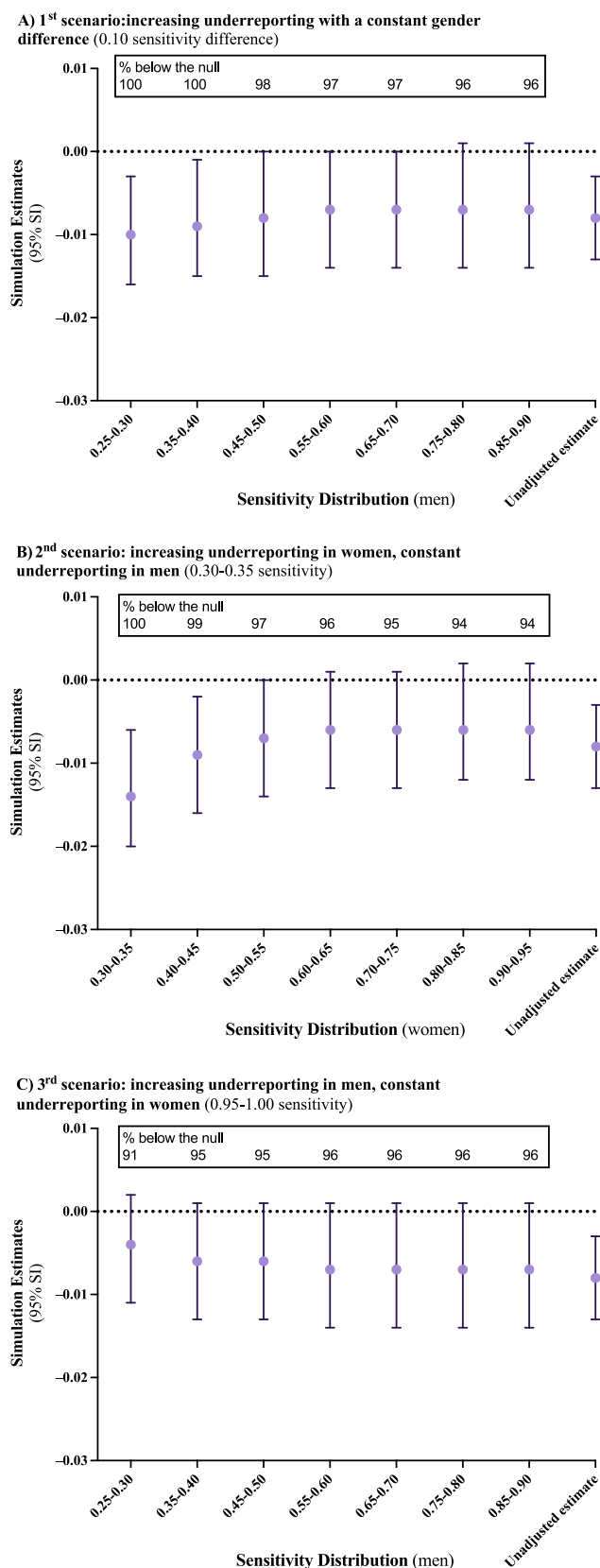
Figure 2. Simulation estimates and 95% simulation intervals (SIs) for the 3-way interaction between loneliness exposure duration (continuous), years of follow-up, and gender in each of the three simulation scenarios, the US Health and Retirement Study ( n = 9032 ), 1996-2016. A) First scenario; B) second scenario; C) third scenario. The % below the null represents the proportion of the simulation estimates below the null in the 10 000 replications for each situation.
