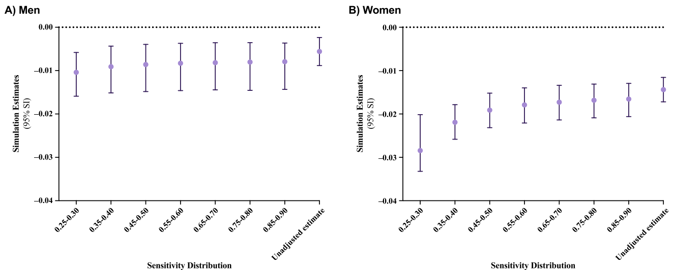
Figure 1. Gender-specific simulation estimates and 95% simulation intervals (SIs) for the interaction between loneliness exposure duration (continuous) and years of follow-up, the US Health and Retirement Study ( n = 9032 ), 1996–2016. These estimates were from gender-stratified subgroup analyses: A) men; B) women. We conducted additional pooled analyses to derive gender-specific simulation estimates (Figure S2). Results were consistent with those shown in Figure 1.
