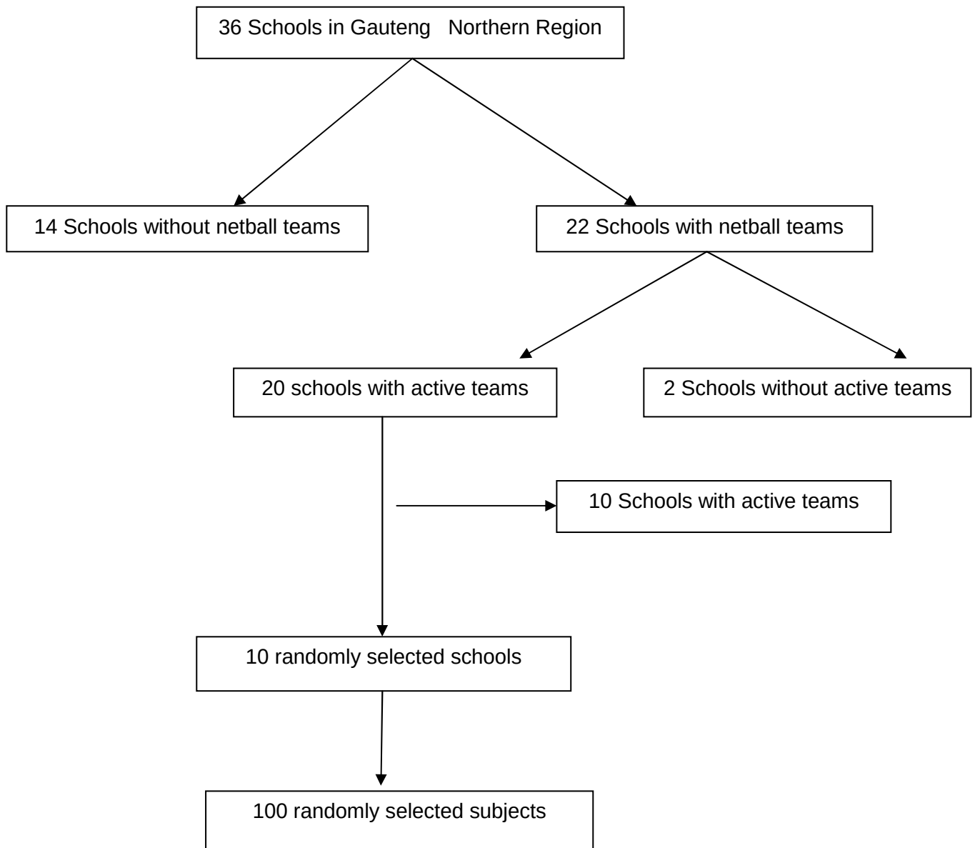
Figure 3.1: Sampling procedure
