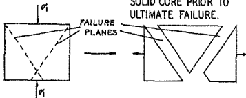
FIGURE 17c. SIDE ELEVATION OF A SANDSTONE MODEL OF LOW WIDTH TO HEIGHT RATIO SHOWING THE DEVELOPMENT OF FAILURE PLANES.
