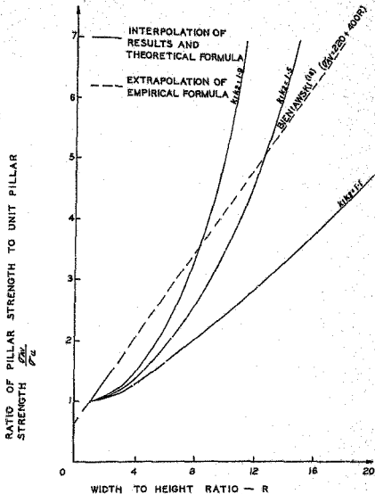
FIGURE 19c. COMPARISON OF THE "STRAIGHT LINE FORMULAE" TO THE POSTULATED THEORETICAL RELATIONSHIP.
