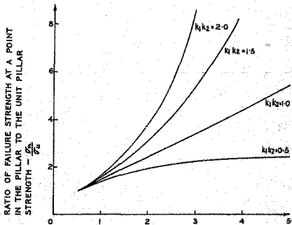
DISTANCE INTO THE PILLAR IN UNITS OF THE UNIT PILLAR - x
