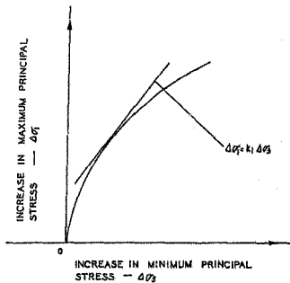
FIGURE I b. DETERMINATION OF THE STRENGTH MULTIPLICATION FACTOR — k_1
