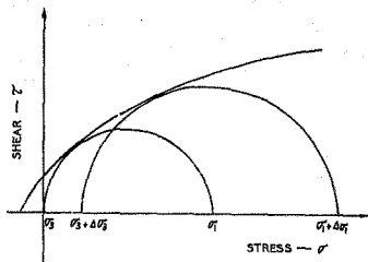
FIGURE I a. MOHR RUPTURE DIAGRAM.
