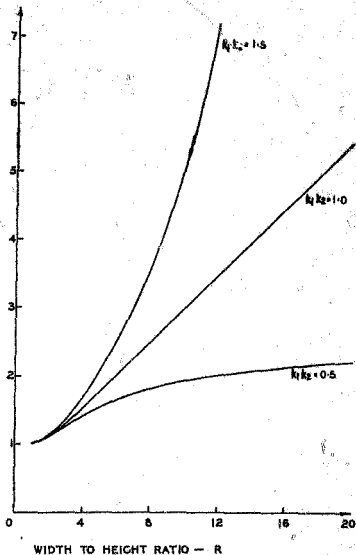
FIGURE 14(b) THE RELATIONSHIP BETWEEN THE AVERAGE FAILURE STRENGTH AND THE WIDTH TO HEIGHT RATIO OF WIDE STRIP PILLARS USING THE CONTINUOUS RATE OF INCREASE APPROACH.
