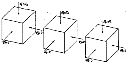
FIGURE 11a. THE STRESSES ON THREE INDEPENDENT UNIT PILLARS AT FAILURE.
