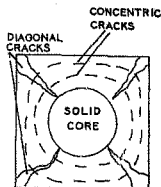
FIGURE 17b. PLAN VIEW OF A SANDSTONE MODEL OF LARGE ( >4 ) WIDTH TO HEIGHT RATIO SHOWING DIAGONAL CRACKS, CONCENTRIC CRACKS AND SOLID CORE PRIOR TO ULTIMATE FAILURE.
