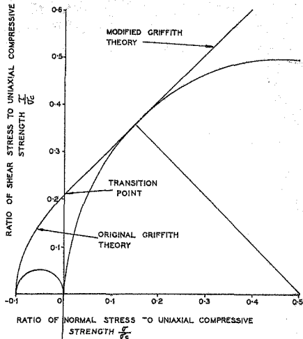
FIGURE 1. MOHR ENVELOPE FOR ORIGINAL AND MODIFIED GRIFFITH'S BRITTLE FRACTURE CRITERIA IN TERMS OF THE UNIAXIAL COMPRESSIVE STRENGTH \sigma_c FOR \mu = 1.0 . (AFTER HOEK (20) )
