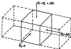
FIGURE 11b. THE EFFECT ON THE STRESSES ON THE CENTRE UNIT PILLAR WHEN RESTRAINED IN THE \sigma_3 -DIRECTION BY ADJACENT UNIT PILLARS.
