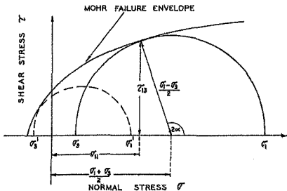
FIGURE 2b. MOHR DIAGRAM SHOWING THE RELATIONSHIP BETWEEN THE STRESSES ON A TWO-DIMENSIONAL ELASTIC BODY AT FAILURE, AND THE COMMON FAILURE ENVELOPE FOR FAILURE AT VARIOUS STRESSES.
