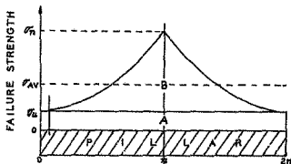
FIGURE 14a. FAILURE STRENGTH DISTRIBUTION OVER A WIDE PILLAR.
