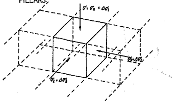
FIGURE 11c. THE EFFECT ON THE STRESSES ON THE UNIT PILLAR WHEN RESTRAINED EQUALLY IN THE \sigma_2 -AND \sigma_3 -DIRECTIONS BY ADJACENT UNIT PILLARS.
