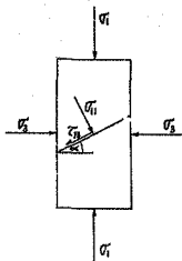
FIGURE 2a. TWO-DIMENSIONAL STRESS SYSTEM ON AN ELASTIC BODY.
