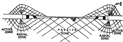
FIGURE 7d. DIAGRAMMATIC SKETCH SHOWING SHEAR ZONES AROUND A STOPING EXCAVATION (AFTER WIGGILL (12) )
