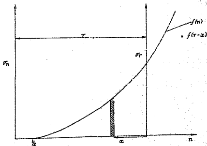
FIGURE 16b. MATHEMATICAL TECHNIQUE FOR FINDING AVERAGE STRENGTH OF A CIRCULAR WIDE PILLAR FOR VARYING RADIUS.
