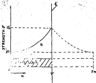
FIGURE 16a. STRENGTH DISTRIBUTION ALONG DIAMETER OF A CIRCULAR WIDE PILLAR.
