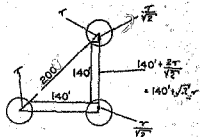
DIAGRAM OF CIRCULAR PILLAR PLAN.
