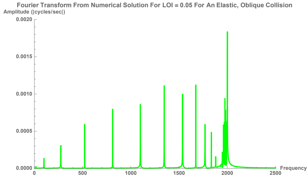
Figure 6.49: The Fourier Transform from the numerical solution for Location of Impact near the fixed-end of the bat of the bat (at 0.05m) for an elastic, oblique collision
