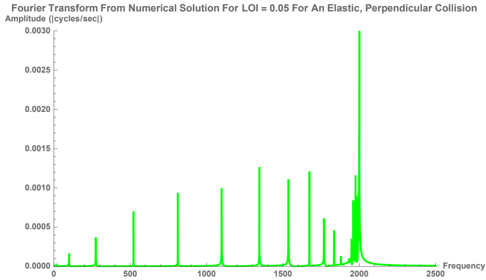
Figure 6.30: The Fourier Transform from the numerical solution for Location of Impact near the fixed-end of the bat of the bat (at 0.05m) for an elastic, perpendicular collision
