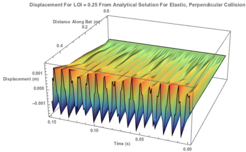
Figure 6.22: The displacement profile from analytical solution for Location of Impact at the middle of the bat of the bat (at 0.25m) for an elastic, perpendicular collision
