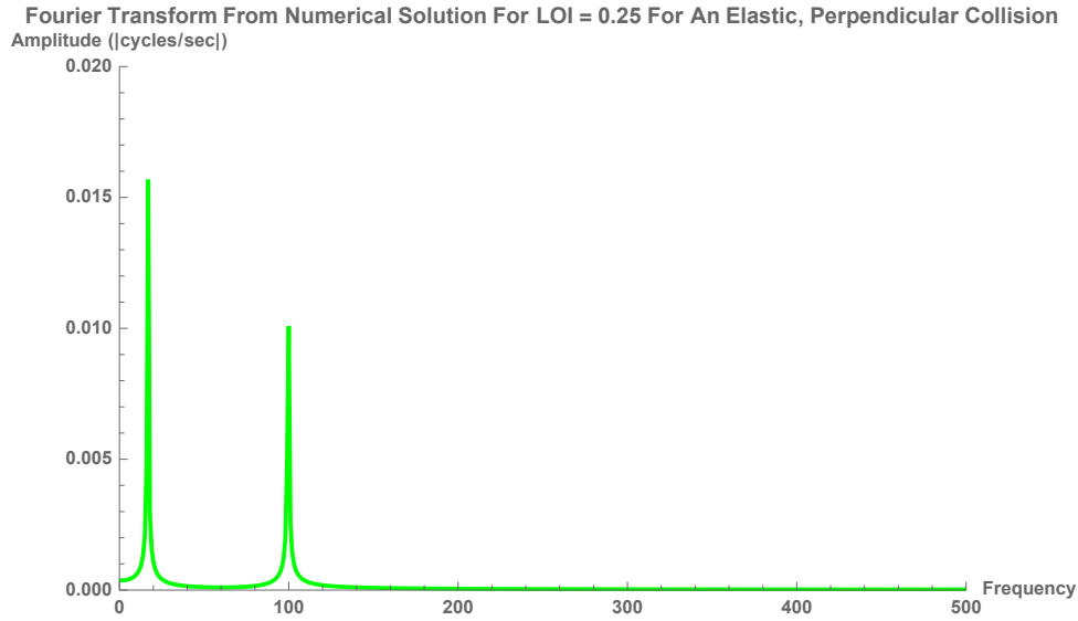
Figure 6.25: The Fourier Transform from the numerical solution for Location of Impact at the middle of the bat of the bat (at 0.25m) for an elastic, perpendicular collision
