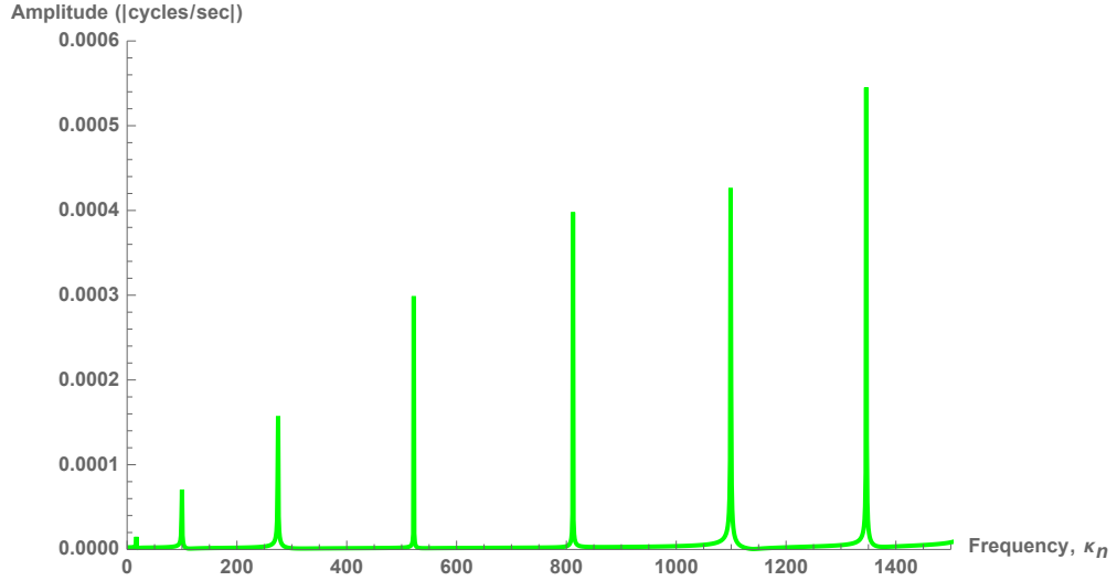
Fourier Transform From Numerical Solution For LOI = 0.05 For An Impulsive, Perpendicular Collision
