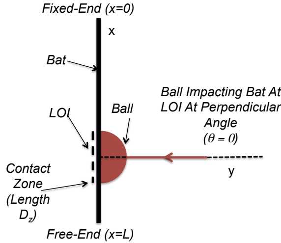
Figure 3.4: Diagram portraying the perpendicular, elastic collision between bat and ball in the second scenario.
