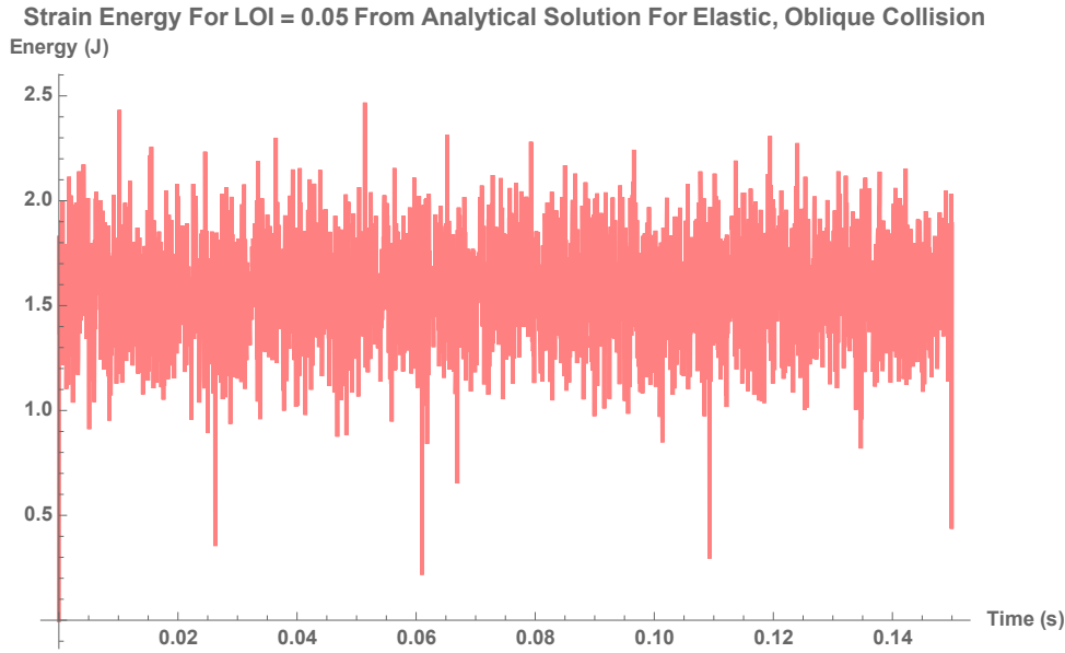
Figure 6.50: The strain energy over the entire time period from the analytical solution for Location of Impact near the fixed-end of the bat of the bat (at 0.05m) for an elastic, oblique collision
