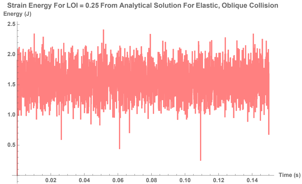
Figure 6.45: The strain energy over the entire time period from the analytical solution for Location of Impact at the middle of the bat of the bat (at 0.25m) for an elastic, oblique collision
