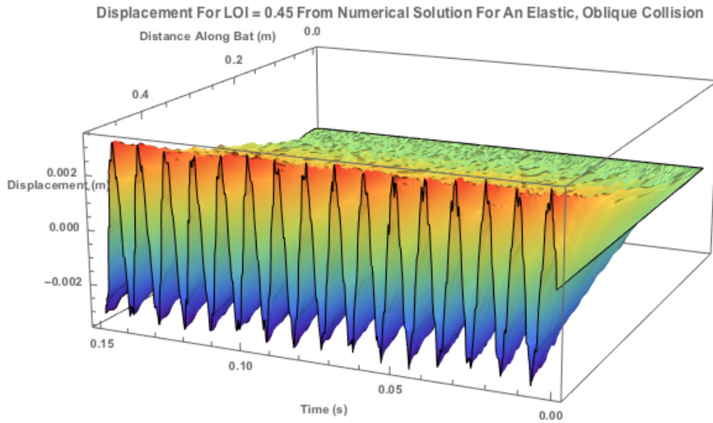
Figure 6.36: The displacement profile from numerical solution for Location of Impact near the free-end of the bat (at 0.45m) for an elastic, oblique collision
