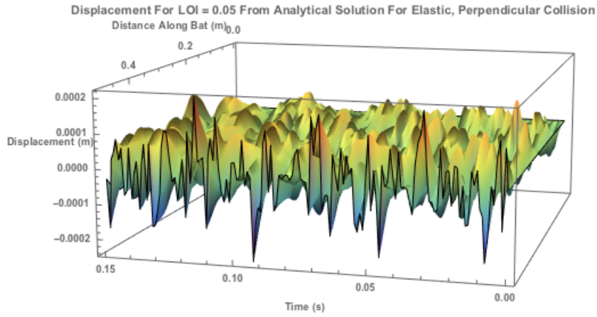
Figure 6.27: The displacement profile from analytical solution for Location of Impact near the fixed-end of the bat of the bat (at 0.05m) for an elastic, perpendicular collision
