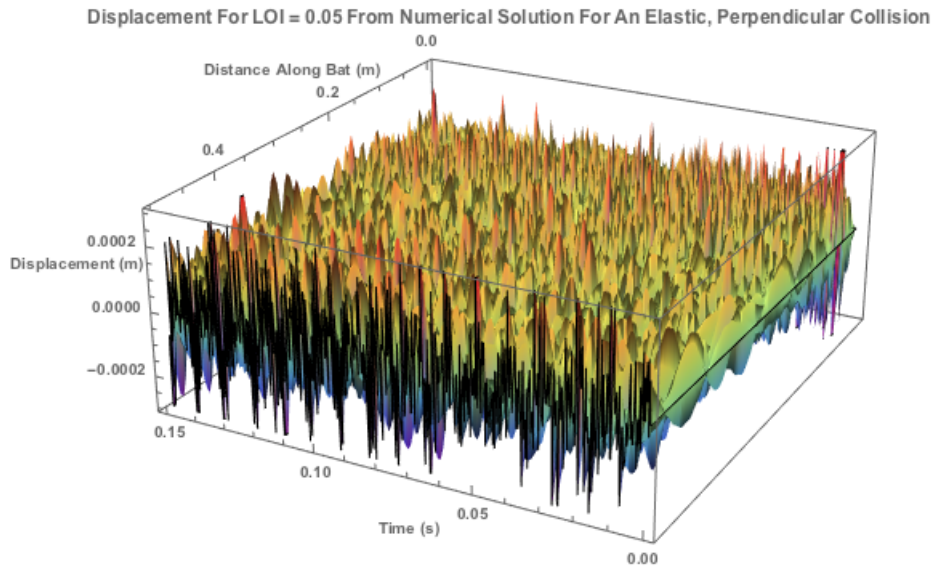
Figure 6.28: The displacement profile from numerical solution for Location of Impact near the fixed-end of the bat of the bat (at 0.05m) for an elastic, perpendicular collision
