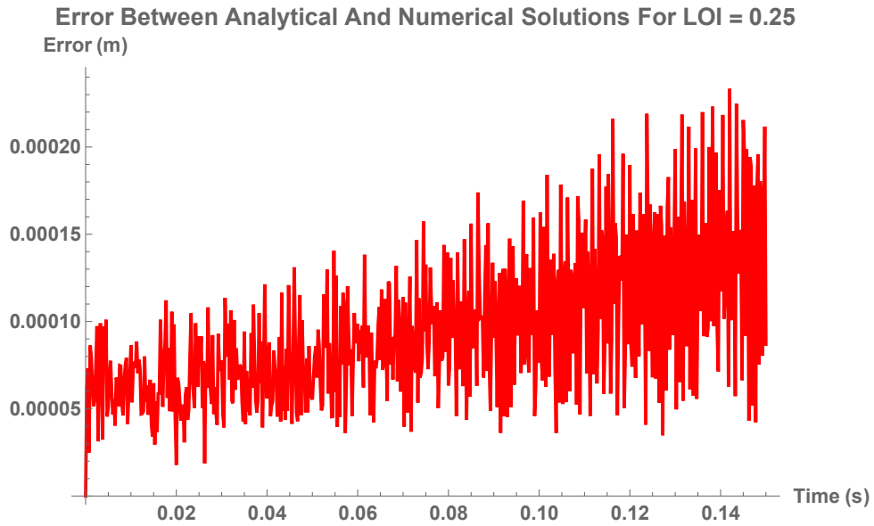
Figure 6.24: The error between the analytical solution and the numerical solution for Location of Impact at the middle of the bat of the bat (at 0.25m) for an elastic, perpendicular collision
