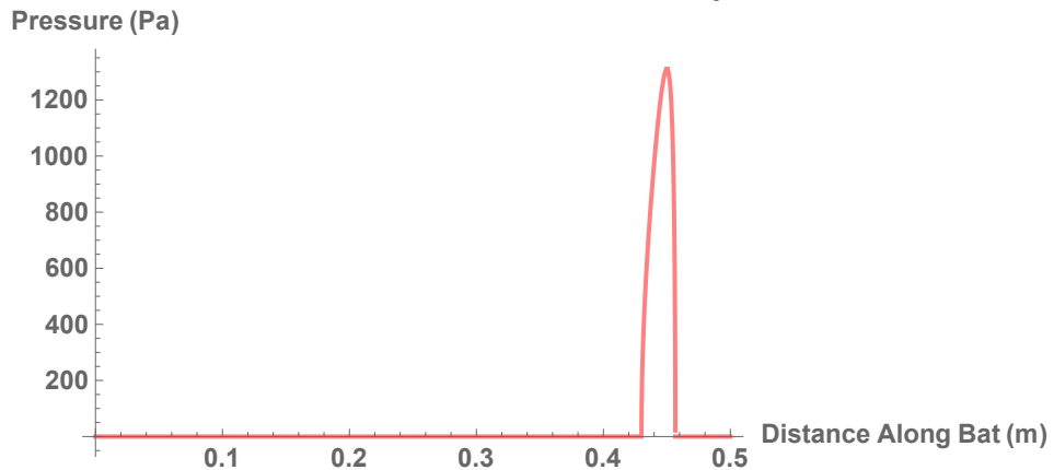
Figure 6.32: The pressure distribution caused by the ball impacting the bat for Location of Impact near the free-end of the bat (0.45m) for an elastic, oblique collision
