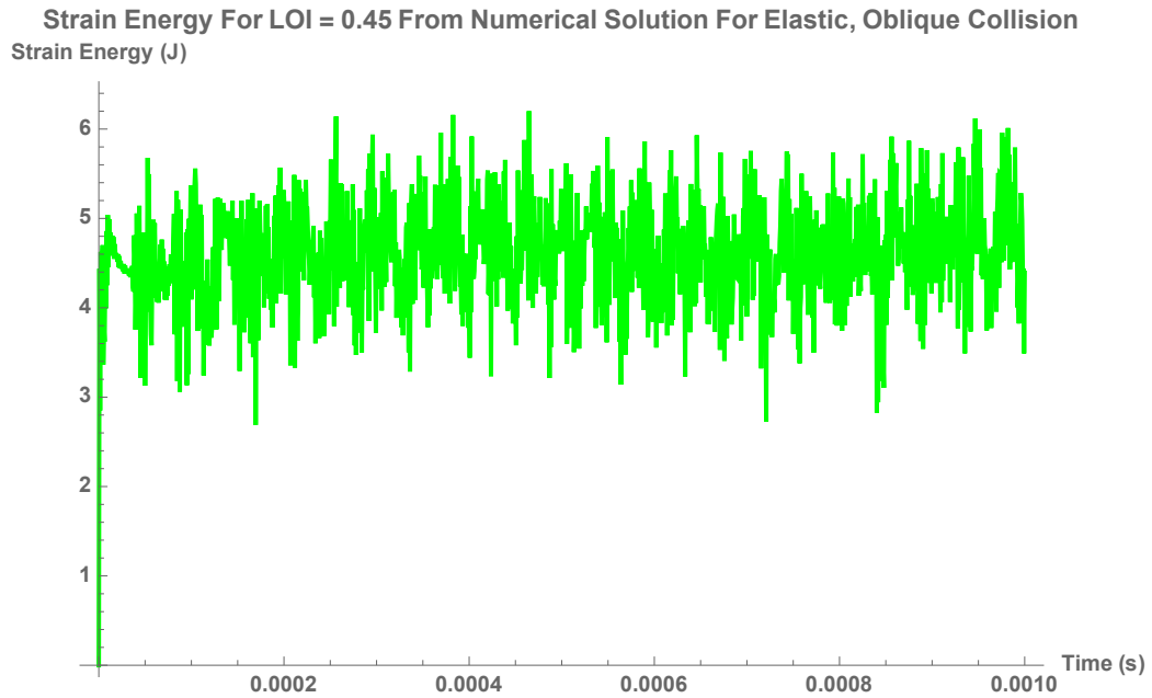
Figure 6.40: The strain energy over the short time period from the numerical solution to be compared to the analytical solution for Location of Impact near the free-end of the bat (at 0.45m) for an elastic, oblique collision
