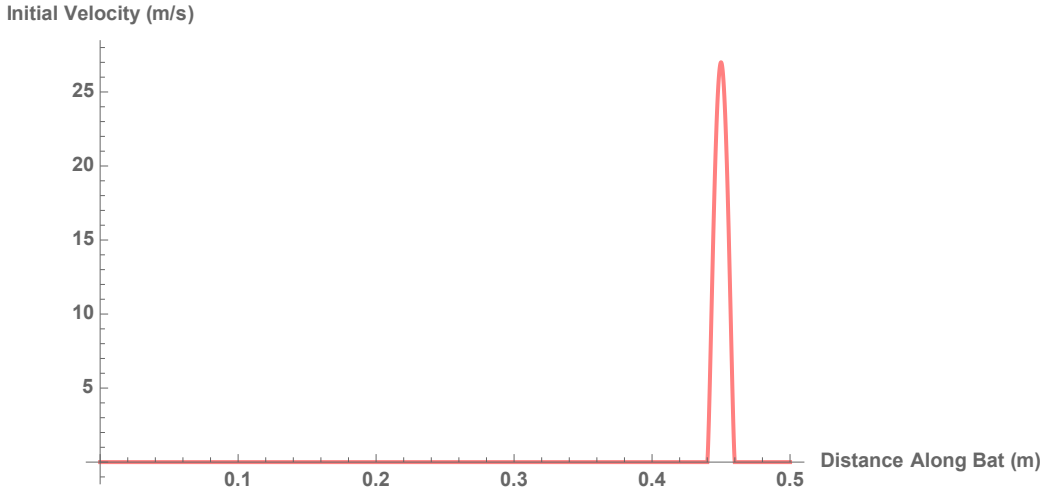
Figure 6.14: The initial velocity distribution for Location of Impact near the free-end of the bat (0.45m) for an elastic, perpendicular collision
