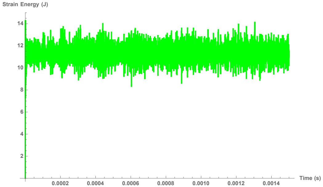
Strain Energy For LOI = 0.05 From Numerical Solution For An Impulsive, Perpendicular Collision
