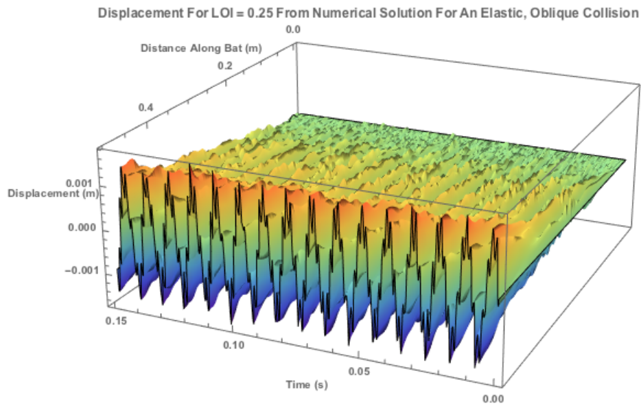
Figure 6.42: The displacement profile from numerical solution for Location of Impact at the middle of the bat of the bat (at 0.25m) for an elastic, oblique collision
