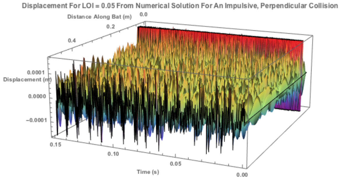
Figure 6.10: The displacement solution for Location of Impact near the fixed-end of the bat (at 0.05m) for an impulsive, perpendicular collision
