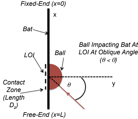
Figure 3.5: Diagram portraying the oblique, elastic collision between bat and ball in the third scenario.
