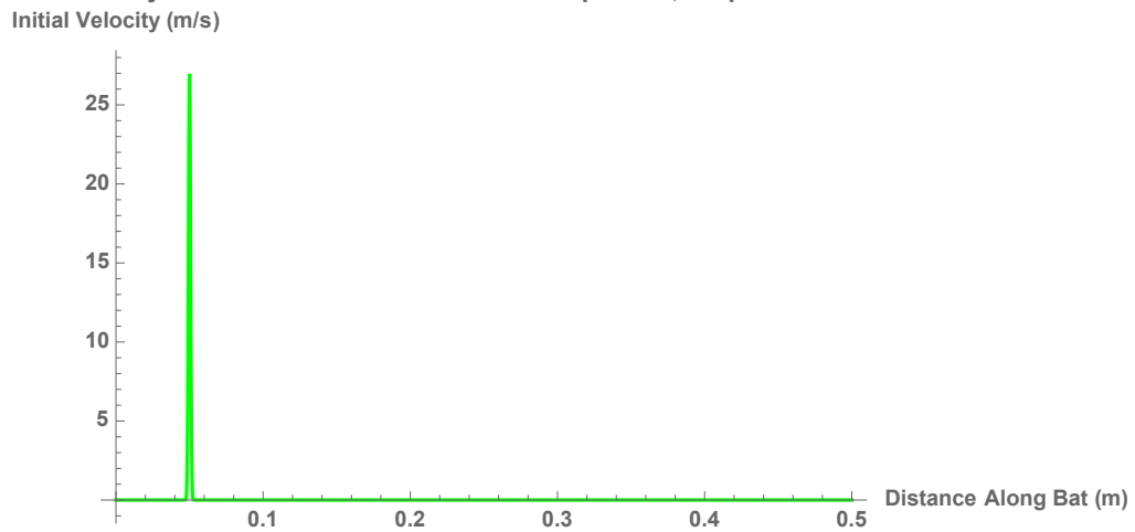
Figure 6.9: The initial velocity distribution for Location of Impact near the fixed-end of the bat (0.05m) for an impulsive, perpendicular collision
