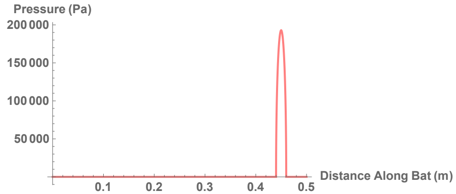
Figure 6.13: The pressure distribution caused by the ball impacting the bat for Location of Impact near the free-end of the bat (0.45m) for an elastic, perpendicular collision
