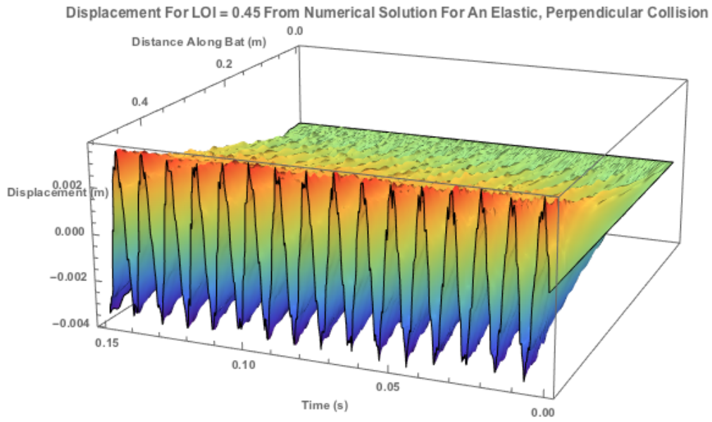
Figure 6.17: The displacement profile from numerical solution for Location of Impact near the free-end of the bat (at 0.45m) for an elastic, perpendicular collision
