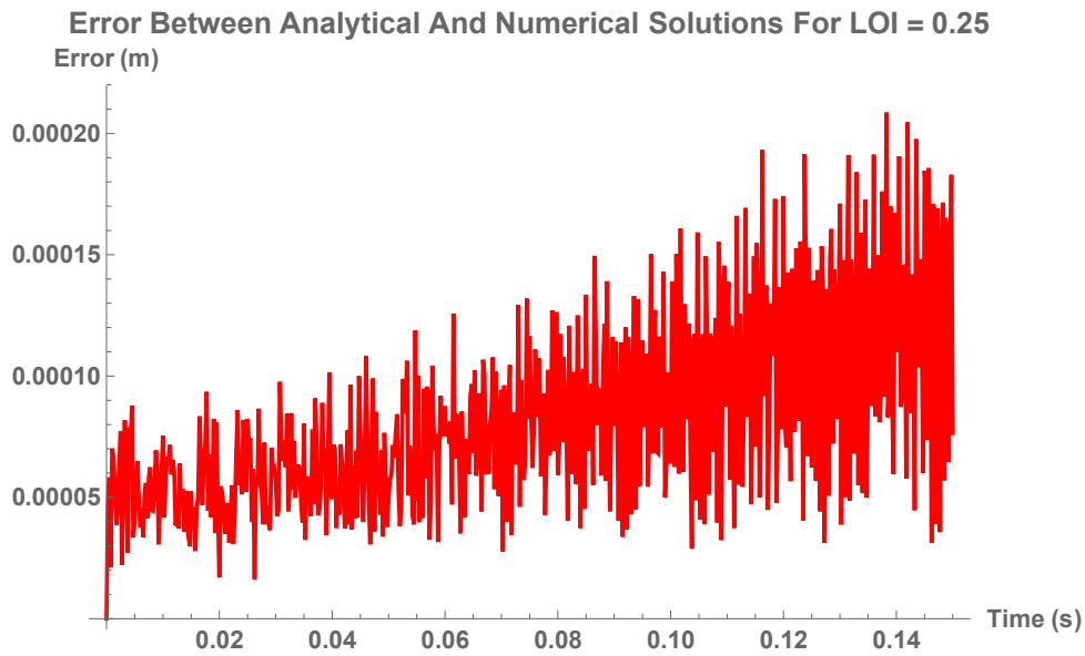
Figure 6.43: The error between the analytical solution and the numerical solution for Location of Impact at the middle of the bat of the bat (at 0.25m) for an elastic, oblique collision
