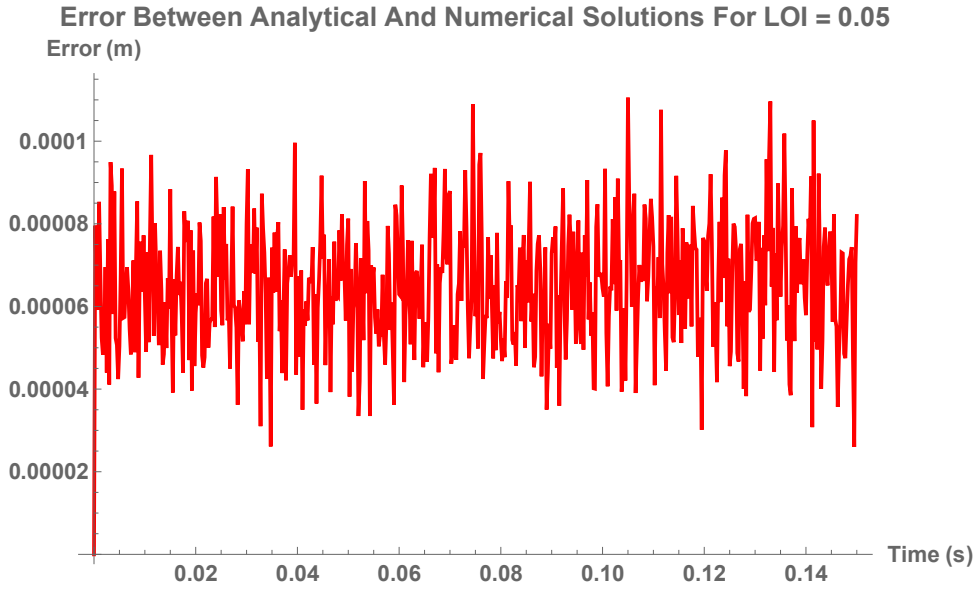
Figure 6.29: The error between the analytical solution and the numerical solution for Location of Impact near the fixed-end of the bat of the bat (at 0.05m) for an elastic, perpendicular collision
