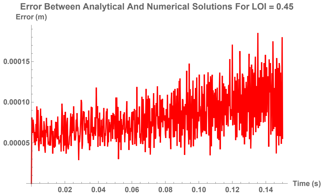
Figure 6.18: The error between the analytical solution and the numerical solution for Location of Impact near the free-end of the bat (at 0.45m) for an elastic, perpendicular collision
