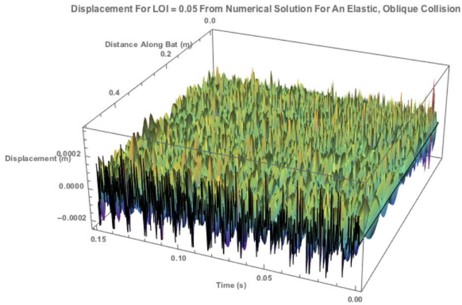
Figure 6.47: The displacement profile from numerical solution for Location of Impact near the fixed-end of the bat of the bat (at 0.05m) for an elastic, oblique collision
