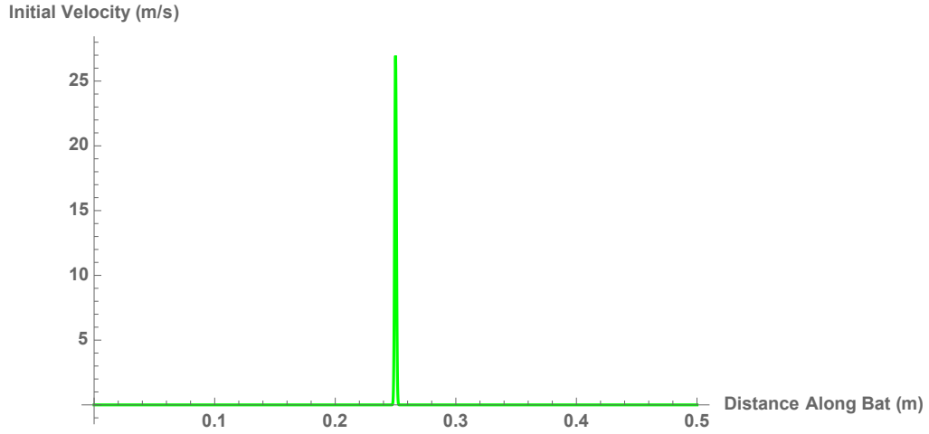
Figure 6.5: The initial velocity distribution for Location of Impact at the middle of the bat (0.25m) for an impulsive, perpendicular collision
