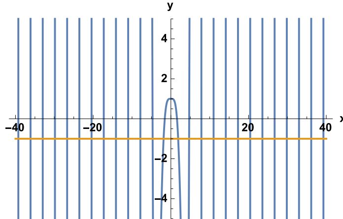
Figure 5.1: The graphs of y = \cos(x) \cosh(x) and y = -1 illustrating an infinite number of intersections between the functions.
