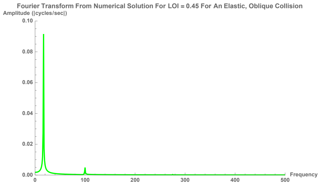
Figure 6.38: The Fourier Transform from the numerical solution for Location of Impact near the free-end of the bat (at 0.45m) for an elastic, oblique collision
