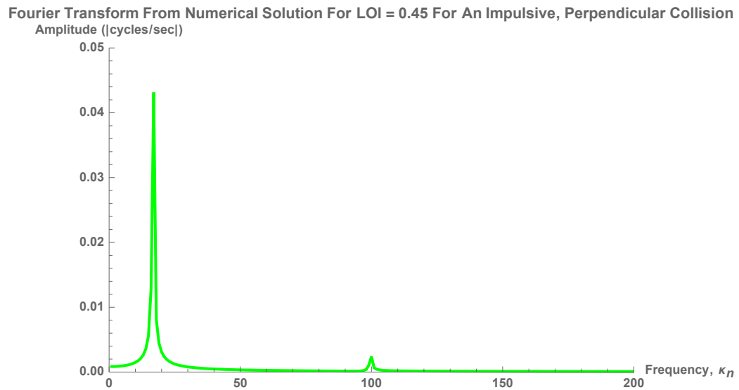
Figure 6.3: The Fourier Transform for Location of Impact near the free-end of the bat (at 0.45m) for an impulsive, perpendicular collision
