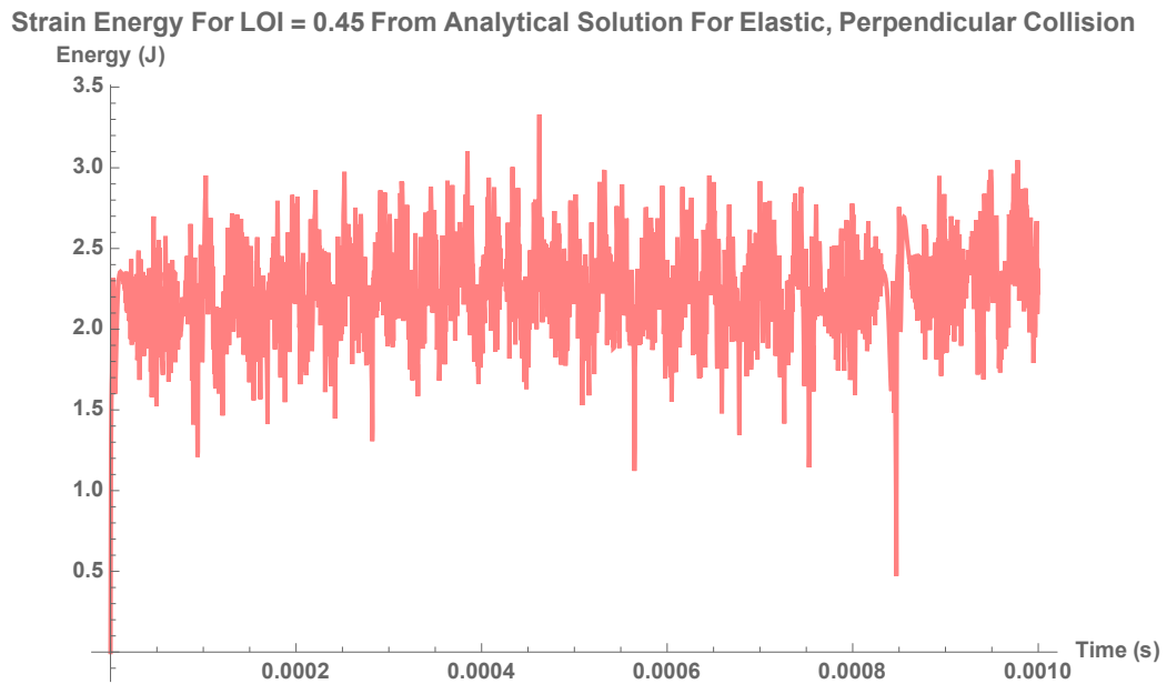
Figure 6.20: The strain energy over the short time period from the analytical solution to be compared to the numerical solution for Location of Impact near the free-end of the bat (at 0.45m) for an elastic, perpendicular collision
