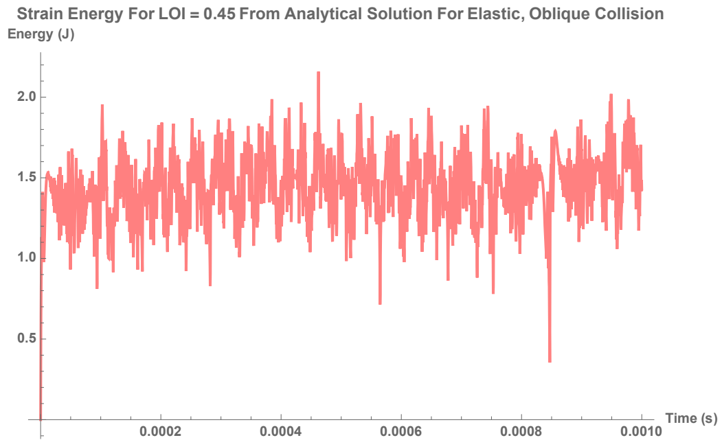
Figure 6.39: The strain energy over the short time period from the analytical solution to be compared to the numerical solution for Location of Impact near the free-end of the bat (at 0.45m) for an elastic, oblique collision
