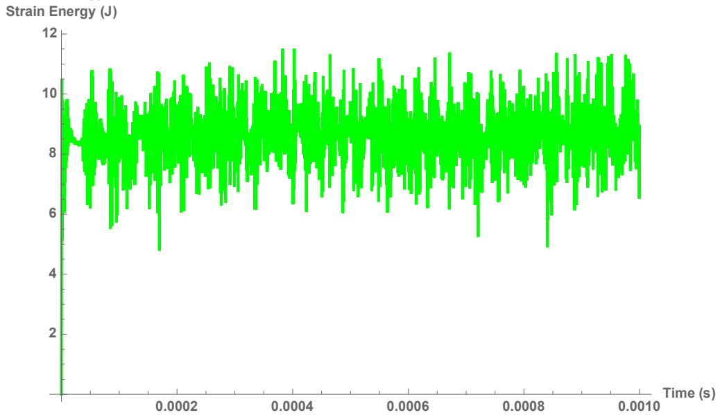
Figure 6.21: The strain energy over the short time period from the numerical solution to be compared to the analytical solution for Location of Impact near the free-end of the bat (at 0.45m) for an elastic, perpendicular collision
