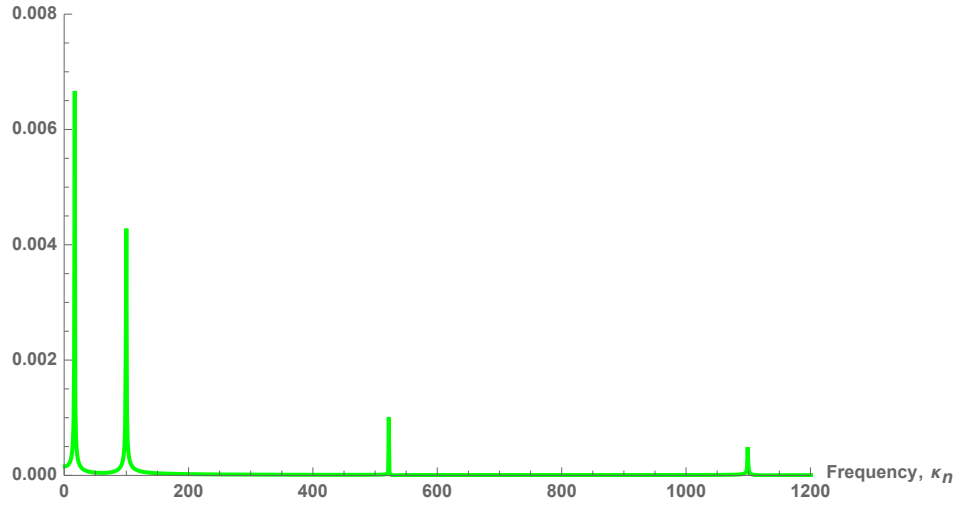
Fourier Transform From Numerical Solution For LOI = 0.25 For An Impulsive, Perpendicular Collision Amplitude (cycles/sec)
