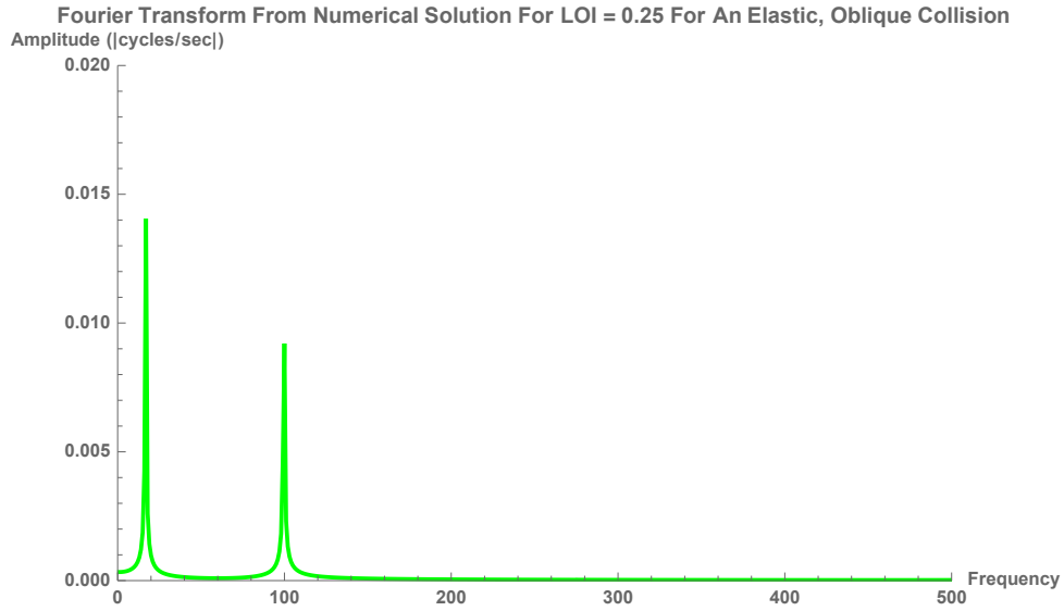
Figure 6.44: The Fourier Transform from the numerical solution for Location of Impact at the middle of the bat of the bat (at 0.25m) for an elastic, oblique collision
