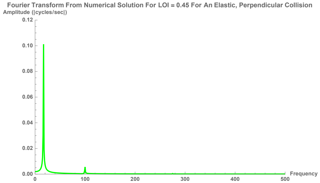
Figure 6.19: The Fourier Transform from the numerical solution for Location of Impact near the free-end of the bat (at 0.45m) for an elastic, perpendicular collision
