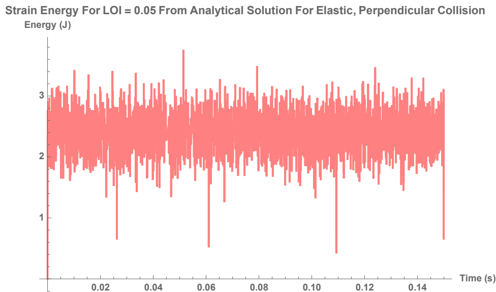
Figure 6.31: The strain energy over the entire time period from the analytical solution for Location of Impact near the fixed-end of the bat of the bat (at 0.05m) for an elastic, perpendicular collision
