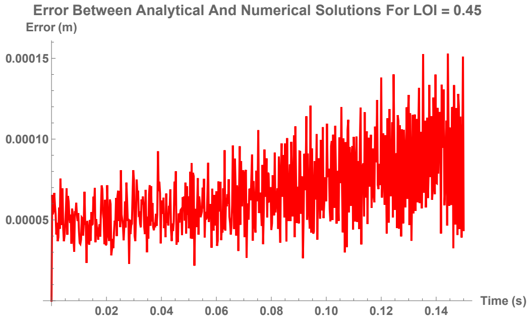
Figure 6.37: The error between the analytical solution and the numerical solution for Location of Impact near the free-end of the bat (at 0.45m) for an elastic, oblique collision
