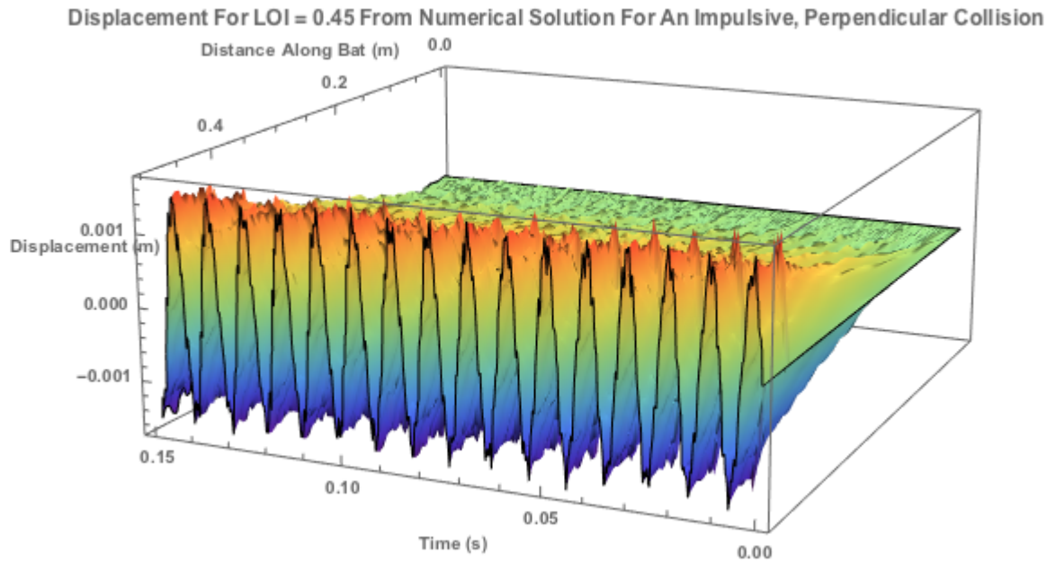
Figure 6.2: The displacement solution for Location of Impact near the free-end of the bat (at 0.45m) for an impulsive, perpendicular collision
