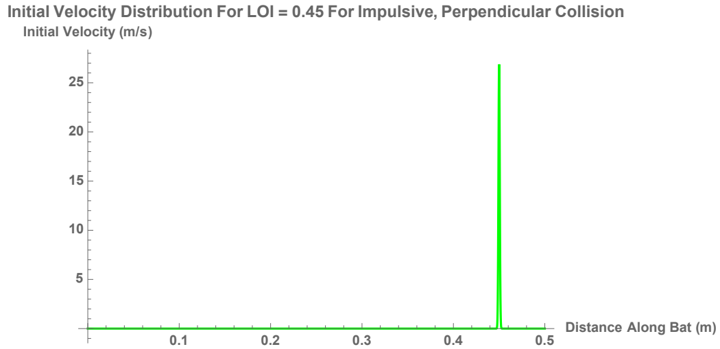
Figure 6.1: The initial velocity distribution for Location of Impact near the free-end of the bat (0.45m) for an impulsive, perpendicular collision
