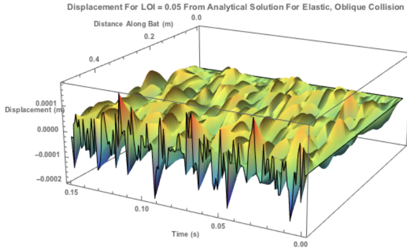
Figure 6.46: The displacement profile from analytical solution for Location of Impact near the fixed-end of the bat of the bat (at 0.05m) for an elastic, oblique collision
