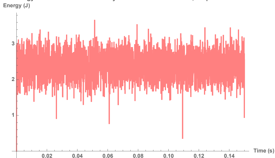
Strain Energy For LOI = 0.25 From Analytical Solution For Elastic, Perpendicular Collision
