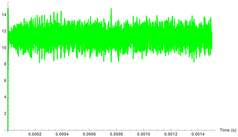
Strain Energy For LOI = 0.25 From Numerical Solution For An Impulsive, Perpendicular Collision Strain Energy (J)
