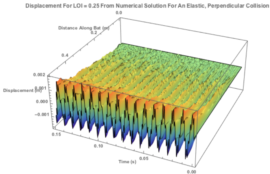
Figure 6.23: The displacement profile from numerical solution for Location of Impact at the middle of the bat of the bat (at 0.25m) for an elastic, perpendicular collision
