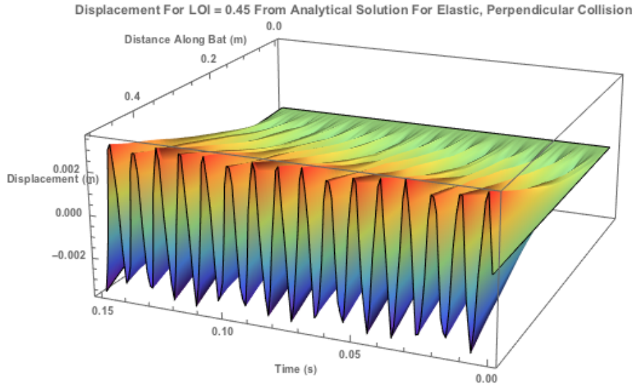
Figure 6.16: The displacement profile from analytical solution for Location of Impact near the free-end of the bat (at 0.45m) for an elastic, perpendicular collision
