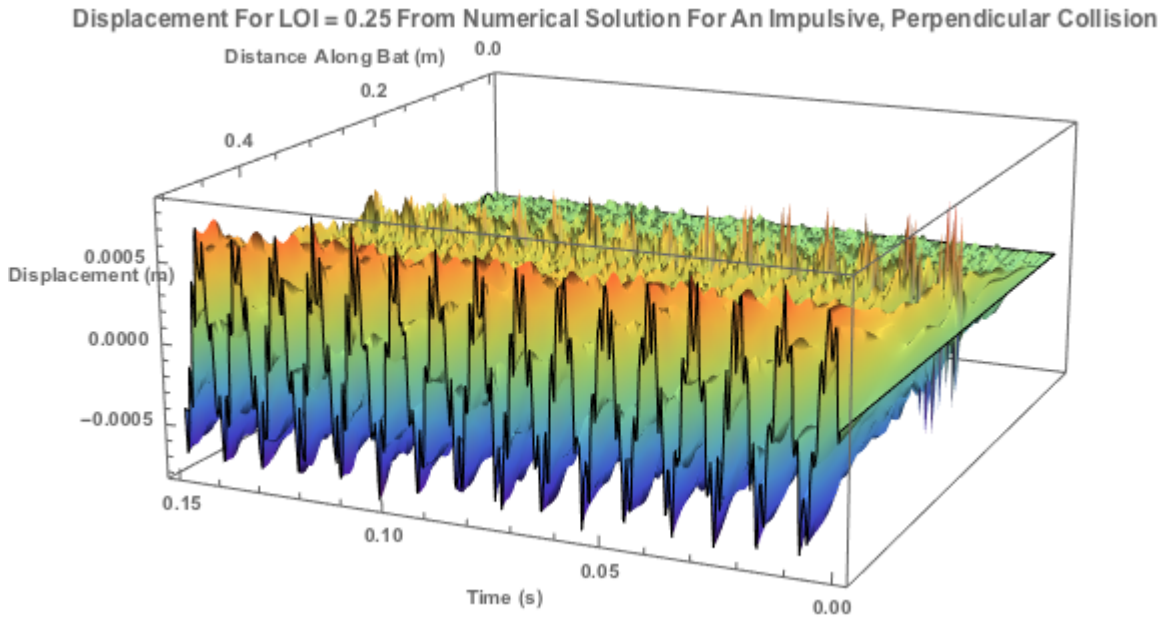
Figure 6.6: The displacement solution for Location of Impact at the middle of the bat (at 0.25m) for an impulsive, perpendicular collision
