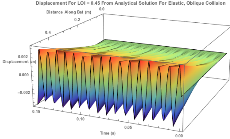
Figure 6.35: The displacement profile from analytical solution for Location of Impact near the free-end of the bat (at 0.45m) for an elastic, oblique collision
