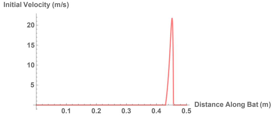
Figure 6.33: The initial velocity distribution for Location of Impact near the free-end of the bat (0.45m) for an elastic, oblique collision
