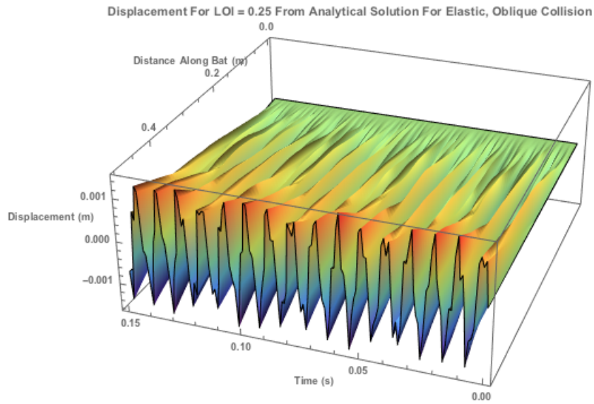
Figure 6.41: The displacement profile from analytical solution for Location of Impact at the middle of the bat of the bat (at 0.25m) for an elastic, oblique collision
