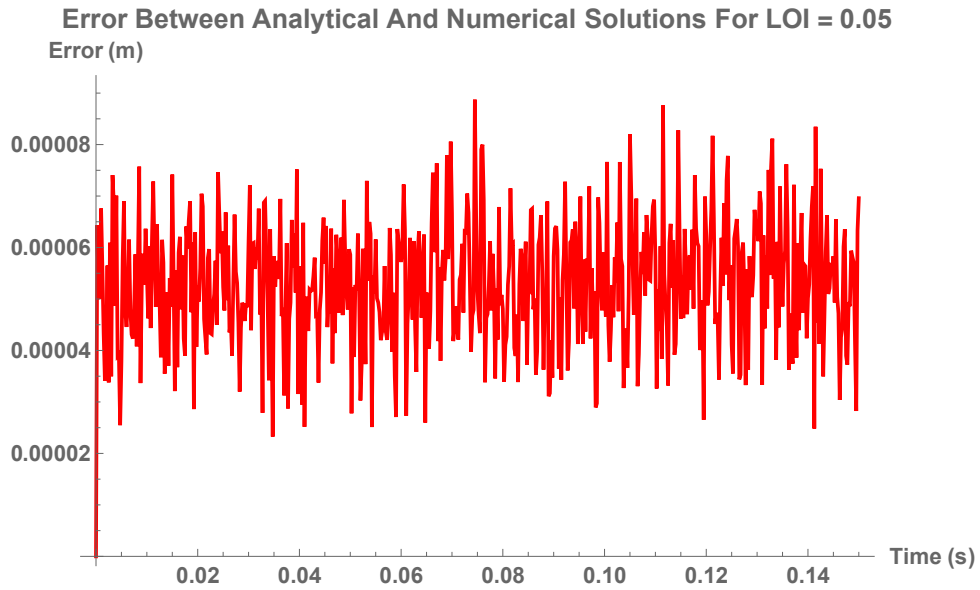
Figure 6.48: The error between the analytical solution and the numerical solution for Location of Impact near the fixed-end of the bat of the bat (at 0.05m) for an elastic, oblique collision
