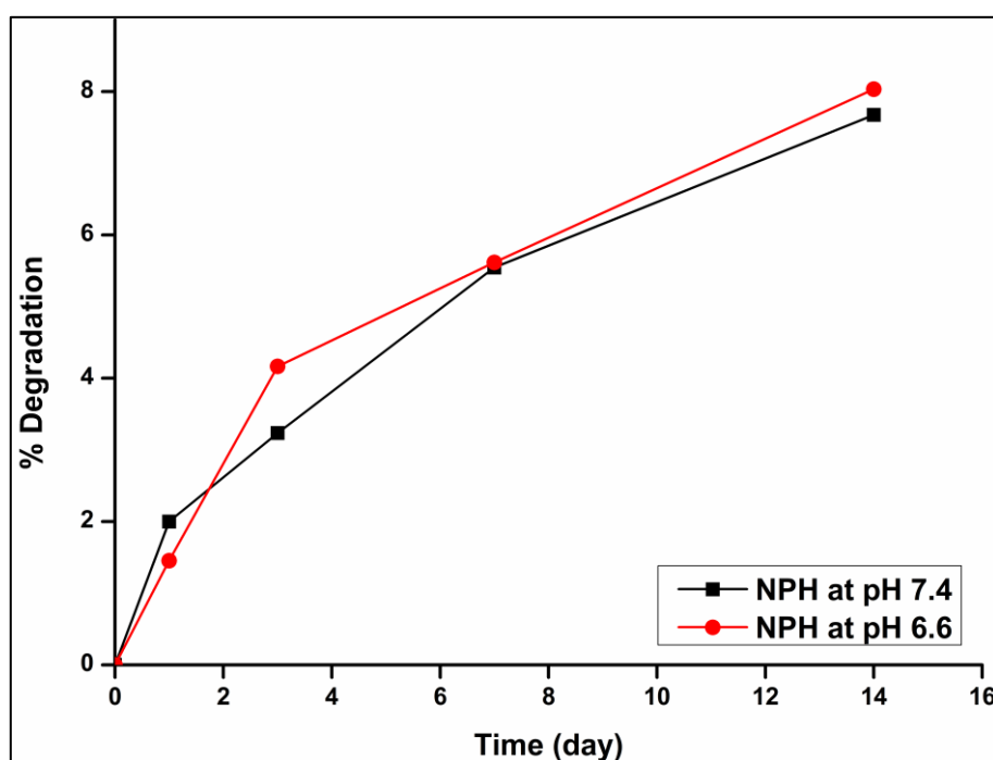
Figure 3.14. Biodegradation behaviour of the NPH in PBS solution (pH 6.6 and 7.4) at 37°C. The error bars were small, indicating that the data obtained did not differ among themselves the standard deviation ranged is (0-4.62 \times 10^{-15}) .
