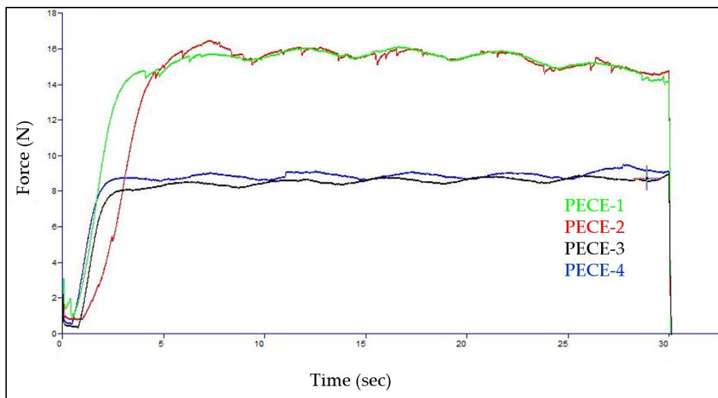
Figure 3.11 Required force to inject PECE hydrogel at different concentration from 1 mL syringes equipped with 27 G needle, PECE-1 (25% w/v hydrogel), PECE-2 (25% w/v NP-loaded hydrogel), PECE-3 (20% w/v hydrogel) and PECE-4 (20% w/v NP-loaded hydrogel).
