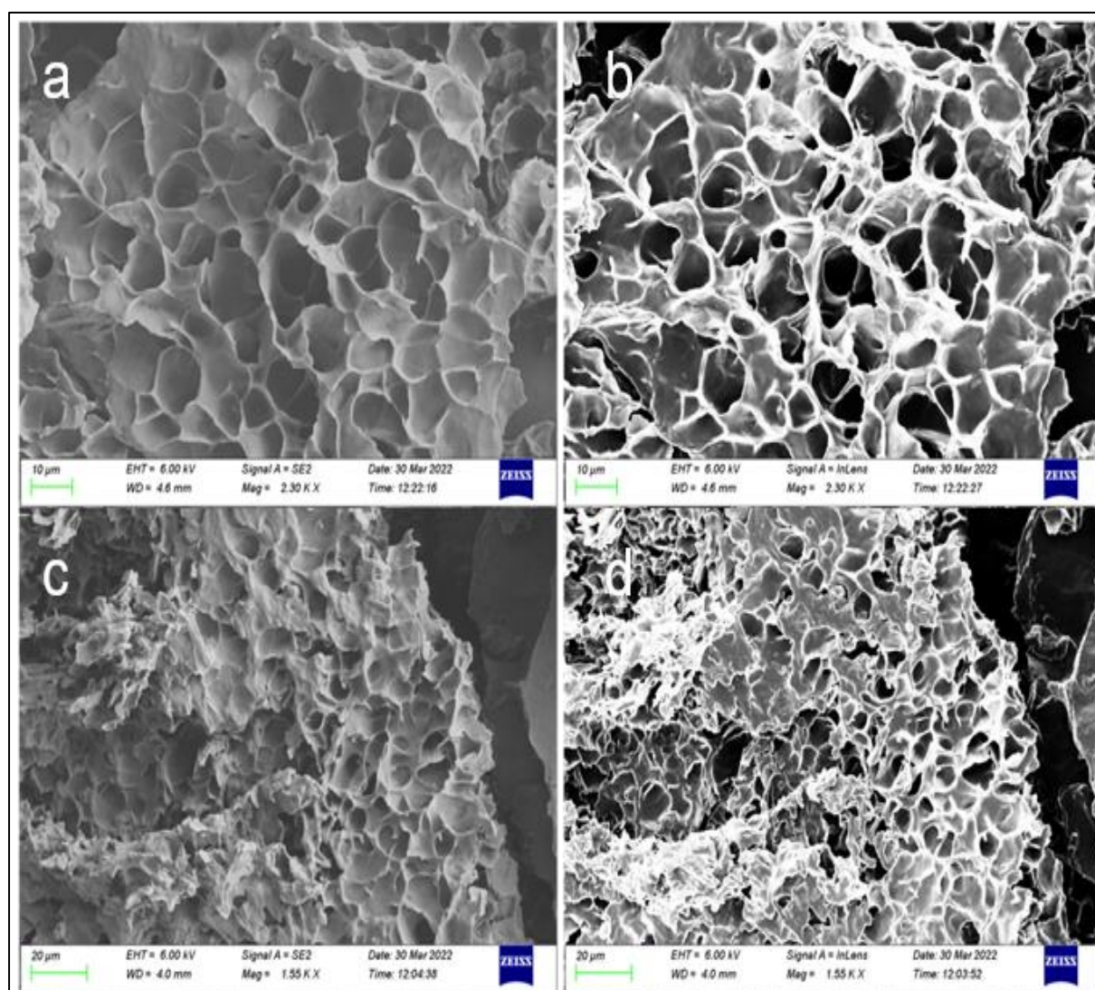
Figure 3.8 SEM images of PECE-1 (a) and (b) at 10 \mu\text{m} , PECE-2 (c) and (d) at 20 \mu\text{m} .
