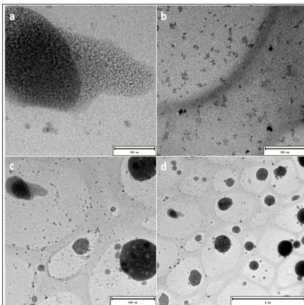
Figure 3.7 TEM images of PBAE nanoparticles. The scale bar for (a) and (b) is 100 nm, for (c) 500 nm and for (d) 2 μm of the drug free NPs.
