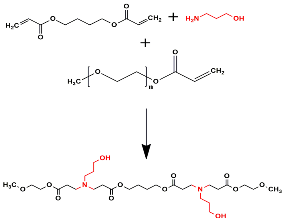
Figure 3.2 Synthetic scheme of PBAE copolymer.
