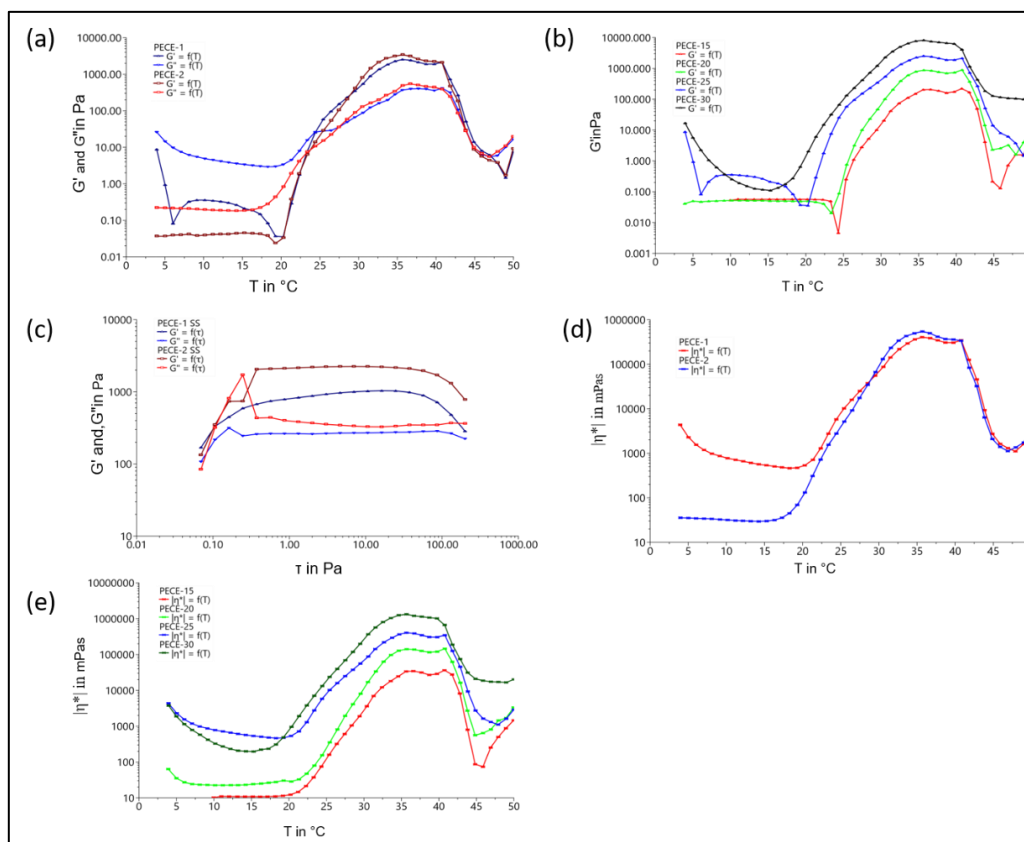
Figure 3.10 a) Temperature ramp of PECE-1 and PECE-2; (b) Temperature ramp of PECE hydrogel at different concentrations (15%, 20%, 25% and 30% w/v); (c) Stress sweep of PECE-1 and PECE-2 at 25°C; (d) Viscosity of PECE-1 and PECE-2 and (e) Viscosity of PECE hydrogel.
