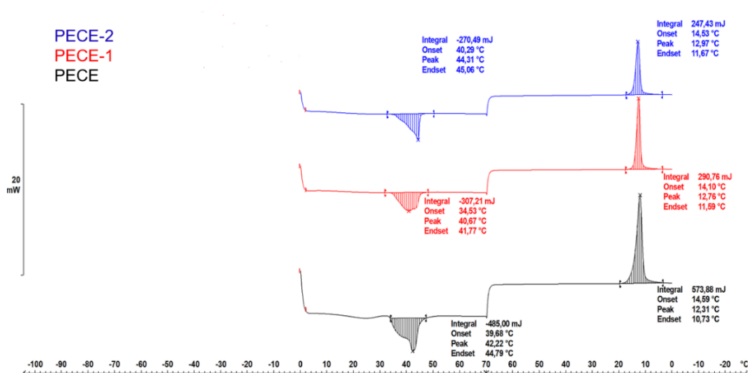
Figure 3.5 DSC thermograms of the PECE copolymer, PECE-1 and PECE-2.
