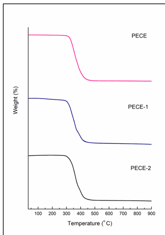
Figure 3.6 TGA thermograms of PECE, PECE-1 and PECE-2.
