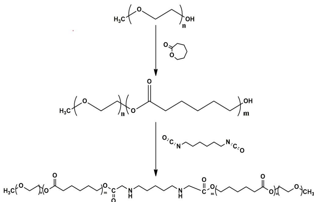
Figure 3.1 Synthetic scheme of PEG-PCL-PEG triblock copolymer.
