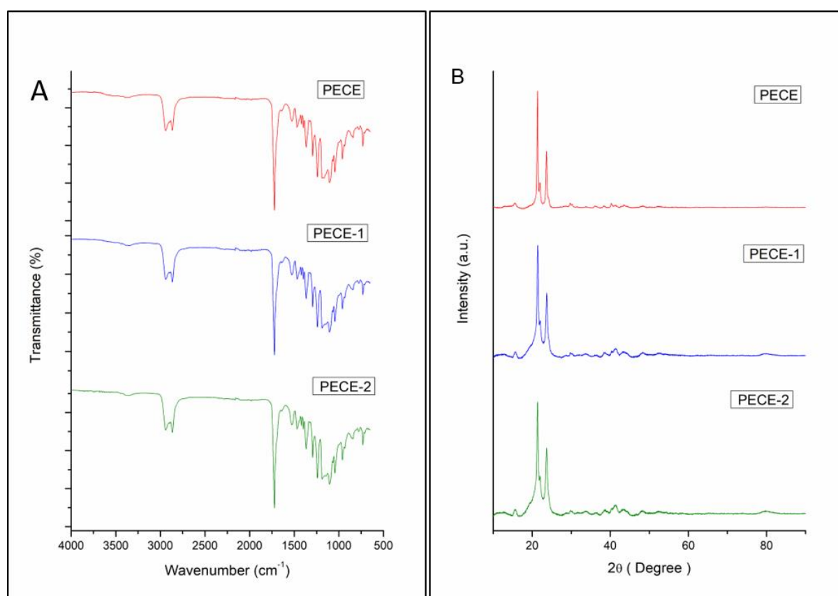
Figure 3.4 A) FTIR of PECE, PECE-1 and PECE-2; B) XRPD images of PECE, PECE-1 and PECE-2.
