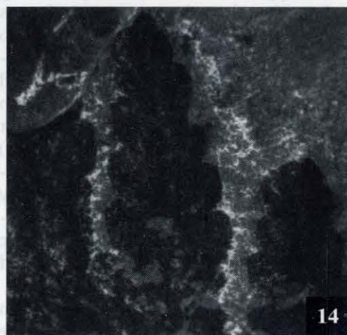
Figs 13 & 14. Triassic fern foliage; Little Switzerland. x2.
