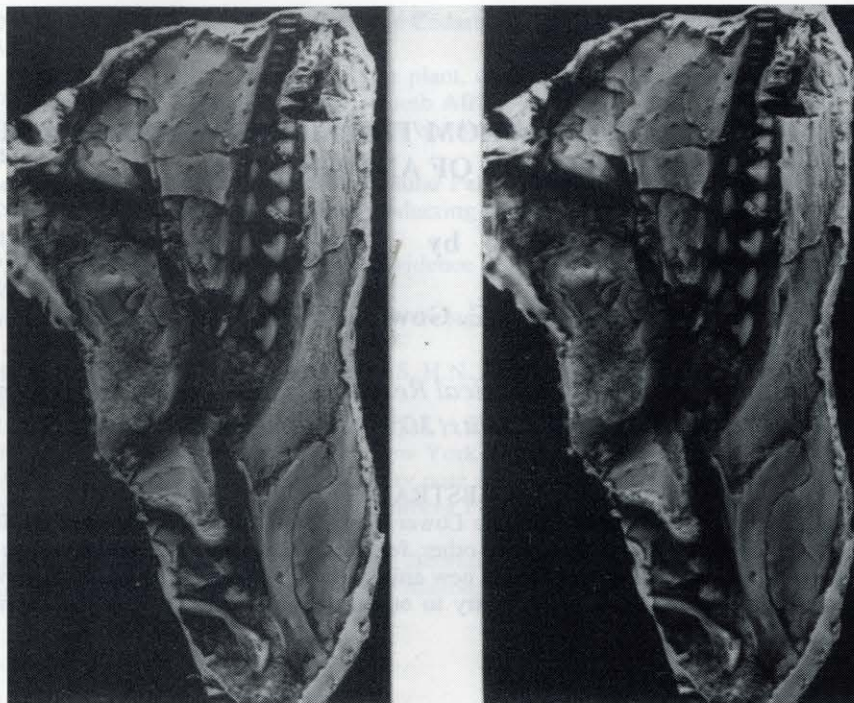
Figure 1: Fremouwosaurus geludens – stereophotographs of a latex peel taken from the specimen
