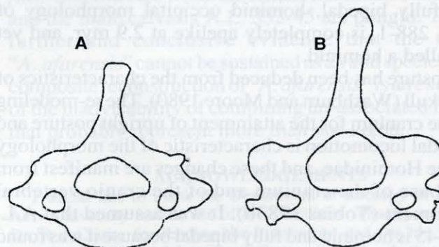
Figure 9 Cervical vertebrae of hominoids (superior view). A) Homo sapiens , 7th cervical vertebra. B) A.L. 333-106, 6th or 7th cervical vertebra (after Lovejoy et al. , 1982). Drawn to the same breadth. Note the very long spinous process of A.L. 333-106.
