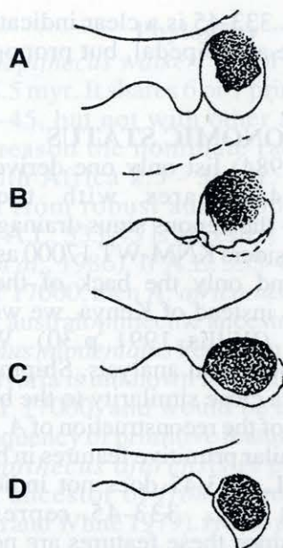
Figure 8 Postglenoid process in relation to the external acoustic meatus in A) Gorilla , B) A.L.333-45, C) A. robustus , D) H. sapiens (after Broom, except A.L. 333-45). In A.L.333-45 the outer part of the tympanic is situated mainly behind the postglenoid process, as in Gorilla .
