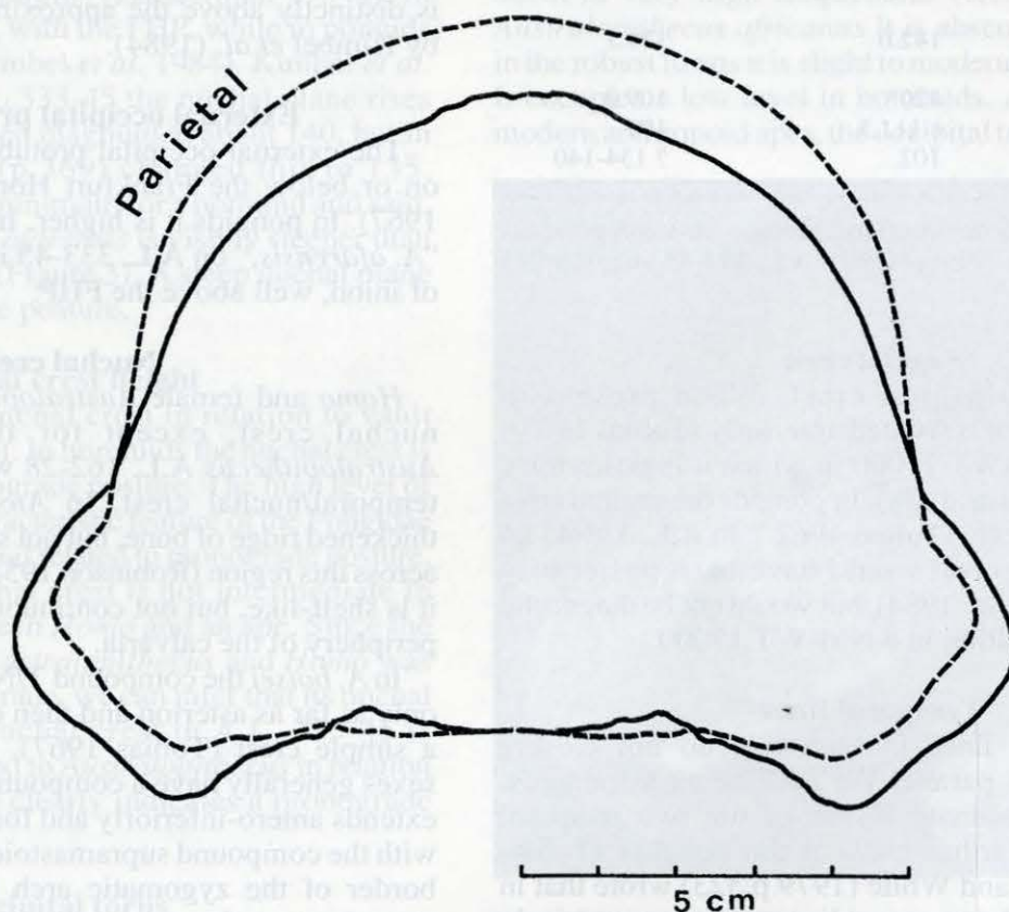
Fig.2. Norma occipitalis of the calvaria A.L. 333-45 (solid line) superimposed on that of A. africanus (broken line). Note lack of parietal expansion in A.L. 333-45.
