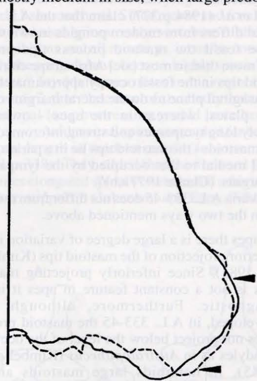
Figure 7 Norma occipitalis of the contour of right half of the calvaria A.L. 333-45 (solid line) superimposed on that of A. boisei O.H. 5 (broken line). Note that the supramastoid sulcus is absent in A.L. 333-45, and that the masoid process in O.H. 5 bulges laterally whereas in A.L. 333-45 it is inflected.
