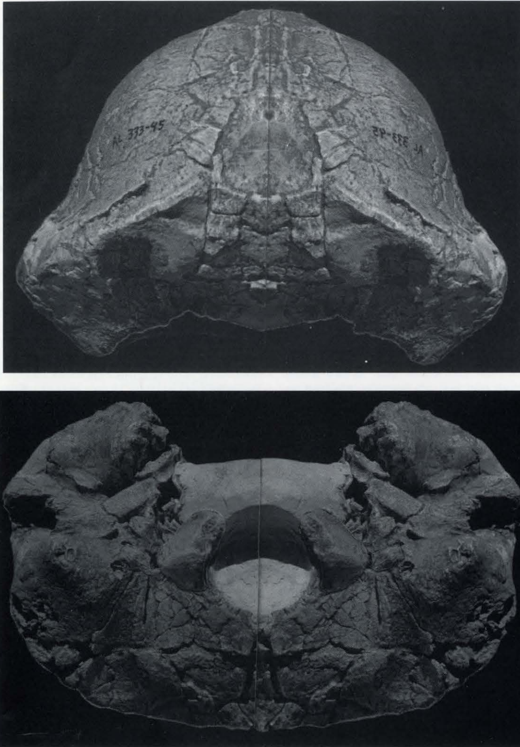
Figure 1. Restoration of the calvaria A.L.333-45. Above, norma occipitalis. Below, norma basalis.
