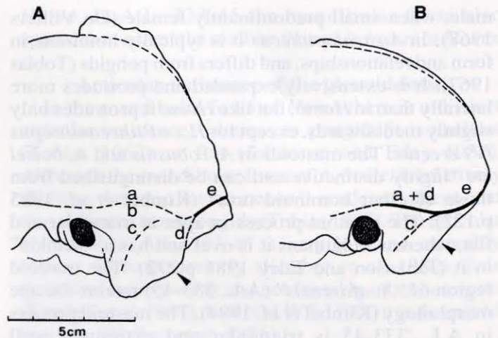
Figure 6 Left norma lateralis of A) A. boisei O.H. 5 and B) A.L. 333-45, depicting the occipitomastoid region. Simple crest (broken line), compound crest (solid line). Structures indicated: a) supramastoid crest, b) supramastoid sulcus, c) mastoid crest, d) superior nuchal crest, e) temporal/nuchal crest. Arrow points to posterolateral face of the mastoid
