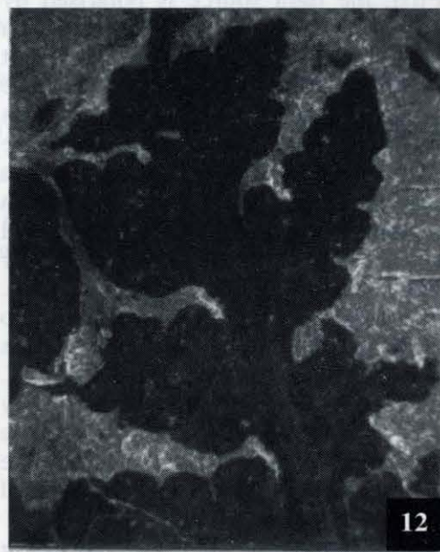
Figs 11 & 12. A portion of a Triassic fern; Little Switzerland. x2.
