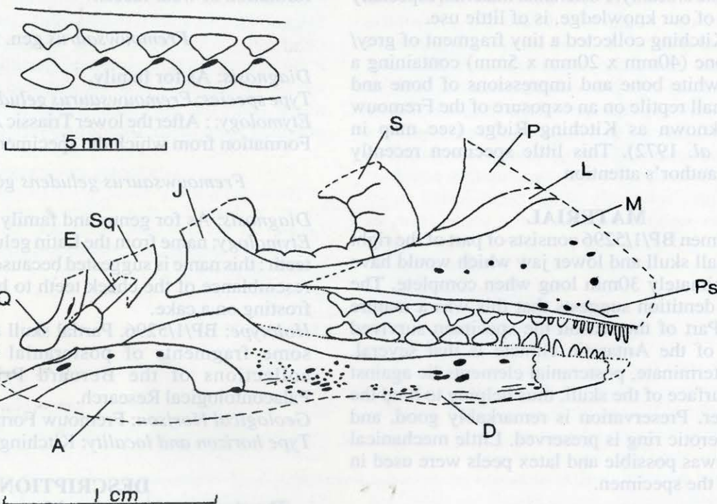
Figure 2: Fremouwosaurus geludens expansory sketch with inset detail of the wear facets and pattern of occlusion of the cheek teeth.
