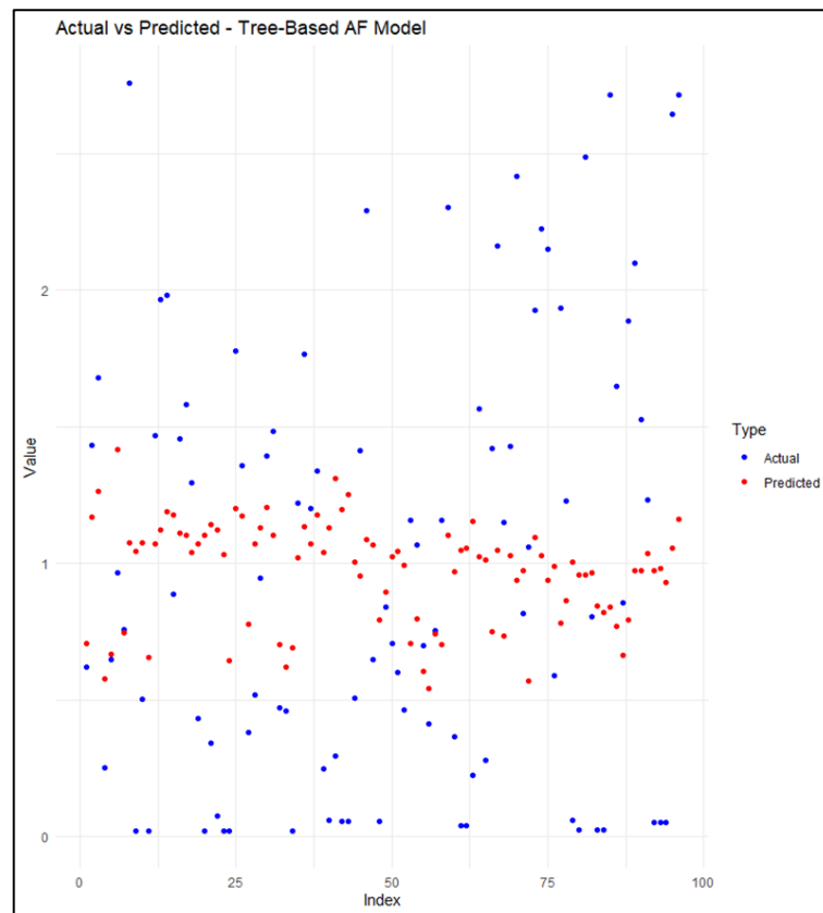
Figure 7: The actual vs predicted plot of the Tree-Based All-Features Model. The true values are represented by the blue points while the predicted are represented by the red points. For each record pair of actual/predicted at an index in the test set, the smaller the distance between one another, the closer the predictions are to the true values.
