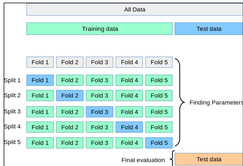
Figure 17: Cross validation estimation; five models are built with a different subset of the data and validated on a percentage not included in the training process. The error estimation is averaged (Source: https://scikit-learn.org ).
