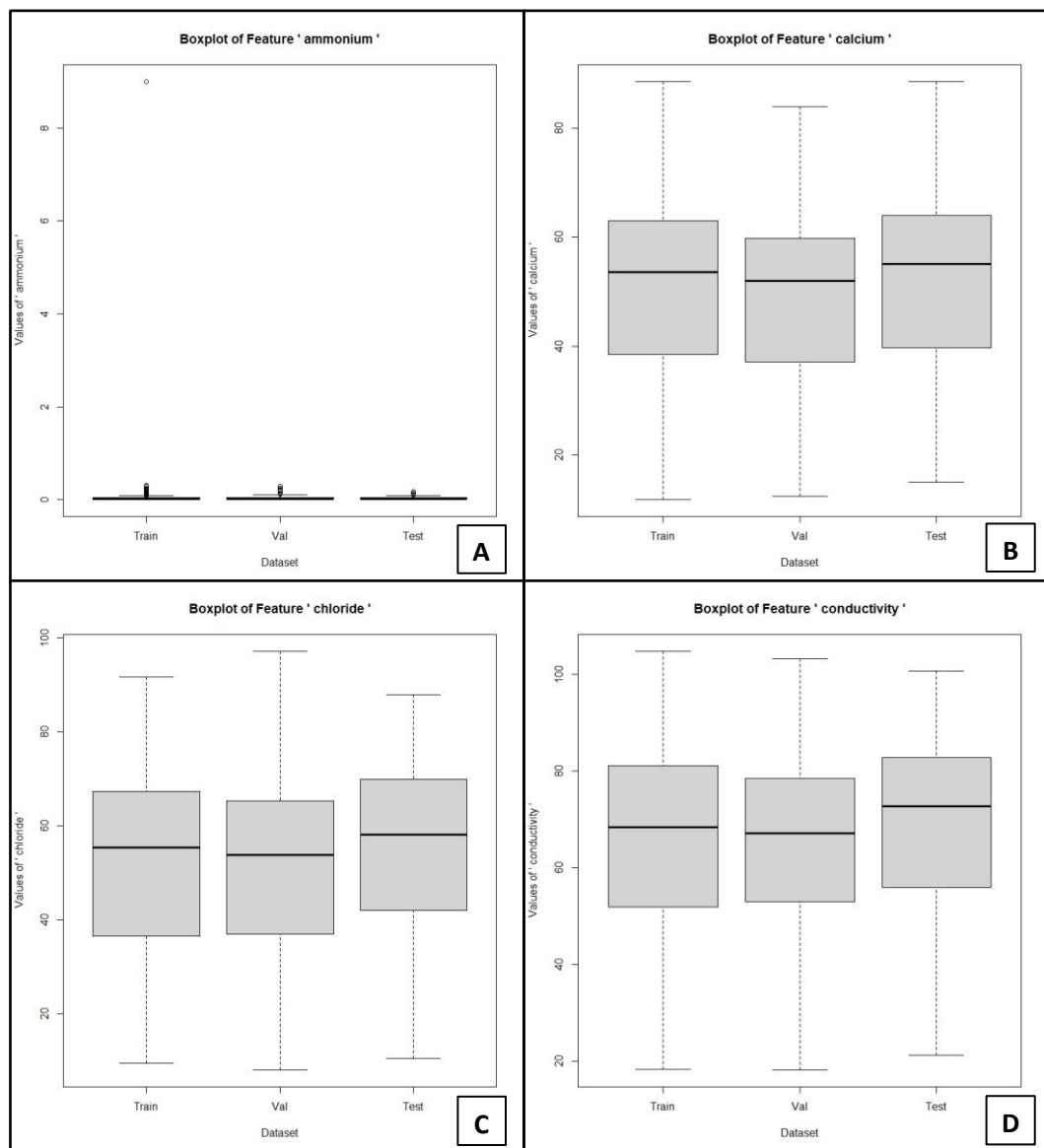
Figure 11: The boxplots for A) ammonium, B) calcium, C) chloride and D) conductivity.
