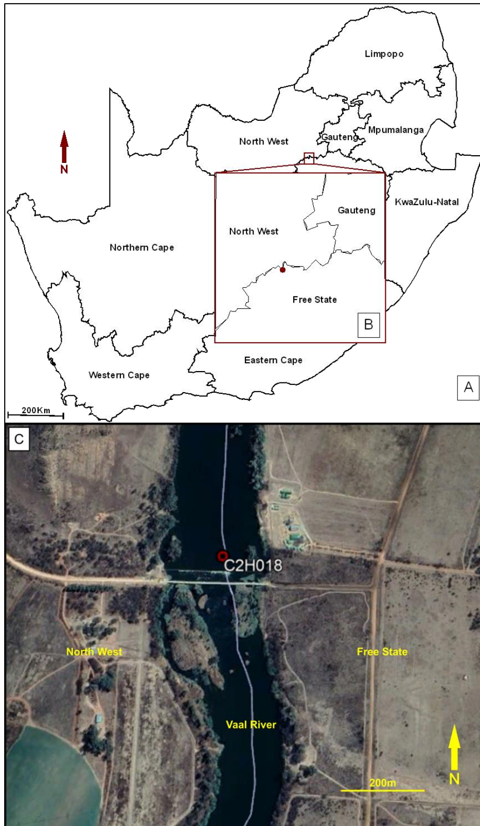
Figure 2: A) Monitoring sample station (C2H018) in South Africa. B) The approximate location of the site. C) The satellite image of the station on the Vaal River. (Data Sources: https://data.humdata.org and Google Earth).
