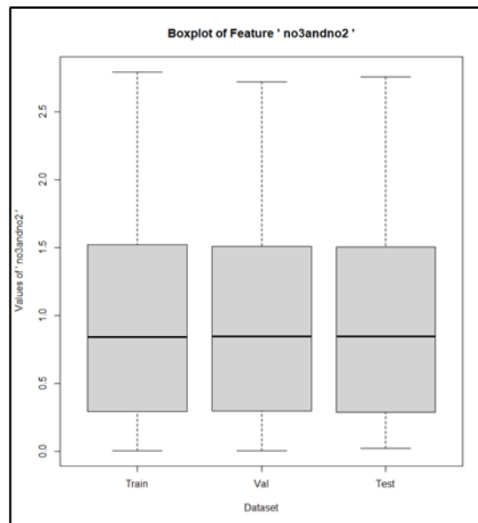
Figure 6: The boxplot for nitrate and nitrite.
