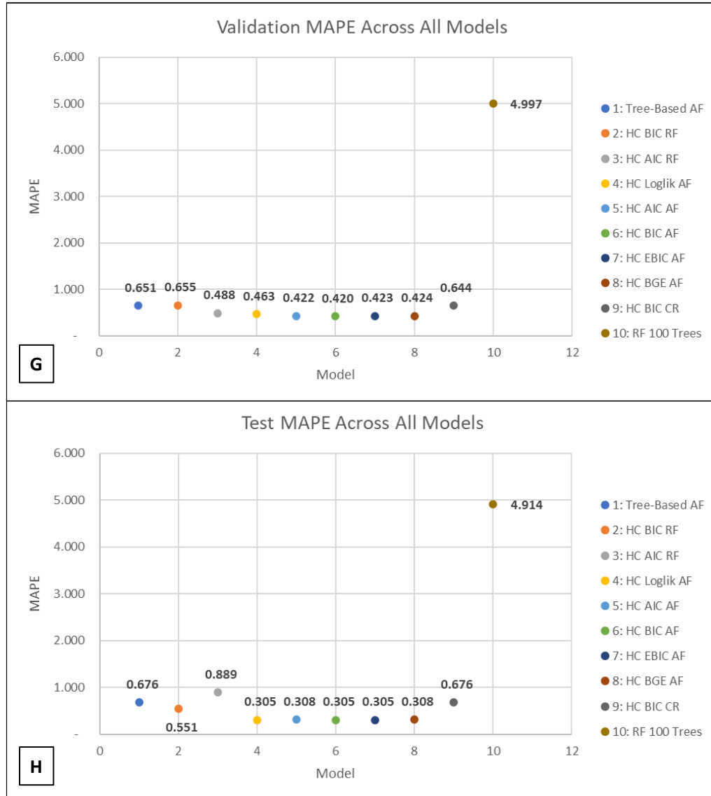
Figure 27: The MAPE evaluation metric values per model for the G) validation set and H) test set.
