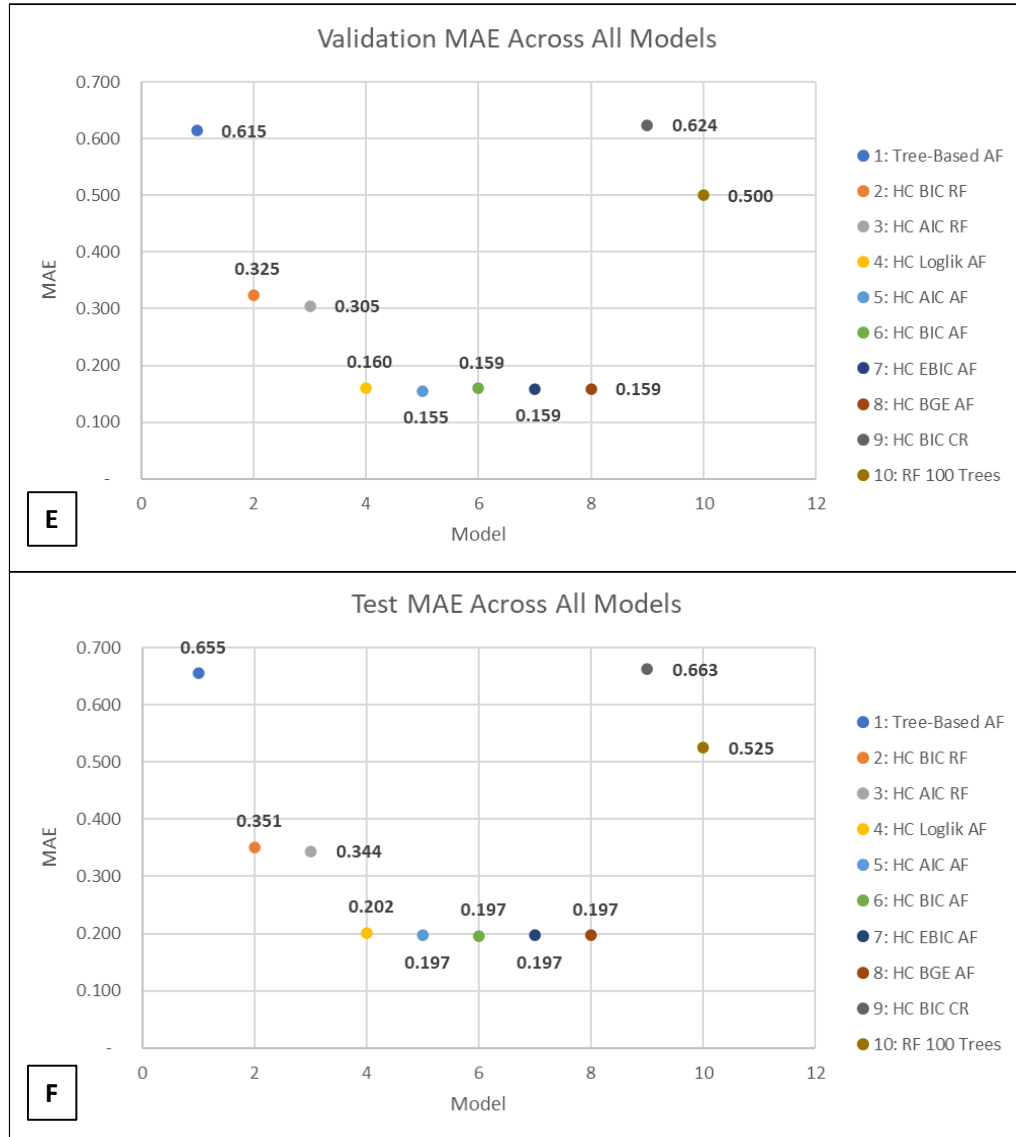
Figure 26: The MAE evaluation metric values per model for the E) validation set and F) test set.
