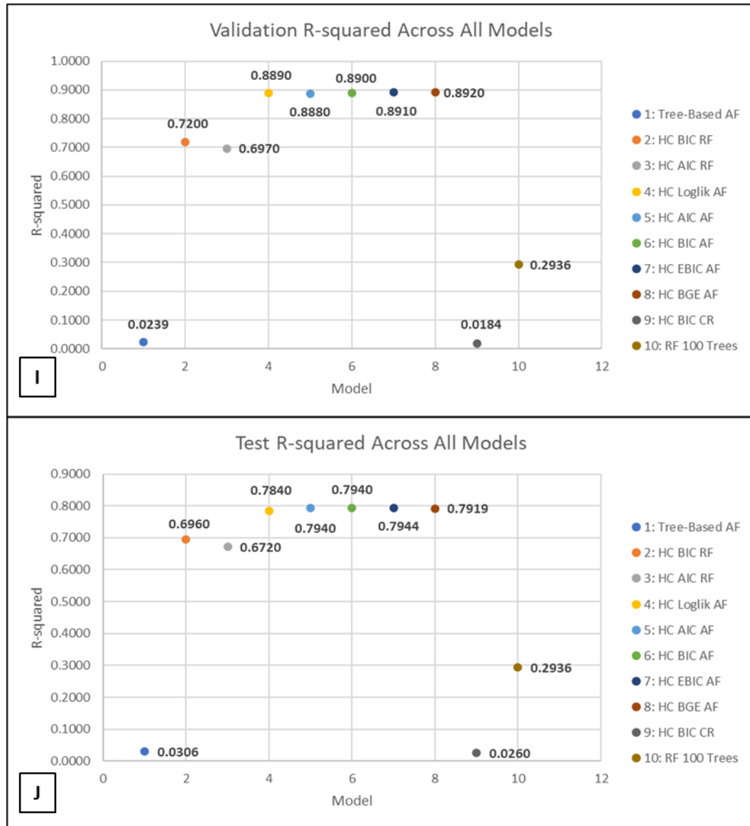
Figure 28: The R-squared evaluation metric values per model for the I) validation set and J) test set.
