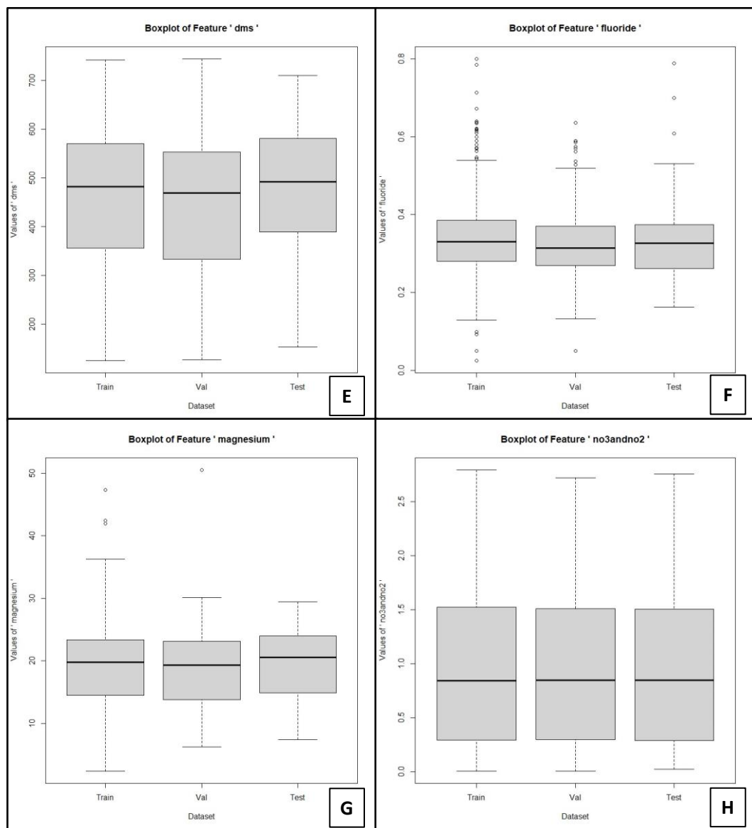
Figure 12: The boxplots for E) DMS, F) fluoride, G) magnesium and H) nitrate and nitrite.
