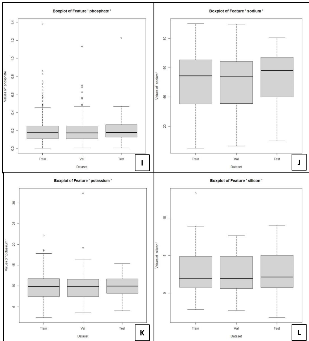
Figure 13: The boxplots for I) phosphate, J) sodium, K) potassium and L) silicon.
