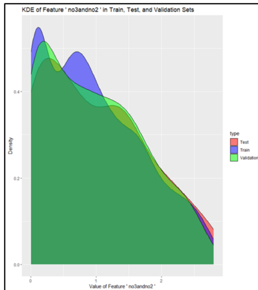
Figure 5: The kernel density estimation plot for nitrate and nitrite.
