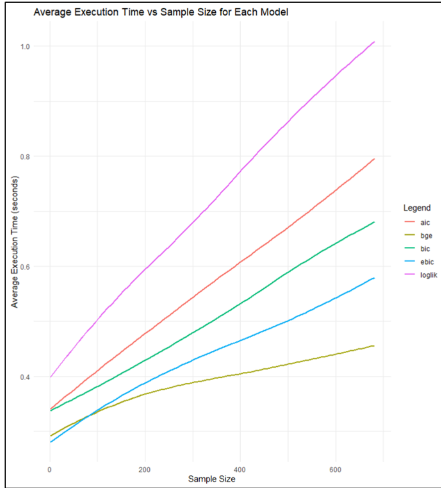
Figure 23: Execution Time per Sample Size for each model. As the sample size increases so does the time for the models to complete a training run with selected sample size.
