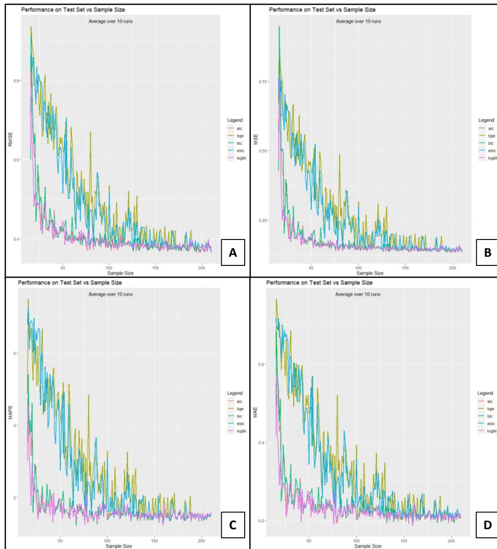
Figure 22: The prediction error for the models for A) RMSE, B) MSE, C) MAPE and D) MAE evaluation metrics.
