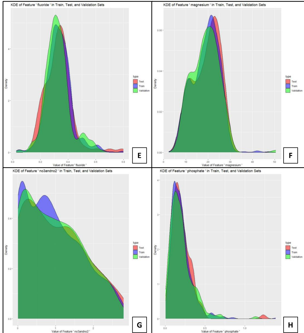
Figure 9: The Kernel Density Estimation plots for E) fluoride, F) magnesium, G) nitrate and nitrite and H) phosphate.
