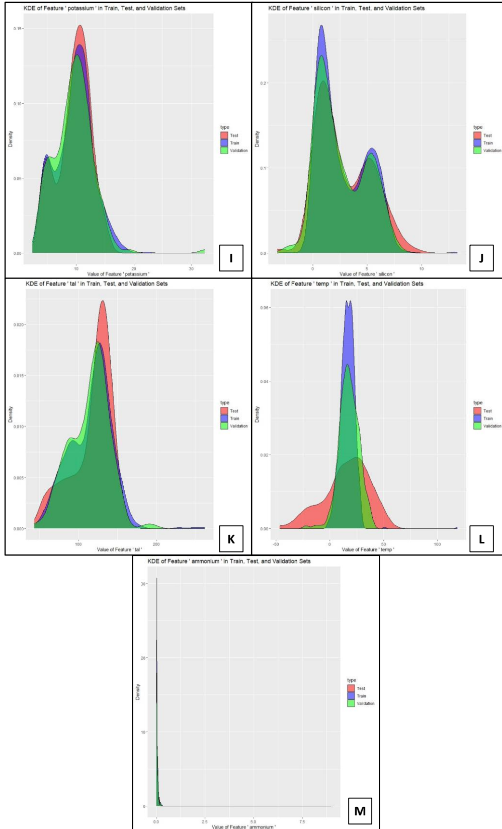
Figure 10: The Kernel Density Estimation plots for I) potassium, J) silicon, K) TAL, L) temperature and M) ammonium.
