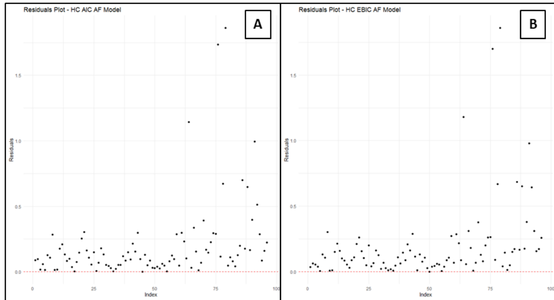
Figure 31: The residual plots for the A) HC-AIC-AF and B) HC-EBIC-AF models.
