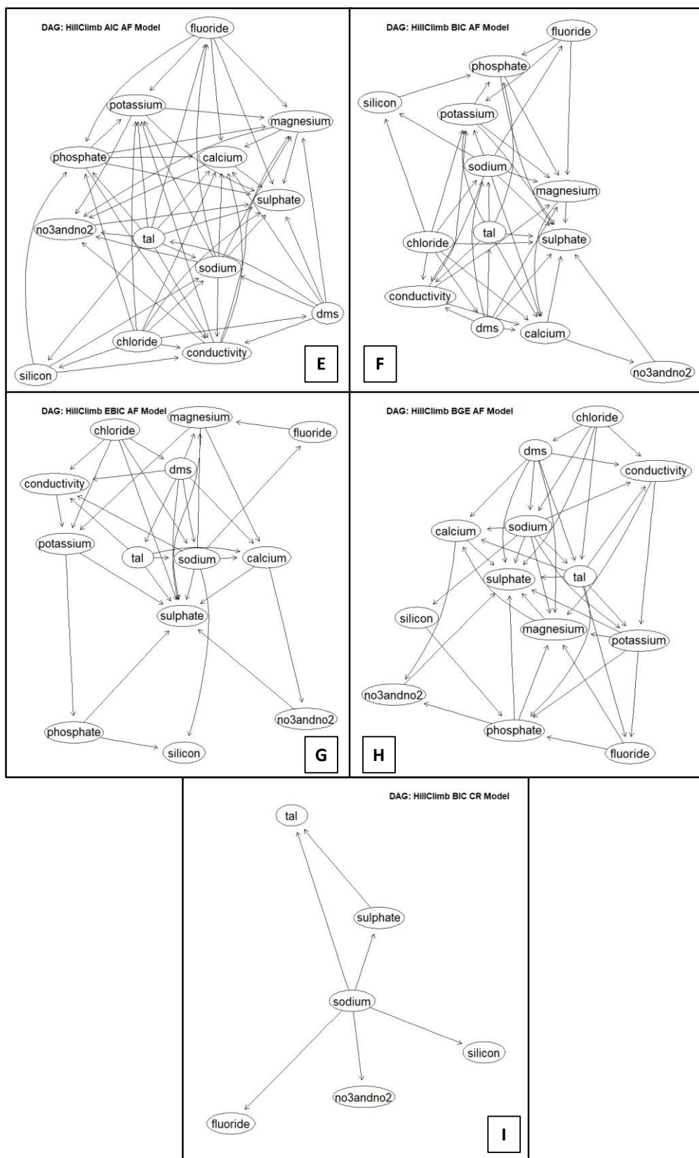
Figure 16: Directed Acyclic Graph (DAG) for E) HC-AIC-AF, F) HC-BIC-AF, G) HC_EBIC-AF, H) HC-BGE-AF and I) HC-BIC-CR.
