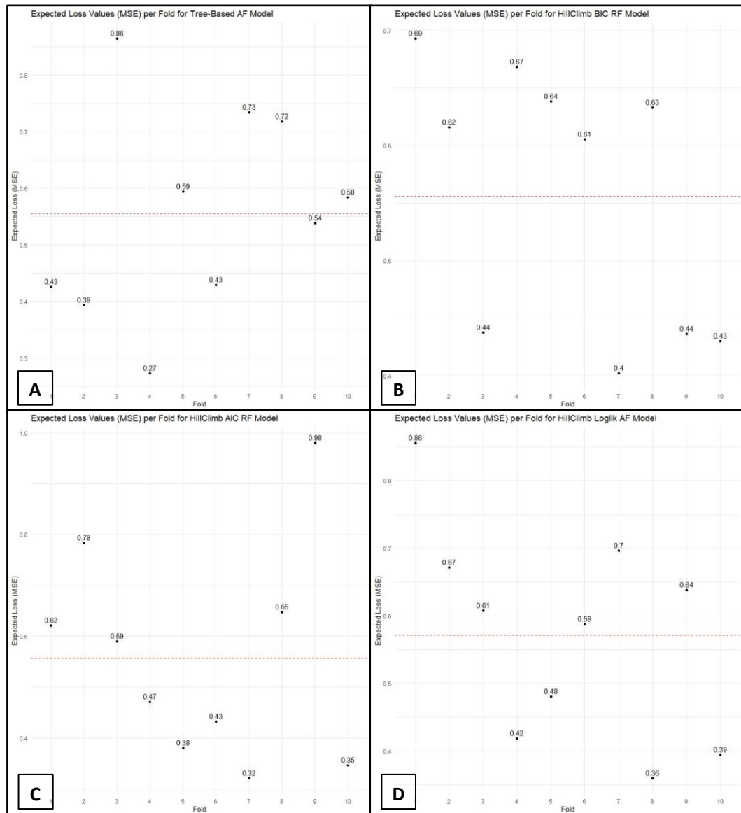
Figure 18: The cross-validation performance of the per fold for the A) Tree-Based-AF, B) HC-BIC-RF, C) HC-AIC-RF and D) HC-Loglik-AF models.
