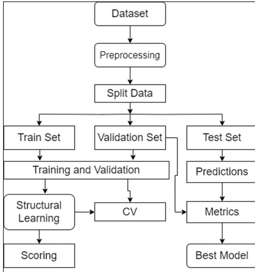
Figure 3: Flow chart of the data and modelling process as described in the research methodology, summarising the steps as taken from the machine-learning life cycle framework but include the modelling process using the Bnlearn R package.
