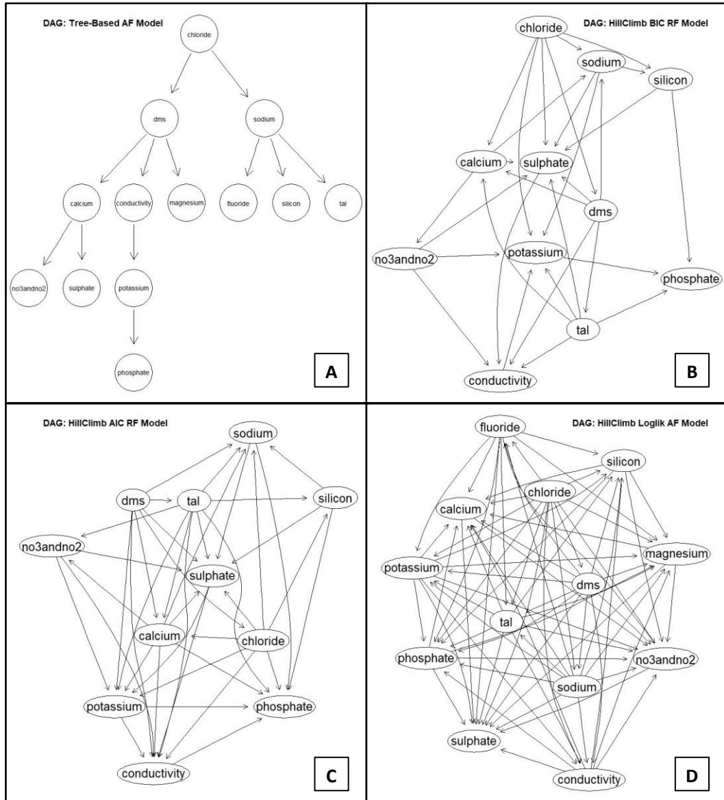
Figure 15: Directed Acyclic Graph (DAG) for A) Tree-Based-AF, B) HC-BIC-RF, C) HC-AIC-RF and D) HC-Loglik-AF.
