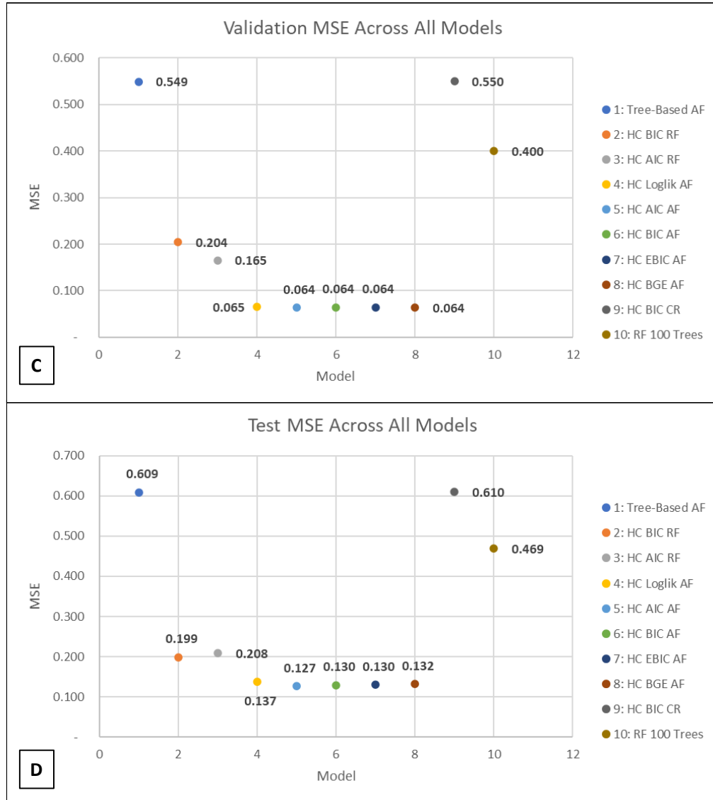
Figure 25: The MSE evaluation metric values per model for the C) validation set and D) test set.
