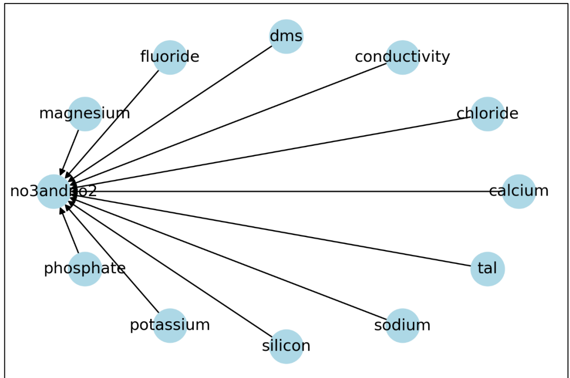
Figure 30: Features that influence nitrate and nitrite predictions, collated from all Bayesian Belief Networks.
