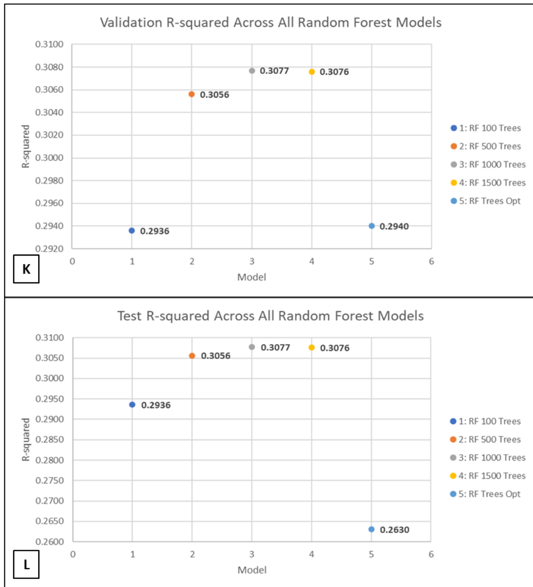
Figure 29: The R-squared evaluation metric values for all the Random Forest models for the K) validation set and L) test set.
