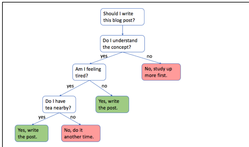
Figure 1: An example of a decision tree, designed with an explainable structure. By starting at the top and going down, level by level the final decisioning can be determined (source: (Xu et al. , 2019)).
