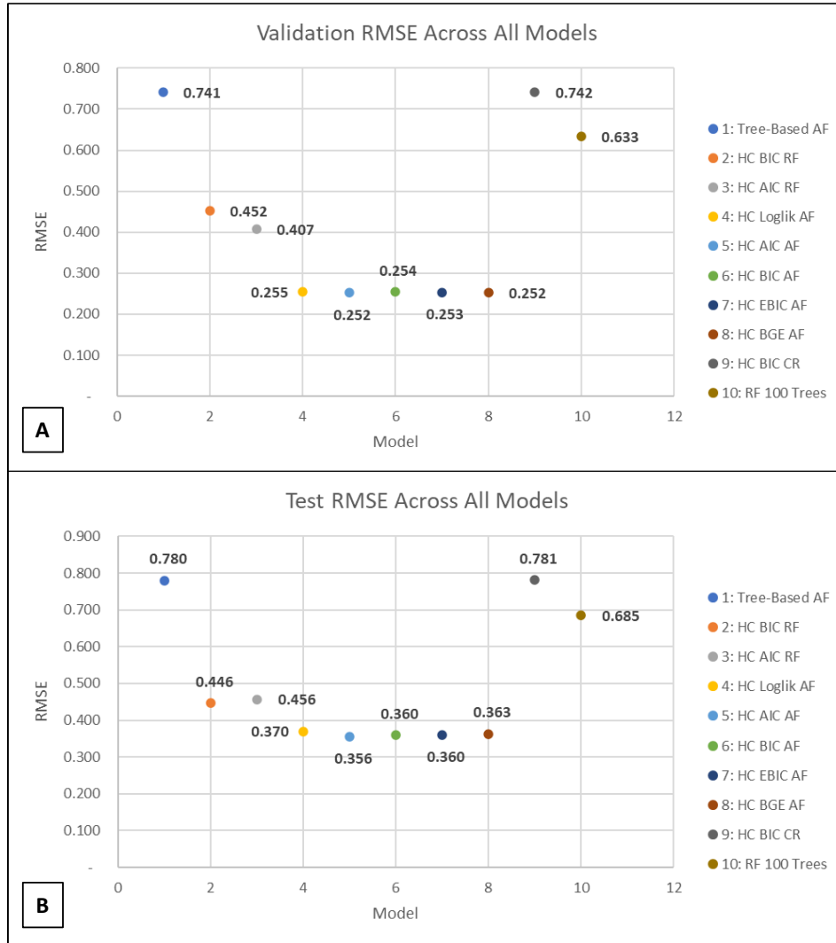
Figure 24: The RMSE evaluation metrics values per model for the A) validation set and B) test set.
