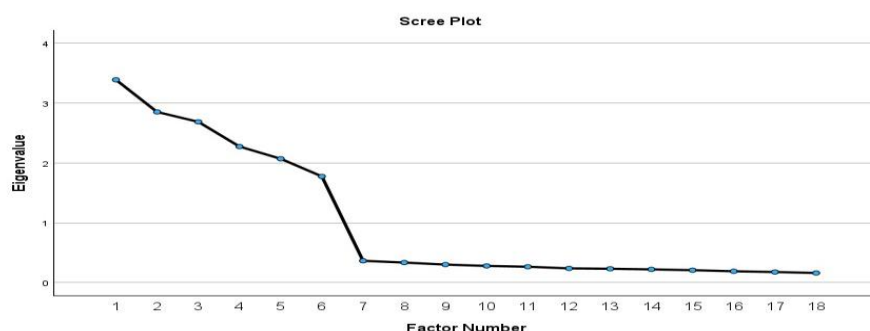
Figure 4. 6: Scree plot.
