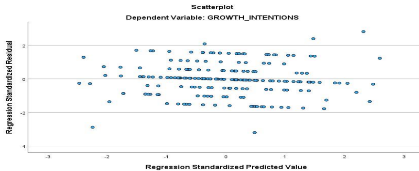
Figure 4. 10: Scatterplot.
