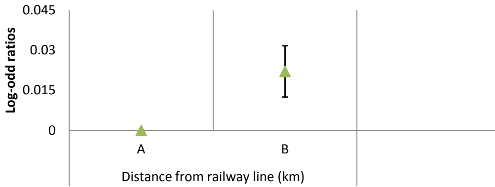
Figure 25: Distance from railway line estimates ( \pm 95\% confidence intervals) by female elephants for the wet season. A= 0-31.40 km and B = 31.41-62.80 km. Females occurred mostly at the distance furthest from railway lines.
