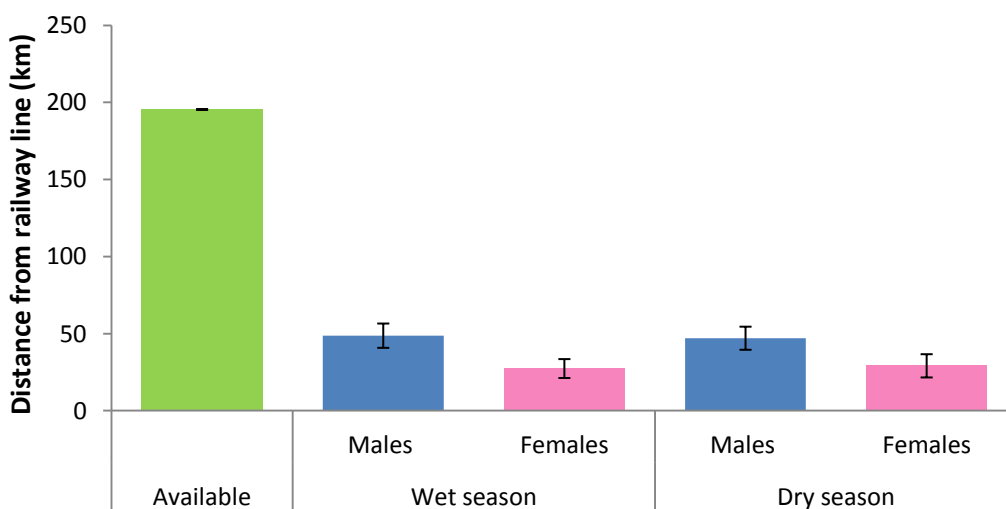
Figure 10: Mean ( \pm SE) distance (km) of male and female elephants from railways in relation to the furthest available distance for railway lines in the study site (shown in green) in the wet and dry seasons.
