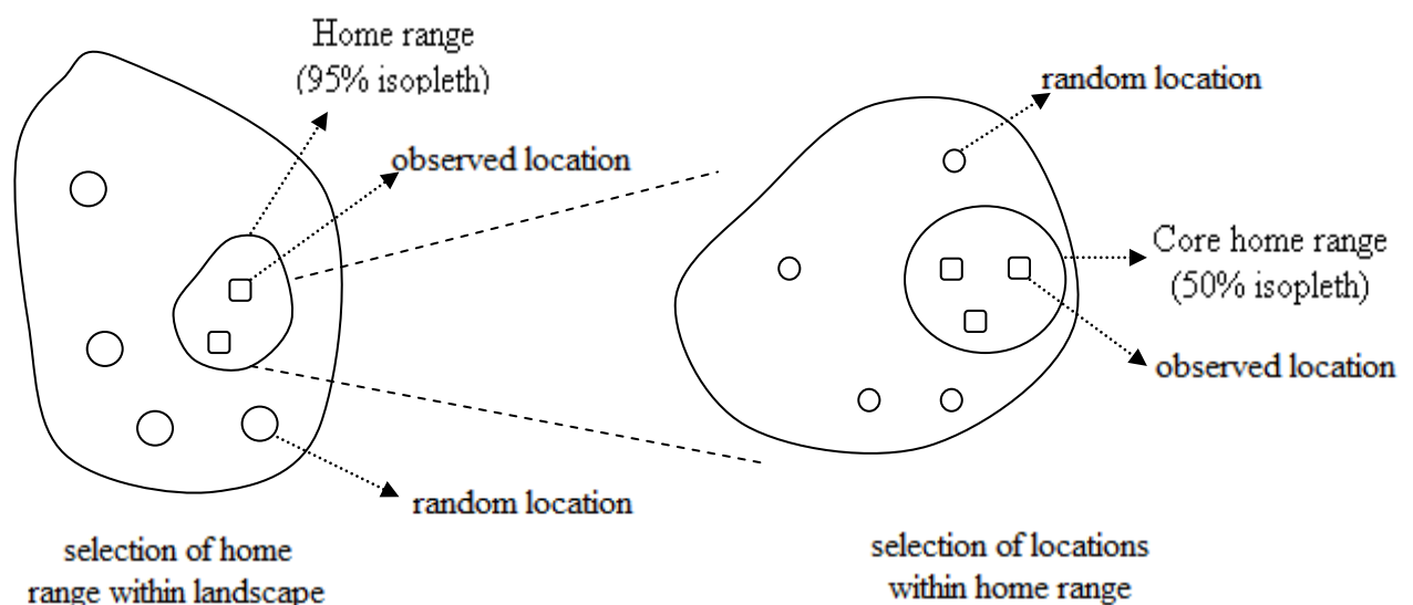
Figure 2: Diagram showing 2 nd order selection on the left and 3 rd order selection on the right.
