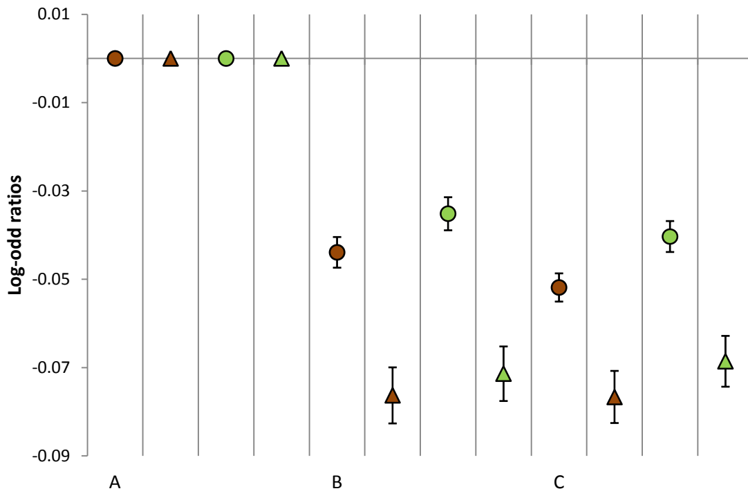
Figure 9: Distance from road estimates ( \pm 95\% confidence intervals) by male (○) and female (Δ) elephants for the dry (brown) and wet (green) season. A= near. B= intermediate and C=far. Males occurred at far locations from roads more than females.
