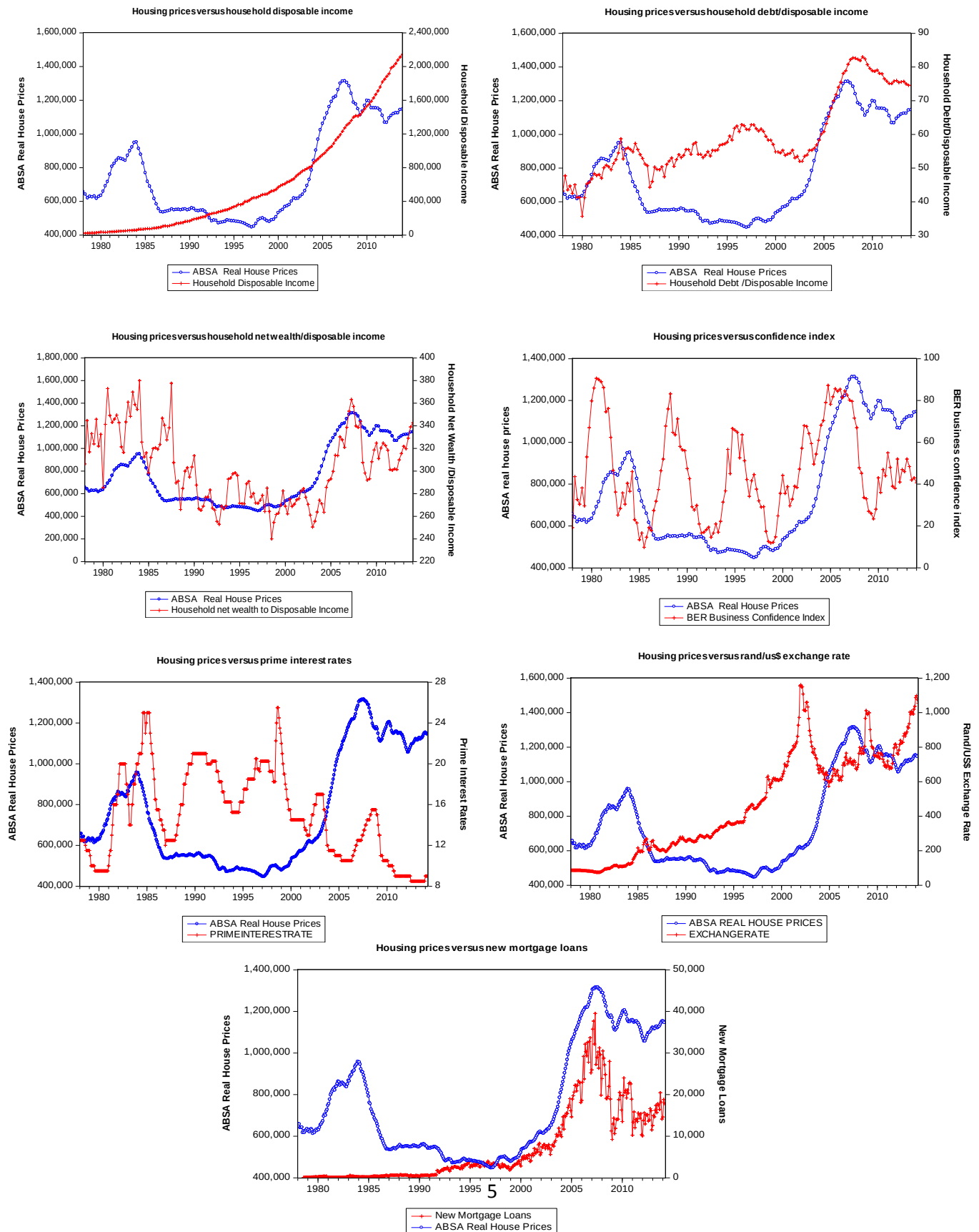
Figure 1: Time series trends in ABSA real house prices and macroeconomic variables
