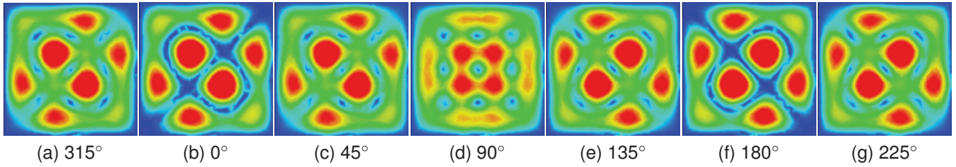
Fig. 11. Simulated colourmap of the EM near-field depicting the hotspot positions as a function of phase shift at 2.385 GHz for Model 2. Simulation generated by CST Studio Suite.
