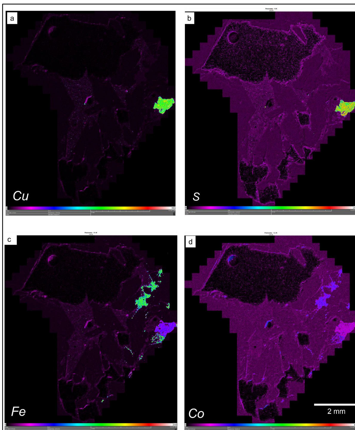
Figure 33: (a-d) Elemental maps showing concentrations of Cu=copper, S=sulphur, Fe=iron, and Co=cobalt in sample 19077 copper sulphides.
