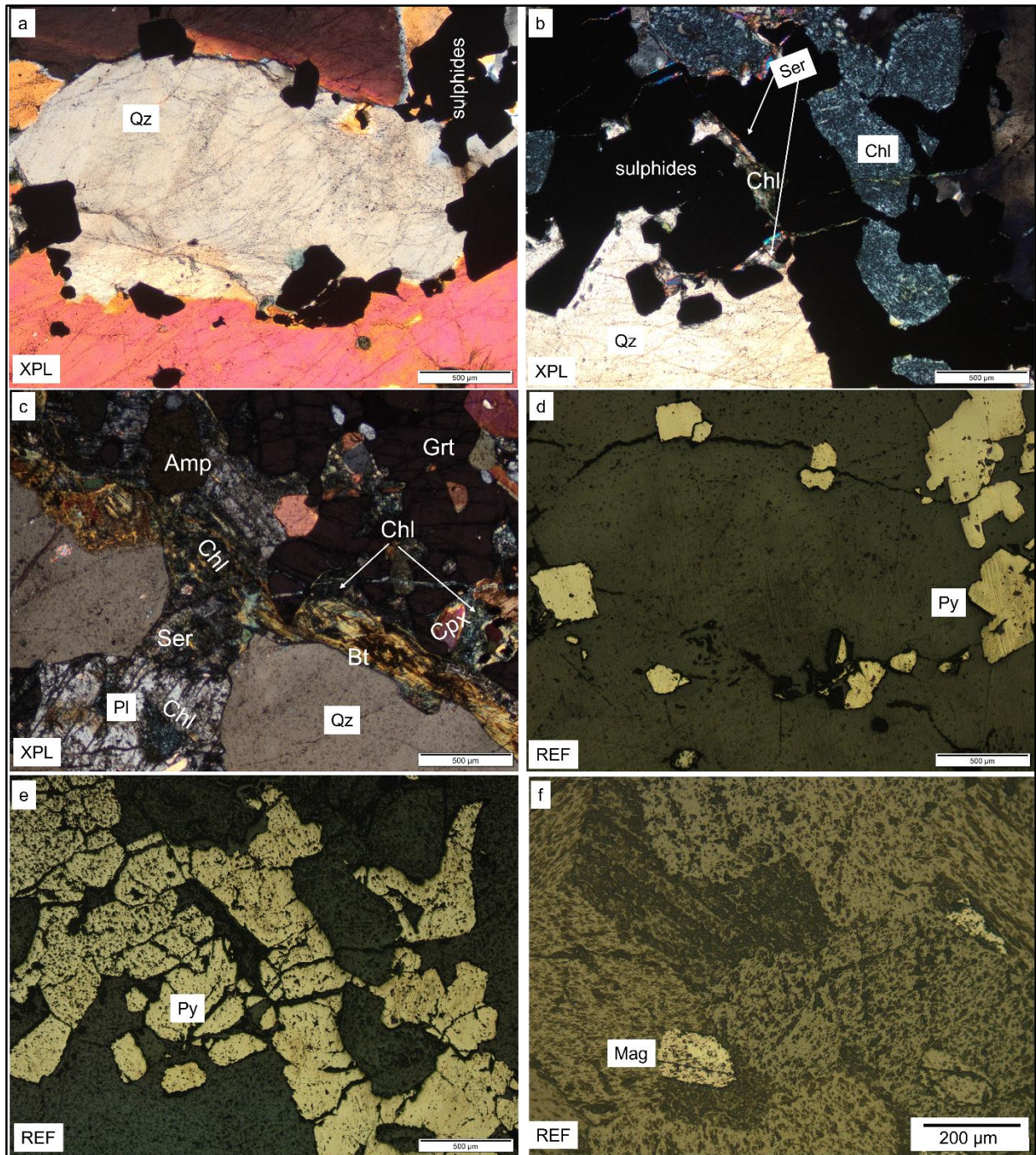
Figure 25: Photomicrographs showing: (a) interconnected, large clear quartz (Qz) grains, typical of blocky vein cementing the opaque minerals; (b) subhedral blue chlorite (Chl) with sericite (Ser) cut through the opaque minerals. Sericite also occurs along quartz margins and granular chlorite; (c) contact between the quartz vein and brecciated country rock. The country rock contains fragments of partially altered garnet (Grt), amphibole (Amp), clinopyroxene (Cpx), and biotite (Bt) embedded within plagioclase (Pl). These fragments penetrate the quartz vein; (d) disseminated pyrite grains preferentially aligned around quartz grain boundaries; (e) fractured and porous clusters of pyrite with inclusions of tiny magnetite grains; (f) subhedral magnetite within the altered country rock. Magnification scale = 500 µm and 200 µm.
