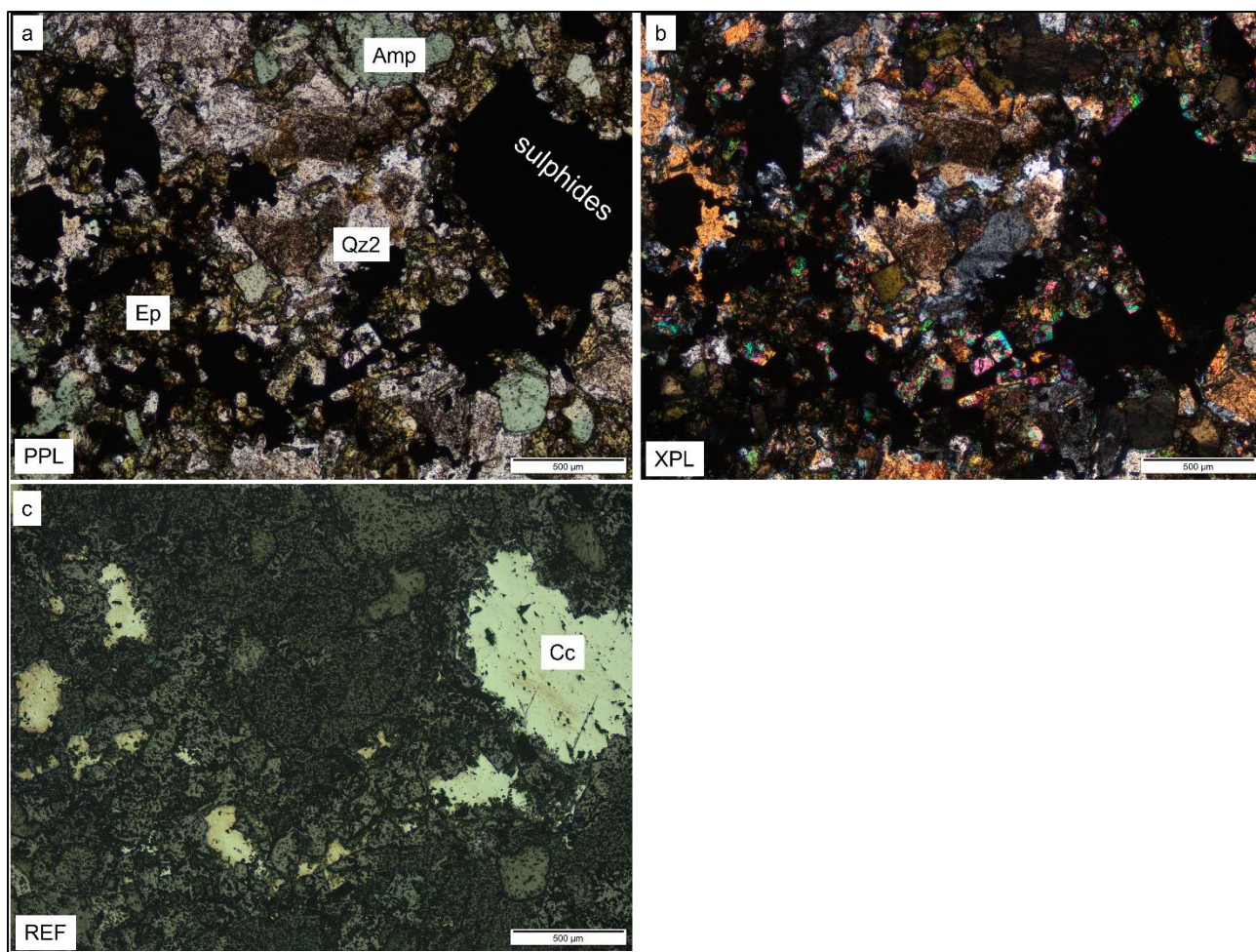
B30: (a-c) extension of B27 with disseminated chalcocite (small to large, 0.2-0.6 mm) within the gangue and enclosed by the gangue (mostly epidote). Epidote and amphibole occur as inclusions within the quartz grains in places.
