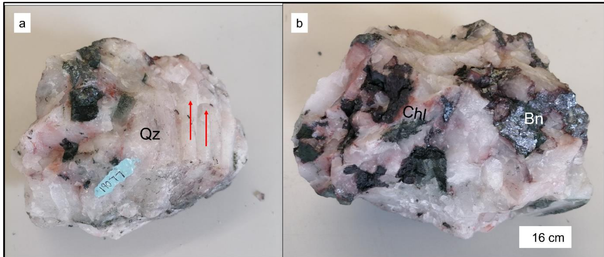
Figure 10: Sample 19077 showing massive interconnected and brecciated quartz crystals (Qz) which contain minor chlorite (Chl) and bornite (Bn). Red arrows in (a) show the elongation of individual quartz crystals, typical of comb veining.
