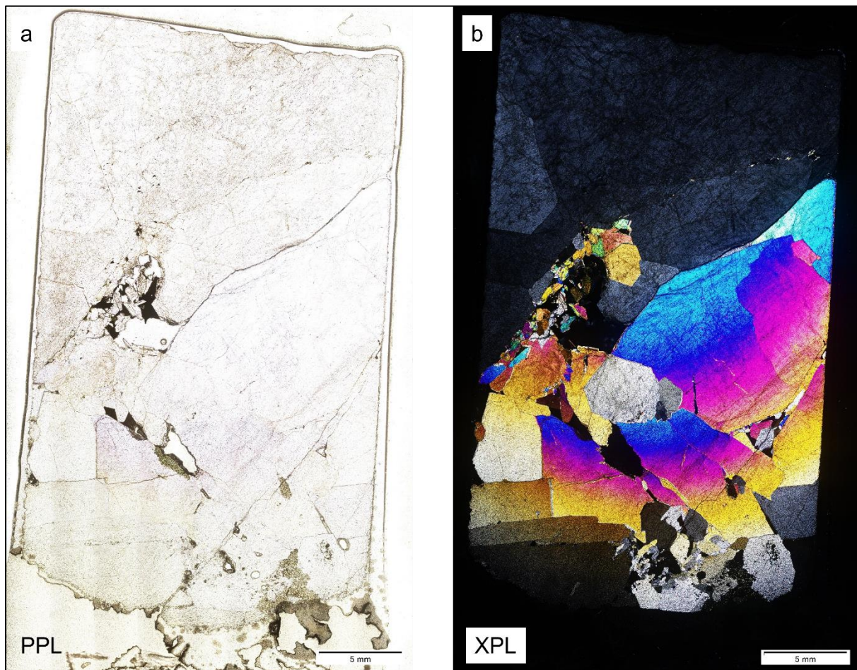
A5: Full-scan photomicrographs for sample 19077 in (a) PPL and (b) XPL. The sample is dominated by quartz grains. Other silicate minerals and the sulphides are concentrated in open spaces/fractures between the large quartz grains. The thin section size = 5 mm.
