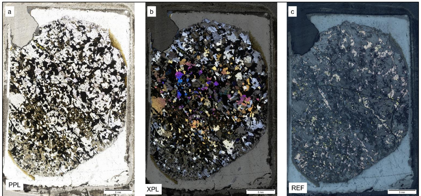
B21: Full scan photomicrographs for Sample P679 in PPL (a), XPL (b), and REF (c). The sample is dominated by brecciated quartz grains intergrown with brownish-green chlorite. Sulphides (mainly bornite) occurs between the open spaces of quartz and altered biotite as disseminations and anhedral grains. Sample size = 5 mm.
