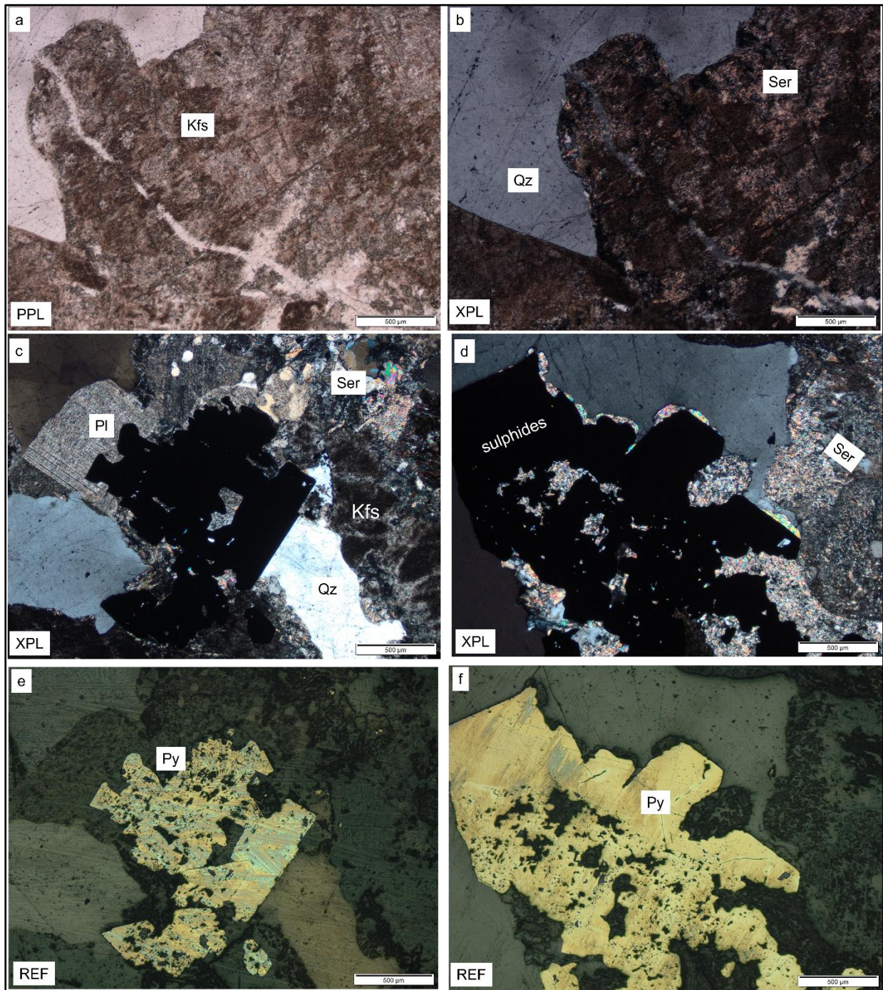
Figure 22: Photomicrographs showing: (a-b) fine-grained sericite (Ser) associated with large, clear quartz grains (Qz) and alters K-feldspar (Kfs, dark brown); (c-d) anhedral quartz grains surrounded by partially sericitised K-feldspar associated with a single plagioclase grain. Sericite partially rims quartz and the opaque minerals. Corroded ser, pl, and kfs occur within the opaque minerals; (e-f) clustered pyrite (Py) grains with inclusions of corroded gangue minerals. Some smaller pyrite grains also occur as disseminated grains within sericite gangue. Pyrite grains are tarnished due to polishing. Magnification scale = 500 µm.
