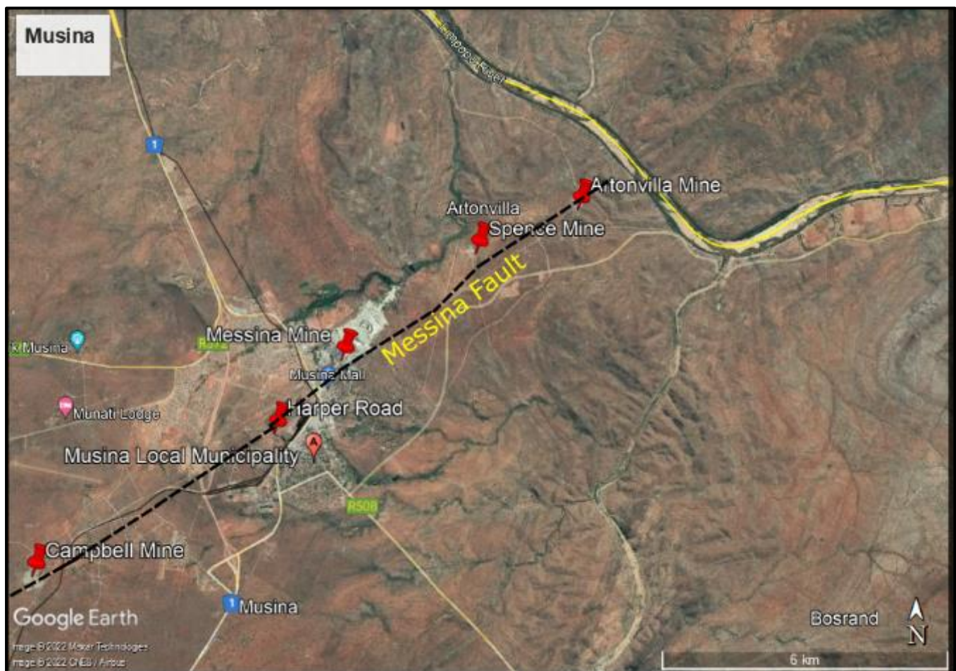
Figure 1: Google Earth image showing the location of Musina town and different mines within Messina mining district. The stippled line shows Messina Fault.
