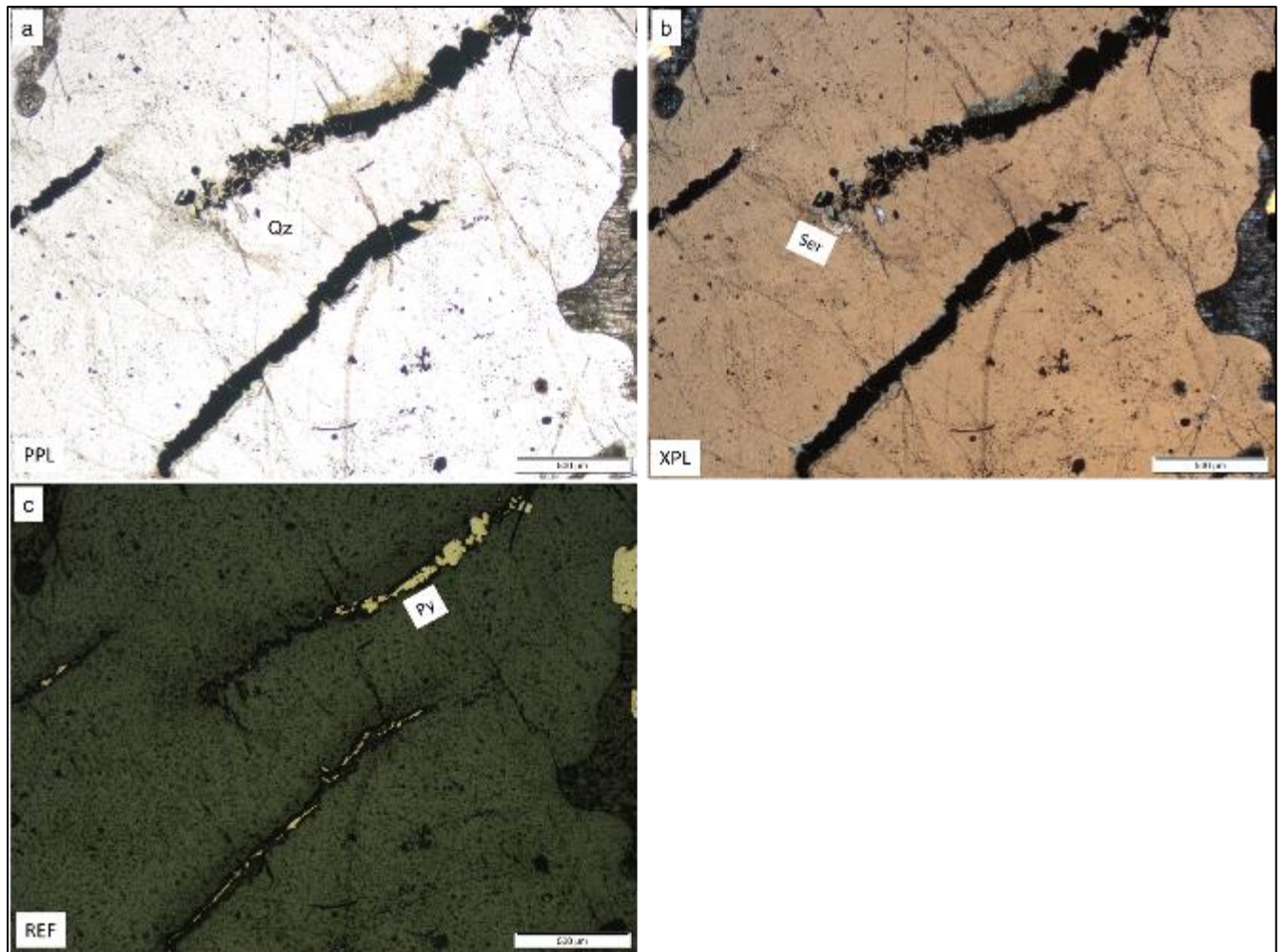
B46: (a-b) large, clear quartz grains contain isolated linear open spaces that are filled by the opaque minerals. Minor sericite is seen along the margins of the open spaces within the quartz grains. Interstitial sericite also invades the large, clear quartz grains; (c) the open spaces are filled by anhedral pyrite grains.
