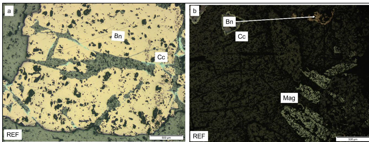
A2: (a) subhedral massive bornite is surrounded by chlorite groundmass and other chlorite veinlets cut across it; (b) magnetite laths are surrounded by fine-grained chlorite groundmass which also occurs between the laths. The remnant gangue is seen being corroded by the magnetite in some parts. The bright colour of the bornite is due to reflected light exposure/reflectance.
