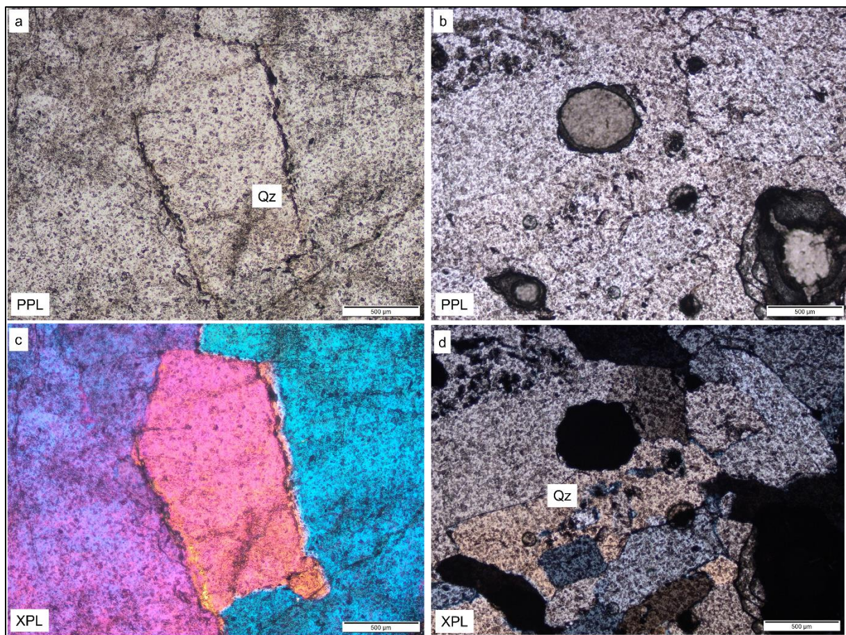
A8: (a-c) interconnected quartz grains with irregular-smooth grain boundaries. The rounded dark grey grains represent polishing pits; (d) subhedral and sub-rounded quartz inclusions also occur between large grains. The grains appear to be partly brecciated though still in contact with one another. The black areas within the grains are polishing pits.
