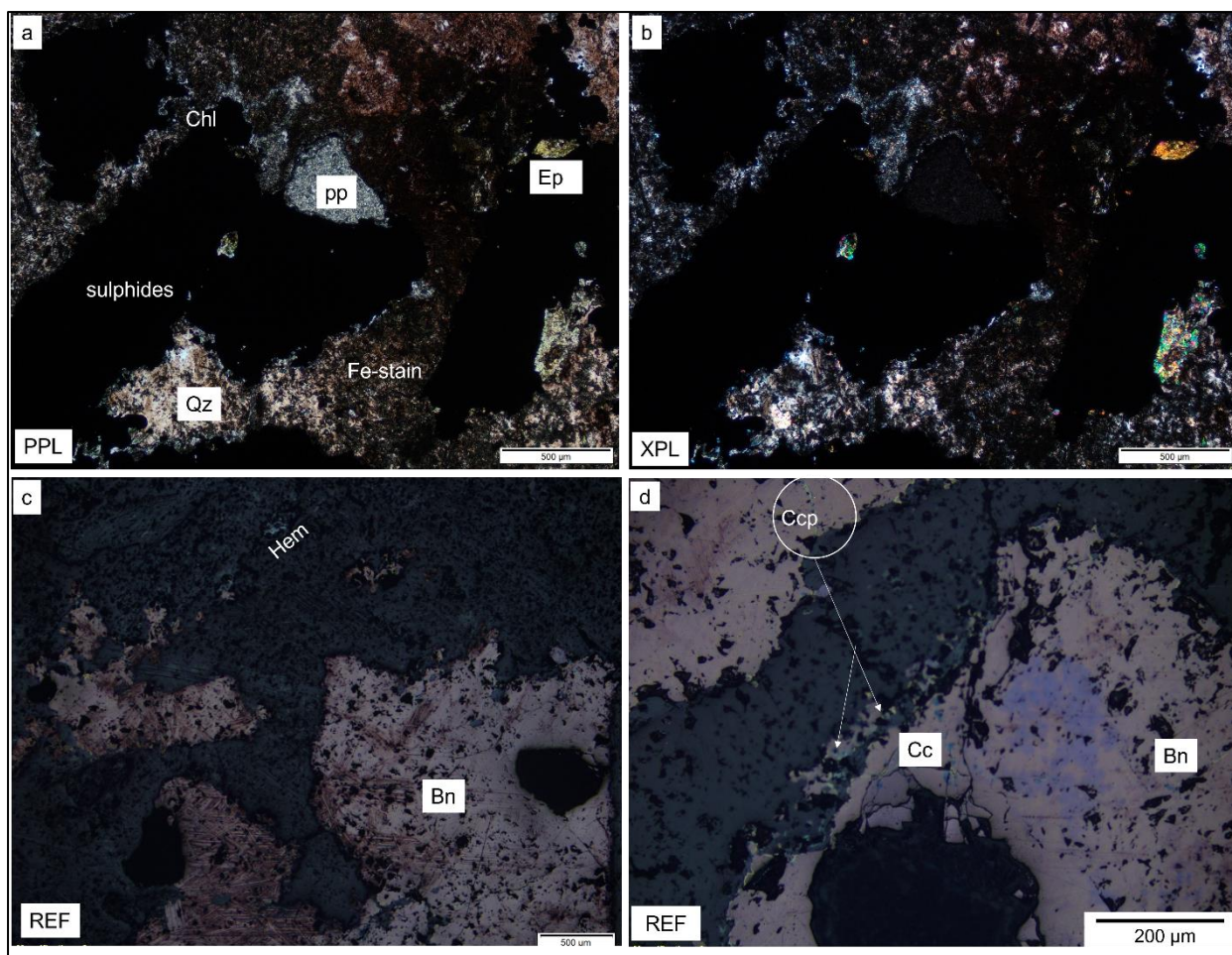
A13: (a-b) heavily iron-stained cryptocrystalline is intergrown with irregular chlorite that is partially altered into epidote and enclose the opaque minerals; (c-d) coarse-grained subhedral bornite is enclosed by quartz and chlorite-epidote gangue. Bornite contains tiny spots of a blue chalcocite (white circle and arrows) and yellow chalcopyrite relics.
