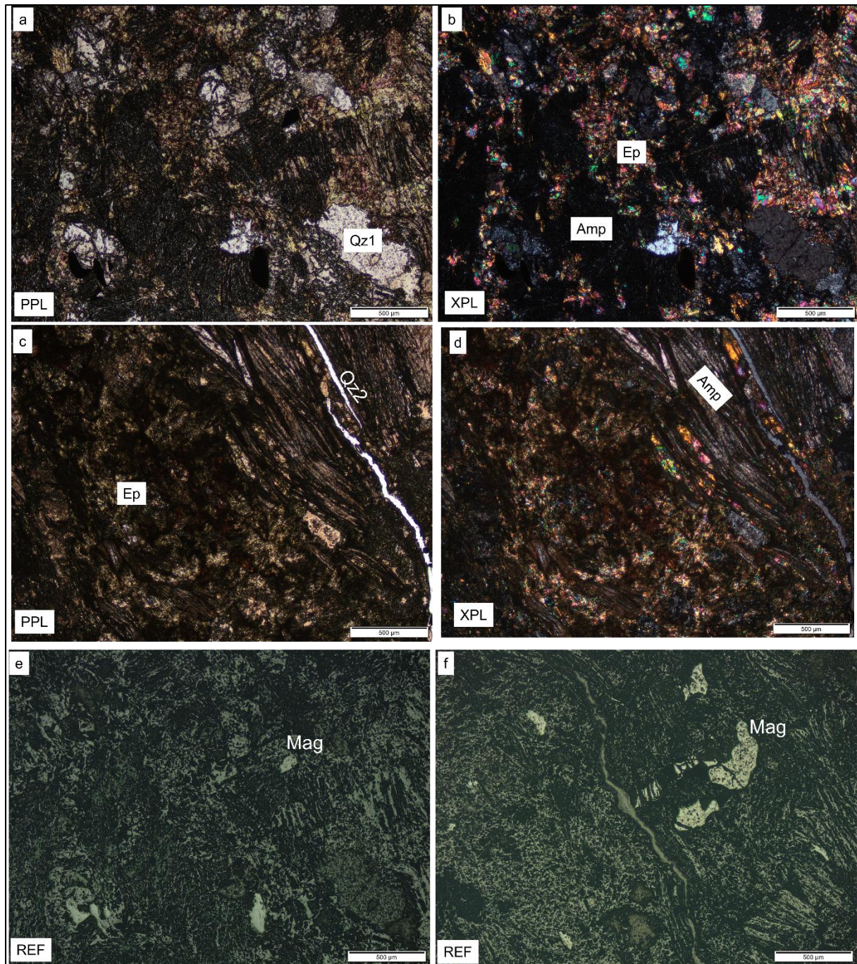
Figure 28: Photomicrographs showing: (a-b) epidote (Ep) aggregates enclose and partially alter subhedral amphibole (Amp) grains. Subhedral secondary quartz 1 cements epidote aggregates and amphibole relics. Some epidote grains are included within quartz 1; (c-d) discontinuous thin veins of secondary quartz 2 cuts through epidote aggregates and occur between elongated amphibole prismatic grains; (e-f) subhedral magnetite grains within epidote and amphibole grains. Magnification scale = 500 µm.
