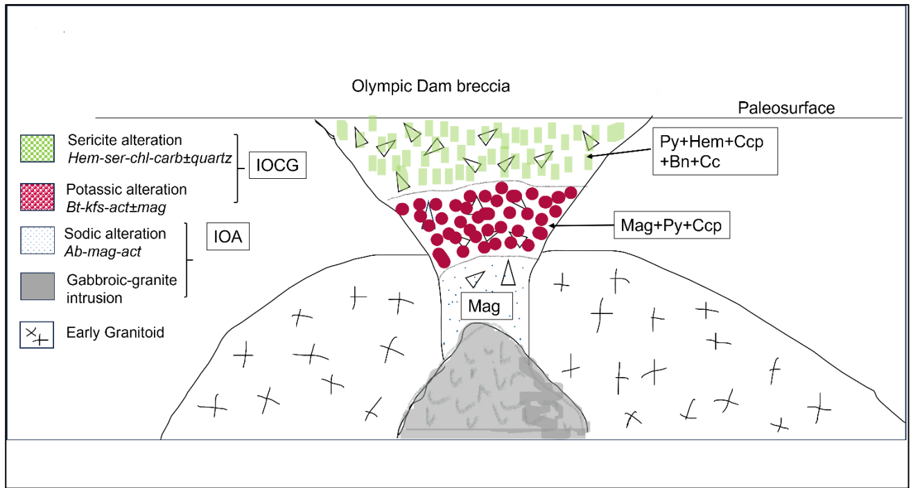
Figure 49: A sketch of the Olympic Dam IOCG breccia complex intrusion into early granitoid rocks showing mineralisation and the associated alteration within the breccia (after Reid, 2019 and Skirrow, 2022).
