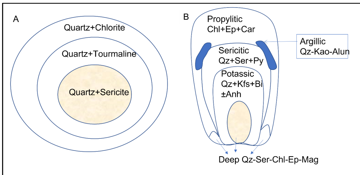
Figure 48: Zonation of hydrothermal halos in (A) Greisen deposits (from Elliot et al. , 1995) and (B) Porphyry copper systems (Lowell and Guilbert, 1970). Kao=Kaolinite, Alun=Alunite, Anh=Anhydrite, Car=Carbonates.
