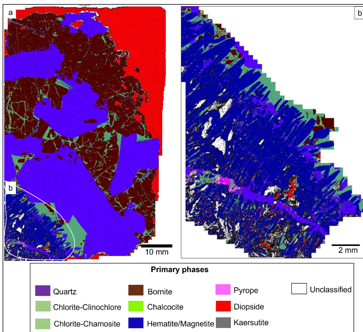
Figure 29: Phase maps showing detected minerals in sample 19068: (a) Full scan phase map; (b) high-resolution phase map.
