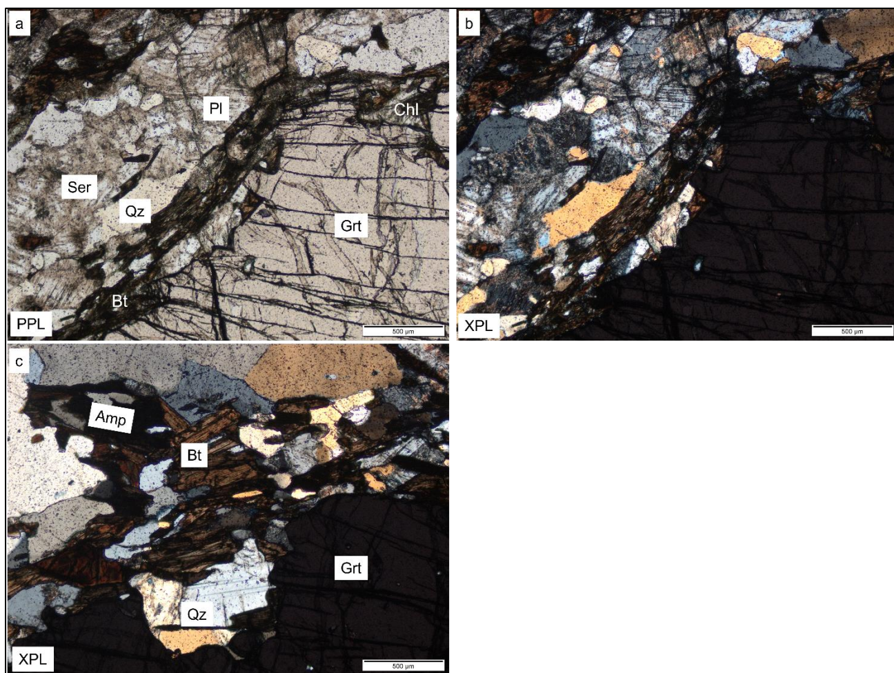
B16: (a-b) secondary quartz, biotite, fractured garnet, and fine-grained sericite are the dominant silicate minerals of this sample. The biotite flakes preferentially wrap the garnet grains and occur in contact with amphibole grains. Fine-grained sericite is altering plagioclase (recognized by multiple twinning). All the silicate minerals are overprinted by subhedral-subrounded quartz grains. The biotite and garnet grains are being partially replaced by chlorite (blue in XPL); (c) fractured garnet (isotropic) and brown biotite irregular flakes are overprinted by subhedral quartz grains.
