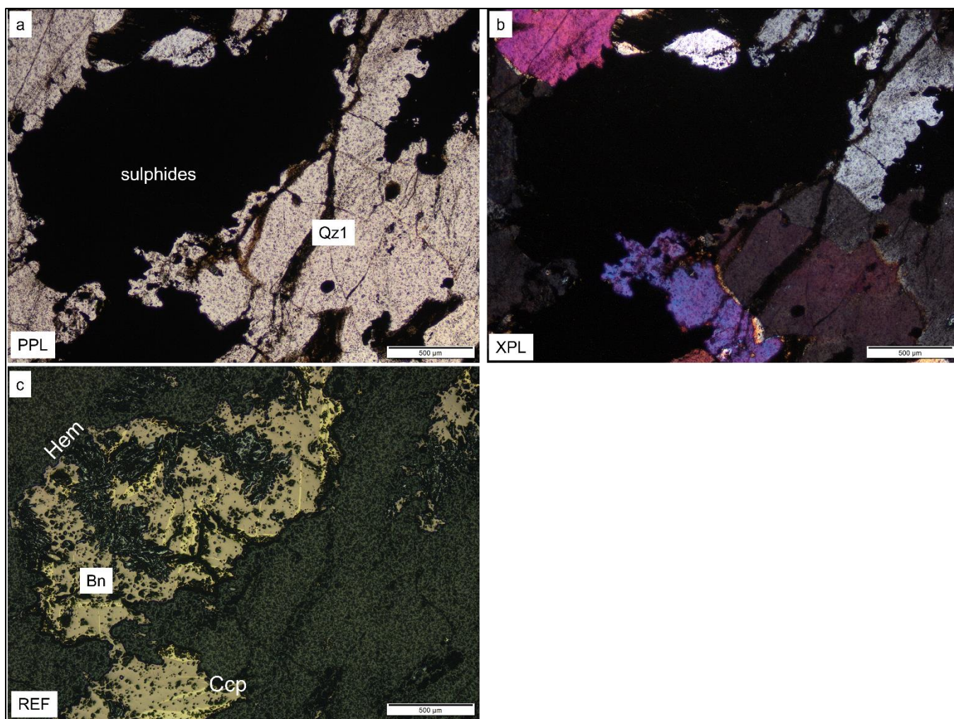
B22: (a-b) corroded and partly fractured quartz grains with distinct grain boundaries enclose the opaque minerals between them and some opaque minerals fill corrosion spaces within quartz. In crossed polarising light, the quartz grains exhibit interconnection of the grains; (c) preferential orientation of thin flame-like relics of chalcopyrite occurs within the host bornite and represents replacement of chalcopyrite by bornite. Small bladed hematite aggregates occur within the host Bn and in contact with chalcopyrite. Minor bornite grains occur as inclusions within the hematite aggregates.
