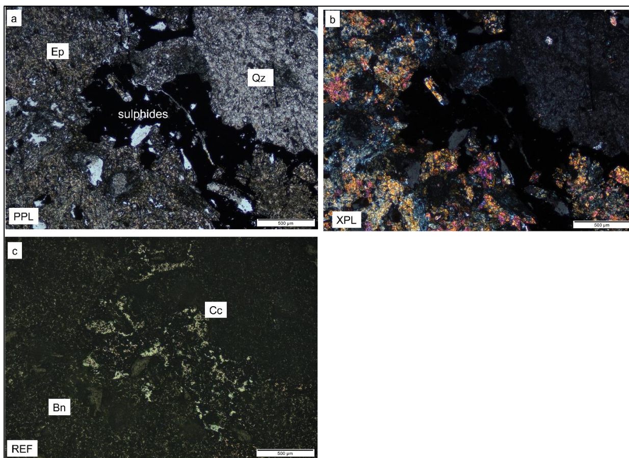
A19: (a) small irregular secondary clear quartz grains occur within the granular brownish-yellow epidote aggregates. The epidote aggregates surround the opaque minerals, which are also disseminated between the aggregates; (b) blue chlorite is altering into epidote. Minor epidote aggregates occur within the opaque minerals in other places; (c) tarnished bornite is anhedral between primary cloudy quartz grains and epidote aggregates and is being replaced by chalcocite along margins.
