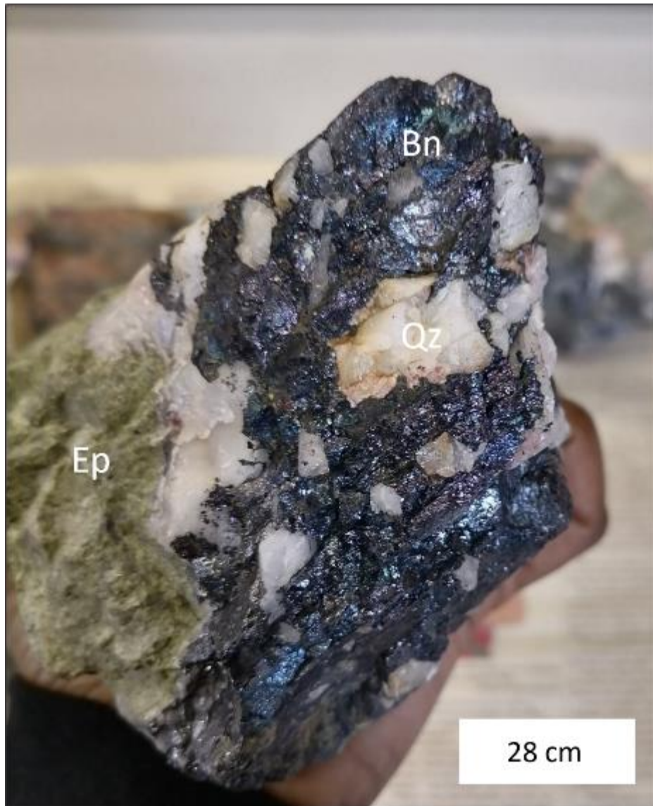
Figure 16: Sample 19078 showing one part representing epidotised (Ep) country rock and the other part representing a mineralised brecciated milky white quartz vein. The contact between them shows irregular quartz (Qz) as a rim. In other parts, bornite is in direct contact with the epidotised country rock. Minor large, subhedral quartz crystals also occur within the epidotised country rock. Fine-grained epidote (Ep) groundmass is also in direct contact with the massive bluish-purple black bornite (Bn).
