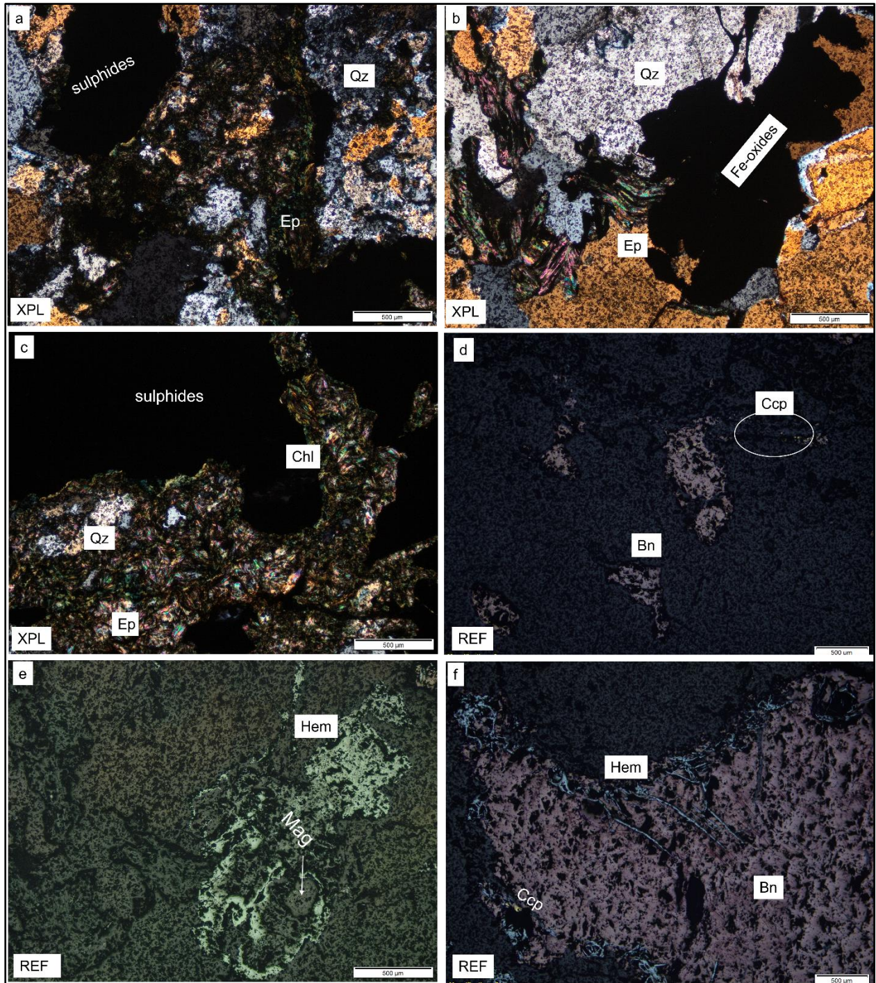
Figure 15: Photomicrographs showing: (a) brecciated quartz (Qz) fragments with interstitial granular chlorite-epidote; (b) quartz fragments with irregular fibrous epidote (Ep) between the fragments; (c) interstitial granular chlorite (Chl) with quartz inclusions invade the opaque minerals; (d) disseminated and anhedral lenses of bornite with minor chalcopyrite replaced by bornite along a fracture; (e) anhedral hematite (Hem) enclosing grey magnetite grains (Mag); (f) coarse-grained bornite (Bn) with minor bright yellow chalcopyrite is abutted by irregular to elongated hematite blades along the margins. Magnification scale = 500 µm.
