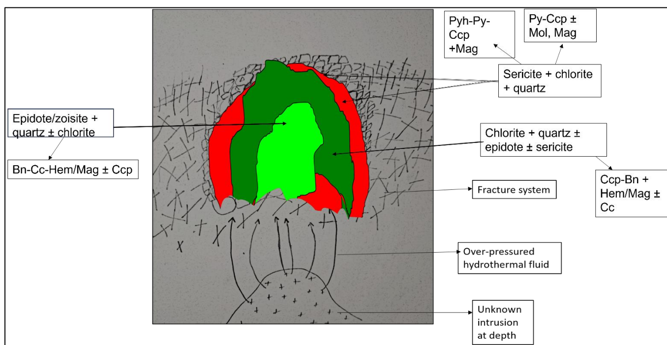
Figure 47: Idealised sketch of the concentric zonation of alteration and associated sulphides and iron oxides of the Messina Cu deposit. The overlapping sequences of mineral crystallisation due to alteration and metasomatism is shown by irregular shapes of alteration zones. The red zone is evident in samples P817, P812, P782, P814, P579, dark green zone in samples 19075, 19077, 19068, P679, P613, and lime-green zone in samples 19078, 19073, P744, and P580.
