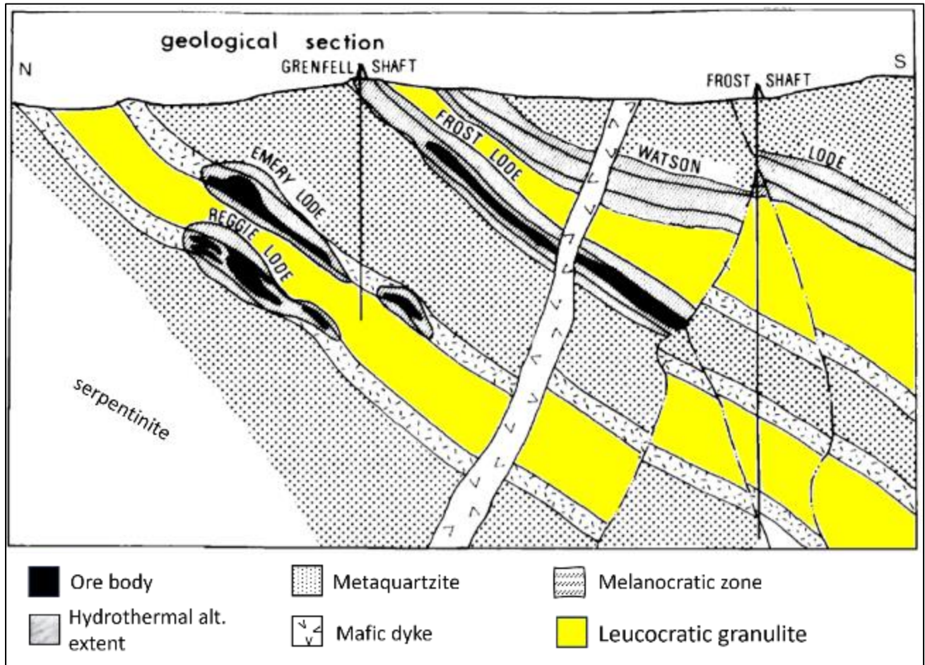
Figure 4: Geological cross-section of Artonvilla mine shafts showing the occurrence of mineralisation within mafic and felsic granulites at Frost Lode, Emery Lode, and Reggie Lode (after Jacobsen and McCarthy, 1976).
