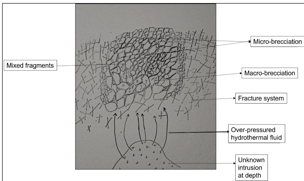
Figure 46: Sketch showing characteristics of Messina Cu deposit breccia pipe(s). Black fillings between fragments are alteration minerals, quartz, and sulphides.
