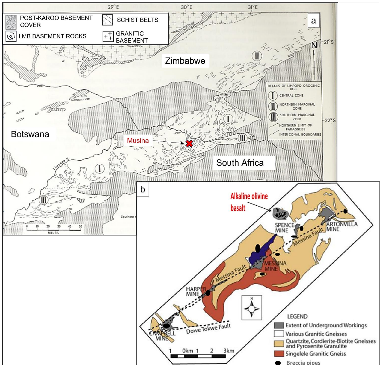
Figure 3: Simplified geology of the location of (a) Musina area within the Central Zone of the Limpopo Mobile Belt and (b) the distribution of mines along the Messina Fault in Messina mining district. Breccia pipes are represented by the small, black circular-like shapes (after Cox et al. , 1965; Mundalamo, 2019). LMB = Limpopo Mobile Belt.
