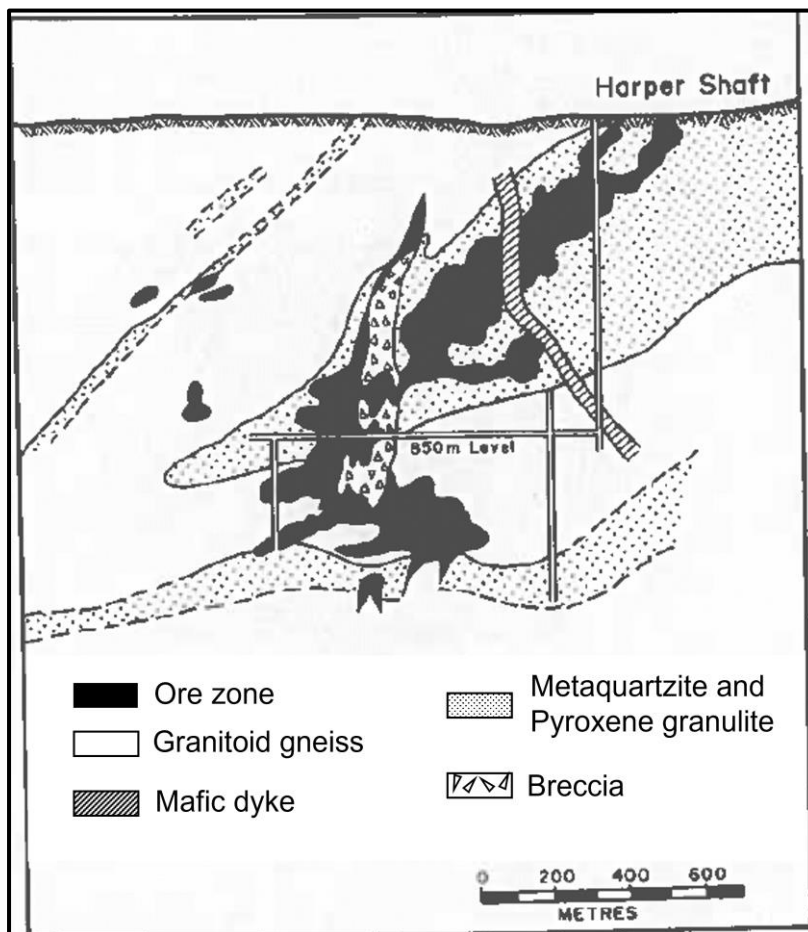
Figure 2: A cross-section showing mineralisation styles within the metamorphic country rocks of Musina area in Harper mine (Bahnemann, 1986).
