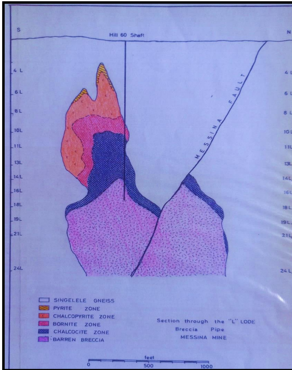
Figure 5: Sketch showing sulphide zonation in the L Lode breccia pipe of Messina mine (from Jacobsen, 1967).
