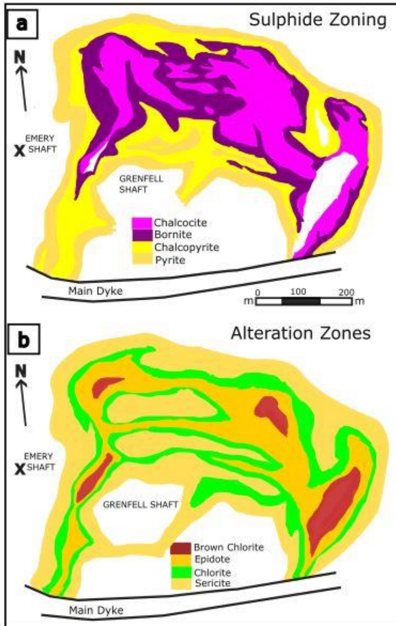
Figure 6: Sketch showing the concentric zonation of (a) the sulphides and (b) associated hydrothermal alteration zones in Emery Lode of Artonvilla mine (after Jacobsen and McCarthy, 1976). The white areas within sulphide zoning represent leached ore.
