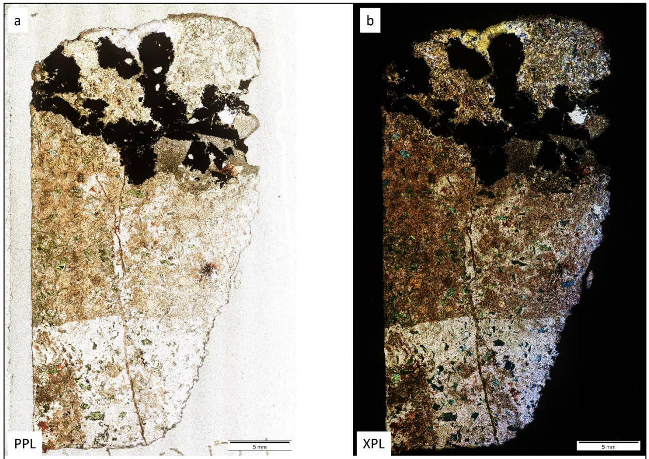
A9: Full-scan photomicrographs for Sample 19073 in (a) PPL and (b) XPL. Microcrystalline quartz makes up the groundmass for this sample. It is heavily coated by Fe-staining such that the quartz appears brown red. Small, elongated and subhedral grains of green-blue chlorite and harlequin epidote are embedded within the microcrystalline quartz groundmass. Fe-stained quartz veins cut through the groundmass and not the opaque minerals. Subhedral to irregular opaque minerals are surrounded by the microcrystalline groundmass and also contain irregular grains of quartz, chlorite and epidote. Sample size = 5 mm.
