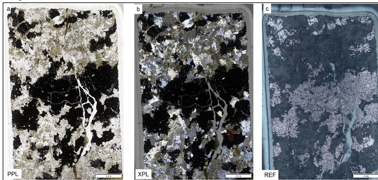
B1: Full-scan photomicrographs for Sample P580 in PPL(a), XPL (b), and REF (c). The sample contains quartz, sericite, chlorite, and epidote. Under reflected light, massive coarse-grained bornite represent the dominant opaque mineral with minor chalcocite. The elongated thin vein-like features represent resin and not an actual vein. Sample size = 5 mm.
