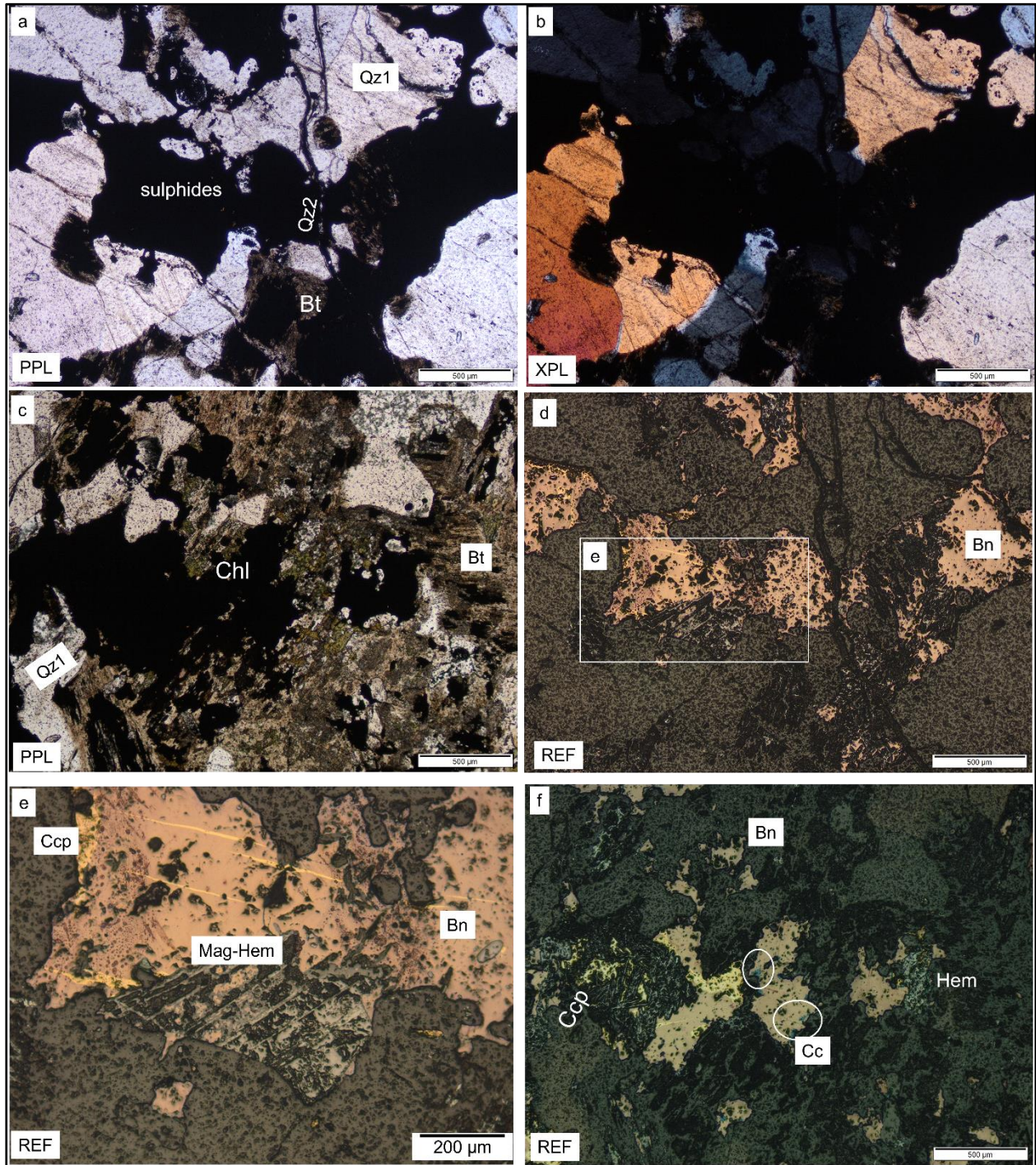
Figure 20: Photomicrographs showing: (a-c) subhedral and subrounded quartz (Qz1) grains intergrown with iron-stained biotite (Bt). Quartz veinlets (Qz2) cut through quartz 1, biotite and opaque minerals. Biotite is partially altered and replaced by chlorite; (d-e) subhedral and anhedral lenses of bornite (Bn) with flame-like lamellae and islands of chalcopyrite (Ccp) occur between quartz and biotite gangue. Hematite-magnetite exsolution lamellae is seen abutting bornite; (f) subhedral disseminations of bornite within corroded spaces of quartz 1 grains. Minor chalcocite spots occur along bornite margins (white circles). Irregular hematite (Hem) grains occur along cleavage planes of biotite and are in places enclosing chalcopyrite. Figure (e) represents a high-magnification image of the area outlined by a white square in Fig (d). Magnification scale = 500 µm and 200 µm.
