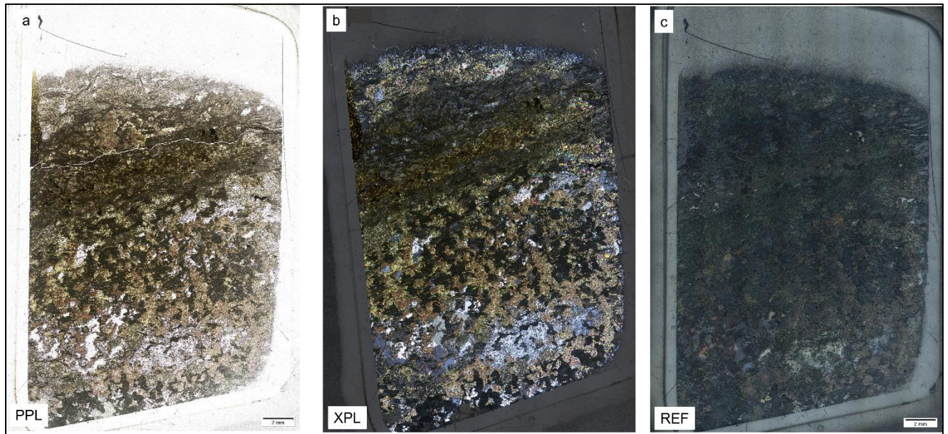
B25: Full-scan photomicrographs for Sample P740 in PPL (a), XPL (b), and REF (c). The sample represents a completely altered country rock. Epidote aggregates form the dominant silicate minerals enclosing dark brownish-black amphibole relics. Quartz grains appear to be overprinting epidote aggregates in places. Thin veins of quartz also cut across the sample. Minor grey Fe-oxides are also present. Sample size = 5 mm.
