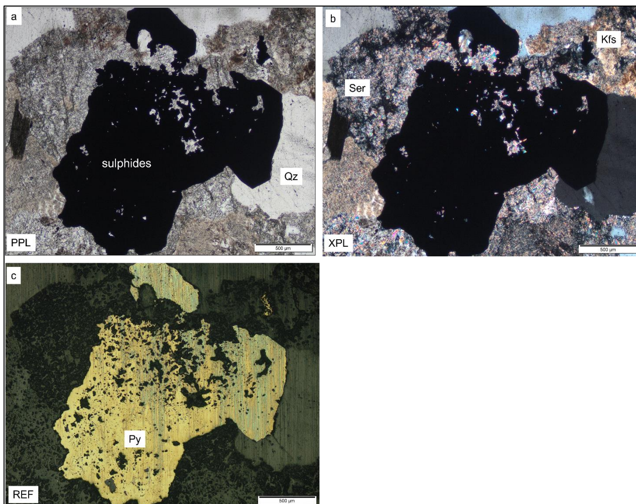
B35: (a-b) large, clear quartz grains invaded by interstitial fine-grained sericite. The opaque minerals corroded the sericite which occurs within it as irregular grains. The quartz has smooth to sharp grain boundaries with the opaque minerals but where it is associated with sericite the boundaries are irregular; (c) tarnished cluster of pyrite contains inclusions of sericite gangue (forming a porous texture on pyrite).
