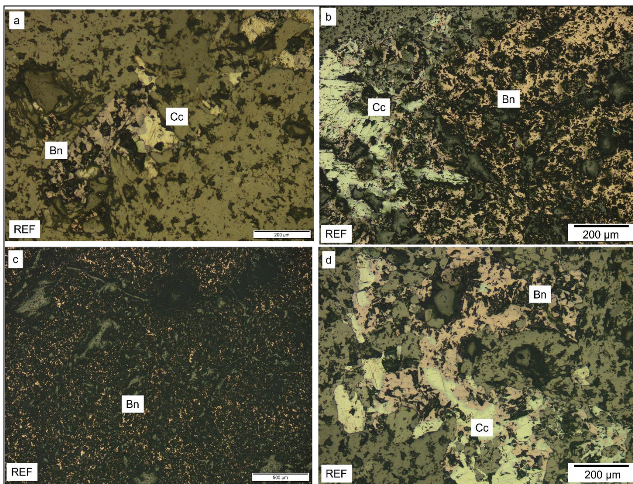
A21: (a) irregular tarnished bornite disseminations are partially being replaced by chalcocite; (b) coarse-grained tarnished bornite being replaced by chalcocite along the margins; (c) coarse-grained, massive, tarnished bornite contains elongate and angular fragments of quartz gangue; (d) interstitial tarnished bornite with chalcocite replacing it along the margins.
