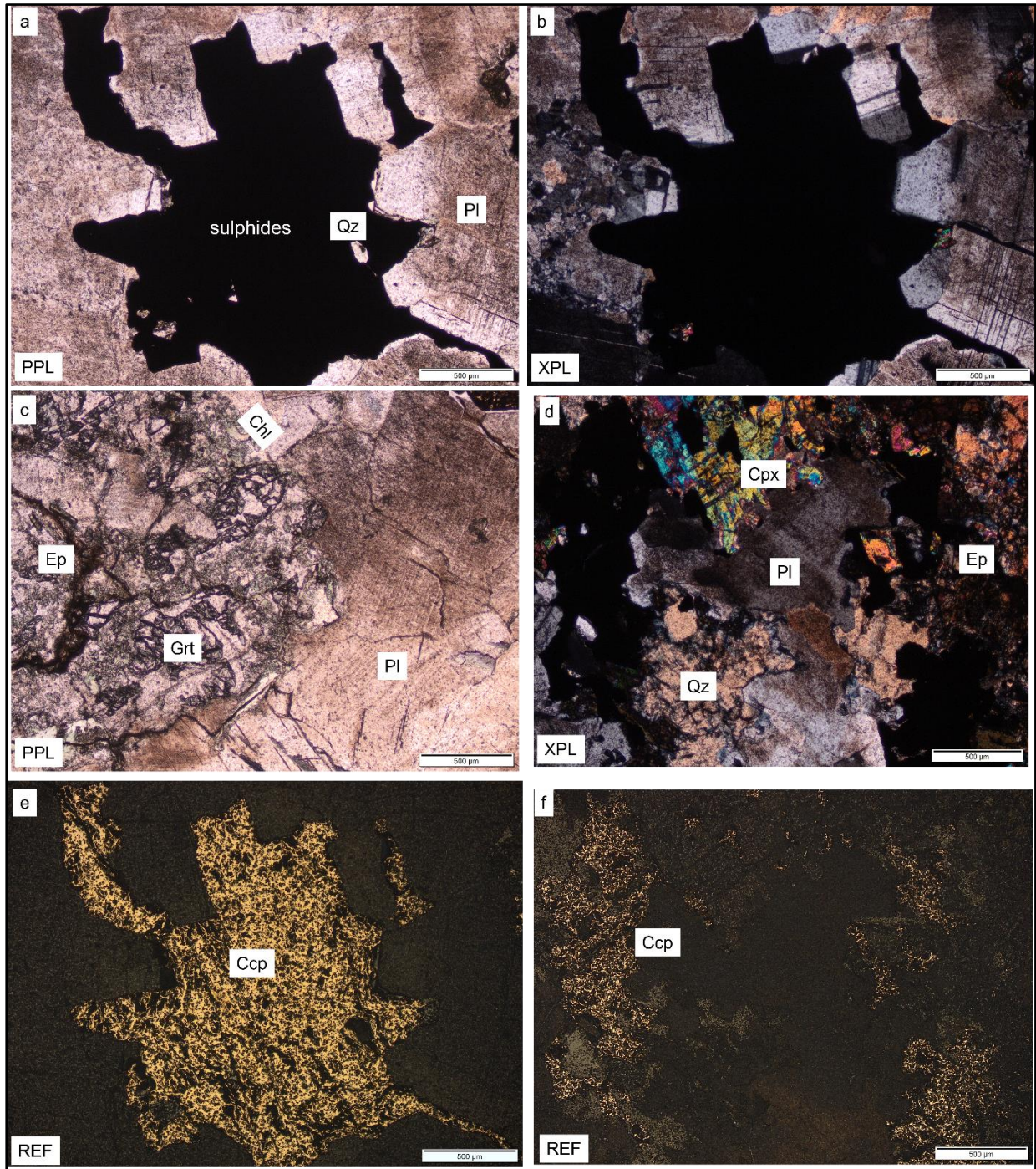
Figure 26: Photomicrograph showing: (a-b) interconnected plagioclase (Pl) grains enclosing interstitial opaque minerals; (c) a curvy epidote vein cuts fractured garnet (Grt) intergrown with plagioclase and quartz. The garnet is weakly altered by pale green chlorite in places; (d) brecciated, corroded, and partially altered clinopyroxene (Cpx) and plagioclase intergrown with quartz. Epidote (Ep) aggregates partially altered and replaced plagioclase and clinopyroxene; (e) interstitial chalcopyrite (Ccp) cementing plagioclase; (f) subhedral and anhedral disseminated chalcopyrite within corroded gangue minerals. Magnification scale = 500 µm.
