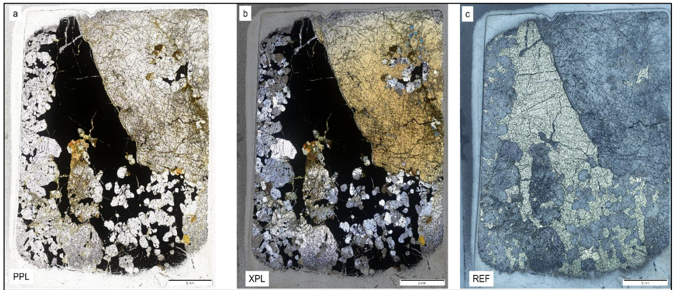
B6: Full-scan photomicrographs for Sample P579 in PPL (a), XPL (b), and REF (c). A large, fractured orthopyroxene and brecciated subhedral and subrounded grains of plagioclase enclose the opaque minerals. Some plagioclase grains occur within open spaces within fractured orthopyroxene. Dismembered plagioclase grains also occur within the opaque minerals. Pyrrhotite dominates the opaque minerals and contains small euhedral pyrite grains. Sample size = 5 mm.
