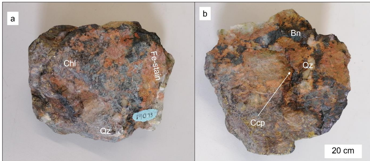
Figure 12: Sample 19073 comprises very fine-grained quartz (Qz) groundmass with subhedral, elongated, and irregular chlorite grains (Chl) in the groundmass. Quartz groundmass is heavily coated by orange-red iron oxide (Fe-stain). Interstitial bornite occurs within the quartz groundmass and is cut by chlorite in places. Some subhedral quartz grains occur within interstitial bornite. Fine-grained chalcopyrite grains (Ccp) are enclosed within the quartz groundmass. Other chalcopyrite (white arrow) is in contact with interstitial bornite (Bn).
