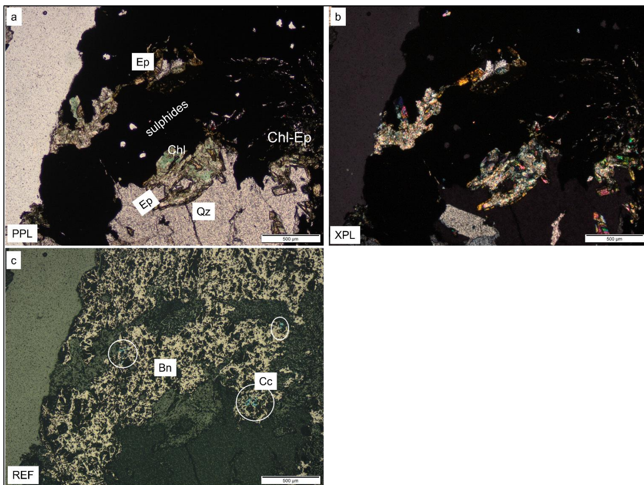
B3: (a-b) euhedral to subhedral epidote grains occur with interstitial chlorite along margins of subhedral quartz grains and within the opaque minerals. Epidote also appears as a rim around chlorite and fine-grained sericite (lower reflectance than epidote). Small irregular disintegrated chlorite-epidote grains occur within the opaque minerals. The quartz grains show undulate extinction; (c) minor tiny chalcocite grains are present within the massive tarnished bornite (white circles) and indicate incipient replacement of bornite by chalcocite.
