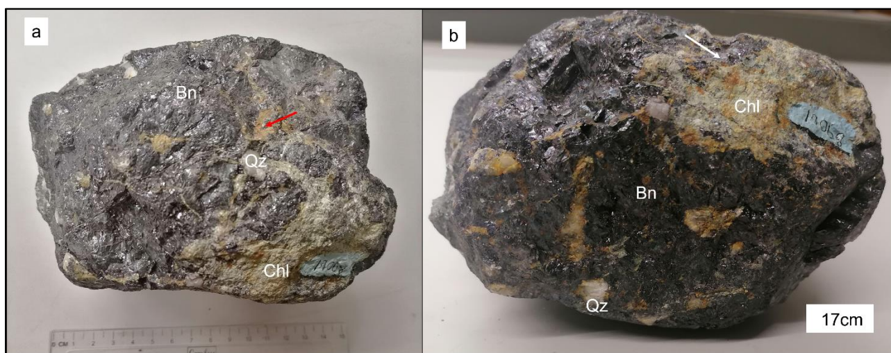
Figure 7: Sample 19068 showing massive bornite (Bn) enclosing discrete subhedral quartz (Qz) fragments and fine-grained irregular chlorite (Chl) veins. Fine-grained multiple chlorite veinlets cut through the massive bornite, whereas another fine-grained chlorite groundmass occurs around it. The chlorite has orange-red iron oxide stains (red arrow in a). White arrow in (b) indicates needle-like specularite between the massive bornite and fine-grained chlorite.
