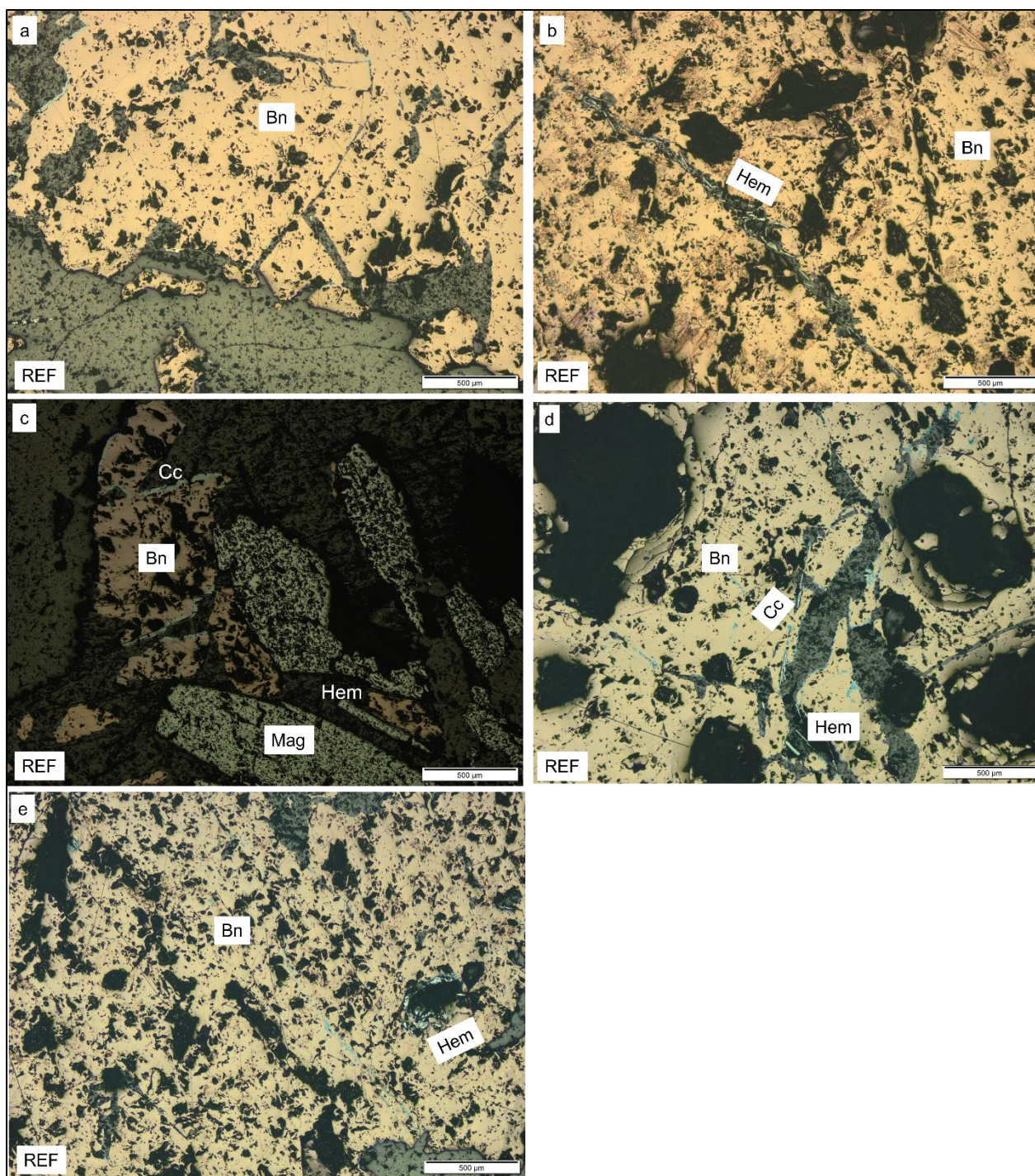
A4: (a-b) tarnished bornite is invaded and bordered by the chlorite gangue. Other isolated bornite grains occur within the surrounding quartz gangue. Small, bladed hematite grains occur within the chlorite vein cutting through the massive bornite. The change in colour of bornite could be due to oxidation or reflected light exposure effect because no chalcopyrite was observed in the hand specimen; (c) subhedral and tabular magnetite laths occur in association with bornite that is rimmed by chalcocite. A single hematite platelet occurs between the magnetite and is hosted by chlorite veins/interstitial gangue; (d) hematite platelets are embedded in chlorite gangue that cuts across the coarse-grained bornite. Irregular blue chalcocite occurs within the bornite and along the contact between bornite and chlorite. The black holes are polishing pits; (e) in other parts, coarse-grained massive bornite occurs with inclusions of subrounded and angular quartz and chlorite gangue. Hematite grains are present in fractures within the host bornite.
