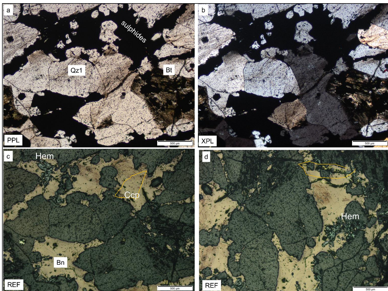
B23: (a-b) corroded quartz grains with irregular boundaries are intergrown with biotite (recognised by basal cleavage destroyed by corrosion). Quartz grains are brecciated, fractured, and dismembered whereby small fragments occur within the opaque minerals. Opaque minerals are enclosed within quartz and corrosion halos in biotite and quartz grains. Quartz grains exhibit undulose extinction; (c-d) the cleavage planes of biotite host hematite aggregates set within bornite. Hematite grains show overgrowth in places as small blades appear to be overgrowing from the fine ones. Bornite is enclosed by quartz and biotite as anhedral grains and cements the brecciated grains. Yellow chalcopyrite relics occur along the margins (orange polygons) of host bornite.
