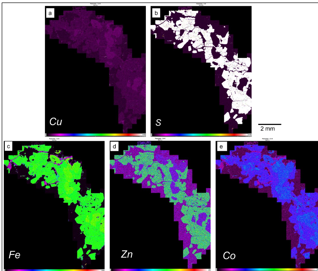
Figure 41: (a-e) Elemental maps showing concentrations of Cu=copper, S=sulphur, Fe=iron, Zn=zinc, and Co=cobalt in sample P817 iron sulphides and oxides.
