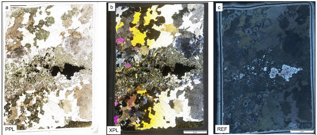
B28: Full-scan photomicrographs for Sample P744 in PPL (a), XPL (b), and REF (c). The sample is composed of a vein cutting through large, interconnected quartz grains. The vein contains micro-brecciated green epidote grains, which enclose the sulphides. Large, interconnected quartz grains are invaded by interstitial dusty brown (sericite) and dark green (chlorite). Sample size = 5 mm.
