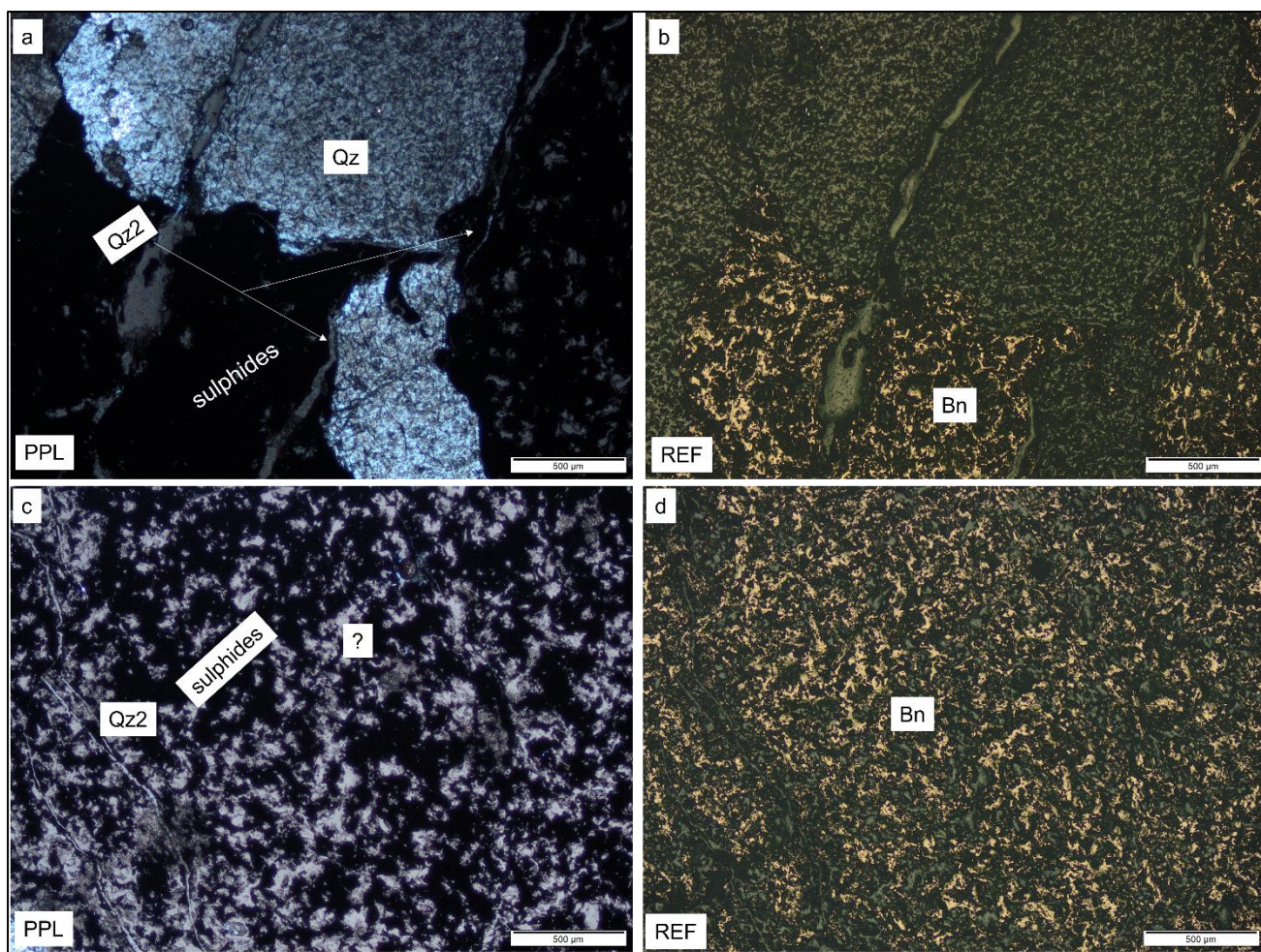
A22: (a) secondary veinlet of clear quartz cuts through the opaque minerals and large primary cloudy quartz; (b) coarse-grained tarnished bornite represent the opaque minerals. The large quartz encloses the bornite; (c) thin discontinuous secondary quartz veins cut through the opaque minerals. The micro-brecciated spots represent broken material during sample preparation; (d) coarse-grained, massive, tarnished bornite.
