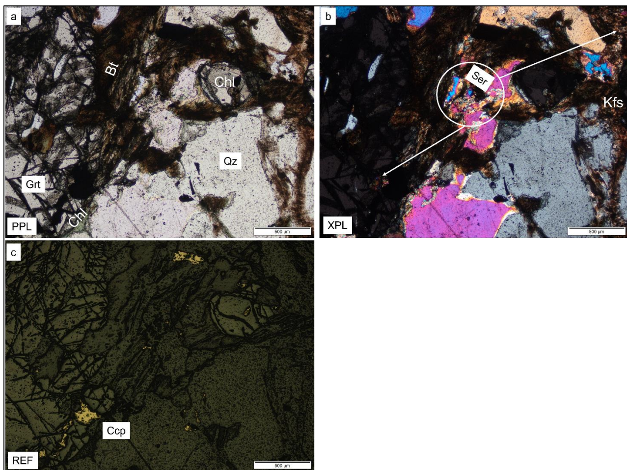
B37: (a-b) fractured garnet is intergrown with biotite and quartz. The garnet and biotite are partially altering into green chlorite. Quartz grains are stained or weakly fractured by K-feldspars. Fine-grained sericite is concentrated in an open space within the quartz grains (white circle), which also occurs within garnet fractures and alters K-feldspars along the margins (white arrows); (c) small chalcopyrite disseminations occur along garnet cracks and within quartz gangue.
