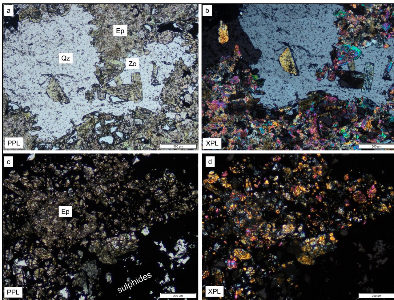
A20: (a-b) subhedral, large, secondary clear quartz grains are surrounded by brownish-yellow epidote aggregates which also occur as tabular to irregular grains overprinting quartz; (c) micro-brecciated fragments of brownish-yellow epidote occur within the opaque minerals; (d) high birefringence of brecciated epidote. The opaque minerals are disseminated between the aggregates.
