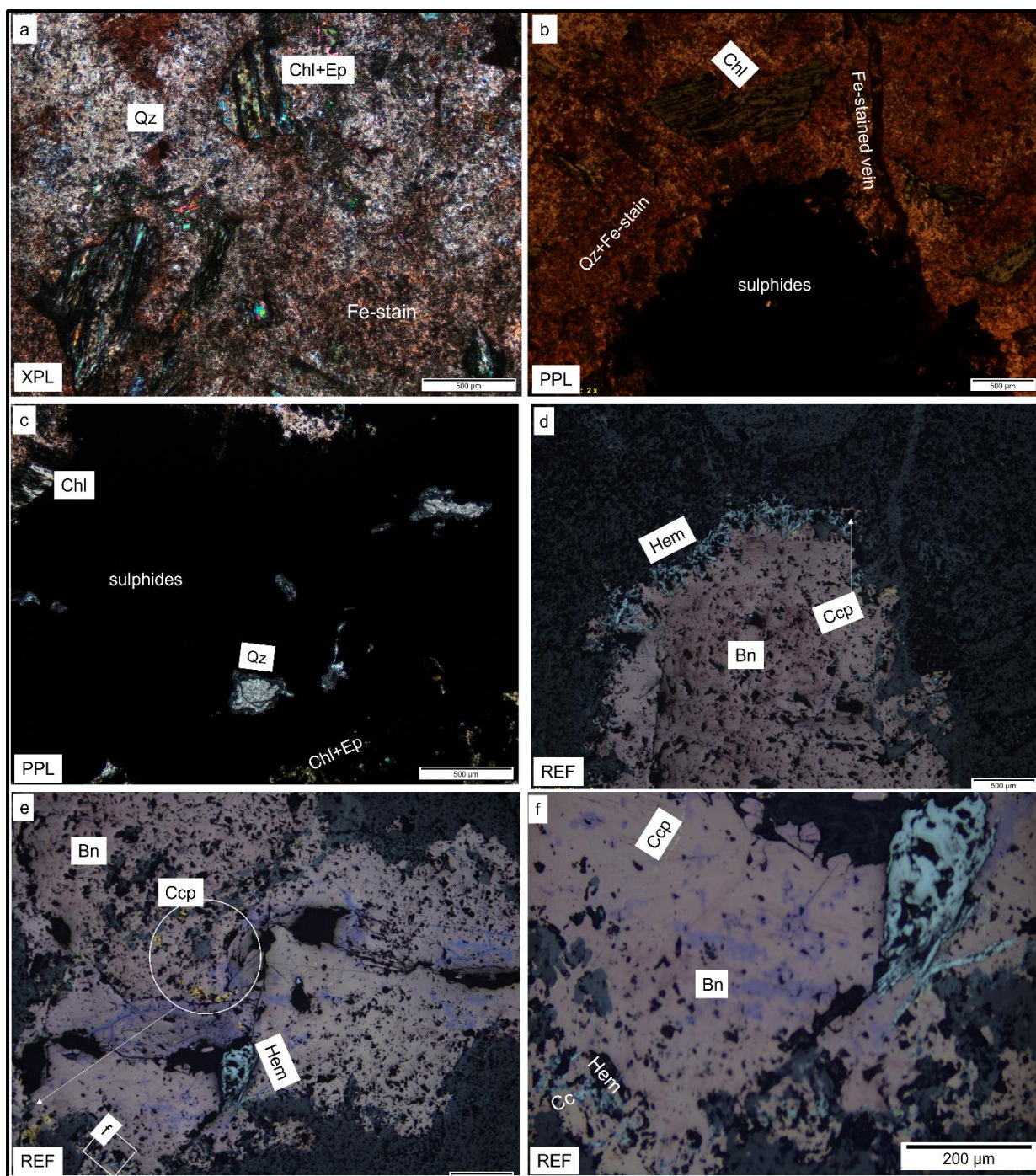
Figure 13: Photomicrographs showing: (a) chlorite (Chl) grains within Fe-stained cryptocrystalline quartz (Qz) are partially altered into epidote (Ep) along cleavage planes; (b) Fe-stained vein cut through cryptocrystalline groundmass and opaque minerals. Irregular grains of green chlorite grains within cryptocrystalline quartz; (c) subhedral quartz and irregular chlorite-epidote veinlets within the opaque minerals; (d) subhedral coarse-grained bornite (Bn) in contact with disseminated chalcopyrite. Hematite platelets rim the bornite along margins; (e) bornite with minor chalcopyrite (Ccp) flame-like relics within bornite. Subhedral hematite developing into elongate blades (light bluish-green) in a fracture in host bornite; (f) tiny blades of hematite and chalcocite along minor fractures of bornite under high-magnification (white square in Fig. 13e). Magnification scale = 500 µm and 200 µm.
