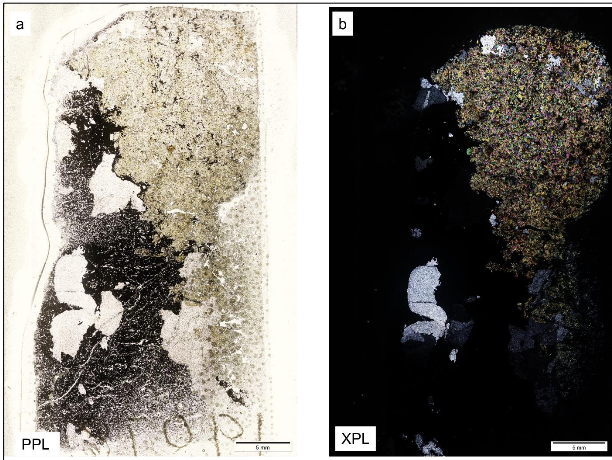
A18: Full-scan photomicrographs for Sample 19078 in PPL and XPL: (a) brownish-yellow granular aggregates of epidote surround the opaque minerals. Subhedral and angular quartz grains occur within the opaque minerals. Other opaque minerals are disseminated within the granular aggregates; (b) epidote granular aggregates show high reflectance in XPL and angular greyish-white quartz appears to occur within and in contact with epidote aggregates in places. Sample size = 5 mm.
