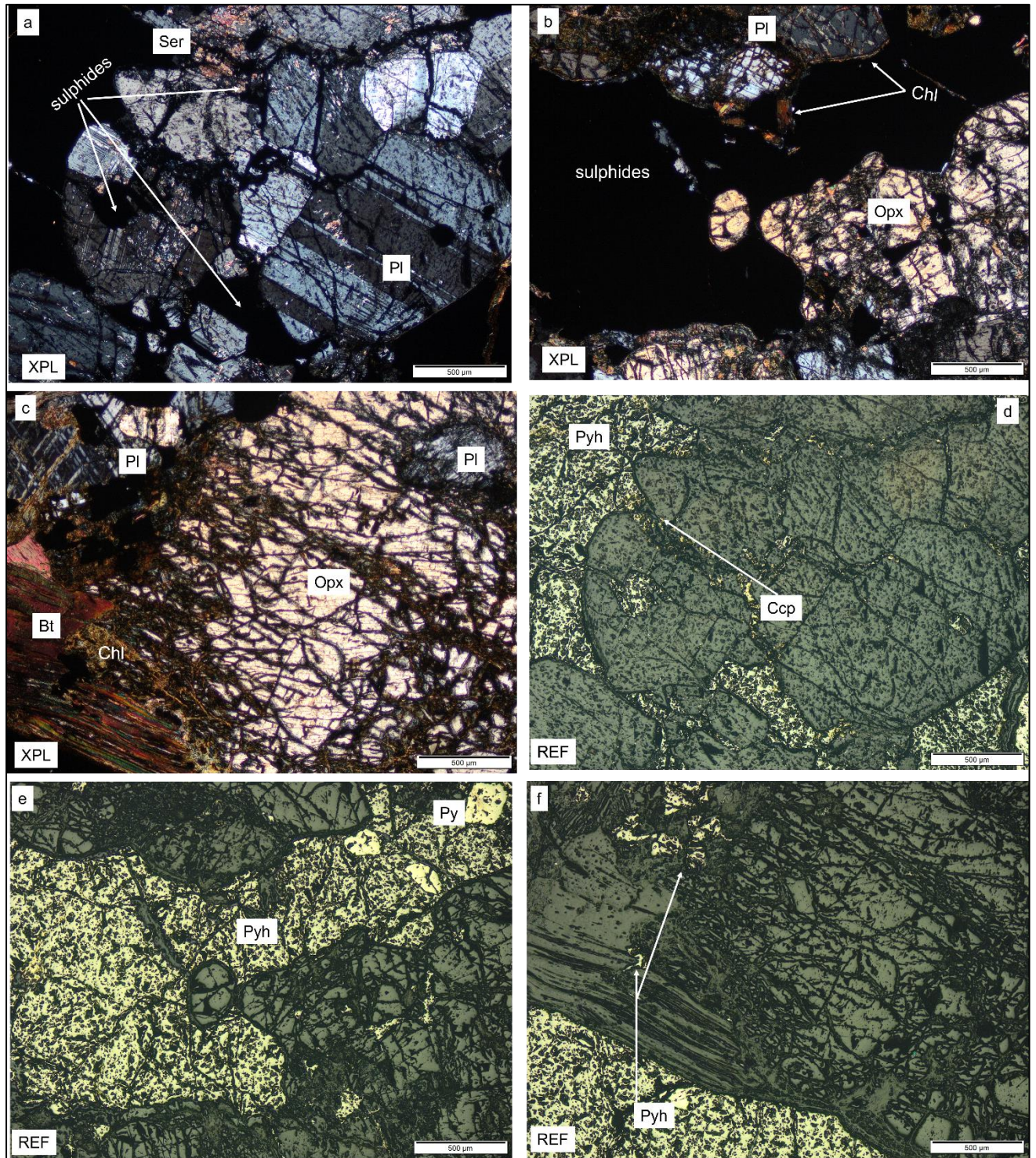
Figure 19: Photomicrographs showing: (a) albitised plagioclase (Pl) partially altered by fine-grained sericite (Ser); (b-c) fractured orthopyroxene (Opx) and plagioclase fragments associated with chloritic (Chl) networks veins filling the fractures, rimming opx and pl, and cementing and overprinting some pl fragments. Some veins occur within the opaque minerals; (d) anhedral pyrrhotite (Pyh) cements albitised plagioclase fragments and is associated with anhedral chalcopyrite (Ccp, white arrow) encroaching onto pyh; (e) massive, granular, interstitial pyh intergrown with individual euhedral and subhedral pyrite (Py) grains; (f) disseminated subhedral and anhedral pyrrhotite filling corroded halos within albitised plagioclase, chloritised biotite and orthopyroxene. Magnification scale = 500 µm.
