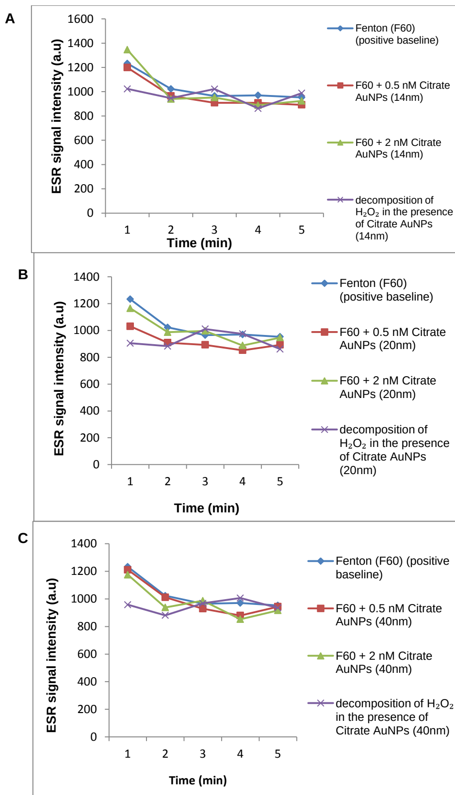
Figure 5.18: ESR signal intensity showing the effect of (A) 14nm, (B) 20nm and (C) 40nm citrate stabilized AuNPs on the generation of \cdot OH at pH 4.6.
