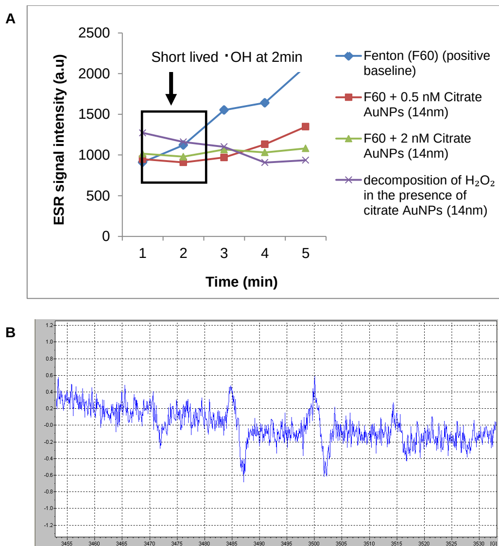
Figure 5.8: ESR signal intensity in the reaction of hydrogen peroxide and 14nm citrate stabilized AuNPs. F60 represented a positive baseline in reaction medium containing hydrogen peroxide and \text{Fe}^{2+} . AuNPs were added at different concentrations to the F60 reaction (red and green plot). AuNPs (in the absence of \text{Fe}^{2+} ) were used to catalyze the decomposition of hydrogen peroxide (purple plot). The ESR scan shows the DMPO·OH obtained in the reaction of \text{H}_2\text{O}_2 and citrate AuNPs (pH 3.6) at about 2 minutes after initiating the reaction.
