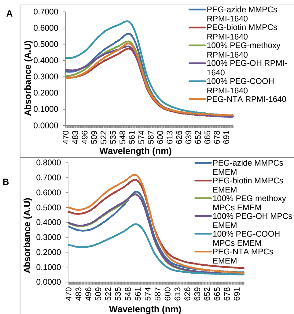
Figure 2.6: UV-Vis spectra of 14nm PEG-azide MMPCs, PEG-biotin MMPCs, PEG-NTA MMPCs, PEG-OH MPCs, PEG-OCH 3 MPCs and PEG-COOH MPCs in RPMI-1640 and EMEM growth medium.
