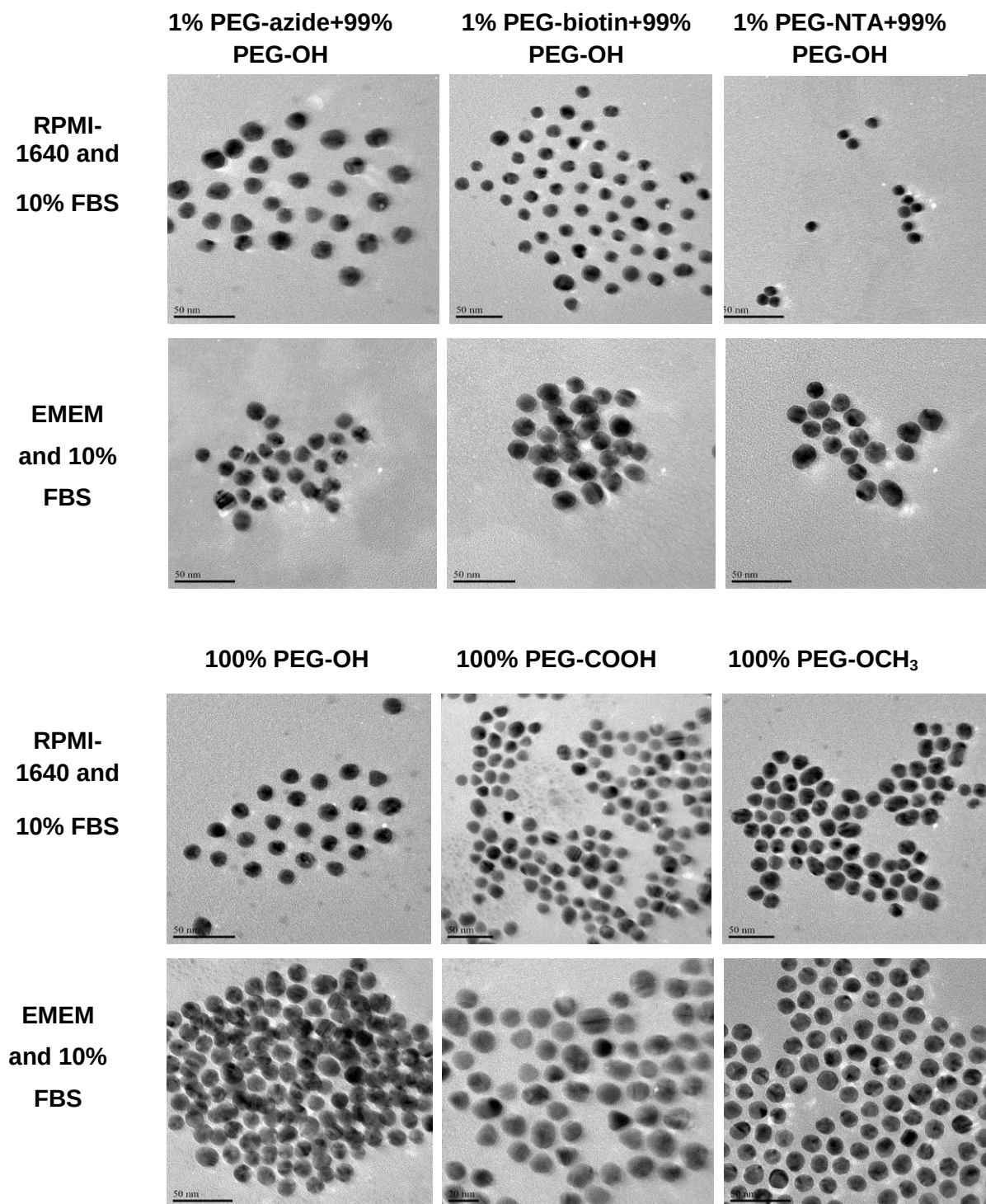
Figure 2.4: TEM micrographs of PEG-azide MMPCs, PEG-biotin MMPCs, PEG-NTA MMPCs, PEG-OH MPCs, PEG-OCH 3 MPCs and PEG-COOH MPCs in RPMI-1640 and EMEM growth medium.
