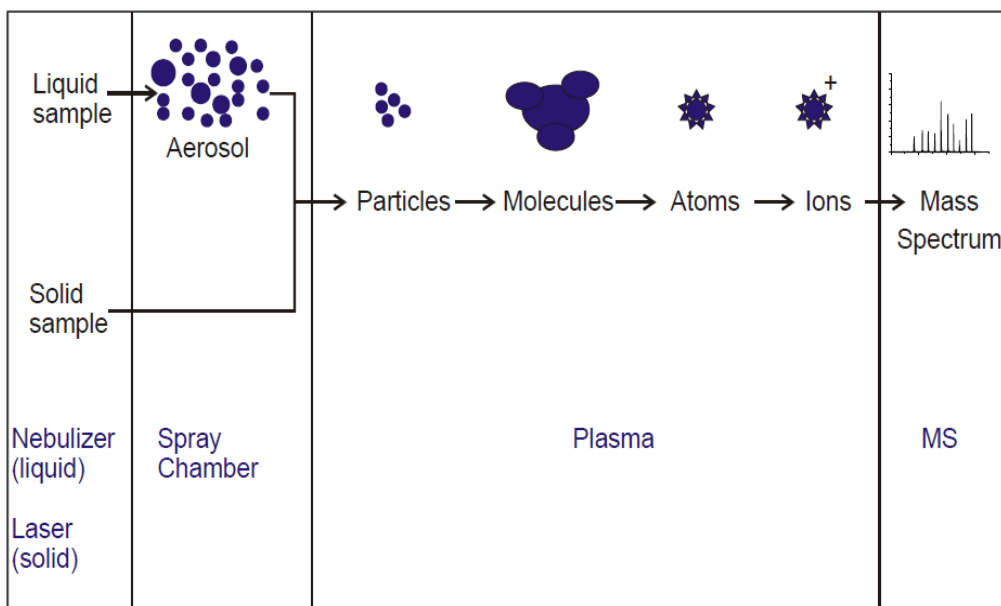
Figure 3.1: Schematic diagram of ICP- MS sample introduction, ion formation and analysis. (Ammann, 2007).
