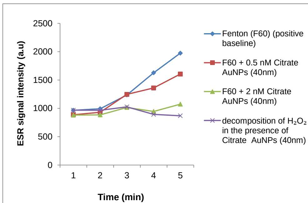
Figure 5.10: ESR signal intensity in the reaction of hydrogen peroxide and 40nm citrate stabilized AuNPs. AuNPs were added at different concentration in the presence of hydrogen peroxide and \text{Fe}^{2+} . AuNPs (in the absence of \text{Fe}^{2+} ) were used to catalyze the decomposition of hydrogen peroxide at pH 3.6.
