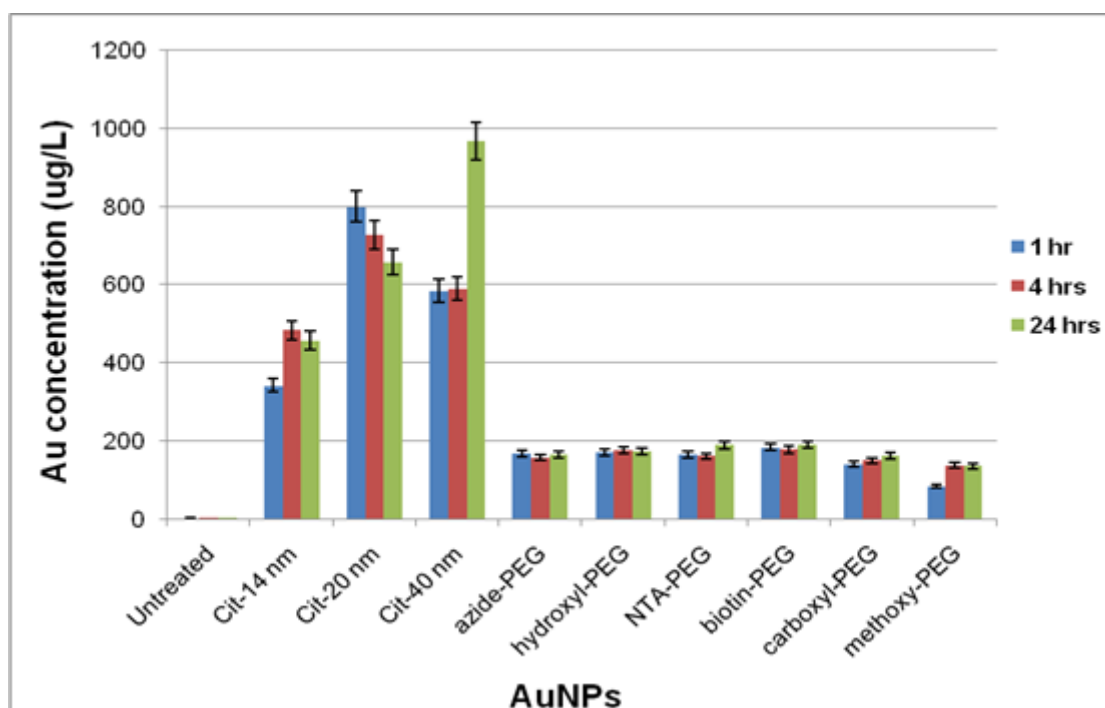
Figure 3.15: Quantification by ICP-MS showing the concentrations (in \mu\text{g/L} ) of Au in HepG2 cells after 1, 4 and 24 hrs incubation with citrate stabilized and PEG-coated gold nanoparticles.
