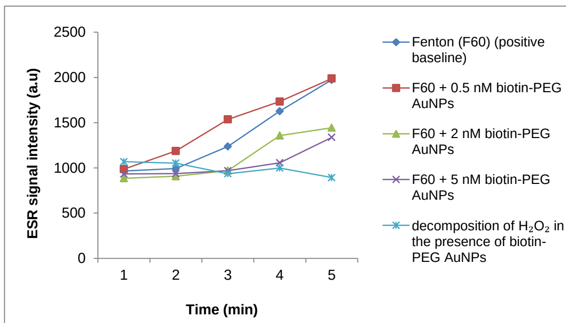
Figure 5.14: ESR signal intensity in the reaction of hydrogen peroxide and biotin-PEG AuNPs. The biotin-PEG AuNPs were added at different concentration). AuNPs were assessed for their ability used to catalyze the decomposition of hydrogen peroxide in the absence of \text{Fe}^{2+} .
