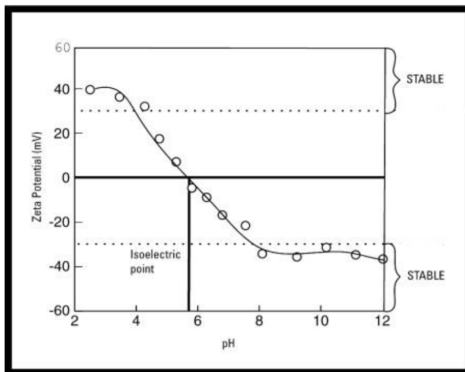
Figure 2.1: A plot of zeta potential vs. pH showing values where nanoparticle would be expected to be stable (downloaded from http://www.silver-colloids.com , accessed 25 May 2012).
