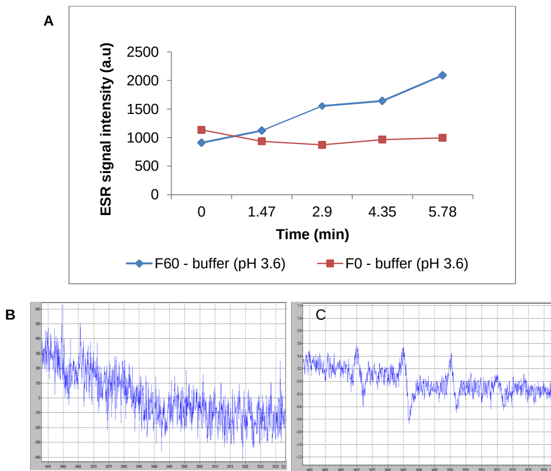
Figure 5.7: ESR signal intensity of \text{H}_2\text{O}_2 decomposition in the presence of \text{Fe}^{2+} (F60). (F0) represent the negative baseline without \text{Fe}^{2+} . The ESR spectra of the reactions F0 (b) and F60 (c) are shown.
