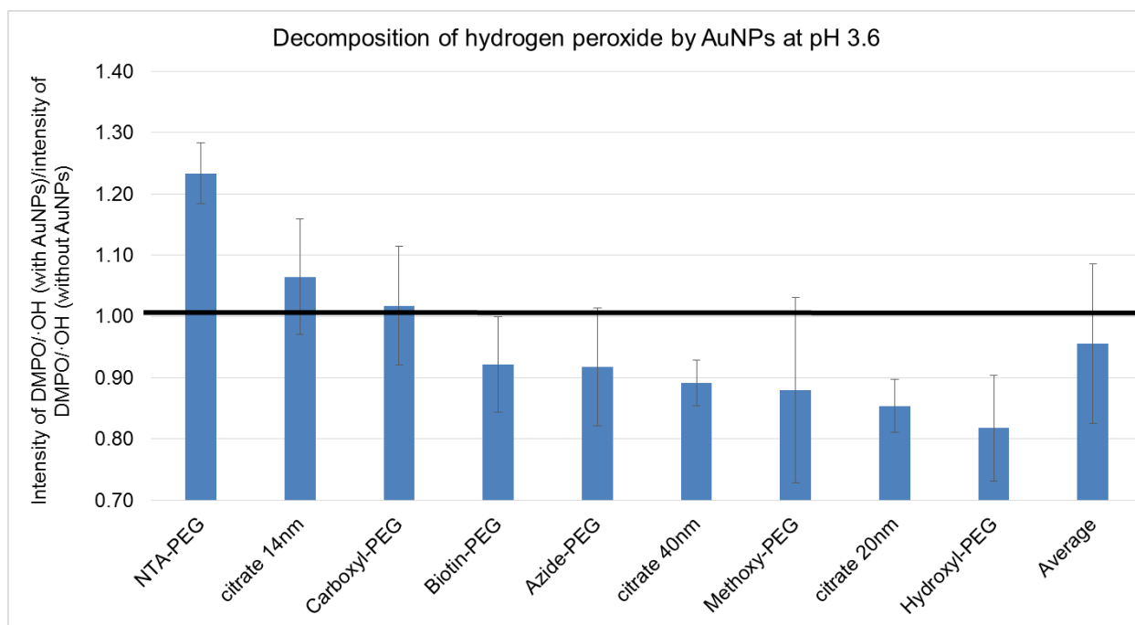
Figure 5.17: Decomposition of hydrogen peroxide by AuNPs at pH 3.6. The data represents each particle displacement ratio from the negative baseline
