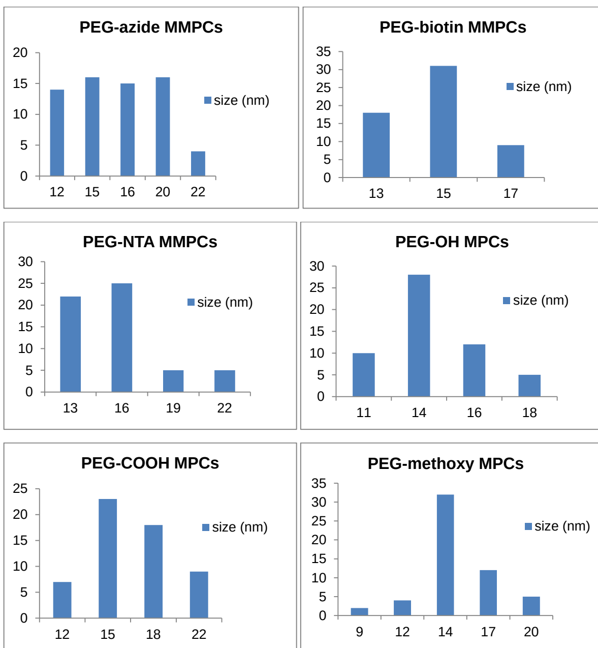
Figure 2.5 Particle size distributions of PEG-azide MMPCs, PEG-biotin MMPCs, PEG-NTA MMPCs, PEG-OH MPCs, PEG-OCH 3 MPCs and PEG-COOH MPCs.
