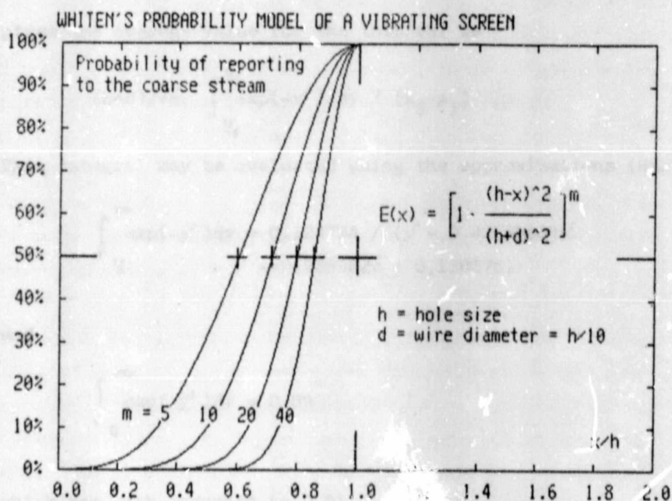
Figure 4.3 Efficiency curves obtained using Whiten's probability model
