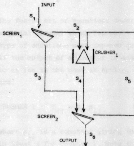
Figure 5.1 Example plant-circuit diagram
