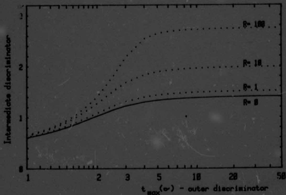
Fig. 6.6b Discriminator positions in two channel analysis for minimum variance in R
