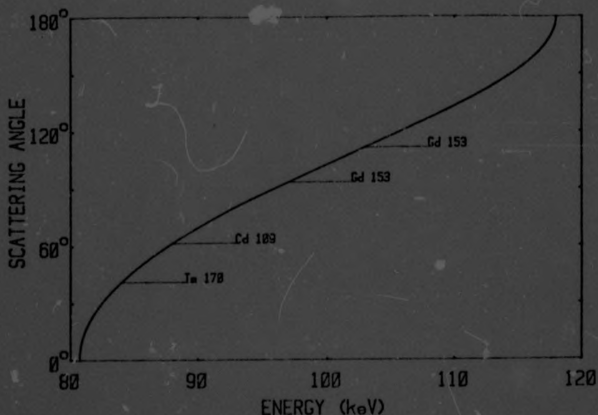
Fig. 3.2 Angle required in incoherent scattering to reduce energy of primary photon to 81 keV
