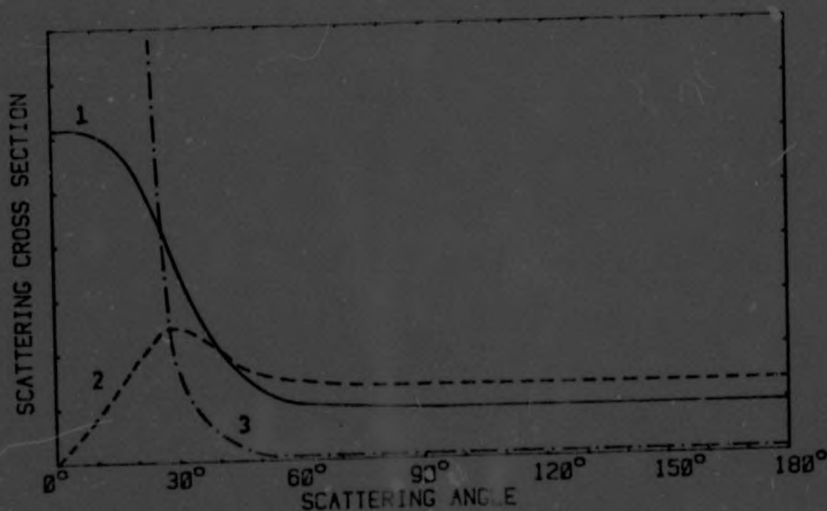
4.2 Shape of differential cross sections per unit solid angle for scattering of 88 keV photons from iron. (1)-Compton free electrons, (2)-incoherent and (3)-coherent (after Davisson, 1963).
