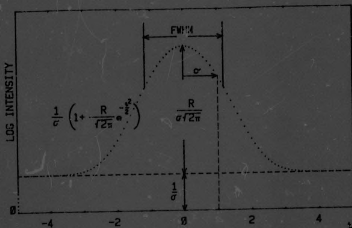
Fig. 6.1 Normalized Gaussian peak and background
