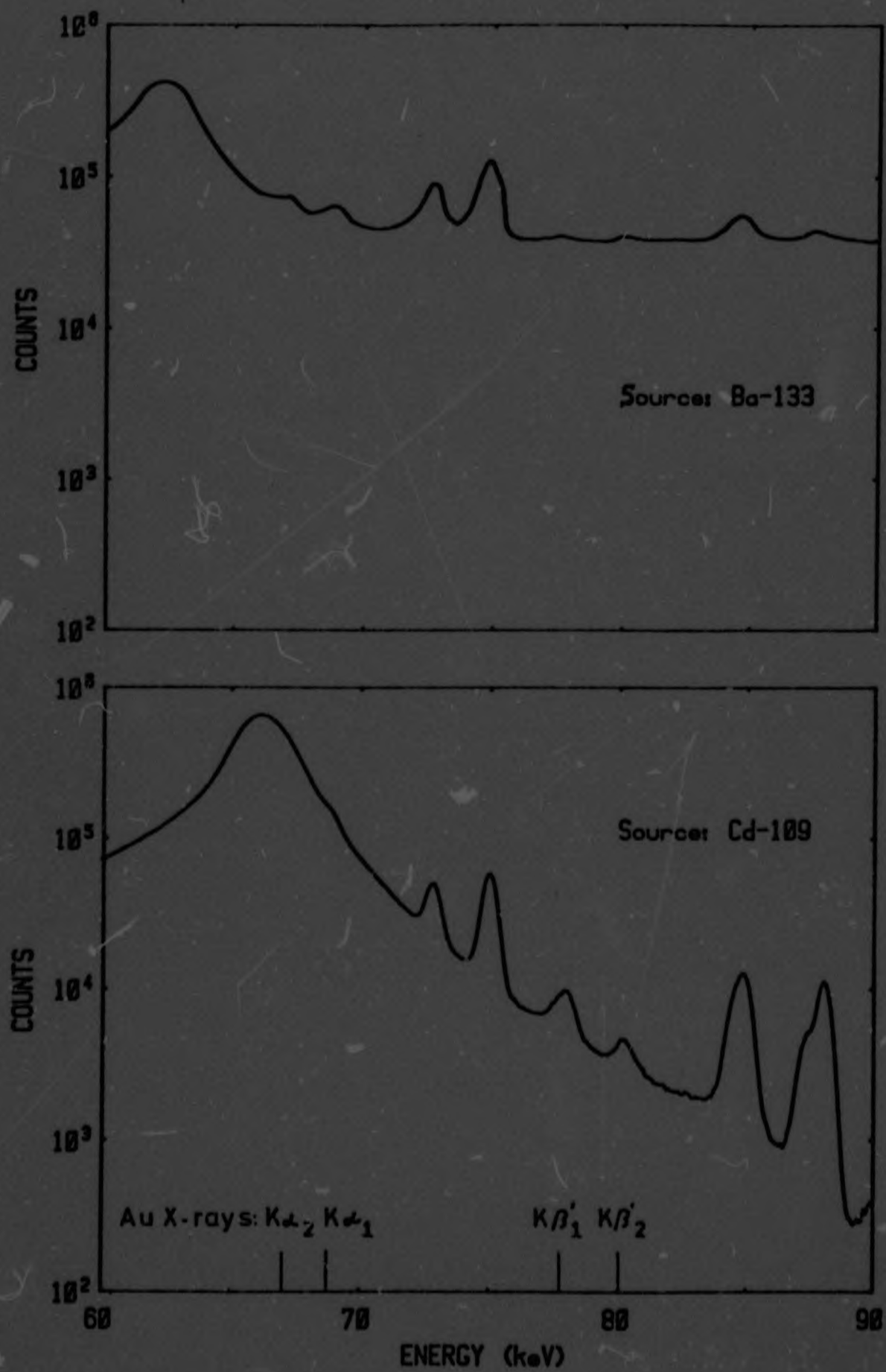
Fig. 7.1 Fluorescence spectra of a standard gold ore sample
