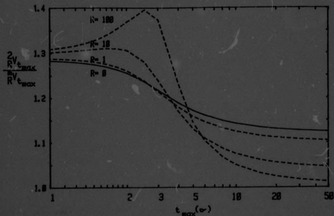
Fig. 6.6a Minimum two channel variance in R (divided by multichannel variance)
