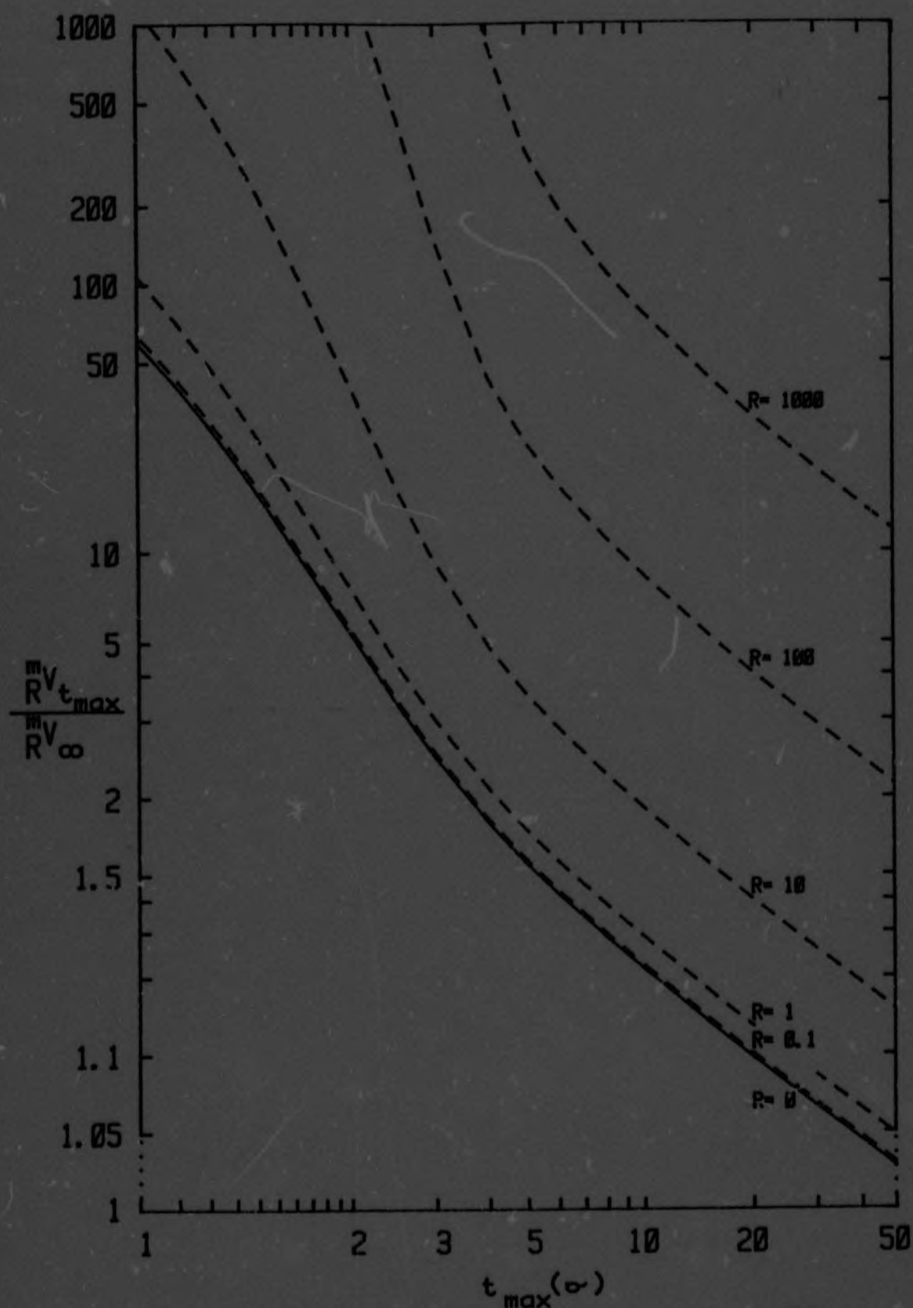
Fig. 6.5 Standardized multichannel variance mv_{t_{max}} relative to mv_{\infty}
