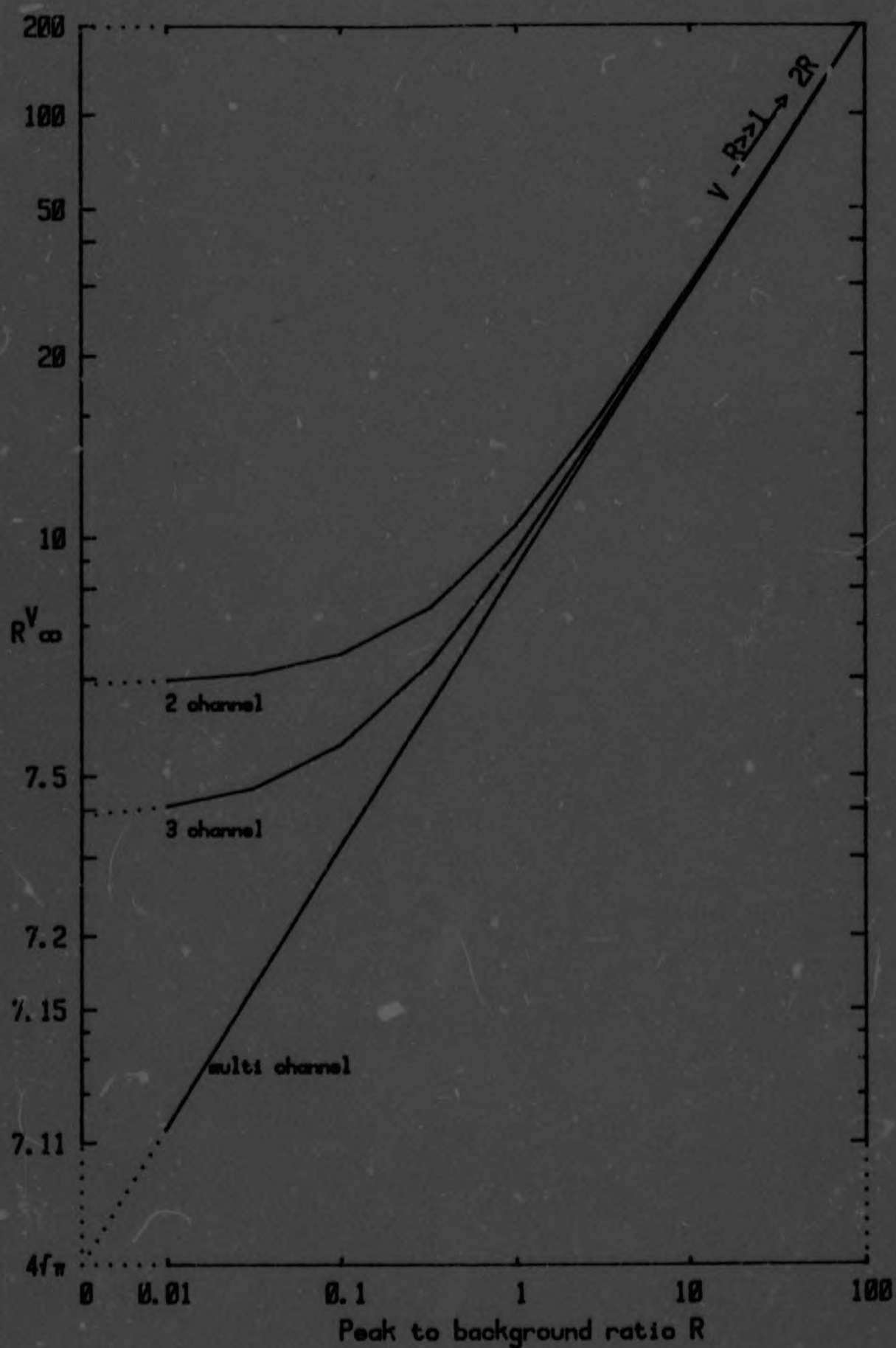
Fig. 6.4 Standardized background variances of R ; background region unlimited
