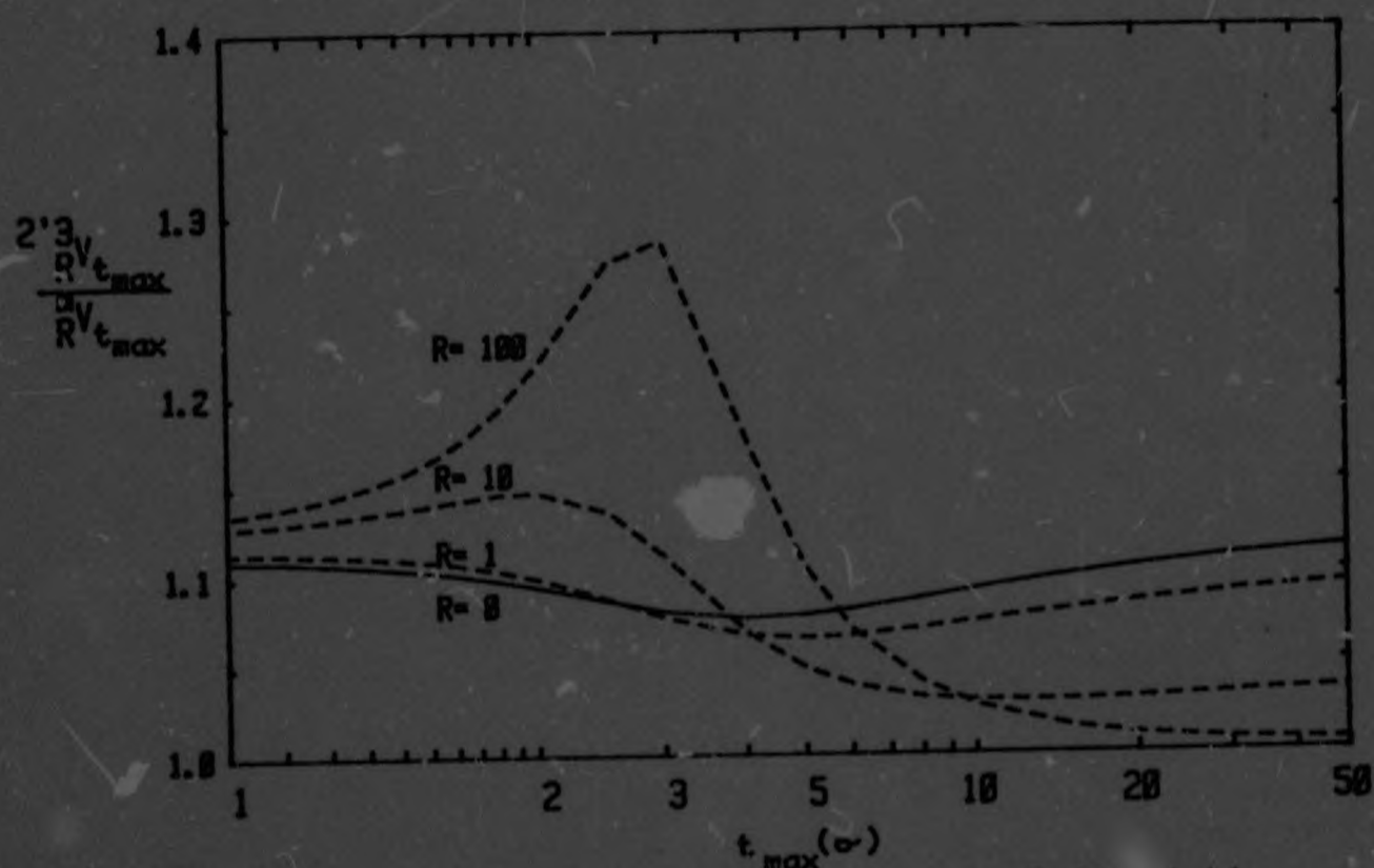
Fig. 6.7a Minimum pseudo two channel variance in R (divided by multichannel variance)
