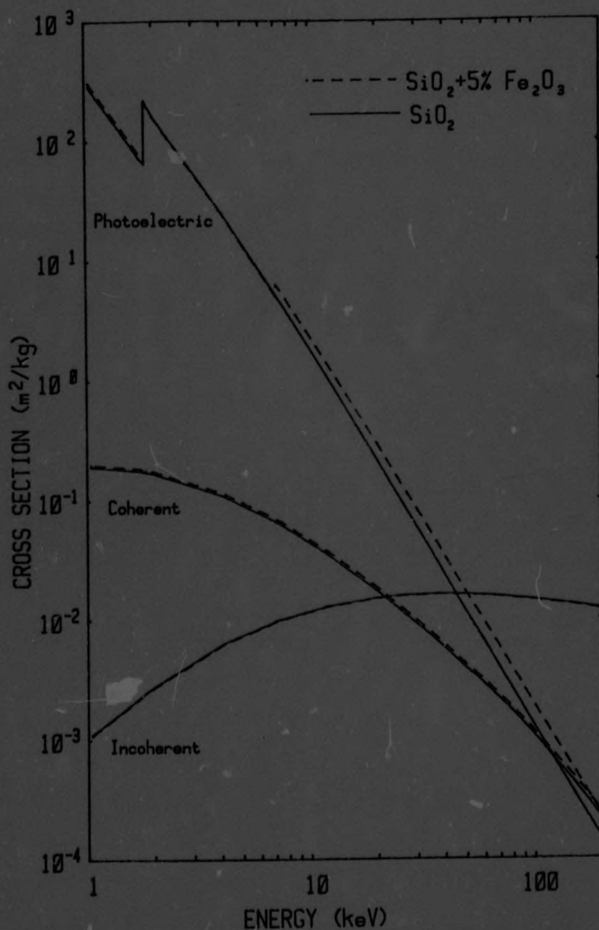
Fig. 4.2 Photon interaction data for 'rock'
