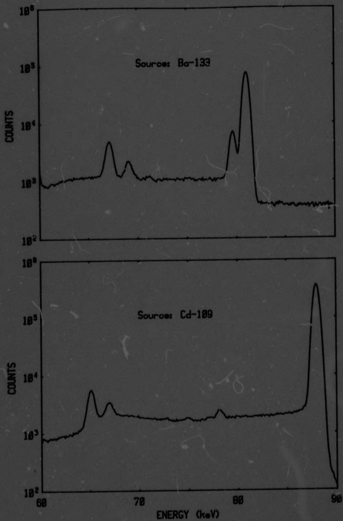
Fig. 3.1 Spectra of sources for gold K X-ray fluorescence
