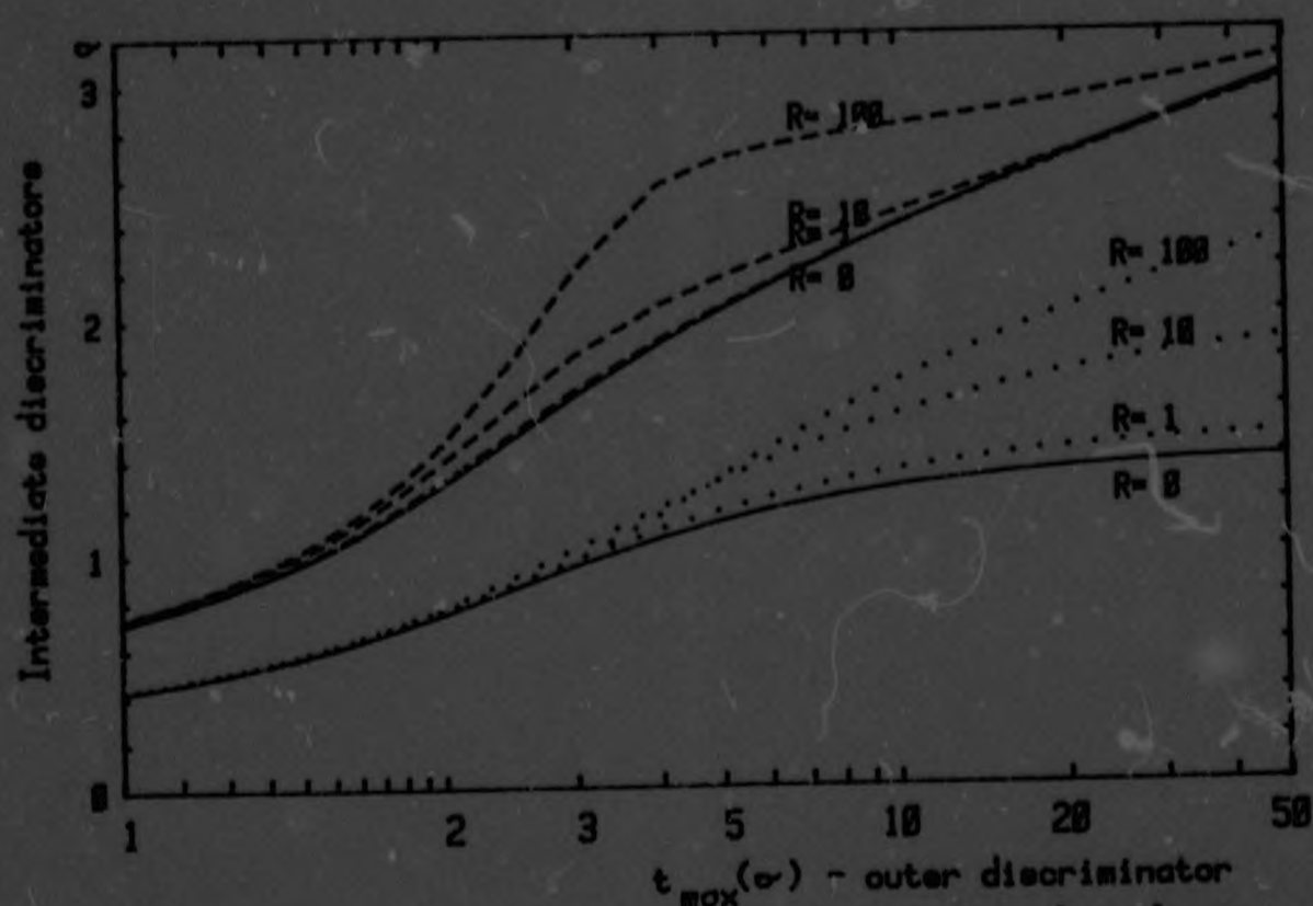
Fig. 6.7a Minimum pseudo two channel variance in R (divided by multichannel variance)
