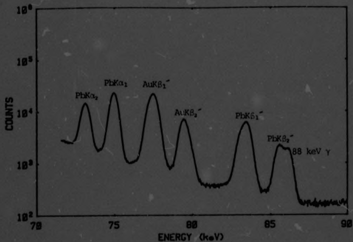
Fig. 7.2 Fluorescence spectra of pure gold and lead
