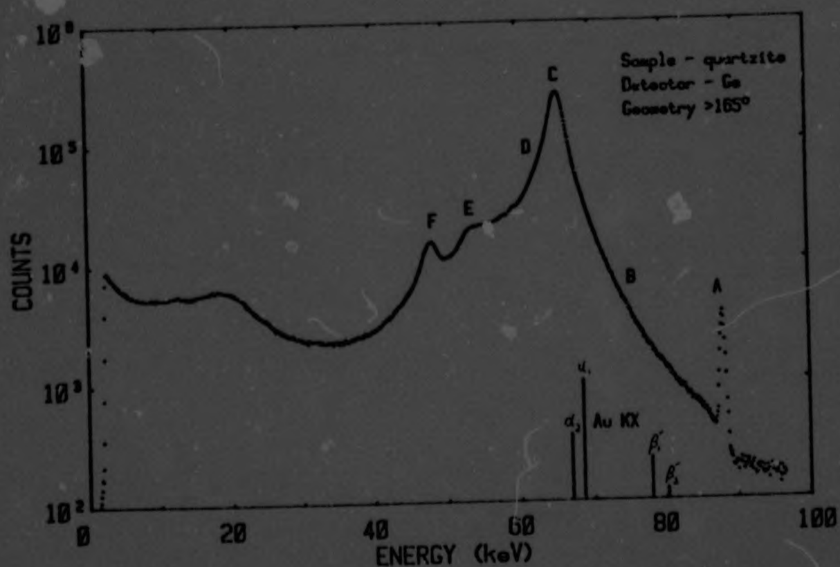
Fig. 4.1 Cd 109 backscatter spectrum from blank rock
