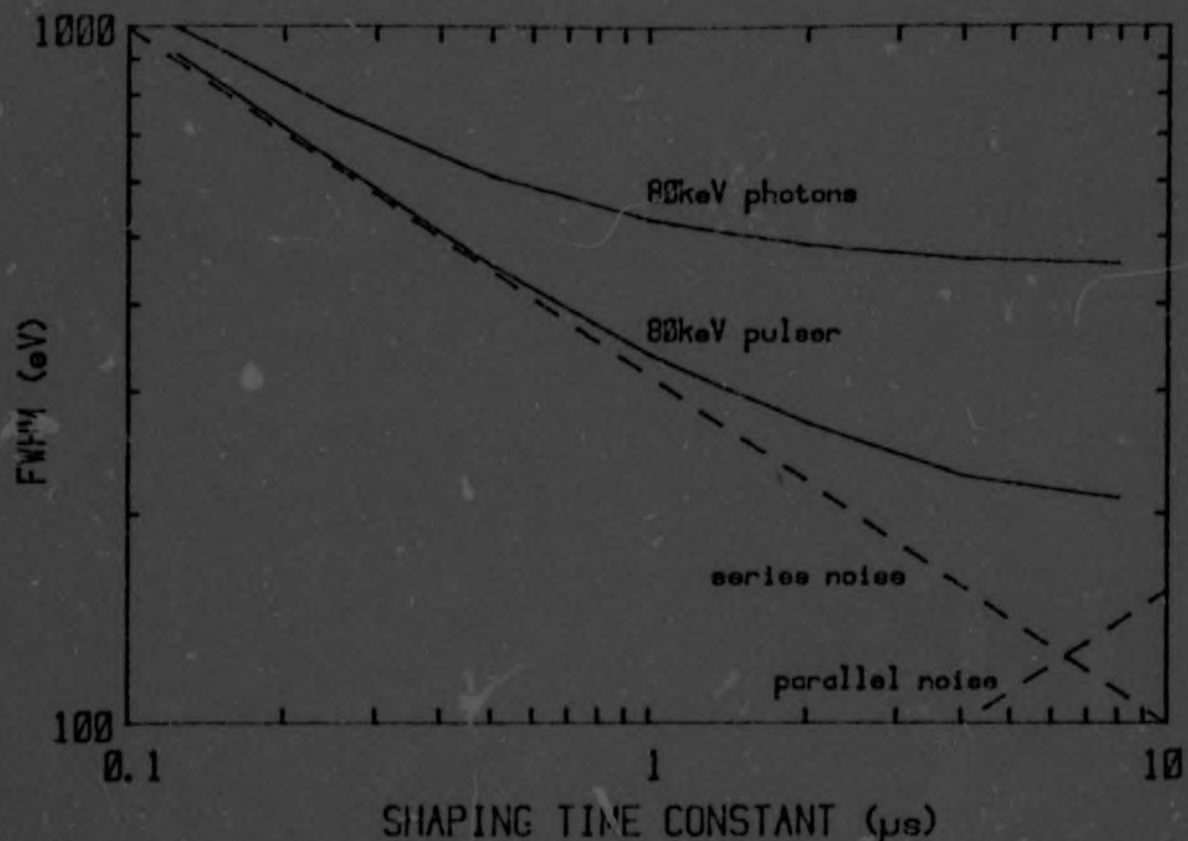
Fig. 5.2 Energy resolution of a 200\text{mm}^2 \times 7\text{mm} Ge detector
