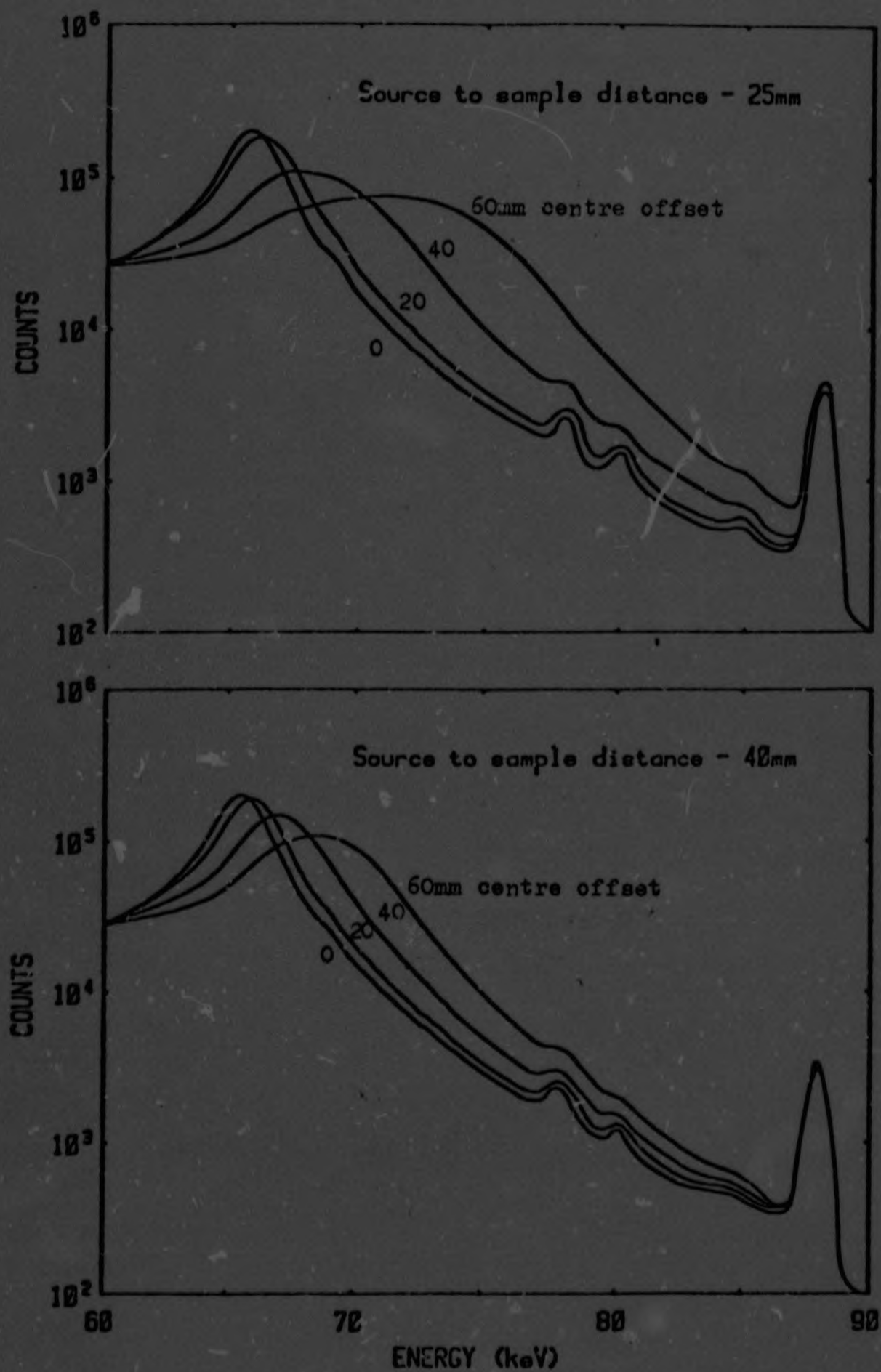
Fig. 4.5 Backscatter spectra from large sample of standard ore for different measuring geometries.
