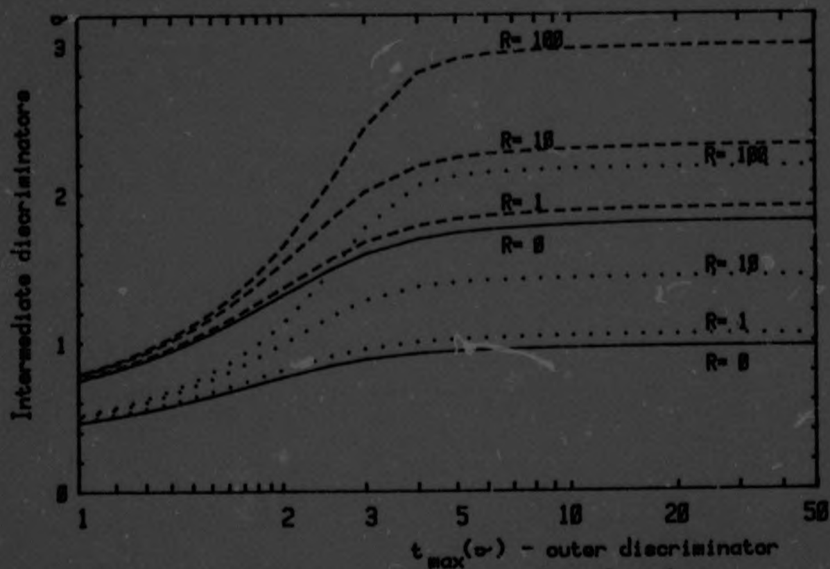
Fig. 6.8b Discriminator positions in three channel analysis for minimum variance in R
