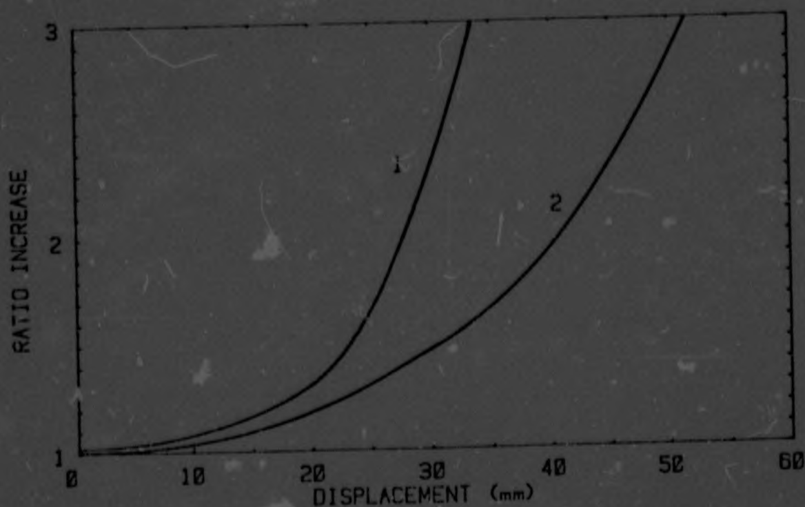
Fig. 4.6 Increase in backscatter intensity at 80keV from peripheral sources relative to that from a central source. Probe-to-sample distance: (1)-25mm, (2)-40mm
