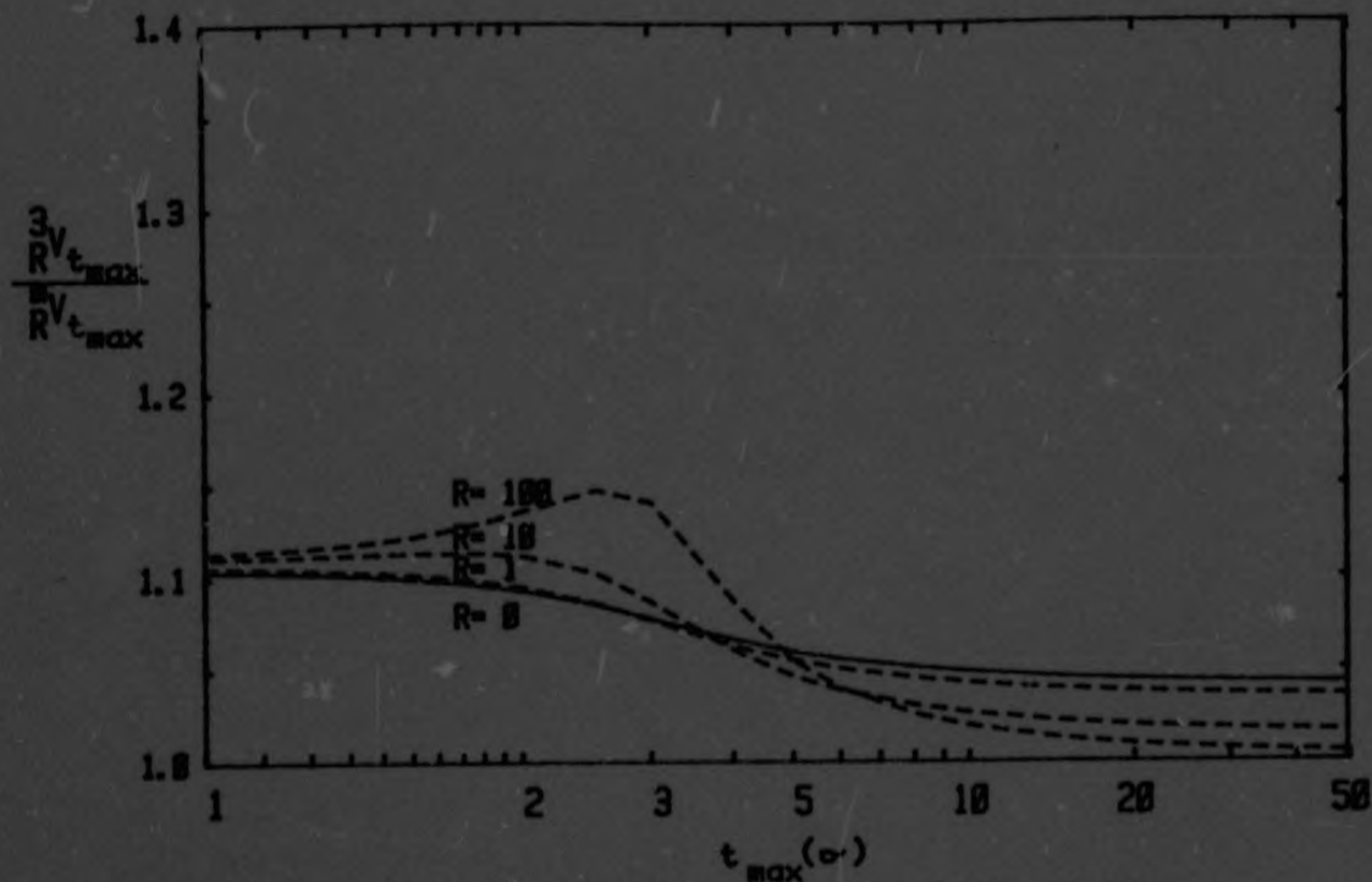
Fig. 6.8a Minimum three channel variance in R (divided by multichannel variance)
