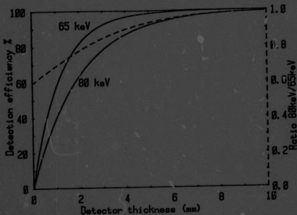
Fig. 5.1 Linear detection efficiencies and their ratio vs. Ge detector thickness
