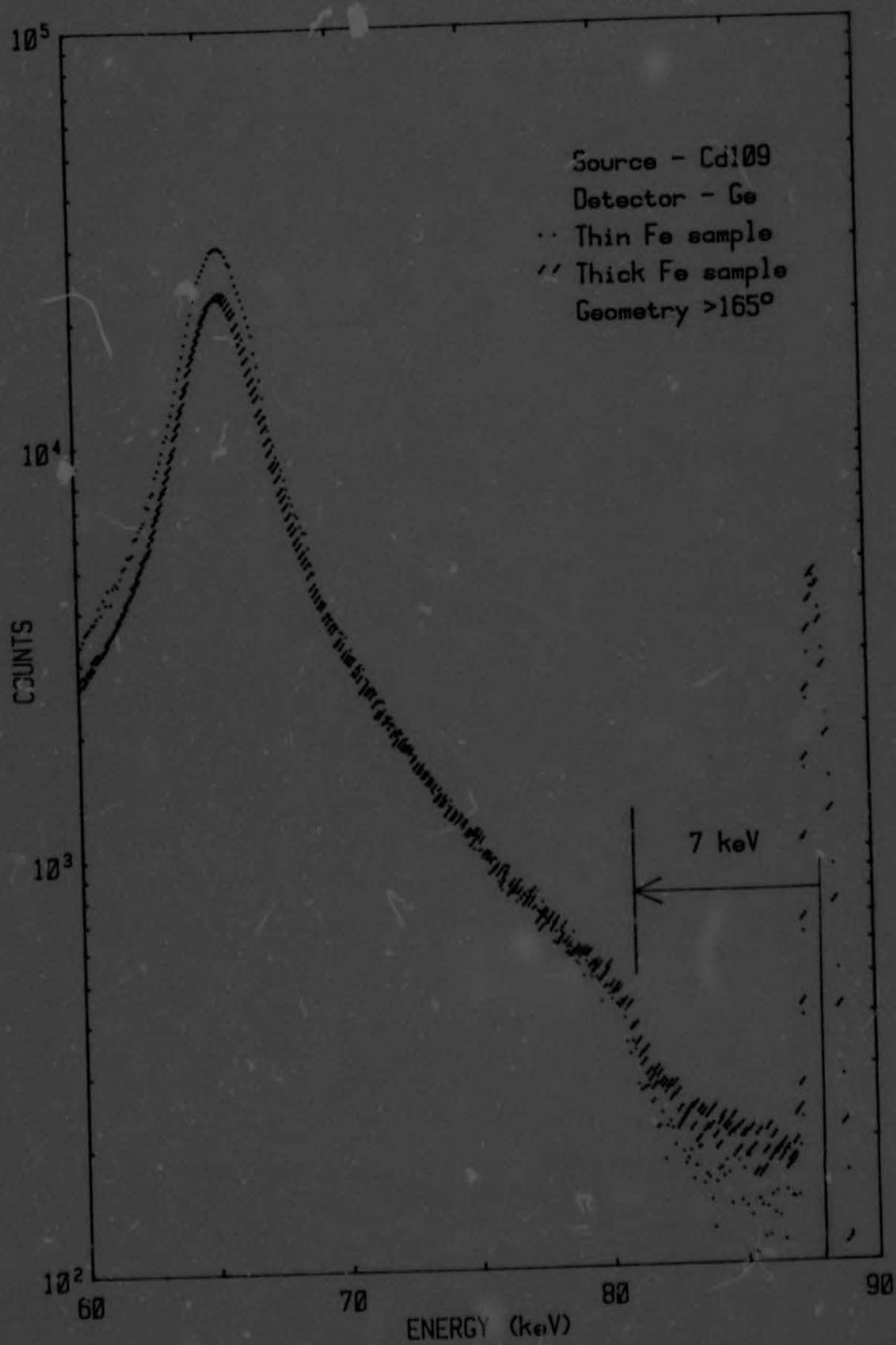
Fig. 4.4 Backscatter spectra from iron samples
