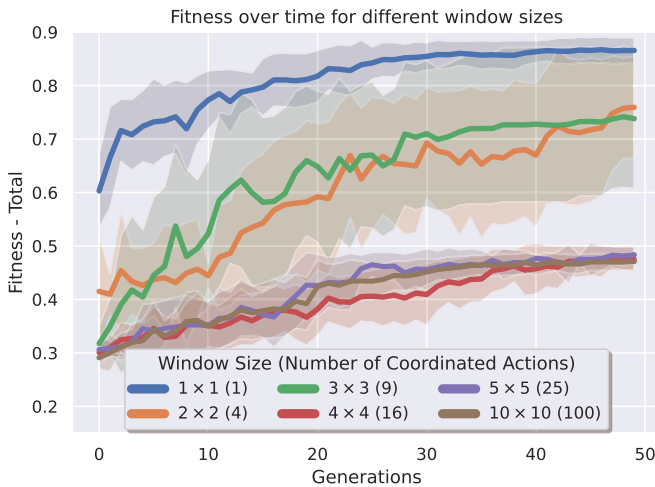
Fig. 5. Plot showing the maximum fitness value in the population (i.e., how “correct” the generated levels are) over time for different window sizes (i.e., how many coordinated actions are required to build the lower-level structures). The mean over 10 seeds is shown, with standard deviation shaded.
