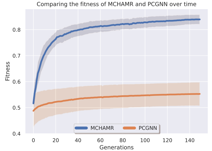
Fig. 6. Illustrating the fitness over time on 20 random town layouts for MCHAMR (consisting of the composed town and house generators) compared to the flat, noncompositional method, corresponding to vanilla PCGNN. We first compute the average fitness across 10 seeds and plot the mean and standard deviation over the 20 layouts.
