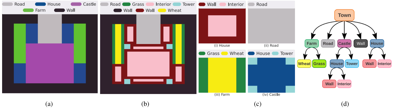
Fig. 1. Example of MCHAMR, with the (a) high-level and (b) composed towns and (c) the base components. The tree structure defining how components are combined is shown in (d), with leaf nodes corresponding to low-level tiles. (a) High-level view of a town. (b) Town after composition. (c) Base components. (d) Tree structure for (b).
