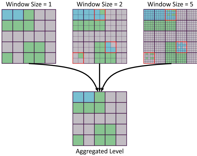
Fig. 4. Top row illustrates three generated levels, with window sizes of 1 \times 1 , 2 \times 2 , and 5 \times 5 , respectively. The bottom row shows the aggregated level, i.e., the level that each of the above ones reduces to. The red squares indicate logical tiles that were collapsed to the default tile of grass due to not being fully populated with the same tile. Here, blue tiles are houses, green tiles are gardens, and gray corresponds to roads.
