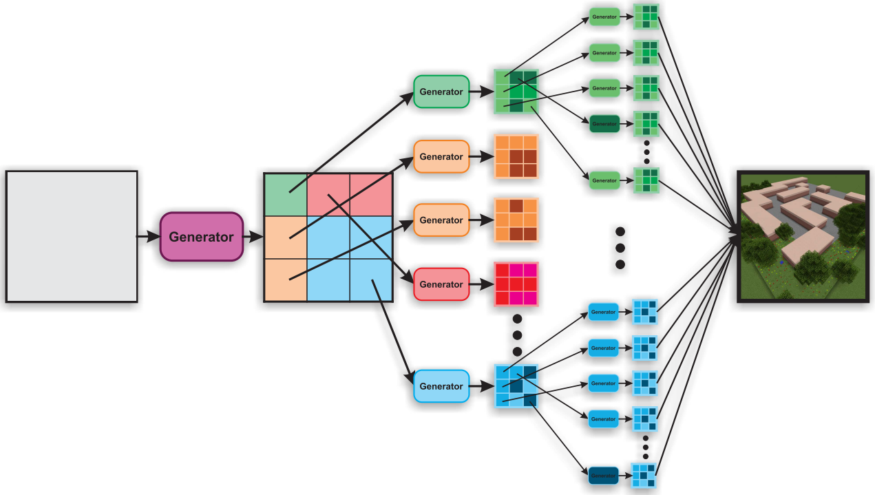
Fig. 2. High-level illustration of MCHAMR. We begin with a top-level generator, which generates an abstract tilemap. Each tile in this map is an instruction to use a lower-level generator and to place its output at that location. Each of these generators can be further composed of other generators. In the end, we obtain a fully-fledged level.
