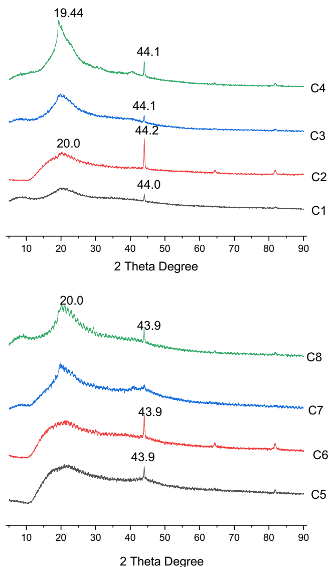
FIGURE 3 | XRD thermographs of C1–C4 and C5–C8. [Color figure can be viewed at wileyonlinelibrary.com ]
