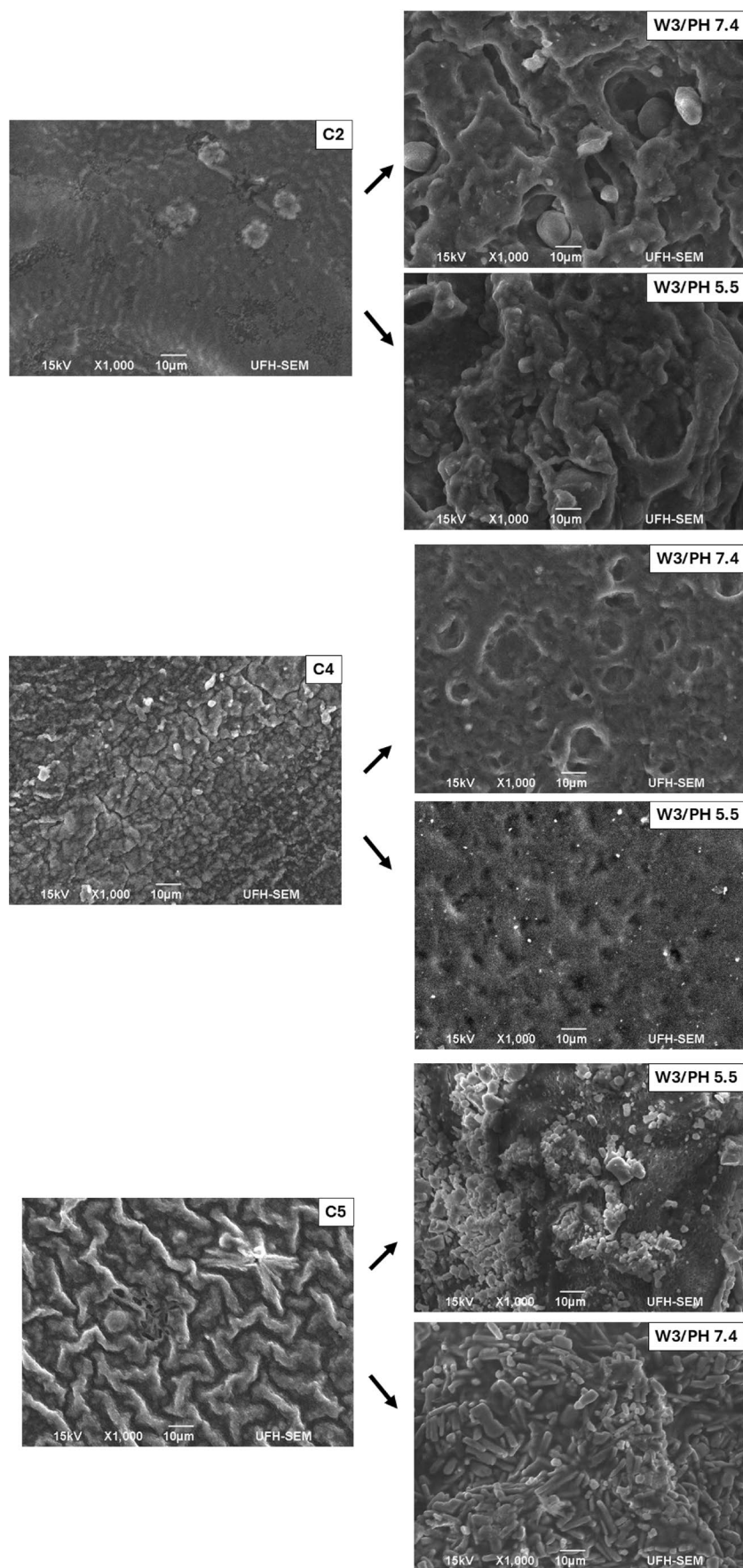
FIGURE 4 | SEM images for cryogels (C2, C4, and C5) before and after 3 weeks of biodegradation at pH 5.5 and 7.4.
