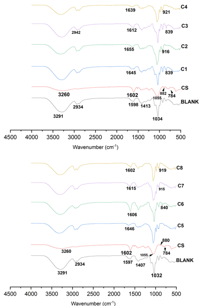
FIGURE 1 | FTIR spectra of plant extract, blank, and synthesized cryogel wound dressings, blank, C1–C4 and CS, C5–C8. [Color figure can be viewed at wileyonlinelibrary.com ]
