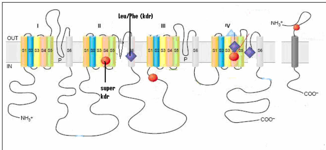
Figure 1.1: Diagrammatic representation of domain I-IV of the sodium channel showing the kdr and super kdr mutations on the domain II that have been implicated in conferring pyrethroid resistance in insect species (modified from Hemingway and Ranson, 2000).
