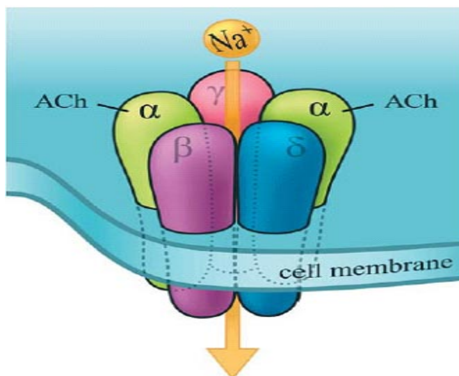
Figure 1.2: Schematic illustration of an Acetylcholine receptor with its binding sites
