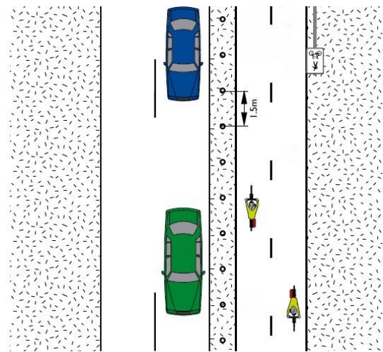
Figure 4 Example of the use of bollards to prevent illegal parking (New South Wales Roads and Traffic Authority, 2005).
